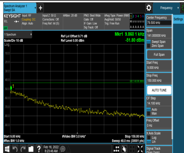
Band66-1.4MHz-16QAM-132665-1-0-High-0.009-0.15--51.8-PASS
