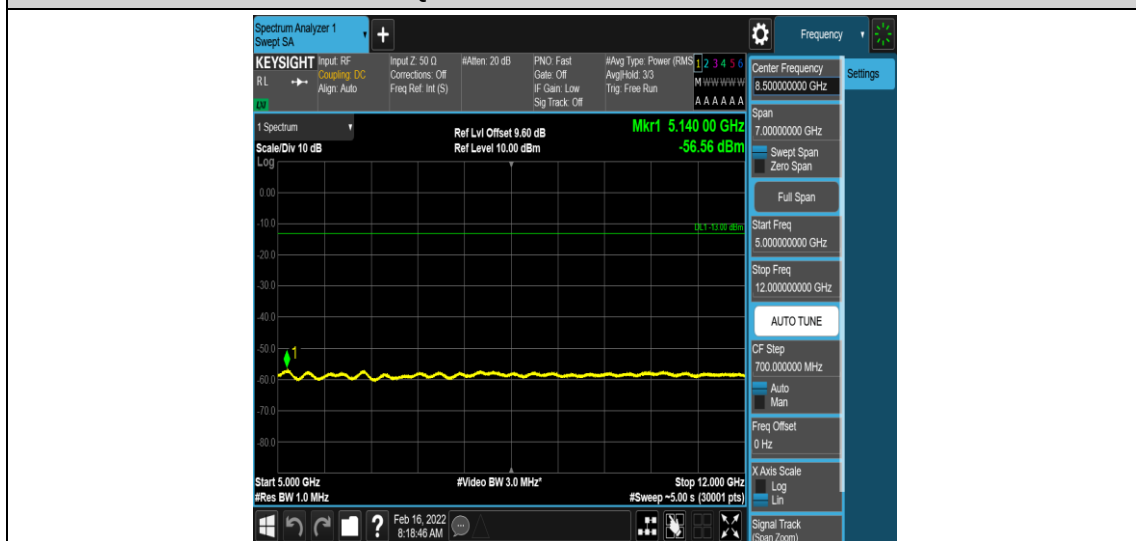
Band66-1.4MHz-16QAM-131979-1-0-Low-5000-12000--56.56-PASS
