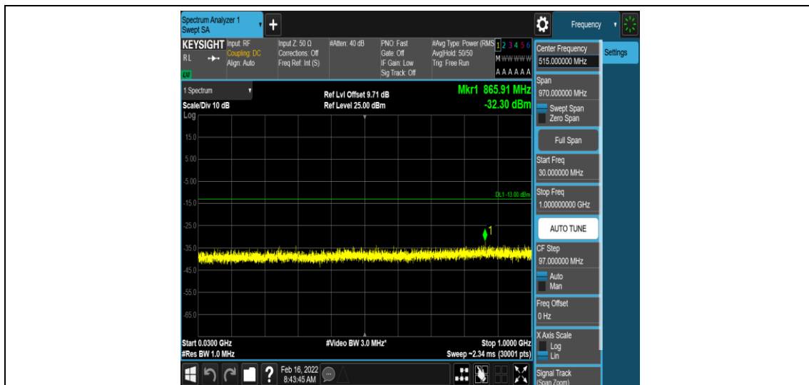
Band66-3MHz-16QAM-132657-1-0-High-30-1000--32.3-PASS
