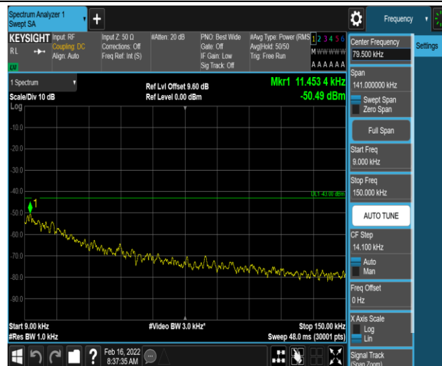
Band66-3MHz-16QAM-131987-1-0-Low-0.009-0.15--50.49-PASS
