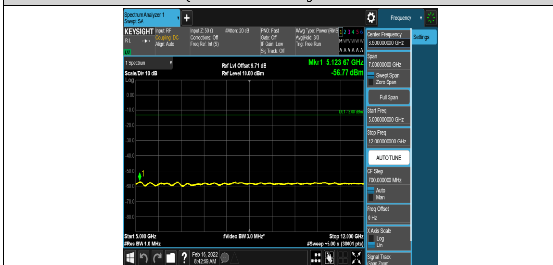
Band66-3MHz-QPSK-132657-1-0-High-5000-12000--56.77-PASS
