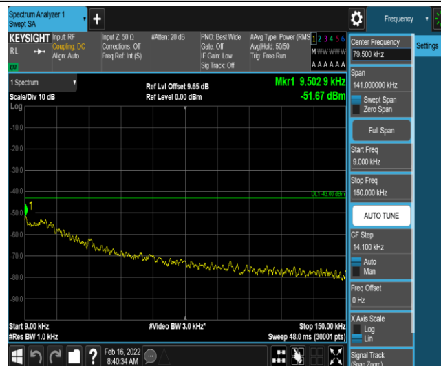
Band66-3MHz-16QAM-132322-1-0-Low-0.009-0.15--51.67-PASS
