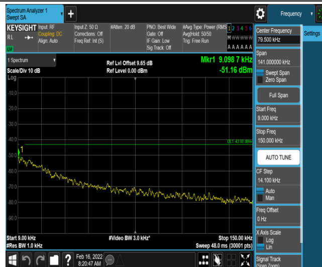
Band66-1.4MHz-16QAM-132322-1-0-Low-0.009-0.15--51.16-PASS
