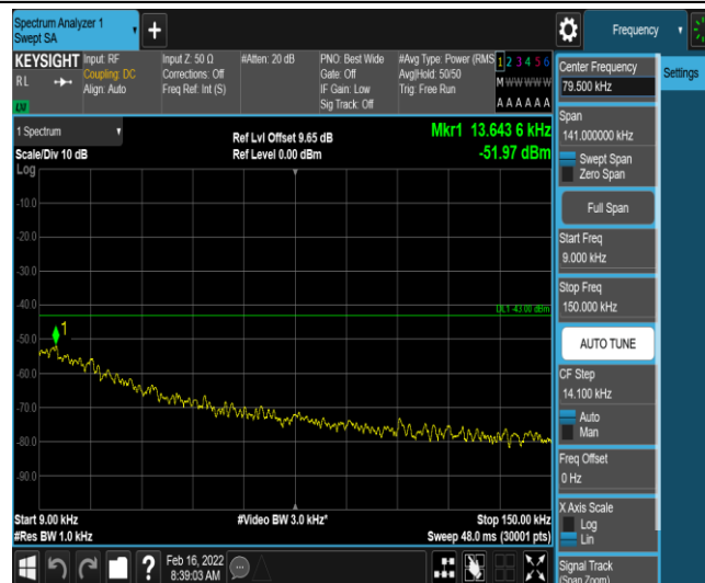
Band66-3MHz-QPSK-132322-1-0-Low-0.009-0.15--51.97-PASS
