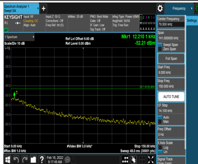
Band66-1.4MHz-16QAM-131979-1-0-Low-0.009-0.15--52.21-PASS
