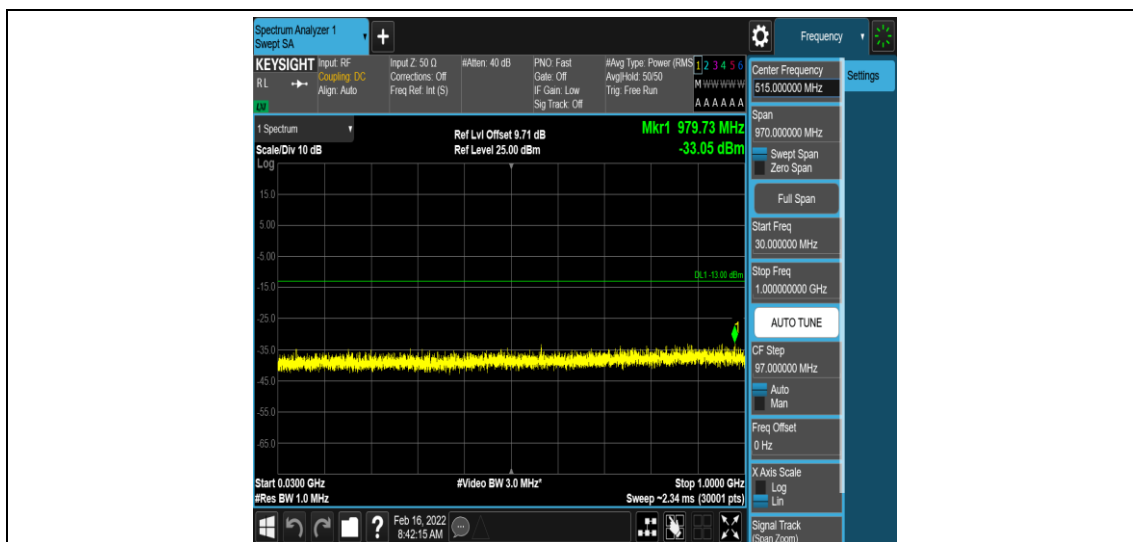
Band66-3MHz-QPSK-132657-1-0-High-30-1000--33.05-PASS
