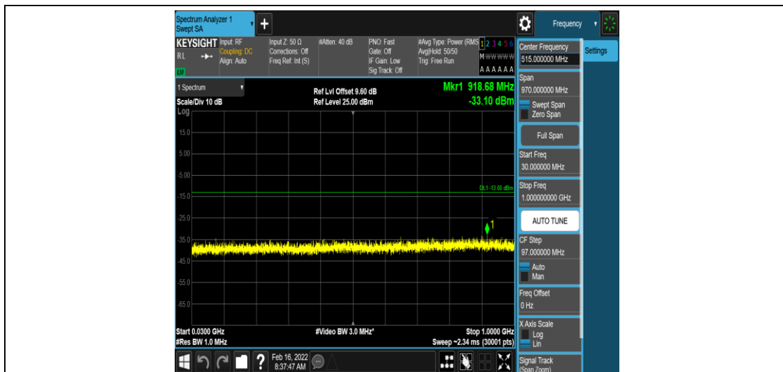
Band66-3MHz-16QAM-131987-1-0-Low-30-1000--33.1-PASS
