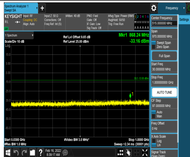
Band66-3MHz-QPSK-132322-1-0-Low-30-1000--33.16-PASS
