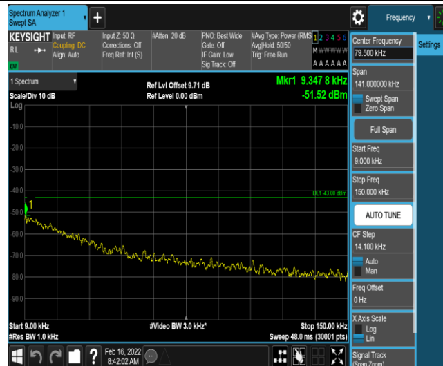
Band66-3MHz-QPSK-132657-1-0-High-0.009-0.15--51.52-PASS
