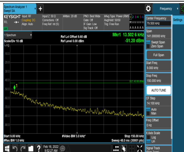
Band66-5MHz-QPSK-131997-1-0-Low-0.009-0.15--51.2-PASS
