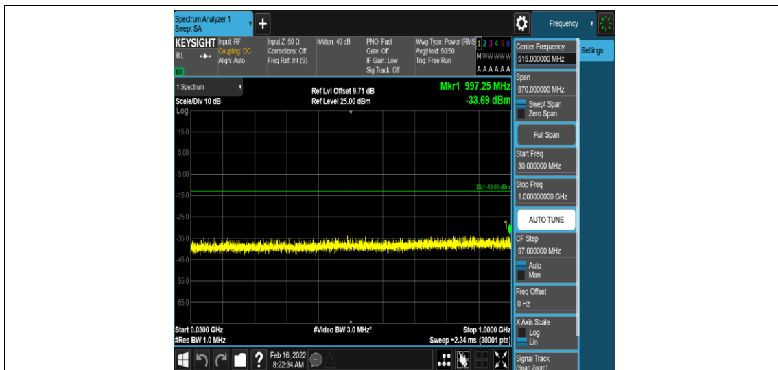
Band66-1.4MHz-QPSK-132665-1-0-High-30-1000--33.69-PASS
