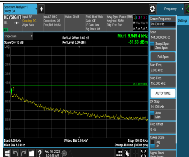
Band66-3MHz-QPSK-131987-1-0-Low-0.009-0.15--51.63-PASS
