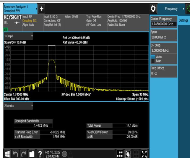
Band66-15MHz-QPSK-132322-6-0-Low-1.4472-1.793-PASS
