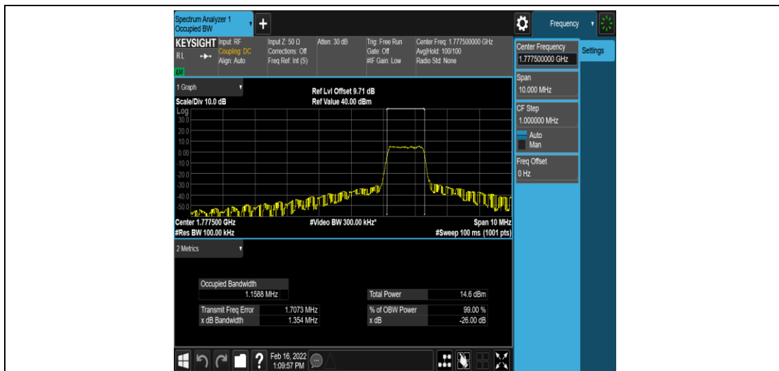
Band66-5MHz-QPSK-132647-6-0-High-1.1588-1.354-PASS
