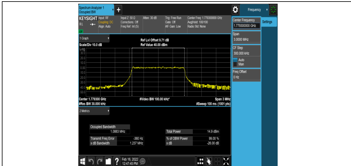
Band66-1.4MHz-16QAM-132665-6-0-High-1.0883-1.237-PASS
