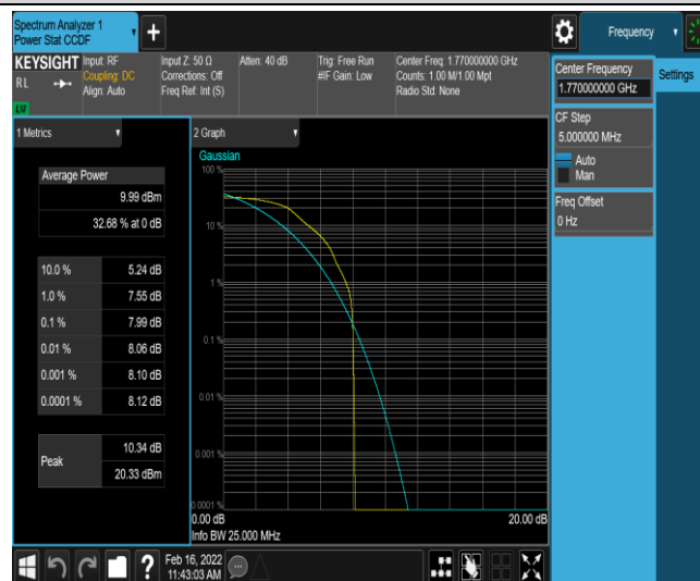
Band66-20MHz-QPSK-132572-1-0-High-7.99-&lt;=13-PASS
