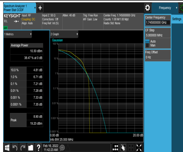
Band66-20MHz-QPSK-132322-1-0-Low-7.21-&lt;=13-PASS
