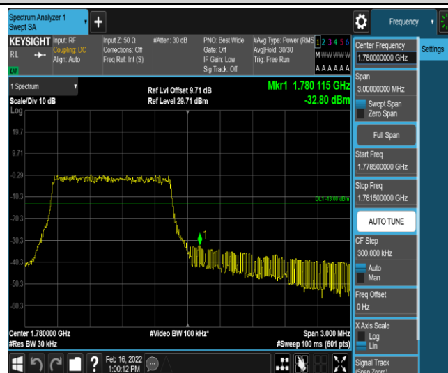
Band66-1.4MHz-16QAM-132665-6-0-High--32.80-PASS
