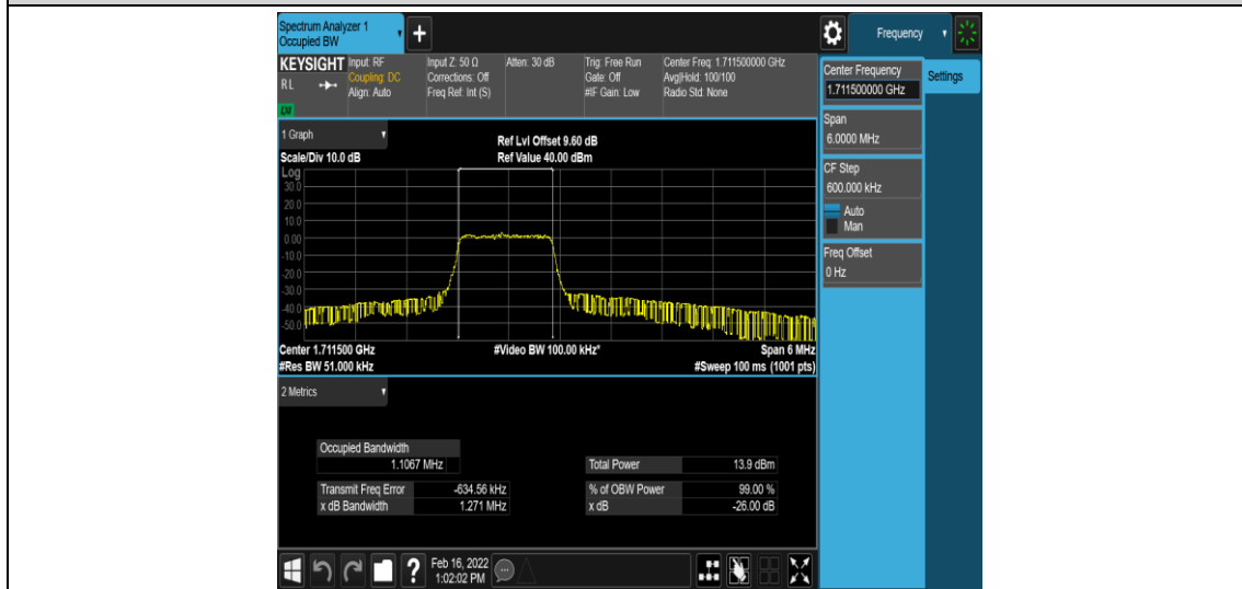
Band66-3MHz-QPSK-131987-6-0-Low-1.1067-1.271-PASS
