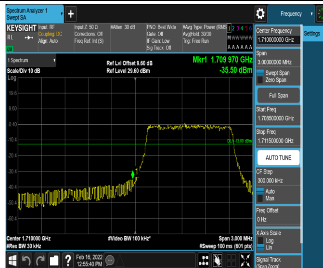
Band66-1.4MHz-16QAM-131979-6-0-Low--35.50-PASS
