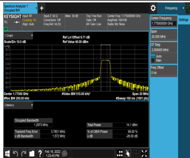
Band66-10MHz-16QAM-132622-6-0-High-1.2973-1.572-PASS
