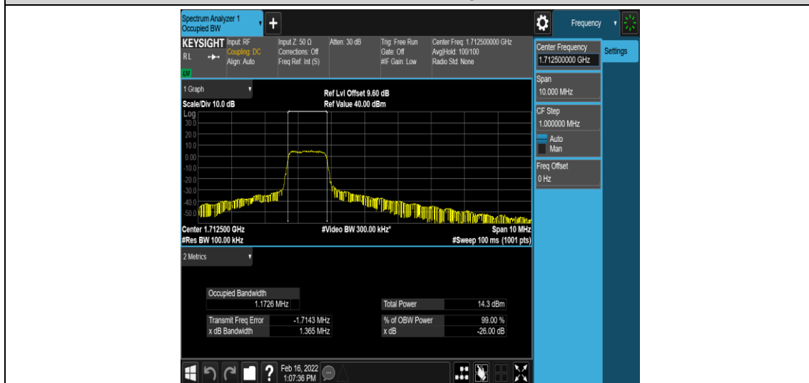
Band66-5MHz-16QAM-131997-6-0-Low-1.1726-1.365-PASS
