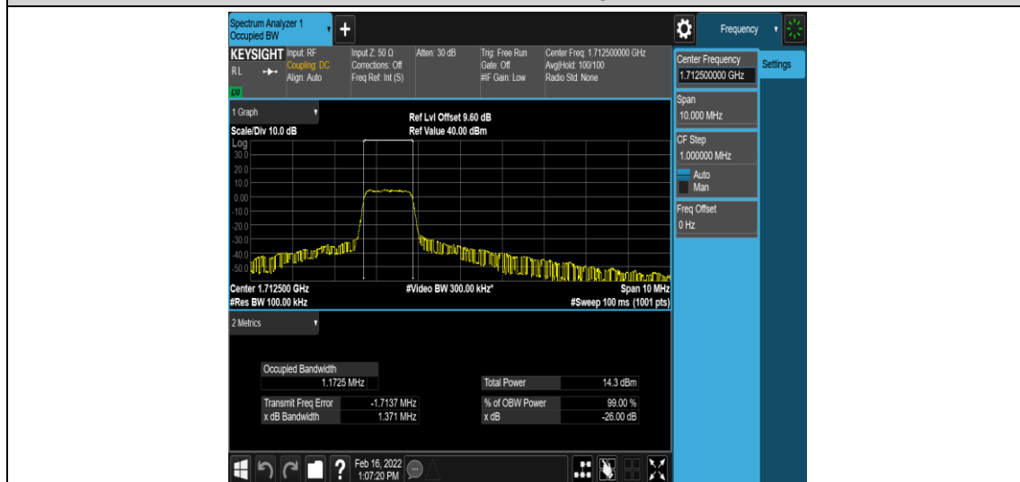
Band66-5MHz-QPSK-131997-6-0-Low-1.1725-1.371-PASS
