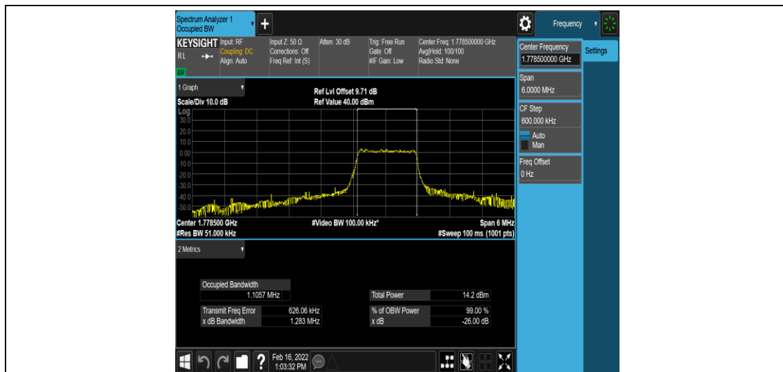
Band66-3MHz-16QAM-132657-6-0-High-1.1057-1.283-PASS
