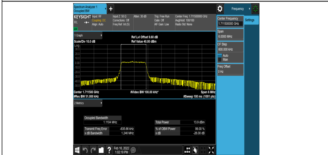
Band66-3MHz-16QAM-131987-6-0-Low-1.1104-1.246-PASS
