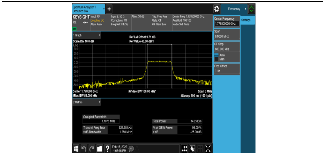
Band66-3MHz-QPSK-132657-6-0-High-1.1078-1.289-PASS
