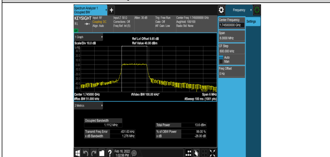
Band66-3MHz-16QAM-132322-6-0-Low-1.1112-1.276-PASS
