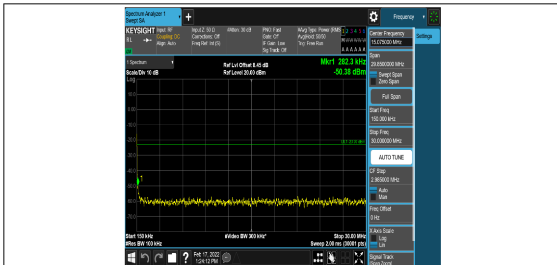
Band26-15MHz-QPSK-26915-1-0-Low-0.15-30--50.38-PASS
