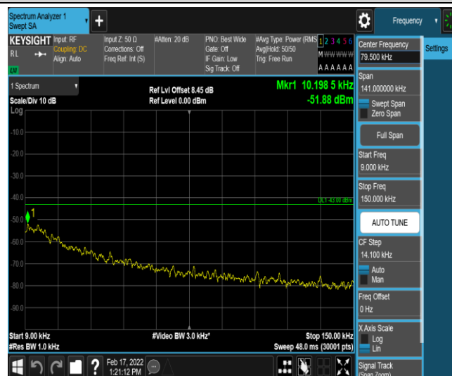
Band26-15MHz-QPSK-26865-1-0-Low-0.009-0.15--51.88-PASS
