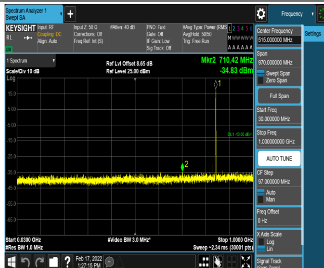
Band26-15MHz-QPSK-26965-1-0-High-30-1000--34.83-PASS
