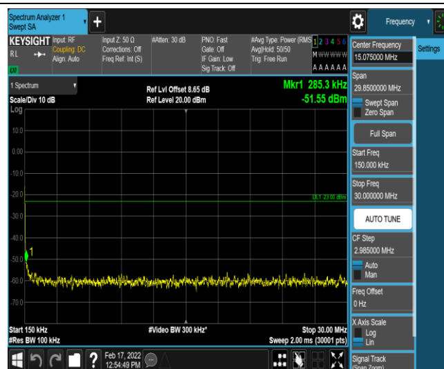
Band26-5MHz-16QAM-27015-1-0-High-0.15-30--51.55-PASS
