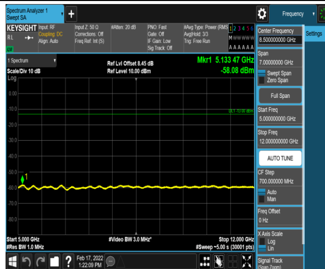
Band26-15MHz-QPSK-26865-1-0-Low-5000-12000--58.08-PASS
