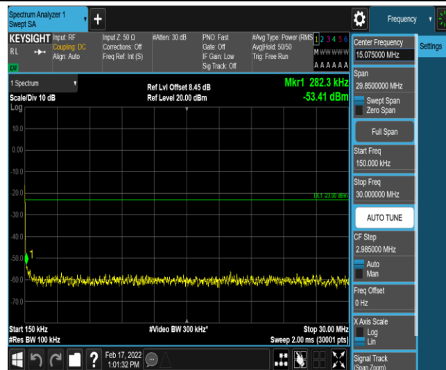
Band26-10MHz-QPSK-26840-1-0-Low-0.15-30--53.41-PASS
