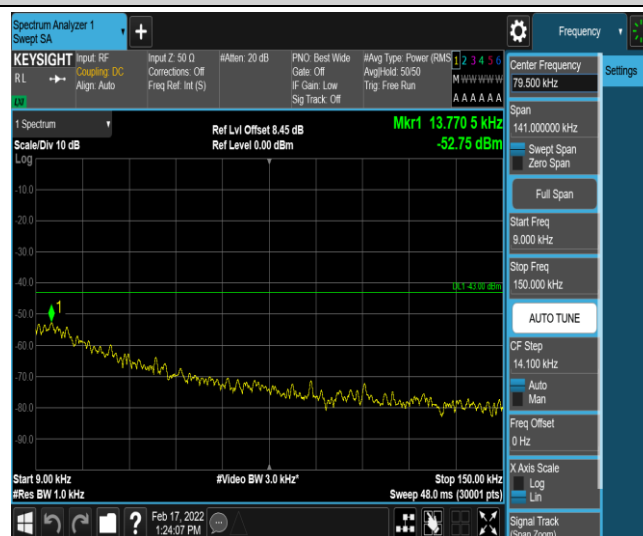
Band26-15MHz-QPSK-26915-1-0-Low-0.009-0.15--52.75-PASS
