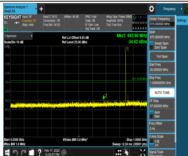
Band26-5MHz-16QAM-27015-1-0-High-30-1000--34.62-PASS
