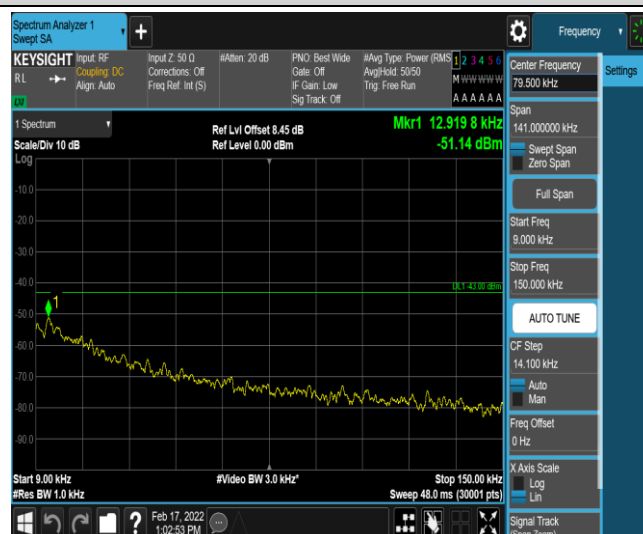
Band26-10MHz-16QAM-26840-1-0-Low-0.009-0.15--51.15-PASS
