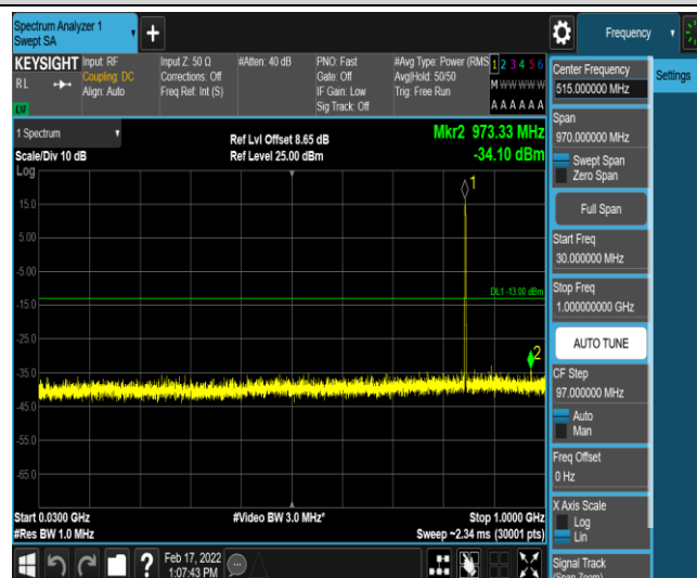
Band26-10MHz-QPSK-26990-1-0-High-30-1000--34.1-PASS
