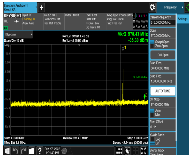
Band26-10MHz-QPSK-26840-1-0-Low-30-1000--35.3-PASS
