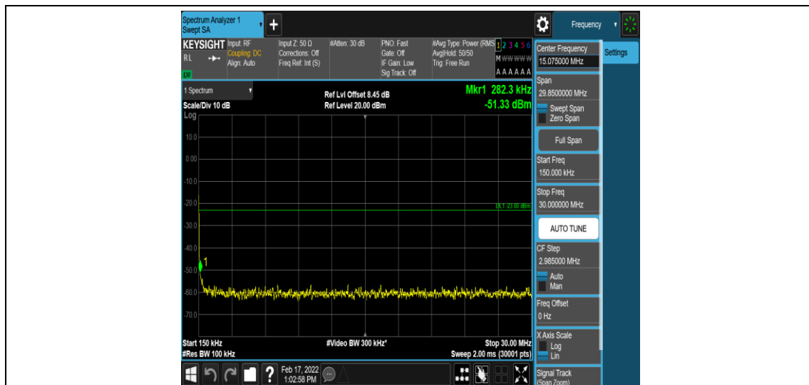
Band26-10MHz-16QAM-26840-1-0-Low-0.15-30--51.33-PASS
