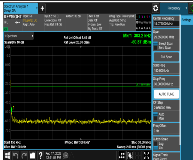
Band26-5MHz-16QAM-26915-1-0-Low-0.15-30--50.87-PASS
