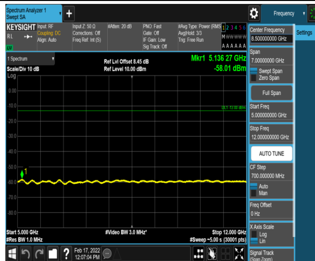
Band26-3MHz-16QAM-26915-1-0-Low-5000-12000--58.01-PASS
