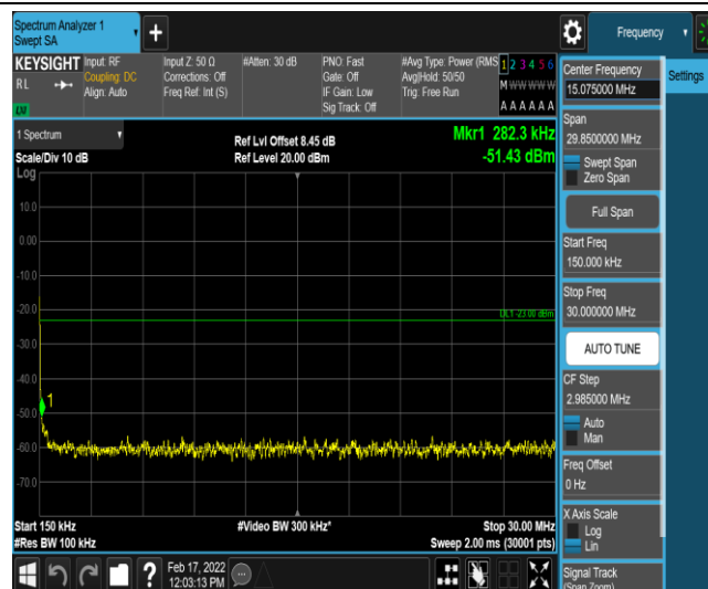
Band26-3MHz-16QAM-26805-1-0-Low-0.15-30--51.43-PASS
