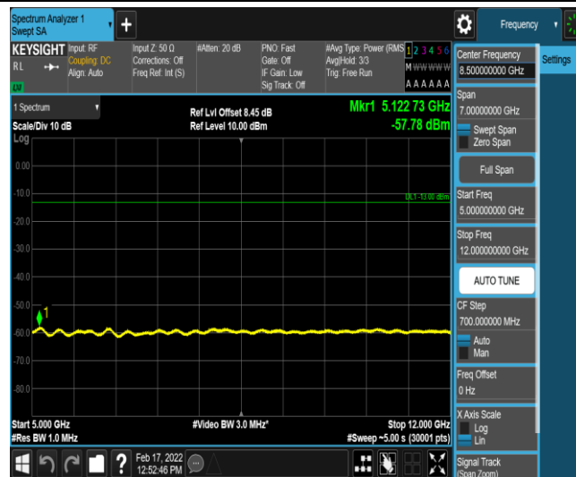
Band26-5MHz-16QAM-26915-1-0-Low-5000-12000--57.78-PASS
