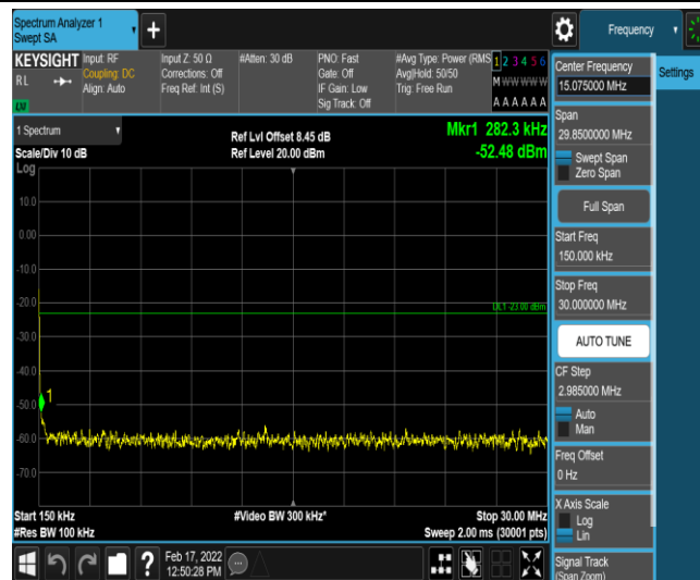
Band26-5MHz-QPSK-26915-1-0-Low-0.15-30--52.48-PASS
