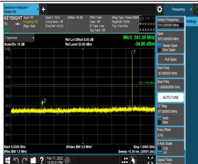
Band26-5MHz-QPSK-27015-1-0-High-30-1000--34.86-PASS
