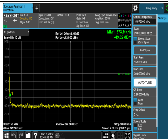
Band26-5MHz-16QAM-26815-1-0-Low-0.15-30--49.83-PASS
