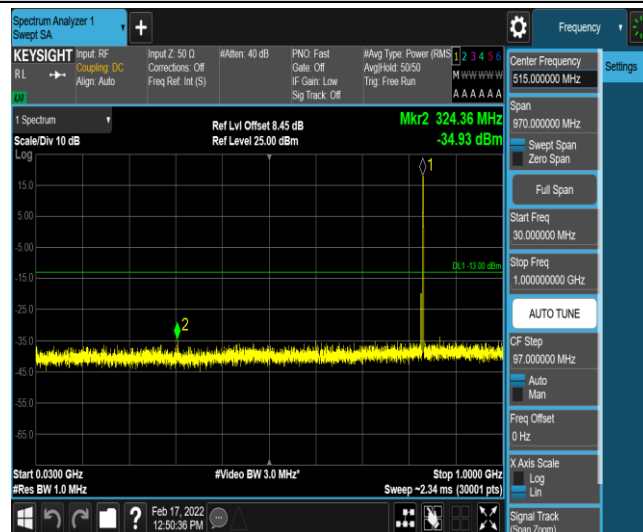
Band26-5MHz-QPSK-26915-1-0-Low-30-1000--34.93-PASS
