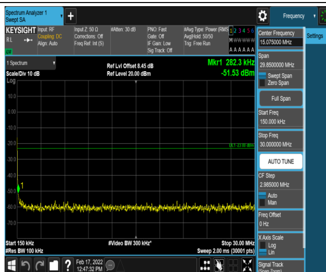
Band26-5MHz-QPSK-26815-1-0-Low-0.15-30--51.53-PASS
