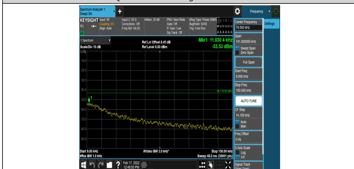
Band26-5MHz-16QAM-26815-1-0-Low-0.009-0.15--53.53-PASS
