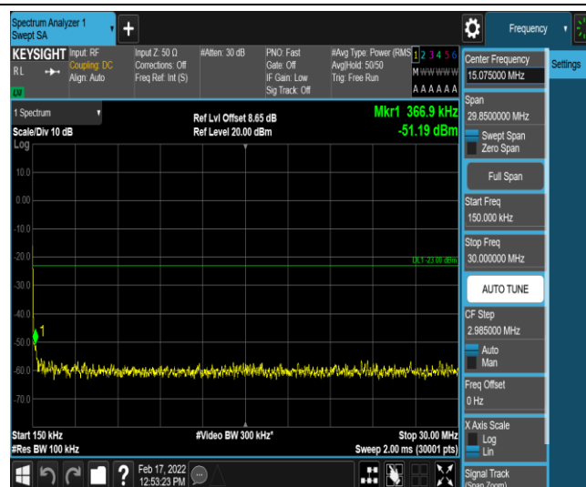
Band26-5MHz-QPSK-27015-1-0-High-0.15-30--51.19-PASS
