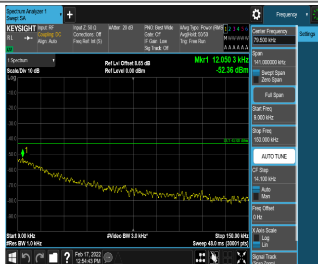
Band26-5MHz-16QAM-27015-1-0-High-0.009-0.15--52.36-PASS
