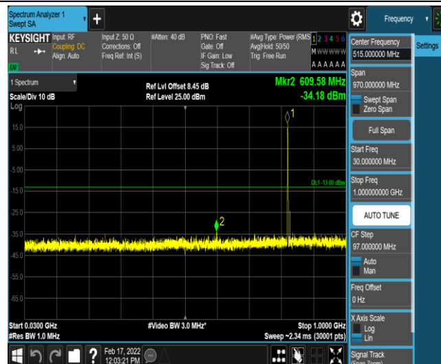
Band26-3MHz-16QAM-26805-1-0-Low-30-1000--34.18-PASS
