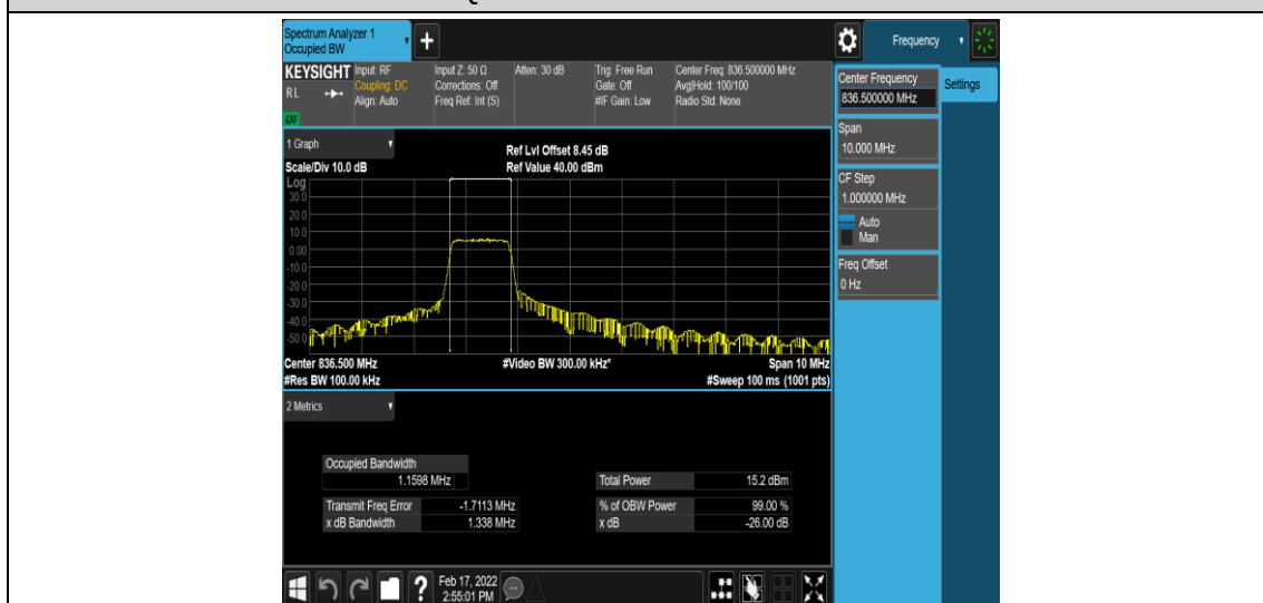
Band26-5MHz-QPSK-26915-6-0-Low-1.1598-1.338-PASS
