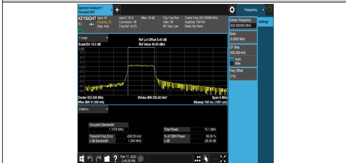
Band26-3MHz-16QAM-26805-6-0-Low-1.1078-1.284-PASS
