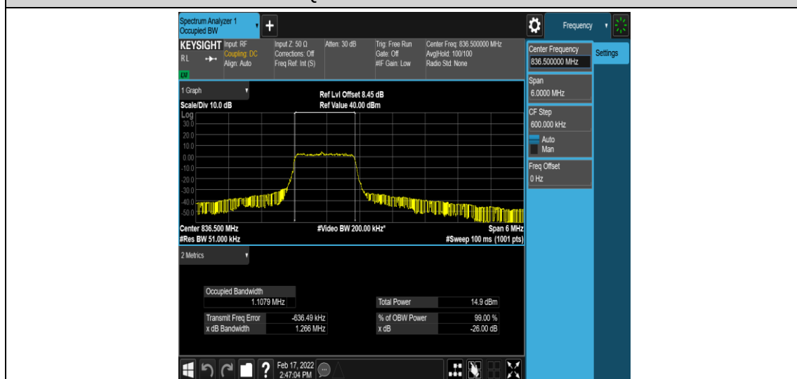
Band26-3MHz-16QAM-26915-6-0-Low-1.1079-1.266-PASS
