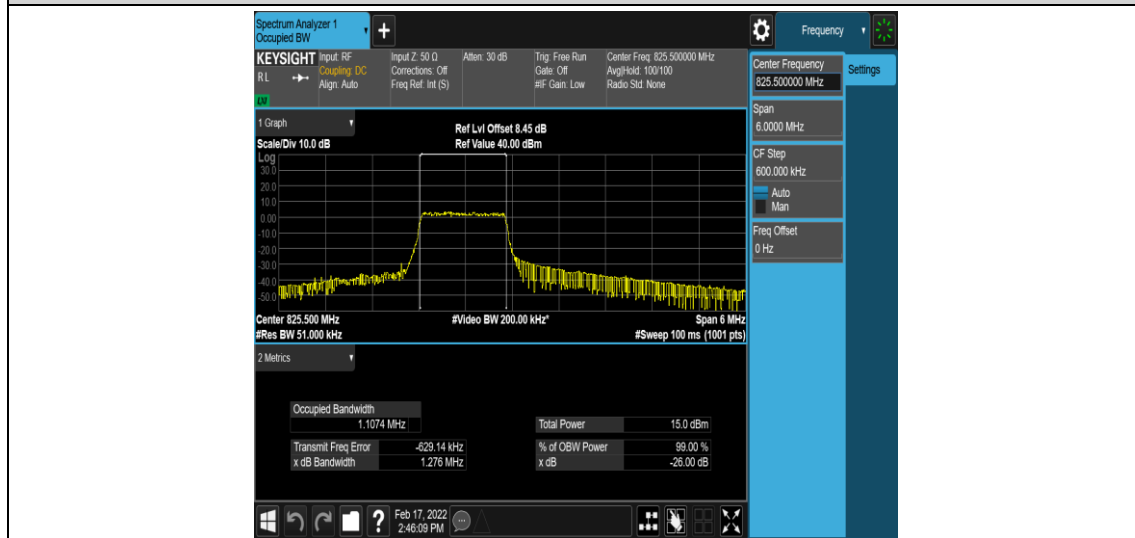
Band26-3MHz-QPSK-26805-6-0-Low-1.1074-1.276-PASS
