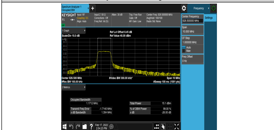
Band26-5MHz-QPSK-26815-6-0-Low-1.1712-1.354-PASS
