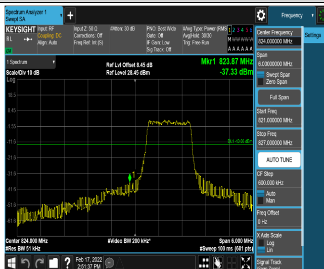
Band26-3MHz-QPSK-26805-6-0-Low--37.33-PASS
