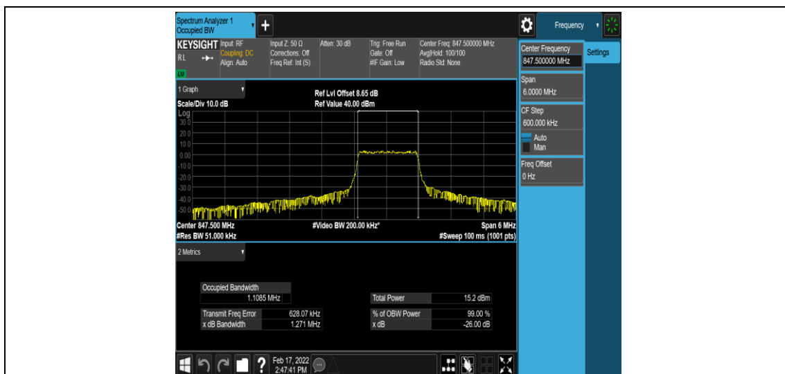
Band26-3MHz-16QAM-27025-6-0-High-1.1085-1.271-PASS
