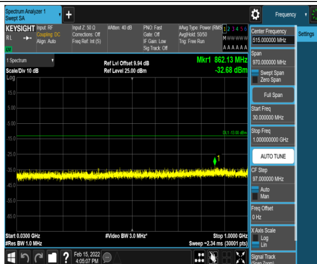
Band25-5MHz-16QAM-26665-1-0-High-30-1000--32.69-PASS
