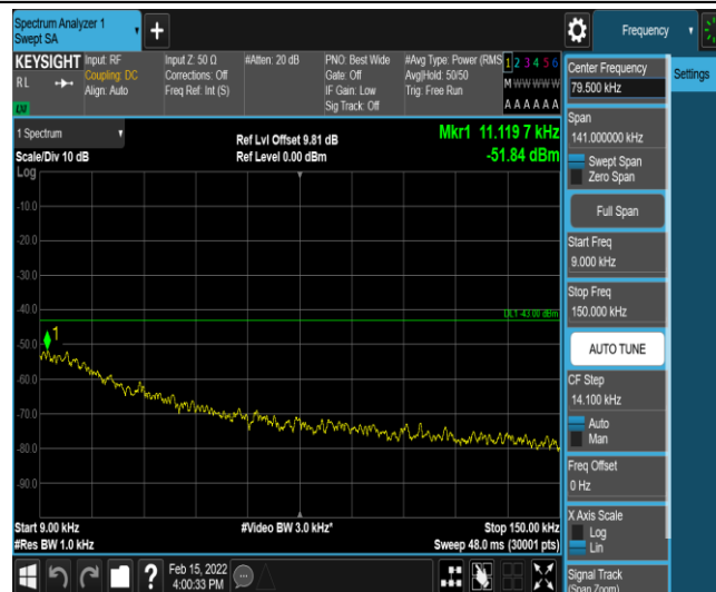
Band25-5MHz-QPSK-26365-1-0-Low-0.009-0.15--51.84-PASS
