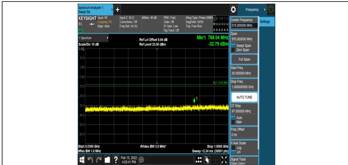
Band25-5MHz-QPSK-26665-1-0-High-30-1000--32.79-PASS
