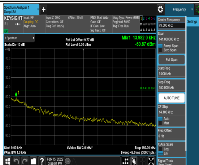
Band25-5MHz-16QAM-26065-1-0-Low-0.009-0.15--50.88-PASS
