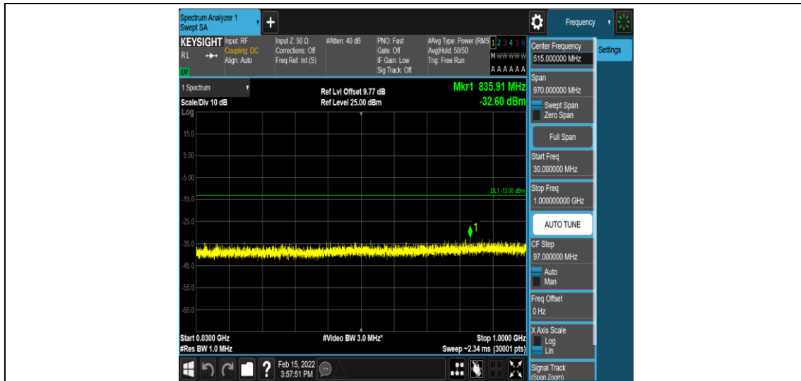
Band25-5MHz-QPSK-26065-1-0-Low-30-1000--32.6-PASS
