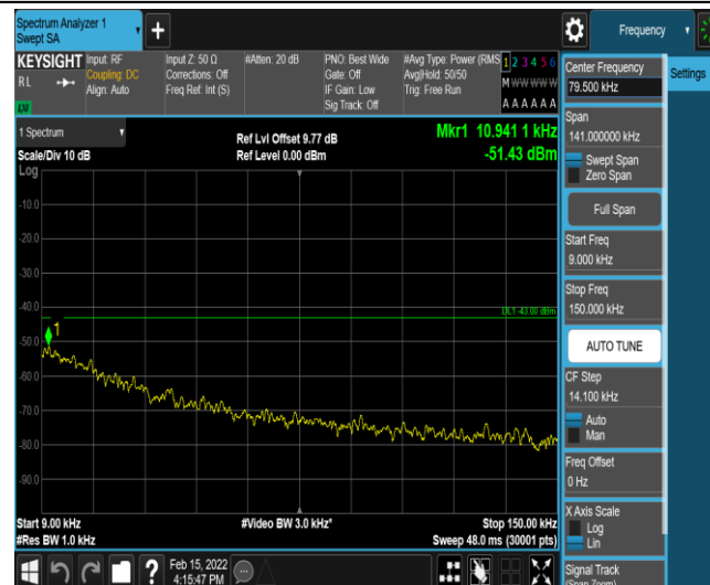
Band25-10MHz-16QAM-26090-1-0-Low-0.009-0.15--51.43-PASS
