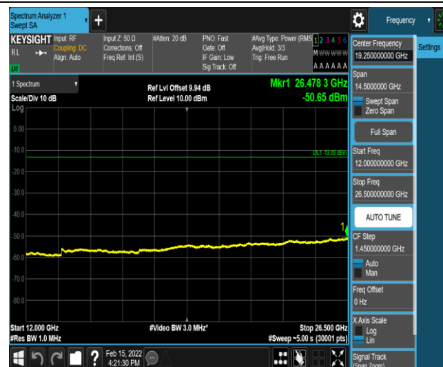
Band25-10MHz-QPSK-26640-1-0-High-12000-26500--50.65-PASS
