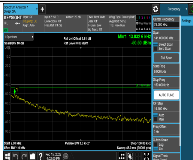
Band25-5MHz-16QAM-26365-1-0-Low-0.009-0.15--50.5-PASS
