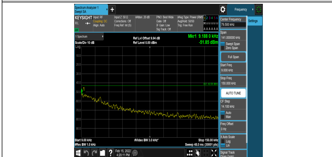
Band25-10MHz-QPSK-26640-1-0-High-0.009-0.15--51.85-PASS
