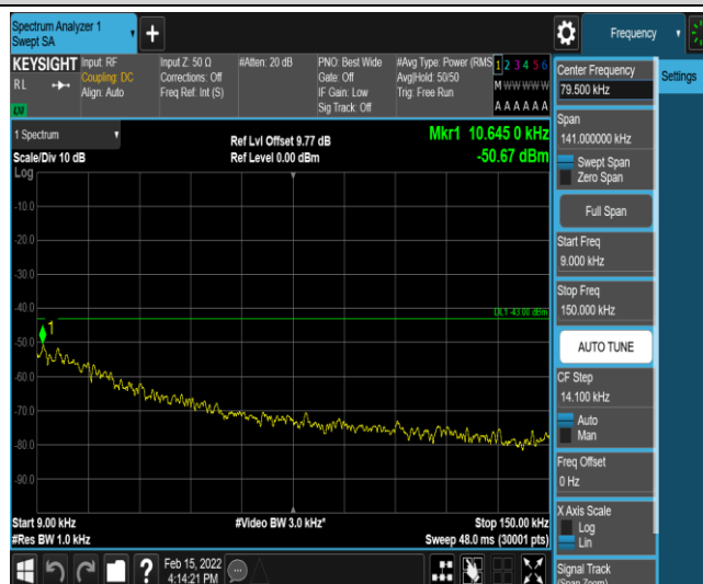
Band25-10MHz-QPSK-26090-1-0-Low-0.009-0.15--50.67-PASS
