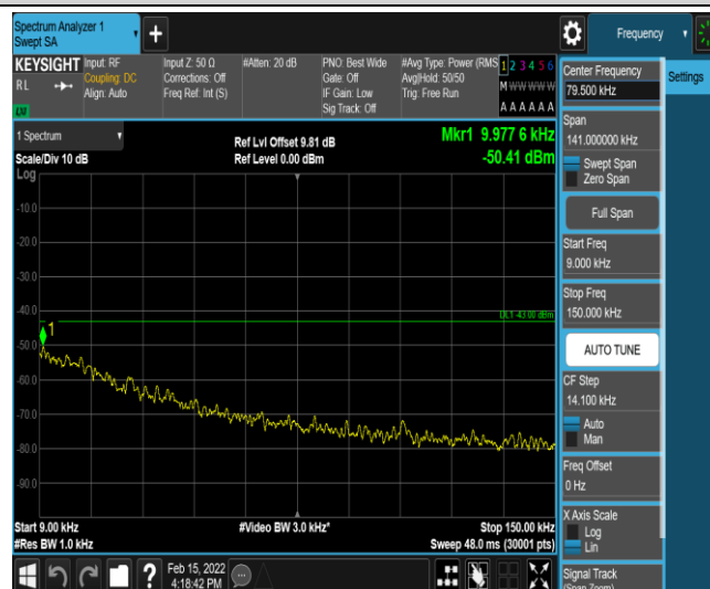
Band25-10MHz-16QAM-26365-1-0-Low-0.009-0.15--50.41-PASS
