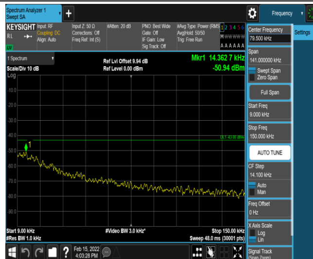
Band25-5MHz-QPSK-26665-1-0-High-0.009-0.15--50.94-PASS
