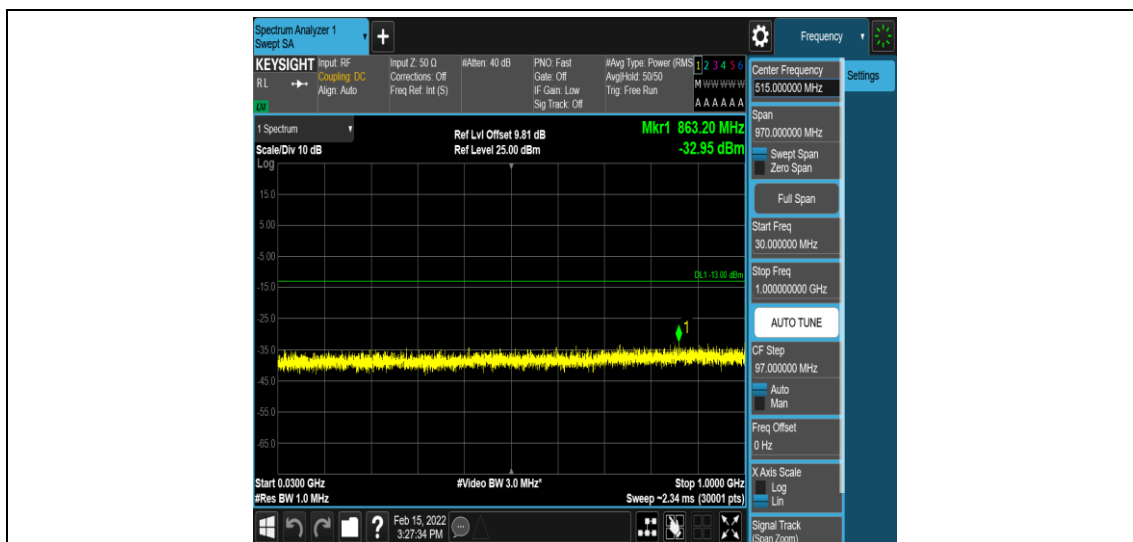
Band25-1.4MHz-QPSK-26365-1-0-Low-30-1000--32.95-PASS
