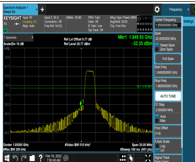
Band25-10MHz-16QAM-26090-6-0-Low--32.35-PASS
