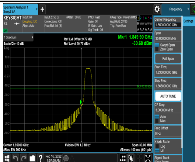
Band25-15MHz-QPSK-26115-6-0-Low--30.68-PASS
