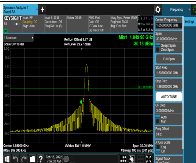
Band25-15MHz-QPSK-26115-1-0-Low--30.13-PASS
