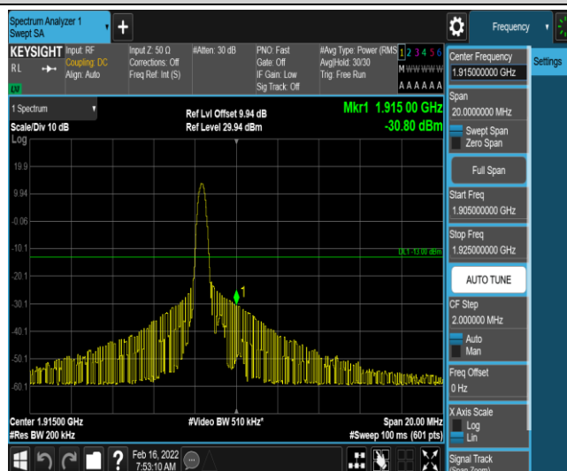
Band25-10MHz-16QAM-26640-1-0-High--30.80-PASS
