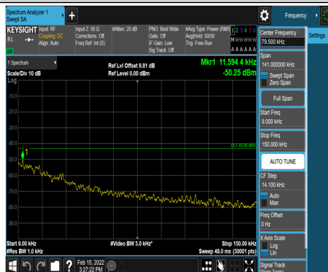
Band25-1.4MHz-QPSK-26365-1-0-Low-0.009-0.15--50.25-PASS
