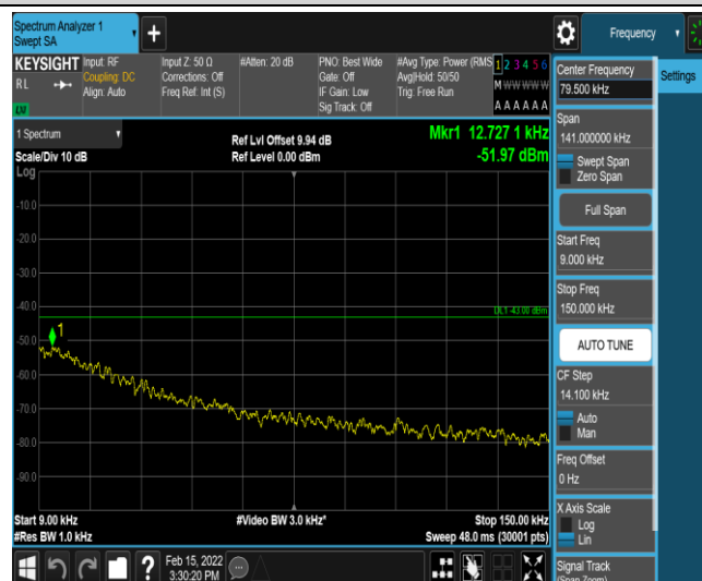
Band25-1.4MHz-QPSK-26683-1-0-High-0.009-0.15--51.97-PASS
