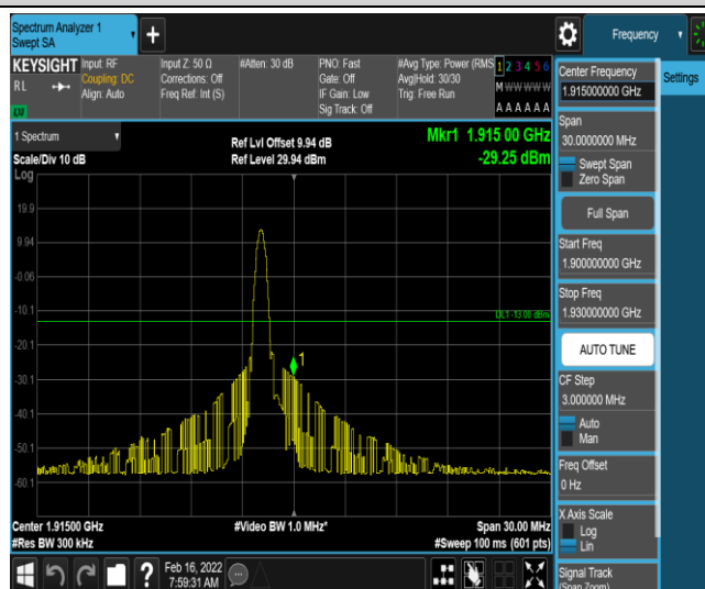
Band25-15MHz-QPSK-26615-1-0-High--29.25-PASS
