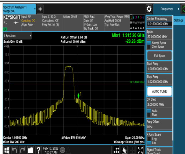
Band25-10MHz-16QAM-26640-6-0-High--29.26-PASS
