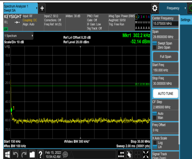
Band12-5MHz-16QAM-23095-1-0-Low-0.15-30--52.14-PASS
