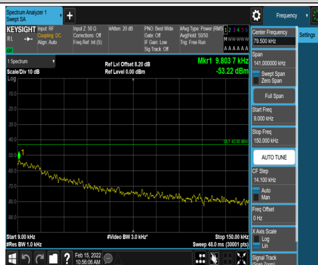
Band12-5MHz-QPSK-23155-1-0-High-0.009-0.15--53.22-PASS
