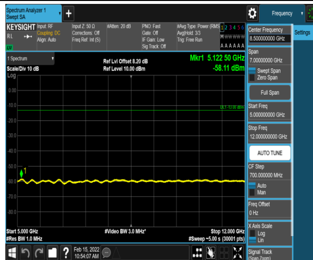
Band12-5MHz-QPSK-23095-1-0-Low-5000-12000--58.11-PASS
