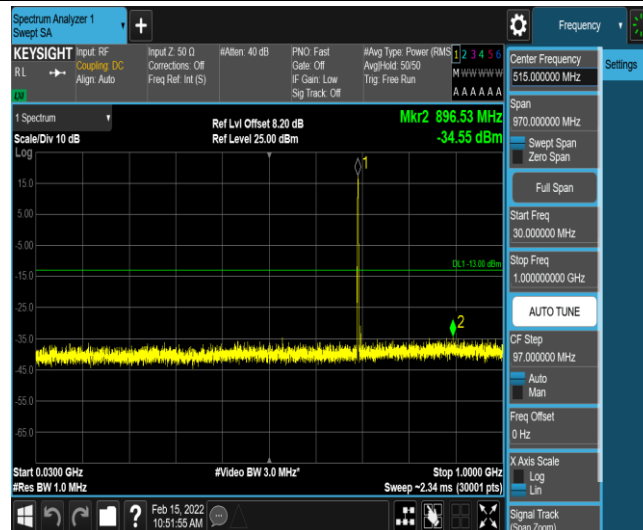
Band12-5MHz-16QAM-23035-1-0-Low-30-1000--34.55-PASS
