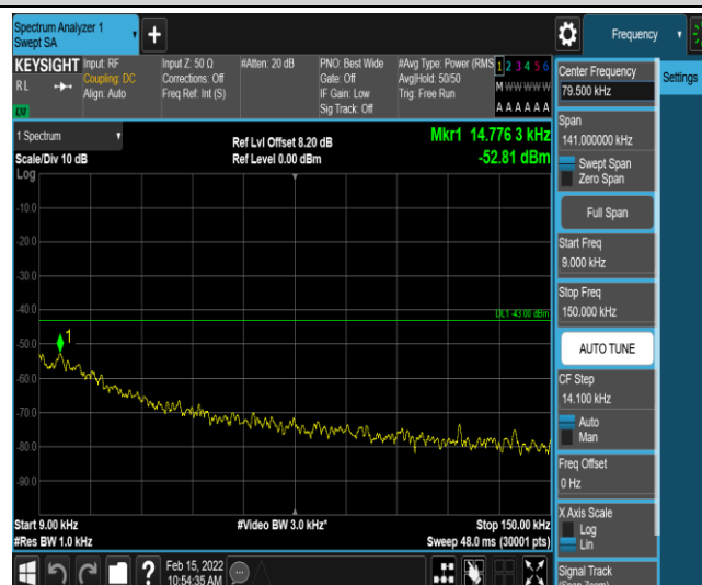
Band12-5MHz-16QAM-23095-1-0-Low-0.009-0.15--52.81-PASS
