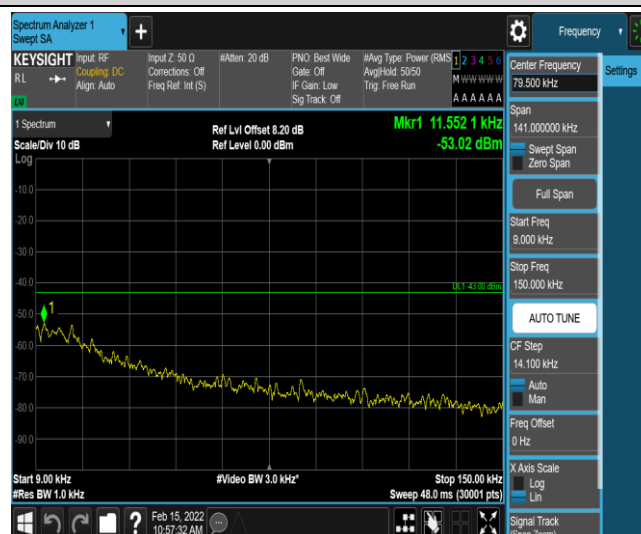
Band12-5MHz-16QAM-23155-1-0-High-0.009-0.15--53.02-PASS
