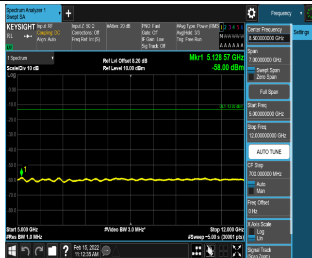
Band12-10MHz-QPSK-23130-1-0-High-5000-12000--58-PASS
