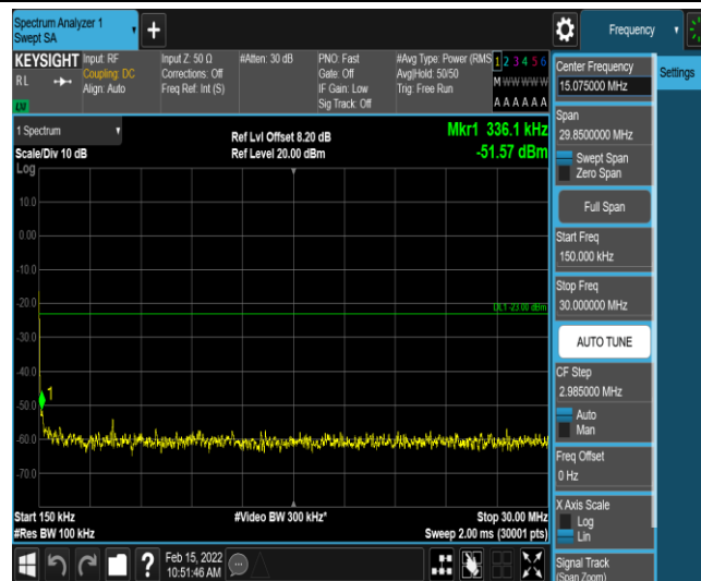
Band12-5MHz-16QAM-23035-1-0-Low-0.15-30--51.57-PASS
