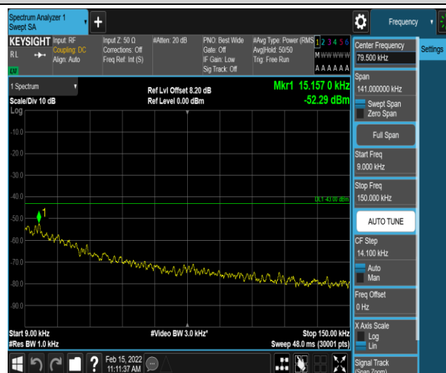
Band12-10MHz-QPSK-23130-1-0-High-0.009-0.15--52.3-PASS
