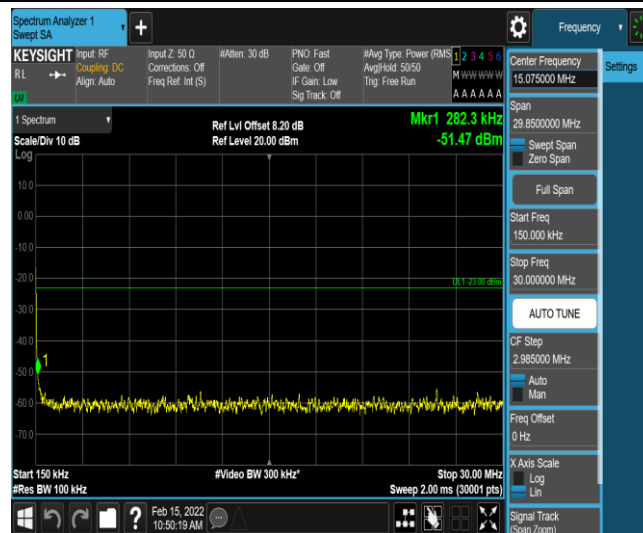
Band12-5MHz-QPSK-23035-1-0-Low-0.15-30--51.47-PASS
