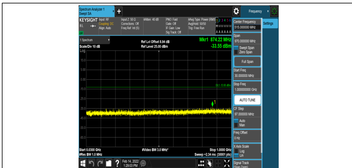
Band2-1.4MHz-16QAM-19193-1-5-Low-30-1000--33.55-PASS
