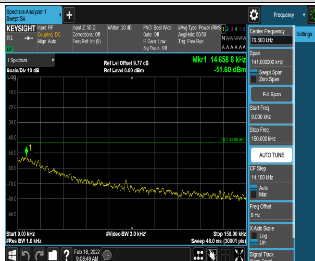
Band2-3MHz-16QAM-18615-1-0-Low-0.009-0.15--51.6-PASS
