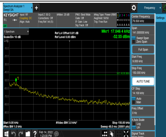
Band2-1.4MHz-16QAM-18900-1-0-Low-0.009-0.15--52.55-PASS
