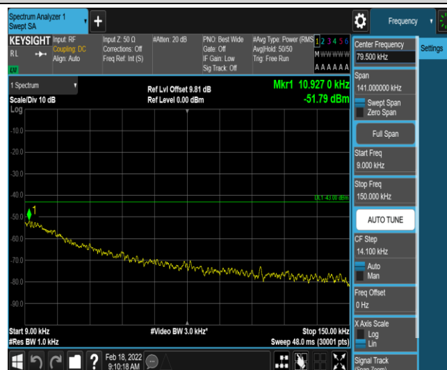
Band2-3MHz-QPSK-18900-1-0-Low-0.009-0.15--51.79-PASS
