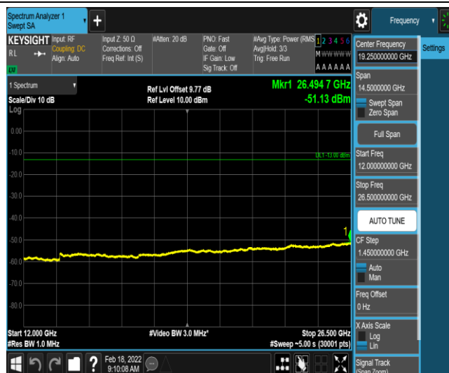
Band2-3MHz-16QAM-18615-1-0-Low-12000-26500--51.13-PASS
