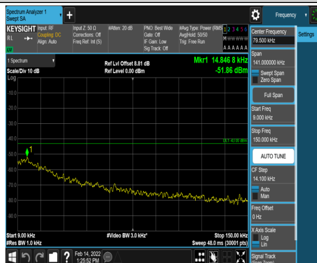
Band2-1.4MHz-16QAM-18900-6-0-Low-0.009-0.15--51.86-PASS
