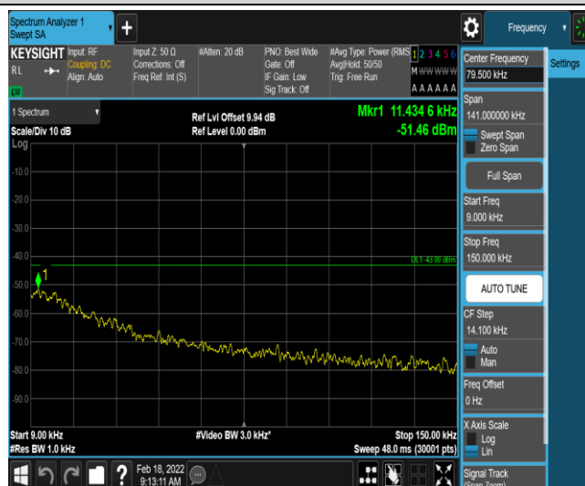
Band2-3MHz-QPSK-19185-1-0-High-0.009-0.15--51.46-PASS
