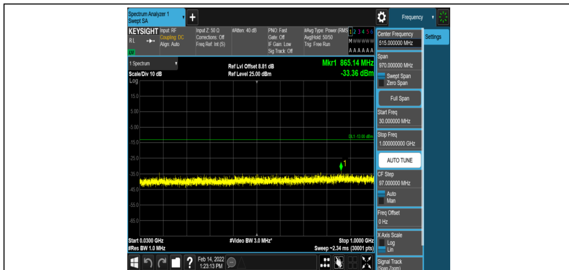
Band2-1.4MHz-16QAM-18900-1-0-Low-30-1000--33.36-PASS
