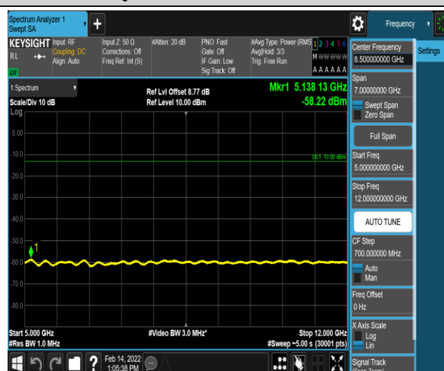
Band2-1.4MHz-16QAM-18607-1-0-Low-5000-12000--58.22-PASS
