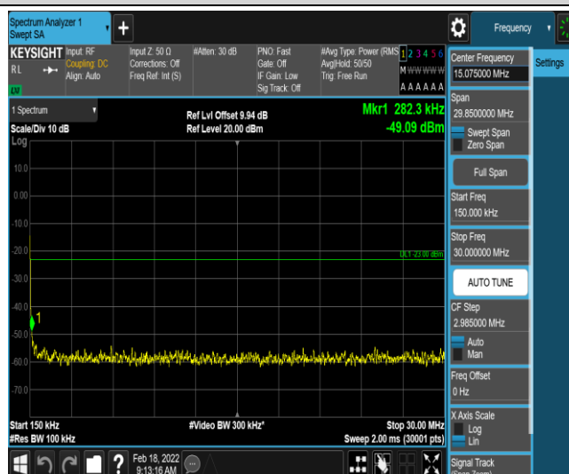
Band2-3MHz-QPSK-19185-1-0-High-0.15-30--49.09-PASS
