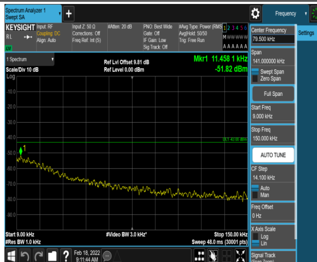
Band2-3MHz-16QAM-18900-1-0-Low-0.009-0.15--51.82-PASS
