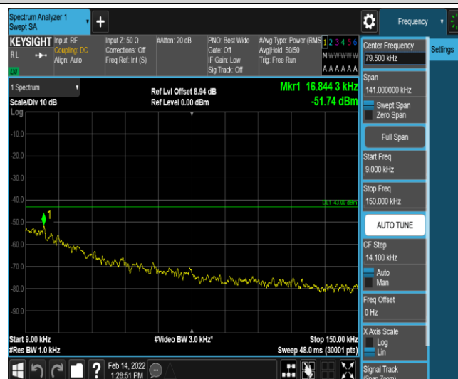
Band2-1.4MHz-16QAM-19193-1-5-Low-0.009-0.15--51.74-PASS
