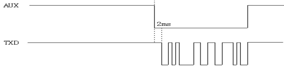
Timing Sequence in Standard Mode
