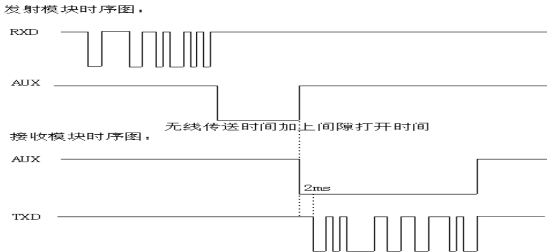
Timing Sequence in Sleep Mode
