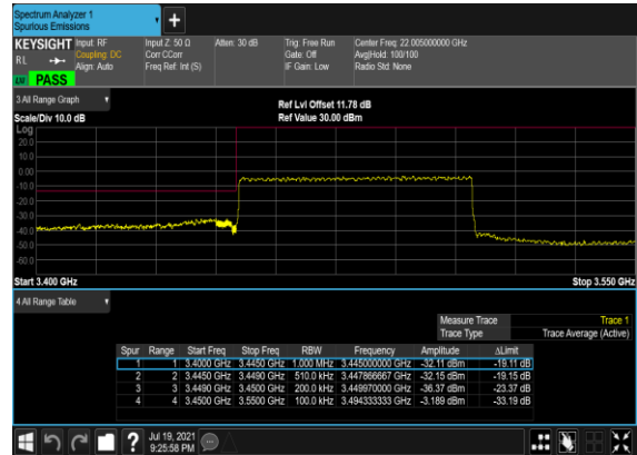
B2_N77(60M)_DFT-s-OFDM_QPSK_Outer_Full_Low_CH
