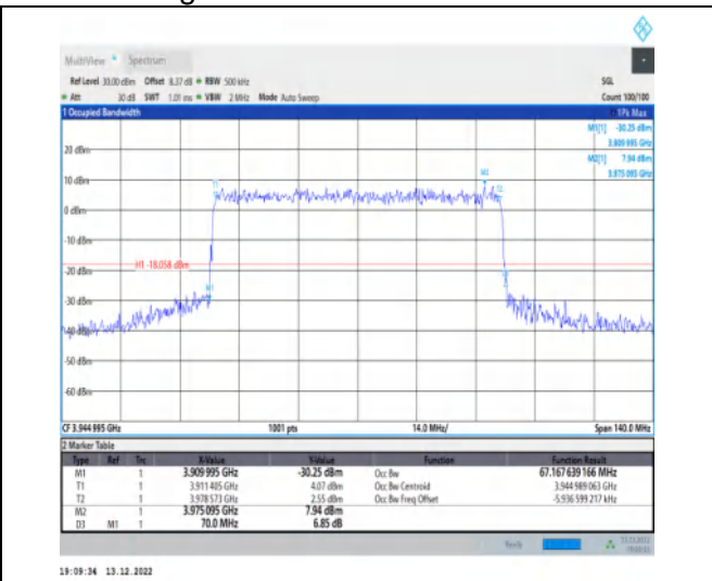
1-N77-3700-3980-30-70-H-7-CP-16QAM-Outer_Full-189@0-Ant1-67.168-70.000-≤70-PASS
