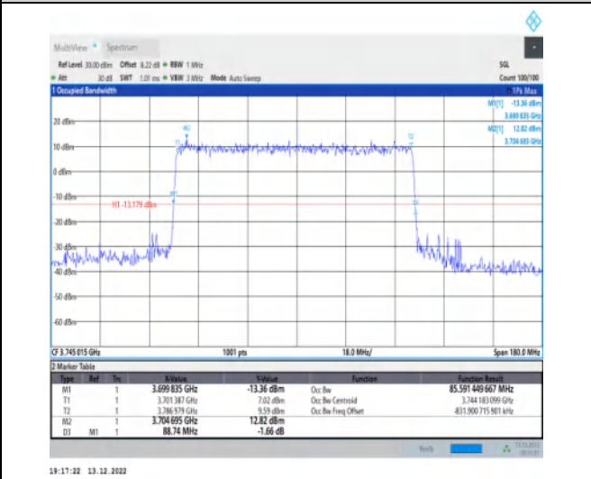
1-N77-3700-3980-30-90-L-1-DFT-QPSK-Outer_Full-240@0-Ant1-85.591-88.740-≤90-PASS
