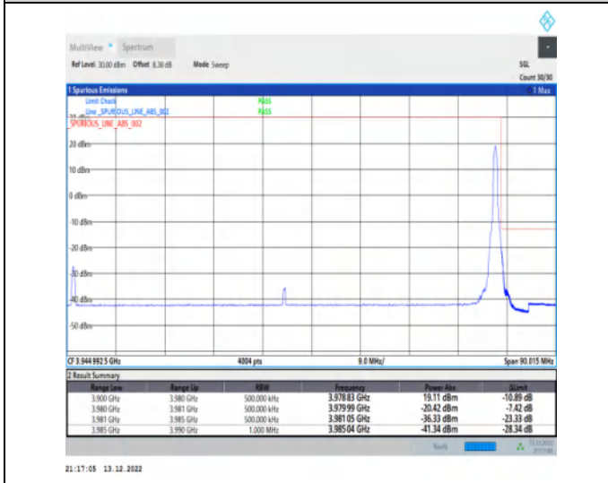
1-N77-3700-3980-30-80-H-5-CP-QPSK-Edge_1RB_Right-1@216-Ant1-1--PASS-see graph
