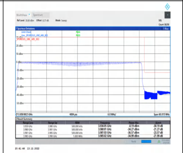
1-N77-3700-3980-30-50-H-6-CP-QPSK-Outer_Full-133@0-Ant1-1--PASS-see graph
