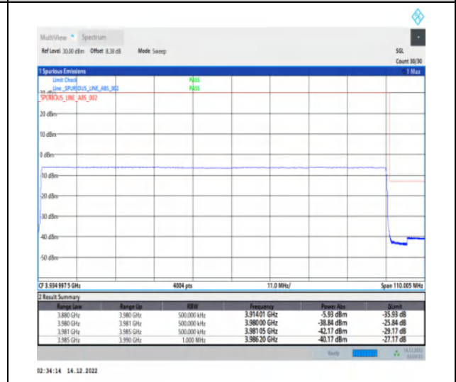
1-N77-3700-3980-30-100-H-6-CP-QPSK-Outer_F ull-273@0-Ant1-1--PASS-see graph
