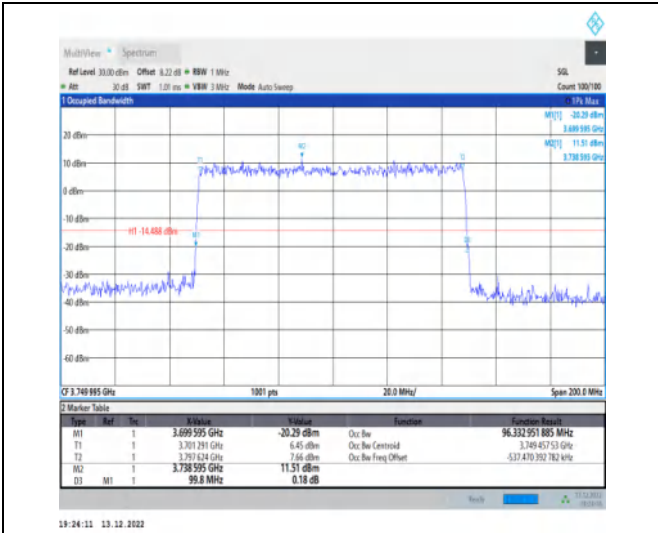
1-N77-3700-3980-30-100-L-3-DFT-16QAM-Outer_Fu II-270@0-Ant1-96.333-99.800-≤100-PASS
