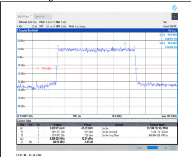
1-N77-3700-3980-30-90-H-1-DFT-QPSK-Outer_Full-240@0-Ant1-85.595-88.920-≤90-PASS
