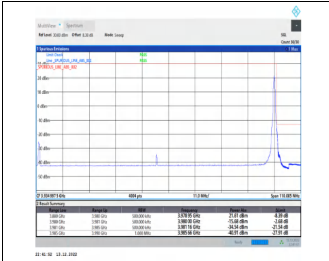
1-N77-3700-3980-30-100-H-2-DFT-PI2BPSK-Edge_1R_B_Right-1@272-Ant1-1--PASS-see graph
