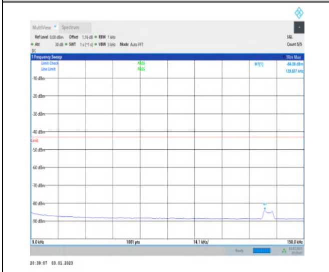
1-N77-3700-3980-30-100-H-1-DFT-QPSK-Edge_1R B_Left-1@0-0.009-0.15-Ant1-0.13--84.08--43-PASS
