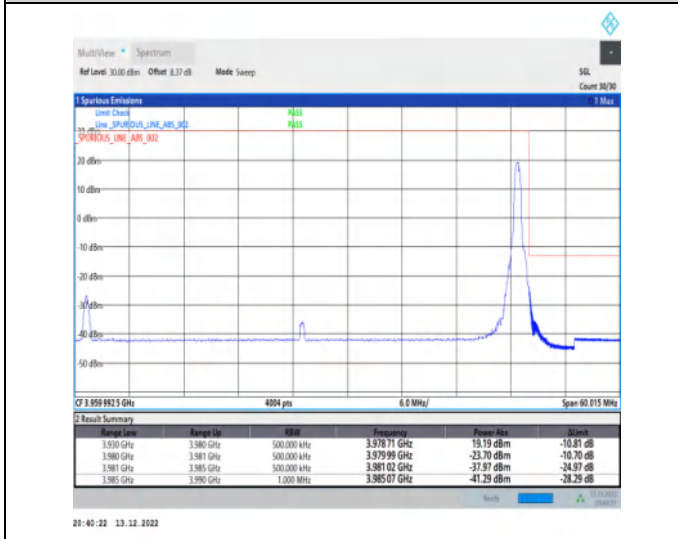
1-N77-3700-3980-30-50-H-5-CP-QPSK-Edge_1RB_Right-1@132-Ant1-1--PASS-see graph
