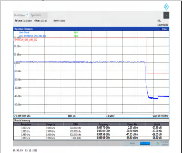
1-N77-3700-3980-30-60-H-3-DFT-PI2BPSK-Outer_Full-162@0-Ant1-1--PASS-see graph
