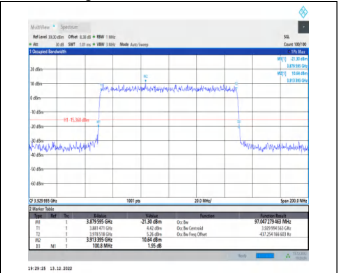
1-N77-3700-3980-30-100-H-6-CP-QPSK-Outer_Full-273@0-Ant1-97.047-100.800-≤100-PASS
