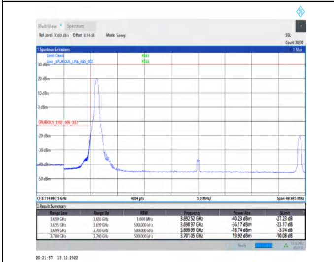
1-N77-3700-3980-30-40-L-4-CP-QPSK-Edge_1RB_Lef t-1@0-Ant1-1--PASS-see graph
