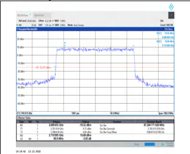
1-N77-3700-3980-30-90-L-7-CP-16QAM-Outer_Full-245@0-Ant1-87.205-90.900≤90-PASS
