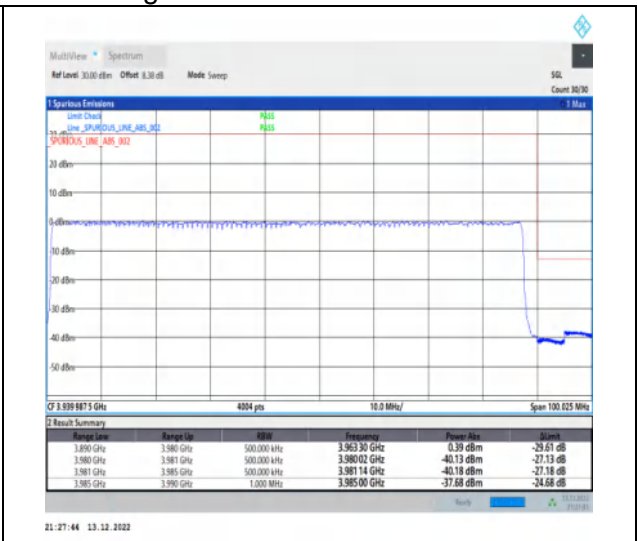
1-N77-3700-3980-30-90-H-3-DFT-PI2BPSK-Outer_Full-240@0-Ant1-1--PASS-see graph
