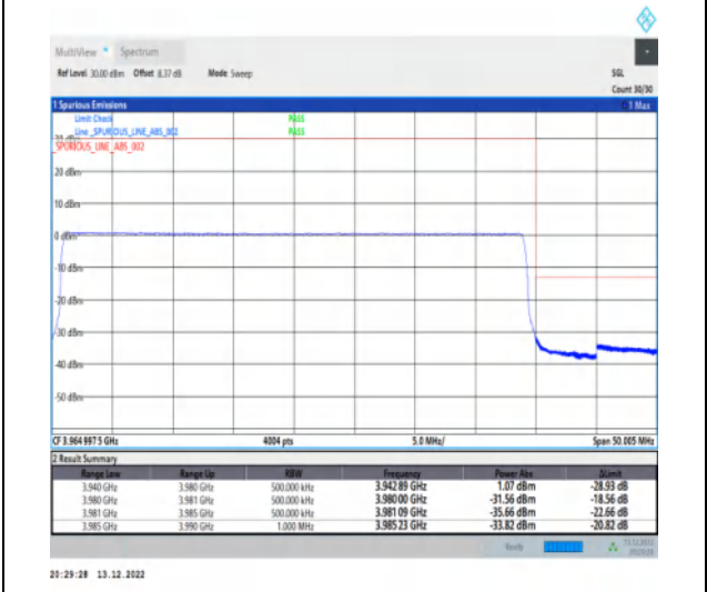
1-N77-3700-3980-30-40-H-6-CP-QPSK-Outer_Full-106@0-Ant1-1--PASS-see graph
