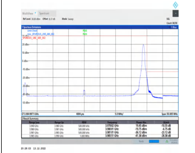
1-N77-3700-3980-30-40-H-5-CP-QPSK-Edge_1RB_Right-1@105-Ant1-1--PASS-see graph
