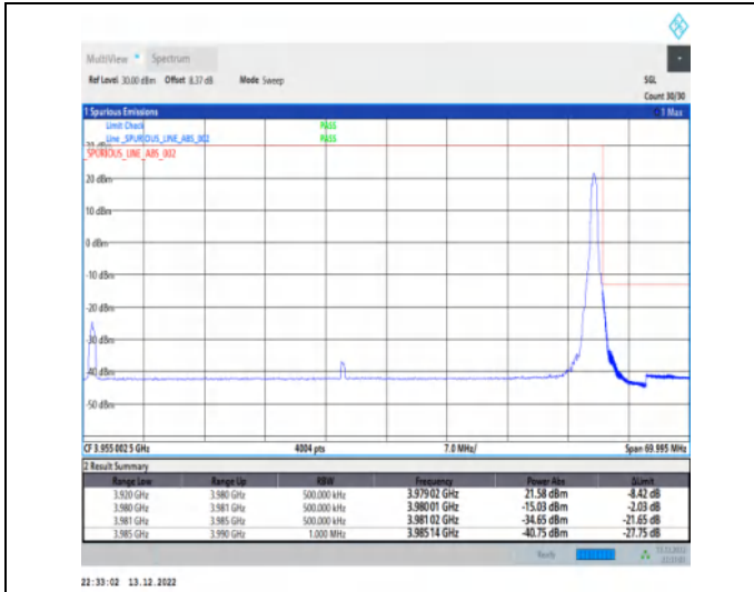
1-N77-3700-3980-30-60-H-2-DFT-PI2BPSK-Edge_1R_B_Right-1@161-Ant1-1--PASS-see graph
