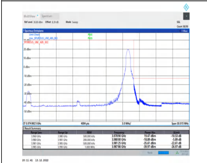
1-N77-3700-3980-30-20-H-5-CP-QPSK-Edge_1RB_Right-1@50-Ant1-1--PASS-see graph
