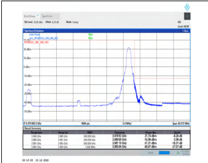
1-N77-3700-3980-30-20-H-2-DFT-PI2BPSK-Edge_1R_B_Right-1@50-Ant1-1--PASS-see graph
