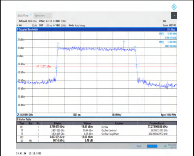
1-N77-3700-3980-30-80-M-3-DFT-16QAM-Outer_Full-216@0-Ant1-77.274-80.160-≤80-PASS
