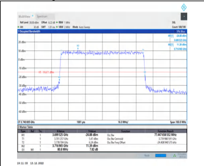
1-N77-3700-3980-30-80-L-6-CP-QPSK-Outer_Full-2 17@0-Ant1-77.448-80.800-≤80-PASS
