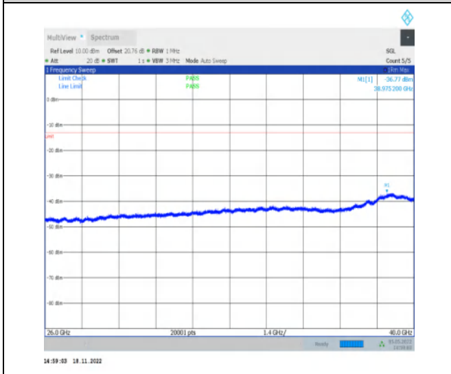
1-N77-3700-3980-30-100-L-1-DFT-QPSK-Edge_1R B_Left-1@0-26000-40000-Ant1-26000.00--42.90--13 -PASS
