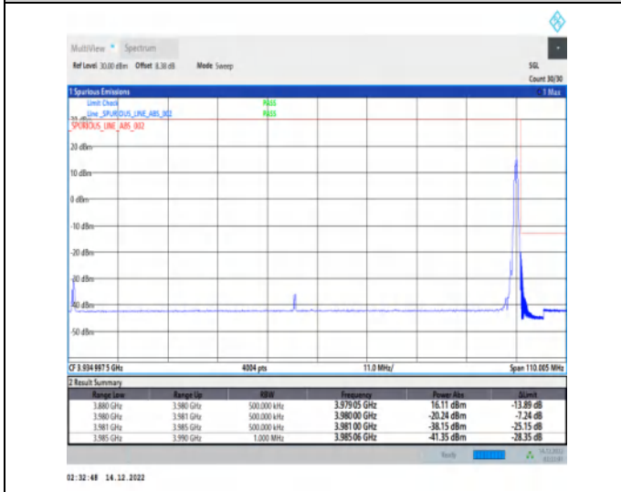
1-N77-3700-3980-30-100-H-5-CP-QPSK-Edge_1RB_R ight-1@272-Ant1-1--PASS-see graph
