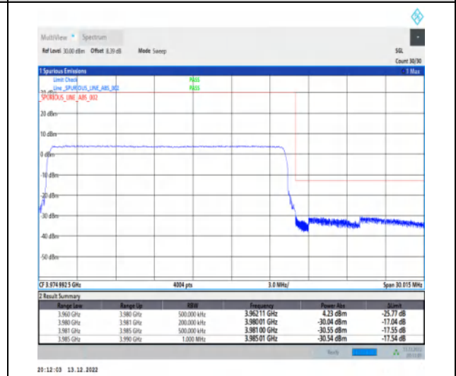
1-N77-3700-3980-30-20-H-6-CP-QPSK-Outer_Full-51@0-Ant1-1--PASS-see graph
