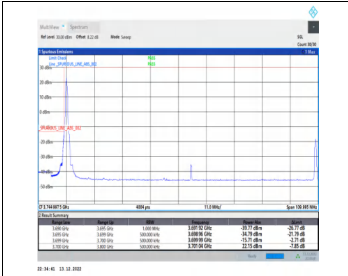
1-N77-3700-3980-30-100-L-1-DFT-PI2BPSK-Edge_1R B_Left-1@0-Ant1-1--PASS-see graph
