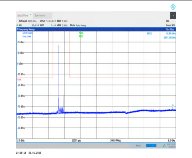
1-N77-3700-3980-30-100-M-1-DFT-QPSK-Edge_1R B_Left-1@0-3000-6000-Ant1-5941.35--42.34--13-PA SS
