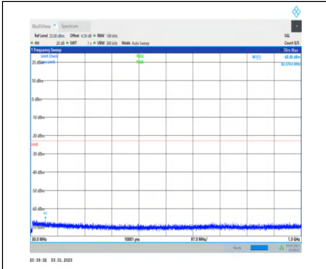
1-N77-3700-3980-30-100-H-1-DFT-QPSK-Edge_1R B_Left-1@0-30-1000-Ant1-82.57--65.96--23-PASS
