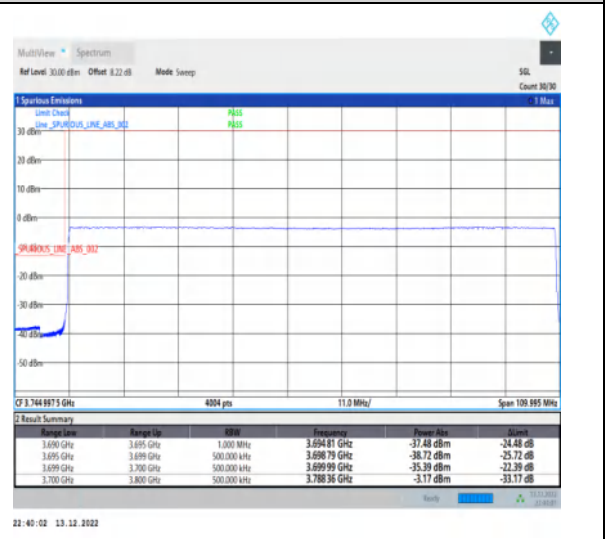
1-N77-3700-3980-30-100-L-6-CP-QPSK-Outer_Full-273@0-Ant1-1--PASS-see graph
