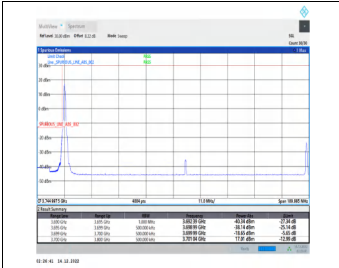
1-N77-3700-3980-30-100-L-4-CP-QPSK-Edge_1RB_L eft-1@0-Ant1-1--PASS-see graph
