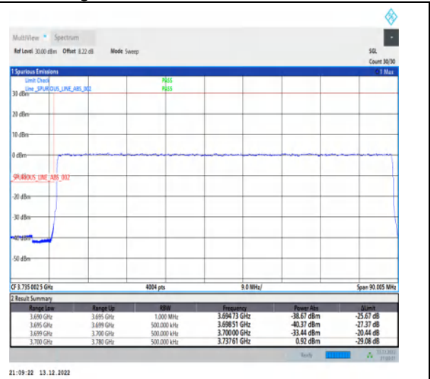
1-N77-3700-3980-30-80-L-3-DFT-PI2BPSK-Outer _Full-216@0-Ant1-1--PASS-see graph
