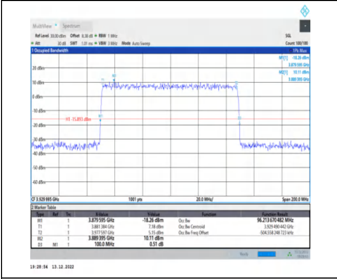
1-N77-3700-3980-30-100-H-3-DFT-16QAM-Outer_Full -270@0-Ant1-96.214-100.000-≤100-PASS
