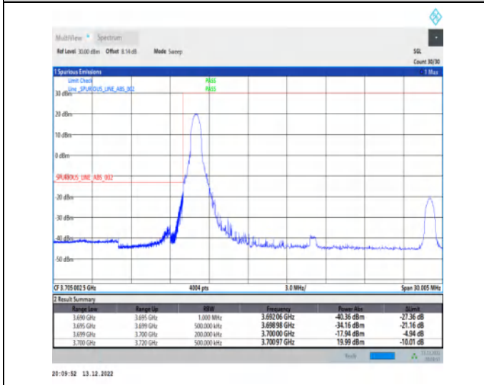
1-N77-3700-3980-30-20-L-4-CP-QPSK-Edge_1RB_Lef t-1@0-Ant1-1--PASS-see graph
