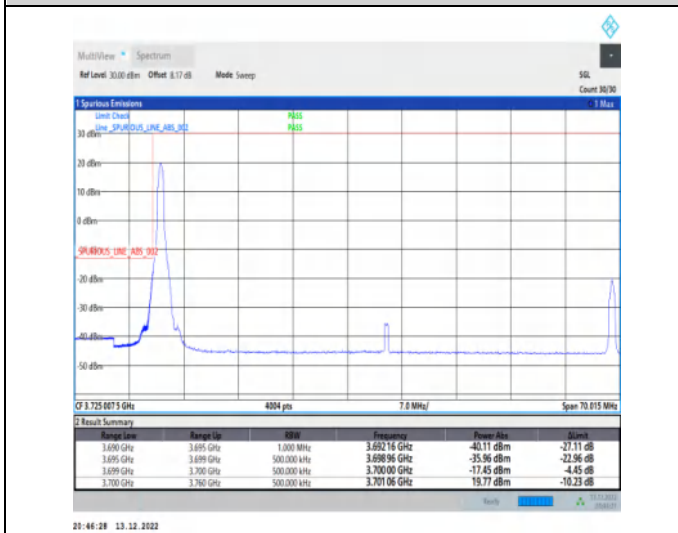
1-N77-3700-3980-30-60-L-4-CP-QPSK-Edge_1RB_Lef t-1@0-Ant1-1--PASS-see graph
