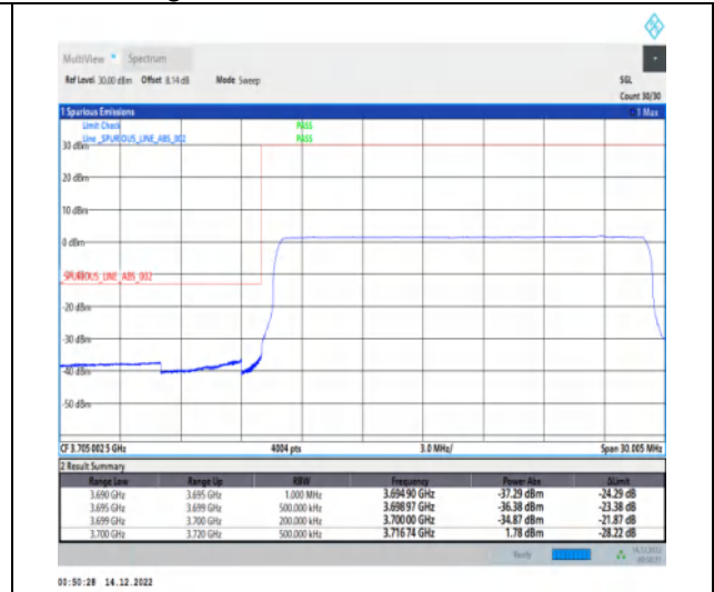
1-N77-3700-3980-30-20-L-6-CP-QPSK-Outer_Full -51@0-Ant1-1--PASS-see graph
