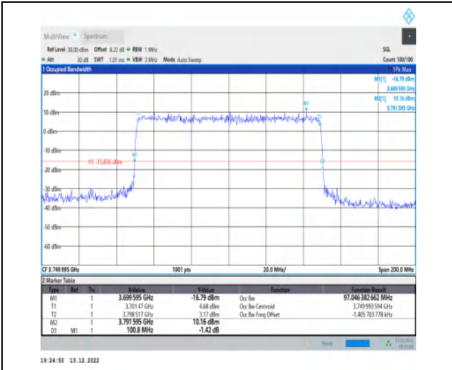
1-N77-3700-3980-30-100-L-7-CP-16QAM-Outer_Full -273@0-Ant1-97.046-100.800-≤100-PASS
