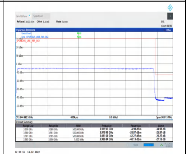
1-N77-3700-3980-30-80-H-6-CP-QPSK-Outer_Full -217@0-Ant1-1--PASS-see graph
