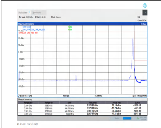
1-N77-3700-3980-30-90-H-5-CP-QPSK-Edge_1RB_Right-1@244-Ant1-1--PASS-see graph
