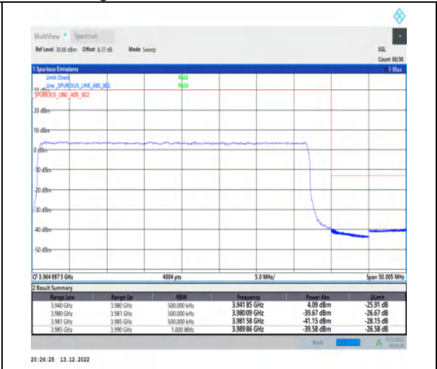
1-N77-3700-3980-30-40-H-3-DFT-PI2BPSK-Outer_Full-100@0-Ant1-1--PASS-see graph
