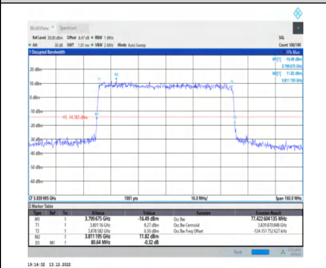
1-N77-3700-3980-30-80-M-7-CP-16QAM-Outer_Full-217@0-Ant1-77.423-80.640-≤80-PASS
