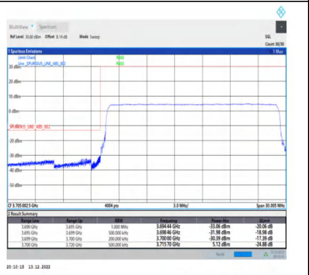
1-N77-3700-3980-30-20-L-6-CP-QPSK-Outer_Full -51@0-Ant1-1--PASS-see graph
