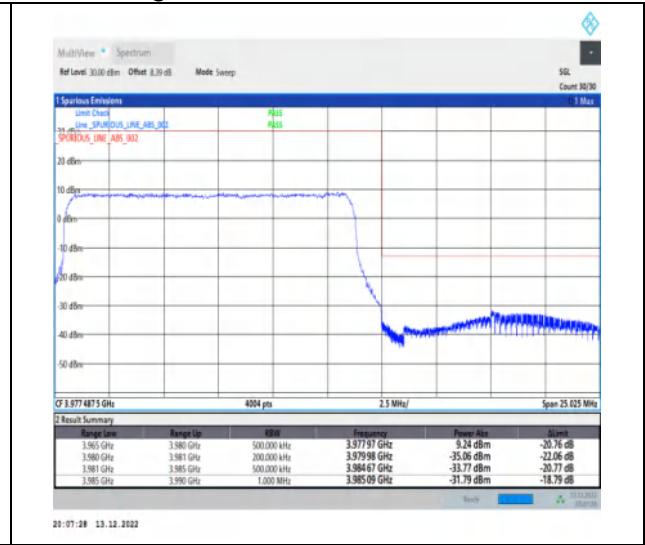
1-N77-3700-3980-30-15-H-3-DFT-PI2BPSK-Outer_Full-36@0-Ant1-1--PASS-see graph
