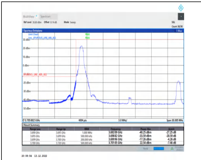
1-N77-3700-3980-30-20-L-1-DFT-PI2BPSK-Edge_1RB _Left-1@0-Ant1-1--PASS-see graph
