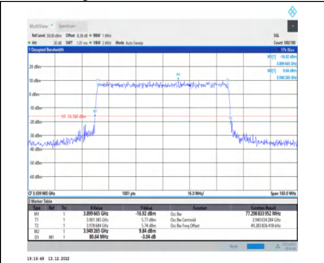
1-N77-3700-3980-30-80-H-8-CP-64QAM-Outer_Full-217@0-Ant1-77.299-80.640-≤80-PASS
