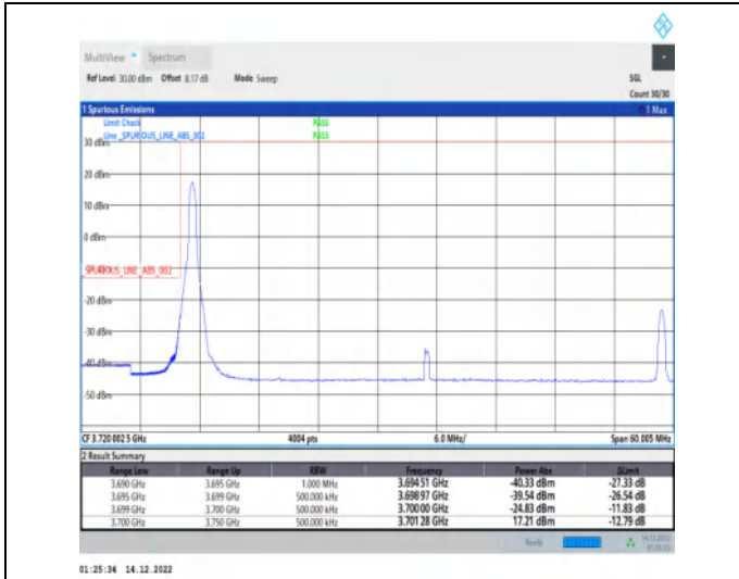
1-N77-3700-3980-30-50-L-4-CP-QPSK-Edge_1RB_Lef t-1@0-Ant1-1--PASS-see graph
