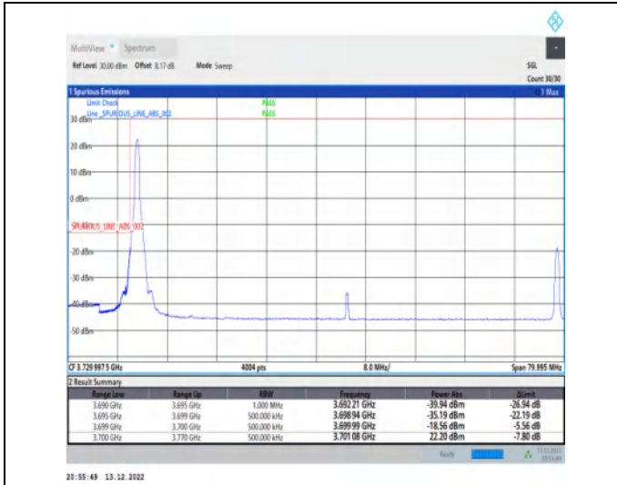
1-N77-3700-3980-30-70-L-1-DFT-PI2BPSK-Edge_1RB _Left-1@0-Ant1-1--PASS-see graph
