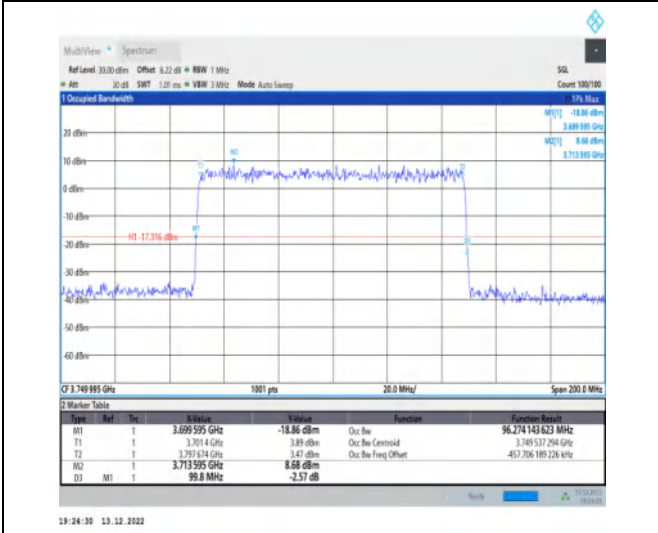
1-N77-3700-3980-30-100-L-5-DFT-256QAM-Outer_Full-270@0-Ant1-96.274-99.800-≤100-PASS
