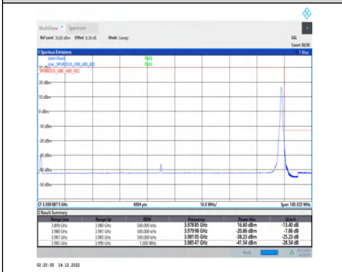
1-N77-3700-3980-30-90-H-5-CP-QPSK-Edge_1RB_Ri ght-1@244-Ant1-1--PASS-see graph
