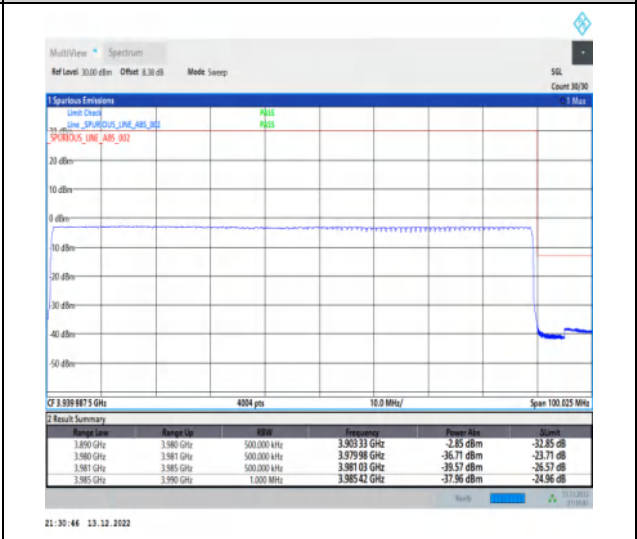
1-N77-3700-3980-30-90-H-6-CP-QPSK-Outer_Full-245@0-Ant1-1--PASS-see graph
