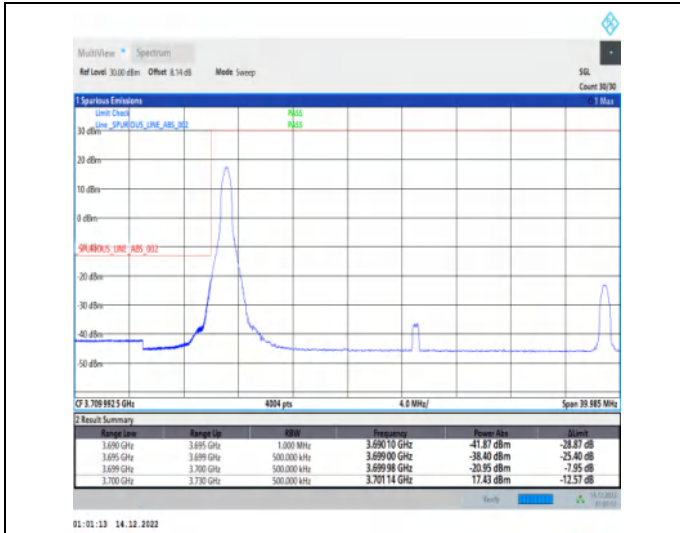
1-N77-3700-3980-30-30-L-4-CP-QPSK-Edge_1RB_Lef t-1@0-Ant1-1--PASS-see graph
