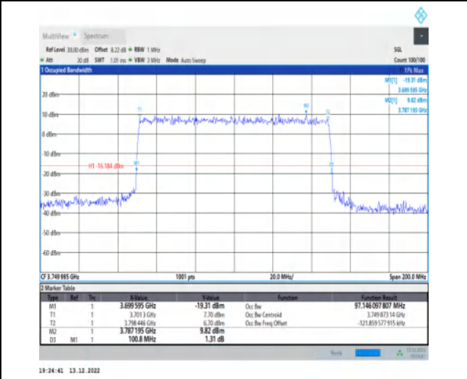
1-N77-3700-3980-30-100-L-6-CP-QPSK-Outer_Full-273@0-Ant1-97.146-100.800-≤100-PASS
