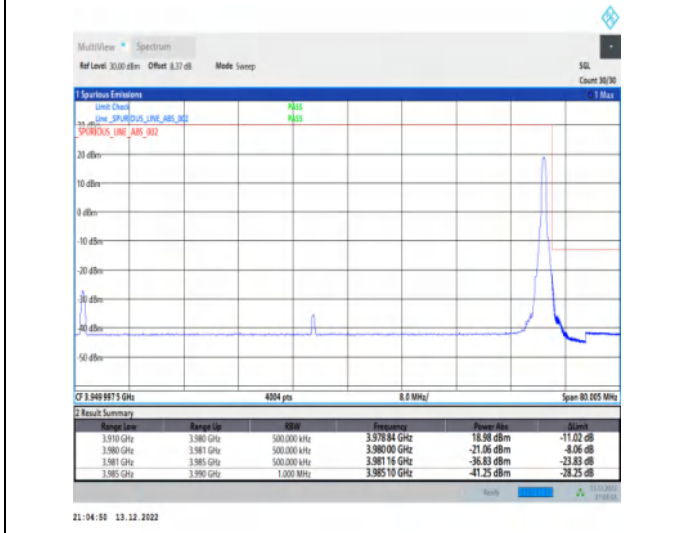
1-N77-3700-3980-30-70-H-5-CP-QPSK-Edge_1RB_Right-1@188-Ant1-1--PASS-see graph
