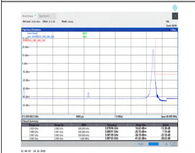
1-N77-3700-3980-30-60-H-5-CP-QPSK-Edge_1RB_Ri ght-1@161-Ant1-1--PASS-see graph
