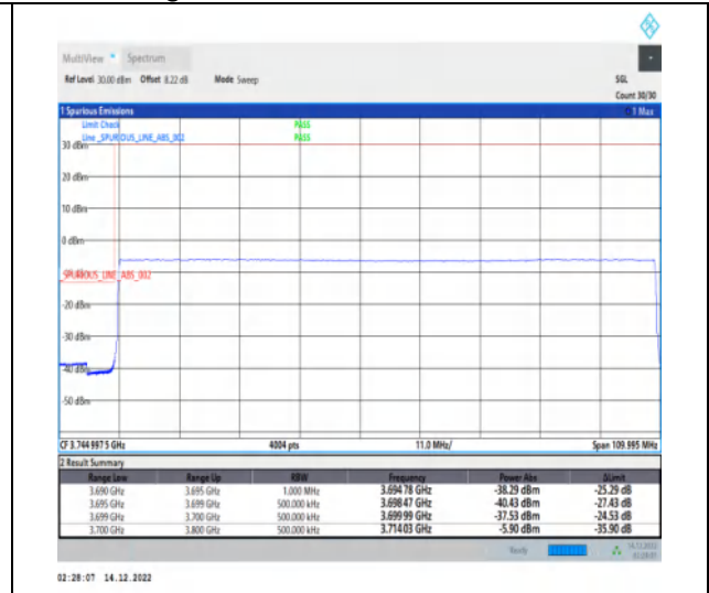
1-N77-3700-3980-30-100-L-6-CP-QPSK-Outer_Fu ll-273@0-Ant1-1--PASS-see graph
