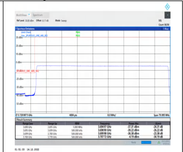
1-N77-3700-3980-30-70-L-6-CP-QPSK-Outer_Full -189@0-Ant1-1--PASS-see graph
