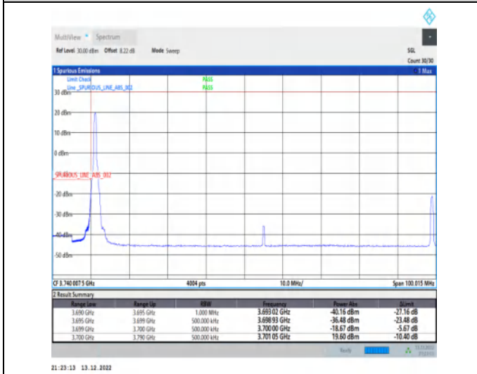
1-N77-3700-3980-30-90-L-4-CP-QPSK-Edge_1RB_Lef t-1@0-Ant1-1--PASS-see graph
