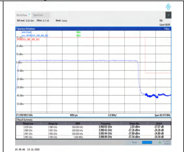
1-N77-3700-3980-30-50-H-3-DFT-PI2BPSK-Outer_Full-128@0-Ant1-1--PASS-see graph
