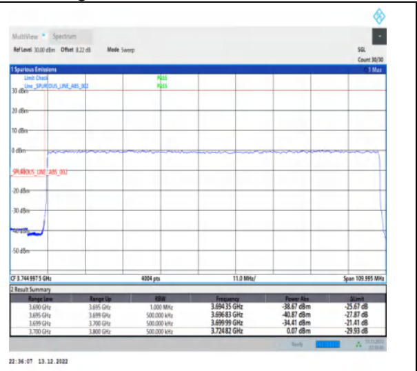
1-N77-3700-3980-30-100-L-3-DFT-PI2BPSK-Outer_Full-270@0-Ant1-1--PASS-see graph
