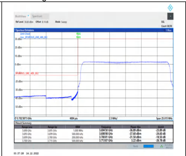
1-N77-3700-3980-30-15-L-6-CP-QPSK-Outer_Full -38@0-Ant1-1--PASS-see graph
