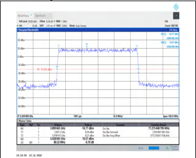
1-N77-3700-3980-30-80-H-4-DFT-64QAM-Outer_Ful I-216@0-Ant1-77.215-80.320-≤80-PASS
