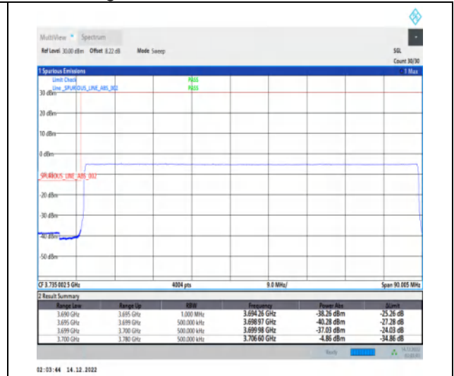
1-N77-3700-3980-30-80-L-6-CP-QPSK-Outer_Full -217@0-Ant1-1--PASS-see graph
