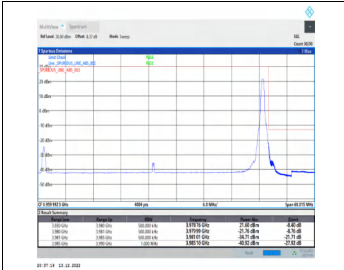
1-N77-3700-3980-30-50-H-2-DFT-PI2BPSK-Edge_1R_B_Right-1@132-Ant1-1--PASS-see graph
