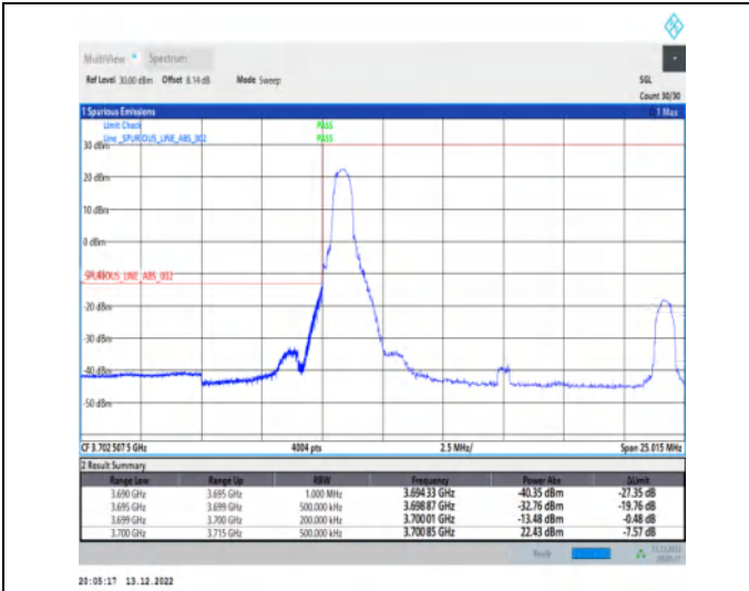
1-N77-3700-3980-30-15-L-1-DFT-PI2BPSK-Edge_1RB _Left-1@0-Ant1-1--PASS-see graph
