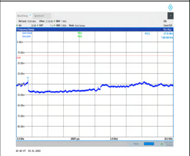
1-N77-3700-3980-30-100-H-1-DFT-QPSK-Edge_1R B_Left-1@0-6000-26000-Ant1-7482.00--37.25--13-P ASS
