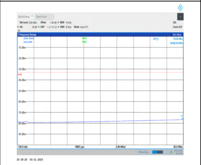
1-N77-3700-3980-30-100-H-1-DFT-QPSK-Edge_1R B_Left-1@0-0.15-30-Ant1-29.80--76.58--33-PASS
