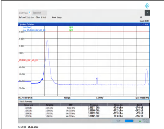
1-N77-3700-3980-30-40-L-4-CP-QPSK-Edge_1RB_Lef t-1@0-Ant1-1--PASS-see graph
