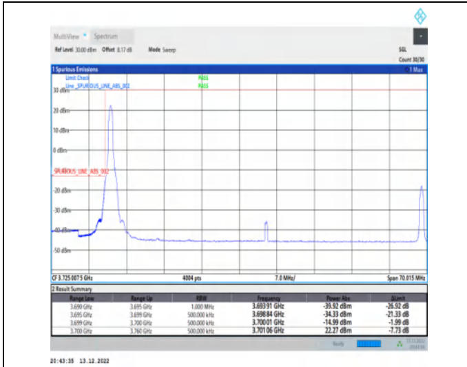
1-N77-3700-3980-30-60-L-1-DFT-PI2BPSK-Edge_1RB _Left-1@0-Ant1-1--PASS-see graph
