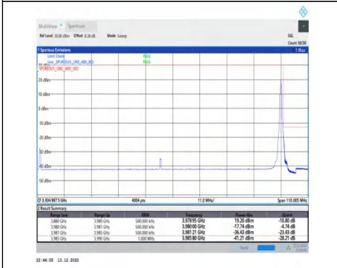
1-N77-3700-3980-30-100-H-5-CP-QPSK-Edge_1RB_Right-1@272-Ant1-1--PASS-see graph
