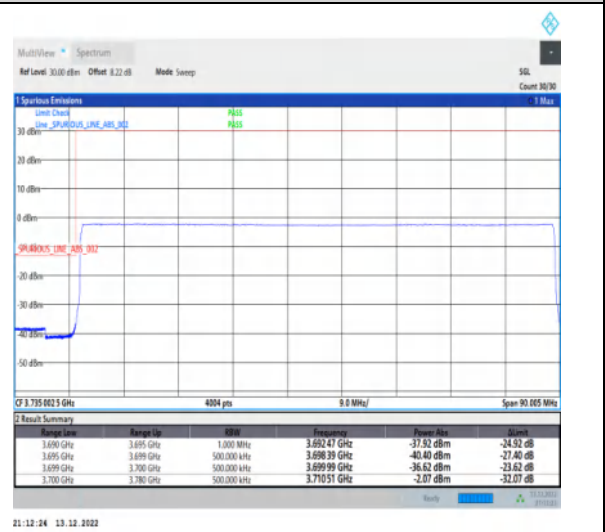
1-N77-3700-3980-30-80-L-6-CP-QPSK-Outer_Full -217@0-Ant1-1--PASS-see graph
