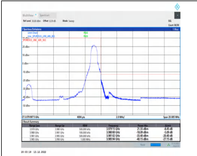
1-N77-3700-3980-30-10-H-2-DFT-PI2BPSK-Edge_1R_B_Right-1@23-Ant1-1--PASS-see graph
