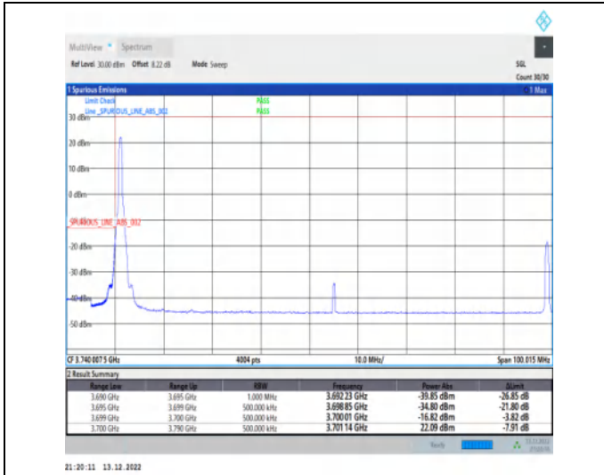
1-N77-3700-3980-30-90-L-1-DFT-PI2BPSK-Edge_1RB _Left-1@0-Ant1-1--PASS-see graph
