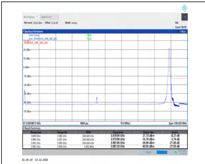
1-N77-3700-3980-30-90-H-2-DFT-PI2BPSK-Edge_1R_B_Right-1@244-Ant1-1--PASS-see graph
