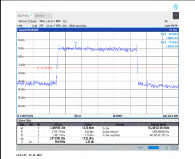
1-N77-3700-3980-30-100-M-1-DFT-QPSK-Outer_Full-270@0-Ant1-96.239-99.800-≤100-PASS
