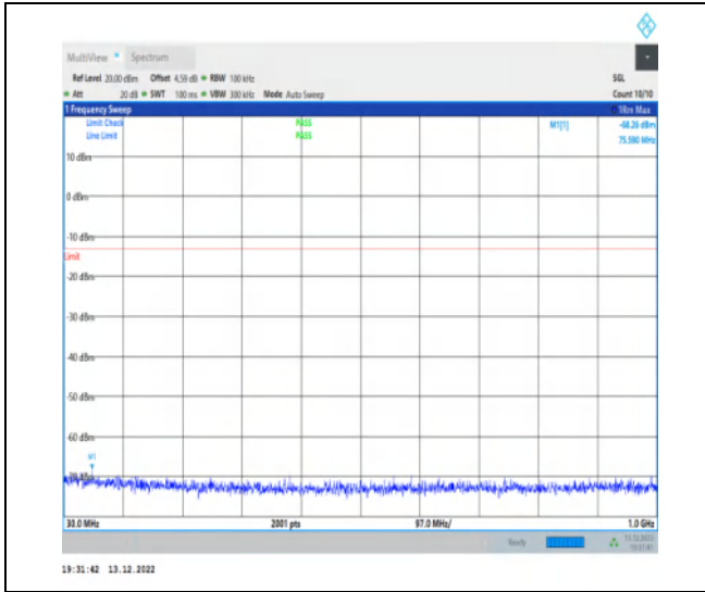
1-N77-3700-3980-30-100-M-1-DFT-PI2BPSK-Inner_1RB_Left-1@1-30-1000-Ant1-75.59--68.26--13-PAS S
