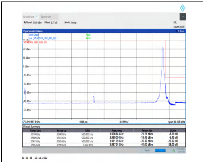
1-N77-3700-3980-30-70-H-2-DFT-PI2BPSK-Edge_1R B_Right-1@188-Ant1-1--PASS-see graph
