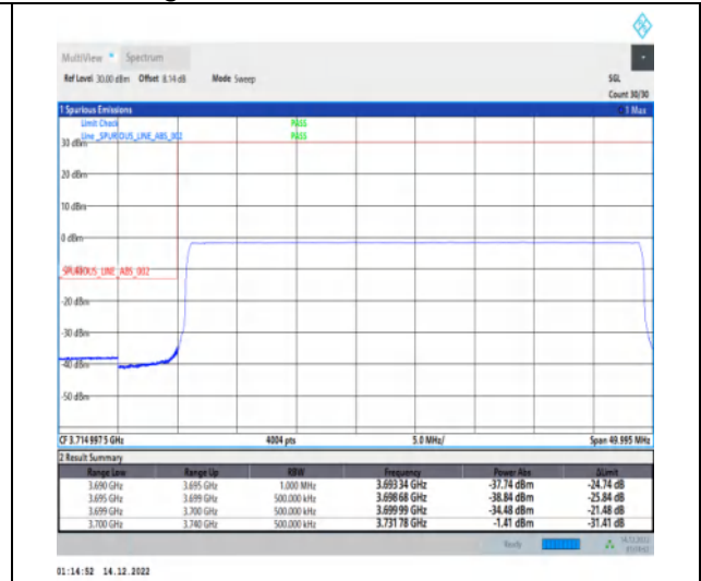
1-N77-3700-3980-30-40-L-6-CP-QPSK-Outer_Full -106@0-Ant1-1--PASS-see graph
