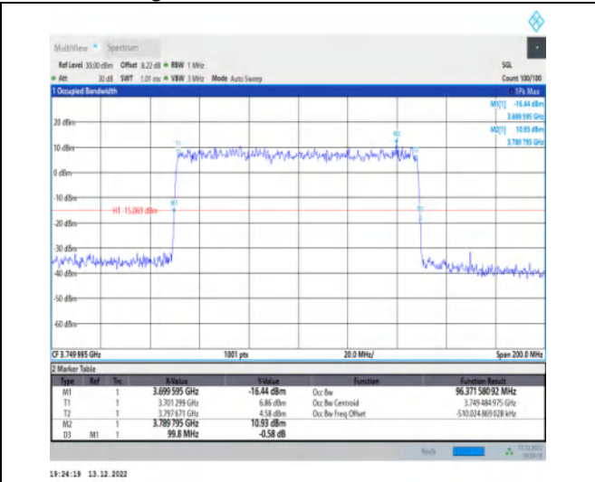
1-N77-3700-3980-30-100-L-4-DFT-64QAM-Outer_Full-270@0-Ant1-96.372-99.800-≤100-PASS
