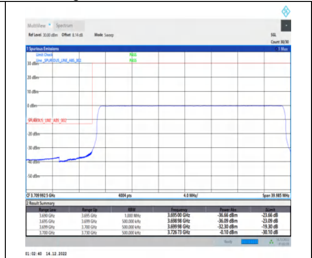
1-N77-3700-3980-30-30-L-6-CP-QPSK-Outer_Full -78@0-Ant1-1--PASS-see graph
