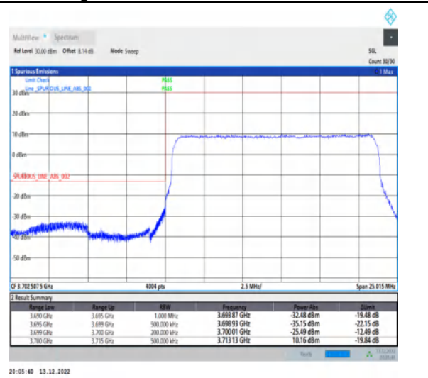
1-N77-3700-3980-30-15-L-3-DFT-PI2BPSK-Outer _Full-36@0-Ant1-1--PASS-see graph
