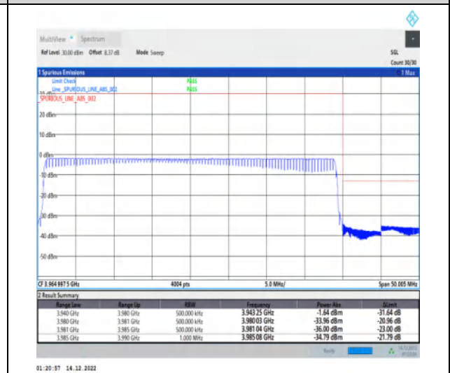
1-N77-3700-3980-30-40-H-6-CP-QPSK-Outer_Full -106@0-Ant1-1--PASS-see graph
