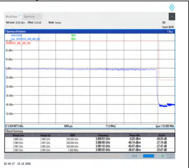
1-N77-3700-3980-30-100-H-3-DFT-PI2BPSK-Outer_Full-270@0-Ant1-1--PASS-see graph
