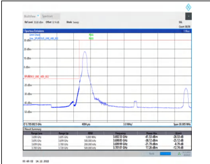
1-N77-3700-3980-30-20-L-4-CP-QPSK-Edge_1RB_Lef t-1@0-Ant1-1--PASS-see graph
