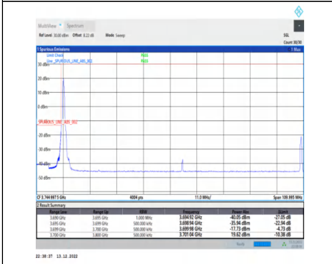
1-N77-3700-3980-30-100-L-4-CP-QPSK-Edge_1RB_Left-1@0-Ant1-1--PASS-see graph
