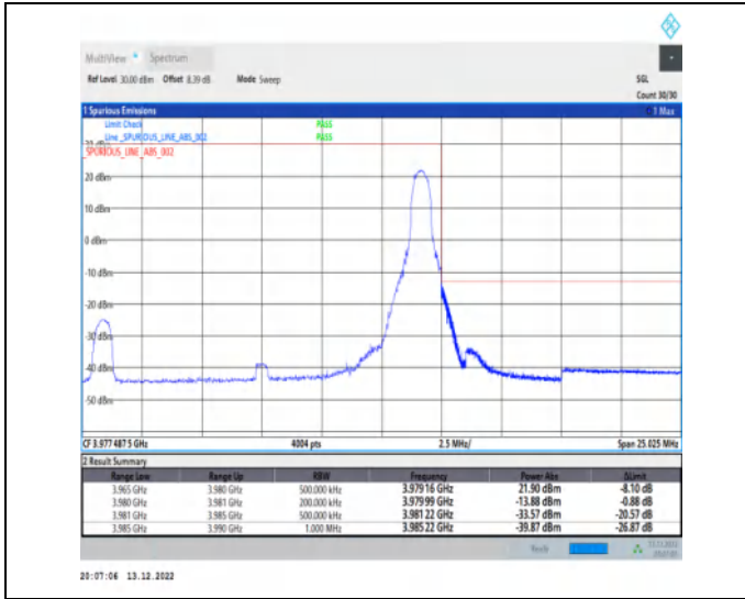
1-N77-3700-3980-30-15-H-2-DFT-PI2BPSK-Edge_1R_B_Right-1@37-Ant1-1--PASS-see graph
