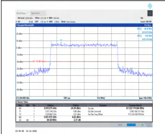
1-N77-3700-3980-30-70-H-8-CP-64QAM-Outer_Full-189@0-Ant1-67.522-69.580-≤70-PASS
