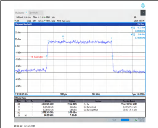
1-N77-3700-3980-30-80-L-5-DFT-256QAM-Outer_Fu II-216@0-Ant1-77.327-80.320-≤80-PASS
