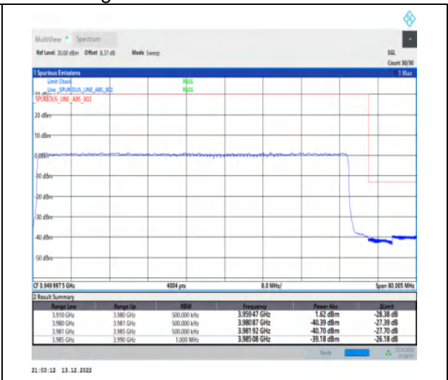
1-N77-3700-3980-30-70-H-3-DFT-PI2BPSK-Outer_Full-180@0-Ant1-1--PASS-see graph
