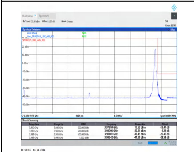
1-N77-3700-3980-30-70-H-5-CP-QPSK-Edge_1RB_Ri ght-1@188-Ant1-1--PASS-see graph
