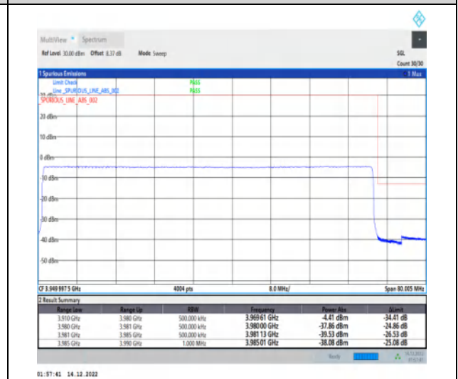
1-N77-3700-3980-30-70-H-6-CP-QPSK-Outer_Full -189@0-Ant1-1--PASS-see graph
