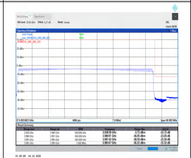
1-N77-3700-3980-30-60-H-6-CP-QPSK-Outer_Full -162@0-Ant1-1--PASS-see graph
