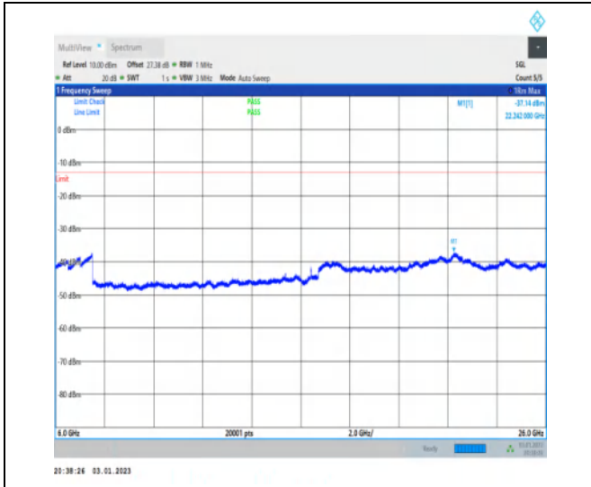
1-N77-3700-3980-30-100-M-1-DFT-QPSK-Edge_1R B_Left-1@0-6000-26000-Ant1-22242.00--37.14--13- PASS
