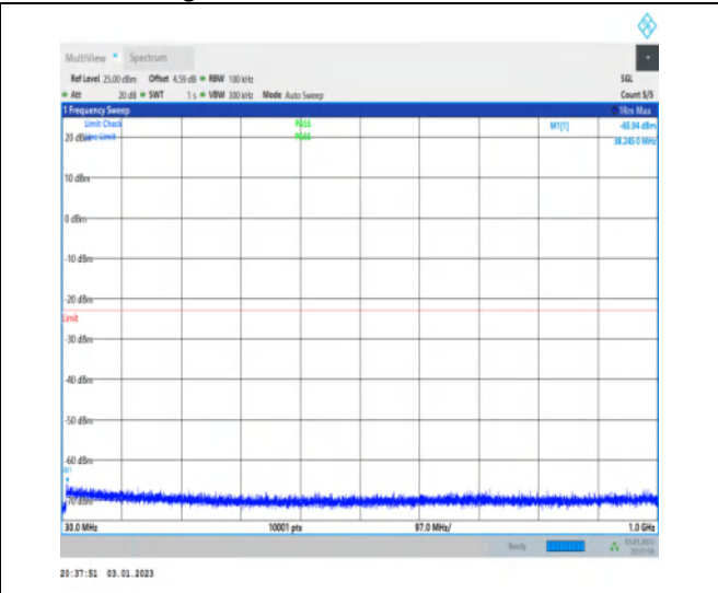
1-N77-3700-3980-30-100-M-1-DFT-QPSK-Edge_1R B_Left-1@0-30-1000-Ant1-38.25--65.94--23-PASS
