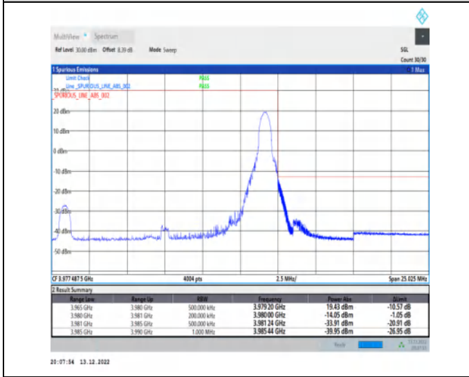
1-N77-3700-3980-30-15-H-5-CP-QPSK-Edge_1RB_Right-1@37-Ant1-1--PASS-see graph
