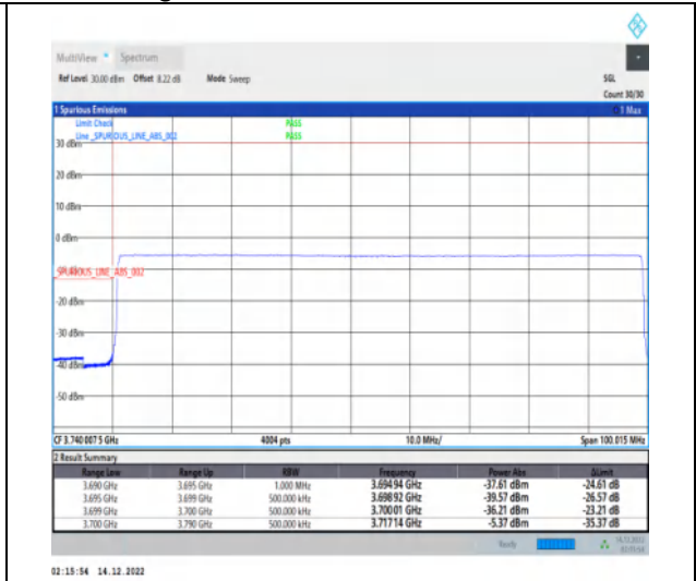
1-N77-3700-3980-30-90-L-6-CP-QPSK-Outer_Full -245@0-Ant1-1--PASS-see graph
