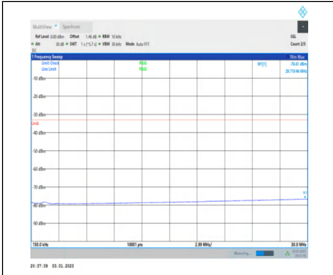
1-N77-3700-3980-30-100-M-1-DFT-QPSK-Edge_1R B_Left-1@0-0.15-30-Ant1-29.71--76.61--33-PASS
