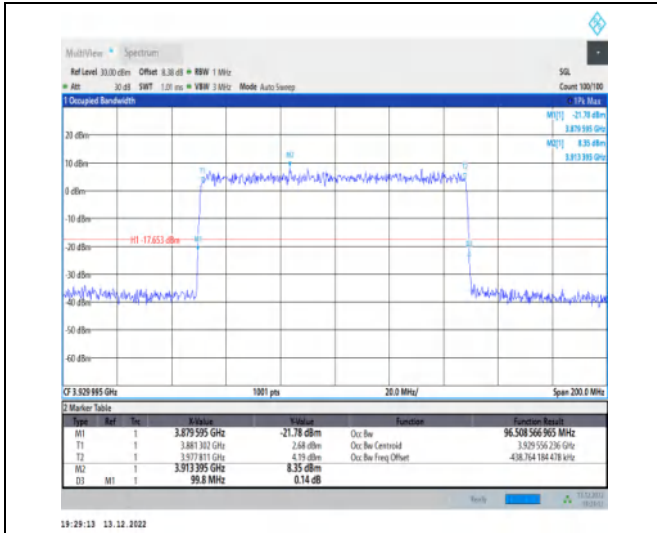
1-N77-3700-3980-30-100-H-5-DFT-256QAM-Outer_Full-270@0-Ant1-96.509-99.800-≤100-PASS
