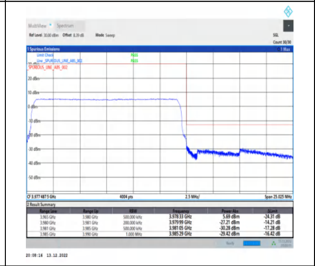
1-N77-3700-3980-30-15-H-6-CP-QPSK-Outer_Full-38@0-Ant1-1--PASS-see graph
