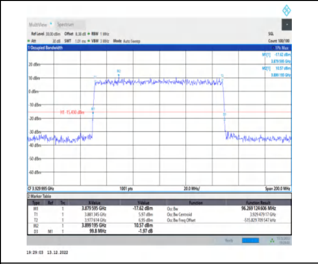
1-N77-3700-3980-30-100-H-4-DFT-64QAM-Outer_Full -270@0-Ant1-96.269-99.800-≤100-PASS
