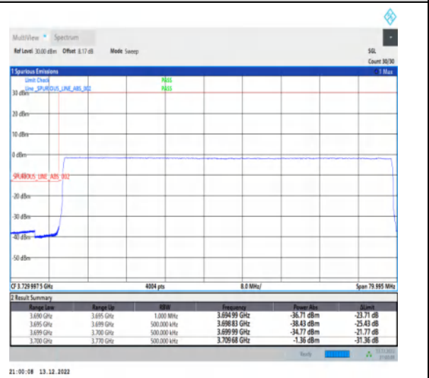
1-N77-3700-3980-30-70-L-6-CP-QPSK-Outer_Full -189@0-Ant1-1--PASS-see graph
