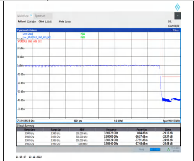
1-N77-3700-3980-30-80-H-3-DFT-PI2BPSK-Outer_Full-216@0-Ant1-1--PASS-see graph
