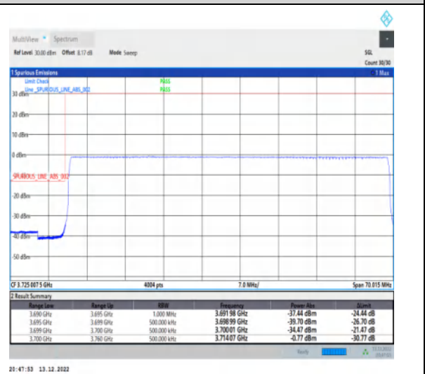
1-N77-3700-3980-30-60-L-6-CP-QPSK-Outer_Full -162@0-Ant1-1--PASS-see graph
