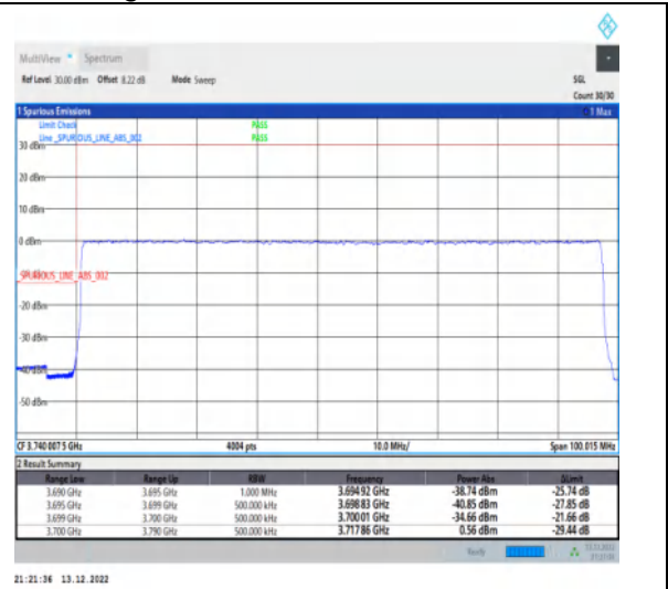
1-N77-3700-3980-30-90-L-3-DFT-PI2BPSK-Outer _Full-240@0-Ant1-1--PASS-see graph
