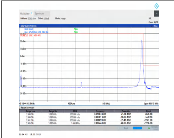
1-N77-3700-3980-30-80-H-2-DFT-PI2BPSK-Edge_1R_B_Right-1@216-Ant1-1--PASS-see graph
