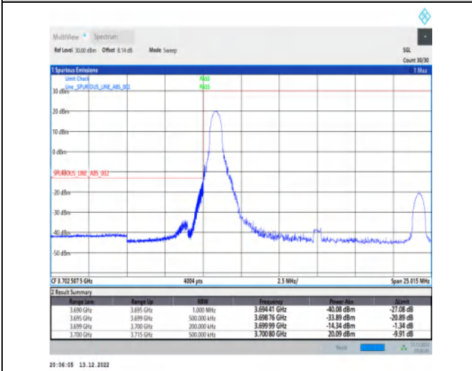
1-N77-3700-3980-30-15-L-4-CP-QPSK-Edge_1RB_Lef t-1@0-Ant1-1--PASS-see graph
