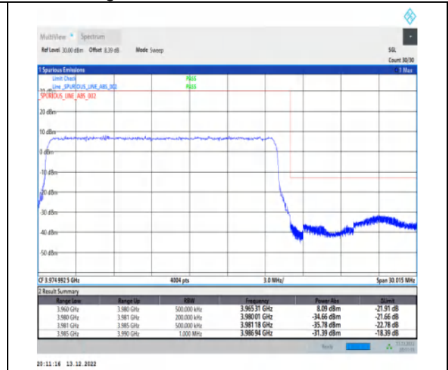
1-N77-3700-3980-30-20-H-3-DFT-PI2BPSK-Outer_Full-50@0-Ant1-1--PASS-see graph
