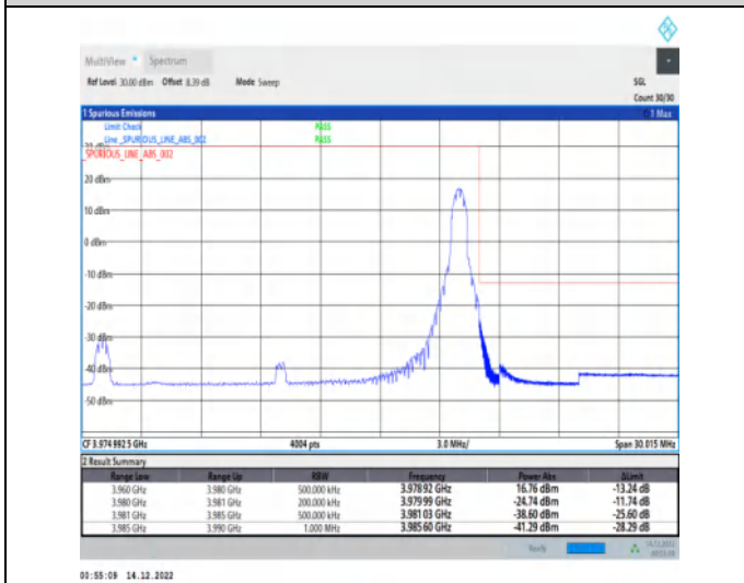
1-N77-3700-3980-30-20-H-5-CP-QPSK-Edge_1RB_Ri ght-1@50-Ant1-1--PASS-see graph
