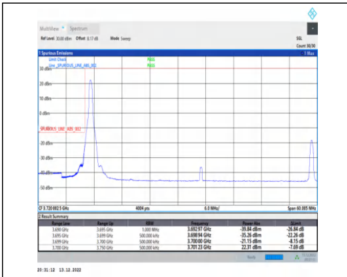
1-N77-3700-3980-30-50-L-1-DFT-PI2BPSK-Edge_1RB _Left-1@0-Ant1-1--PASS-see graph
