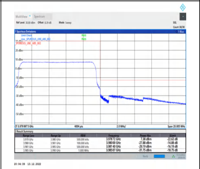
1-N77-3700-3980-30-10-H-6-CP-QPSK-Outer_Full-24@0-Ant1-1--PASS-see graph
