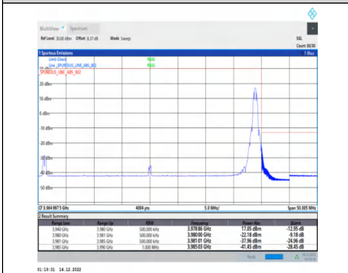
1-N77-3700-3980-30-40-H-5-CP-QPSK-Edge_1RB_Ri ght-1@105-Ant1-1--PASS-see graph
