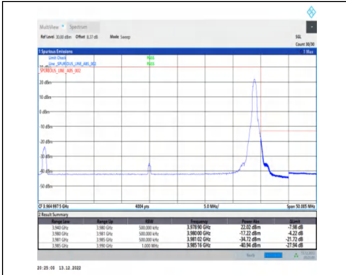
1-N77-3700-3980-30-40-H-2-DFT-PI2BPSK-Edge_1R_B_Right-1@105-Ant1-1--PASS-see graph
