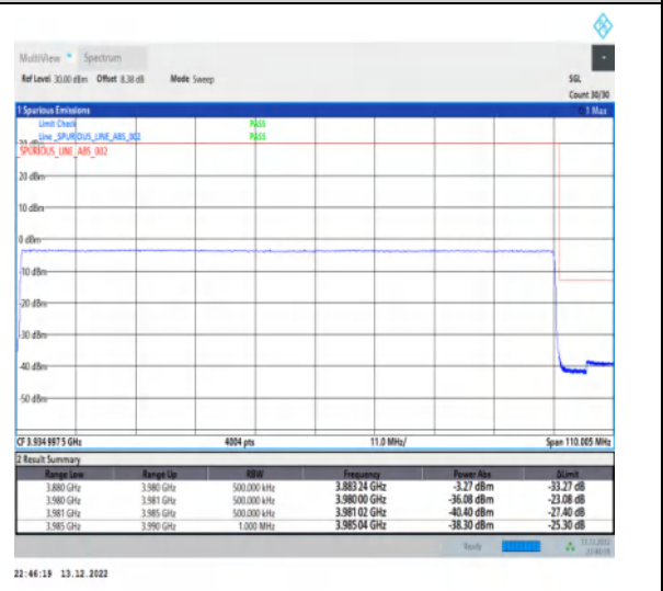
1-N77-3700-3980-30-100-H-6-CP-QPSK-Outer_Full-273@0-Ant1-1--PASS-see graph
