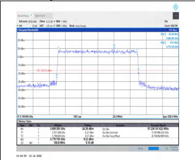
1-N77-3700-3980-30-100-L-8-CP-64QAM-Outer_Full -273@0-Ant1-97.236-100.800-≤100-PASS
