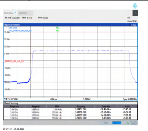
1-N77-3700-3980-30-40-L-3-DFT-PI2BPSK-Outer _Full-100@0-Ant1-1--PASS-see graph
