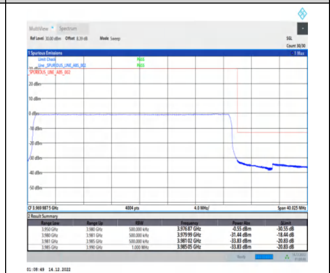
1-N77-3700-3980-30-30-H-6-CP-QPSK-Outer_Full -78@0-Ant1-1--PASS-see graph
