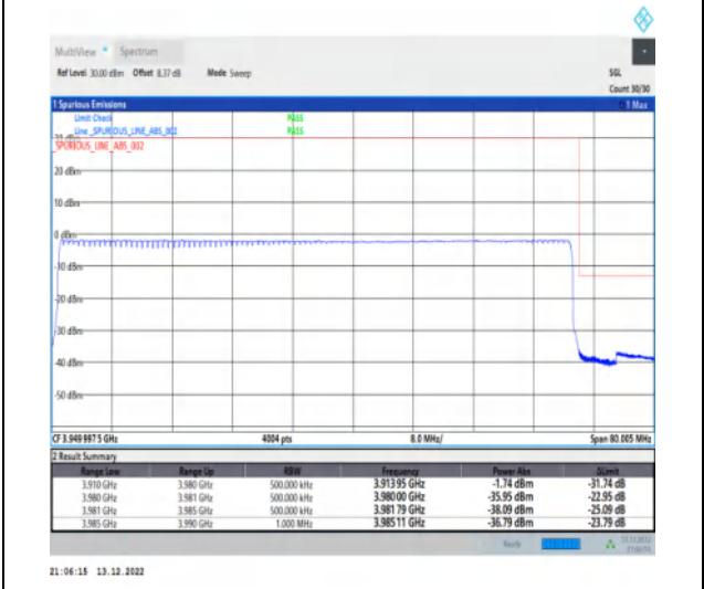
1-N77-3700-3980-30-70-H-6-CP-QPSK-Outer_Full-189@0-Ant1-1--PASS-see graph
