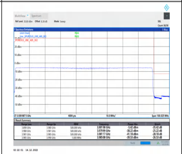
1-N77-3700-3980-30-90-H-6-CP-QPSK-Outer_Full -245@0-Ant1-1--PASS-see graph
