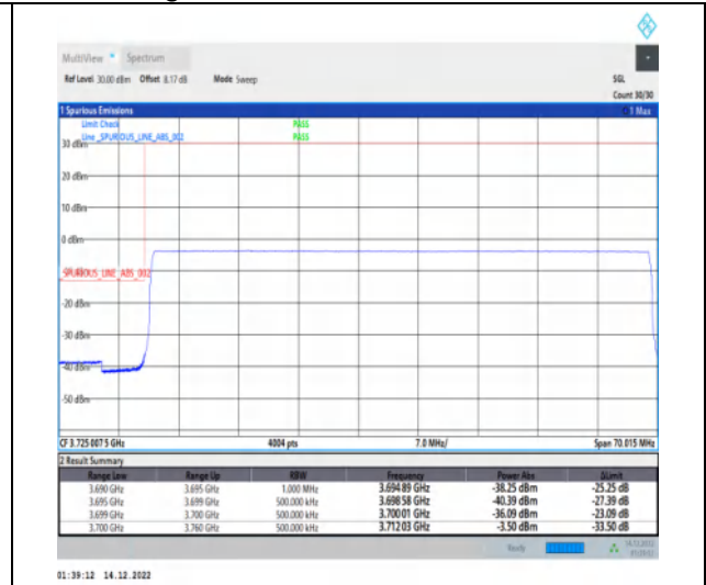
1-N77-3700-3980-30-60-L-6-CP-QPSK-Outer_Full -162@0-Ant1-1--PASS-see graph
