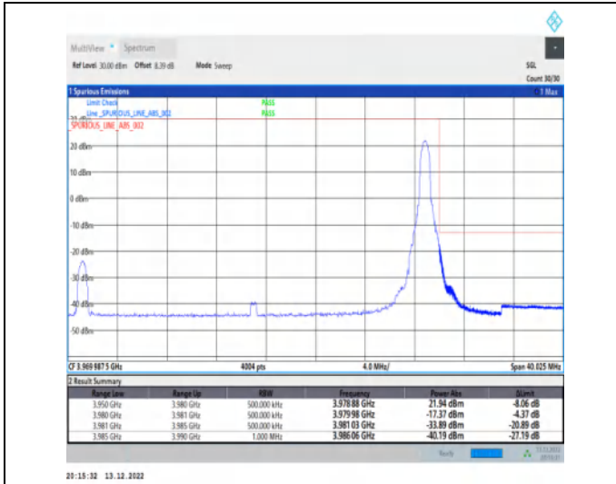
1-N77-3700-3980-30-30-H-2-DFT-PI2BPSK-Edge_1R_B_Right-1@77-Ant1-1--PASS-see graph
