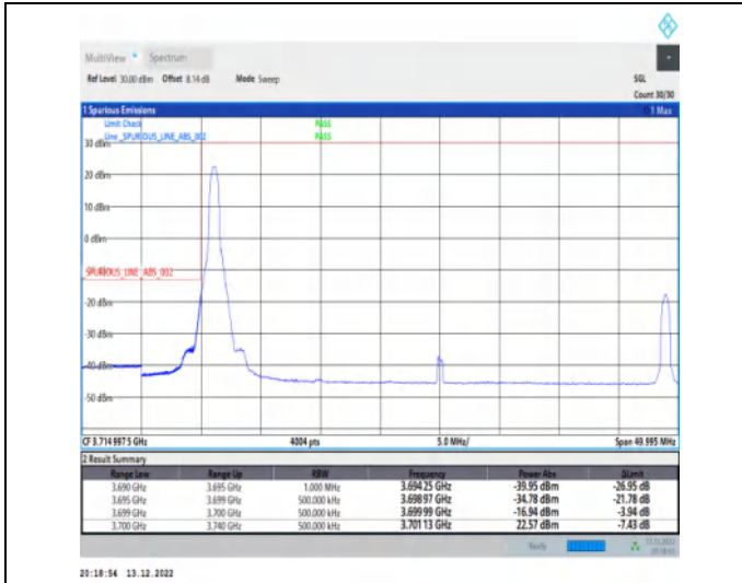
1-N77-3700-3980-30-40-L-1-DFT-PI2BPSK-Edge_1RB _Left-1@0-Ant1-1--PASS-see graph
