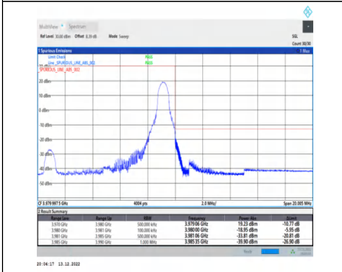
1-N77-3700-3980-30-10-H-5-CP-QPSK-Edge_1RB_Right-1@23-Ant1-1--PASS-see graph
