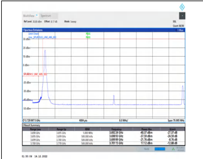
1-N77-3700-3980-30-70-L-4-CP-QPSK-Edge_1RB_Lef t-1@0-Ant1-1--PASS-see graph
