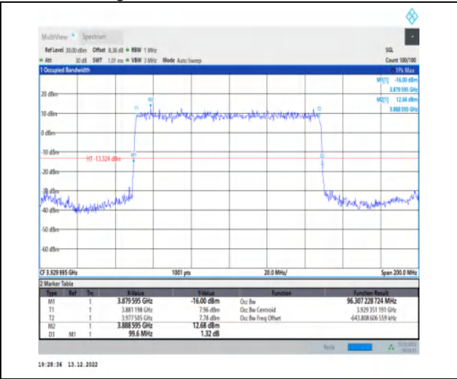
1-N77-3700-3980-30-100-H-2-DFT-PI2BPSK-Outer_Full -270@0-Ant1-96.307-99.600-≤100-PASS
