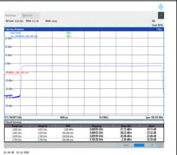
1-N77-3700-3980-30-90-L-6-CP-QPSK-Outer_Full -245@0-Ant1-1--PASS-see graph
