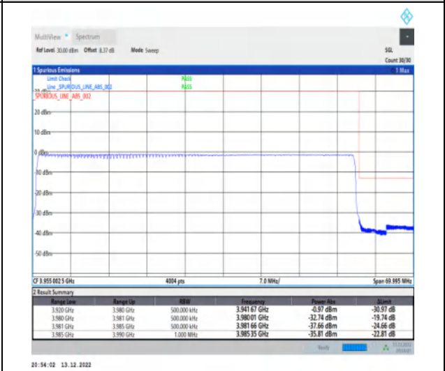
1-N77-3700-3980-30-60-H-6-CP-QPSK-Outer_Full-162@0-Ant1-1--PASS-see graph
