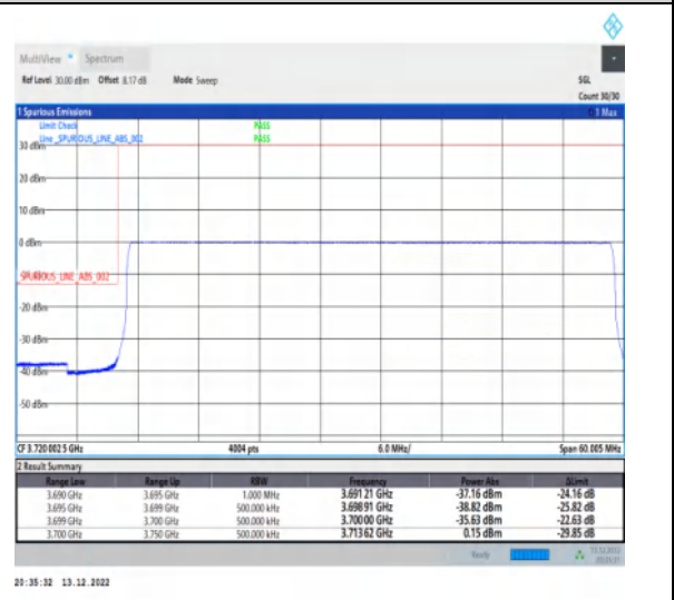
1-N77-3700-3980-30-50-L-6-CP-QPSK-Outer_Full -133@0-Ant1-1--PASS-see graph
