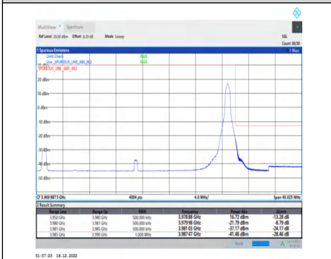
1-N77-3700-3980-30-30-H-5-CP-QPSK-Edge_1RB_Ri ght-1@77-Ant1-1--PASS-see graph
