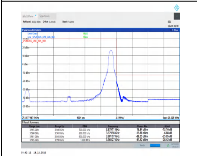
1-N77-3700-3980-30-15-H-5-CP-QPSK-Edge_1RB_Ri ght-1@37-Ant1-1--PASS-see graph
