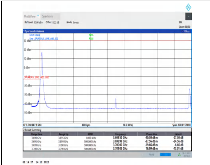
1-N77-3700-3980-30-90-L-4-CP-QPSK-Edge_1RB_Lef t-1@0-Ant1-1--PASS-see graph
