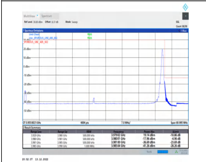
1-N77-3700-3980-30-60-H-5-CP-QPSK-Edge_1RB_Right-1@161-Ant1-1--PASS-see graph
