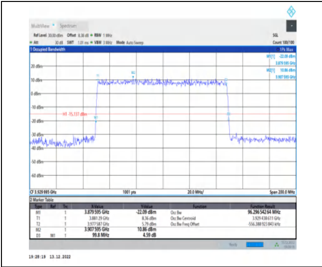
1-N77-3700-3980-30-100-H-1-DFT-QPSK-Outer_Full -270@0-Ant1-96.297-99.800-≤100-PASS
