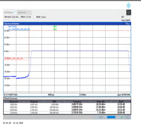
1-N77-3700-3980-30-40-L-6-CP-QPSK-Outer_Full -106@0-Ant1-1--PASS-see graph
