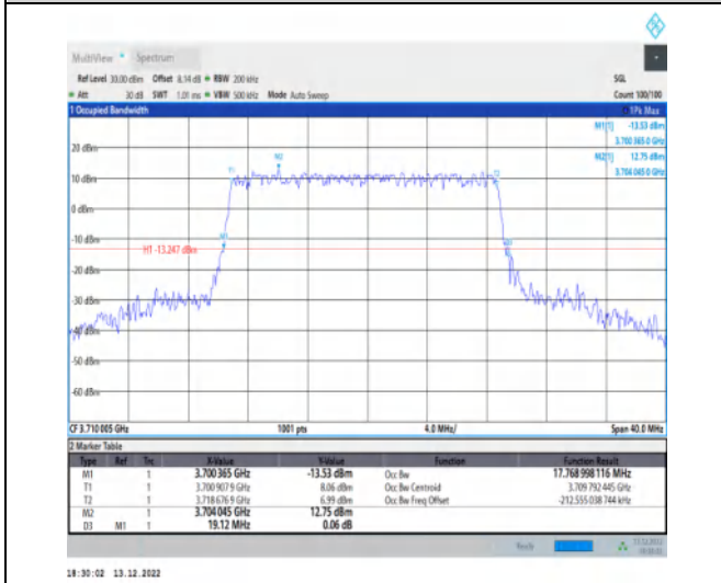
1-N77-3700-3980-30-20-L-1-DFT-QPSK-Outer_Full-50@0-Ant1-17.769-19.120-≤20-PASS
