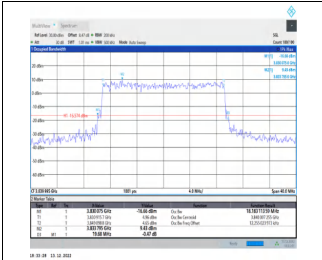
1-N77-3700-3980-30-20-M-6-CP-QPSK-Outer_Full-5 1@0-Ant1-18.183-19.680-≤20-PASS
