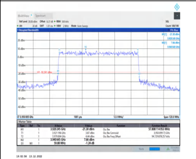
1-N77-3700-3980-30-60-H-8-CP-64QAM-Outer_Full-162@0-Ant1-57.808-59.880-≤60-PASS
