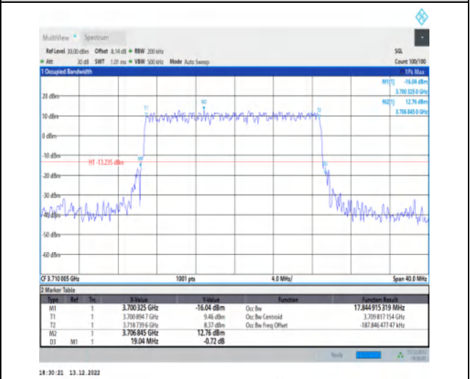
1-N77-3700-3980-30-20-L-2-DFT-PI2BPSK-Outer_Full-50@0-Ant1-17.845-19.040-≤20-PASS
