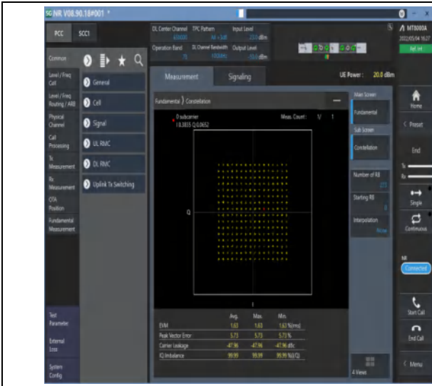
1-N78-3700-3800--30-100-M-9-CP-256QAM-Outer_F ull-273@0-Ant1-see graph-PASS
