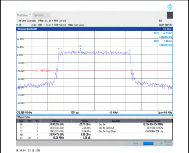
1-N77-3700-3980-30-20-M-9-CP-256QAM-Outer_Fu II-51@0-Ant1-18.135-19.280-≤20-PASS
