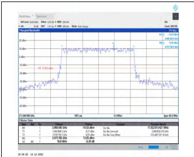
1-N77-3700-3980-30-20-H-1-DFT-QPSK-Outer_Full-50@0-Ant1-17.922-18.800-≤20-PASS
