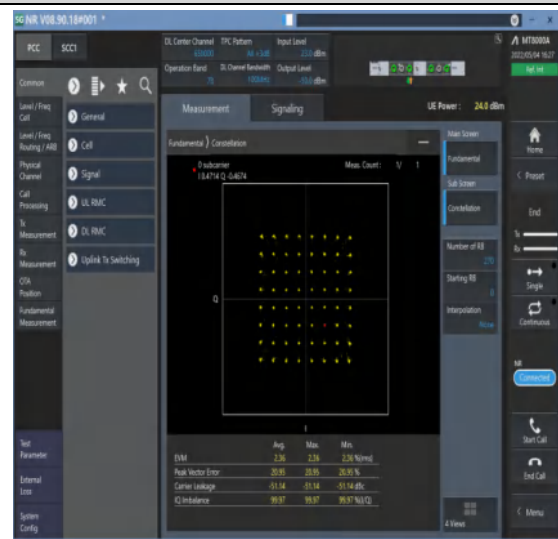
1-N78-3700-3800--30-100-M-4-DFT-64QAM-Outer_Full-270@0-Ant1-see graph-PASS
