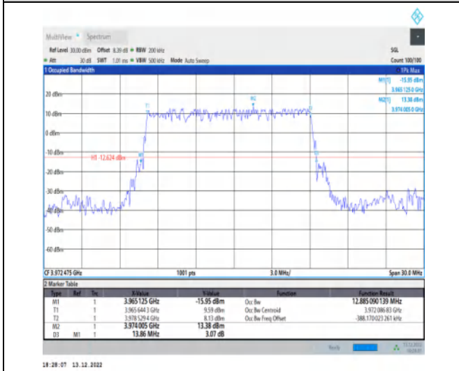
1-N77-3700-3980-30-15-H-2-DFT-PI2BPSK-Outer_Full-36@0-Ant1-12.885-13.860-≤15-PASS
