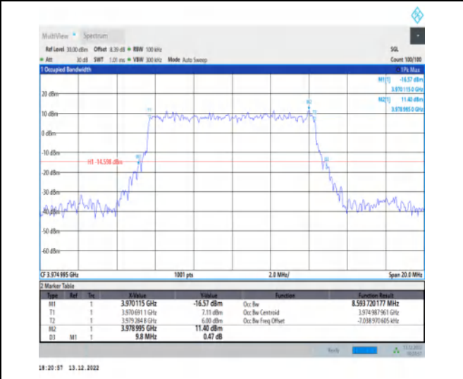
1-N77-3700-3980-30-10-H-2-DFT-PI2BPSK-Outer_F ull-24@0-Ant1-8.594-9.800-≤10-PASS
