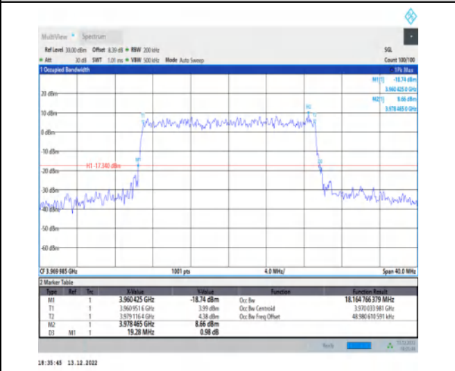
1-N77-3700-3980-30-20-H-8-CP-64QAM-Outer_Full-51@0-Ant1-18.165-19.280-≤20-PASS
