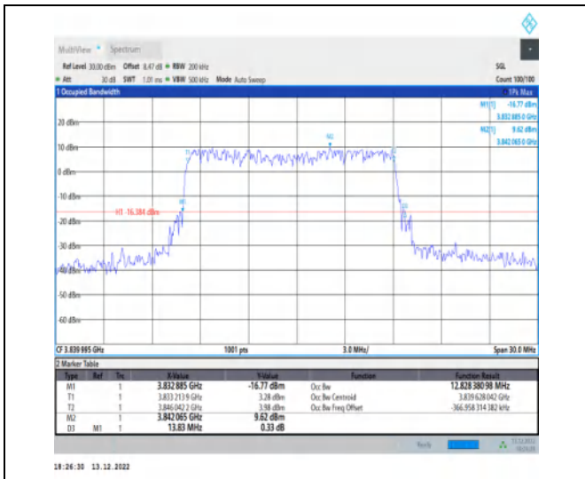
1-N77-3700-3980-30-15-M-5-DFT-256QAM-Outer_Full-36@0-Ant1-12.828-13.830-≤15-PASS
