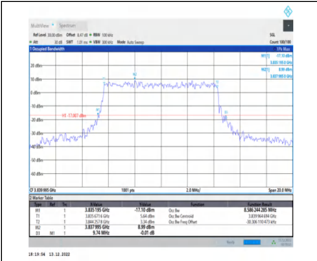
1-N77-3700-3980-30-10-M-8-CP-64QAM-Outer_Full-24@0-Ant1-8.586-9.740-≤10-PASS
