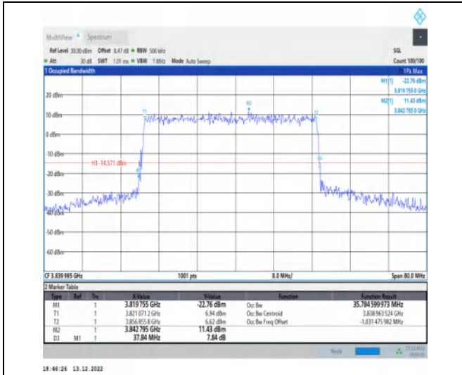
1-N77-3700-3980-30-40-M-4-DFT-64QAM-Outer_Full-100@0-Ant1-35.785-37.840-≤40-PASS
