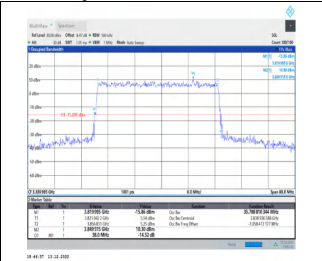
1-N77-3700-3980-30-40-M-5-DFT-256QAM-Outer_Full-100@0-Ant1-35.789-38.000-≤40-PASS
