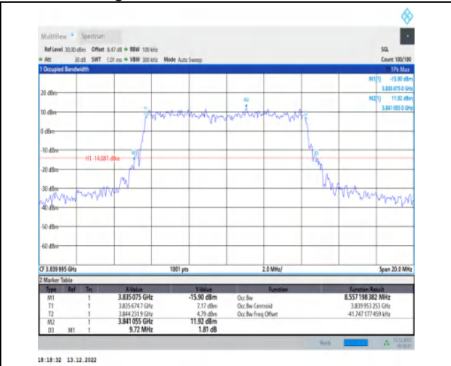
1-N77-3700-3980-30-10-M-1-DFT-QPSK-Outer_Full -24@0-Ant1-8.557-9.720-≤10-PASS
