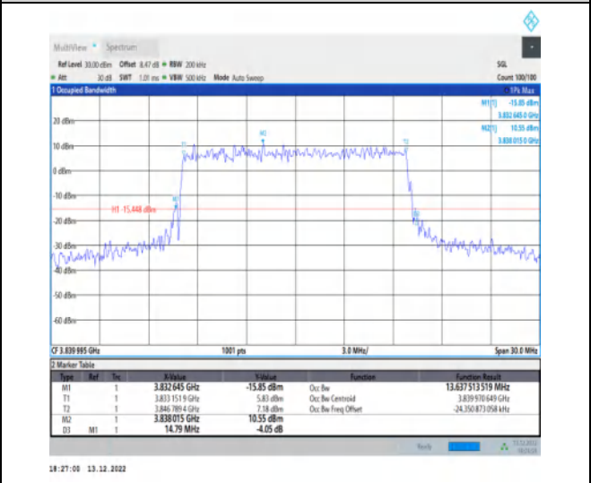
1-N77-3700-3980-30-15-M-8-CP-64QAM-Outer_Full-38@0-Ant1-13.638-14.790-≤15-PASS
