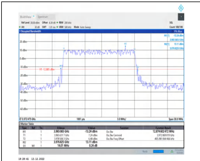
1-N77-3700-3980-30-15-H-4-DFT-64QAM-Outer_Full-36@0-Ant1-12.875-14.010-≤15-PASS
