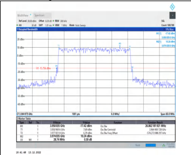
1-N77-3700-3980-30-30-H-3-DFT-16QAM-Outer_Full-75@0-Ant1-26.862-28.740-≤30-PASS
