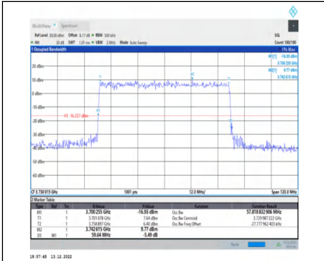
1-N77-3700-3980-30-60-L-3-DFT-16QAM-Outer_Full -162@0-Ant1-57.819-59.640-≤60-PASS
