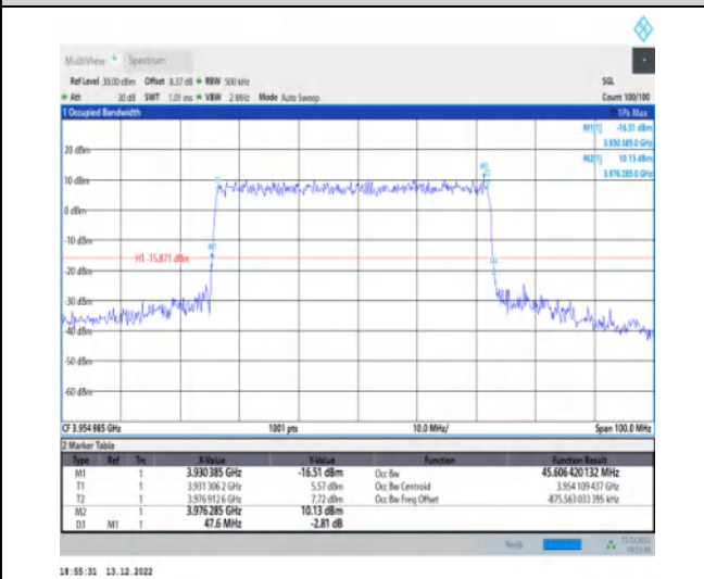
1-N77-3700-3980-30-50-H-3-DFT-16QAM-Outer_Full-128@0-Ant1-45.606-47.600-≤50-PASS
