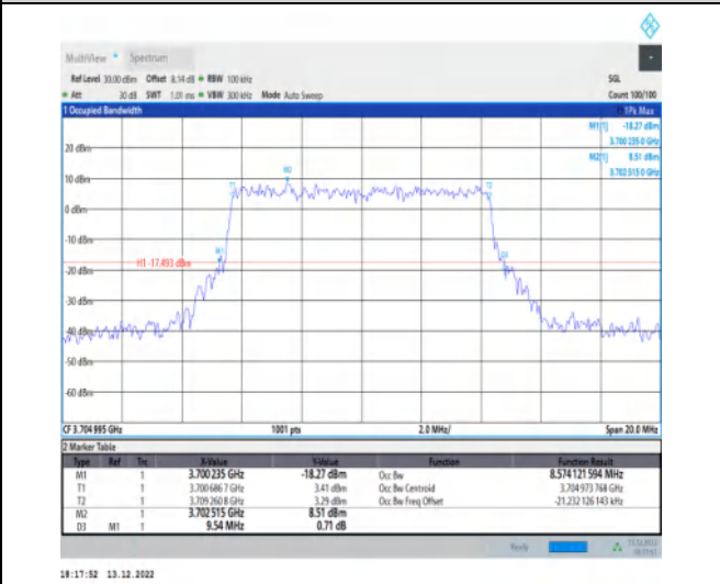
1-N77-3700-3980-30-10-L-8-CP-64QAM-Outer_Full-24@0-Ant1-8.574-9.540-≤10-PASS
