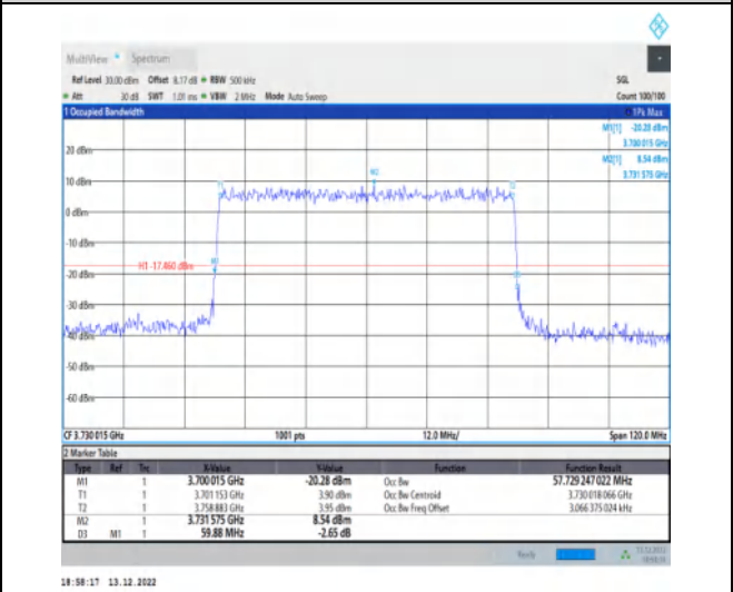
1-N77-3700-3980-30-60-L-6-CP-QPSK-Outer_Full-1 62@0-Ant1-57.729-59.880-≤60-PASS
