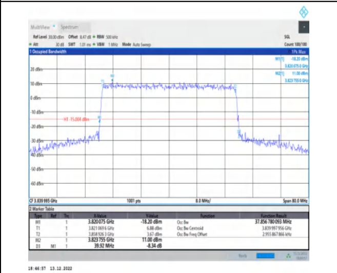
1-N77-3700-3980-30-40-M-7-CP-16QAM-Outer_Full-106@0-Ant1-37.857-39.920-≤40-PASS
