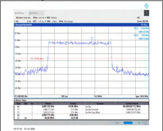
1-N77-3700-3980-30-70-M-4-DFT-64QAM-Outer_Full-180@0-Ant1-64.34-66.640-≤70-PASS
