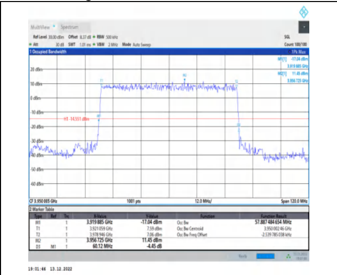
1-N77-3700-3980-30-60-H-2-DFT-PI2BPSK-Outer_Full-162@0-Ant1-57.887-60.120-≤60-PASS
