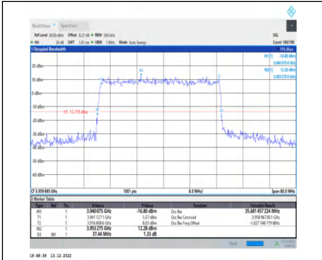
1-N77-3700-3980-30-40-H-3-DFT-16QAM-Outer_Full-100@0-Ant1-35.681-37.440-≤40-PASS
