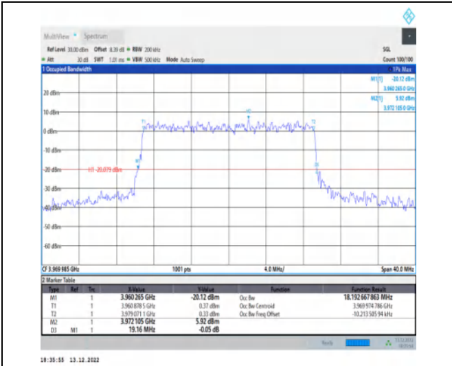
1-N77-3700-3980-30-20-H-9-CP-256QAM-Outer_Ful I-51@0-Ant1-18.193-19.160-<=20-PASS
