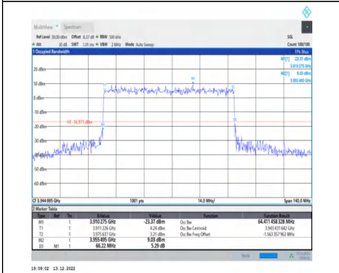
1-N77-3700-3980-30-70-H-4-DFT-64QAM-Outer_Full-180@0-Ant1-64.411-66.220-≤70-PASS
