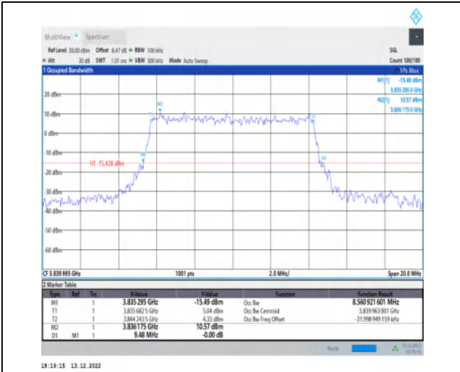
1-N77-3700-3980-30-10-M-4-DFT-64QAM-Outer_Full I-24@0-Ant1-8.561-9.480-≤10-PASS
