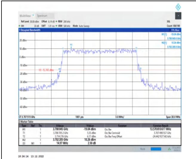
1-N77-3700-3980-30-15-L-6-CP-QPSK-Outer_Full-38@0-Ant1-13.571-14.970-≤15-PASS
