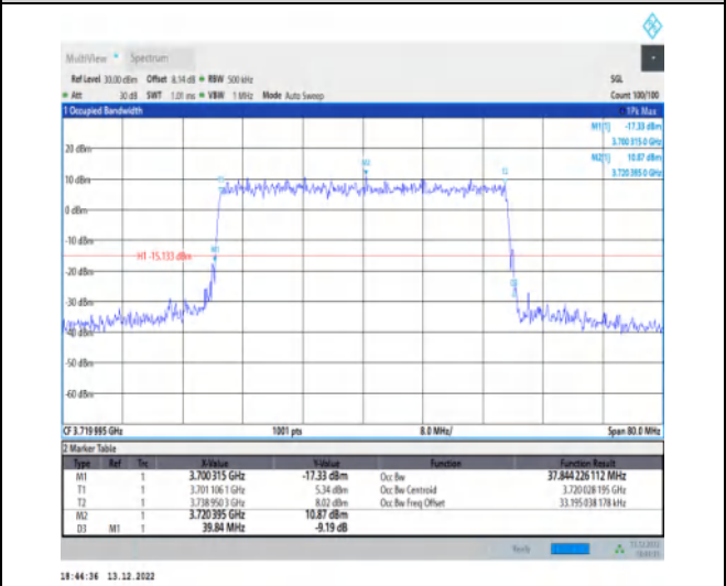
1-N77-3700-3980-30-40-L-8-CP-64QAM-Outer_Full-106@0-Ant1-37.844-39.840-≤40-PASS
