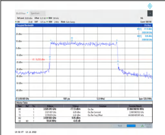
1-N77-3700-3980-30-60-H-3-DFT-16QAM-Outer_Full-162@0-Ant1-57.867-59.640-≤60-PASS
