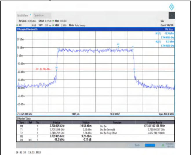
1-N77-3700-3980-30-50-L-7-CP-16QAM-Outer_Full-133@0-Ant1-47.341-49.200-≤50-PASS
