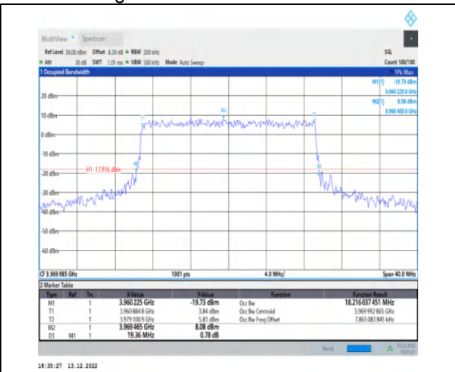
1-N77-3700-3980-30-20-H-6-CP-QPSK-Outer_Full-51@0-Ant1-18.216-19.360-≤20-PASS
