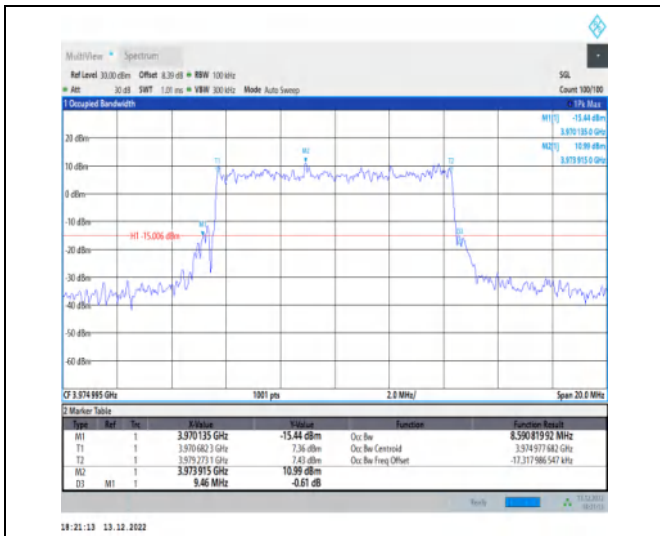
1-N77-3700-3980-30-10-H-3-DFT-16QAM-Outer_Ful I-24@0-Ant1-8.591-9.460-≤10-PASS
