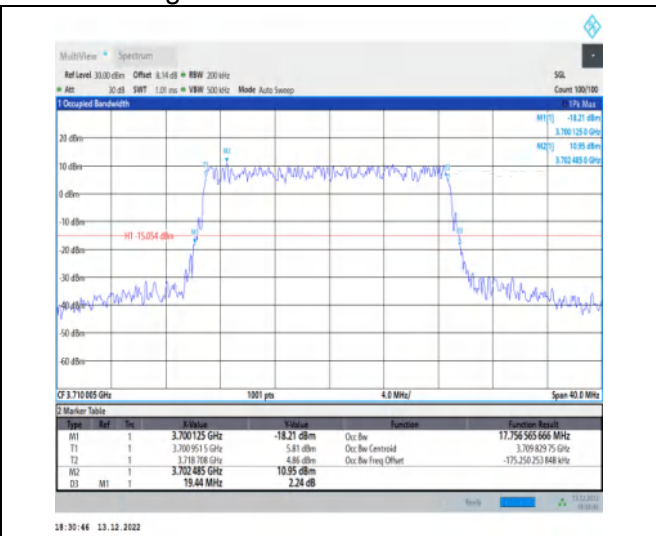
1-N77-3700-3980-30-20-L-4-DFT-64QAM-Outer_Full -50@0-Ant1-17.757-19.440-≤20-PASS
