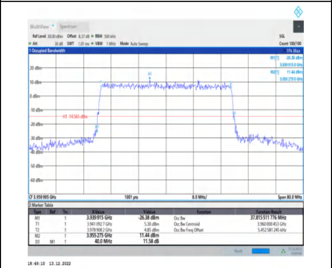
1-N77-3700-3980-30-40-H-6-CP-QPSK-Outer_Full-100@0-Ant1-37.816-40.000-≤40-PASS
