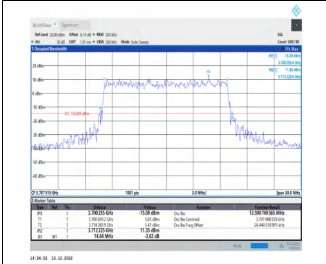
1-N77-3700-3980-30-15-L-8-CP-64QAM-Outer_Full-38@0-Ant1-13.591-14.640-≤15-PASS
