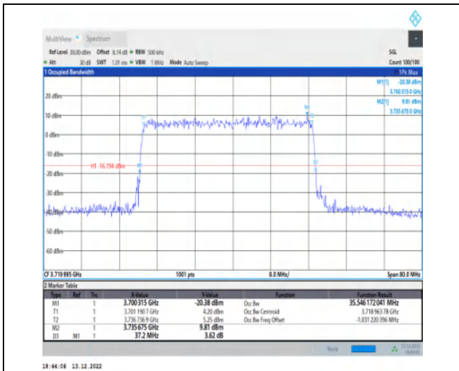
1-N77-3700-3980-30-40-L-5-DFT-256QAM-Outer_Fu II-100@0-Ant1-35.546-37.200-≤40-PASS
