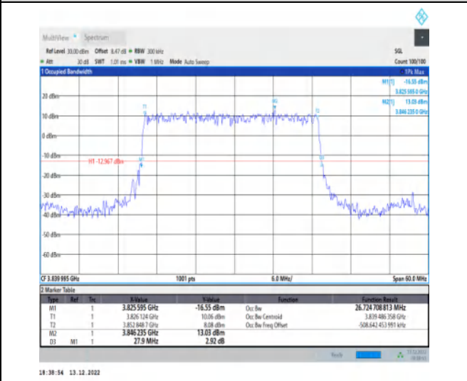
1-N77-3700-3980-30-30-M-2-DFT-Pl2BPSK-Outer_Full-75@0-Ant1-26.725-27.900-≤30-PASS
