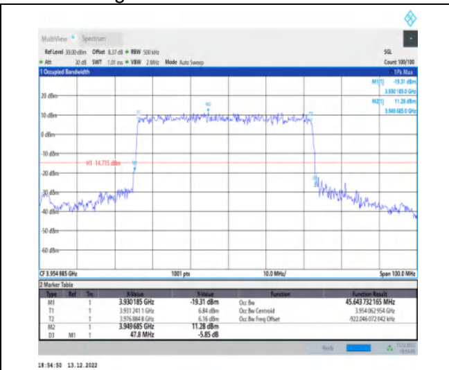
1-N77-3700-3980-30-50-H-1-DFT-QPSK-Outer_Full-128@0-Ant1-45.644-47.800-≤50-PASS
