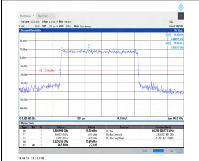
1-N77-3700-3980-30-70-M-1-DFT-QPSK-Outer_Full-180@0-Ant1-64.216-66.500-≤70-PASS
