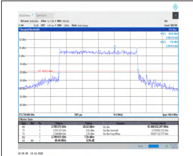
1-N77-3700-3980-30-70-L-8-CP-64QAM-Outer_Full-189@0-Ant1-67.468-69.440-≤70-PASS
