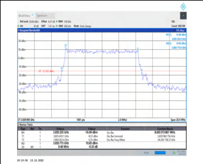
1-N77-3700-3980-30-10-M-3-DFT-16QAM-Outer_Full -24@0-Ant1-8.603-9.480-≤10-PASS
