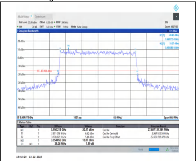
1-N77-3700-3980-30-30-H-7-CP-16QAM-Outer_Full-78@0-Ant1-27.807-29.280-≤30-PASS
