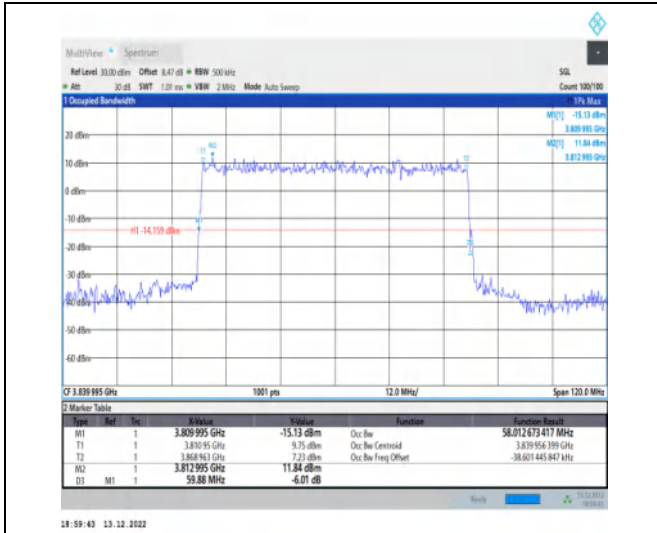
1-N77-3700-3980-30-60-M-2-DFT-PI2BPSK-Outer_Full-162@0-Ant1-58.013-59.880-≤60-PASS
