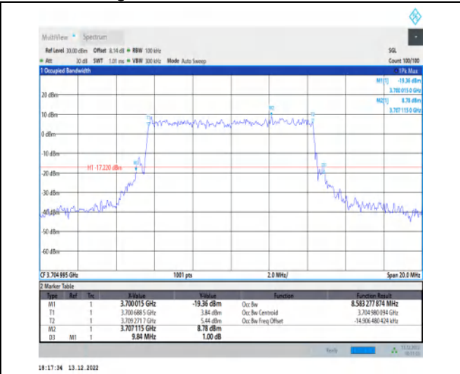
1-N77-3700-3980-30-10-L-6-CP-QPSK-Outer_Full-2 4@0-Ant1-8.583-9.840-≤10-PASS
