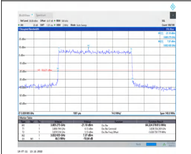
1-N77-3700-3980-30-70-M-5-DFT-256QAM-Outer_Full-180@0-Ant1-64.324-66.500-≤70-PASS
