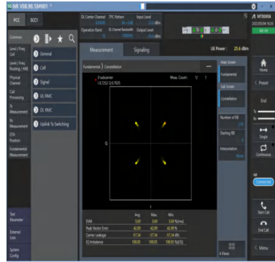
1-N78-3700-3800--30-100-M-2-DFT-QPSK-Outer_Full-270@0-Ant1-see graph-PASS
