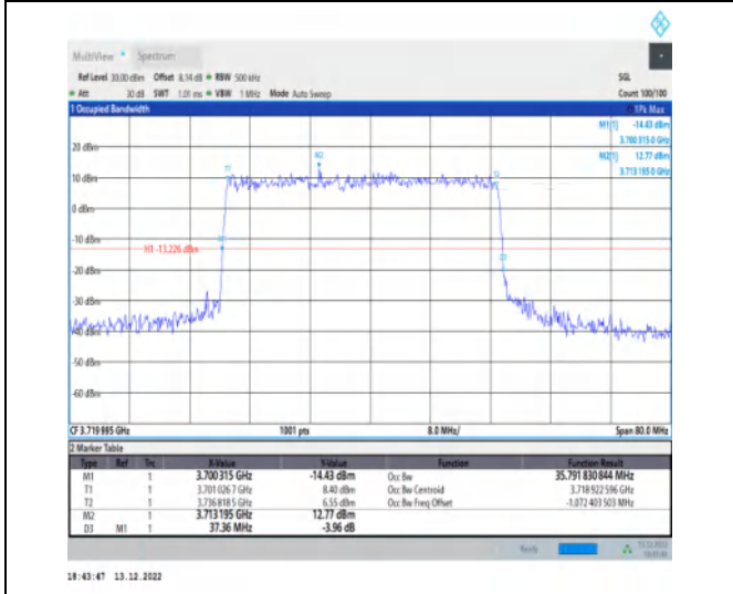
1-N77-3700-3980-30-40-L-3-DFT-16QAM-Outer_Full-100@0-Ant1-35.792-37.360-≤40-PASS
