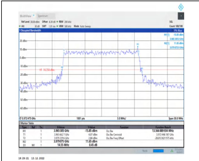
1-N77-3700-3980-30-15-H-8-CP-64QAM-Outer_Full-38@0-Ant1-13.567-14.550-≤15-PASS
