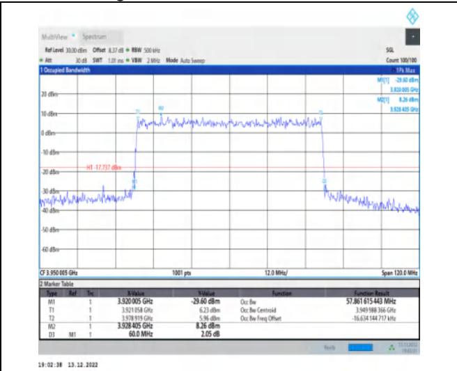
1-N77-3700-3980-30-60-H-6-CP-QPSK-Outer_Full-62@0-Ant1-57.862-60.000-≤60-PASS
