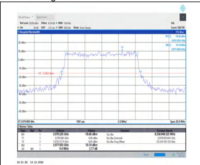
1-N77-3700-3980-30-10-H-4-DFT-64QAM-Outer_Ful I-24@0-Ant1-8.557-9.400-≤10-PASS
