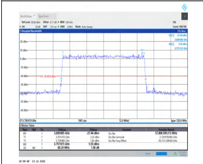
1-N77-3700-3980-30-60-L-9-CP-256QAM-Outer_Full-162@0-Ant1-57.807-60.240-≤60-PASS
