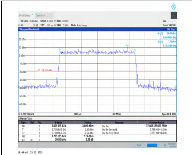
1-N77-3700-3980-30-40-L-9-CP-256QAM-Outer_Full -106@0-Ant1-37.808-39.920-≤40-PASS
