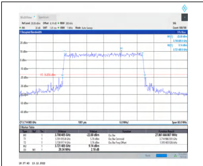
1-N77-3700-3980-30-30-L-8-CP-64QAM-Outer_Full-78@0-Ant1-27.862-29.340-≤30-PASS
