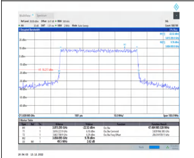
1-N77-3700-3980-30-50-M-7-CP-16QAM-Outer_Full-133@0-Ant1-47.485-49.500-≤50-PASS
