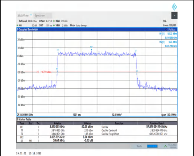
1-N77-3700-3980-30-60-M-9-CP-256QAM-Outer_Full-162@0-Ant1-57.879-59.640-≤60-PASS
