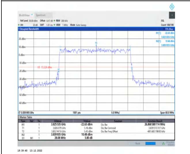
1-N77-3700-3980-30-30-M-5-DFT-256QAM-Outer_Full-75@0-Ant1-26.869-28.080-≤30-PASS
