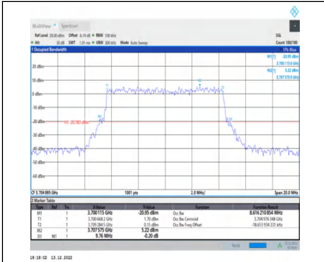
1-N77-3700-3980-30-10-L-9-CP-256QAM-Outer_Full -24@0-Ant1-8.616-9.760-≤10-PASS
