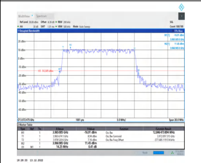
1-N77-3700-3980-30-15-H-3-DFT-16QAM-Outer_Full-36@0-Ant1-12.846-14.250-≤15-PASS
