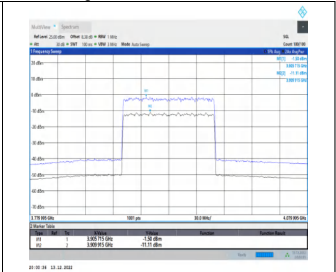
1-N77-3700-3980-30-100-H-2-CP-256QAM-Outer_F ull-273@0-Ant1-9.61-19.56%-7.09-2.52-PASS-≤13
