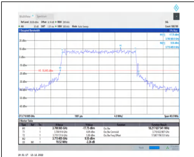
1-N77-3700-3980-30-20-L-7-CP-16QAM-Outer_Full-51@0-Ant1-18.218-19.520-≤20-PASS
