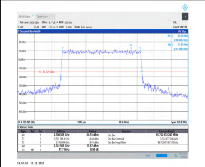
1-N77-3700-3980-30-50-L-1-DFT-QPSK-Outer_Full-128@0-Ant1-45.703-47.700-≤50-PASS
