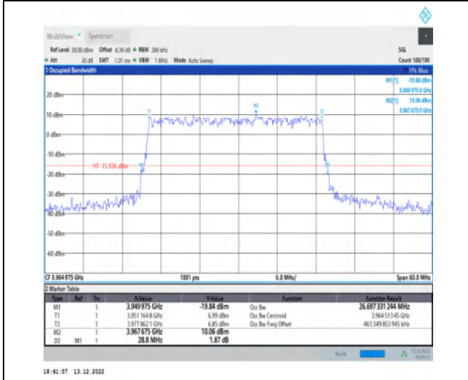
1-N77-3700-3980-30-30-H-4-DFT-64QAM-Outer_Full-75@0-Ant1-26.697-28.800-≤30-PASS
