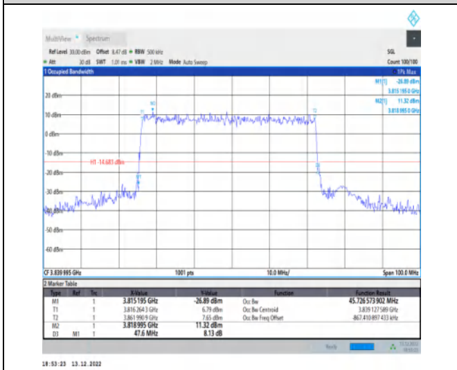
1-N77-3700-3980-30-50-M-3-DFT-16QAM-Outer_Full-128@0-Ant1-45.727-47.600-≤50-PASS
