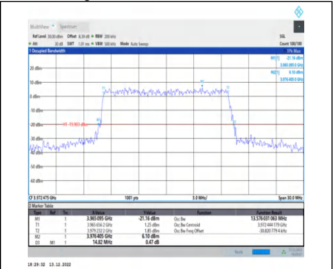
1-N77-3700-3980-30-15-H-9-CP-256QAM-Outer_Full-38@0-Ant1-13.576-14.820-≤15-PASS
