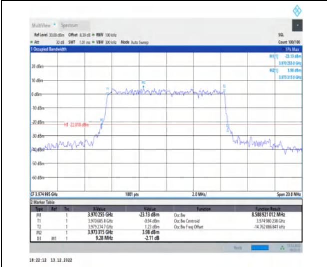
1-N77-3700-3980-30-10-H-9-CP-256QAM-Outer_Ful-I-24@0-Ant1-8.589-9.280-≤10-PASS
