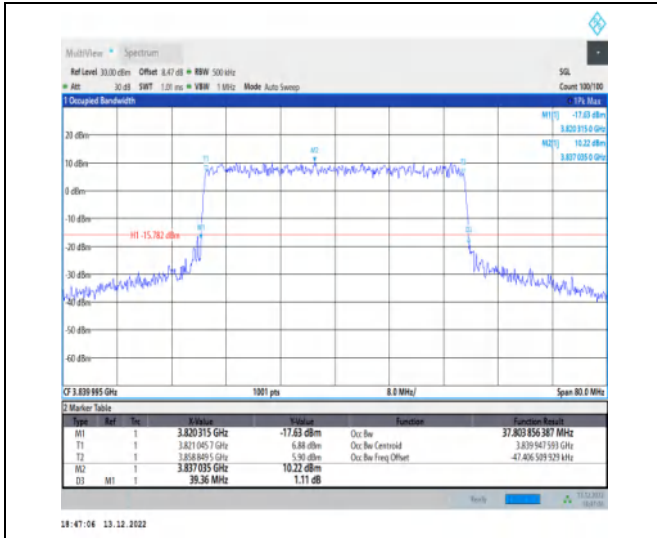
1-N77-3700-3980-30-40-M-8-CP-64QAM-Outer_Full-106@0-Ant1-37.804-39.360-≤40-PASS
