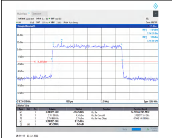
1-N77-3700-3980-30-60-L-5-DFT-256QAM-Outer_Fu ll-162@0-Ant1-57.776-59.520-≤60-PASS
