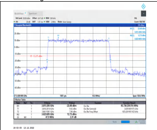
1-N77-3700-3980-30-50-M-2-DFT-PI2BPSK-Outer_Full-128@0-Ant1-45.736-47.900-≤50-PASS
