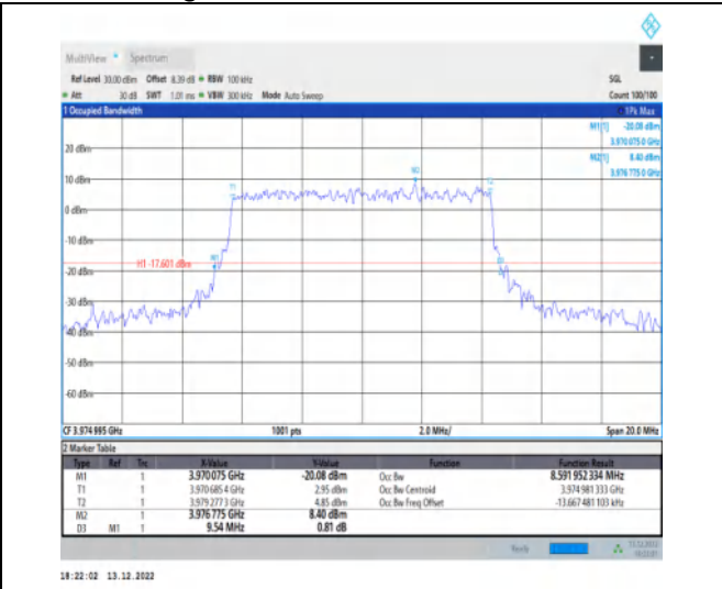
1-N77-3700-3980-30-10-H-8-CP-64QAM-Outer_Full-24@0-Ant1-8.592-9.540-≤10-PASS
