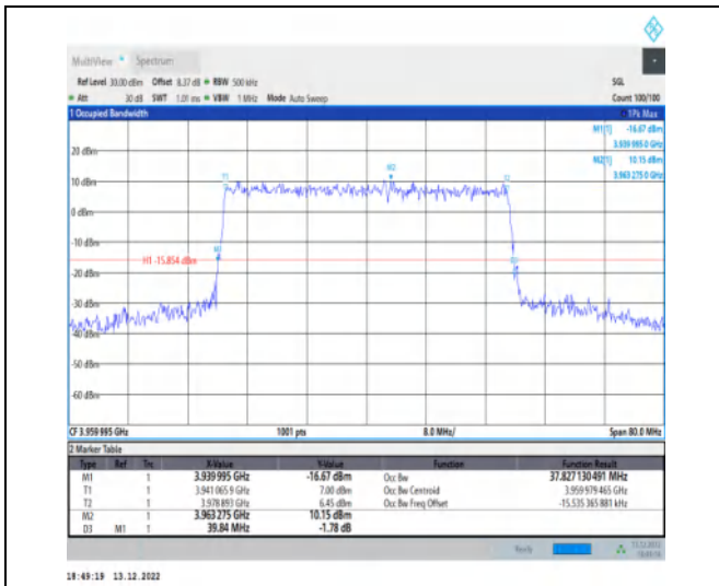
1-N77-3700-3980-30-40-H-7-CP-16QAM-Outer_Full-106@0-Ant1-37.827-39.840-≤40-PASS
