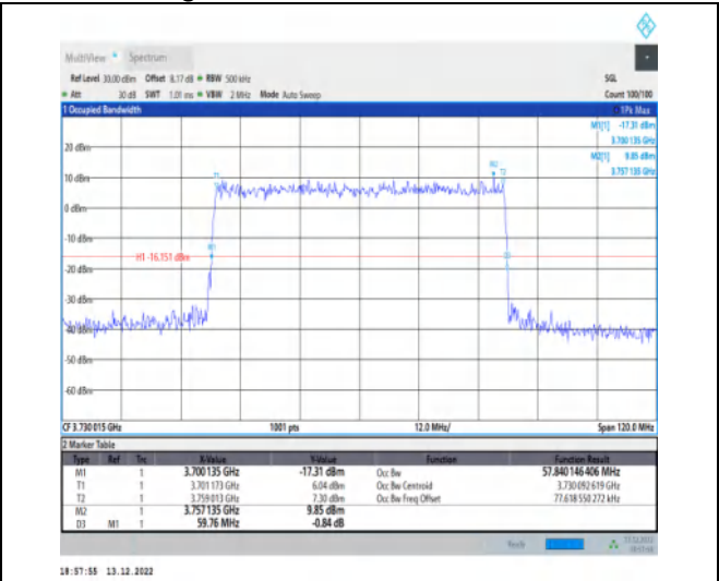
1-N77-3700-3980-30-60-L-4-DFT-64QAM-Outer_Full -162@0-Ant1-57.84-59.760-≤60-PASS
