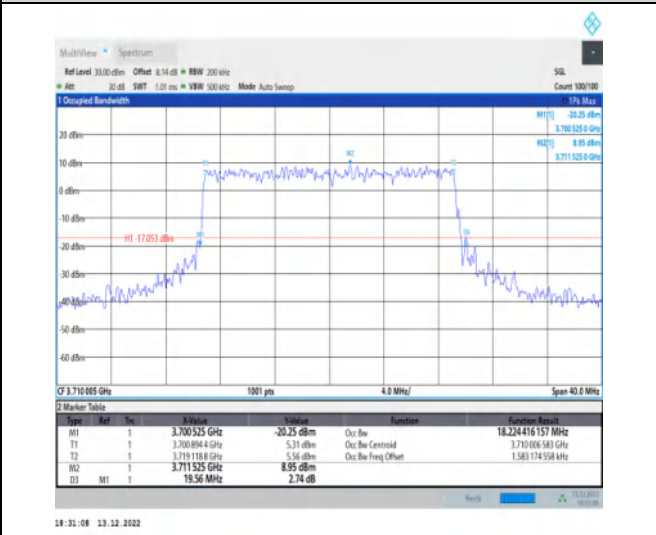
1-N77-3700-3980-30-20-L-6-CP-QPSK-Outer_Full-5 1@0-Ant1-18.224-19.560-≤20-PASS
