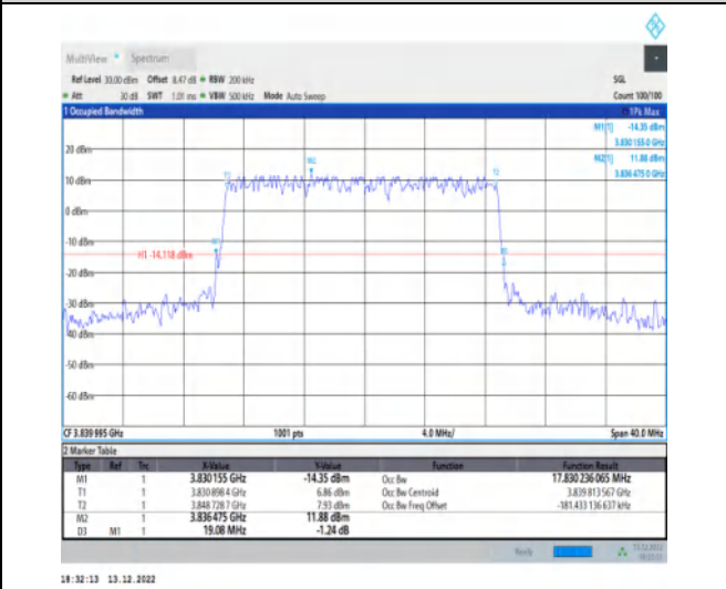
1-N77-3700-3980-30-20-M-1-DFT-QPSK-Outer_Full-50@0-Ant1-17.83-19.080-≤20-PASS
