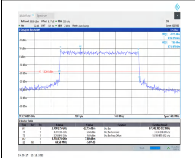
1-N77-3700-3980-30-70-L-6-CP-QPSK-Outer_Full-189@0-Ant1-67.342-69.580-≤70-PASS
