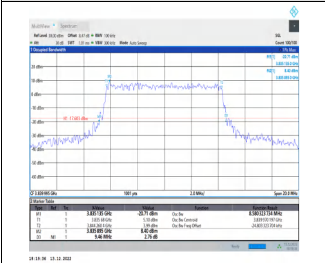
1-N77-3700-3980-30-10-M-6-CP-QPSK-Outer_Full-2 4@0-Ant1-8.58-9.460-≤10-PASS
