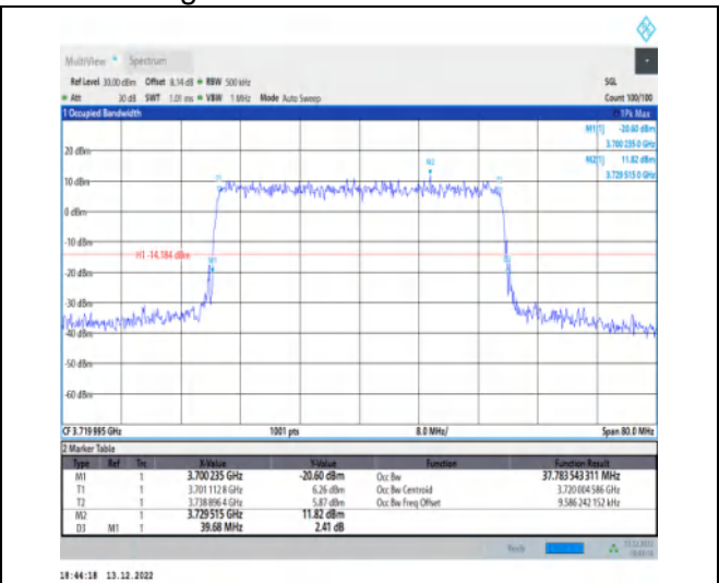
1-N77-3700-3980-30-40-L-6-CP-QPSK-Outer_Full-1 06@0-Ant1-37.784-39.680-≤40-PASS
