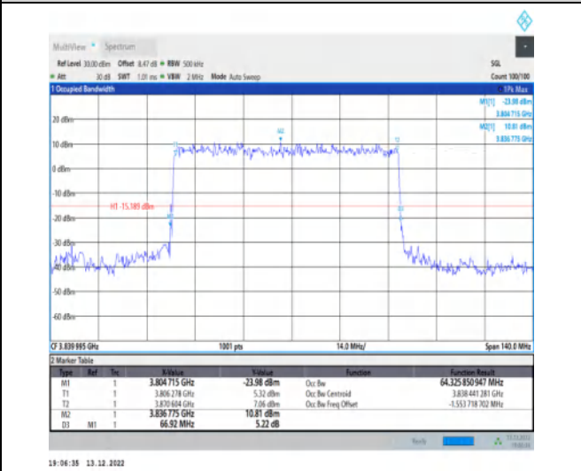
1-N77-3700-3980-30-70-M-2-DFT-Pl2BPSK-Outer_Full-180@0-Ant1-64.326-66.920-≤70-PASS
