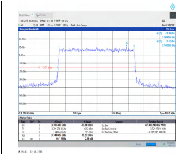
1-N77-3700-3980-30-50-L-6-CP-QPSK-Outer_Full-1 33@0-Ant1-47.39-49.100-≤50-PASS
