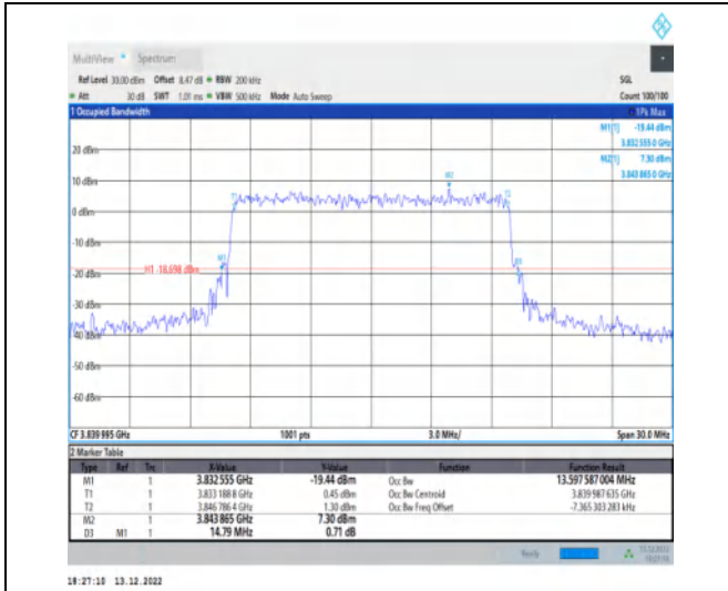
1-N77-3700-3980-30-15-M-9-CP-256QAM-Outer_Ful I-38@0-Ant1-13.598-14.790-≤15-PASS
