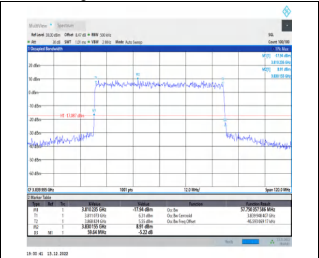
1-N77-3700-3980-30-60-M-7-CP-16QAM-Outer_Full-162@0-Ant1-57.75-59.640-≤60-PASS
