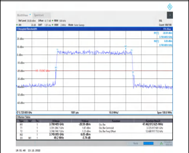
1-N77-3700-3980-30-50-L-9-CP-256QAM-Outer_Full-133@0-Ant1-47.462-49.200-≤50-PASS
