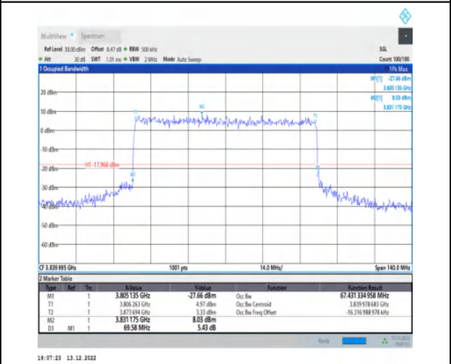
1-N77-3700-3980-30-70-M-6-CP-QPSK-Outer_Full-189@0-Ant1-67.431-69.580-≤70-PASS
