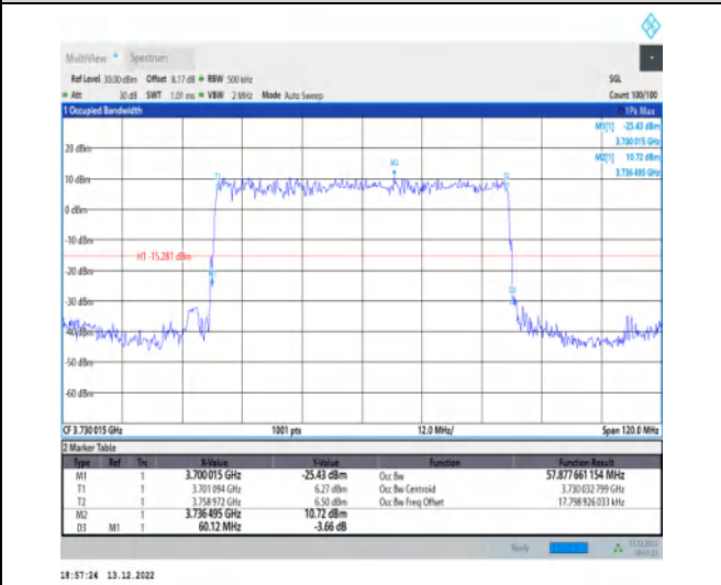
1-N77-3700-3980-30-60-L-2-DFT-PI2BPSK-Outer_Full-162@0-Ant1-57.878-60.120-≤60-PASS
