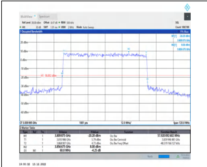
1-N77-3700-3980-30-60-M-6-CP-QPSK-Outer_Full-162@0-Ant1-57.92-60.000-≤60-PASS
