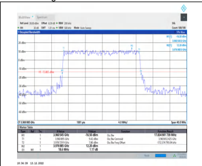
1-N77-3700-3980-30-20-H-2-DFT-PI2BPSK-Outer_Full-50@0-Ant1-17.835-18.600-≤20-PASS
