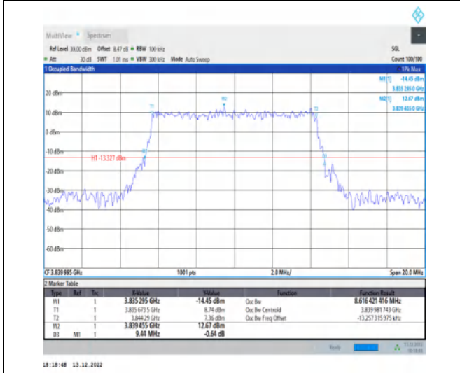
1-N77-3700-3980-30-10-M-2-DFT-PI2BPSK-Outer_Full -24@0-Ant1-8.616-9.440-≤10-PASS
