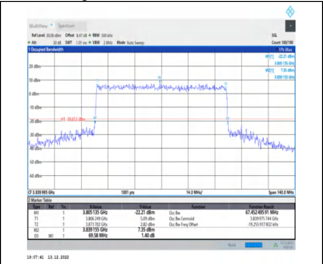
1-N77-3700-3980-30-70-M-8-CP-64QAM-Outer_Full-189@0-Ant1-67.452-69.580-≤70-PASS
