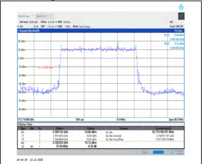
1-N77-3700-3980-30-40-L-2-DFT-PI2BPSK-Outer_Full-100@0-Ant1-35.774-37.440-≤40-PASS
