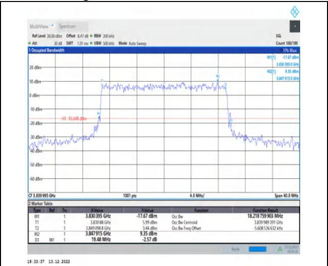
1-N77-3700-3980-30-20-M-7-CP-16QAM-Outer_Full -51@0-Ant1-18.219-19.480-≤20-PASS
