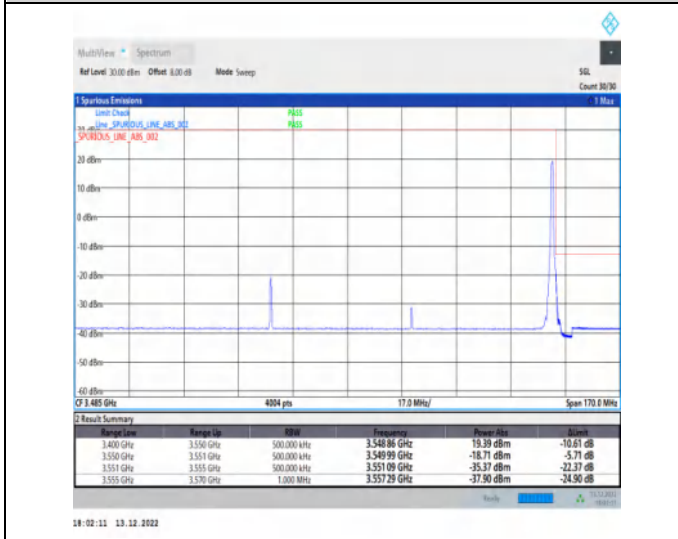
1-N77-3450-3550-30-90-H-5-CP-QPSK-Edge_1RB_Right-1@244-Ant1-1--PASS-see graph
