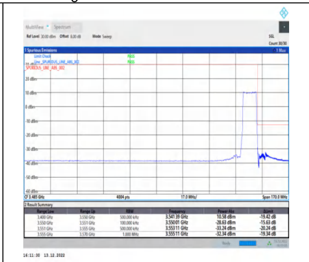
1-N77-3450-3550-30-10-H-3-DFT-PI2BPSK-Outer_Full-24@0-Ant1-1--PASS-see graph
