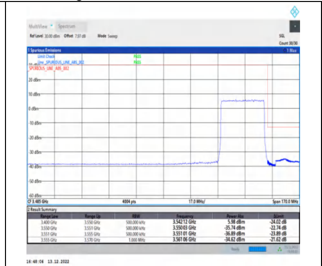
1-N77-3450-3550-30-30-H-3-DFT-PI2BPSK-Outer_Full-75@0-Ant1-1--PASS-see graph
