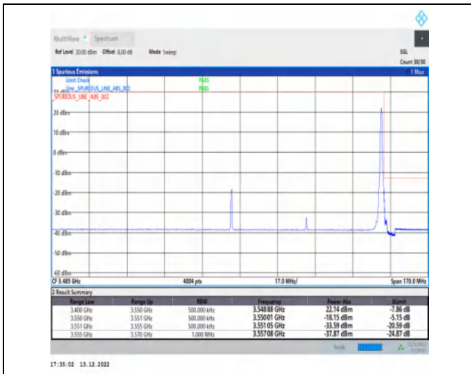
1-N77-3450-3550-30-70-H-2-DFT-PI2BPSK-Edge_1R_B_Right-1@188-Ant1-1--PASS-see graph
