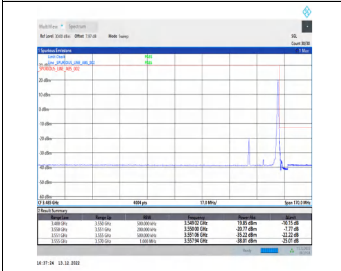
1-N77-3450-3550-30-20-H-5-CP-QPSK-Edge_1RB_Right-1@50-Ant1-1--PASS-see graph
