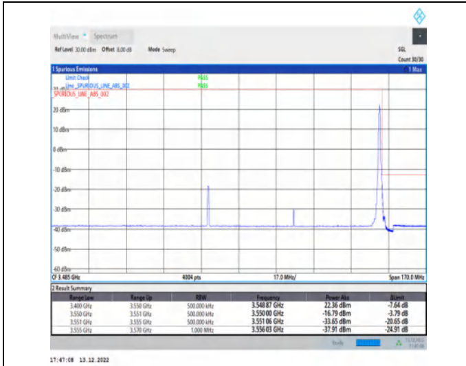
1-N77-3450-3550-30-80-H-2-DFT-PI2BPSK-Edge_1R_B_Right-1@216-Ant1-1--PASS-see graph
