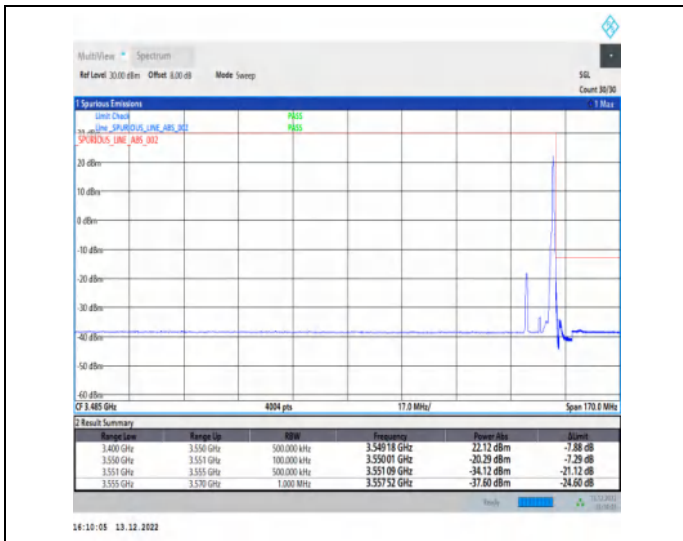
1-N77-3450-3550-30-10-H-2-DFT-PI2BPSK-Edge_1R_B_Right-1@23-Ant1-1--PASS-see graph
