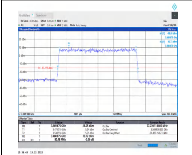
1-N77-3450-3550-30-80-H-5-DFT-256QAM-Outer_Full I-216@0-Ant1-77.239-80.480-≤80-PASS
