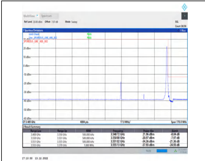
1-N77-3450-3550-30-50-H-2-DFT-PI2BPSK-Edge_1R_B_Right-1@132-Ant1-1--PASS-see graph
