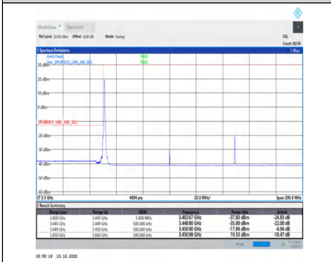
1-N77-3450-3550-30-100-L-4-CP-QPSK-Edge_1RB_Left-1@0-Ant1-1--PASS-see graph
