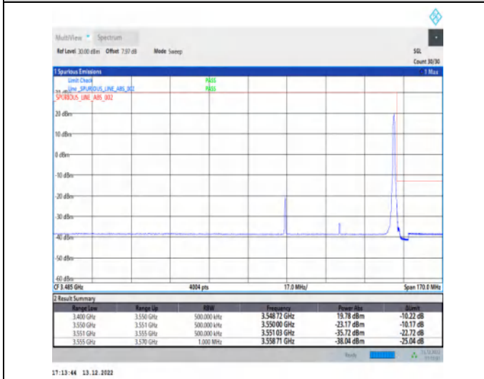
1-N77-3450-3550-30-50-H-5-CP-QPSK-Edge_1RB_Right-1@132-Ant1-1--PASS-see graph
