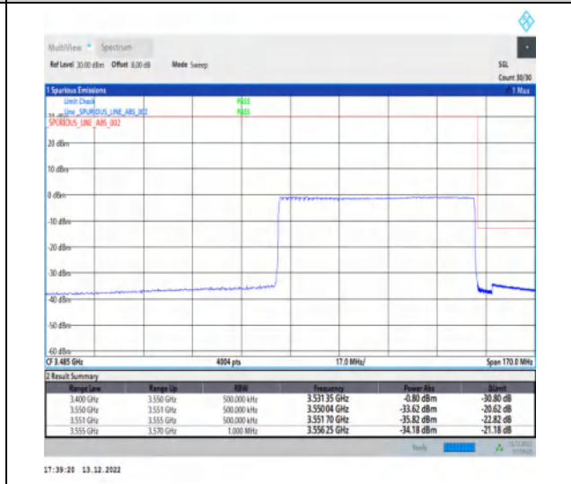
1-N77-3450-3550-30-70-H-6-CP-QPSK-Outer_Full-189@0-Ant1-1--PASS-see graph
