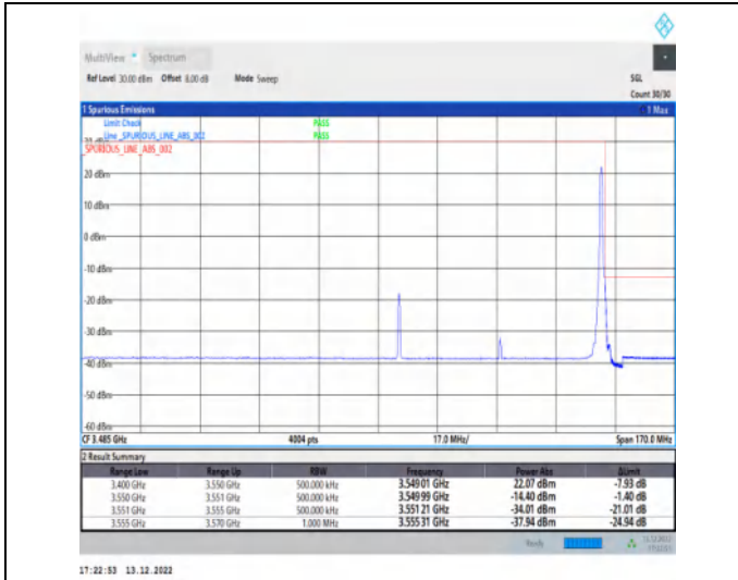
1-N77-3450-3550-30-60-H-2-DFT-PI2BPSK-Edge_1R_B_Right-1@161-Ant1-1--PASS-see graph
