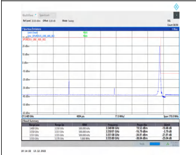
1-N77-3450-3550-30-100-H-5-CP-QPSK-Edge_1RB_Right-1@272-Ant1-1--PASS-see graph
