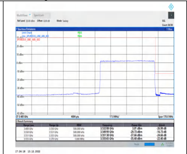
1-N77-3450-3550-30-60-H-3-DFT-PI2BPSK-Outer_Full-162@0-Ant1-1--PASS-see graph
