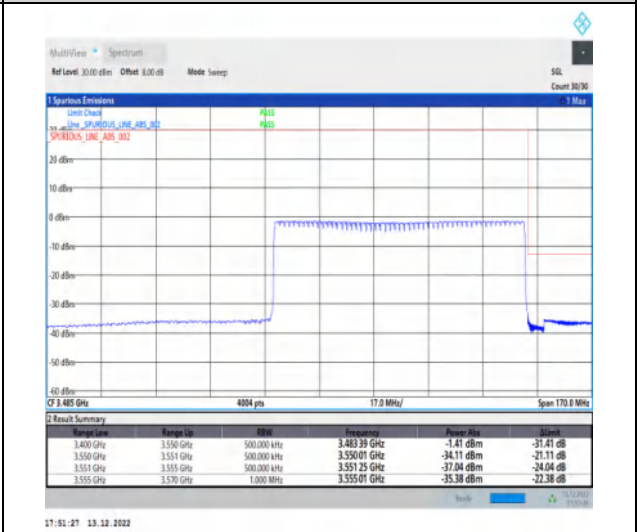
1-N77-3450-3550-30-80-H-6-CP-QPSK-Outer_Full-217@0-Ant1-1--PASS-see graph
