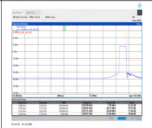
1-N77-3450-3550-30-10-H-6-CP-QPSK-Outer_Full-24@0-Ant1-1--PASS-see graph
