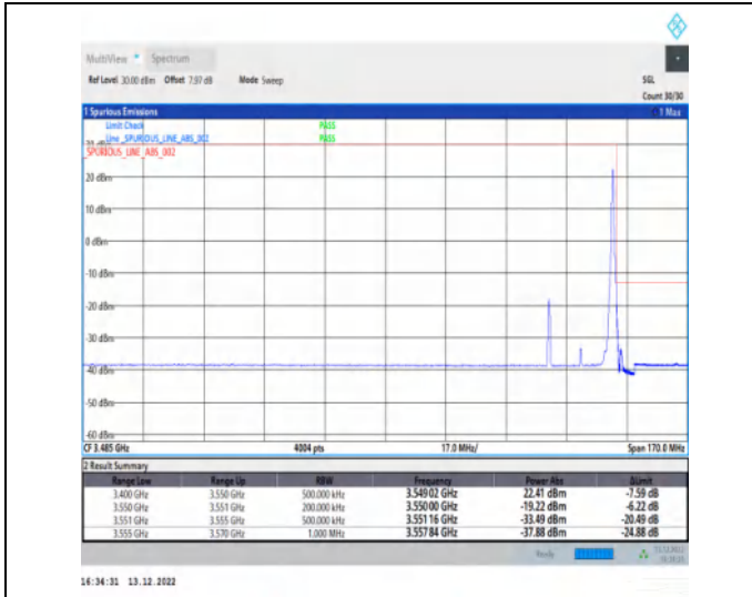
1-N77-3450-3550-30-20-H-2-DFT-PI2BPSK-Edge_1R_B_Right-1@50-Ant1-1--PASS-see graph
