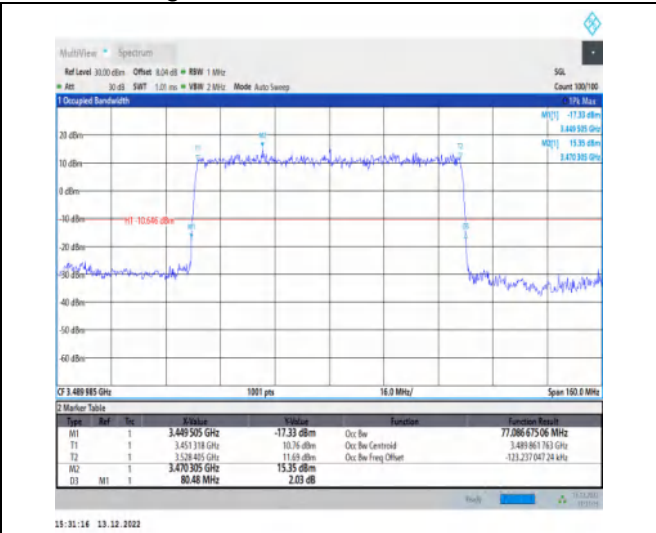
1-N77-3450-3550-30-80-L-2-DFT-PI2BPSK-Outer_Full-216@0-Ant1-77.087-80.480-≤80-PASS
