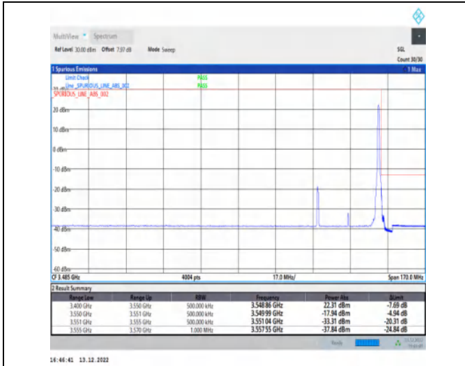
1-N77-3450-3550-30-30-H-2-DFT-PI2BPSK-Edge_1R_B_Right-1@77-Ant1-1--PASS-see graph
