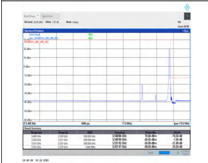
1-N77-3450-3550-30-30-H-5-CP-QPSK-Edge_1RB_Right-1@77-Ant1-1--PASS-see graph
