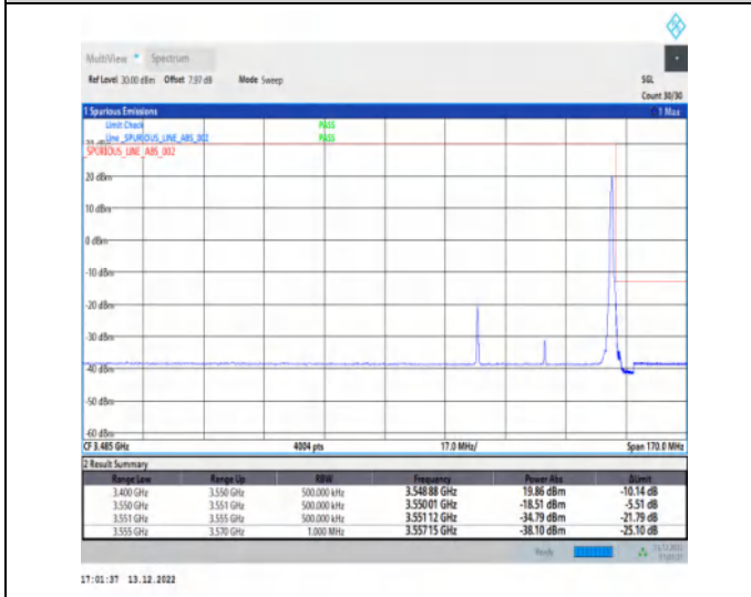
1-N77-3450-3550-30-40-H-5-CP-QPSK-Edge_1RB_Right-1@105-Ant1-1--PASS-see graph
