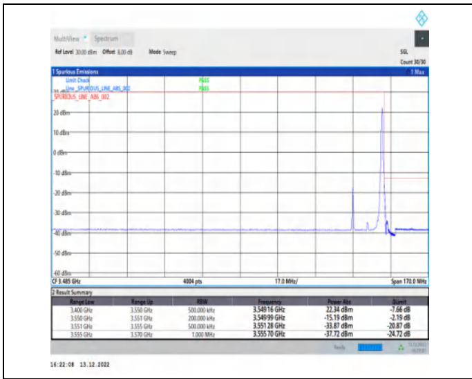
1-N77-3450-3550-30-15-H-2-DFT-PI2BPSK-Edge_1R_B_Right-1@37-Ant1-1--PASS-see graph
