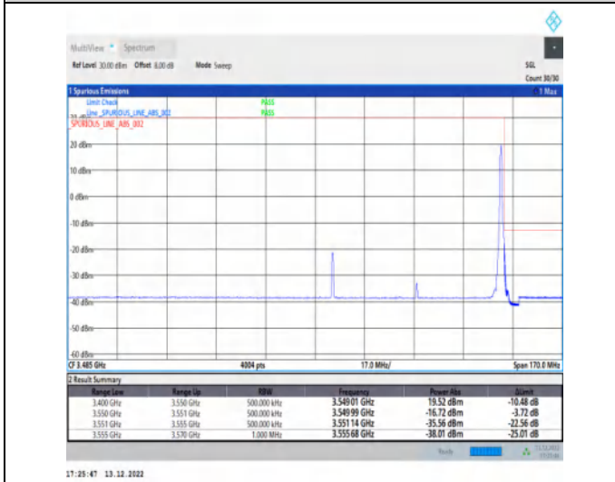
1-N77-3450-3550-30-60-H-5-CP-QPSK-Edge_1RB_Right-1@161-Ant1-1--PASS-see graph
