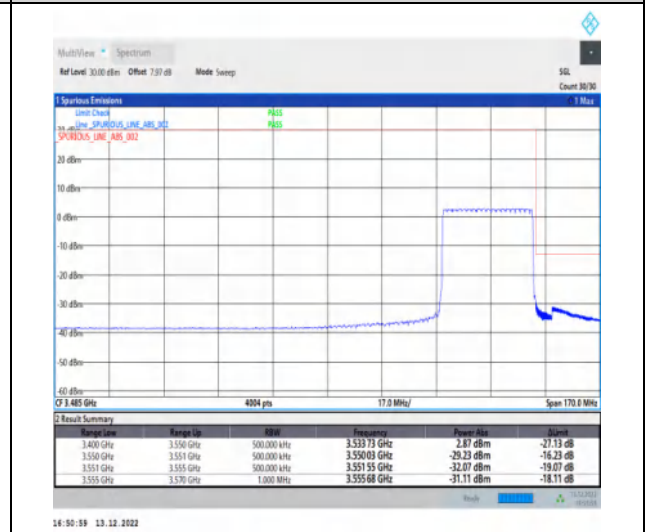
1-N77-3450-3550-30-30-H-6-CP-QPSK-Outer_Full-78@0-Ant1-1--PASS-see graph
