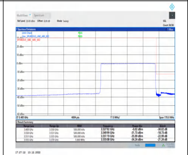
1-N77-3450-3550-30-60-H-6-CP-QPSK-Outer_Full-162@0-Ant1-1--PASS-see graph
