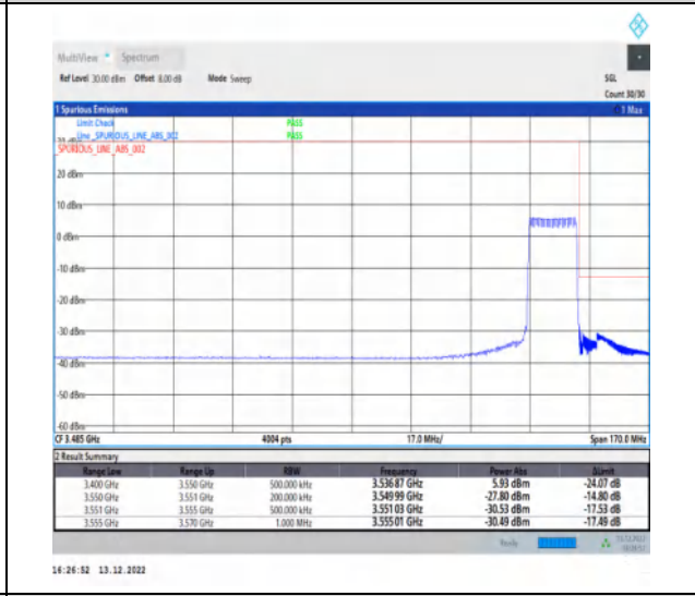
1-N77-3450-3550-30-15-H-6-CP-QPSK-Outer_Full-38@0-Ant1-1--PASS-see graph
