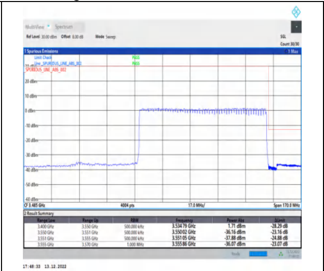
1-N77-3450-3550-30-80-H-3-DFT-PI2BPSK-Outer_Full-216@0-Ant1-1--PASS-see graph
