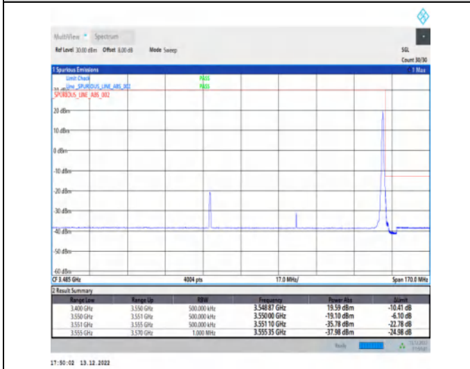
1-N77-3450-3550-30-80-H-5-CP-QPSK-Edge_1RB_Right-1@216-Ant1-1--PASS-see graph
