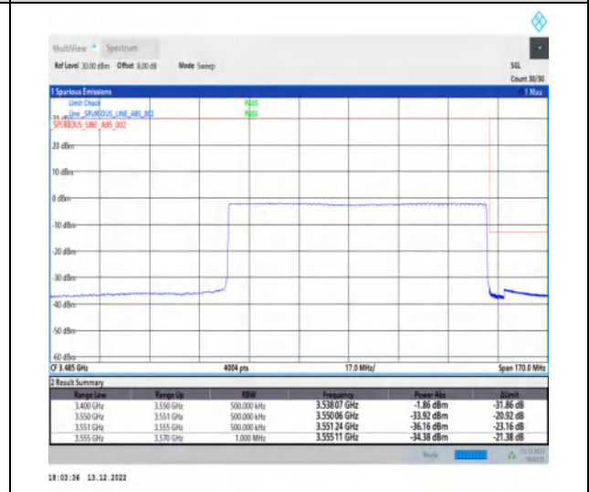
1-N77-3450-3550-30-90-H-6-CP-QPSK-Outer_Full-245@0-Ant1-1--PASS-see graph
