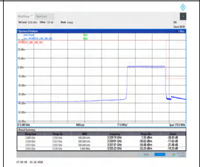
1-N77-3450-3550-30-40-H-6-CP-QPSK-Outer_Full-106@0-Ant1-1--PASS-see graph
