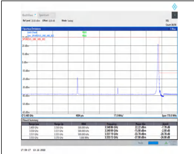
1-N77-3450-3550-30-90-H-2-DFT-PI2BPSK-Edge_1R_B_Right-1@244-Ant1-1--PASS-see graph
