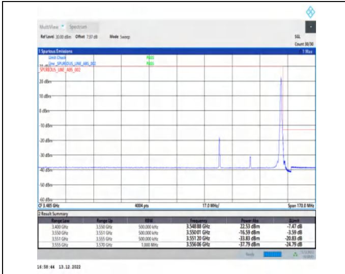
1-N77-3450-3550-30-40-H-2-DFT-PI2BPSK-Edge_1R_B_Right-1@105-Ant1-1--PASS-see graph
