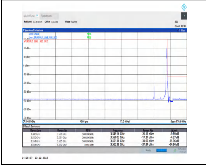
1-N77-3450-3550-30-15-H-5-CP-QPSK-Edge_1RB_Right-1@37-Ant1-1--PASS-see graph
