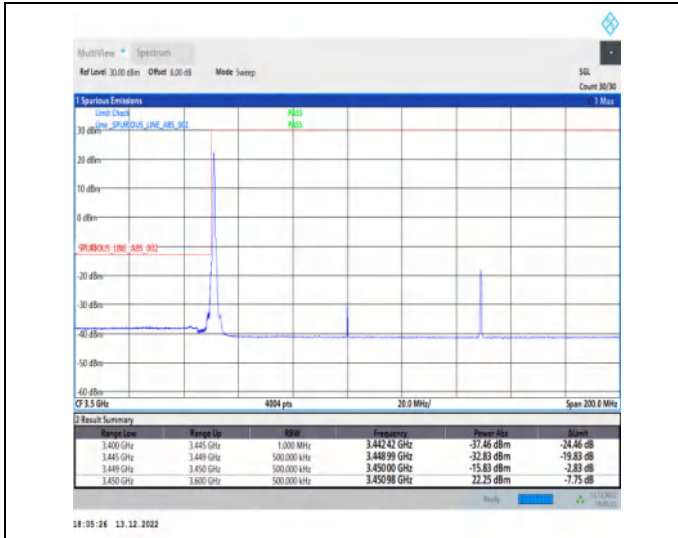
1-N77-3450-3550-30-100-L-1-DFT-PI2BPSK-Edge_1R_B_Left-1@0-Ant1-1--PASS-see graph
