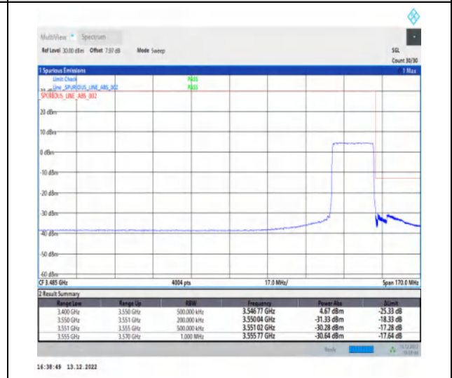
1-N77-3450-3550-30-20-H-6-CP-QPSK-Outer_Full-51@0-Ant1-1--PASS-see graph
