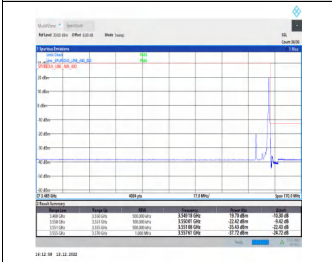
1-N77-3450-3550-30-10-H-5-CP-QPSK-Edge_1RB_Right-1@23-Ant1-1--PASS-see graph
