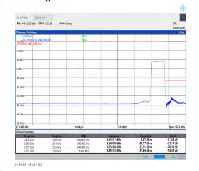
1-N77-3450-3550-30-15-H-3-DFT-PI2BPSK-Outer_Full-36@0-Ant1-1--PASS-see graph
