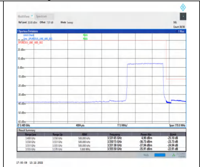
1-N77-3450-3550-30-40-H-3-DFT-PI2BPSK-Outer_Full-100@0-Ant1-1--PASS-see graph
