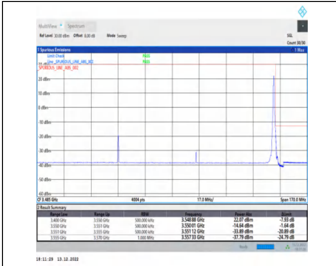
1-N77-3450-3550-30-100-H-2-DFT-PI2BPSK-Edge_1R_B_Right-1@272-Ant1-1--PASS-see graph
