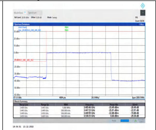
1-N77-3450-3550-30-100-L-3-DFT-PI2BPSK-Outer_Full-270@0-Ant1-1--PASS-see graph
