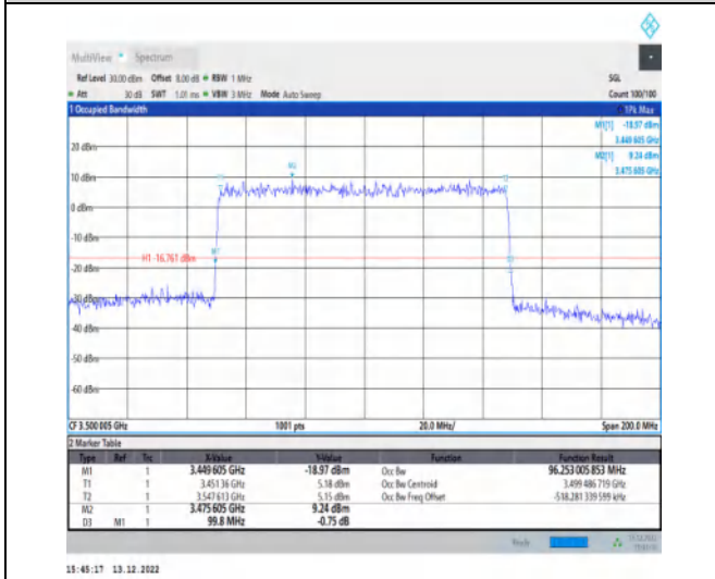
1-N77-3450-3550-30-100-L-5-DFT-256QAM-Outer_F ull-270@0-Ant1-96.253-99.800-≤100-PASS
