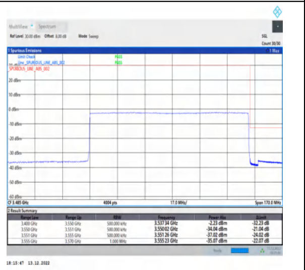
1-N77-3450-3550-30-100-H-6-CP-QPSK-Outer_Full-273@0-Ant1-1--PASS-see graph
