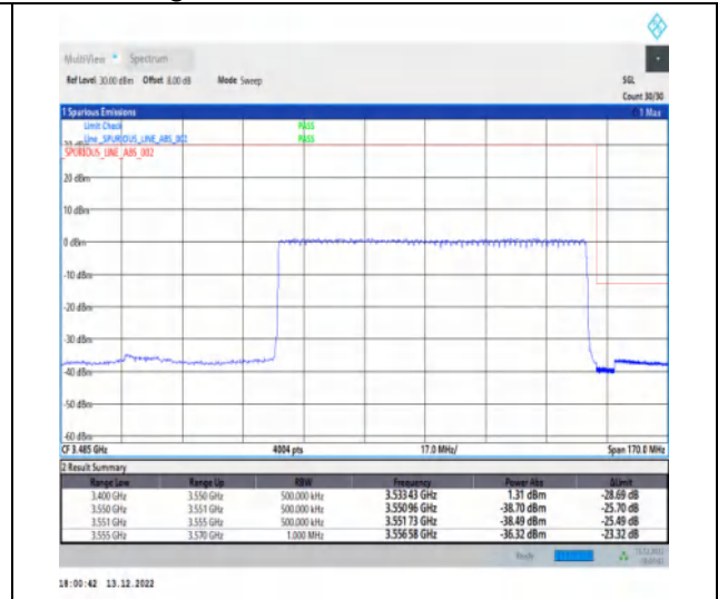
1-N77-3450-3550-30-90-H-3-DFT-PI2BPSK-Outer_Full-240@0-Ant1-1--PASS-see graph
