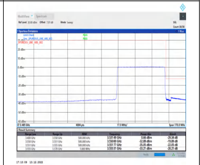
1-N77-3450-3550-30-50-H-6-CP-QPSK-Outer_Full-133@0-Ant1-1--PASS-see graph
