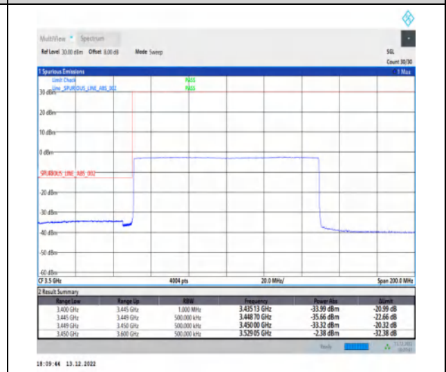
1-N77-3450-3550-30-100-L-6-CP-QPSK-Outer_Full-273@0-Ant1-1--PASS-see graph
