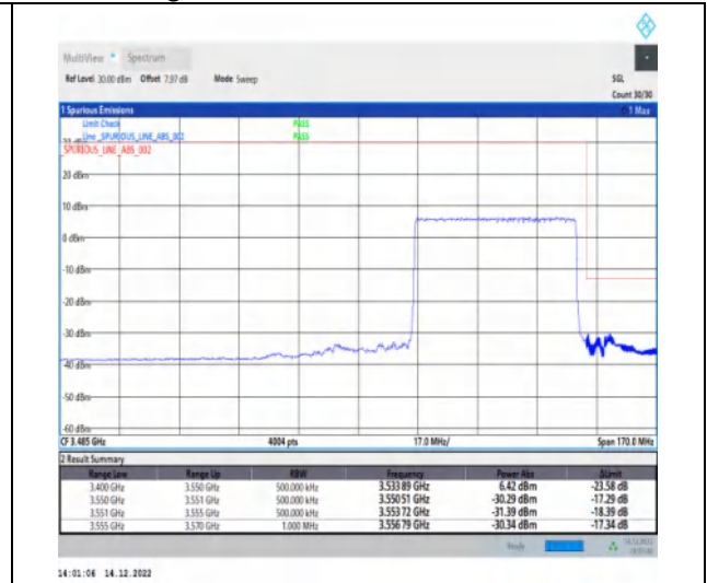
1-N77-3450-3550-30-50-H-3-DFT-PI2BPSK-Outer_Full-128@0-Ant1-1--PASS-see graph
