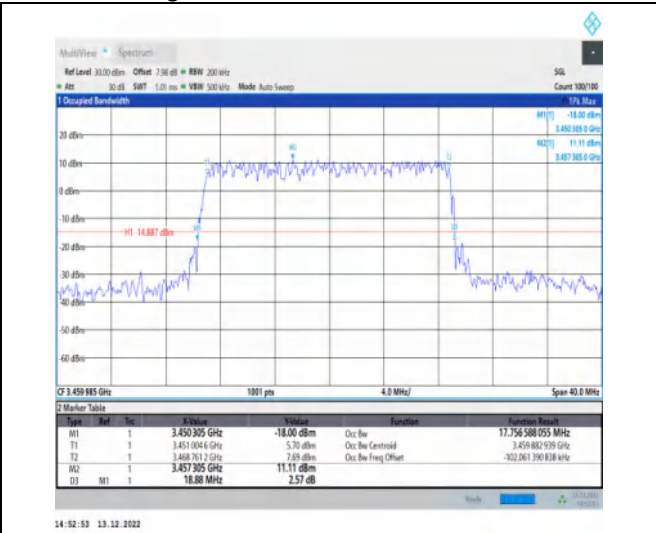
1-N77-3450-3550-30-20-L-4-DFT-64QAM-Outer_Full -50@0-Ant1-17.757-18.880-<=20-PASS
