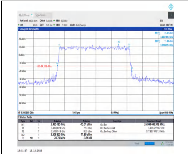
1-N77-3450-3550-30-30-M-3-DFT-16QAM-Outer_Ful I-75@0-Ant1-26.849-28.740-≤30-PASS
