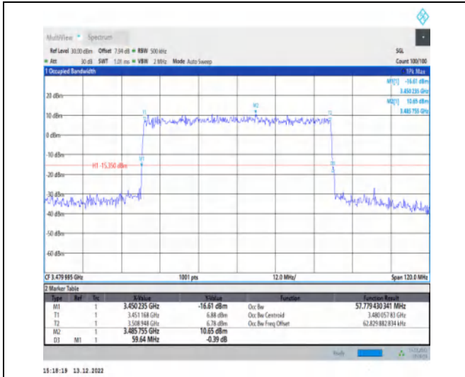
1-N77-3450-3550-30-60-L-3-DFT-16QAM-Outer_Full -162@0-Ant1-57.779-59.640-≤60-PASS
