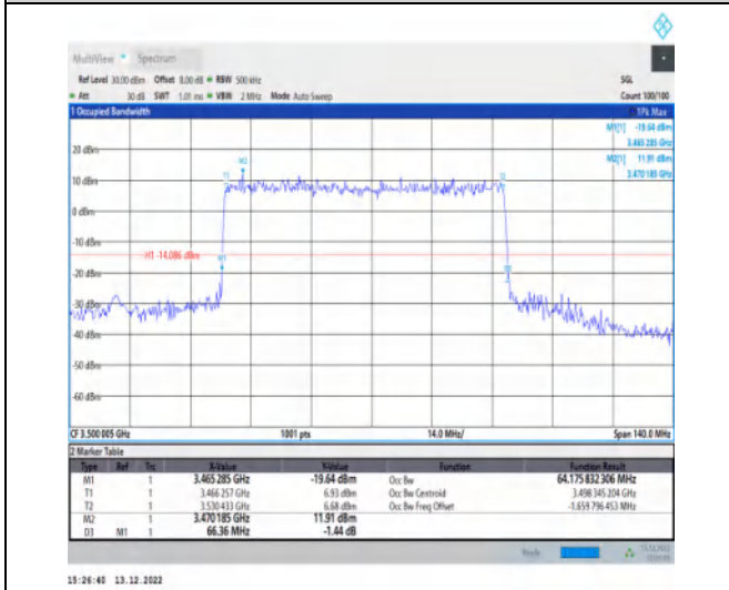
1-N77-3450-3550-30-70-M-1-DFT-QPSK-Outer_Full-180@0-Ant1-64.176-66.360-≤70-PASS
