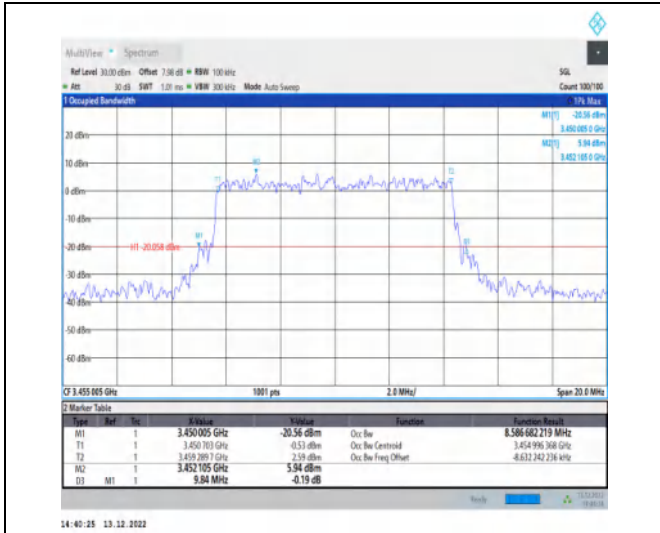
1-N77-3450-3550-30-10-L-9-CP-256QAM-Outer_Full -24@0-Ant1-8.587-9.840-≤10-PASS
