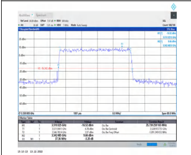
1-N77-3450-3550-30-40-H-5-DFT-256QAM-Outer_Full-100@0-Ant1-35.739-37.360-≤40-PASS
