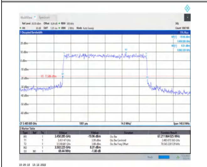
1-N77-3450-3550-30-70-L-6-CP-QPSK-Outer_Full-1 89@0-Ant1-67.212-69.440-≤70-PASS
