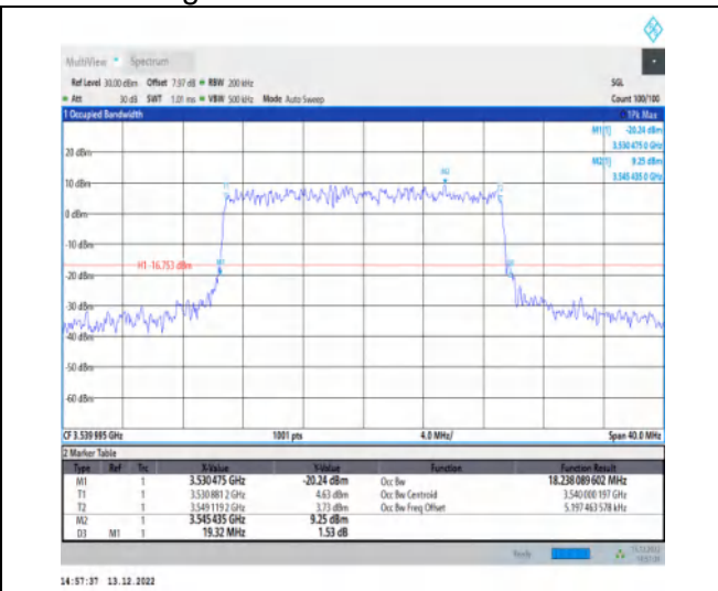
1-N77-3450-3550-30-20-H-6-CP-QPSK-Outer-Full-51@0-Ant1-18.238-19.320-≤20-PASS
