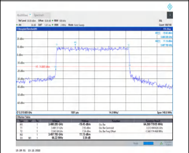
1-N77-3450-3550-30-70-H-1-DFT-QPSK-Outer_Full-180@0-Ant1-64.27-66.220-≤70-PASS
