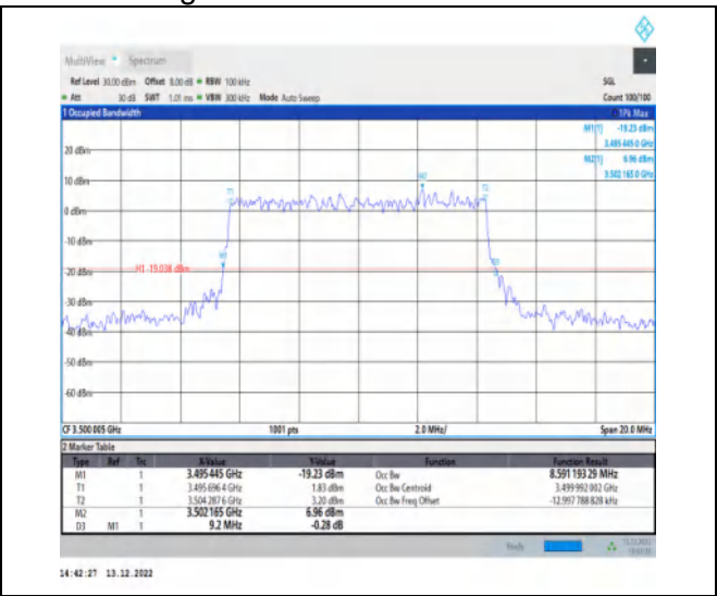
1-N77-3450-3550-30-10-M-9-CP-256QAM-Outer_Fu II-24@0-Ant1-8.591-9.200-≤10-PASS
