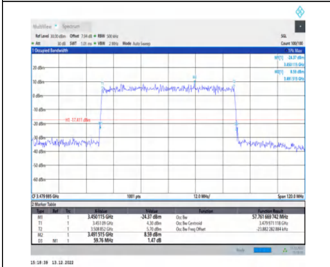
1-N77-3450-3550-30-60-L-5-DFT-256QAM-Outer_Fu ll-162@0-Ant1-57.762-59.760-≤60-PASS
