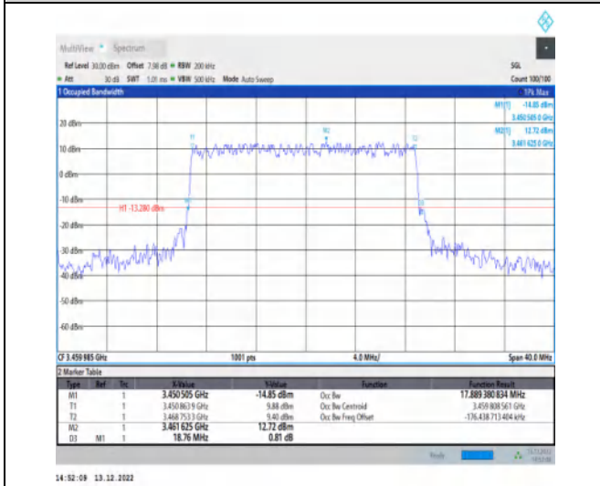
1-N77-3450-3550-30-20-L-1-DFT-QPSK-Outer_Full-50@0-Ant1-17.889-18.760-≤20-PASS
