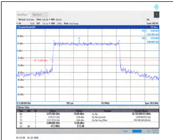
1-N77-3450-3550-30-50-M-1-DFT-QPSK-Outer_Full-128@0-Ant1-45.756-47.500-≤50-PASS
