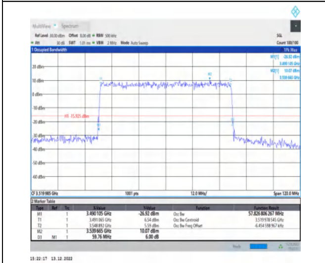
1-N77-3450-3550-30-60-H-3-DFT-16QAM-Outer_Full-162@0-Ant1-57.827-59.760-≤60-PASS
