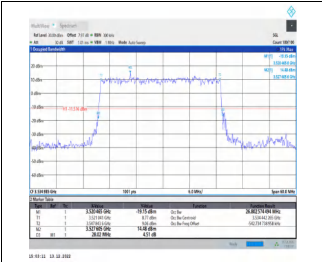
1-N77-3450-3550-30-30-H-2-DFT-PI2BPSK-Outer_Full-75@0-Ant1-26.803-28.020-≤30-PASS
