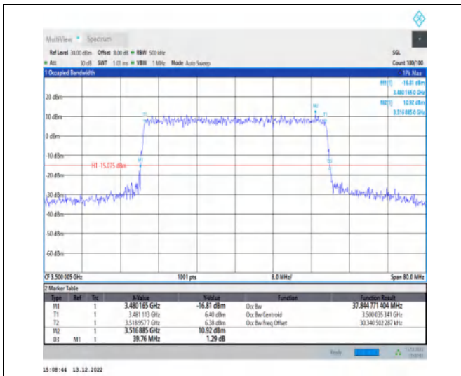
1-N77-3450-3550-30-40-M-8-CP-64QAM-Outer_Full-106@0-Ant1-37.845-39.760-≤40-PASS
