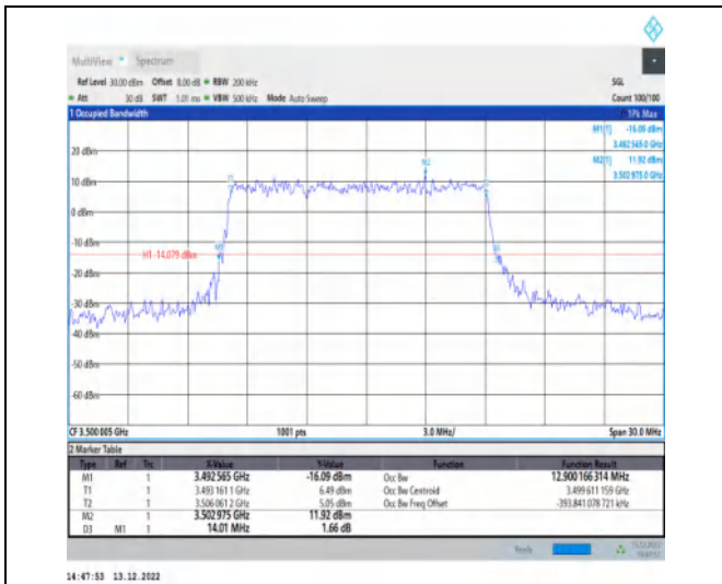
1-N77-3450-3550-30-15-M-1-DFT-QPSK-Outer_Full-36@0-Ant1-12.9-14.010-≤15-PASS
