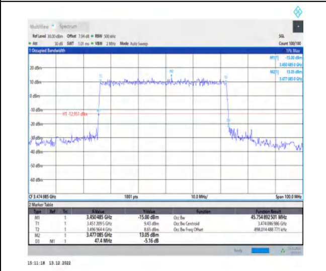
1-N77-3450-3550-30-50-L-1-DFT-QPSK-Outer_Full-128@0-Ant1-45.755-47.400-≤50-PASS
