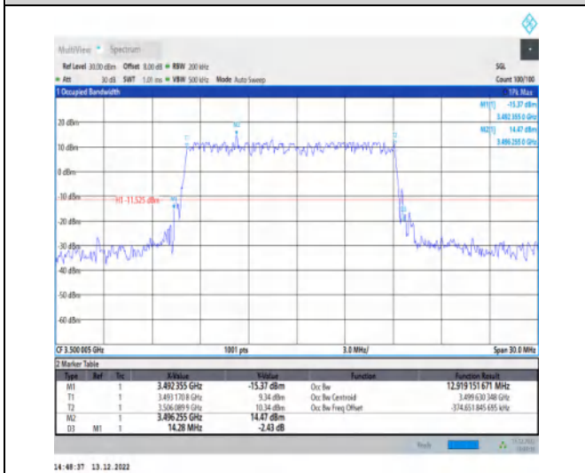
1-N77-3450-3550-30-15-M-3-DFT-16QAM-Outer_Full-36@0-Ant1-12.919-14.280-≤15-PASS
