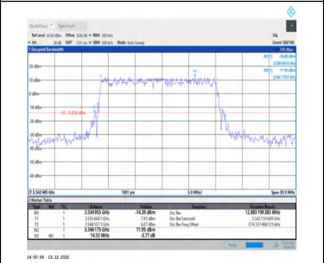
1-N77-3450-3550-30-15-H-3-DFT-16QAM-Outer_Full-36@0-Ant1-12.893-14.550-≤15-PASS
