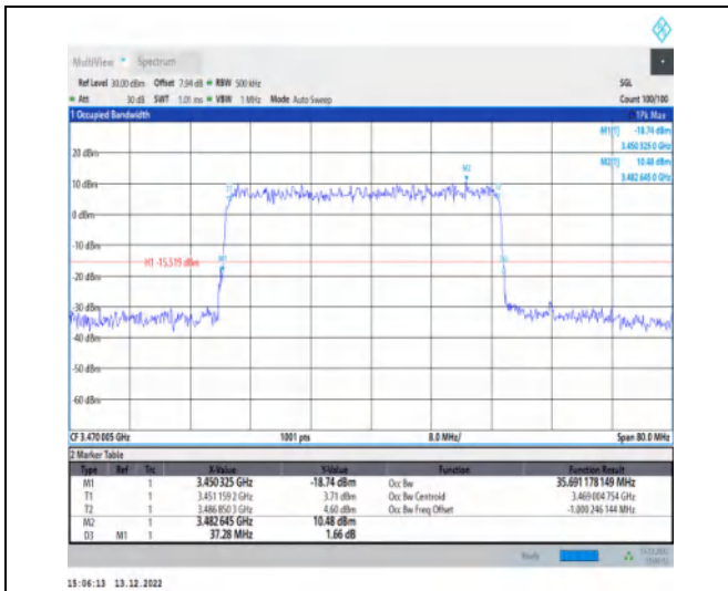
1-N77-3450-3550-30-40-L-5-DFT-256QAM-Outer_Fu II-100@0-Ant1-35.691-37.280-≤40-PASS
