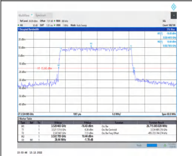
1-N77-3450-3550-30-30-H-4-DFT-64QAM-Outer_Full-75@0-Ant1-26.715-28.440-≤30-PASS
