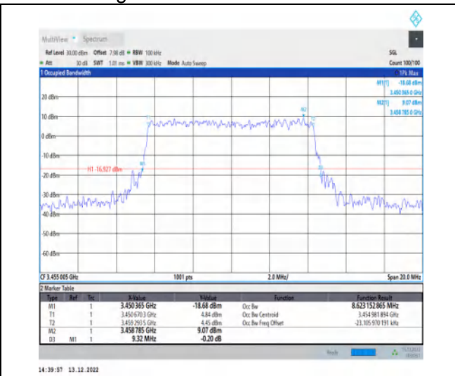
1-N77-3450-3550-30-10-L-6-CP-QPSK-Outer_Full-2 4@0-Ant1-8.623-9.320-≤10-PASS
