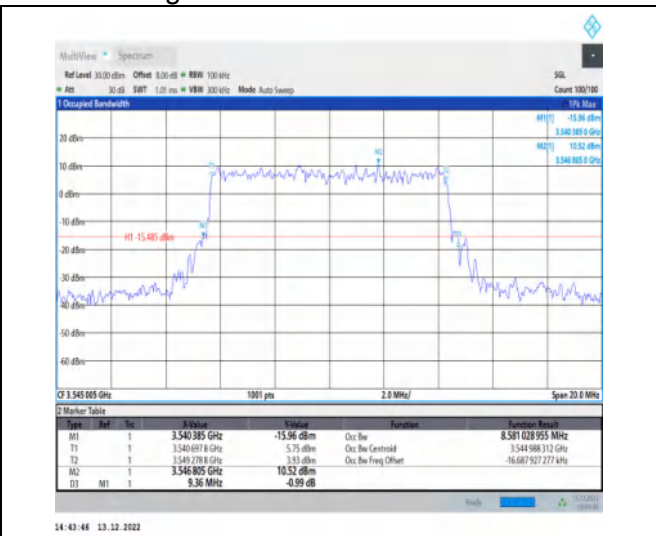
1-N77-3450-3550-30-10-H-4-DFT-64QAM-Outer_Ful I-24@0-Ant1-8.581-9.360-≤10-PASS
