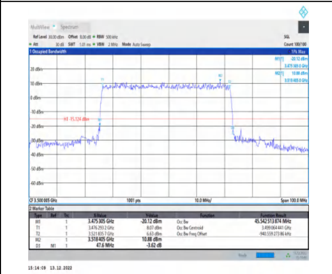
1-N77-3450-3550-30-50-M-4-DFT-64QAM-Outer_Full-128@0-Ant1-45.543-47.600-≤50-PASS
