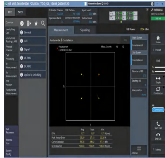
1-N77-3450-3550-30-100-M-2-DFT-QPSK-Outer_Full-270@0-Ant1-see graph-PASS
