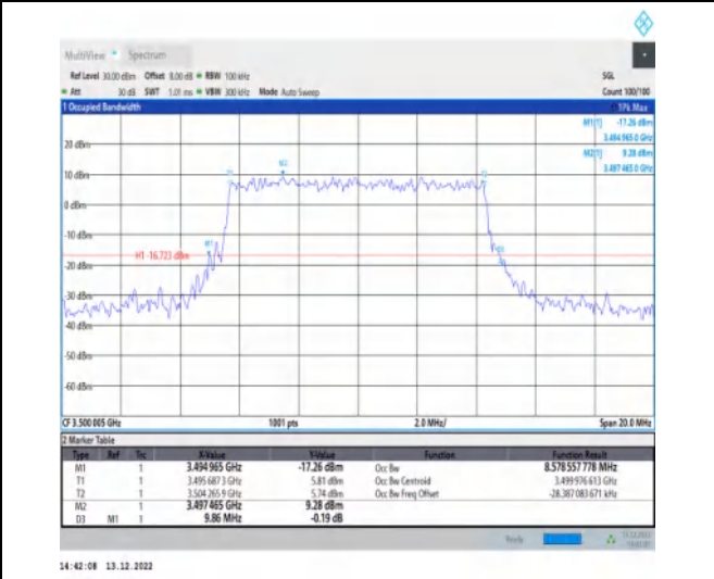
1-N77-3450-3550-30-10-M-7-CP-16QAM-Outer_Full-24@0-Ant1-8.579-9.860-≤10-PASS
