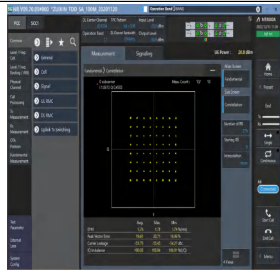
1-N77-3450-3550-30-100-M-4-DFT-64QAM-Outer_Full-270@0-Ant1-see graph-PASS
