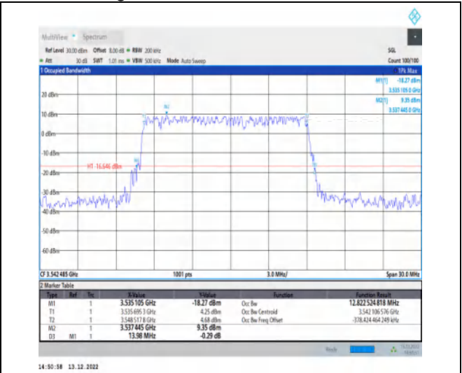
1-N77-3450-3550-30-15-H-5-DFT-256QAM-Outer_Full-I-36@0-Ant1-12.823-13.980-≤15-PASS
