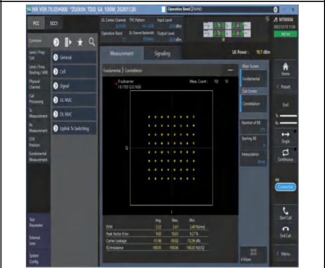
1-N77-3450-3550-30-100-M-8-CP-64QAM-Outer_Full-273@0-Ant1-see graph-PASS
