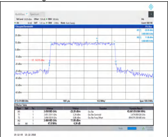
1-N77-3450-3550-30-50-L-3-DFT-16QAM-Outer_Full-128@0-Ant1-45.662-47.800-≤50-PASS
