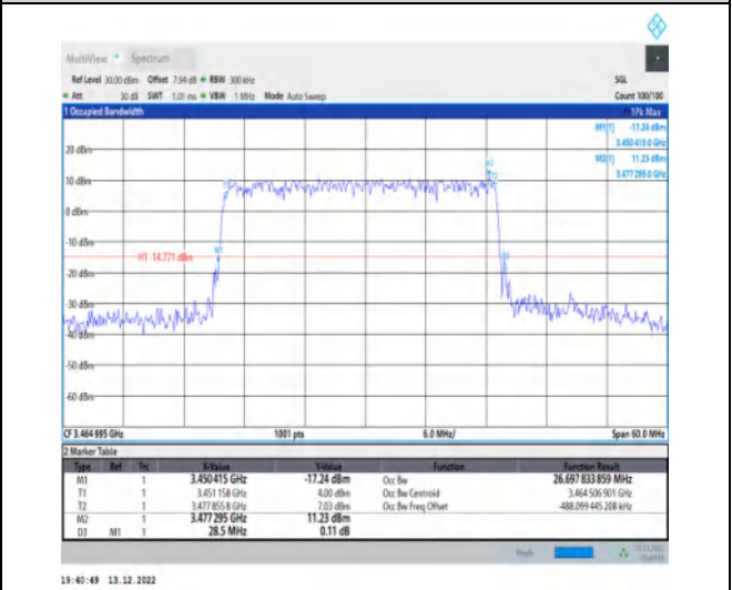
1-N77-3450-3550-30-30-L-3-DFT-16QAM-Outer_Full-75@0-Ant1-26.698-28.500-<=30-PASS
