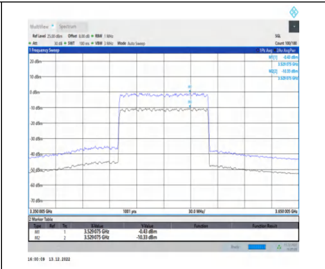
1-N77-3450-3550-30-100-L-2-CP-256QAM-Outer_Full-273@0-Ant1-9.90-100%-0.00-9.90-PASS-≤13
