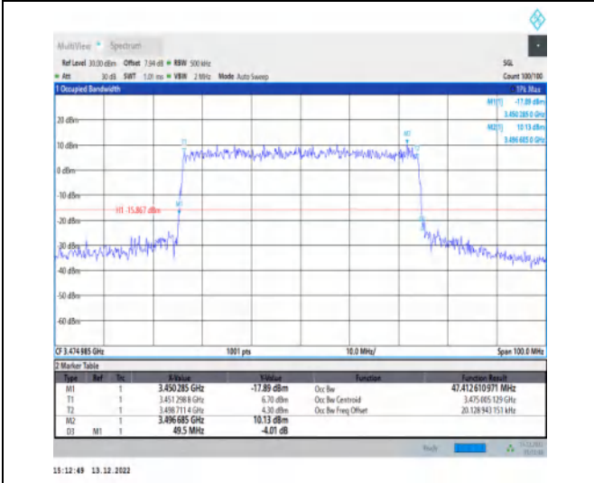
1-N77-3450-3550-30-50-L-8-CP-64QAM-Outer_Full-133@0-Ant1-47.413-49.500-≤50-PASS
