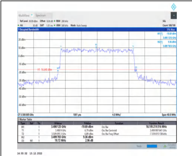
1-N77-3450-3550-30-20-M-6-CP-QPSK-Outer_Full-5 1@0-Ant1-18.195-19.720-≤20-PASS
