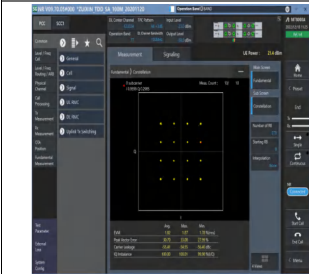
1-N77-3450-3550-30-100-M-3-DFT-16QAM-Outer_Full-270@0-Ant1-see graph-PASS
