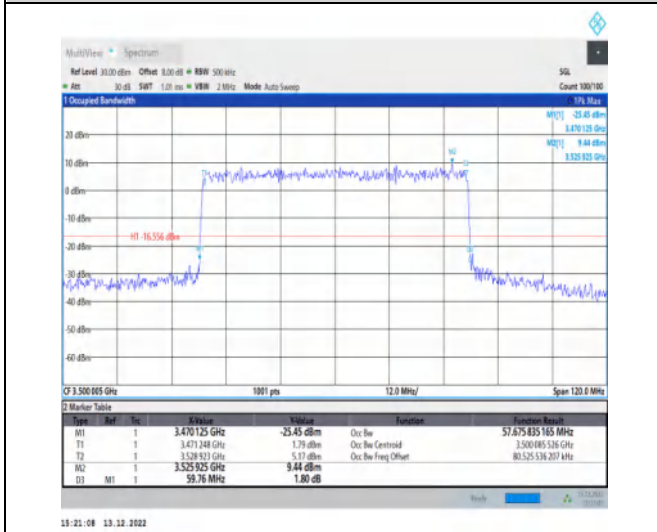
1-N77-3450-3550-30-60-M-8-CP-64QAM-Outer_Full-162@0-Ant1-57.676-59.760-≤60-PASS
