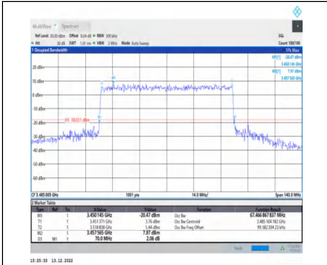
1-N77-3450-3550-30-70-L-8-CP-64QAM-Outer_Full-189@0-Ant1-67.467-70.000-≤70-PASS
