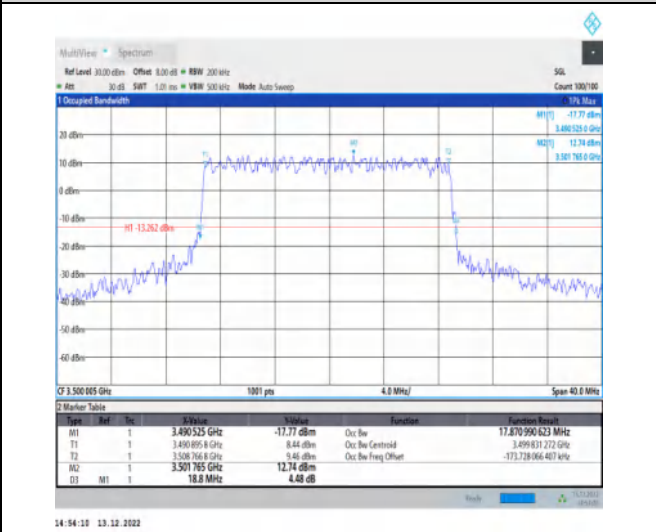
1-N77-3450-3550-30-20-M-1-DFT-QPSK-Outer_Full-50@0-Ant1-17.871-18.800-≤20-PASS
