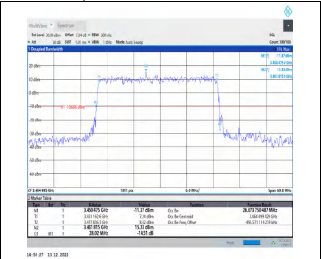
1-N77-3450-3550-30-30-L-1-DFT-QPSK-Outer_Full-75@0-Ant1-26.674-28.020-<=30-PASS
