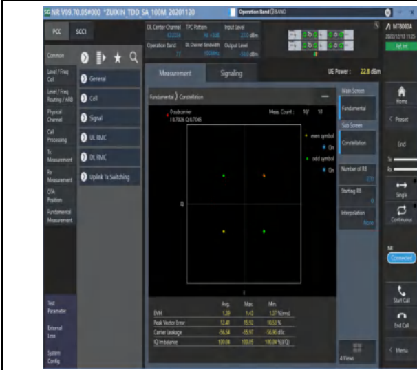
1-N77-3450-3550-30-100-M-1-DFT-PI2BPSK-Outer_Full-270@0-Ant1-see graph-PASS
