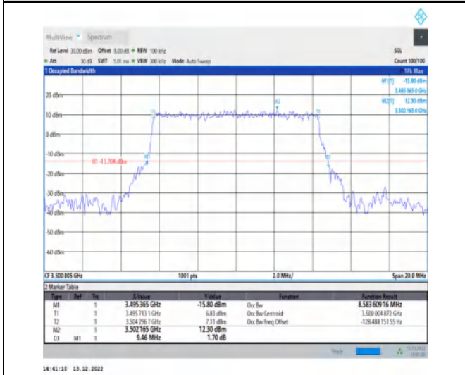
1-N77-3450-3550-30-10-M-2-DFT-PI2BPSK-Outer_F ull-24@0-Ant1-8.584-9.460-≤10-PASS
