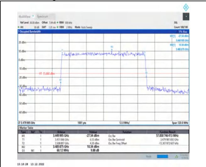
1-N77-3450-3550-30-60-L-4-DFT-64QAM-Outer_Full -162@0-Ant1-57.831-60.120-≤60-PASS
