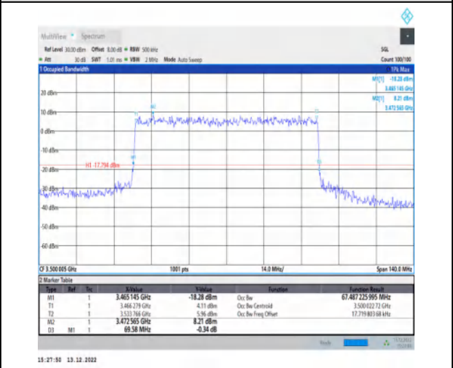
1-N77-3450-3550-30-70-M-6-CP-QPSK-Outer_Full-189@0-Ant1-67.487-69.580-≤70-PASS
