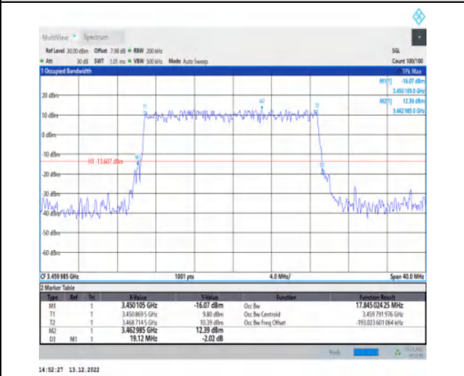
1-N77-3450-3550-30-20-L-2-DFT-PI2BPSK-Outer_Full-50@0-Ant1-17.845-19.120-≤20-PASS
