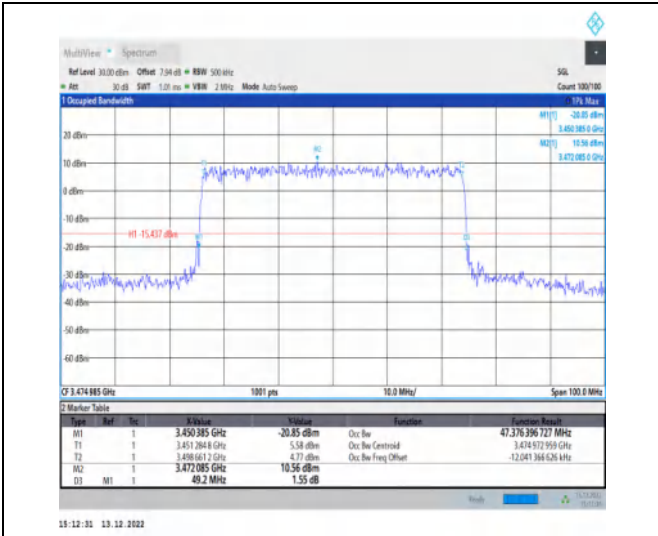
1-N77-3450-3550-30-50-L-6-CP-QPSK-Outer_Full-1 33@0-Ant1-47.376-49.200-≤50-PASS
