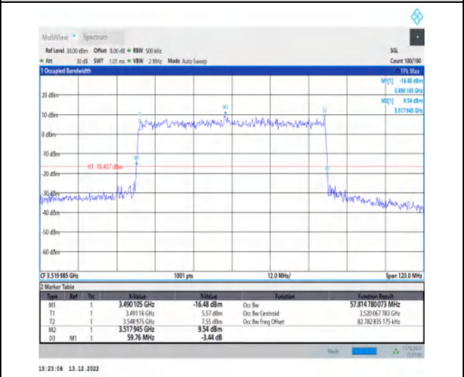
1-N77-3450-3550-30-60-H-8-CP-64QAM-Outer_Full-162@0-Ant1-57.815-59.760-≤60-PASS
