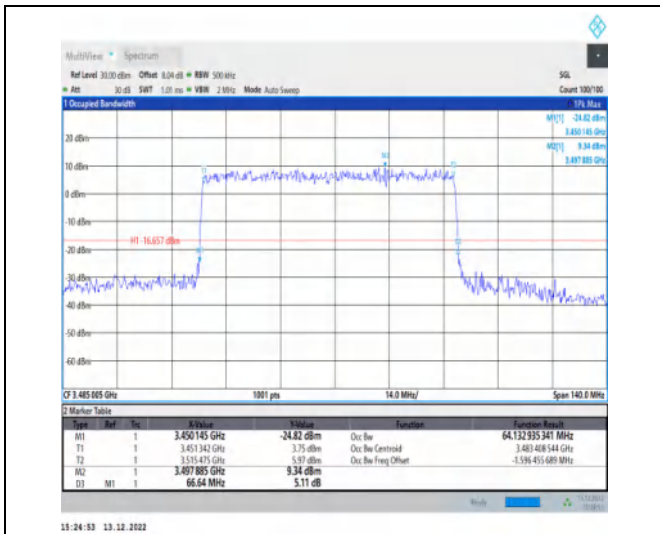
1-N77-3450-3550-30-70-L-4-DFT-64QAM-Outer_Full -180@0-Ant1-64.133-66.640-≤70-PASS
