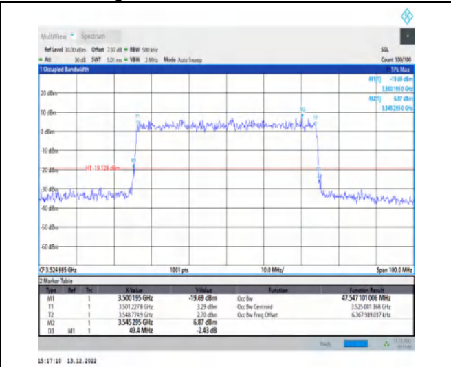
1-N77-3450-3550-30-50-H-9-CP-256QAM-Outer_Full-133@0-Ant1-47.547-49.400-≤50-PASS
