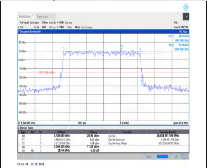
1-N77-3450-3550-30-30-M-4-DFT-64QAM-Outer_Ful I-75@0-Ant1-26.838-28.440-≤30-PASS
