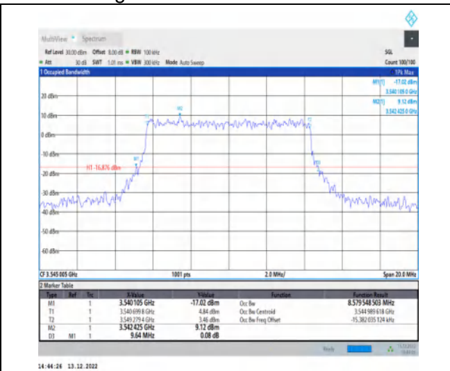
1-N77-3450-3550-30-10-H-8-CP-64QAM-Outer_Full-24@0-Ant1-8.58-9.640-≤10-PASS
