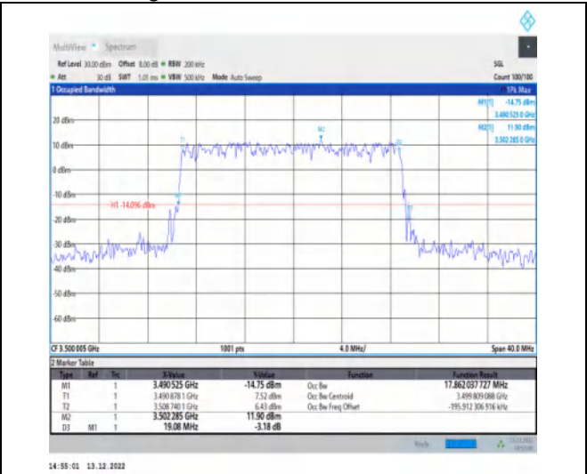
1-N77-3450-3550-30-20-M-3-DFT-16QAM-Outer_Full-50@0-Ant1-17.862-19.080-≤20-PASS
