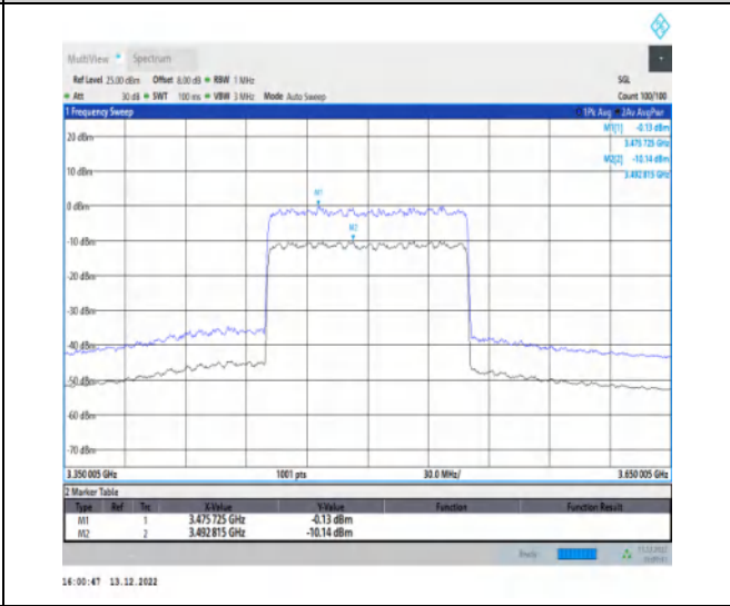
1-N77-3450-3550-30-100-M-2-CP-256QAM-Outer_Full-273@0-Ant1-10.01-100%-0.00-10.01-PASS-≤13
