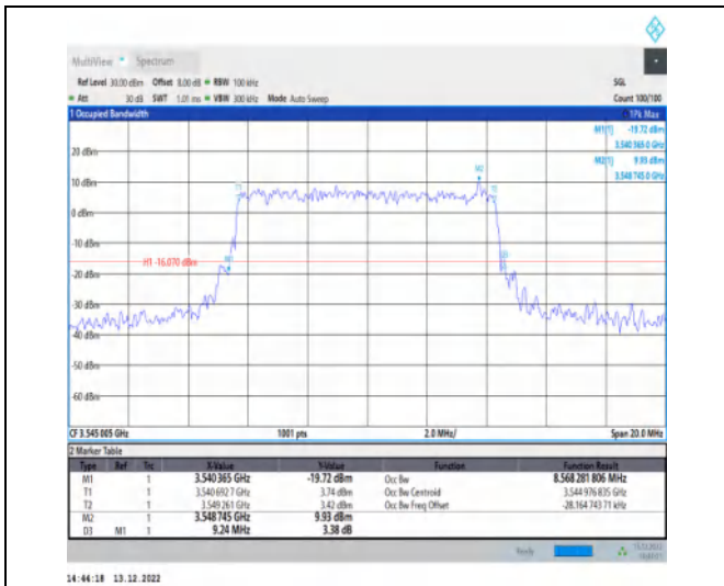
1-N77-3450-3550-30-10-H-7-CP-16QAM-Outer_Full-24@0-Ant1-8.568-9.240-≤10-PASS
