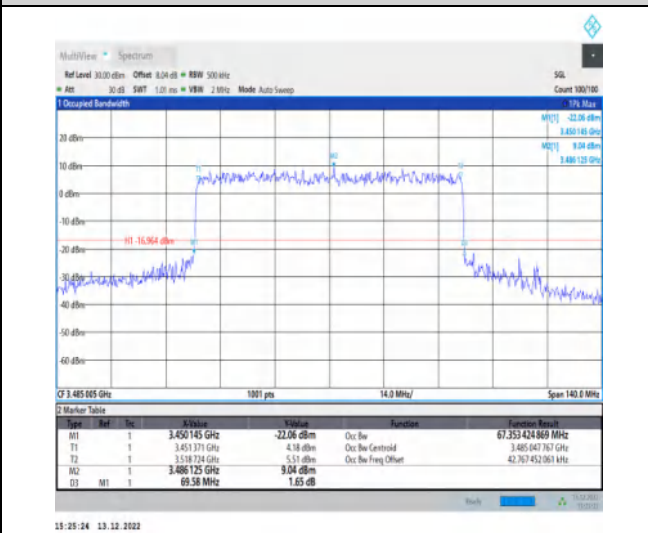
1-N77-3450-3550-30-70-L-7-CP-16QAM-Outer_Full-189@0-Ant1-67.353-69.580-≤70-PASS
