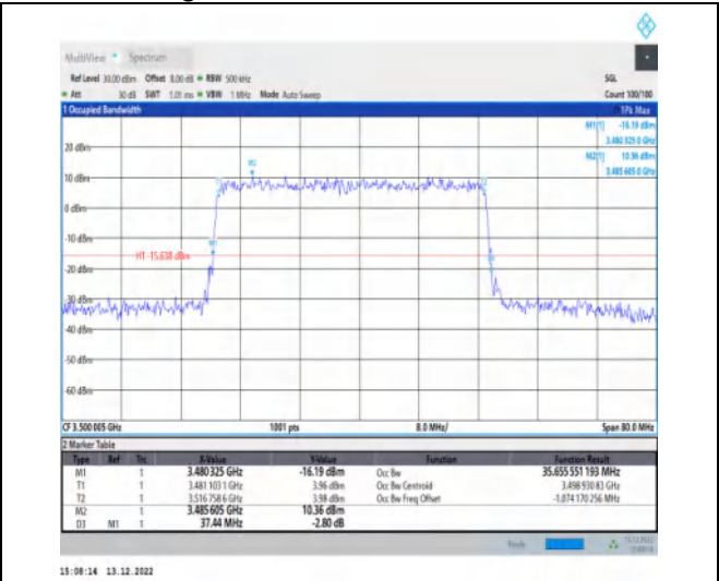
1-N77-3450-3550-30-40-M-5-DFT-256QAM-Outer_Full-100@0-Ant1-35.656-37.440-≤40-PASS
