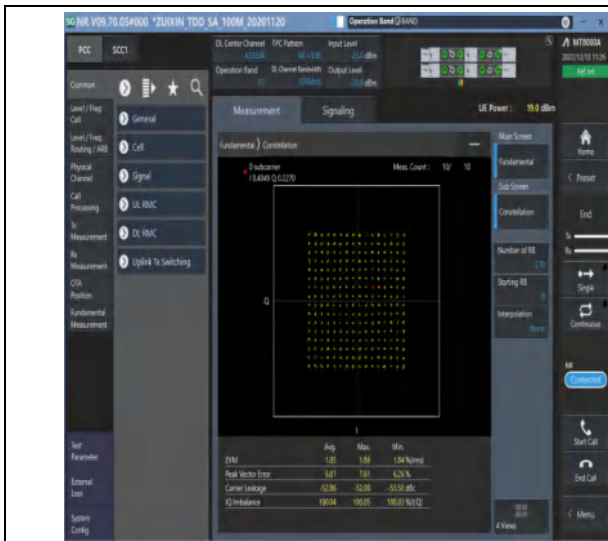
1-N77-3450-3550-30-100-M-5-DFT-256QAM-Outer_Full-270@0-Ant1-see graph-PASS
