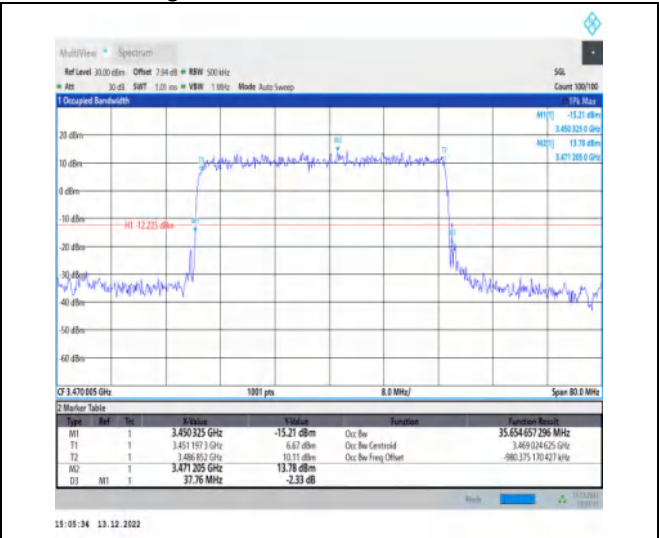
1-N77-3450-3550-30-40-L-2-DFT-PI2BPSK-Outer_Full-100@0-Ant1-35.655-37.760-≤40-PASS
