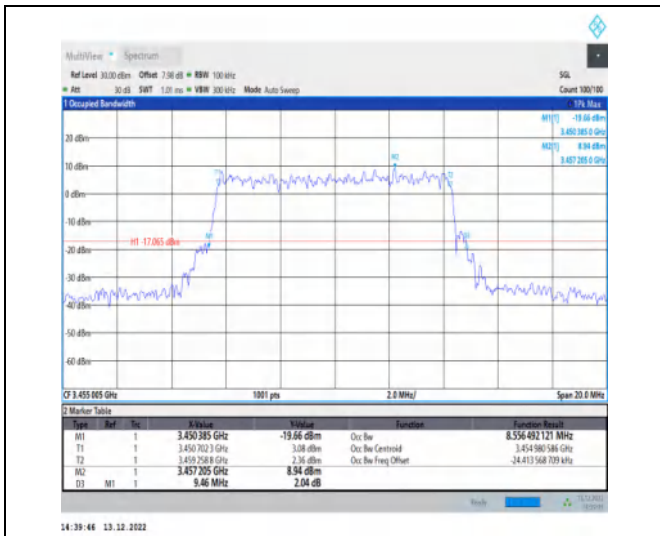
1-N77-3450-3550-30-10-L-5-DFT-256QAM-Outer_Fu II-24@0-Ant1-8.556-9.460-≤10-PASS
