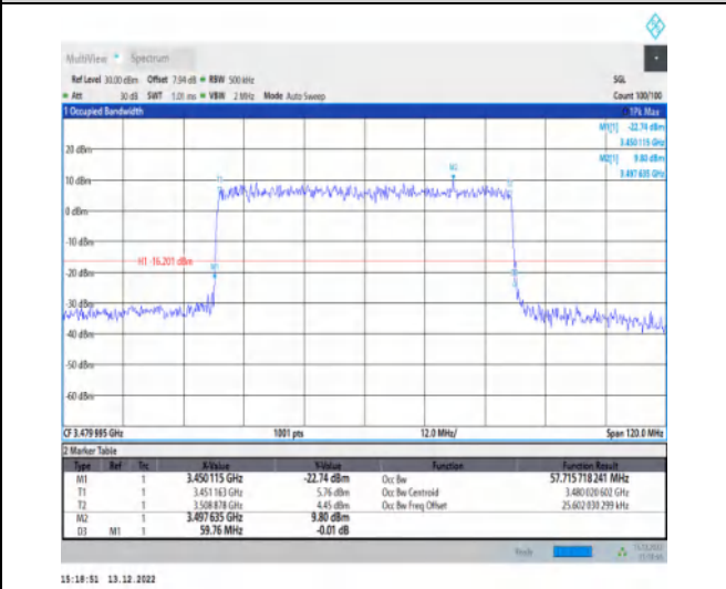
1-N77-3450-3550-30-60-L-6-CP-QPSK-Outer_Full-1 62@0-Ant1-57.716-59.760-≤60-PASS
