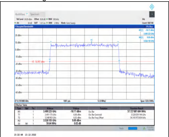
1-N77-3450-3550-30-60-H-6-CP-QPSK-Outer_Full-162@0-Ant1-57.728-59.640-≤60-PASS
