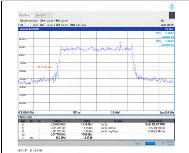
1-N77-3450-3550-30-15-H-8-CP-64QAM-Outer_Full-38@0-Ant1-13.622-15.000-≤15-PASS
