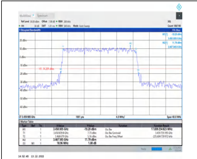
1-N77-3450-3550-30-20-L-3-DFT-16QAM-Outer_Full -50@0-Ant1-17.839-18.960-<=20-PASS
