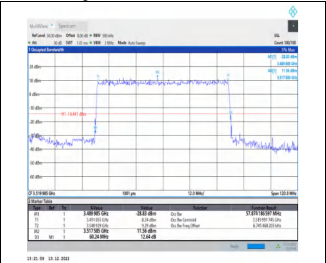
1-N77-3450-3550-30-60-H-2-DFT-PI2BPSK-Outer_Full-162@0-Ant1-57.874-60.240-≤60-PASS
