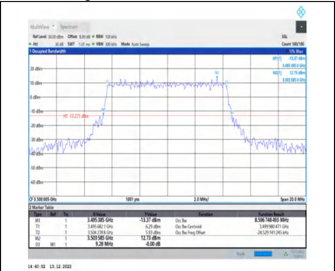
1-N77-3450-3550-30-10-M-1-DFT-QPSK-Outer_Full -24@0-Ant1-8.597-9.280-≤10-PASS
