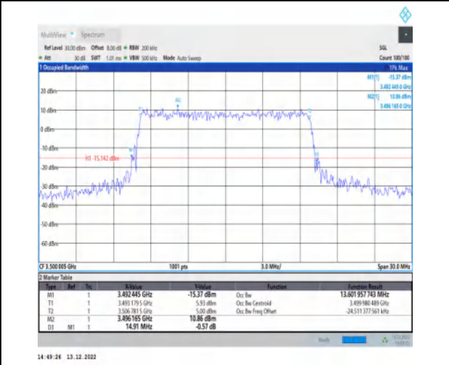
1-N77-3450-3550-30-15-M-8-CP-64QAM-Outer_Full-38@0-Ant1-13.602-14.910-≤15-PASS
