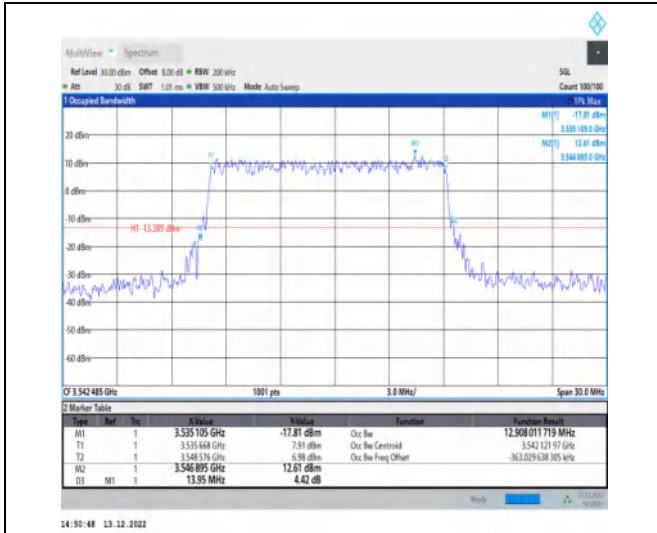
1-N77-3450-3550-30-15-H-4-DFT-64QAM-Outer_Full-I-36@0-Ant1-12.908-13.950-≤15-PASS
