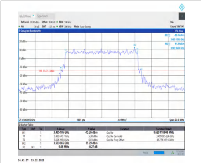
1-N77-3450-3550-30-10-M-4-DFT-64QAM-Outer_Ful I-24@0-Ant1-8.629-9.680-≤10-PASS
