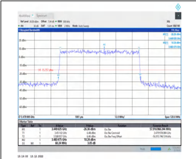
1-N77-3450-3550-30-60-L-7-CP-16QAM-Outer_Full-162@0-Ant1-57.917-60.240-≤60-PASS
