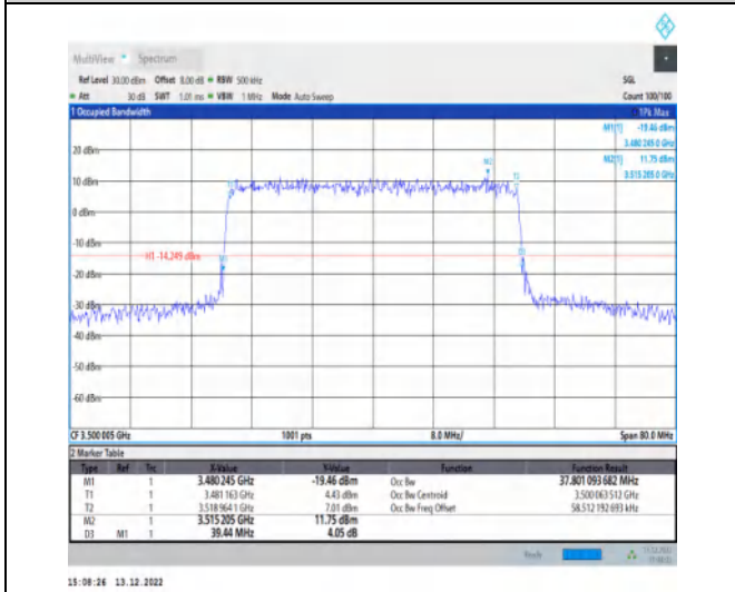
1-N77-3450-3550-30-40-M-6-CP-QPSK-Outer_Full-106@0-Ant1-37.801-39.440-≤40-PASS
