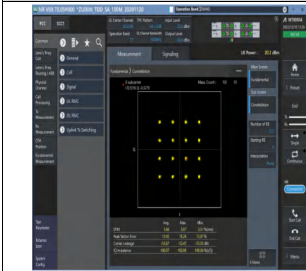
1-N77-3450-3550-30-100-M-7-CP-16QAM-Outer_Full-273@0-Ant1-see graph-PASS
