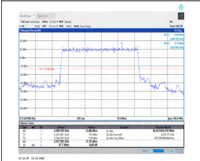
1-N77-3450-3550-30-50-H-2-DFT-PI2BPSK-Outer_Full-128@0-Ant1-45.616-47.700-≤50-PASS
