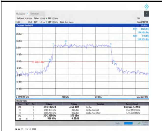
1-N77-3450-3550-30-10-H-9-CP-256QAM-Outer_Ful-I-24@0-Ant1-8.583-9.660-≤10-PASS
