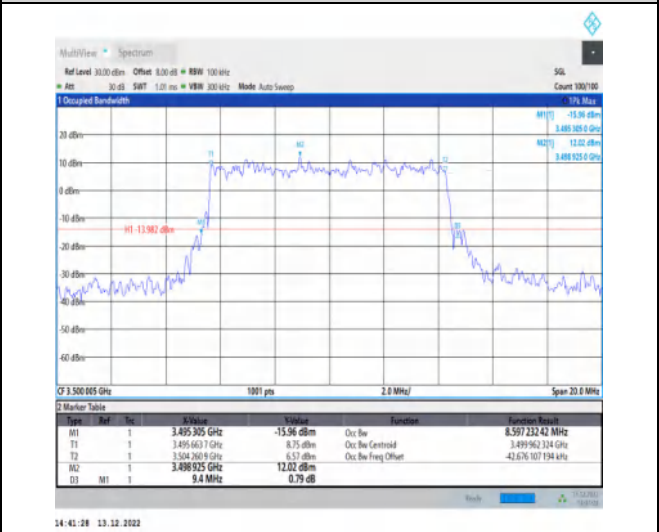
1-N77-3450-3550-30-10-M-3-DFT-16QAM-Outer_Ful l-24@0-Ant1-8.597-9.400-≤10-PASS
