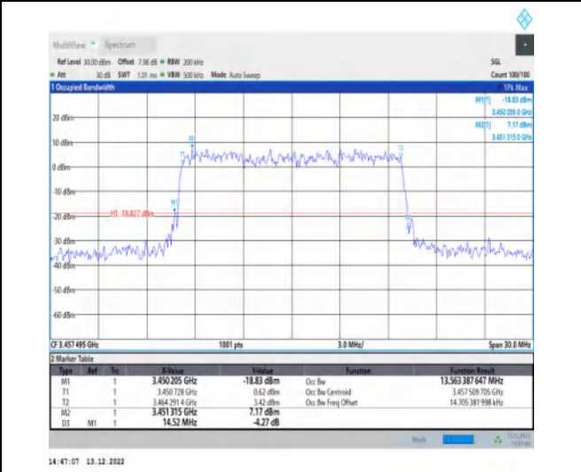
1-N77-3450-3550-30-15-L-9-CP-256QAM-Outer_Full-38@0-Ant1-13.563-14.520-≤15-PASS
