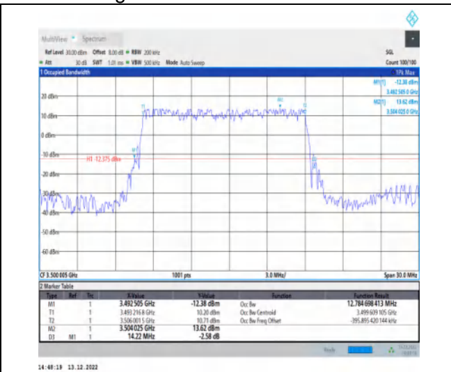
1-N77-3450-3550-30-15-M-2-DFT-PI2BPSK-Outer_Full-36@0-Ant1-12.785-14.220-≤15-PASS
