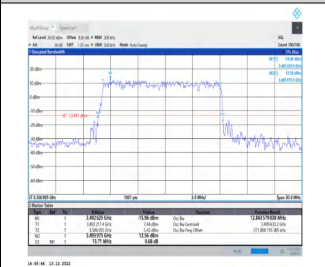
1-N77-3450-3550-30-15-M-4-DFT-64QAM-Outer_Full-36@0-Ant1-12.844-13.710-≤15-PASS
