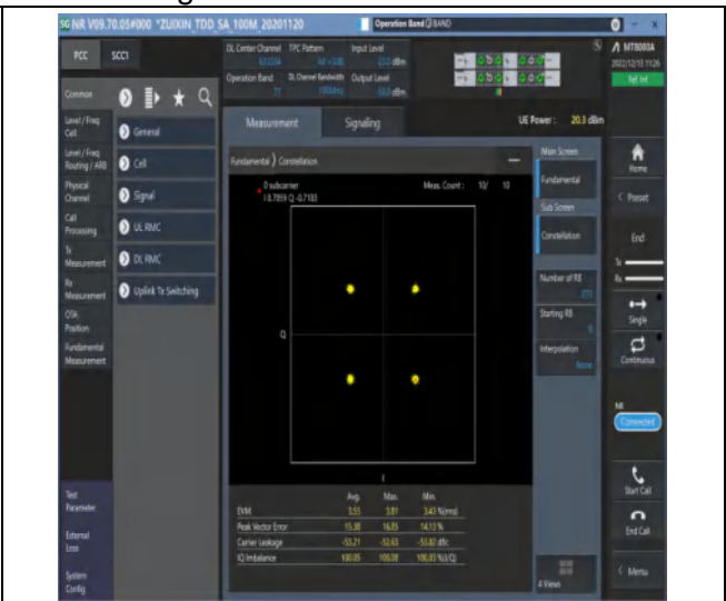
1-N77-3450-3550-30-100-M-6-CP-QPSK-Outer_Full-273@0-Ant1-see graph-PASS
