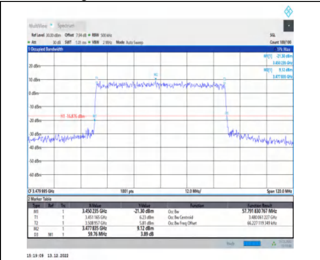
1-N77-3450-3550-30-60-L-8-CP-64QAM-Outer_Full-162@0-Ant1-57.792-59.760-≤60-PASS
