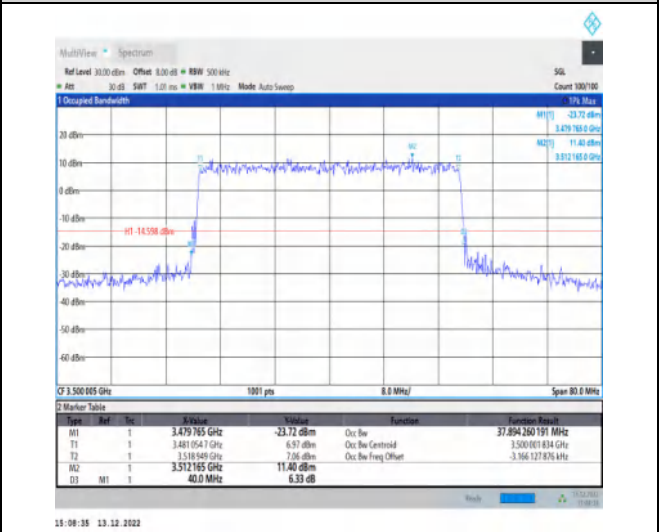
1-N77-3450-3550-30-40-M-7-CP-16QAM-Outer_Full-106@0-Ant1-37.894-40.000-≤40-PASS
