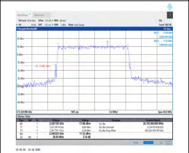
1-N77-3450-3550-30-30-H-1-DFT-QPSK-Outer_Full-75@0-Ant1-26.743-28.440-≤30-PASS
