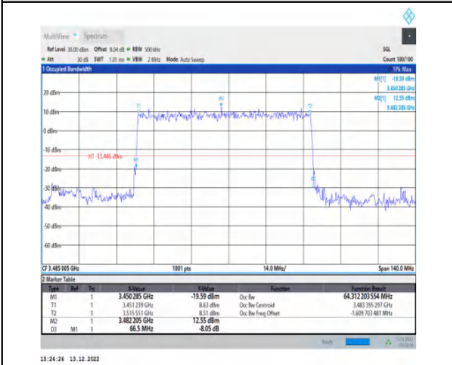
1-N77-3450-3550-30-70-L-2-DFT-PI2BPSK-Outer_Full-180@0-Ant1-64.312-66.500-≤70-PASS
