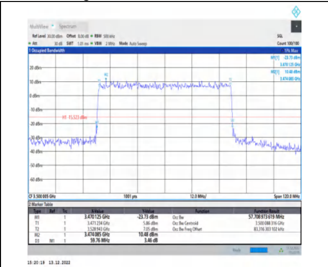
1-N77-3450-3550-30-60-M-3-DFT-16QAM-Outer_Full-162@0-Ant1-57.709-59.760-≤60-PASS
