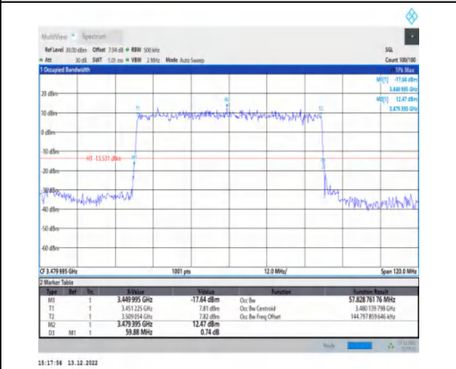
1-N77-3450-3550-30-60-L-2-DFT-PI2BPSK-Outer_Full-162@0-Ant1-57.829-59.880-≤60-PASS
