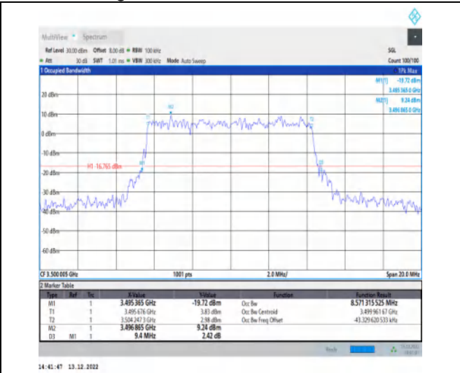
1-N77-3450-3550-30-10-M-5-DFT-256QAM-Outer_Full-24@0-Ant1-8.571-9.400-≤10-PASS
