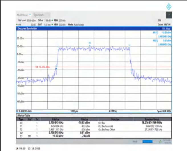
1-N77-3450-3550-30-20-L-6-CP-QPSK-Outer_Full-5 1@0-Ant1-18.217-19.360-<=20-PASS
