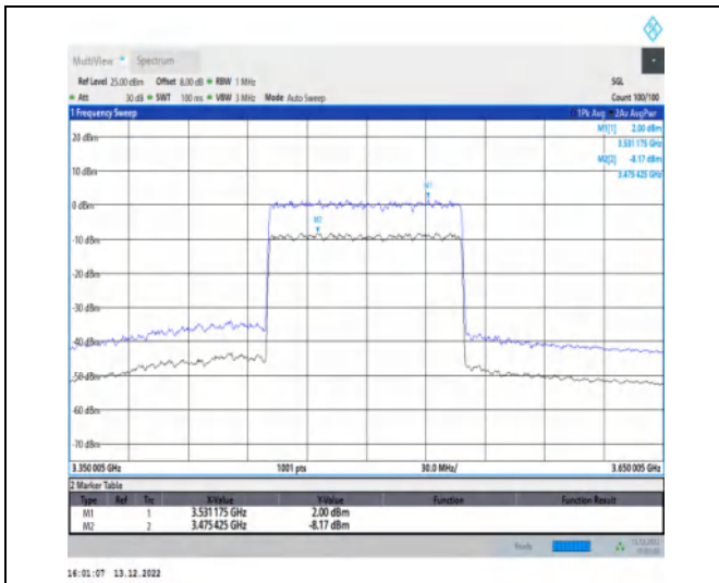
1-N77-3450-3550-30-100-H-1-DFT-256QAM-Outer_Full-270@0-Ant1-10.17-100%-0.00-10.17-PASS- \leq 13
