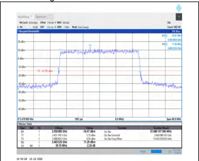
1-N77-3450-3550-30-40-L-6-CP-QPSK-Outer_Full-1 06@0-Ant1-37.68-39.760-≤40-PASS
