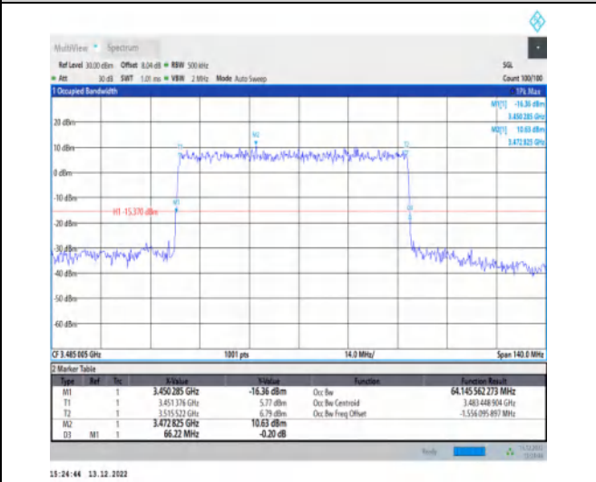
1-N77-3450-3550-30-70-L-3-DFT-16QAM-Outer_Full-180@0-Ant1-64.146-66.220-≤70-PASS
