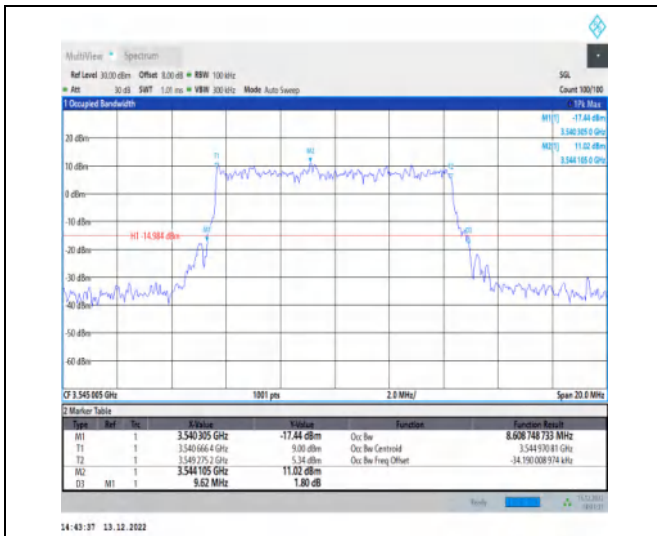
1-N77-3450-3550-30-10-H-3-DFT-16QAM-Outer_Ful I-24@0-Ant1-8.609-9.620-≤10-PASS
