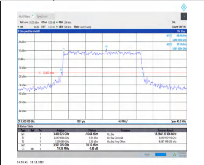
1-N77-3450-3550-30-20-M-7-CP-16QAM-Outer_Full -51@0-Ant1-18.184-19.360-≤20-PASS
