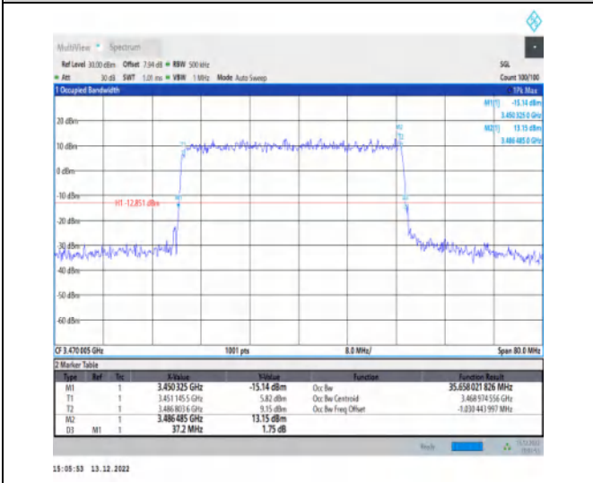
1-N77-3450-3550-30-40-L-3-DFT-16QAM-Outer_Full-100@0-Ant1-35.658-37.200-≤40-PASS
