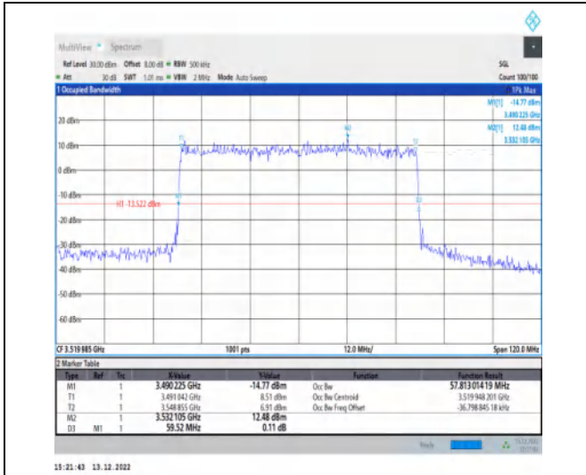
1-N77-3450-3550-30-60-H-1-DFT-QPSK-Outer_Full-162@0-Ant1-57.813-59.520-≤60-PASS
