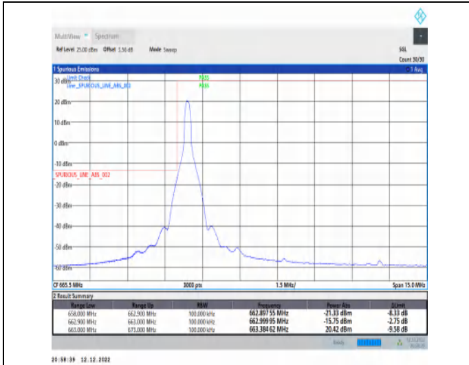
1-N71-15-10-L-1-DFT-PI2BPSK-Edge_1RB_Left-1@0-Ant1-1--PASS-see graph
