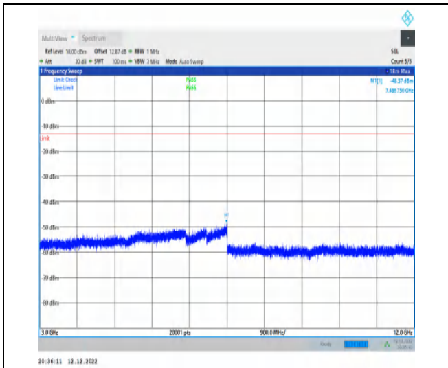
1-N71-15-20-H-1-DFT-PI2BPSK-Inner_1RB_Left-1 @1-3000-12000-Ant1-7488.75--48.57--13-PASS
