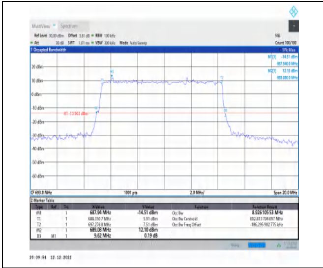
1-N71-15-10-H-4-DFT-64QAM-Outer_Full-50@0-Ant 1-8.926-9.620-≤10-PASS
