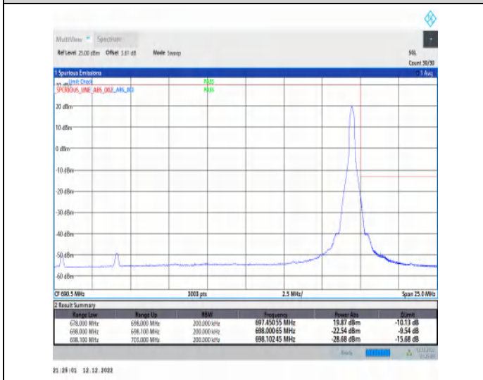
1-N71-15-20-H-5-CP-QPSK-Edge_1RB_Right-1@105-Ant1-1--PASS-see graph
