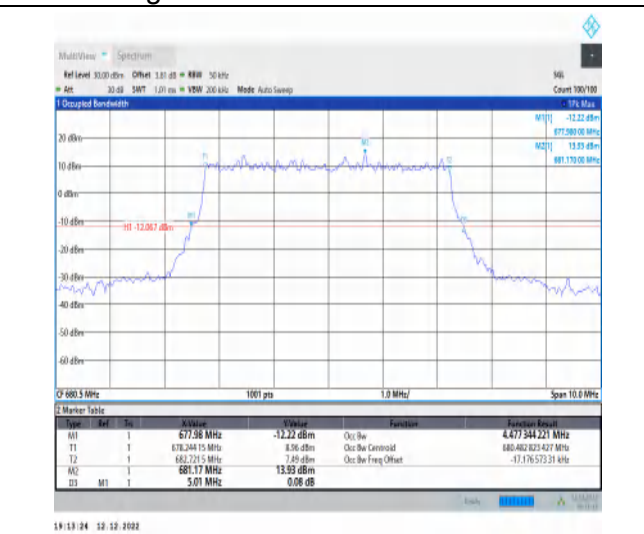
1-N71-15-5-M-1-DFT-QPSK-Outer_Full-25@0-Ant1- 4.477-5.010-≤5-PASS
