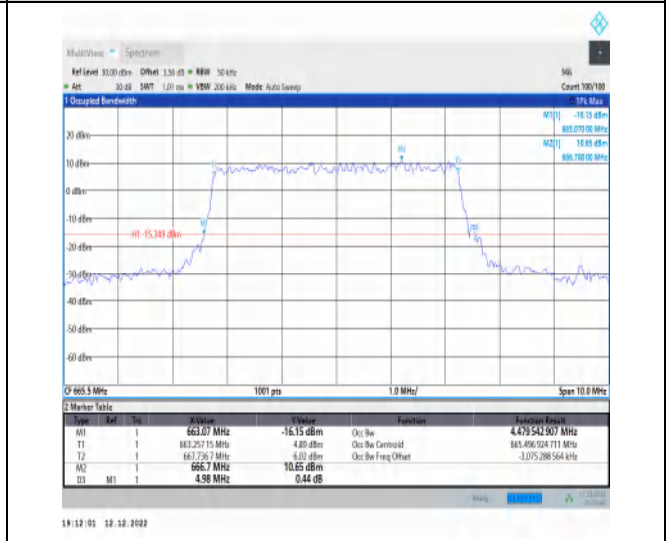
1-N71-15-5-L-4-DFT-64QAM-Outer_Full-25@0-Ant1- 4.48-4.980- \leq 5 -PASS
