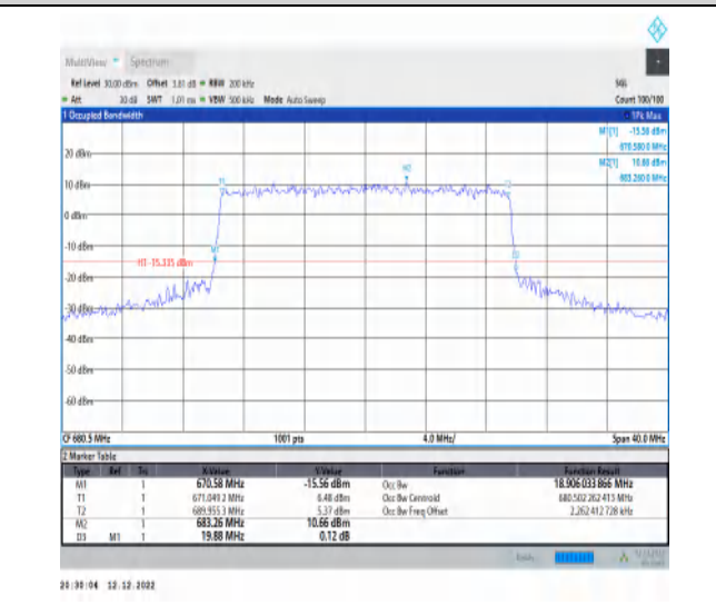
1-N71-15-20-M-6-CP-QPSK-Outer_Full-106@0-Ant1 -18.906-19.880-≤20-PASS
