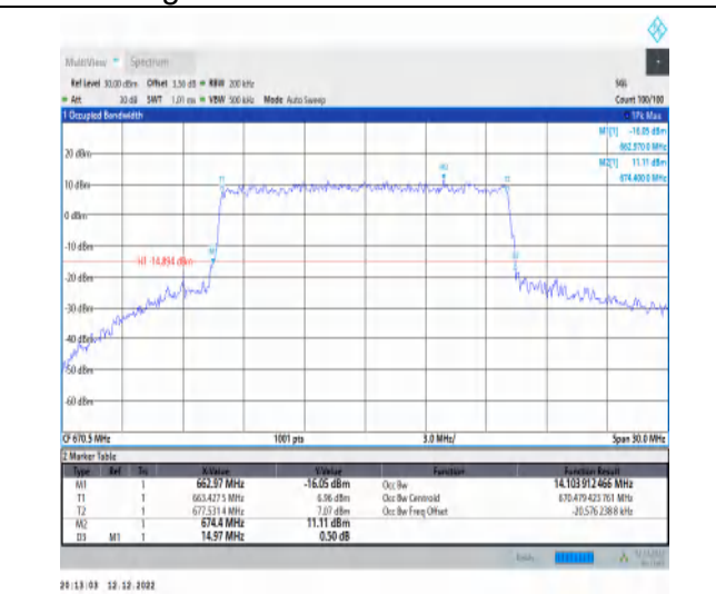
1-N71-15-15-L-8-CP-64QAM-Outer_Full-79@0-Ant1- 14.104-14.970-≤15-PASS
