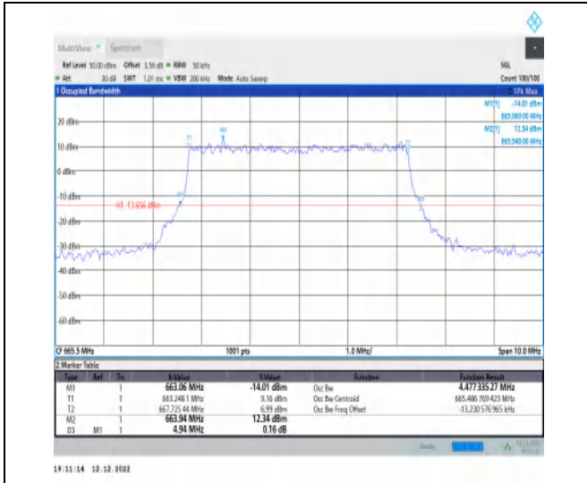
1-N71-15-5-L-1-DFT-QPSK-Outer_Full-25@0-Ant1-4 4.477-4.940- \leq 5 -PASS
