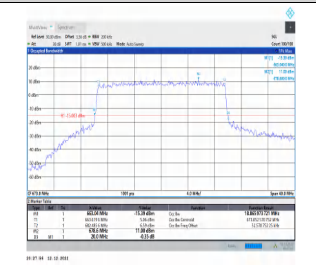
1-N71-15-20-L-7-CP-16QAM-Outer_Full-106@0-Ant 1-18.866-20.000-<20-PASS
