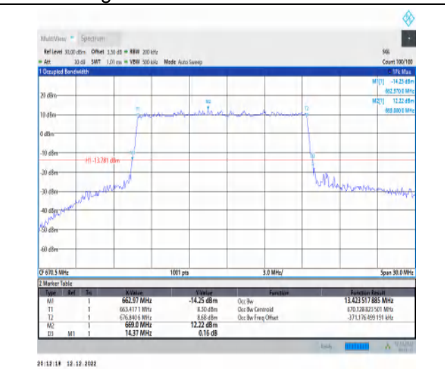
1-N71-15-15-L-4-DFT-64QAM-Outer_Full-75@0-Ant 1-13.424-14.370-≤15-PASS
