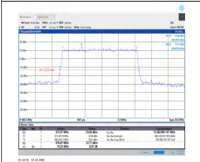
1-N71-15-15-M-4-DFT-64QAM-Outer_Full-75@0-Ant 1-13.402-14.250-≤15-PASS
