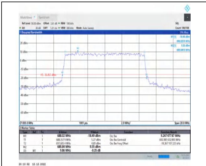
1-N71-15-10-H-8-CP-64QAM-Outer_Full-52@0-Ant1 -9.247-9.860-≤10-PASS
