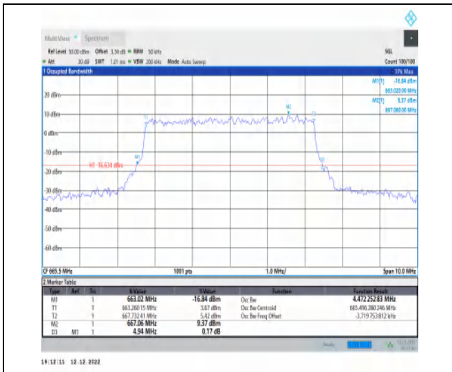
1-N71-15-5-L-5-DFT-256QAM-Outer_Full-25@0-Ant 1-4.472-4.940-≤5-PASS
