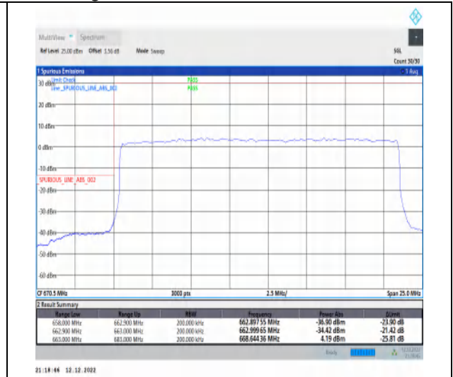
1-N71-15-20-L-3-DFT-PI2BPSK-Outer_Full-100@0-Ant1-1--PASS-see graph
