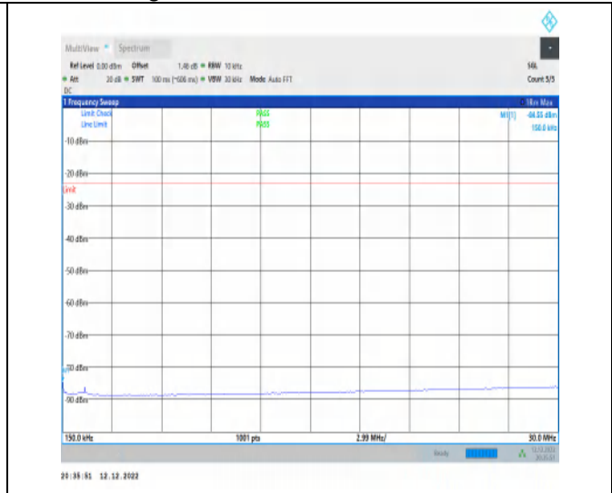
1-N71-15-20-H-1-DFT-PI2BPSK-Inner_1RB_Left-1 @ 1-0.15-30-Ant1-0.15--84.55--23-PASS
