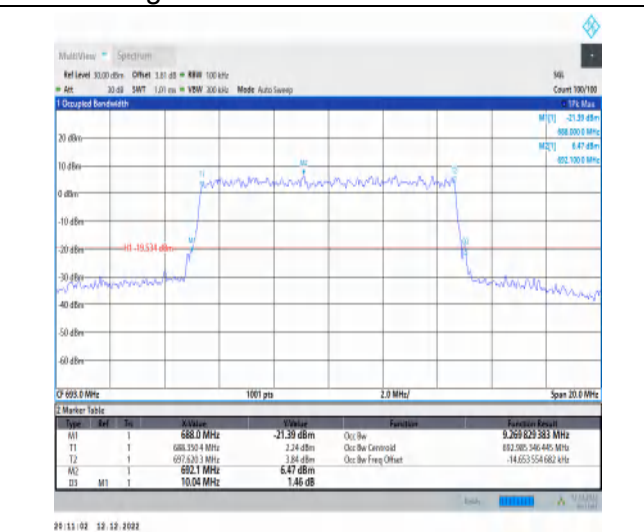
1-N71-15-10-H-9-CP-256QAM-Outer_Full-52@0-Ant 1-9.27-10.040-≤10-PASS
