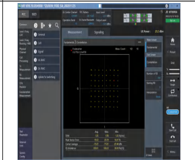
1-N71-15-20-M-4-DFT-64QAM-Outer_Full-100@0-Ant1-see graph-PASS
