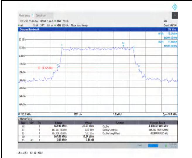
1-N71-15-5-L-3-DFT-16QAM-Outer_Full-25@0-Ant1 -4.499-5.090- \leq 5 -PASS
