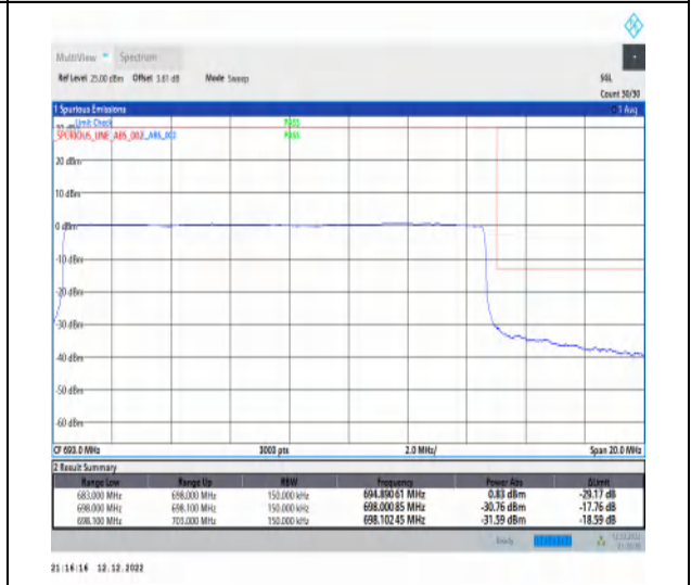
1-N71-15-15-H-6-CP-QPSK-Outer_Full-79@0-Ant1-1--PASS-see graph
