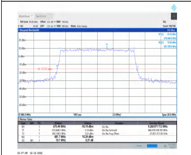
1-N71-15-10-M-7-CP-16QAM-Outer_Full-52@0-Ant 1-9.26-10.100-≤10-PASS
