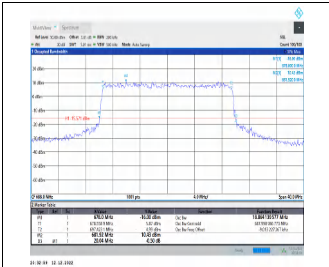
1-N71-15-20-H-6-CP-QPSK-Outer_Full-106@0-Ant1 -18.864-20.040-≤20-PASS
