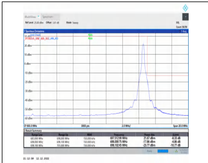
1-N71-15-15-H-2-DFT-PI2BPSK-Edge_1RB_Right-1@78-Ant1-1--PASS-see graph
