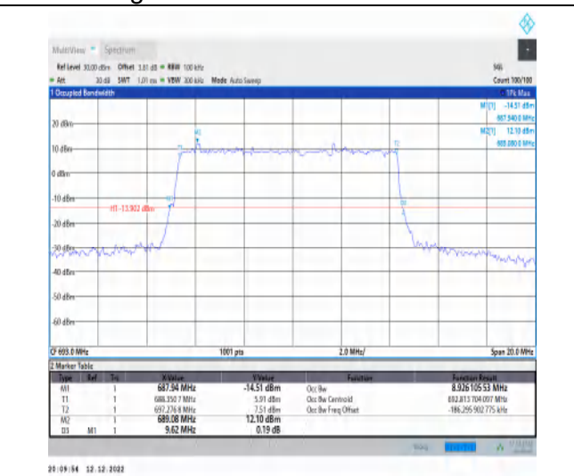
1-N71-15-10-H-1-DFT-QPSK-Outer_Full-50@0-Ant1 -19.797-20.000-≤10-PASS
