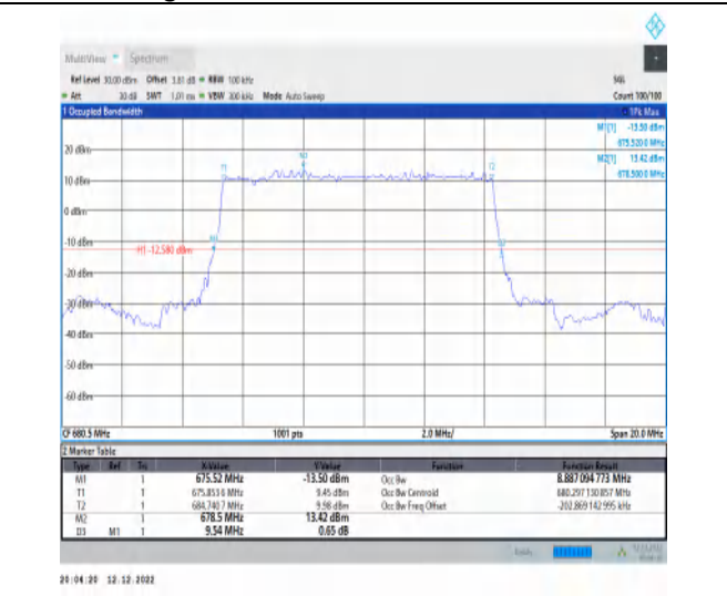
1-N71-15-10-M-2-DFT-PI2BPSK-Outer_Full-50@0-Ant1 8.887-9.540-≤10-PASS
