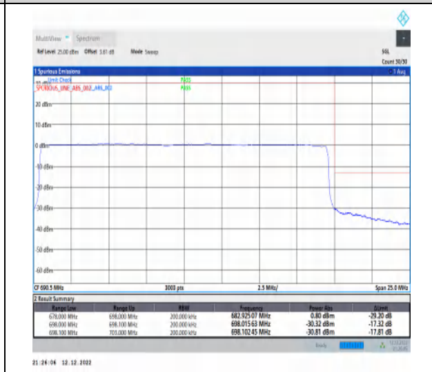
1-N71-15-20-H-6-CP-QPSK-Outer_Full-106@0-Ant1-1--PASS-see graph
