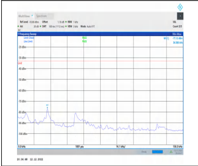
1-N71-15-20-M-1-DFT-PI2BPSK-Inner_1RB_Left-1 @ 1-0.009-0.15-Ant1-0.03--77.12--33-PASS
