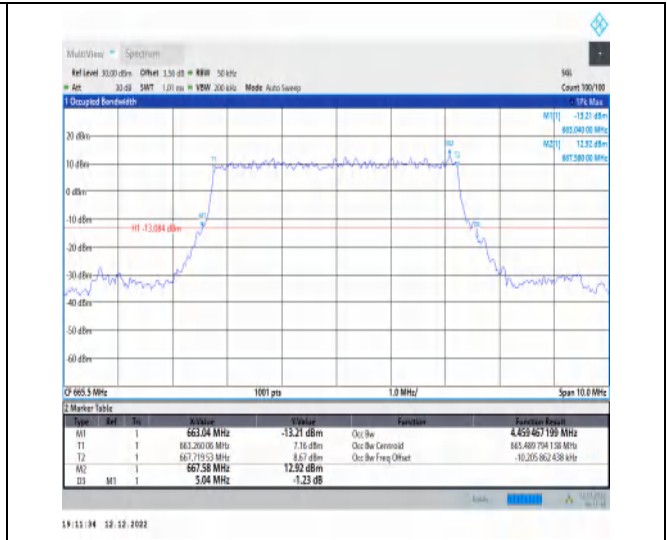
1-N71-15-5-L-2-DFT-PI2BPSK-Outer_Full-25@0-Ant 1-4.459-5.040- \leq 5 -PASS
