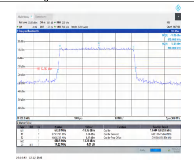
1-N71-15-15-M-3-DFT-16QAM-Outer_Full-75@0-Ant 1-13.444-14.220-≤15-PASS
