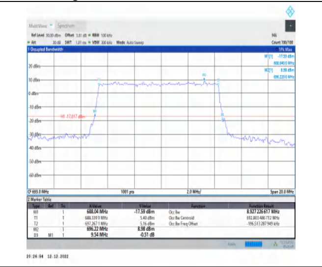
1-N71-15-10-H-5-DFT-256QAM-Outer_Full-50@0-A nt1-8.927-9.540-≤10-PASS
