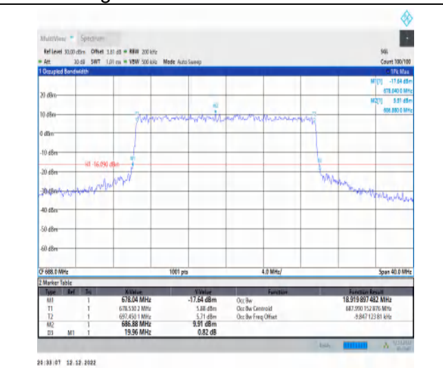
1-N71-15-20-H-7-CP-16QAM-Outer_Full-106@0-Ant 1-18.92-19.960-≤20-PASS
