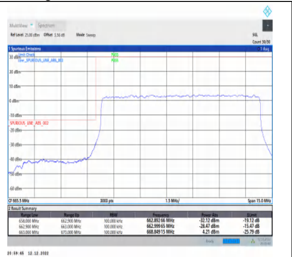
1-N71-15-10-L-3-DFT-PI2BPSK-Outer_Full-50@0-Ant1-1--PASS-see graph
