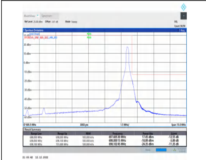
1-N71-15-10-H-5-CP-QPSK-Edge_1RB_Right-1@51-Ant1-1--PASS-see graph
