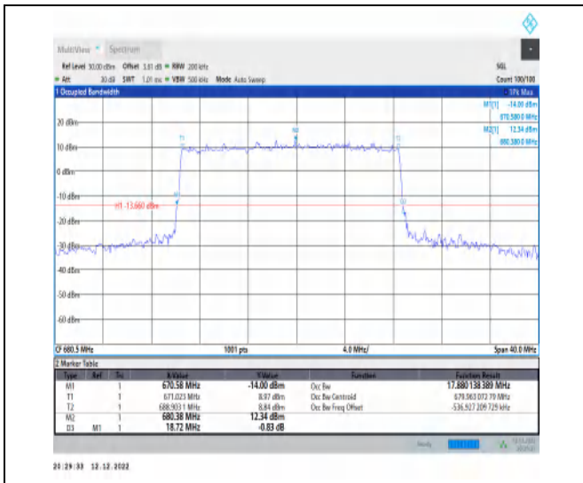
1-N71-15-20-M-3-DFT-16QAM-Outer_Full-100@0-A nt1-17.88-18.720-≤20-PASS
