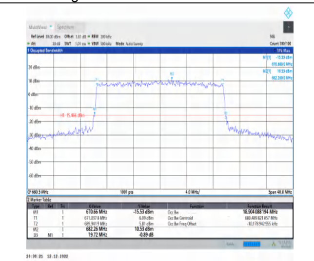
1-N71-15-20-M-8-CP-64QAM-Outer_Full-106@0-Ant 1-18.904-19.720-≤20-PASS
