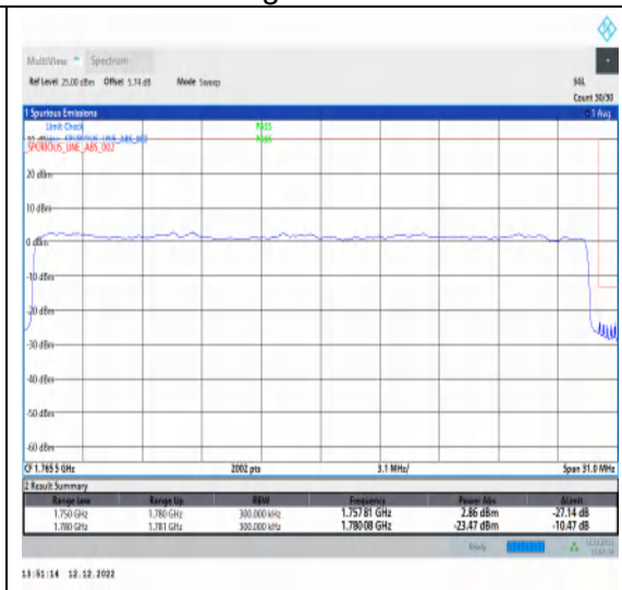
1-N66-15-30-H-3-DFT-PI2BPSK-Outer_Full-160@0-Ant1-1-seegraph-PASS-see graph
