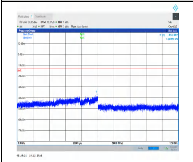
1-N66-15-40-M-1-DFT-PI2BPSK-Inner_1RB_Left-1 @ 1-3000-12000-Ant1-7462.65--37.85--13-PASS
