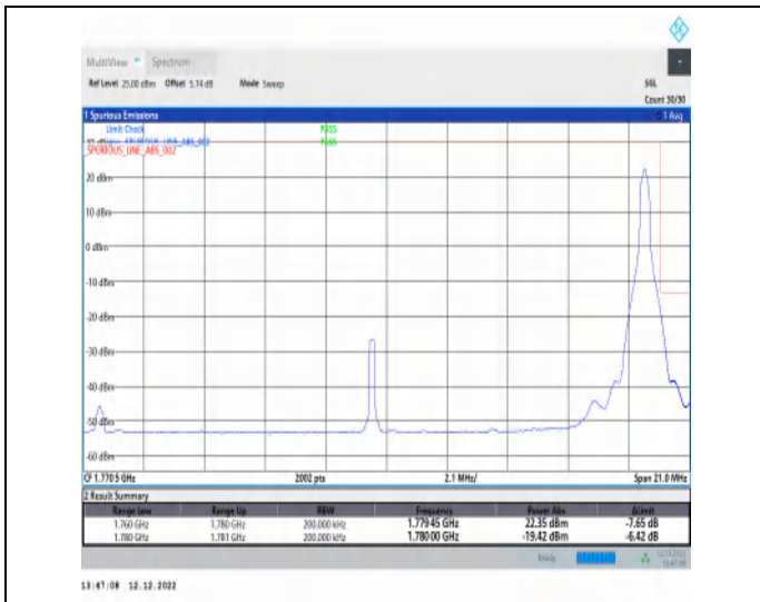
1-N66-15-20-H-2-DFT-PI2BPSK-Edge_1RB_Right-1@105-Ant1-1-seegraph-PASS-see graph
