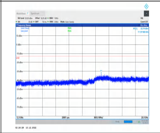
1-N66-15-40-M-1-DFT-PI2BPSK-Inner_1RB_Left-1 @ 1-12000-20000-Ant1-17137.60--32.74--13-PASS
