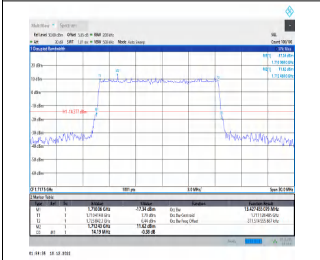
1-N66-15-15-L-5-DFT-256QAM-Outer_Full-75@0-Ant t1-13.427-14.190-≤15-PASS
