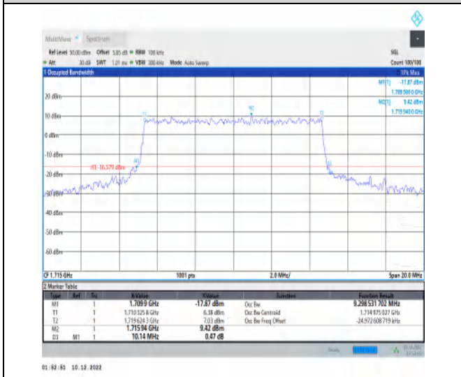
1-N66-15-10-L-8-CP-64QAM-Outer_Full-52@0-Ant1 -9.299-10.140-≤10-PASS
