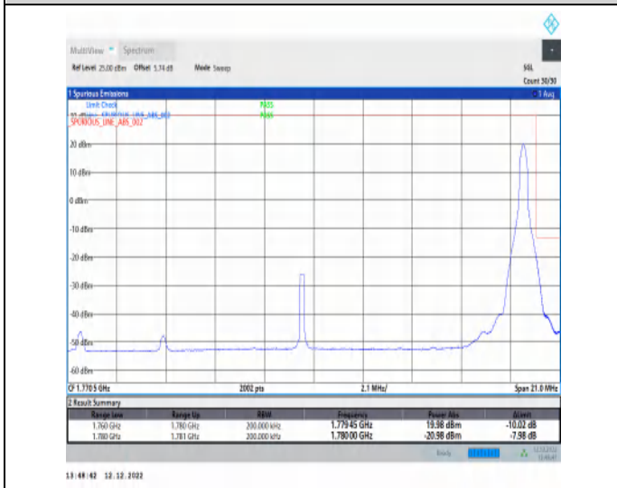
1-N66-15-20-H-5-CP-QPSK-Edge_1RB_Right-1@105-Ant1-1-seegraph-PASS-see graph
