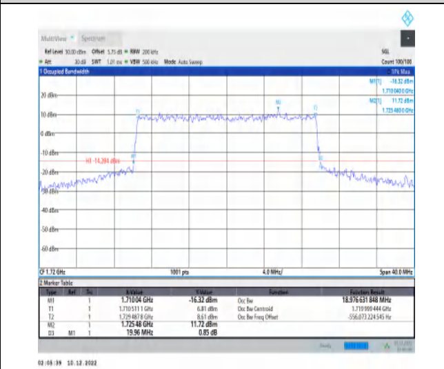
1-N66-15-20-L-7-CP-16QAM-Outer_Full-106@0-Ant 1-18.977-19.960-≤20-PASS
