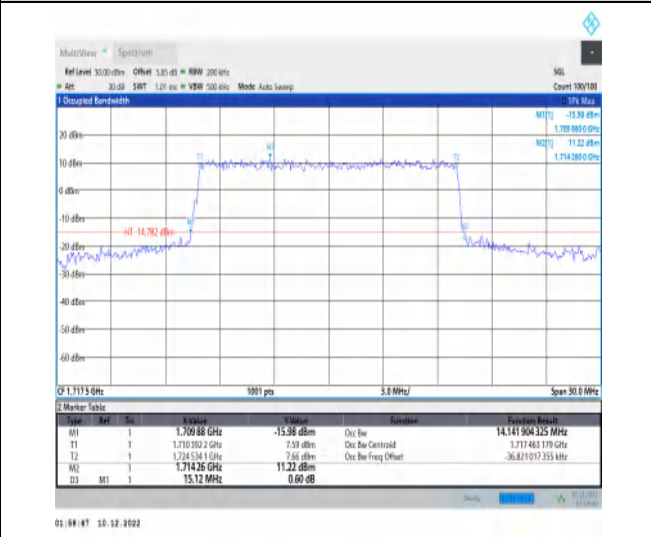
1-N66-15-15-L-6-CP-QPSK-Outer_Full-79@0-Ant1-1 4.142-15.120-≤15-PASS
