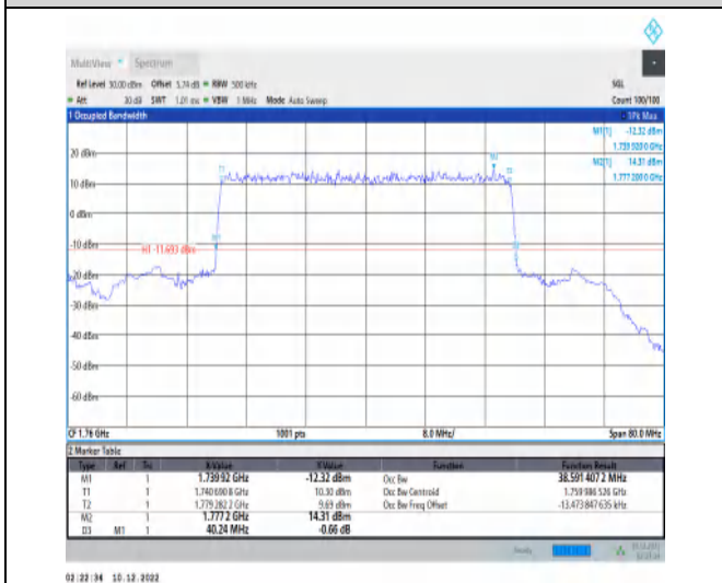
1-N66-15-40-H-2-DFT-PI2BPSK-Outer_Full-216@0-Ant1 1-38.591-40.240-≤40-PASS
