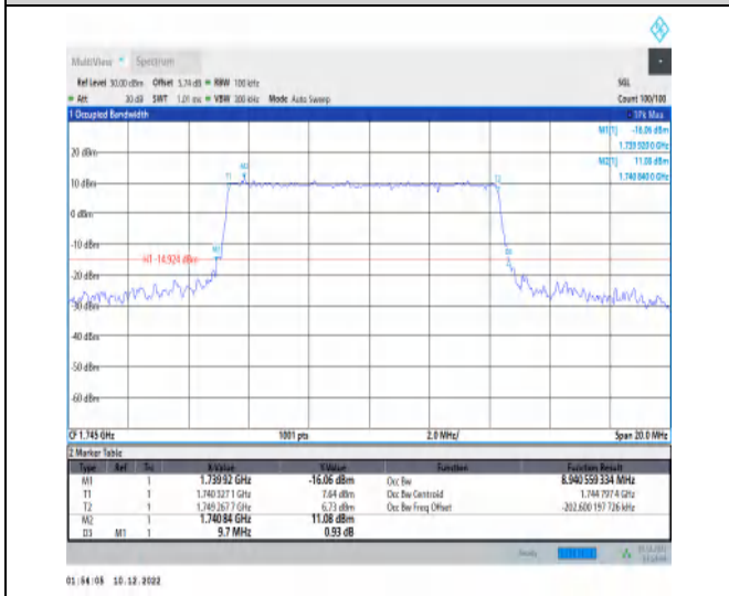
1-N66-15-10-M-3-DFT-16QAM-Outer_Full-50@0-Ant1 1-8.941-9.700-≤10-PASS
