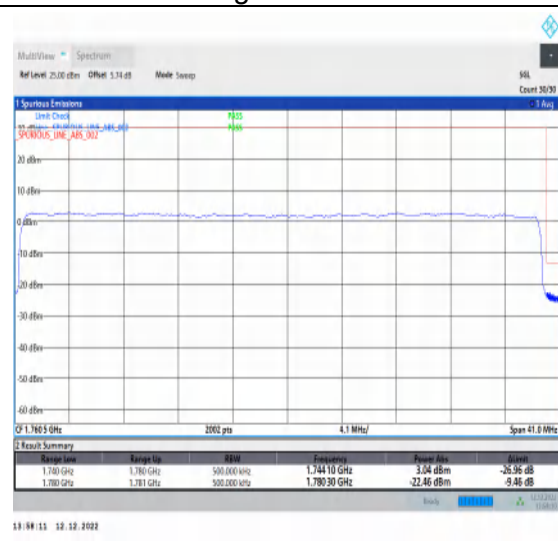
1-N66-15-40-H-3-DFT-PI2BPSK-Outer_Full-216@0-Ant1-1-seegraph-PASS-see graph
