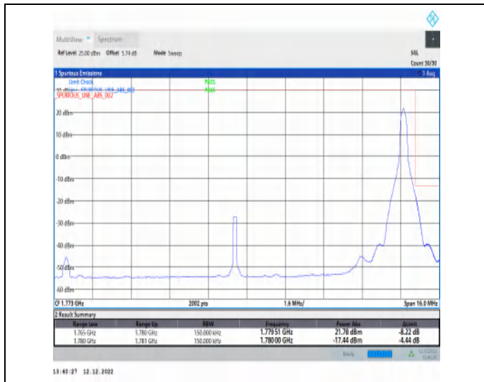
1-N66-15-15-H-2-DFT-PI2BPSK-Edge_1RB_Right-1@78-Ant1-1-seegraph-PASS-see graph
