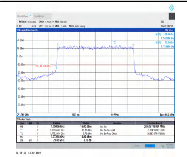
1-N66-15-30-H-2-DFT-PI2BPSK-Outer_Full-160@0-Ant Ant1-28.627-29.820-≤30-PASS
