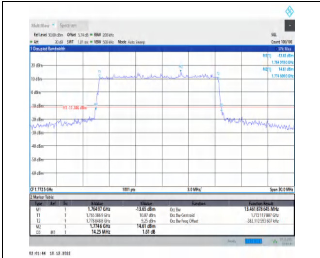
1-N66-15-15-H-1-DFT-QPSK-Outer_Full-75@0-Ant1 -13.462-14.250-≤15-PASS
