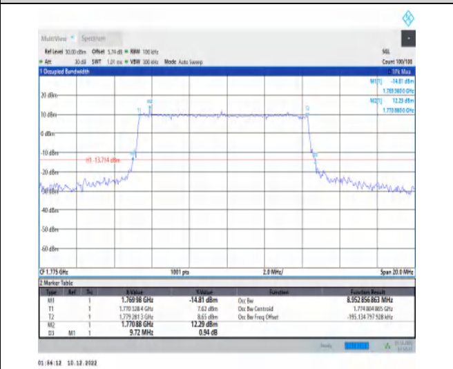
1-N66-15-10-H-3-DFT-16QAM-Outer_Full-50@0-Ant 1-8.953-9.720-≤10-PASS
