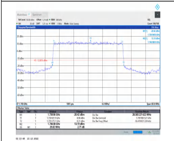
1-N66-15-30-M-2-DFT-PI2BPSK-Outer_Full-160@0-Ant1 Ant1-28.583-29.820-≤30-PASS
