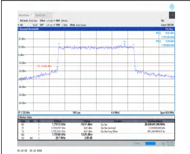
1-N66-15-30-L-3-DFT-16QAM-Outer_Full-160@0-Ant t1-28.639-29.700-≤30-PASS
