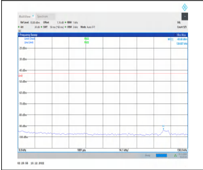
1-N66-15-40-M-1-DFT-PI2BPSK-Inner_1RB_Left-1 @ 1-0.009-0.15-Ant1-0.13--93.68--43-PASS
