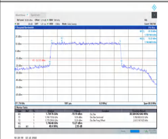
1-N66-15-40-H-3-DFT-16QAM-Outer_Full-216@0-A nt1-38.584-40.400-≤40-PASS
