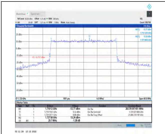
1-N66-15-30-L-1-DFT-QPSK-Outer_Full-160@0-Ant t1-28.571-29.700-≤30-PASS
