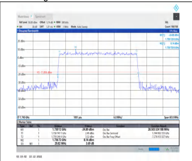
1-N66-15-30-M-9-CP-256QAM-Outer_Full-160@0-Ant nt1-28.503-29.820-≤30-PASS
