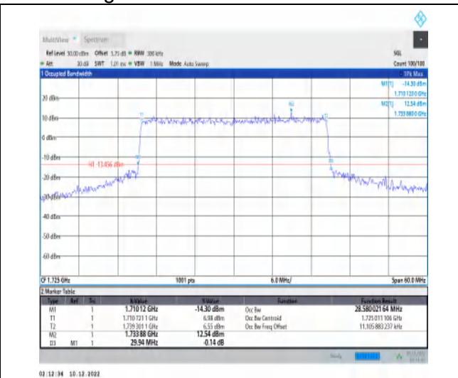
1-N66-15-30-L-6-CP-QPSK-Outer_Full-160@0-Ant1- 28.58-29.940-≤30-PASS
