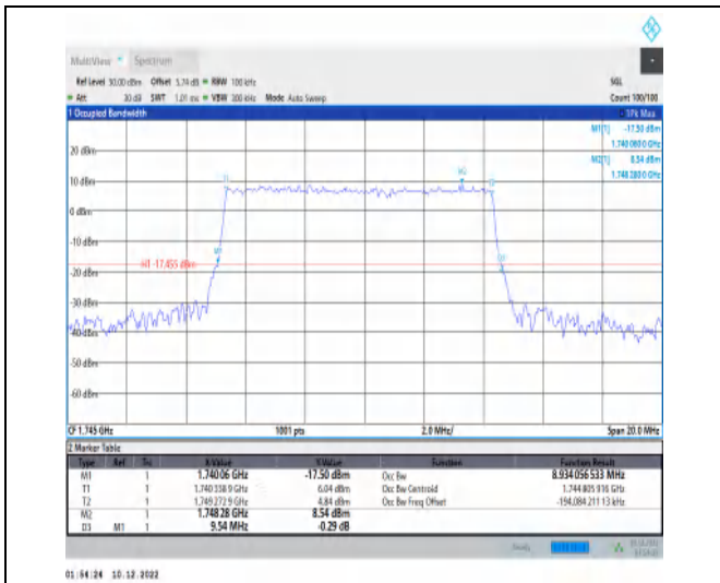
1-N66-15-10-M-5-DFT-256QAM-Outer_Full-50@0-A nt1-8.934-9.540≤10-PASS
