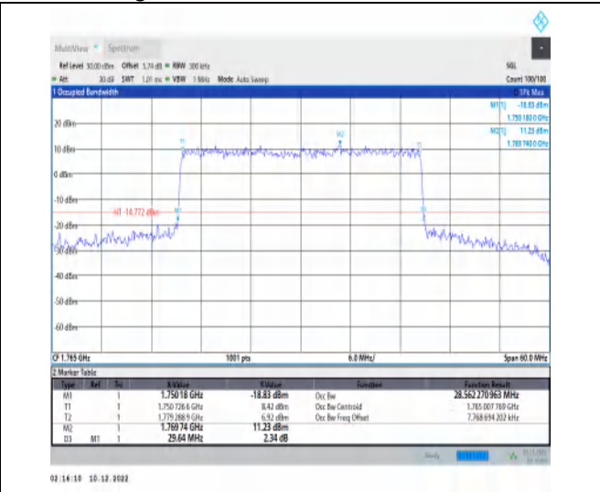
1-N66-15-30-H-4-DFT-64QAM-Outer_Full-160@0-A nt1-28.562-29.640-≤30-PASS
