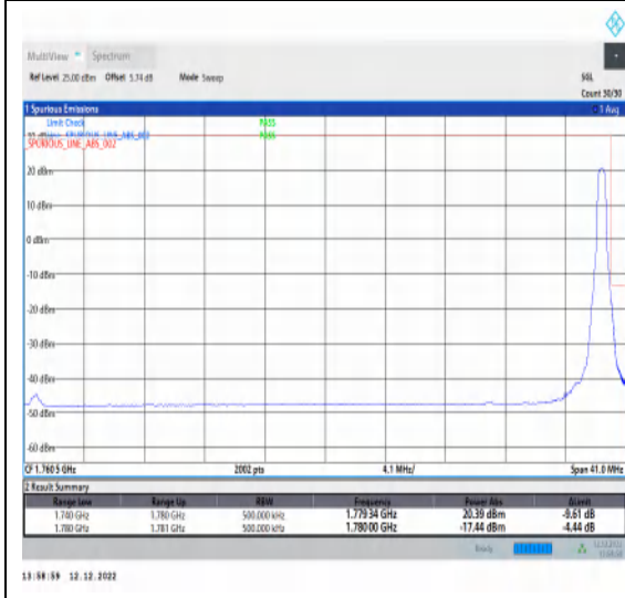
1-N66-15-40-H-5-CP-QPSK-Edge_1RB_Right-1@215-Ant1-1-seegraph-PASS-see graph
