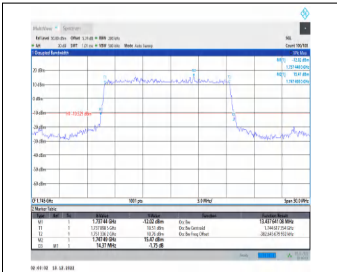
1-N66-15-15-M-2-DFT-PI2BPSK-Outer_Full-75@0-A nt1-13.438-14.370-≤15-PASS
