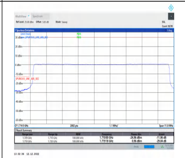
1-N66-15-10-L-6-CP-QPSK-Outer_Full-52@0-Ant1-1-seegraph-PASS-see graph
