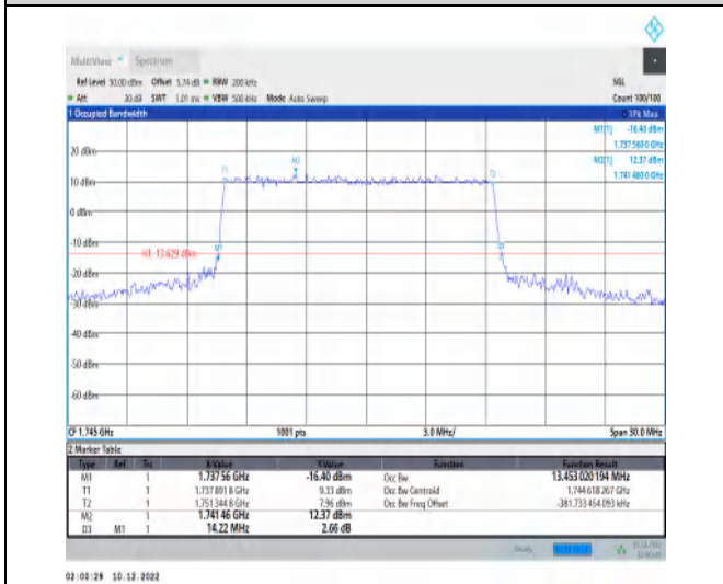
1-N66-15-15-M-4-DFT-64QAM-Outer_Full-75@0-Ant 1-13.453-14.220-≤15-PASS
