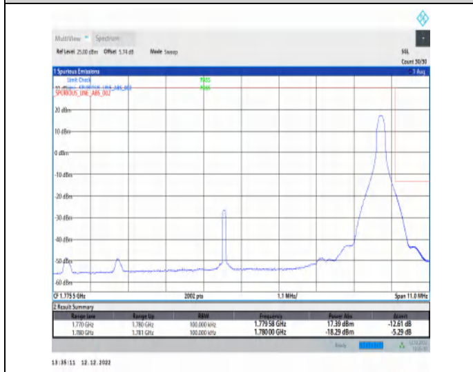
1-N66-15-10-H-5-CP-QPSK-Edge_1RB_Right-1@51-Ant1-1-seegraph-PASS-see graph
