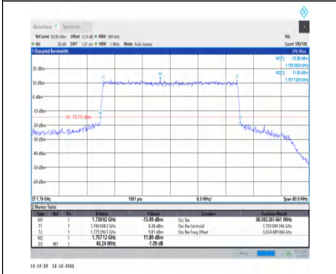
1-N66-15-40-H-6-CP-QPSK-Outer_Full-216@0-Ant1 -38.592-40.240-≤40-PASS
