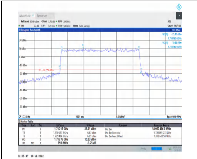
1-N66-15-20-L-8-CP-64QAM-Outer_Full-106@0-Ant 1-18.967-19.800-≤20-PASS
