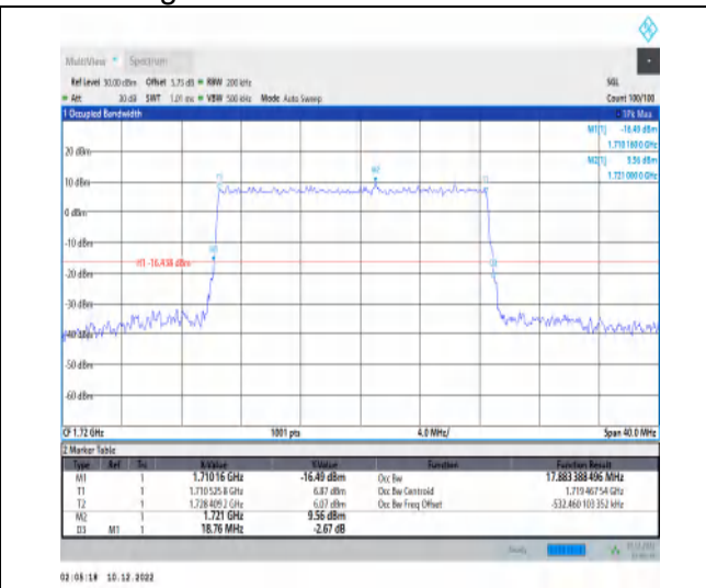
1-N66-15-20-L-5-DFT-256QAM-Outer_Full-100@0-A nt1-17.883-18.760-≤20-PASS
