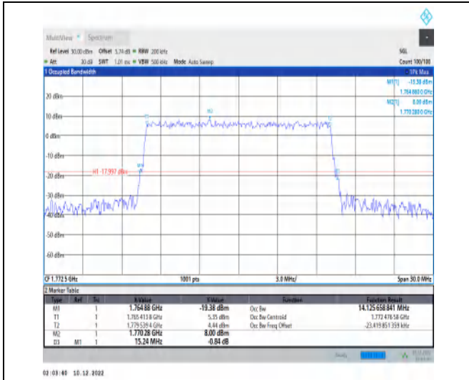
1-N66-15-15-H-9-CP-256QAM-Outer_Full-79@0-Ant 1-14.126-15.240-≤15-PASS
