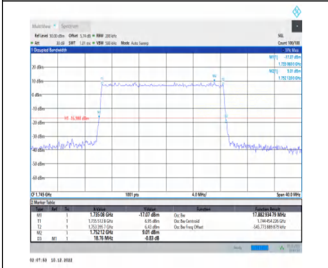
1-N66-15-20-M-5-DFT-256QAM-Outer_Full-100@0-A Ant1-17.883-18.760-≤20-PASS
