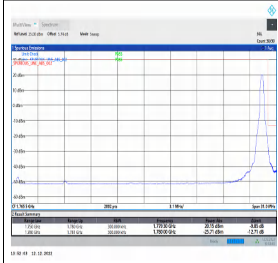
1-N66-15-30-H-5-CP-QPSK-Edge_1RB_Right-1@159-Ant1-1-seegraph-PASS-see graph
