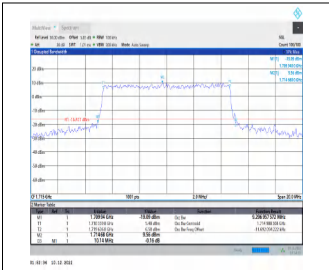
1-N66-15-10-L-6-CP-QPSK-Outer_Full-52@0-Ant1-9 .297-10.140-≤10-PASS
