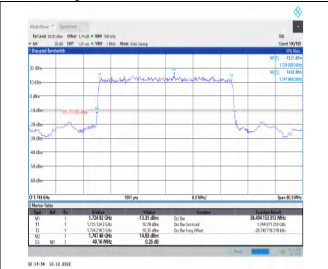
1-N66-15-40-M-2-DFT-PI2BPSK-Outer_Full-216@0-Ant 1-38.494-40.160-≤40-PASS
