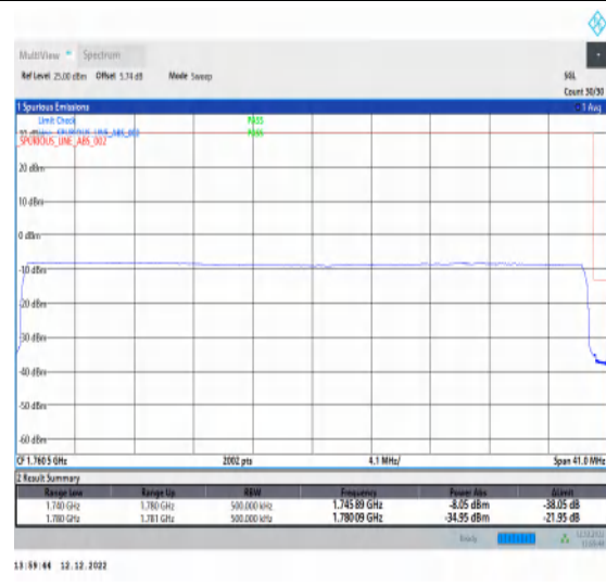
1-N66-15-40-H-6-CP-QPSK-Outer_Full-216@0-Ant1-1-seegraph-PASS-see graph
