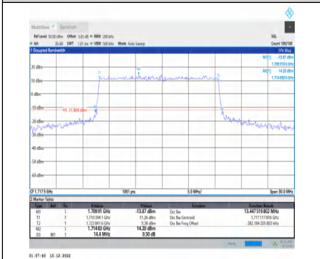
1-N66-15-15-L-1-DFT-QPSK-Outer_Full-75@0-Ant1- 13.448-14.400-≤15-PASS
