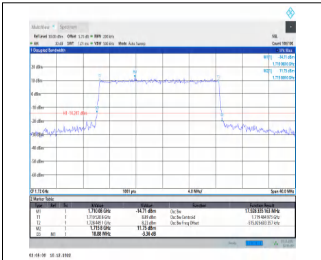
1-N66-15-20-L-4-DFT-64QAM-Outer_Full-100@0-An t1-17.928-18.880-≤20-PASS
