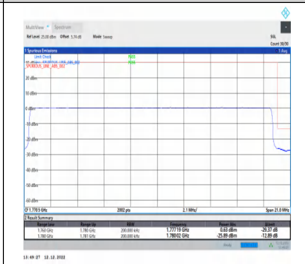
1-N66-15-20-H-6-CP-QPSK-Outer_Full-106@0-Ant1-1-seegraph-PASS-see graph
