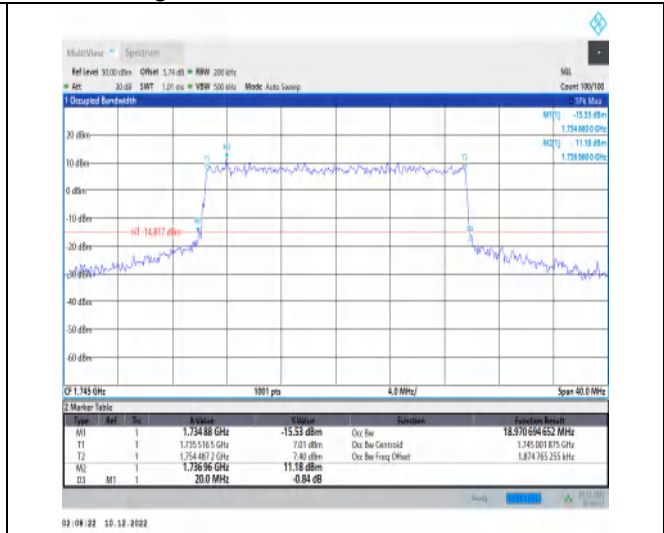
1-N66-15-20-M-8-CP-64QAM-Outer_Full-106@0-Ant 1-18.971-20.000-≤20-PASS
