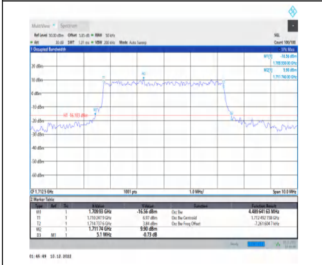
1-N66-15-5-L-7-CP-16QAM-Outer_Full-25@0-Ant1- 4.49-5.100-≤5-PASS
