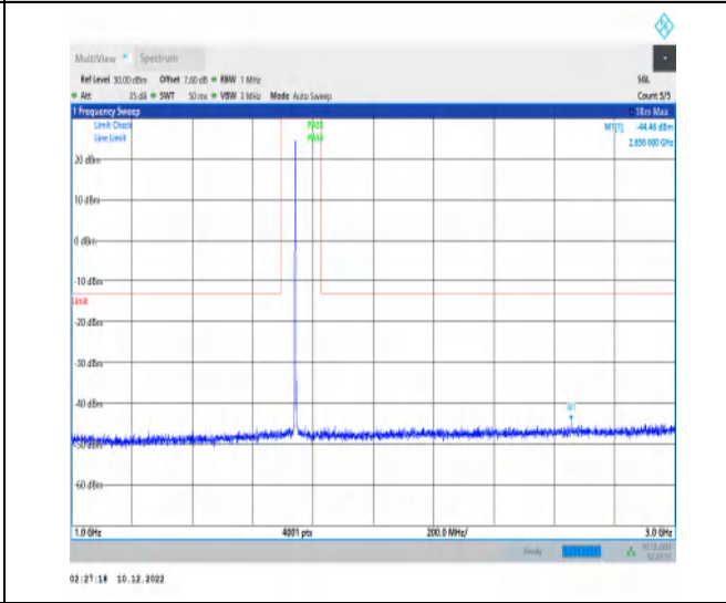
1-N66-15-40-H-1-DFT-PI2BPSK-Inner_1RB_Left-1 @ 1-1000-3000-Ant1-2656.00--44.46--13-PASS
