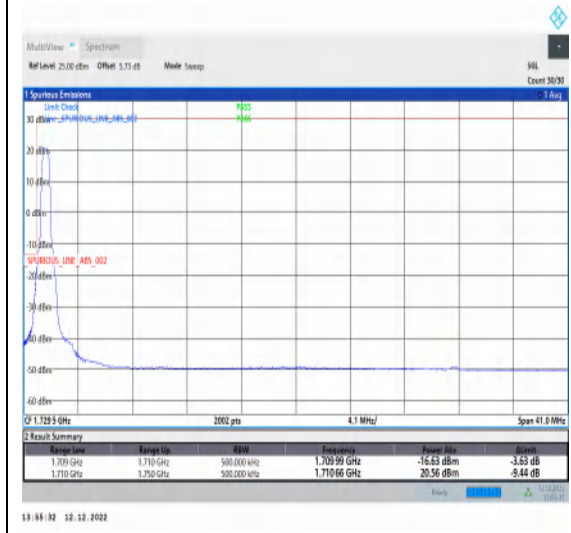
1-N66-15-40-L-4-CP-QPSK-Edge_1RB_Left-1@0-Ant1-1-seegraph-PASS-see graph
