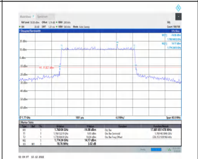
1-N66-15-20-H-1-DFT-QPSK-Outer_Full-100@0-Ant 1-17.882-18.760-≤20-PASS
