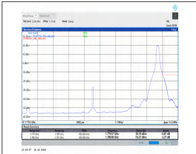
1-N66-15-10-H-2-DFT-PI2BPSK-Edge_1RB_Right-1@51-Ant1-1-seegraph-PASS-see graph
