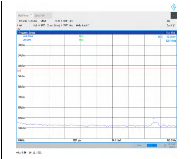
1-N66-15-40-H-1-DFT-PI2BPSK-Inner_1RB_Left-1 @ 1-0.009-0.15-Ant1-0.13--93.82--43-PASS
