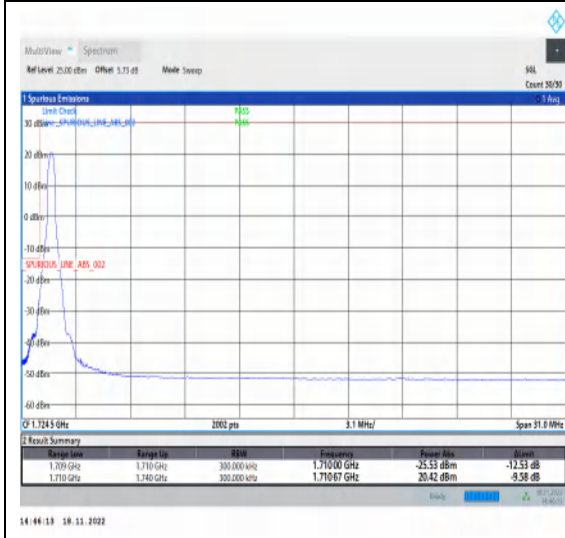
1-N66-PC3-15-30-L-4-CP-QPSK-Edge_1RB_Left-1@0-Ant1-1-seegraph-PASS-see graph
