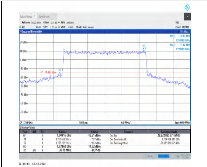
1-N66-15-30-H-7-CP-16QAM-Outer_Full-160@0-Ant 1-28.623-30.780-≤30-PASS
