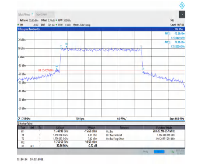
1-N66-15-30-H-6-CP-QPSK-Outer_Full-160@0-Ant1 -28.625-30.960-≤30-PASS
