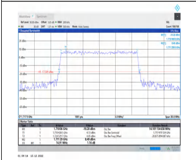
1-N66-15-15-L-9-CP-256QAM-Outer_Full-79@0-Ant 1-14.101-14.910-≤15-PASS
