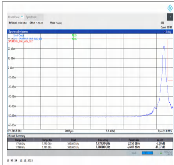
1-N66-15-30-H-2-DFT-PI2BPSK-Edge_1RB_Right-1@159-Ant1-1-seegraph-PASS-see graph
