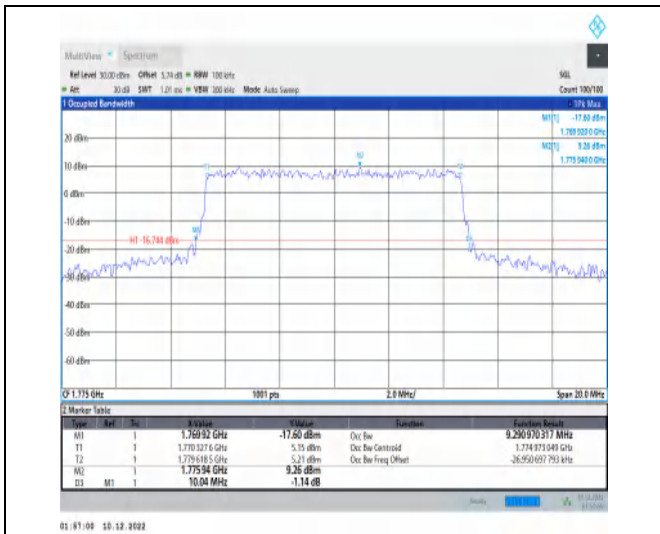
1-N66-15-10-H-8-CP-64QAM-Outer_Full-52@0-Ant1 -9.291-10.040-≤10-PASS
