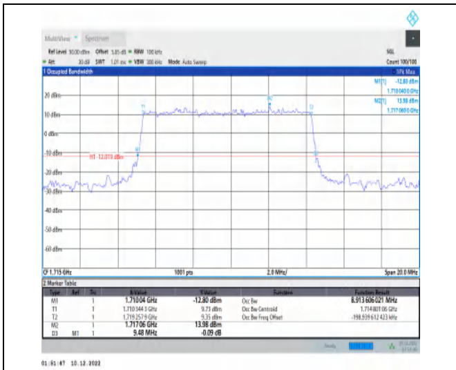
1-N66-15-10-L-2-DFT-PI2BPSK-Outer_Full-50@0-A nt1-8.914-9.480-≤10-PASS
