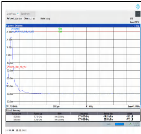
1-N66-15-40-L-1-DFT-PI2BPSK-Edge_1RB_Left-1@0-Ant1-1-seegraph-PASS-see graph
