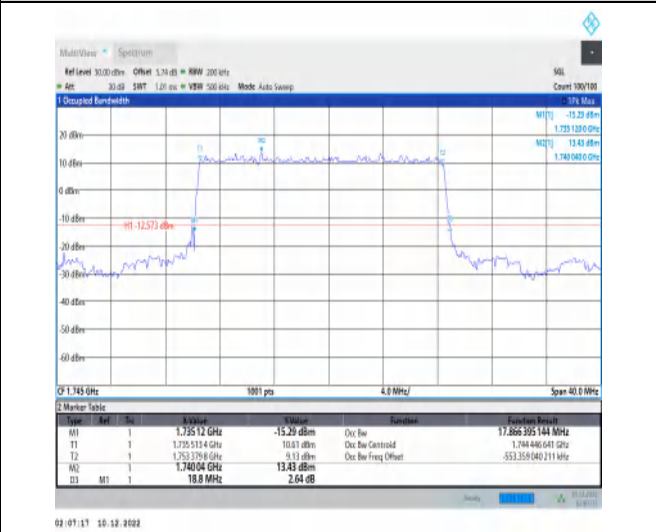
1-N66-15-20-M-2-DFT-PI2BPSK-Outer_Full-100@0-Ant Ant1-17.866-18.800-≤20-PASS
