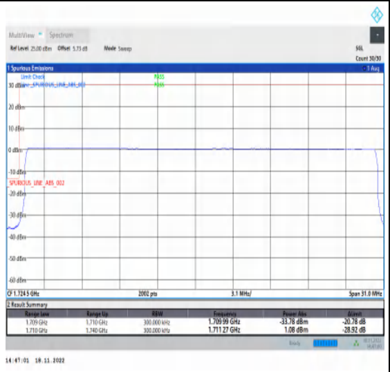
1-N66-PC3-15-30-L-6-CP-QPSK-Outer_Full-160@0-Ant1-1-seegraph-PASS-see graph
