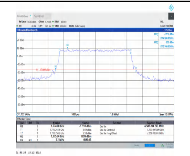
1-N66-15-5-H-6-CP-QPSK-Outer_Full-25@0-Ant1-4. 507-5.100≤5-PASS
