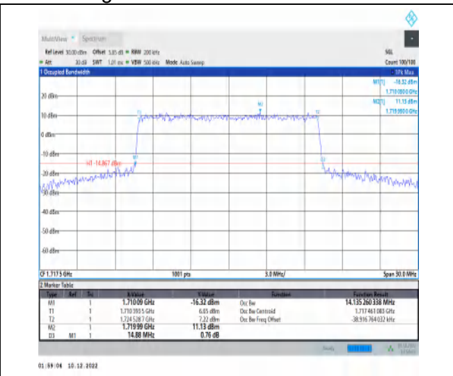
1-N66-15-15-L-8-CP-64QAM-Outer_Full-79@0-Ant1 -14.135-14.880-≤15-PASS
