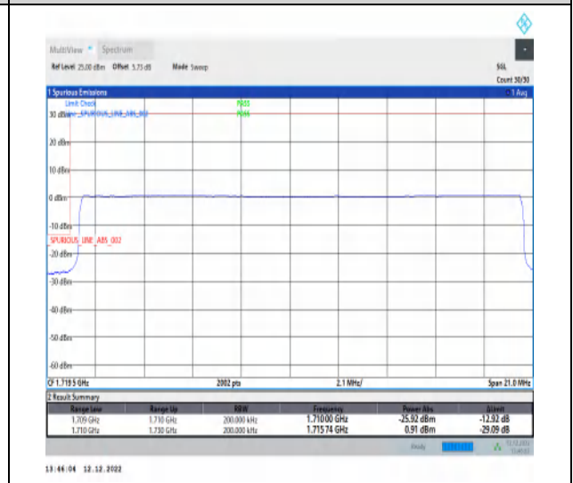
1-N66-15-20-L-6-CP-QPSK-Outer_Full-106@0-Ant1-1-seegraph-PASS-see graph
