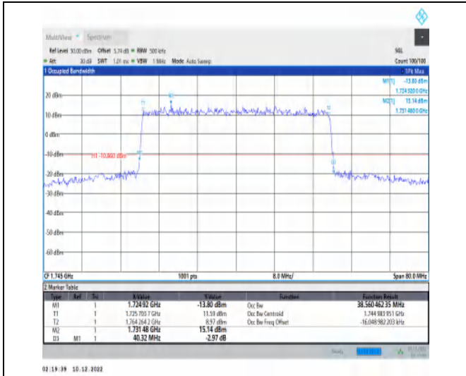
1-N66-15-40-M-1-DFT-QPSK-Outer_Full-216@0-Ant 1-38.56-40.320-≤40-PASS
