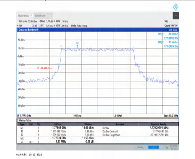
1-N66-15-5-H-4-DFT-64QAM-Outer_Full-25@0-Ant1 -4.476-4.970≤5-PASS
