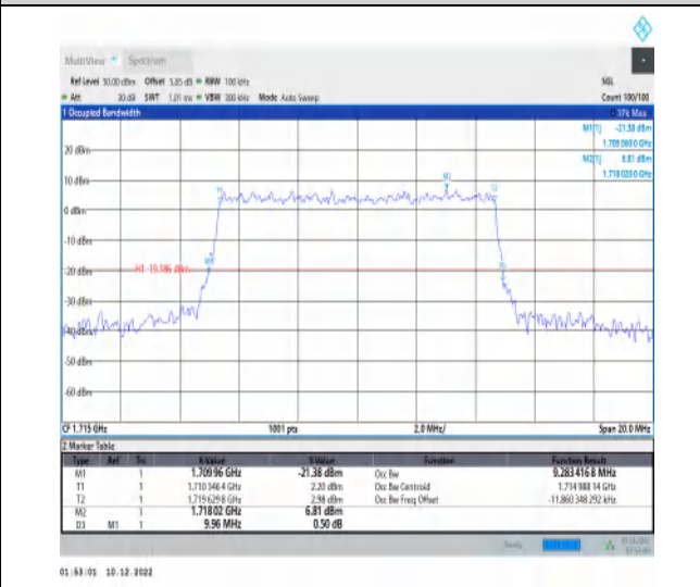
1-N66-15-10-L-9-CP-256QAM-Outer_Full-52@0-Ant 1-9.283-9.960-≤10-PASS
