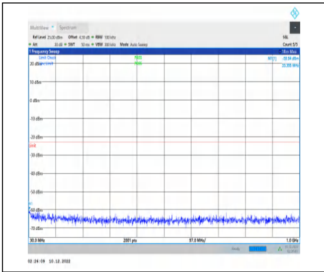
1-N66-15-40-M-1-DFT-PI2BPSK-Inner_1RB_Left-1 @ 1-30-1000-Ant1-33.40--59.94--23-PASS
