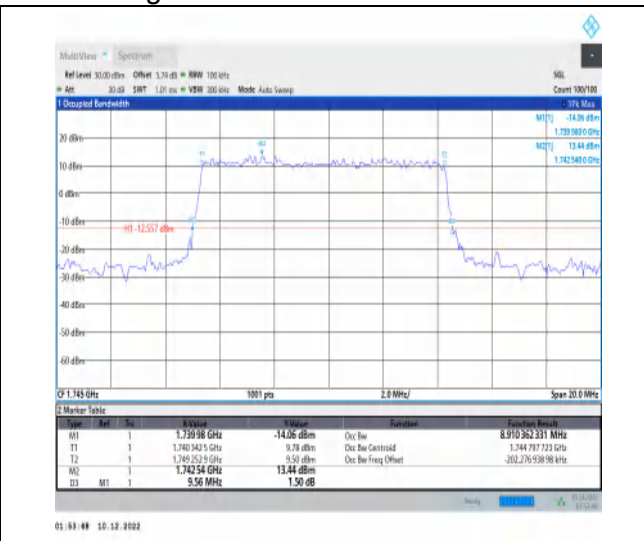
1-N66-15-10-M-2-DFT-PI2BPSK-Outer_Full-50@0-Ant1 -8.91-9.560-≤10-PASS
