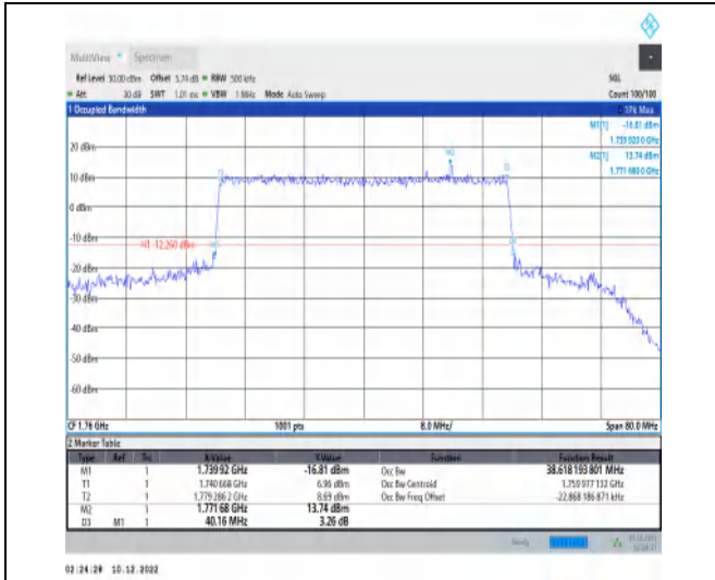
1-N66-15-40-H-8-CP-64QAM-Outer_Full-216@0-Ant 1-38.618-40.160-≤40-PASS
