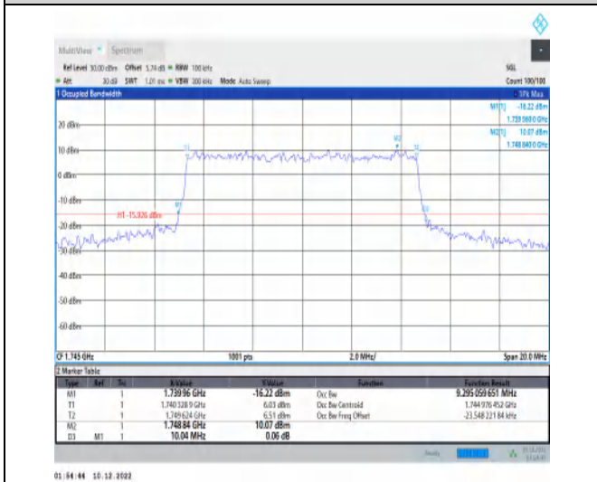
1-N66-15-10-M-7-CP-16QAM-Outer_Full-52@0-Ant1 -9.295-10.040≤10-PASS
