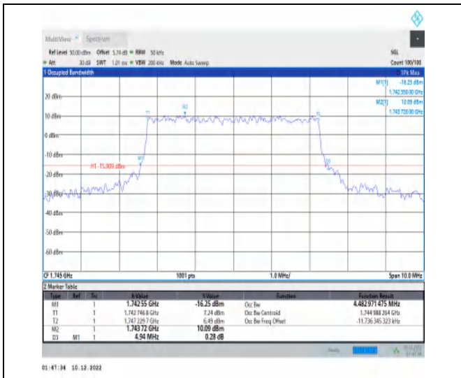
1-N66-15-5-M-4-DFT-64QAM-Outer_Full-25@0-Ant1 -4.483-4.940-≤5-PASS
