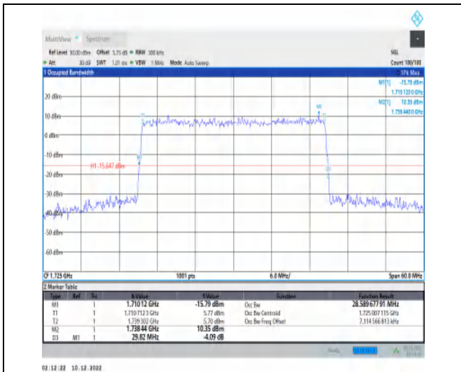
1-N66-15-30-L-5-DFT-256QAM-Outer_Full-160@0-A nt1-28.59-29.820-≤30-PASS
