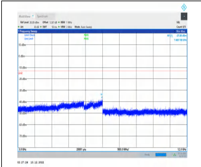
1-N66-15-40-H-1-DFT-PI2BPSK-Inner_1RB_Left-1 @1-3000-12000-Ant1-7463.10--37.00--13-PASS
