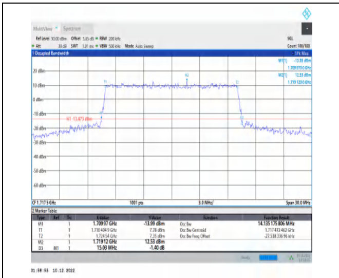
1-N66-15-15-L-7-CP-16QAM-Outer_Full-79@0-Ant1 -14.135-15.030-≤15-PASS
