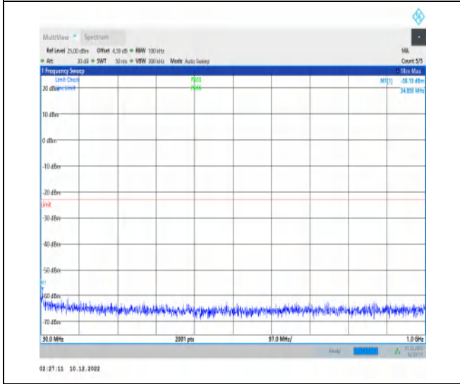
1-N66-15-40-H-1-DFT-PI2BPSK-Inner_1RB_Left-1 @ 1-30-1000-Ant1-34.85--58.19--23-PASS
