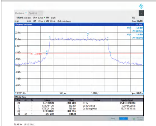
1-N66-15-5-H-1-DFT-QPSK-Outer_Full-25@0-Ant1-4.479-4.970-≤5-PASS
