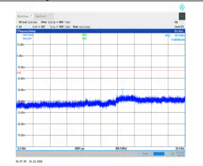
1-N66-15-40-H-1-DFT-PI2BPSK-Inner_1RB_Left-1 @ 1-12000-20000-Ant1-17038.80--33.16--13-PASS
