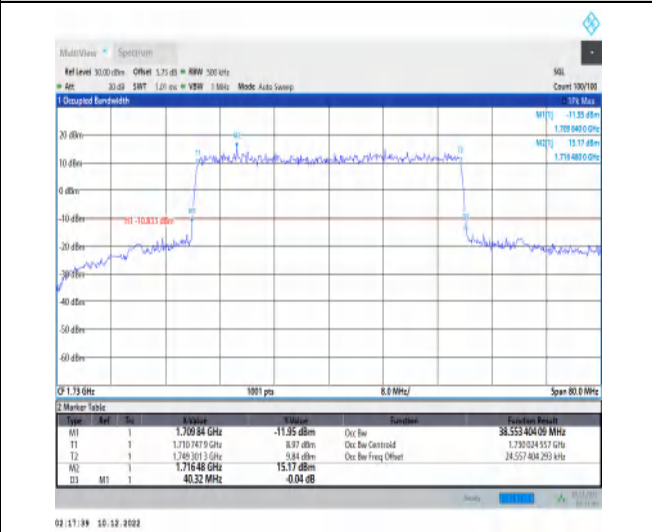
1-N66-15-40-L-1-DFT-QPSK-Outer_Full-216@0-Ant 1-38.553-40.320-≤40-PASS
