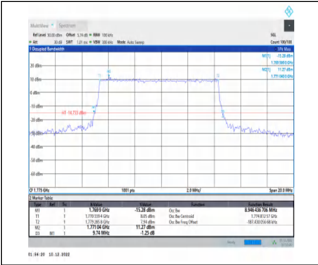
1-N66-15-10-H-4-DFT-64QAM-Outer_Full-50@0-Ant 1-8.946-9.740-≤10-PASS
