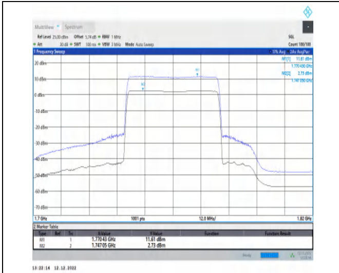
1-N66-15-40-H-1-DFT-256QAM-Outer_Full-216@0-A nt1-8.88-100%-0.00-8.88-PASS-≤13
