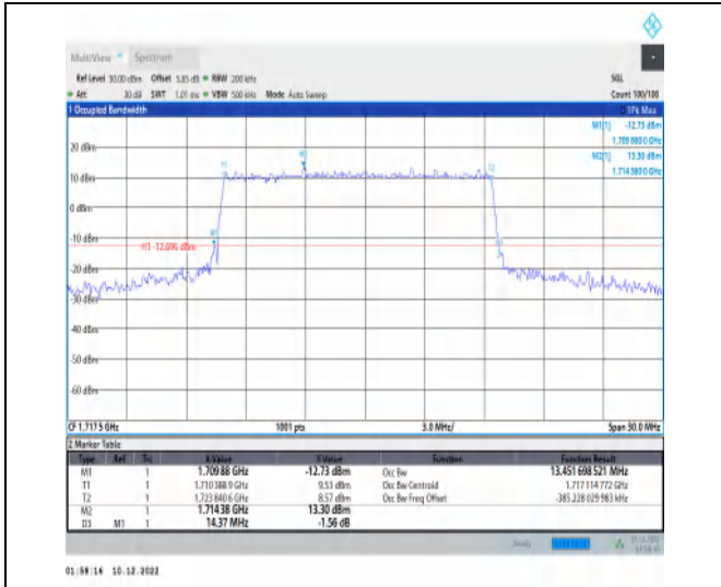
1-N66-15-15-L-3-DFT-16QAM-Outer_Full-75@0-Ant t1-13.452-14.370-≤15-PASS
