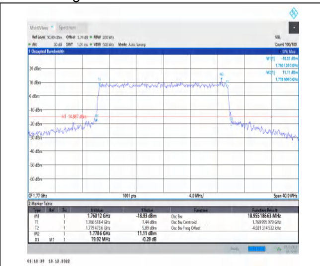
1-N66-15-20-H-7-CP-16QAM-Outer_Full-106@0-Ant 1-18.955-19.920-≤20-PASS
