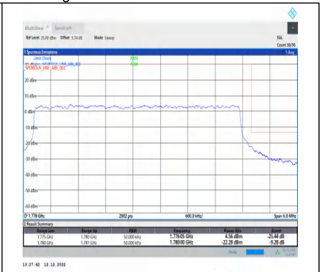
1-N66-15-5-H-3-DFT-PI2BPSK-Outer_Full-25@0-Ant1-1-seegraph-PASS-see graph
