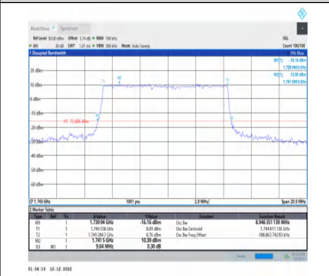
1-N66-15-10-M-4-DFT-64QAM-Outer_Full-50@0-Ant1 1-8.946-9.640-≤10-PASS
