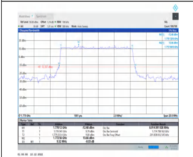
1-N66-15-10-H-2-DFT-PI2BPSK-Outer_Full-50@0-A nt1-8.914-9.520-≤10-PASS
