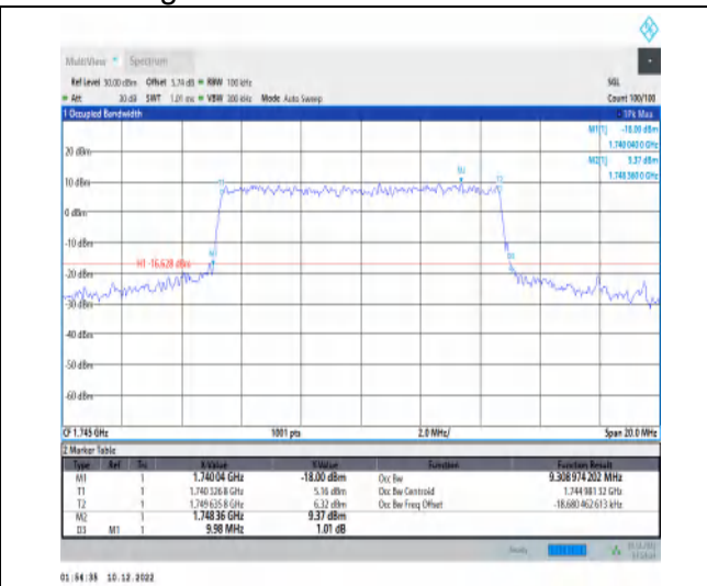
1-N66-15-10-M-6-CP-QPSK-Outer_Full-52@0-Ant1- 9.309-9.980≤10-PASS
