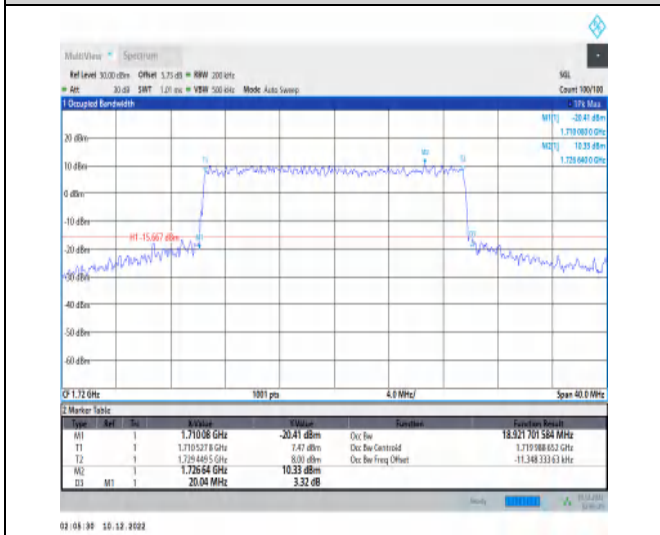
1-N66-15-20-L-6-CP-QPSK-Outer_Full-106@0-Ant1- 18.922-20.040-≤20-PASS
