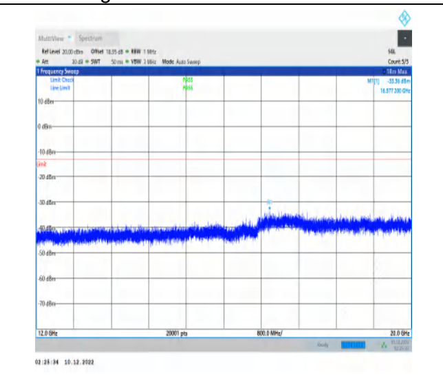
1-N66-15-40-L-1-DFT-PI2BPSK-Inner_1RB_Left-1@ 1-12000-20000-Ant1-16977.20--33.36--13-PASS
