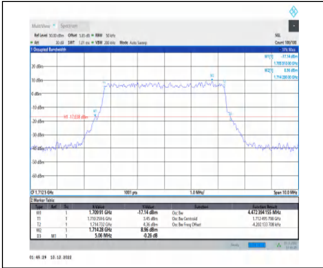
1-N66-15-5-L-5-DFT-256QAM-Outer_Full-25@0-Ant 1-4.472-5.060-≤5-PASS
