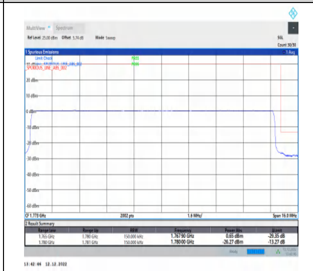
1-N66-15-15-H-6-CP-QPSK-Outer_Full-79@0-Ant1-1-seegraph-PASS-see graph
