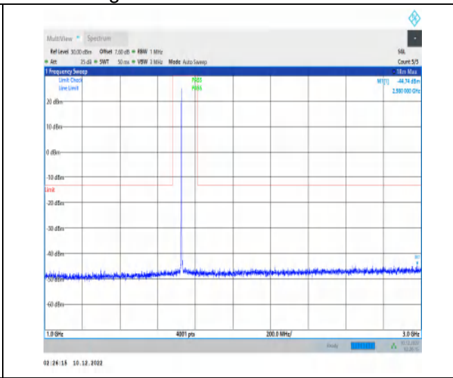
1-N66-15-40-M-1-DFT-PI2BPSK-Inner_1RB_Left-1 @ 1-1000-3000-Ant1-2980.00--44.74--13-PASS
