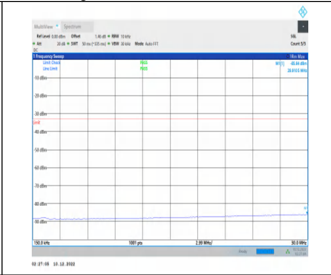
1-N66-15-40-H-1-DFT-PI2BPSK-Inner_1RB_Left-1 @ 1-0.15-30-Ant1-29.91--85.94--33-PASS
