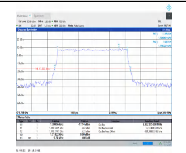
1-N66-15-10-L-5-DFT-256QAM-Outer_Full-50@0-Ant t1-8.932-9.740-≤10-PASS
