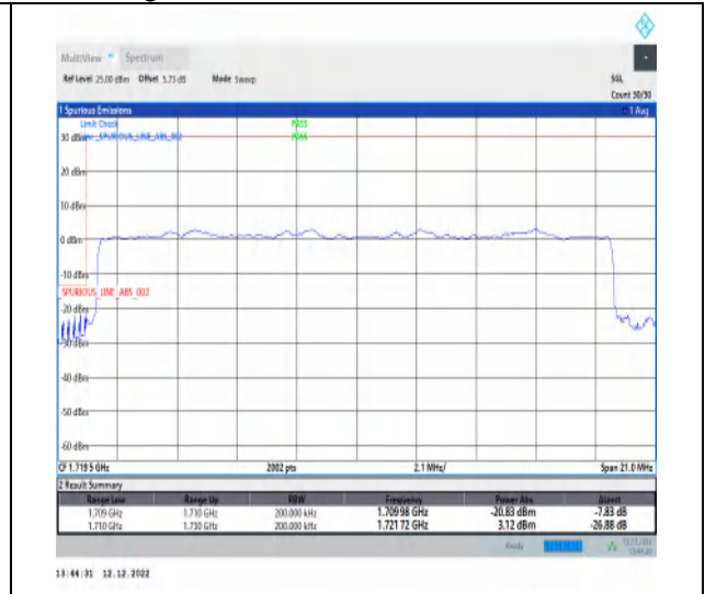
1-N66-15-20-L-3-DFT-PI2BPSK-Outer_Full-100@0-Ant1-1-seegraph-PASS-see graph
