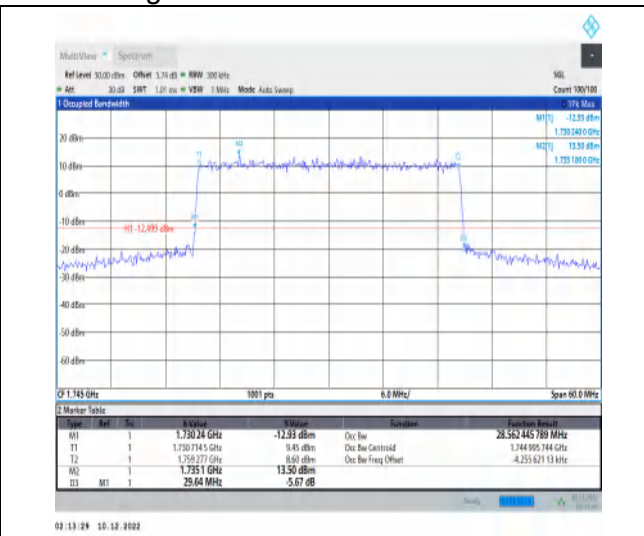
1-N66-15-30-M-1-DFT-QPSK-Outer_Full-160@0-Ant 1-28.562-29.640-≤30-PASS
