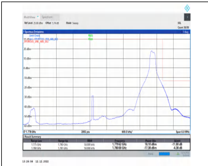
1-N66-15-5-H-2-DFT-PI2BPSK-Edge_1RB_Right-1@2-4-Ant1-1-seegraph-PASS-see graph
