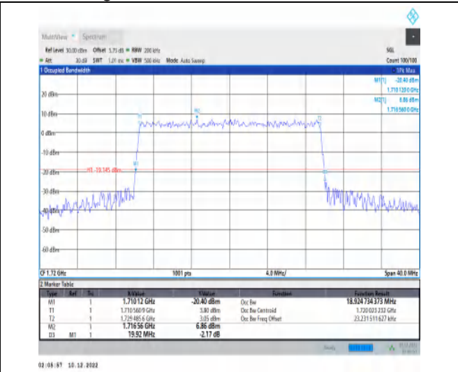
1-N66-15-20-L-9-CP-256QAM-Outer_Full-106@0-Ant t1-18.925-19.920-≤20-PASS
