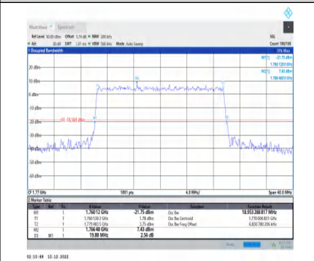
1-N66-15-20-H-9-CP-256QAM-Outer_Full-106@0-A nt1-18.953-19.880-≤20-PASS
