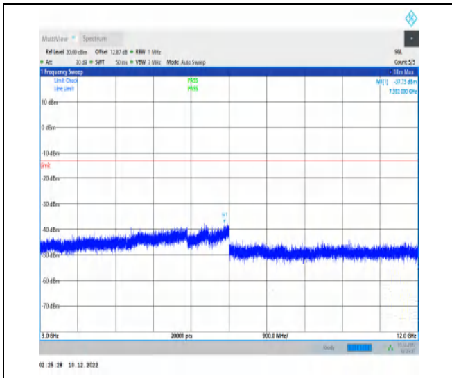
1-N66-15-40-L-1-DFT-PI2BPSK-Inner_1RB_Left-1 @ 1-3000-12000-Ant1-7392.00--37.73--13-PASS
