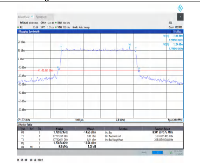
1-N66-15-10-H-1-DFT-QPSK-Outer_Full-50@0-Ant1 -8.941-9.800-≤10-PASS
