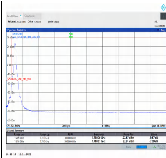
1-N66-PC3-15-30-L-1-DFT-PI2BPSK-Edge_1_RB_Left-1@0-Ant1-1-seegraph-PASS-see graph
