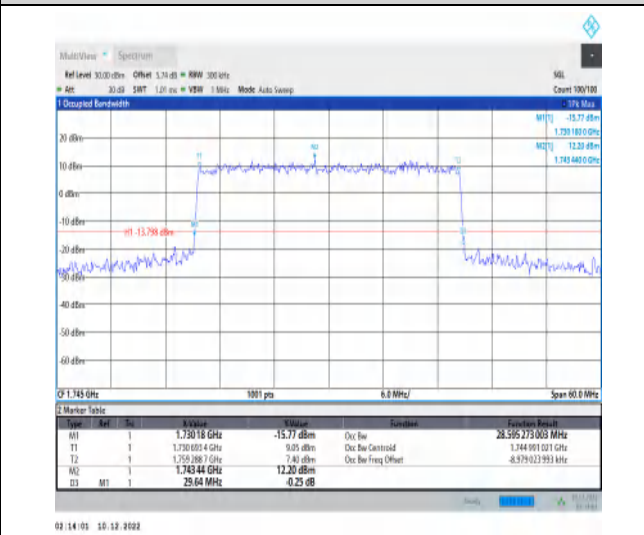
1-N66-15-30-M-3-DFT-16QAM-Outer_Full-160@0-A nt1-28.595-29.640-≤30-PASS
