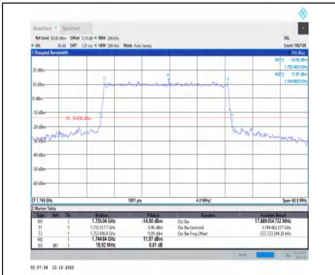
1-N66-15-20-M-3-DFT-16QAM-Outer_Full-100@0-A nt1-17.889-18.920-≤20-PASS
