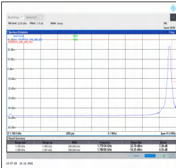
1-N66-15-40-H-2-DFT-PI2BPSK-Edge_1RB_Right-1@215-Ant1-1-seegraph-PASS-see graph
