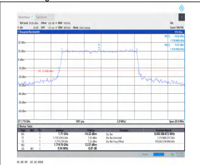
1-N66-15-10-L-3-DFT-16QAM-Outer_Full-50@0-Ant 1-8.943-9.540-≤10-PASS
