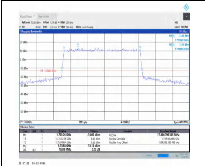
1-N66-15-20-M-1-DFT-QPSK-Outer_Full-100@0-Ant 1-17.887-18.880-≤20-PASS
