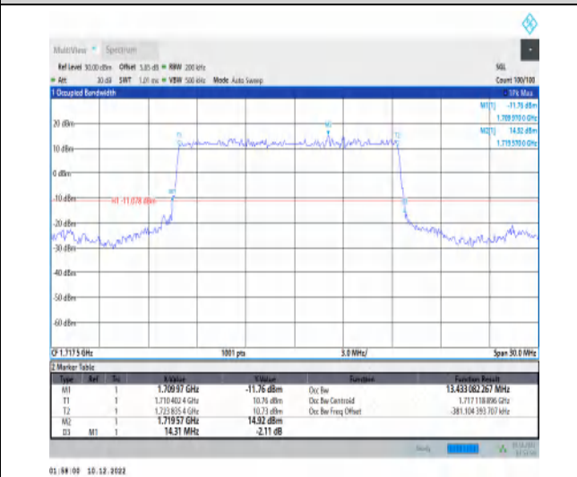
1-N66-15-15-L-2-DFT-PI2BPSK-Outer_Full-75@0-A nt1-13.433-14.310-≤15-PASS
