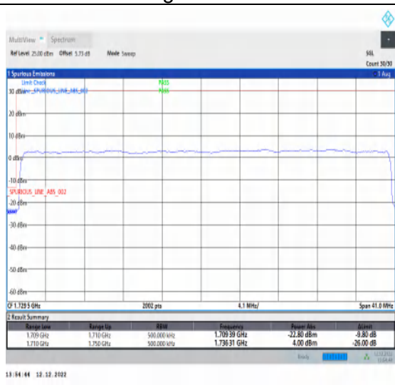
1-N66-15-40-L-3-DFT-PI2BPSK-Outer_Full-216@0-Ant1-1-seegraph-PASS-see graph
