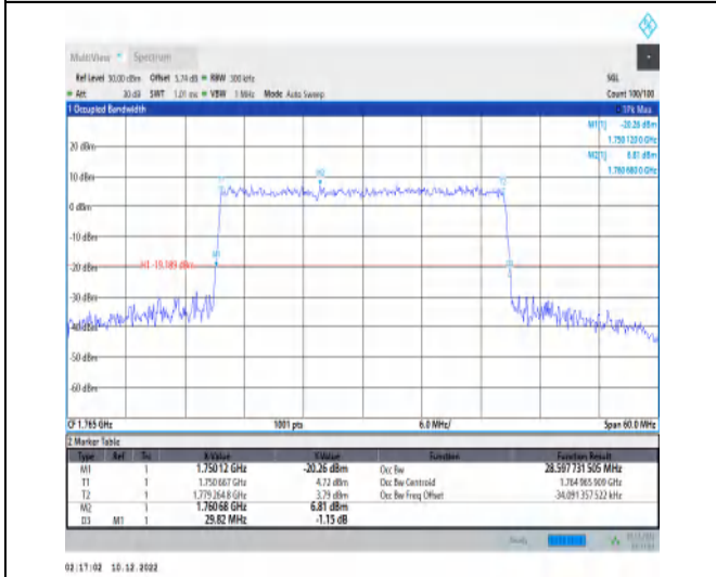
1-N66-15-30-H-9-CP-256QAM-Outer_Full-160@0-A nt1-28.598-29.820-≤30-PASS
