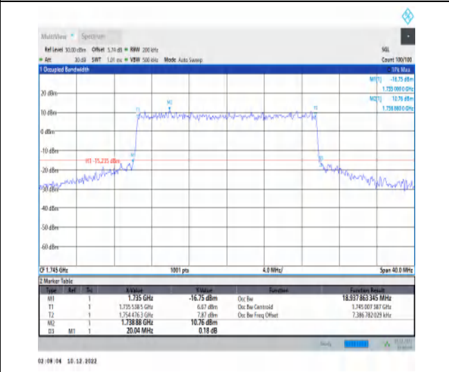
1-N66-15-20-M-6-CP-QPSK-Outer_Full-106@0-Ant1 -18.938-20.040-≤20-PASS
