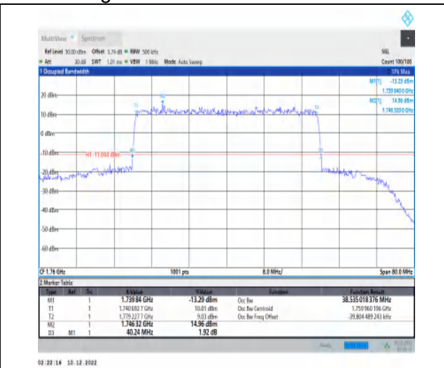
1-N66-15-40-H-1-DFT-QPSK-Outer_Full-216@0-Ant 1-38.535-40.240-≤40-PASS
