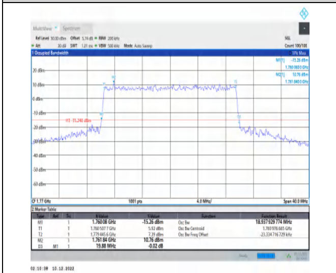
1-N66-15-20-H-8-CP-64QAM-Outer_Full-106@0-Ant 1-18.938-19.880-≤20-PASS
