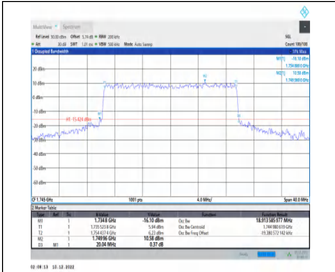
1-N66-15-20-M-7-CP-16QAM-Outer_Full-106@0-Ant 1-18.914-20.040-≤20-PASS
