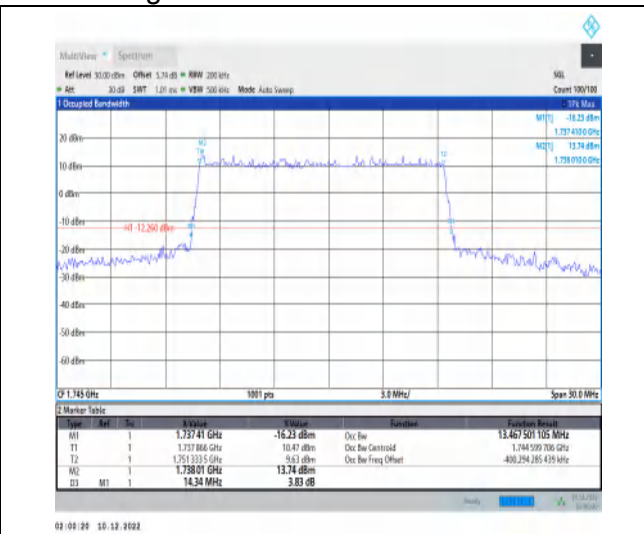
1-N66-15-15-M-3-DFT-16QAM-Outer_Full-75@0-Ant 1-13.468-14.340-≤15-PASS
