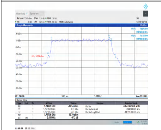
1-N66-15-5-M-2-DFT-PI2BPSK-Outer_Full-25@0-An t1-4.473-5.050-≤5-PASS
