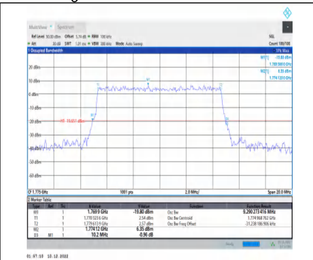
1-N66-15-10-H-9-CP-256QAM-Outer_Full-52@0-Ant1 1-9.29-10.200-≤10-PASS
