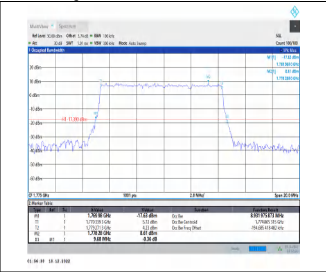
1-N66-15-10-H-5-DFT-256QAM-Outer_Full-50@0-A nt1-8.932-9.680-≤10-PASS
