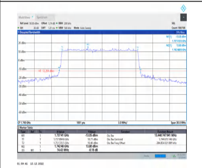
1-N66-15-15-M-1-DFT-QPSK-Outer_Full-75@0-Ant1 -13.441-14.430-≤15-PASS
