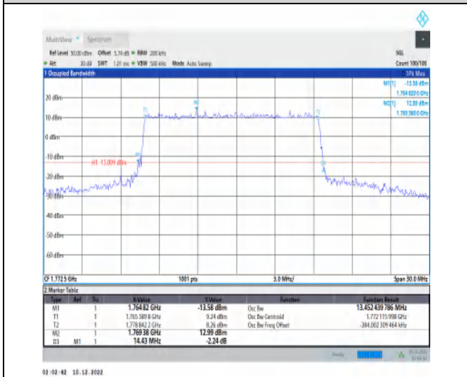
1-N66-15-15-H-3-DFT-16QAM-Outer_Full-75@0-Ant1 1-13.452-14.430-≤15-PASS
