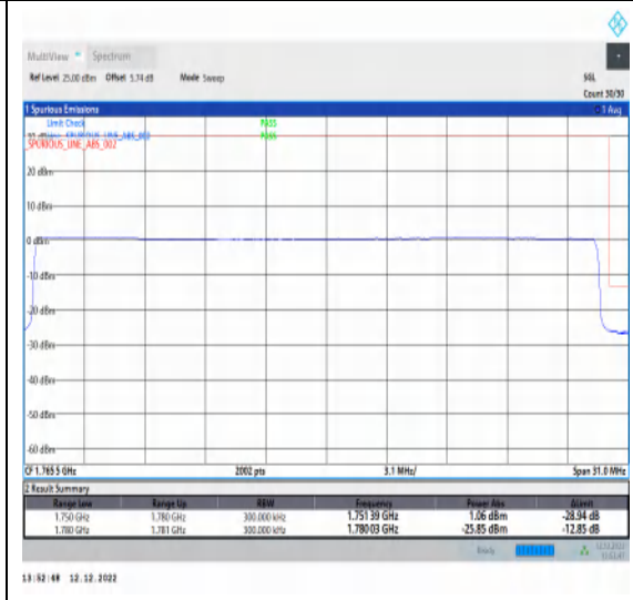
1-N66-15-30-H-6-CP-QPSK-Outer_Full-160@0-Ant1-1-seegraph-PASS-see graph
