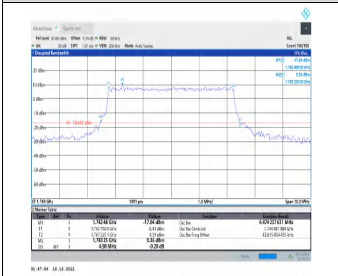
1-N66-15-5-M-6-CP-QPSK-Outer_Full-25@0-Ant1-4. 474-4.980-≤5-PASS
