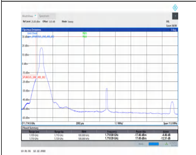
1-N66-15-10-L-4-CP-QPSK-Edge_1RB_Left-1@0-Ant1-1-seegraph-PASS-see graph
