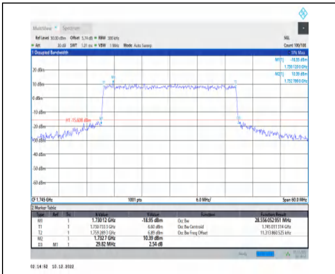
1-N66-15-30-M-8-CP-64QAM-Outer_Full-160@0-Ant 1-28.556-29.820-≤30-PASS
