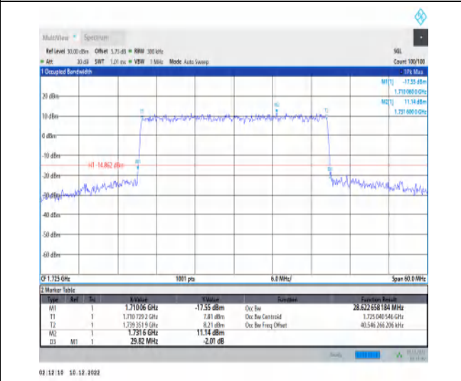
1-N66-15-30-L-4-DFT-64QAM-Outer_Full-160@0-Ant t1-28.623-29.820-≤30-PASS
