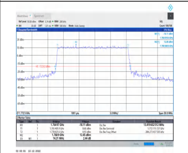
1-N66-15-15-H-4-DFT-64QAM-Outer_Full-75@0-Ant1 1-13.42-14.310-≤15-PASS
