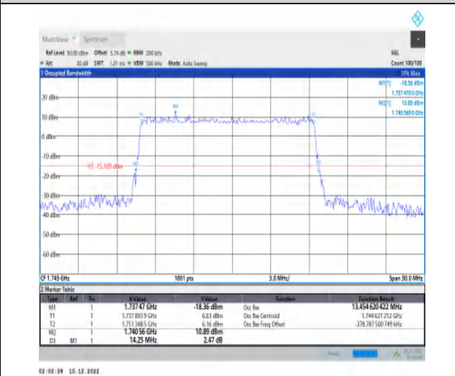
1-N66-15-15-M-5-DFT-256QAM-Outer_Full-75@0-A nt1-13.455-14.250-≤15-PASS
