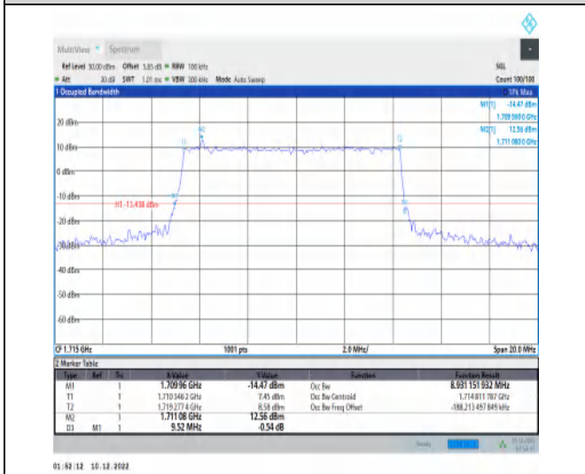
1-N66-15-10-L-4-DFT-64QAM-Outer_Full-50@0-Ant 1-8.931-9.520-≤10-PASS
