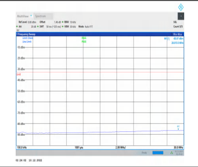
1-N66-15-40-M-1-DFT-PI2BPSK-Inner_1RB_Left-1@ 1-0.15-30-Ant1-29.01--85.97--33-PASS
