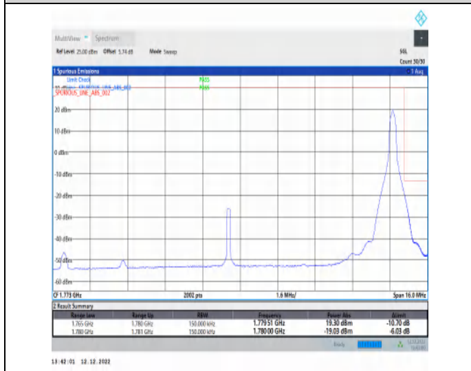
1-N66-15-15-H-5-CP-QPSK-Edge_1RB_Right-1@78-Ant1-1-seegraph-PASS-see graph
