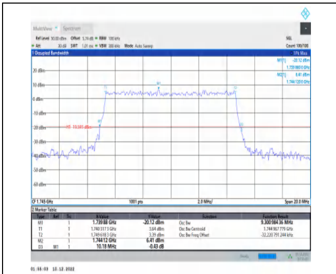
1-N66-15-10-M-9-CP-256QAM-Outer_Full-52@0-Ant 1-9.301-10.180-≤10-PASS
