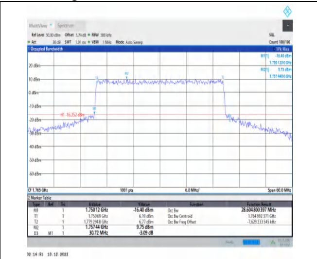
1-N66-15-30-H-8-CP-64QAM-Outer_Full-160@0-Ant 1-28.605-30.720-≤30-PASS
