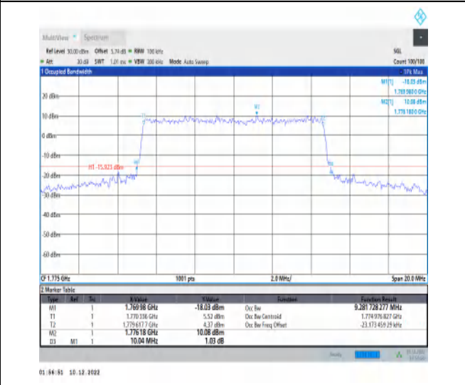
1-N66-15-10-H-7-CP-16QAM-Outer_Full-52@0-Ant1 -9.282-10.040-≤10-PASS
