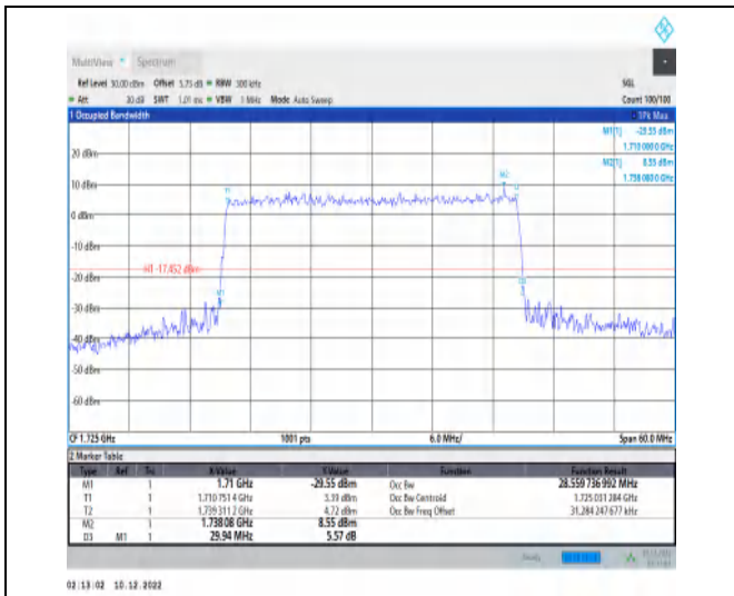
1-N66-15-30-L-9-CP-256QAM-Outer_Full-160@0-Ant t1-28.56-29.940-≤30-PASS
