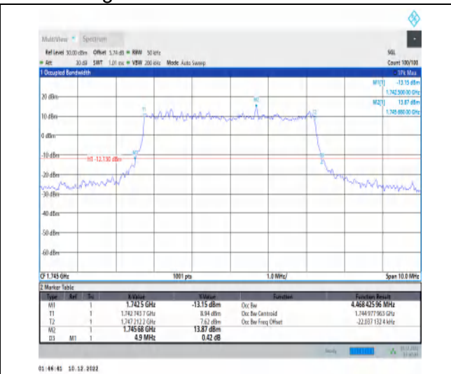
1-N66-15-5-M-1-DFT-QPSK-Outer_Full-25@0-Ant1- 4.468-4.900-≤5-PASS
