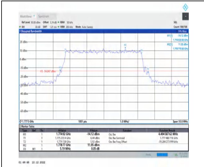
1-N66-15-5-H-3-DFT-16QAM-Outer_Full-25@0-Ant1 -4.495-5.190≤5-PASS
