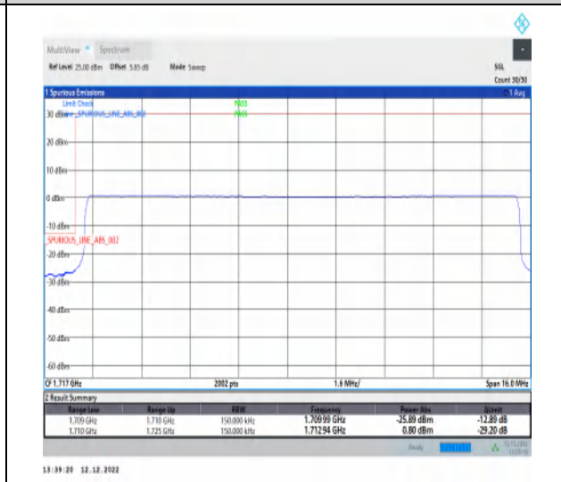
1-N66-15-15-L-6-CP-QPSK-Outer_Full-79@0-Ant1-1-seegraph-PASS-see graph
