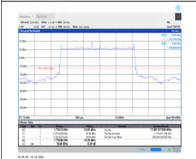
1-N66-15-20-L-2-DFT-PI2BPSK-Outer_Full-100@0-Ant1 1-17.902-18.680-≤20-PASS
