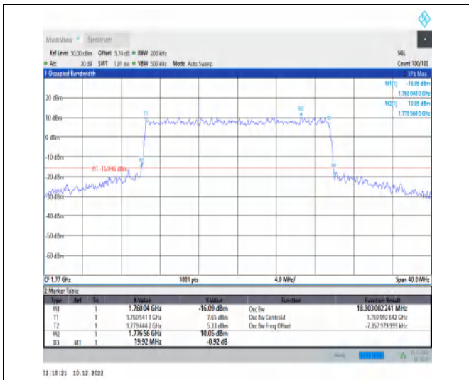
1-N66-15-20-H-6-CP-QPSK-Outer_Full-106@0-Ant1 -18.903-19.920-≤20-PASS
