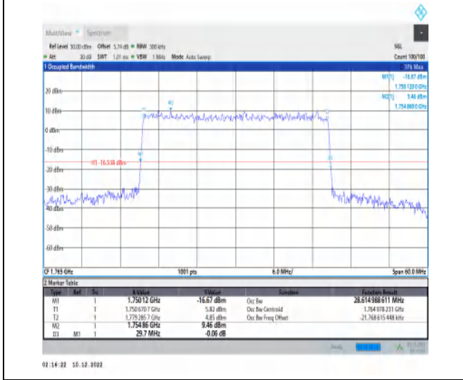
1-N66-15-30-H-5-DFT-256QAM-Outer_Full-160@0-A Ant1-28.615-29.700-≤30-PASS
