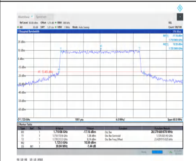
1-N66-15-30-L-8-CP-64QAM-Outer_Full-160@0-Ant 1-28.58-30.840-≤30-PASS
