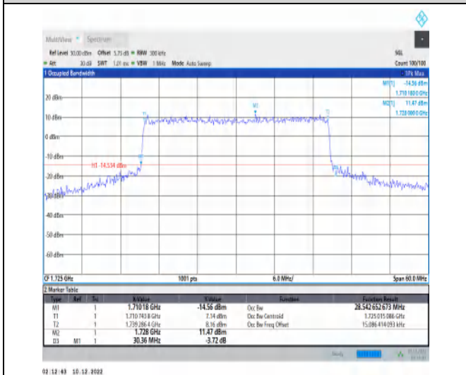
1-N66-15-30-L-7-CP-16QAM-Outer_Full-160@0-Ant 1-28.543-30.360-≤30-PASS
