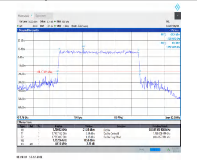
1-N66-15-40-H-9-CP-256QAM-Outer_Full-216@0-A nt1-38.585-40.160-≤40-PASS
