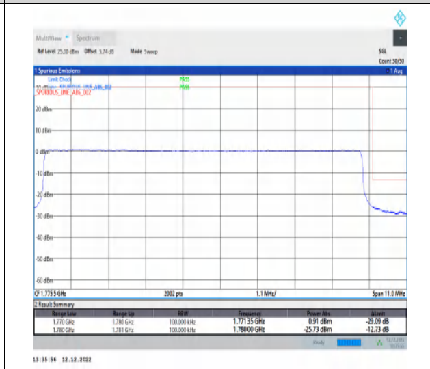
1-N66-15-10-H-6-CP-QPSK-Outer_Full-52@0-Ant1-1-seegraph-PASS-see graph
