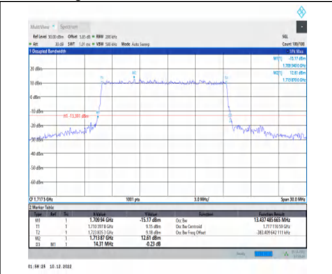
1-N66-15-15-L-4-DFT-64QAM-Outer_Full-75@0-Ant t1-13.437-14.310-≤15-PASS
