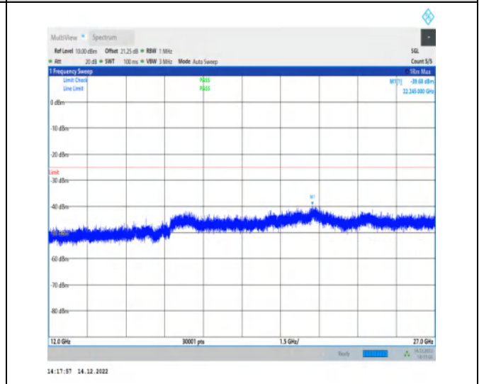
1-N41-30-100-M-1-DFT-PI2BPSK-Inner_1RB_Left-1 @ 1-12000-27000-Ant1-22245.00--39.68--25-PASS
