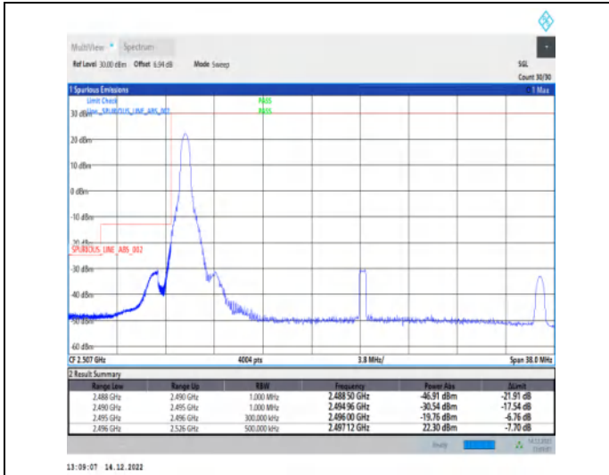
1-N41-30-30-L-4-CP-QPSK-Edge_1RB_Left-1@0-Ant1 1-1--PASS-see graph
