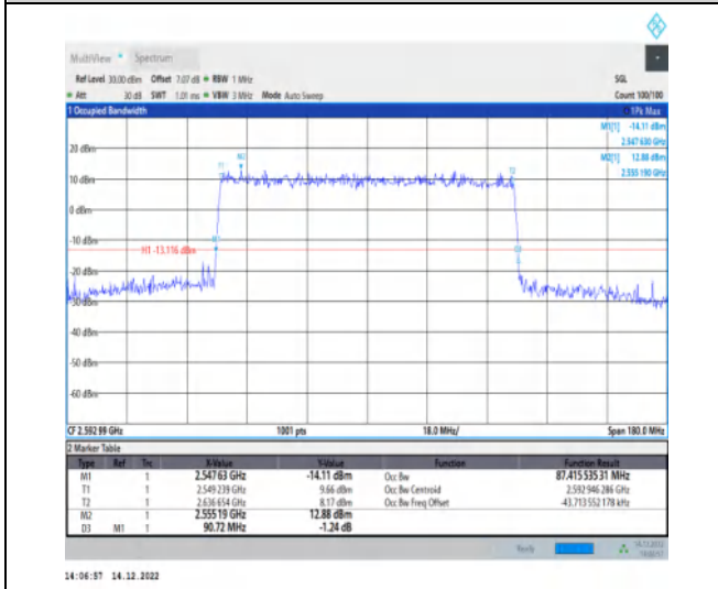
1-N41-30-90-M-9-CP-256QAM-Outer_Full-245@0-A nt1-87.416-90.720-<=90-PASS
