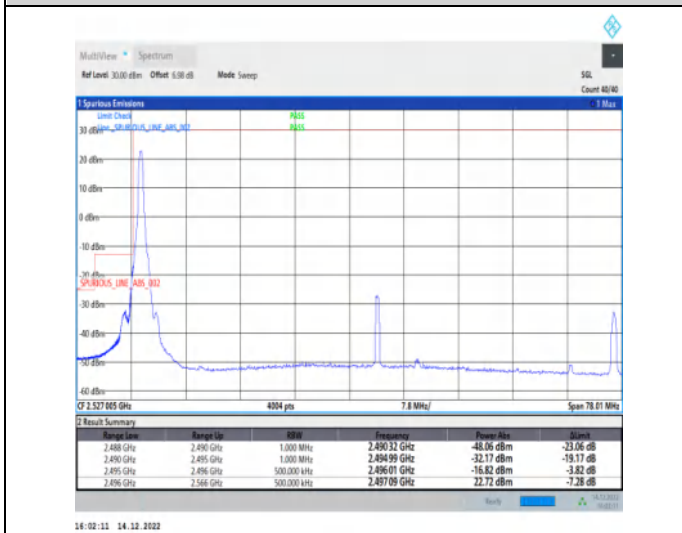
1-N41-30-70-L-4-CP-QPSK-Edge_1RB_Left-1@0-Ant1-1--PASS-see graph
