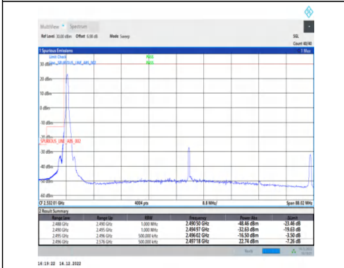
1-N41-30-80-L-4-CP-QPSK-Edge_1RB_Left-1@0-Ant1-1--PASS-see graph
