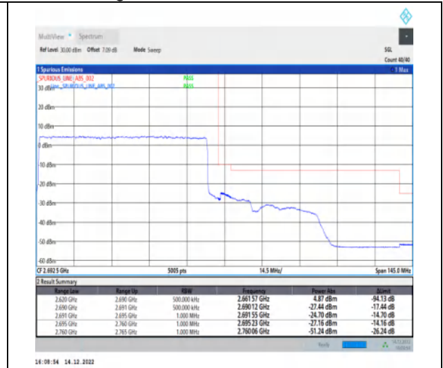
1-N41-30-70-H-3-DFT-PI2BPSK-Outer_Full-180@0-Ant1-1--PASS-see graph
