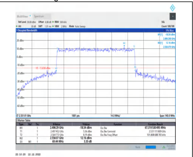
1-N41-30-70-L-7-CP-16QAM-Outer_Full-189@0-Ant1 1-67.32-69.440-≤70-PASS
