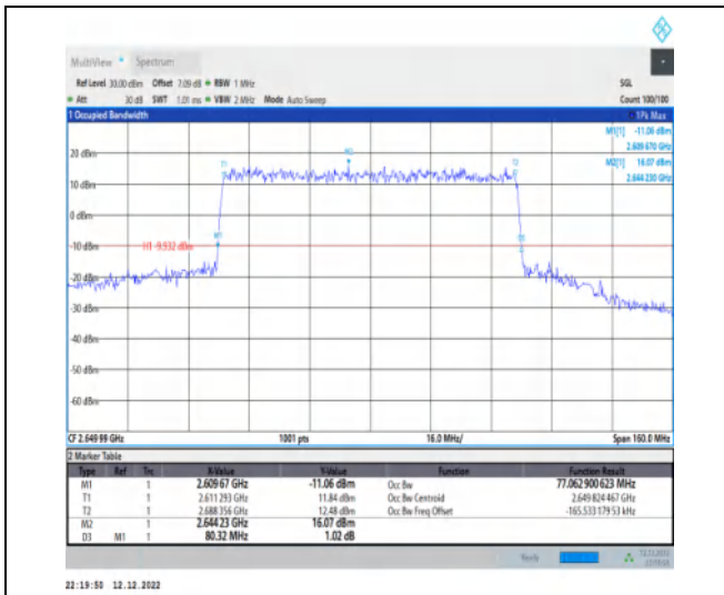
1-N41-30-80-H-1-DFT-QPSK-Outer_Full-216@0-Ant 1-77.063-80.320≤80-PASS
