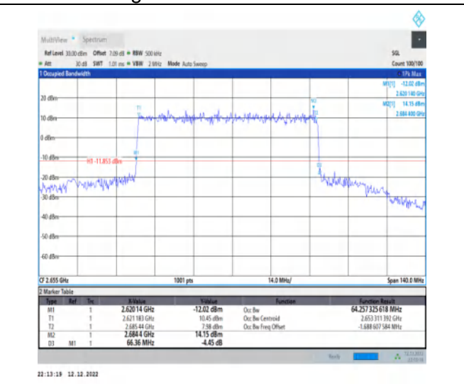
1-N41-30-70-H-1-DFT-QPSK-Outer_Full-180@0-Ant 1-64.257-66.360-≤70-PASS
