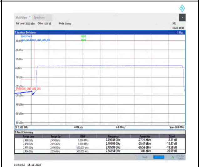
1-N41-30-60-L-6-CP-QPSK-Outer_Full-162@0-Ant1-1--PASS-see graph
