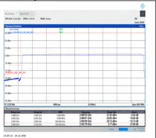
1-N41-30-60-L-6-CP-QPSK-Outer_Full-162@0-Ant1-1--PASS-see graph
