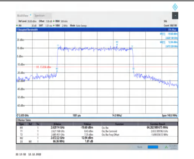
1-N41-30-70-H-3-DFT-16QAM-Outer_Full-180@0-Ant1 1-64.283-66.360-≤70-PASS
