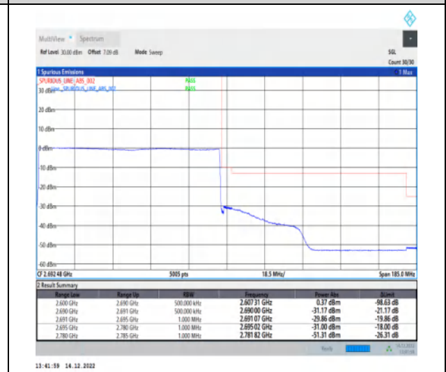
1-N41-30-90-H-6-CP-QPSK-Outer_Full-245@0-Ant1-1--PASS-see graph
