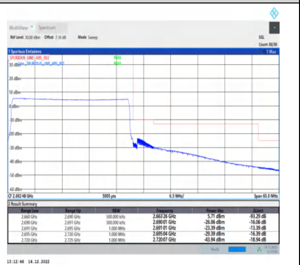
1-N41-30-30-H-6-CP-QPSK-Outer_Full-78@0-Ant1 1-1--PASS-see graph
