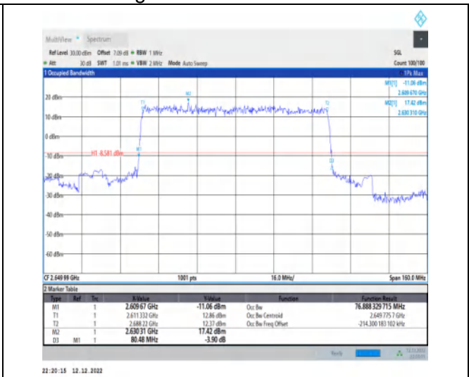
1-N41-30-80-H-2-DFT-PI2BPSK-Outer_Full-216@0-Ant 1-76.888-80.480≤80-PASS
