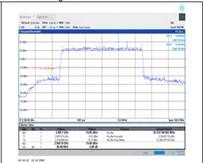
1-N41-30-80-L-4-DFT-64QAM-Outer_Full-216@0-A nt1-76.753-80.480-<math>\leq 80</math>-PASS
