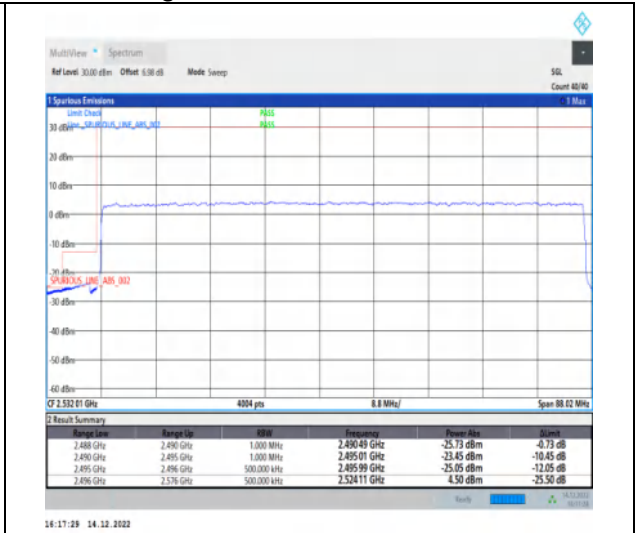
1-N41-30-80-L-3-DFT-PI2BPSK-Outer_Full-216@0-Ant1-1--PASS-see graph
