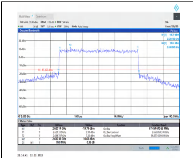
1-N41-30-70-H-8-CP-64QAM-Outer_Full-189@0-Ant 1-67.455-70.000-≤70-PASS
