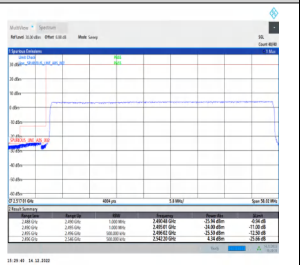
1-N41-30-50-L-6-CP-QPSK-Outer_Full-133@0-Ant1-1--PASS-see graph
