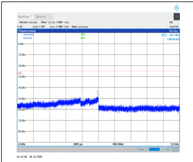
1-N41-30-100-L-1-DFT-PI2BPSK-Inner_1RB_Left-1 @ 1-3000-12000-Ant1-7468.95--46.71--25-PASS
