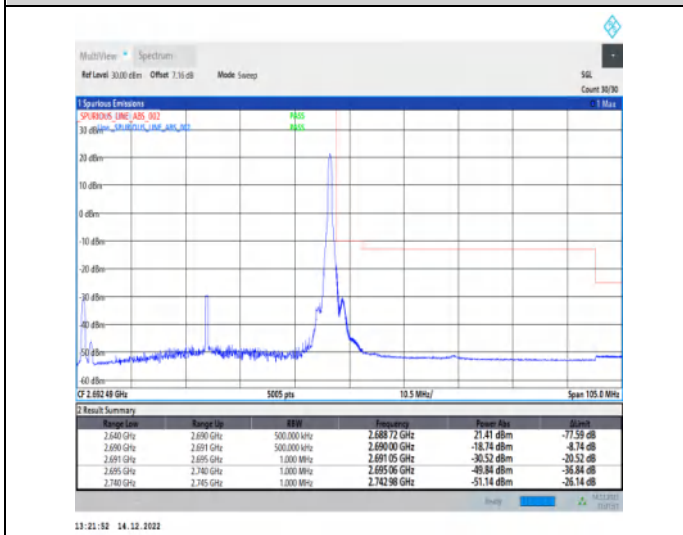
1-N41-30-50-H-5-CP-QPSK-Edge_1RB_Right-1@132-Ant1-1--PASS-see graph
