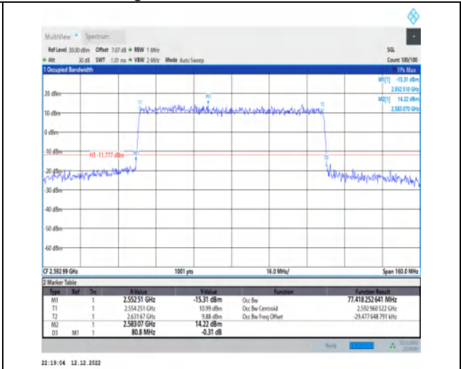
1-N41-30-80-M-7-CP-16QAM-Outer_Full-217@0-Ant 1-77.418-80.800-≤80-PASS
