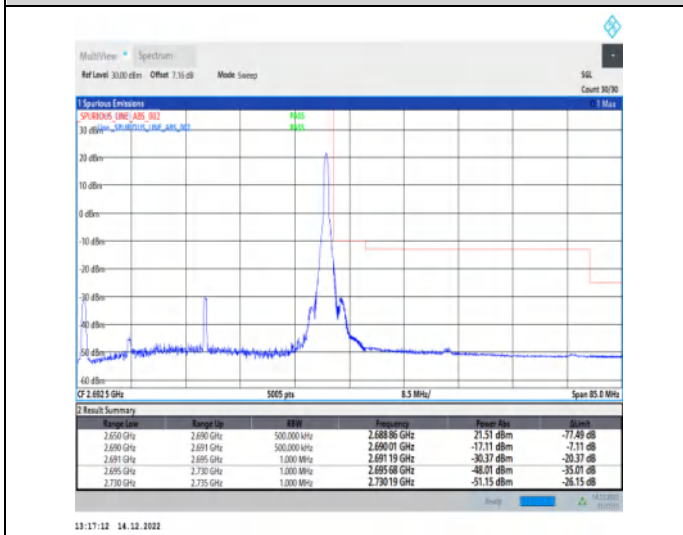
1-N41-30-40-H-5-CP-QPSK-Edge_1RB_Right-1@105-Ant1-1--PASS-see graph
