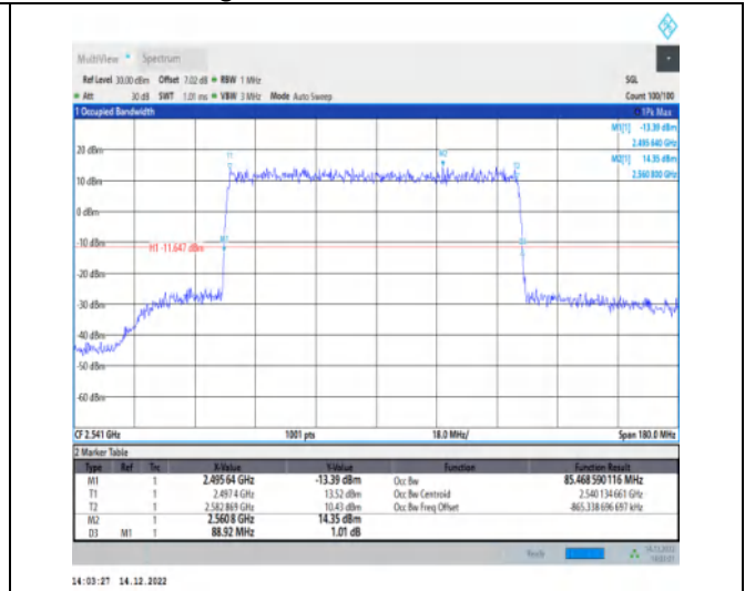
1-N41-30-90-L-5-DFT-256QAM-Outer_Full-240@0-A nt1-85.469-88.920- \leq 90 -PASS
