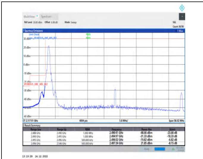
1-N41-30-50-L-4-CP-QPSK-Edge_1RB_Left-1@0-Ant1 -1--PASS-see graph
