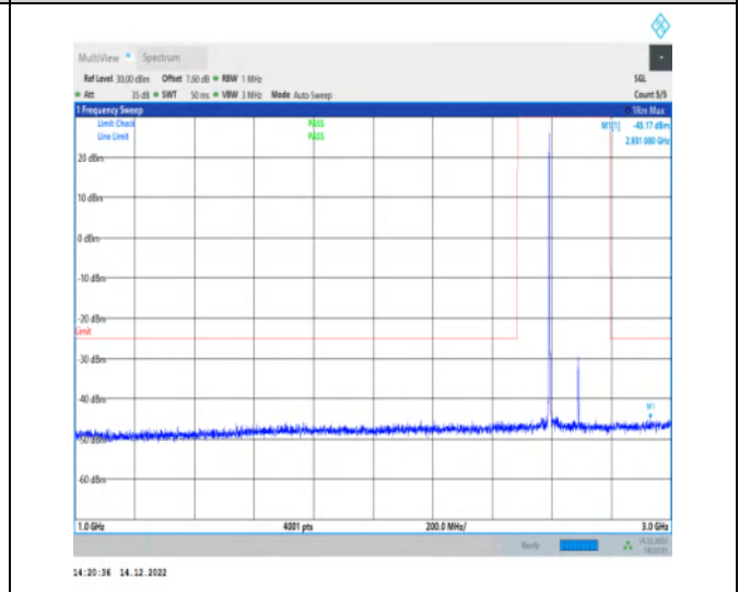
1-N41-30-100-H-1-DFT-PI2BPSK-Inner_1RB_Left-1 @ 1-1000-3000-Ant1-2931.00--45.17--25-PASS
