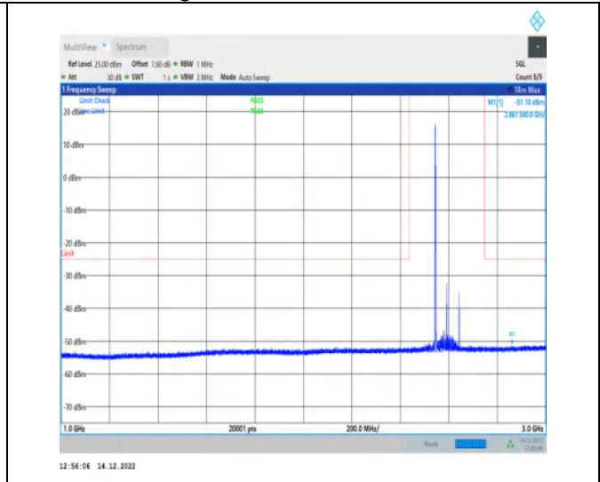
1-N41-30-100-M-1-DFT-QPSK-Edge_1RB_Left-1@0- 1000-3000-Ant1-2861.50--51.18--25-PASS
