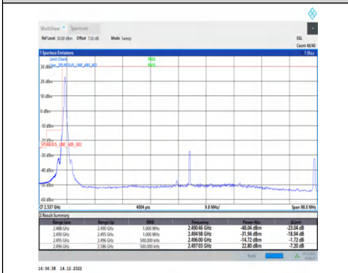
1-N41-30-90-L-4-CP-QPSK-Edge_1RB_Left-1@0-Ant1-1--PASS-see graph
