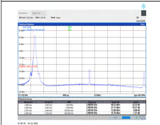
1-N41-30-60-L-4-CP-QPSK-Edge_1RB_Left-1@0-Ant1-1--PASS-see graph
