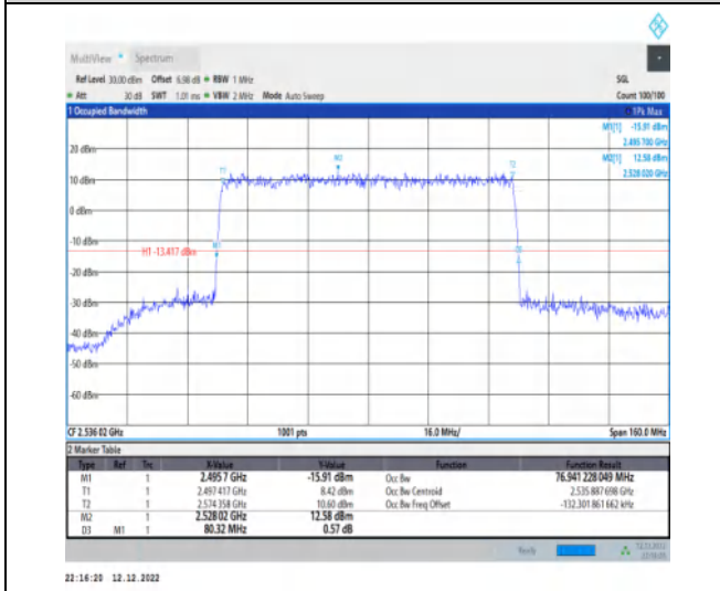
1-N41-30-80-L-5-DFT-256QAM-Outer_Full-216@0-A nt1-76.941-80.320-<math>\leq 80</math>-PASS
