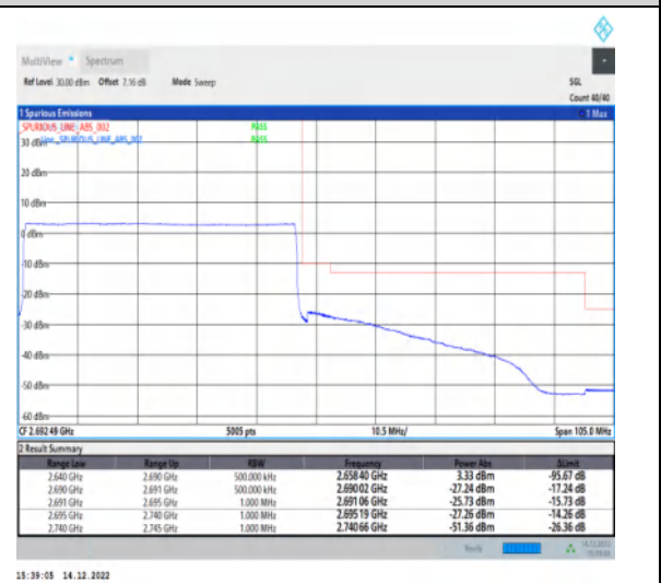
1-N41-30-50-H-6-CP-QPSK-Outer_Full-133@0-Ant1-1--PASS-see graph
