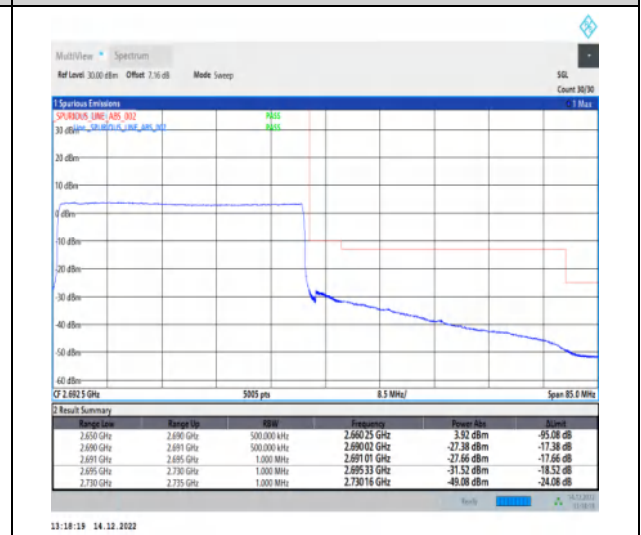
1-N41-30-40-H-6-CP-QPSK-Outer_Full-106@0-Ant1-1--PASS-see graph
