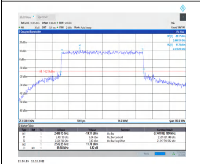
1-N41-30-70-L-8-CP-64QAM-Outer_Full-189@0-Ant1 1-67.402-69.580-≤70-PASS
