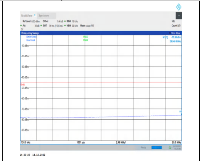
1-N41-30-100-H-1-DFT-PI2BPSK-Inner_1RB_Left-1 @ 1-0.15-30-Ant1-29.94--75.98--45-PASS
