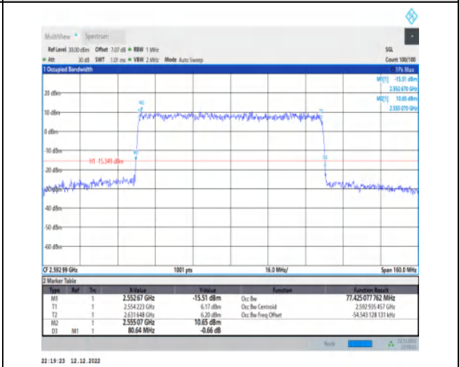
1-N41-30-80-M-9-CP-256QAM-Outer_Full-217@0-Ant nt1-77.425-80.640-≤80-PASS
