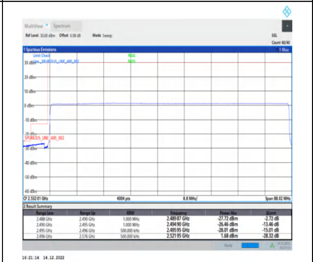
1-N41-30-80-L-6-CP-QPSK-Outer_Full-217@0-Ant1-1--PASS-see graph
