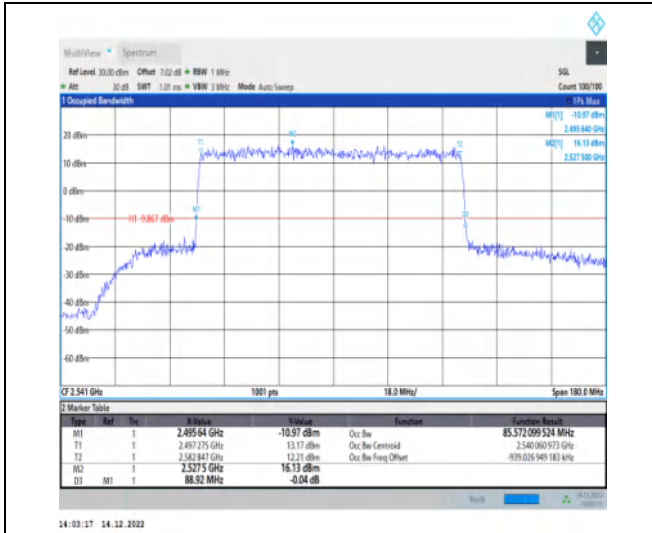
1-N41-30-90-L-4-DFT-64QAM-Outer_Full-240@0-A nt1-85.572-88.920- \leq 90 -PASS
