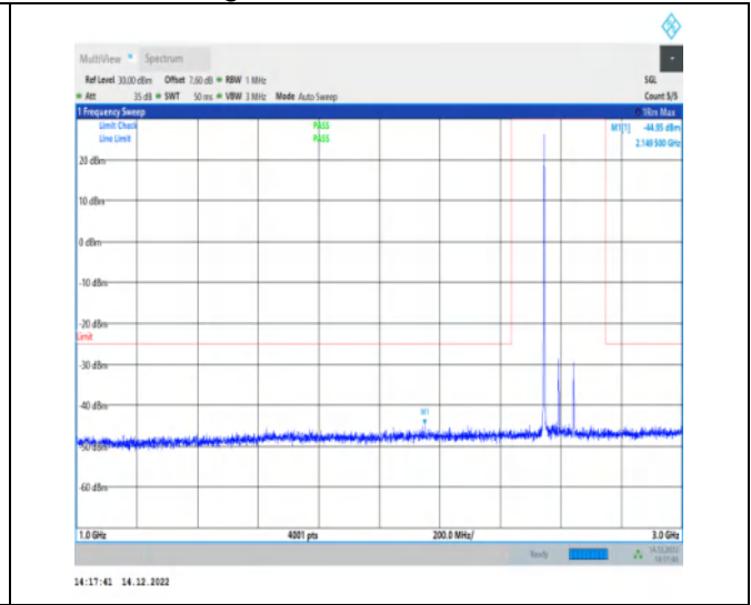
1-N41-30-100-M-1-DFT-PI2BPSK-Inner_1RB_Left-1 @ 1-1000-3000-Ant1-2149.50--44.95--25-PASS
