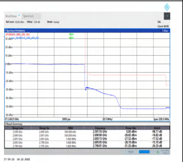
1-N41-30-100-H-6-CP-QPSK-Outer_Full-273@0-Ant1-1--PASS-see graph
