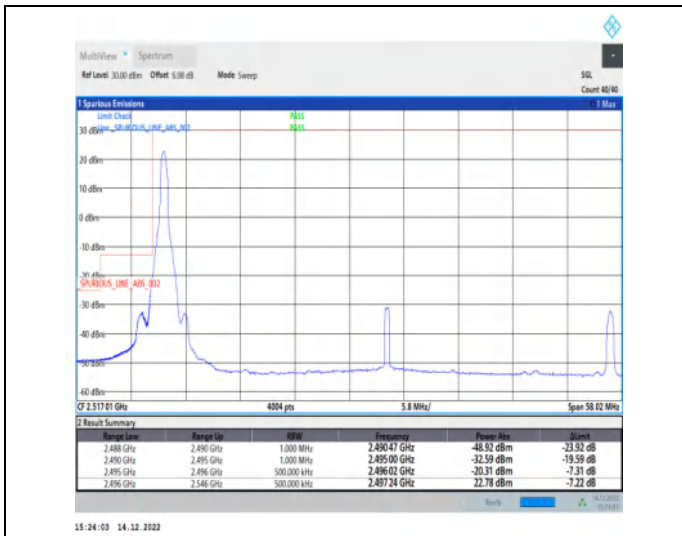
1-N41-30-50-L-1-DFT-PI2BPSK-Edge_1RB_Left-1@0-Ant1-1--PASS-see graph
