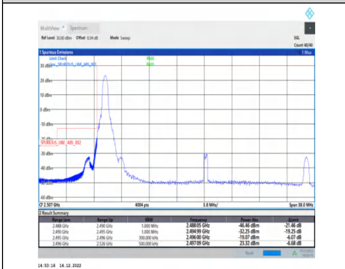
1-N41-30-30-L-4-CP-QPSK-Edge_1RB_Left-1@0-Ant1-1--PASS-see graph
