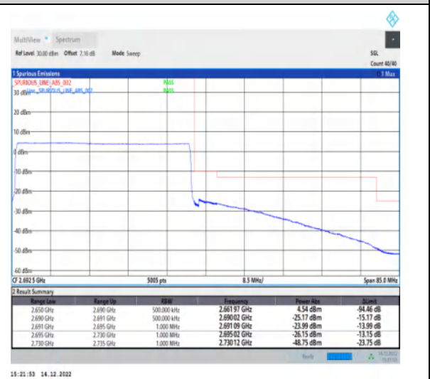
1-N41-30-40-H-6-CP-QPSK-Outer_Full-106@0-Ant1-1--PASS-see graph
