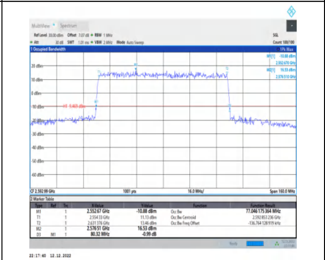
1-N41-30-80-M-1-DFT-QPSK-Outer_Full-216@0-Ant 1-77.046-80.320-≤80-PASS
