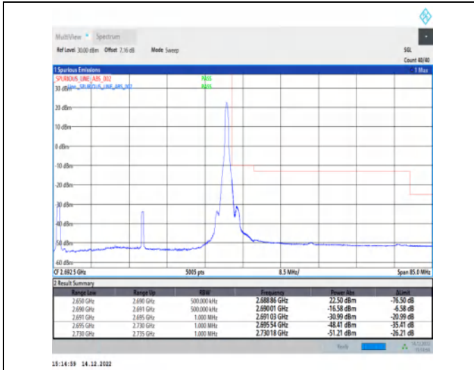
1-N41-30-40-H-2-DFT-PI2BPSK-Edge_1RB_Right-1@105-Ant1-1--PASS-see graph
