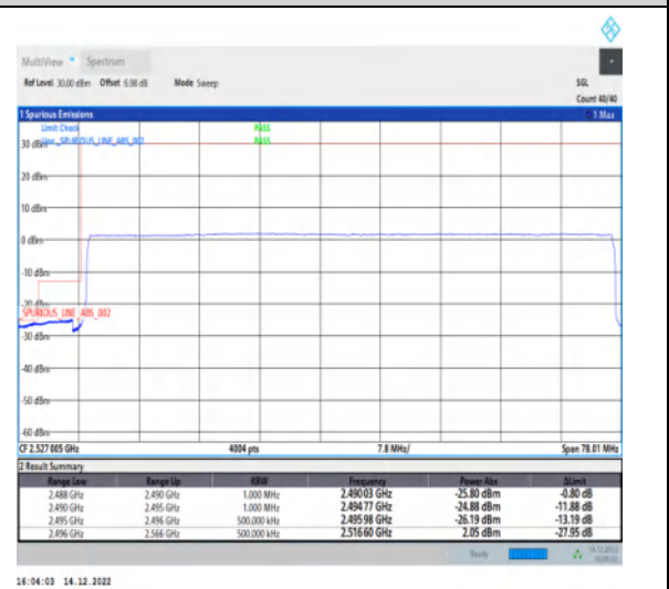
1-N41-30-70-L-6-CP-QPSK-Outer_Full-189@0-Ant1-1--PASS-see graph
