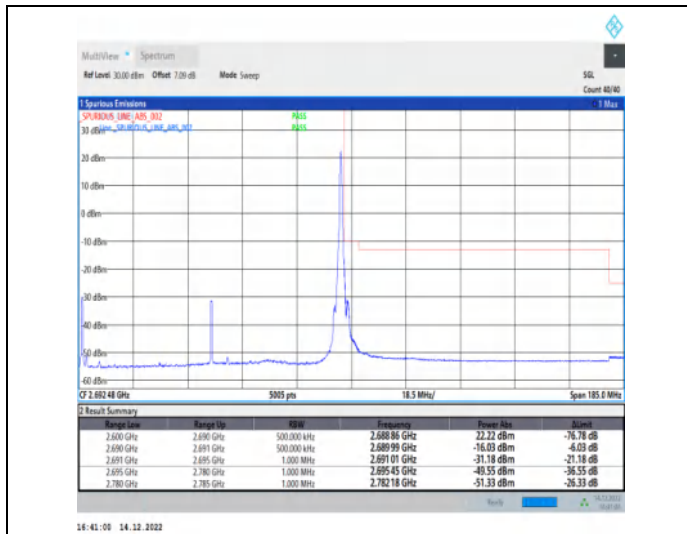
1-N41-30-90-H-2-DFT-PI2BPSK-Edge_1RB_Right-1@244-Ant1-1--PASS-see graph
