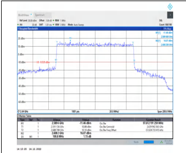
1-N41-30-100-H-7-CP-16QAM-Outer_Full-273@0-A nt1-97.612-100.800≤100-PASS
