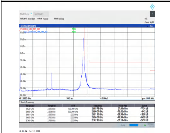
1-N41-30-70-H-5-CP-QPSK-Edge_1RB_Right-1@188-Ant1-1--PASS-see graph
