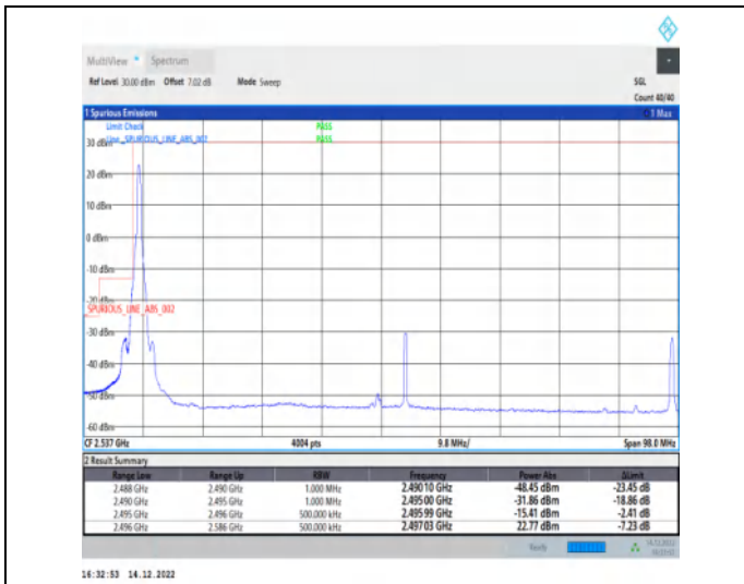
1-N41-30-90-L-1-DFT-PI2BPSK-Edge_1RB_Left-1@0-Ant1-1--PASS-see graph
