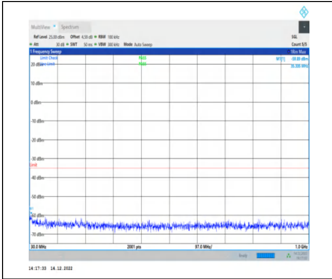
1-N41-30-100-M-1-DFT-PI2BPSK-Inner_1RB_Left-1 @ 1-30-1000-Ant1-35.34--59.89--35-PASS
