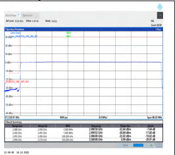
1-N41-30-80-L-6-CP-QPSK-Outer_Full-217@0-Ant1-1--PASS-see graph
