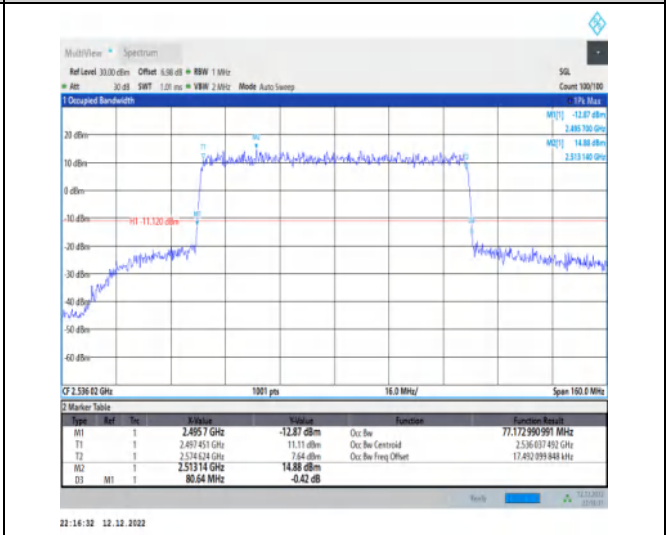
1-N41-30-80-L-6-CP-QPSK-Outer_Full-217@0-A nt1-77.173-80.640-<math>\leq 80</math>-PASS
