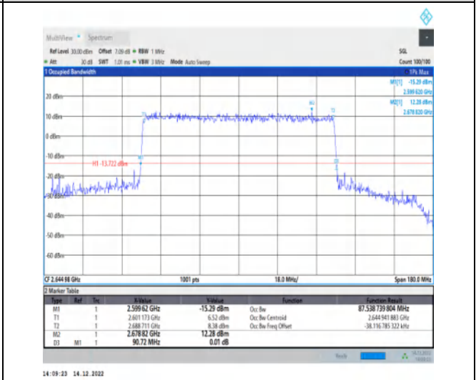
1-N41-30-90-H-9-CP-256QAM-Outer_Full-245@0-Ant1 1-87.539-90.720-≤90-PASS
