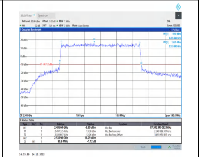
1-N41-30-90-L-7-CP-16QAM-Outer_Full-245@0-Ant1 -87.342-90.900- \leq 90 -PASS
