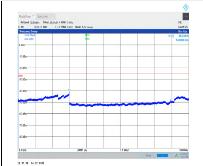
1-N41-30-100-H-1-DFT-QPSK-Edge_1RB_Left-1@ 0-3000-18000-Ant1-7499.00--42.35--25-PASS
