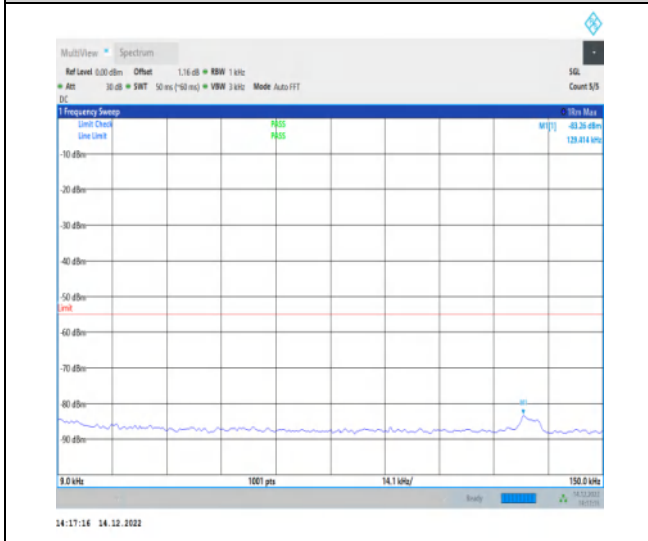
1-N41-30-100-M-1-DFT-PI2BPSK-Inner_1RB_Left-1 @ 1-0.009-0.15-Ant1-0.13--83.26--55-PASS
