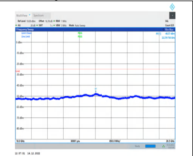
1-N41-30-100-H-1-DFT-QPSK-Edge_1RB_Left-1@0- 18000-26500-Ant1-22279.75--46.57--25-PASS
