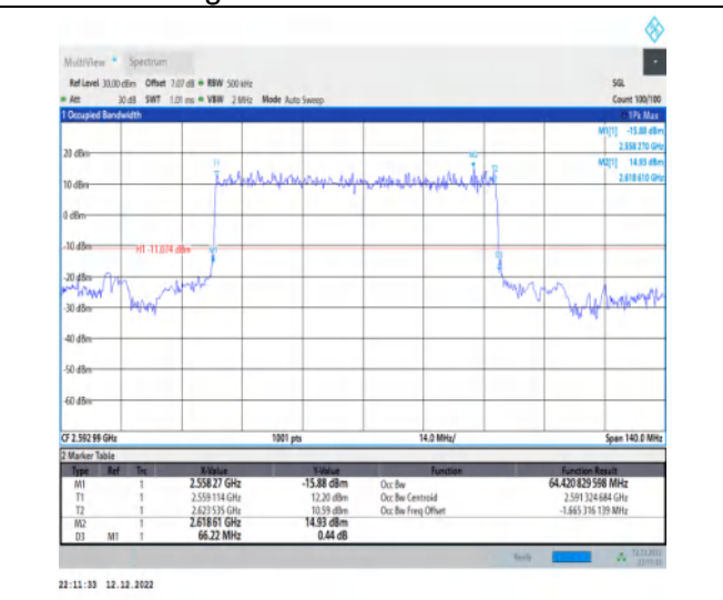
1-N41-30-70-M-2-DFT-PI2BPSK-Outer_Full-180@0-Ant 1-64.421-66.220-≤70-PASS
