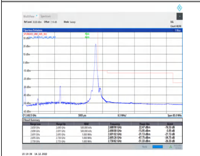
1-N41-30-40-H-5-CP-QPSK-Edge_1RB_Right-1@105-Ant1-1--PASS-see graph
