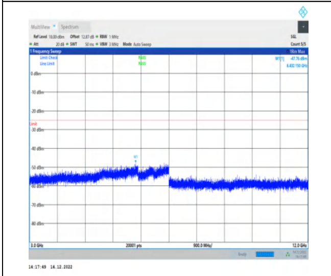
1-N41-30-100-M-1-DFT-PI2BPSK-Inner_1RB_Left-1 @ 1-3000-12000-Ant1-6432.15--47.76--25-PASS
