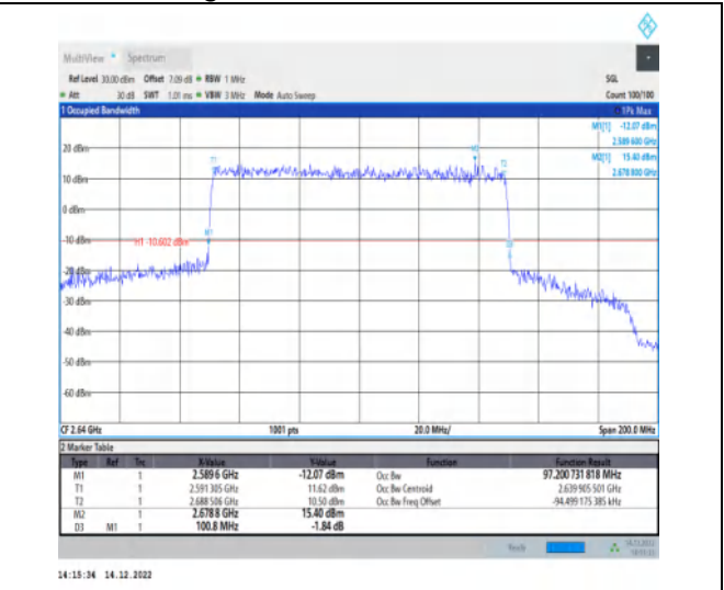
1-N41-30-100-H-8-CP-64QAM-Outer_Full-273@0-A nt1-97.201-100.800≤100-PASS
