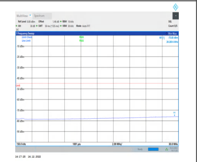
1-N41-30-100-M-1-DFT-PI2BPSK-Inner_1RB_Left-1 @ 1-0.15-30-Ant1-29.28--75.85--45-PASS
