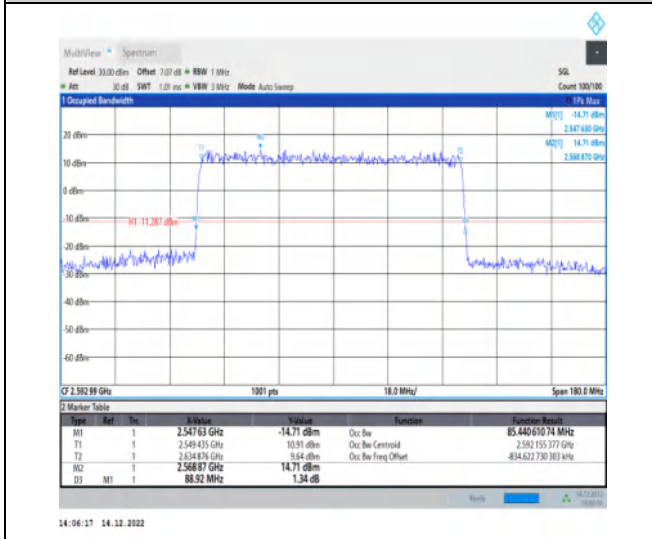
1-N41-30-90-M-5-DFT-256QAM-Outer_Full-240@0-A Ant1-85.441-88.920≤90-PASS
