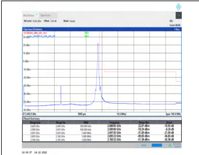
1-N41-30-70-H-2-DFT-PI2BPSK-Edge_1RB_Right-1@188-Ant1-1--PASS-see graph
