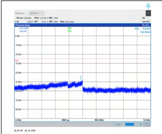
1-N41-30-100-H-1-DFT-PI2BPSK-Inner_1RB_Left-1 @ 1-3000-12000-Ant1-7381.20--47.60--25-PASS
