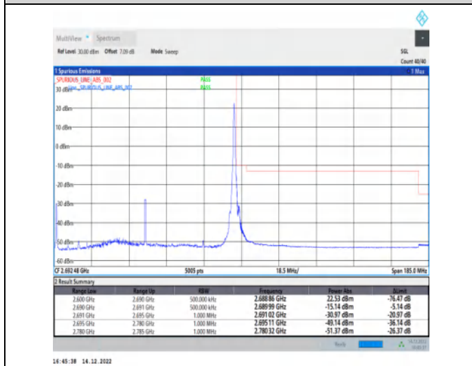
1-N41-30-90-H-5-CP-QPSK-Edge_1RB_Right-1@244-Ant1-1--PASS-see graph
