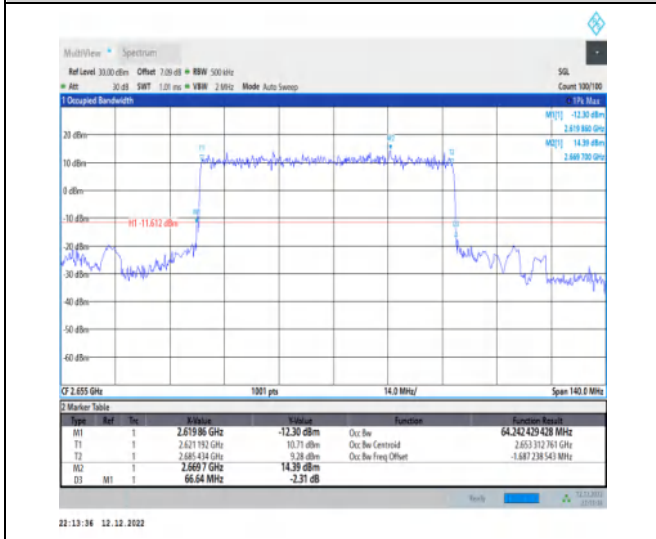
1-N41-30-70-H-2-DFT-PI2BPSK-Outer_Full-180@0-Ant1 1-64.242-66.640-≤70-PASS
