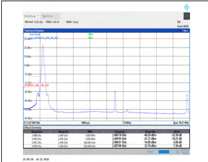
1-N41-30-70-L-1-DFT-PI2BPSK-Edge_1RB_Left-1@0-Ant1-1--PASS-see graph
