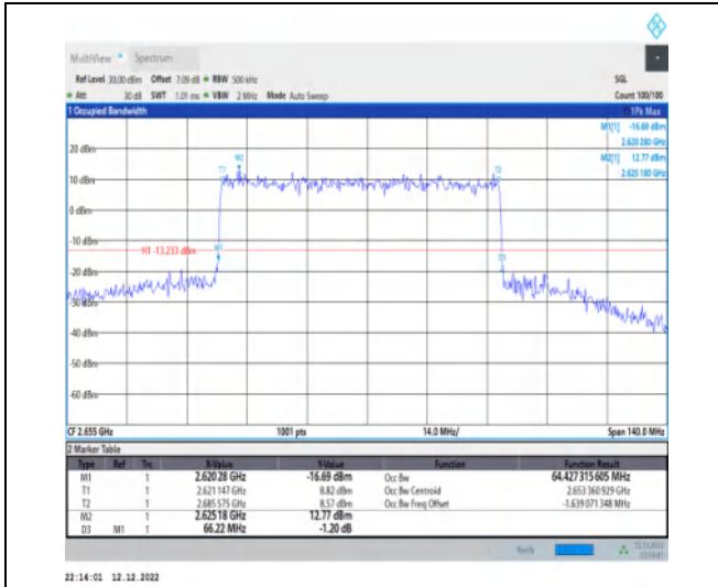
1-N41-30-70-H-4-DFT-64QAM-Outer_Full-180@0-A nt1-64.427-66.220- \leq 70 -PASS
