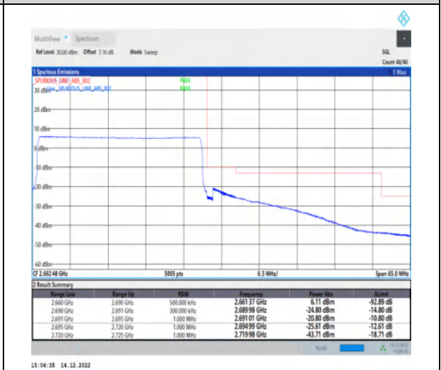
1-N41-30-30-H-6-CP-QPSK-Outer_Full-78@0-Ant1-1--PASS-see graph
