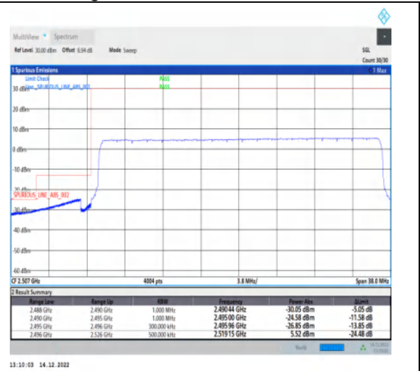
1-N41-30-30-L-6-CP-QPSK-Outer_Full-78@0-Ant1 1-1--PASS-see graph
