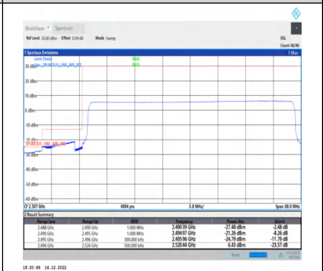
1-N41-30-30-L-6-CP-QPSK-Outer_Full-78@0-Ant1-1--PASS-see graph
