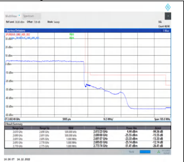
1-N41-30-80-H-3-DFT-PI2BPSK-Outer_Full-216@0-Ant1-1--PASS-see graph
