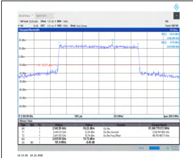
1-N41-30-100-M-8-CP-64QAM-Outer_Full-273@0-A nt1-97.241-101.400-≤100-PASS
