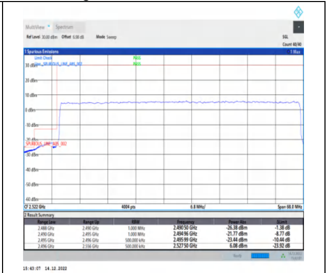
1-N41-30-60-L-3-DFT-PI2BPSK-Outer_Full-162@0-Ant1-1--PASS-see graph
