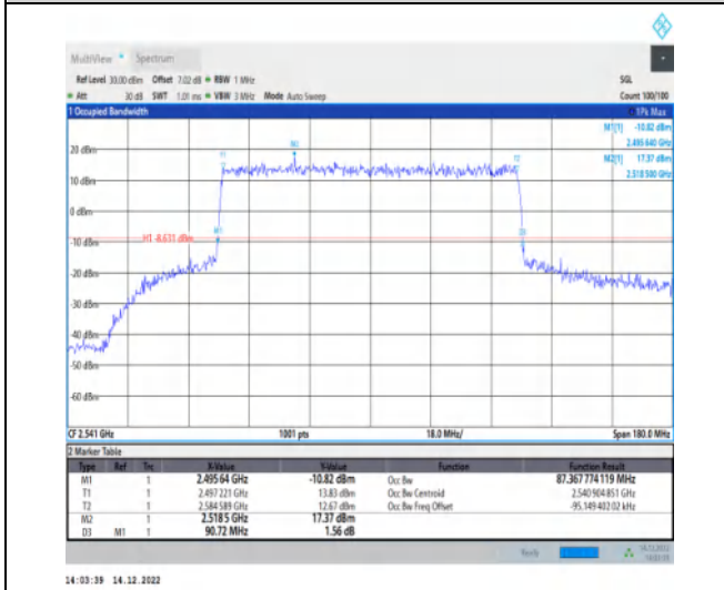
1-N41-30-90-L-6-CP-QPSK-Outer_Full-245@0-Ant1 -87.368-90.720- \leq 90 -PASS
