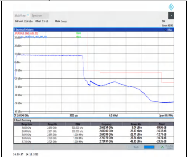
1-N41-30-30-H-3-DFT-PI2BPSK-Outer_Full-75@0-Ant1-1--PASS-see graph
