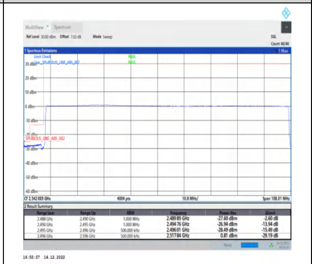
1-N41-30-100-L-6-CP-QPSK-Outer_Full-273@0-Ant1-1--PASS-see graph
