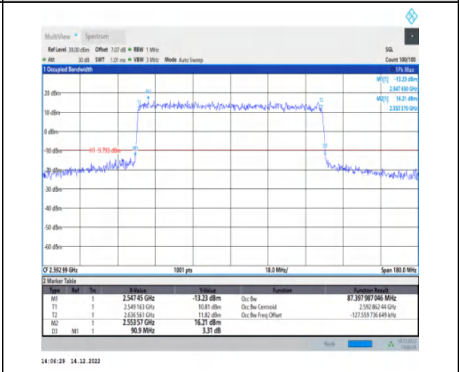
1-N41-30-90-M-6-CP-QPSK-Outer_Full-245@0-Ant1 -87.398-90.900≤90-PASS
