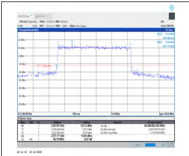
1-N41-30-70-M-1-DFT-QPSK-Outer_Full-180@0-Ant 1-64.304-66.780-≤70-PASS
