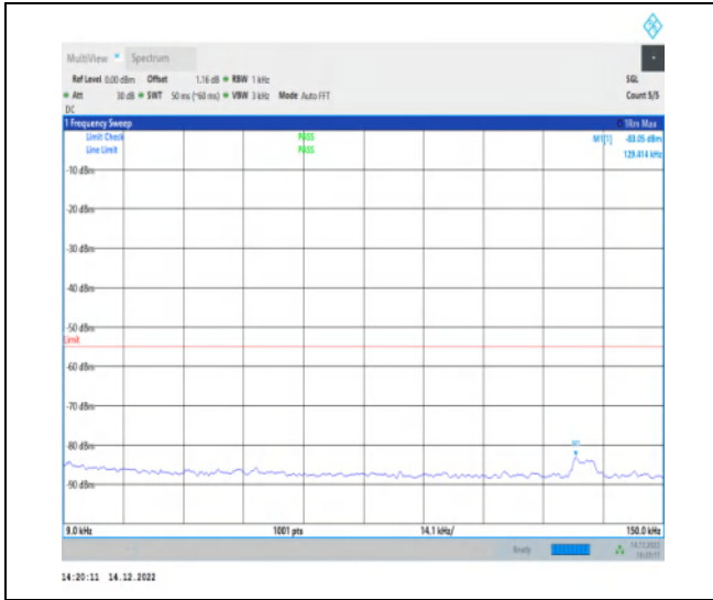
1-N41-30-100-H-1-DFT-PI2BPSK-Inner_1RB_Left-1 @ 1-0.009-0.15-Ant1-0.13--83.05--55-PASS
