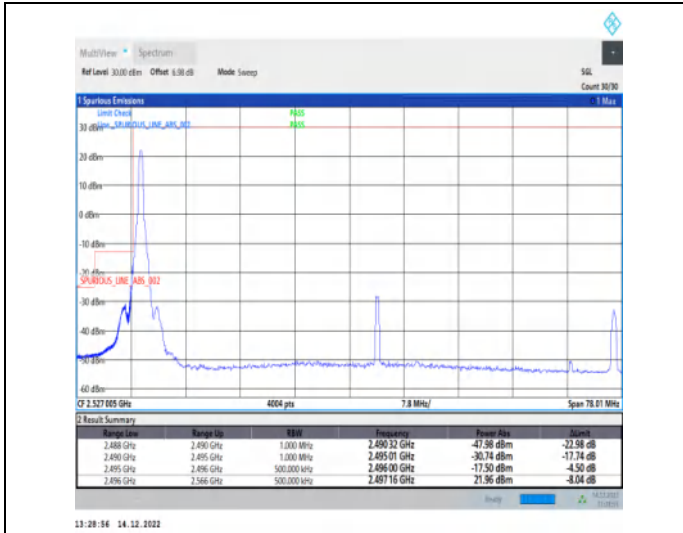
1-N41-30-70-L-4-CP-QPSK-Edge_1RB_Left-1@0-Ant1 -1--PASS-see graph
