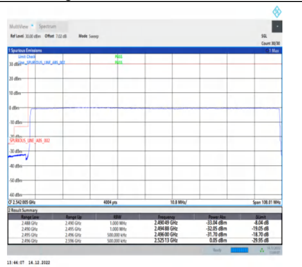
1-N41-30-100-L-6-CP-QPSK-Outer_Full-273@0-A nt1-1--PASS-see graph
