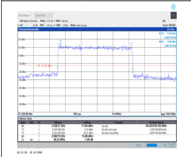
1-N41-30-70-M-3-DFT-16QAM-Outer_Full-180@0-Ant 1-64.293-66.220-≤70-PASS
