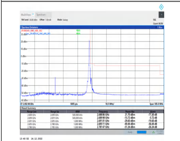
1-N41-30-90-H-5-CP-QPSK-Edge_1RB_Right-1@244-Ant1-1--PASS-see graph
