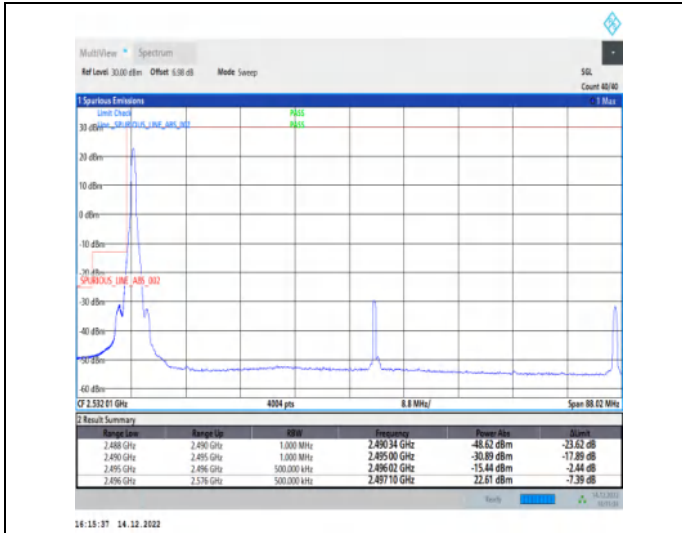
1-N41-30-80-L-1-DFT-PI2BPSK-Edge_1RB_Left-1@0-Ant1-1--PASS-see graph
