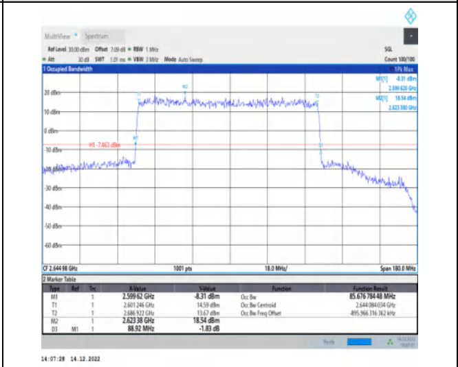
1-N41-30-90-H-1-DFT-QPSK-Outer_Full-240@0-Ant 1-85.677-88.920-<=90-PASS
