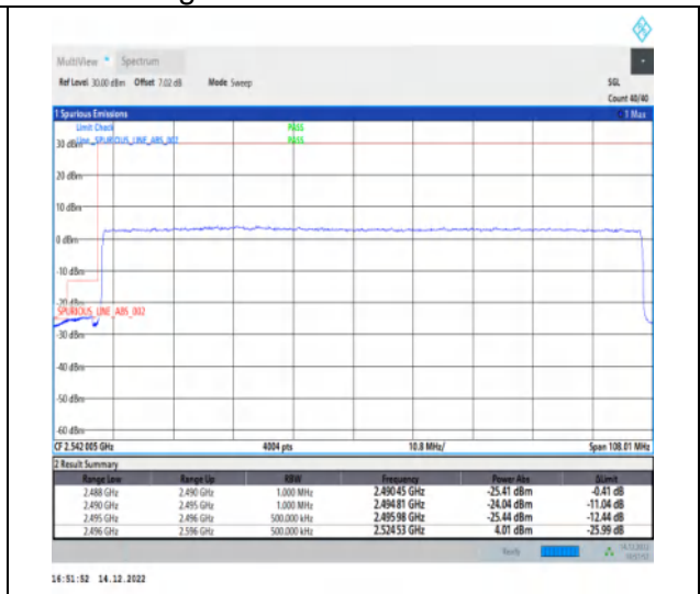
1-N41-30-100-L-3-DFT-PI2BPSK-Outer_Full-270@0-Ant1-1--PASS-see graph
