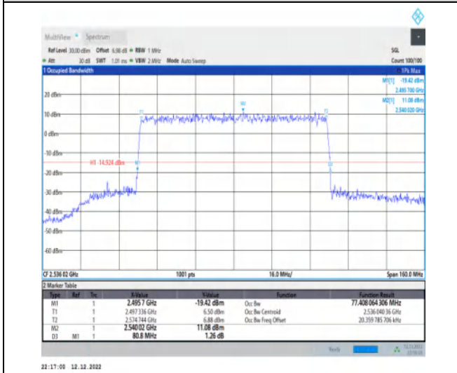
1-N41-30-80-L-9-CP-256QAM-Outer_Full-217@0-A nt1-77.408-80.800-≤80-PASS
