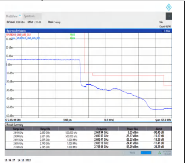
1-N41-30-50-H-3-DFT-PI2BPSK-Outer_Full-128@0-Ant1-1--PASS-see graph
