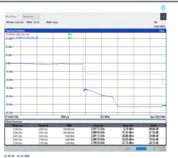
1-N41-30-100-H-6-CP-QPSK-Outer_Full-273@0- Ant1-1--PASS-see graph
