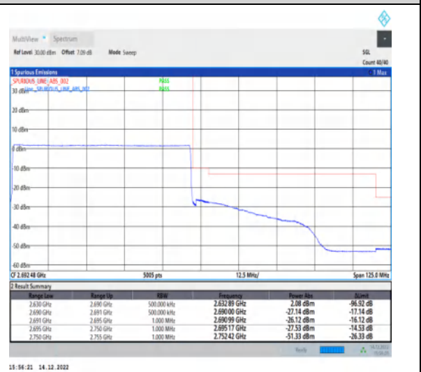
1-N41-30-60-H-6-CP-QPSK-Outer_Full-162@0-Ant1-1--PASS-see graph
