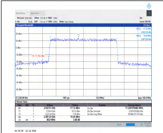
1-N41-30-80-M-6-CP-QPSK-Outer_Full-217@0-Ant 1-77.24-80.800-≤80-PASS
