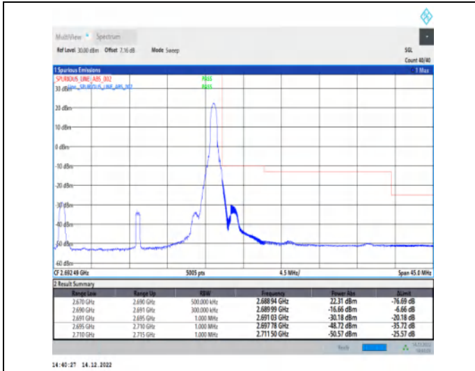
1-N41-30-20-H-2-DFT-PI2BPSK-Edge_1RB_Right-1 @ 50-Ant1-1--PASS-see graph
