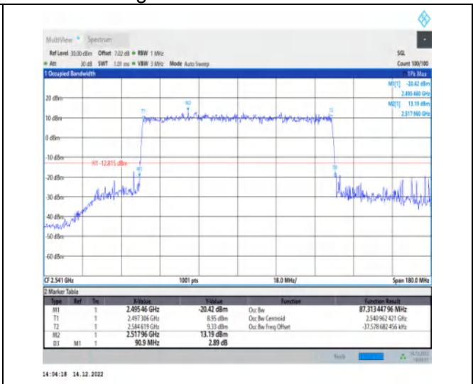
1-N41-30-90-L-9-CP-256QAM-Outer_Full-245@0-Ant t1-87.313-90.900-≤90-PASS
