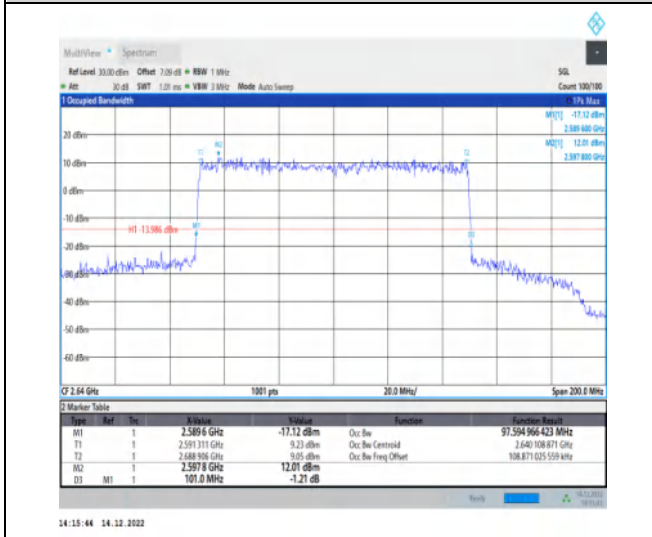
1-N41-30-100-H-9-CP-256QAM-Outer_Full-273@0-A Ant1-97.595-101.000≤100-PASS
