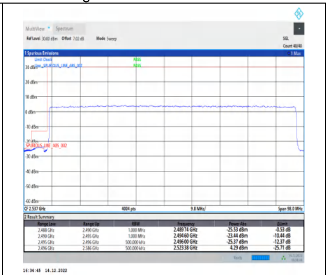
1-N41-30-90-L-3-DFT-PI2BPSK-Outer_Full-240@0-Ant1-1--PASS-see graph
