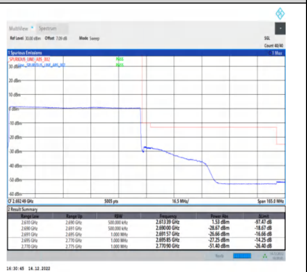
1-N41-30-80-H-6-CP-QPSK-Outer_Full-217@0-Ant1-1--PASS-see graph
