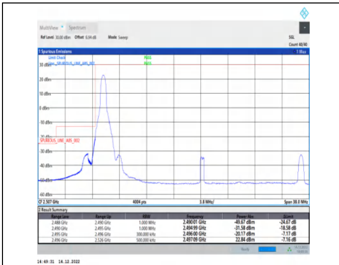
1-N41-30-30-L-1-DFT-PI2BPSK-Edge_1RB_Left-1@0-Ant1-1--PASS-see graph
