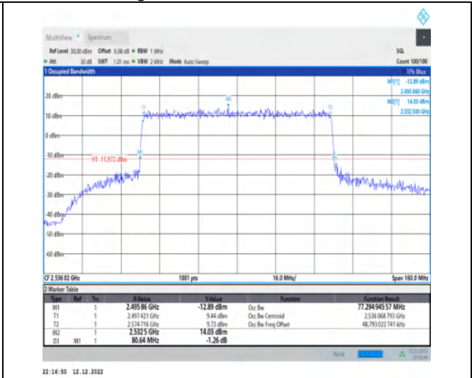
1-N41-30-80-L-8-CP-64QAM-Outer_Full-217@0-Ant 1-77.295-80.640-≤80-PASS
