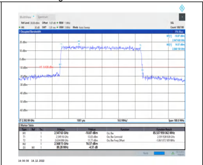
1-N41-30-90-M-4-DFT-64QAM-Outer_Full-240@0-A nt1-85.538-89.280≤90-PASS
