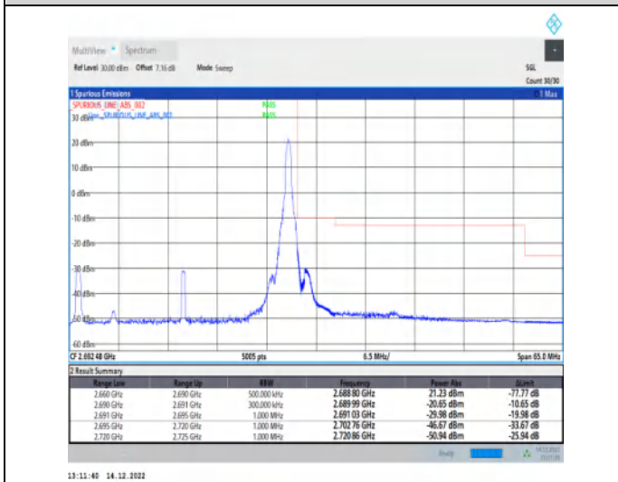
1-N41-30-30-H-5-CP-QPSK-Edge_1RB_Right-1@77-Ant1 1-1--PASS-see graph
