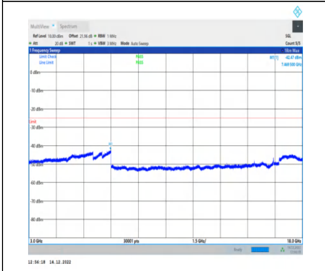
1-N41-30-100-M-1-DFT-QPSK-Edge_1RB_Left-1@ 0-3000-18000-Ant1-7469.50--42.47--25-PASS
