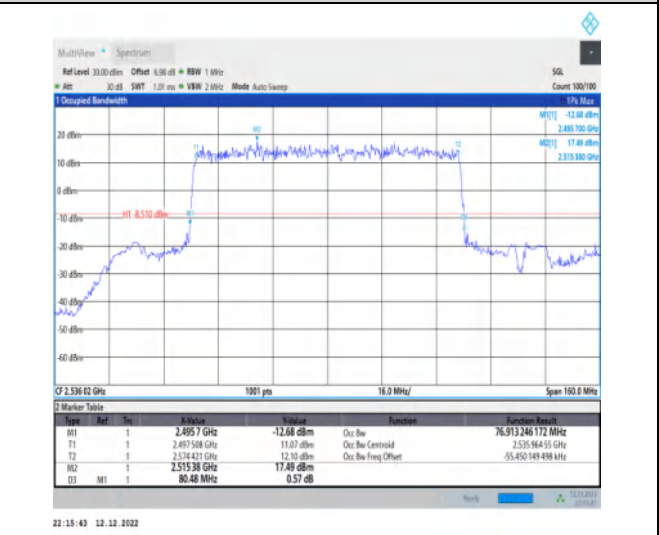
1-N41-30-80-L-2-DFT-PI2BPSK-Outer_Full-216@0-Ant 1-76.913-80.480-≤80-PASS
