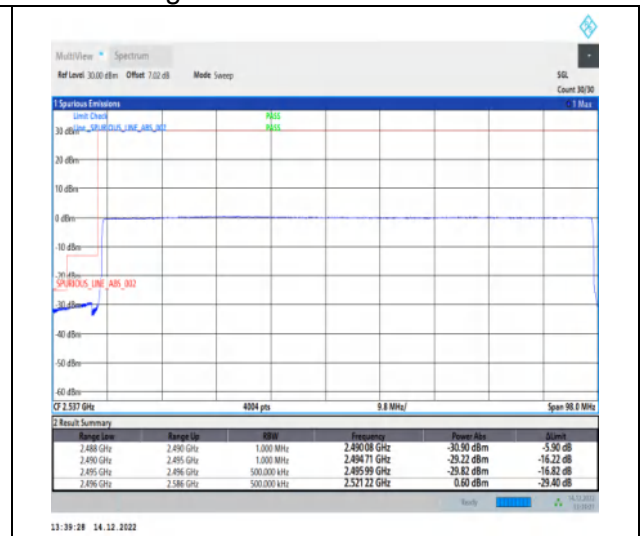
1-N41-30-90-L-6-CP-QPSK-Outer_Full-245@0-Ant1-1--PASS-see graph
