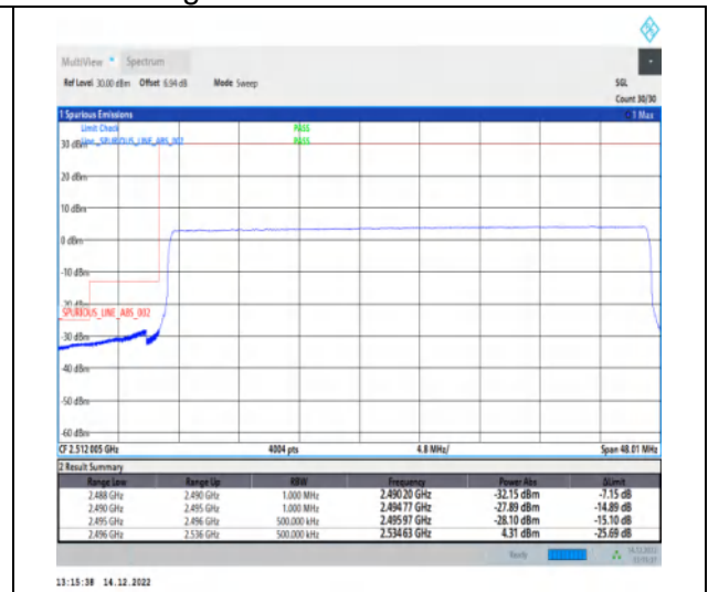
1-N41-30-40-L-6-CP-QPSK-Outer_Full-106@0-Ant1-1--PASS-see graph
