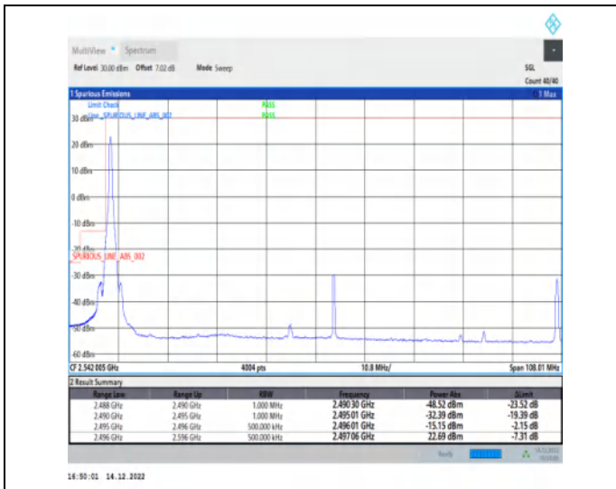
1-N41-30-100-L-1-DFT-PI2BPSK-Edge_1RB_Left-1@0-Ant1-1--PASS-see graph
