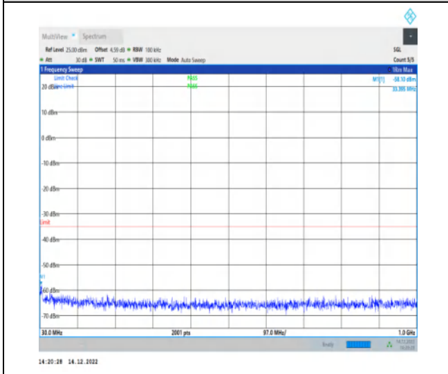
1-N41-30-100-H-1-DFT-PI2BPSK-Inner_1RB_Left-1 @ 1-30-1000-Ant1-33.40--58.10--35-PASS
