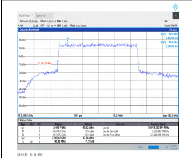
1-N41-30-80-L-1-DFT-QPSK-Outer_Full-216@0-Ant 1-76.913-80.320-≤80-PASS
