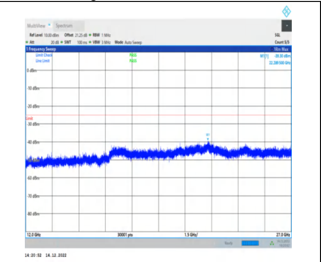
1-N41-30-100-H-1-DFT-PI2BPSK-Inner_1RB_Left-1 @ 1-12000-27000-Ant1-22289.50--39.30--25-PASS
