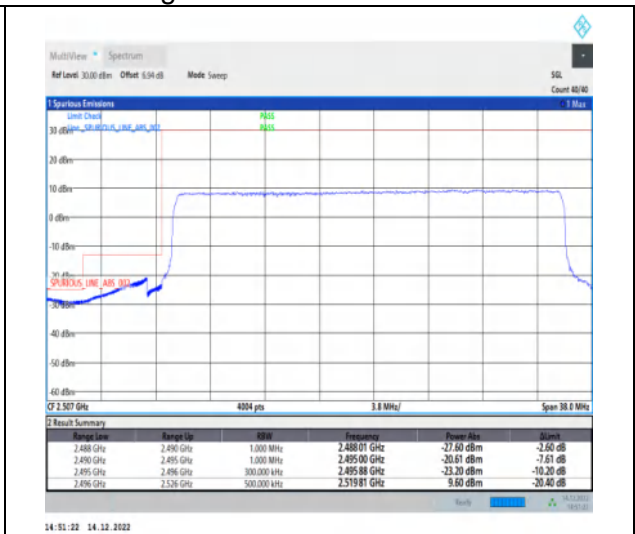
1-N41-30-30-L-3-DFT-PI2BPSK-Outer_Full-75@0-Ant1-1--PASS-see graph
