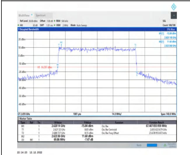
1-N41-30-70-H-6-CP-QPSK-Outer_Full-189@0-Ant1 -67.407-69.860- \leq 70 -PASS
