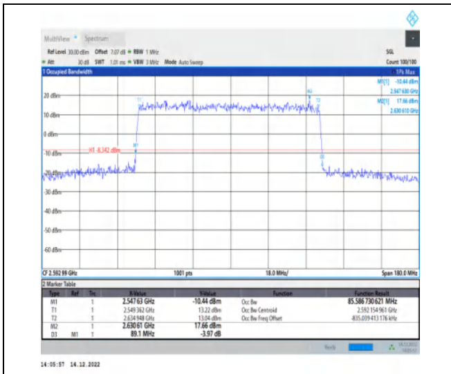
1-N41-30-90-M-3-DFT-16QAM-Outer_Full-240@0-A nt1-85.587-89.100≤90-PASS
