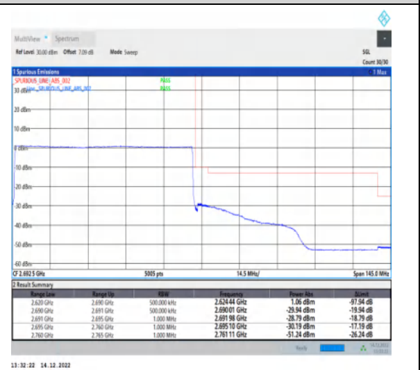
1-N41-30-70-H-6-CP-QPSK-Outer_Full-189@0-Ant1-1--PASS-see graph
