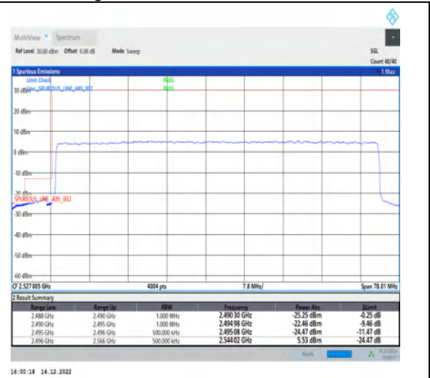
1-N41-30-70-L-3-DFT-PI2BPSK-Outer_Full-180@0-Ant1-1--PASS-see graph
