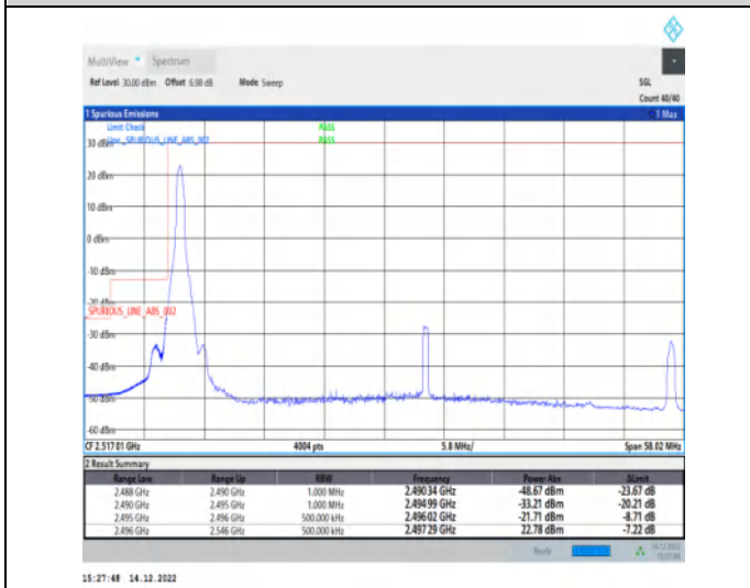
1-N41-30-50-L-4-CP-QPSK-Edge_1RB_Left-1@0-Ant1-1--PASS-see graph
