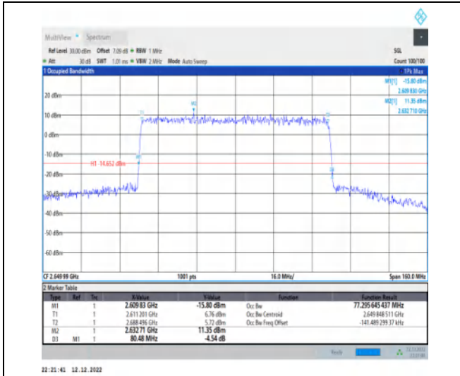
1-N41-30-80-H-9-CP-256QAM-Outer_Full-217@0-A nt1-77.296-80.480- \leq 80 -PASS
