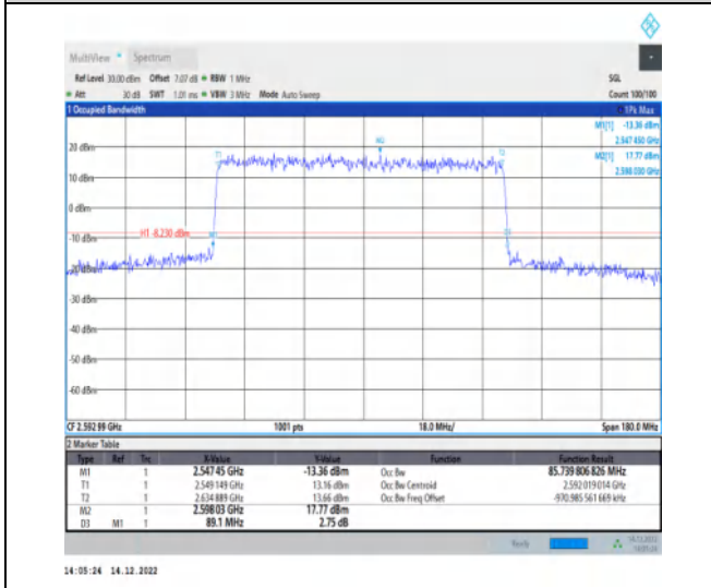
1-N41-30-90-M-1-DFT-QPSK-Outer_Full-240@0-Ant 1-85.74-89.100-≤90-PASS
