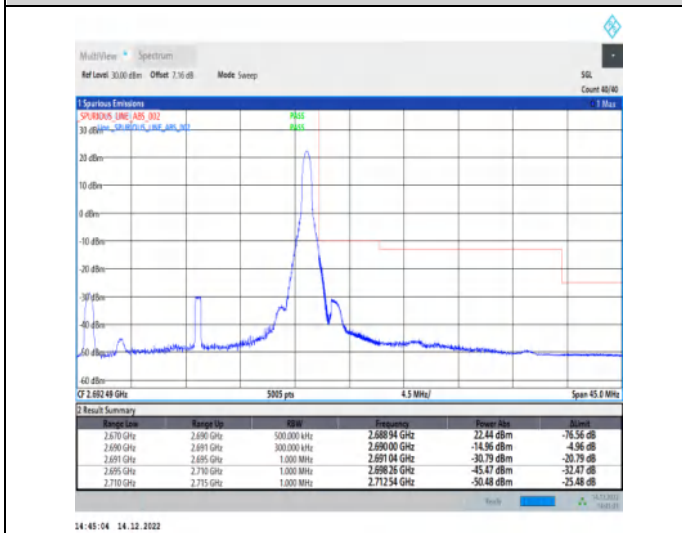
1-N41-30-20-H-5-CP-QPSK-Edge_1RB_Right-1 @ 50-Ant1-1--PASS-see graph
