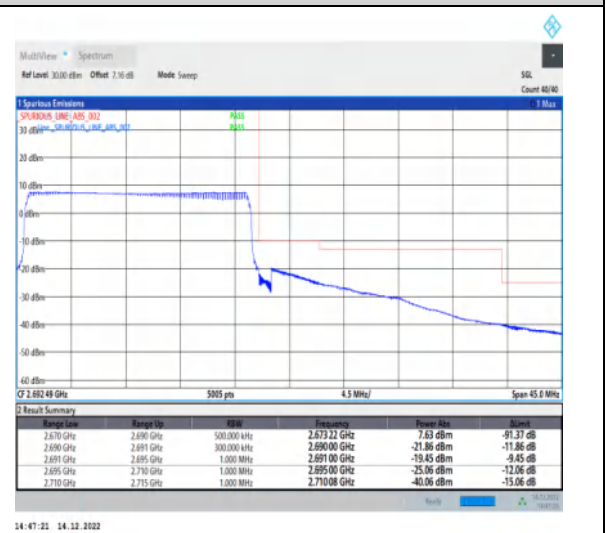
1-N41-30-20-H-6-CP-QPSK-Outer_Full-51@0-Ant1-1--PASS-see graph
