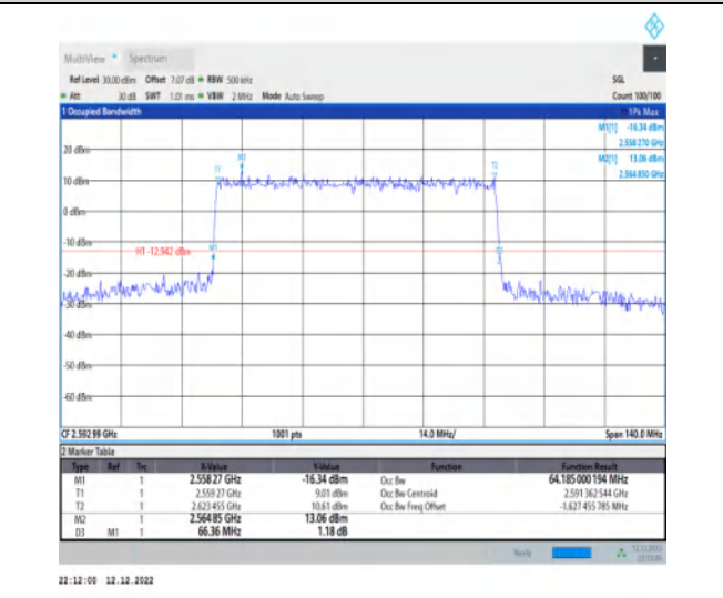
1-N41-30-70-M-4-DFT-64QAM-Outer_Full-180@0-Ant 1-64.185-66.360-≤70-PASS
