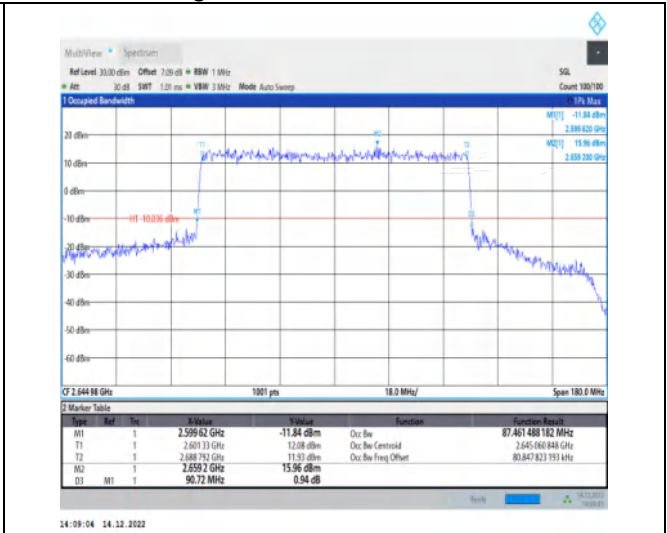
1-N41-30-90-H-7-CP-16QAM-Outer_Full-245@0-Ant1 1-87.461-90.720-≤90-PASS
