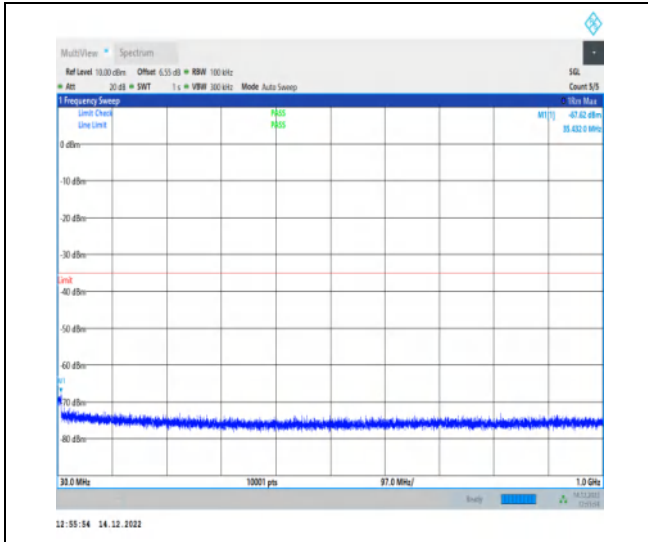
1-N41-30-100-M-1-DFT-QPSK-Edge_1RB_Left-1@ 0-30-1000-Ant1-35.43--67.62--35-PASS
