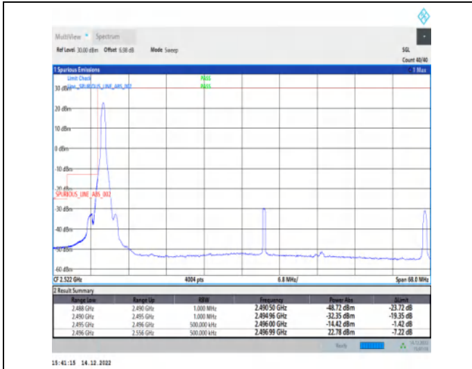
1-N41-30-60-L-1-DFT-PI2BPSK-Edge_1RB_Left-1@0-Ant1-1--PASS-see graph
