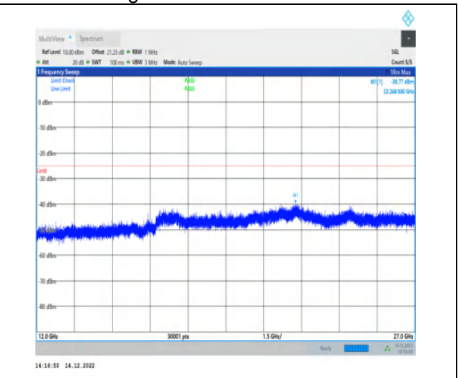
1-N41-30-100-L-1-DFT-PI2BPSK-Inner_1RB_Left-1 @ 1-12000-27000-Ant1-22268.50--39.77--25-PASS
