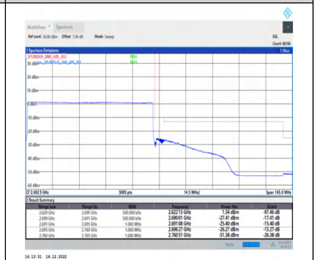
1-N41-30-70-H-6-CP-QPSK-Outer_Full-189@0-Ant1-1--PASS-see graph
