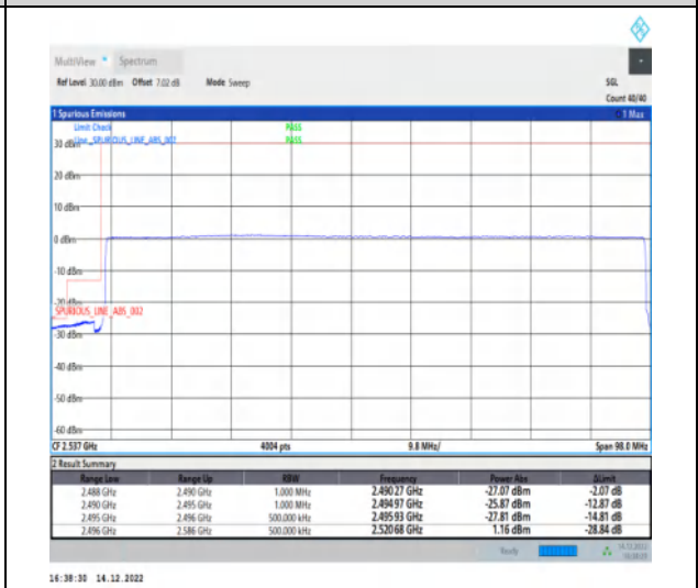
1-N41-30-90-L-6-CP-QPSK-Outer_Full-245@0-Ant1-1--PASS-see graph
