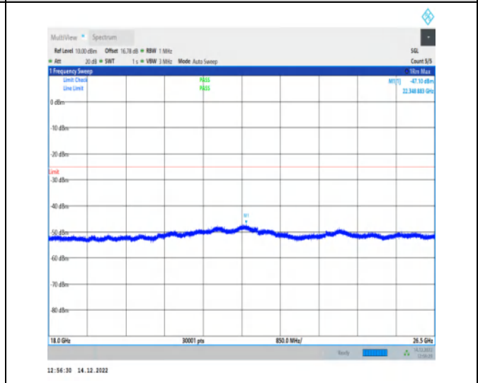
1-N41-30-100-M-1-DFT-QPSK-Edge_1RB_Left-1@0- 18000-26500-Ant1-22348.88--47.10--25-PASS
