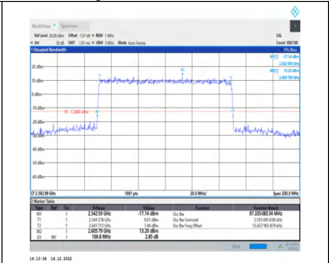
1-N41-30-100-M-9-CP-256QAM-Outer_Full-273@0-A Ant1-97.335-100.800-≤100-PASS
