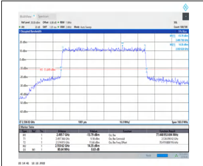
1-N41-30-80-L-7-CP-16QAM-Outer_Full-217@0-Ant 1-77.449-80.640-≤80-PASS
