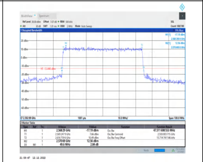
1-N41-30-50-M-6-CP-QPSK-Outer_Full-133@0-Ant1 -47.512-49.600-≤50-PASS
