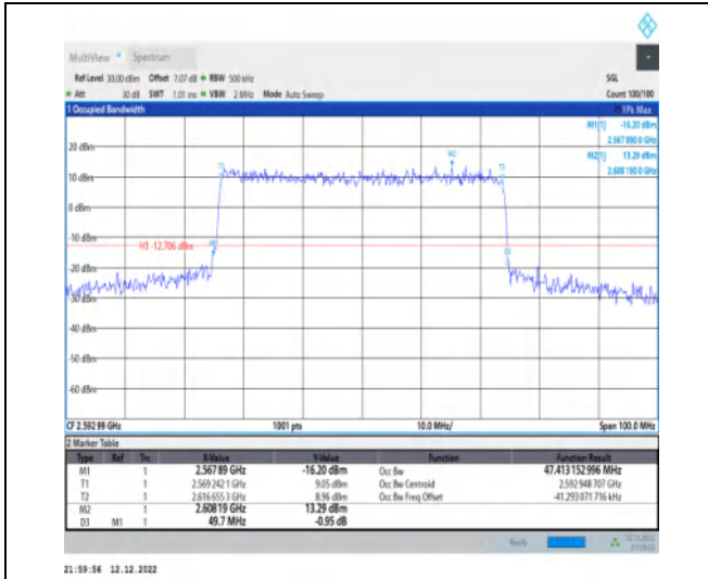
1-N41-30-50-M-7-CP-16QAM-Outer_Full-133@0-An t1-47.413-49.700-≤50-PASS
