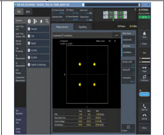
1-N41-30-100-M-6-CP-QPSK-Outer_Full-273@0-Ant1-see graph-PASS
