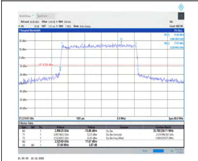
1-N41-30-40-L-1-DFT-QPSK-Outer_Full-100@0-Ant 1-35.76-37.440-≤40-PASS
