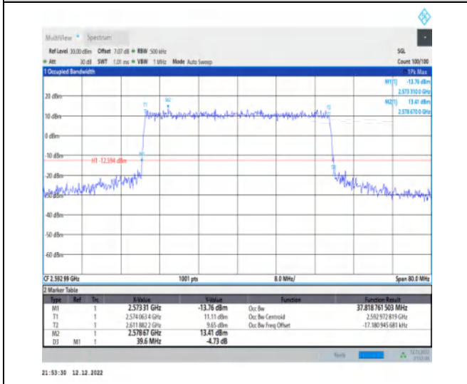
1-N41-30-40-M-8-CP-64QAM-Outer_Full-106@0-Ant t1-37.819-39.600-≤40-PASS
