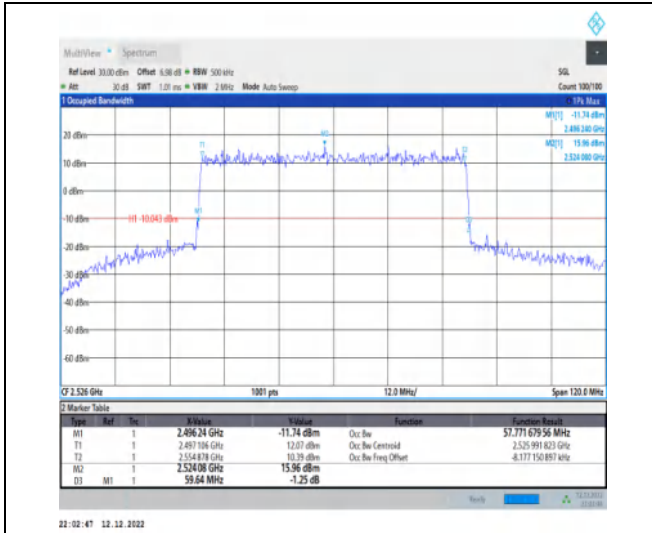
1-N41-30-60-L-1-DFT-QPSK-Outer_Full-162@0-Ant 1-57.772-59.640-≤60-PASS
