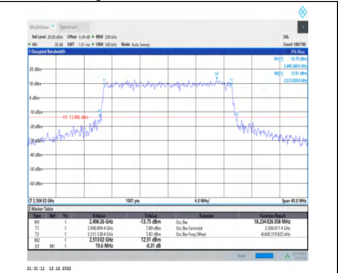
1-N41-30-20-L-6-CP-QPSK-Outer_Full-51@0-Ant1-1 8.234-19.600-≤20-PASS
