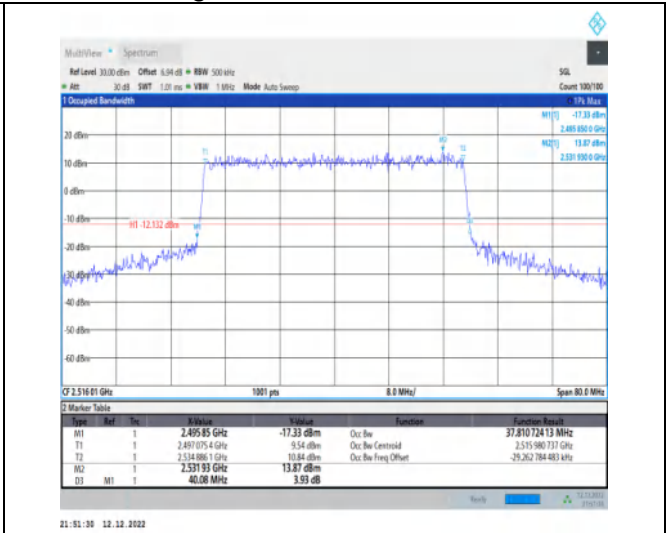
1-N41-30-40-L-8-CP-64QAM-Outer_Full-106@0-Ant 1-37.811-40.080-≤40-PASS
