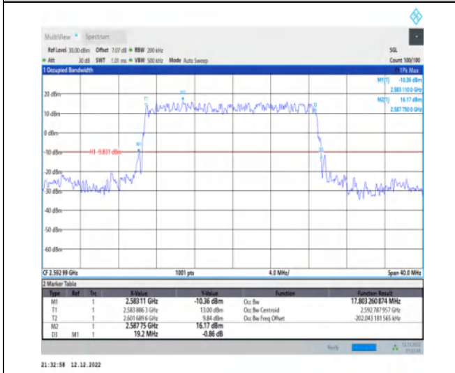
1-N41-30-20-M-2-DFT-PI2BPSK-Outer_Full-50@0-A nt1-17.803-19.200-≤20-PASS
