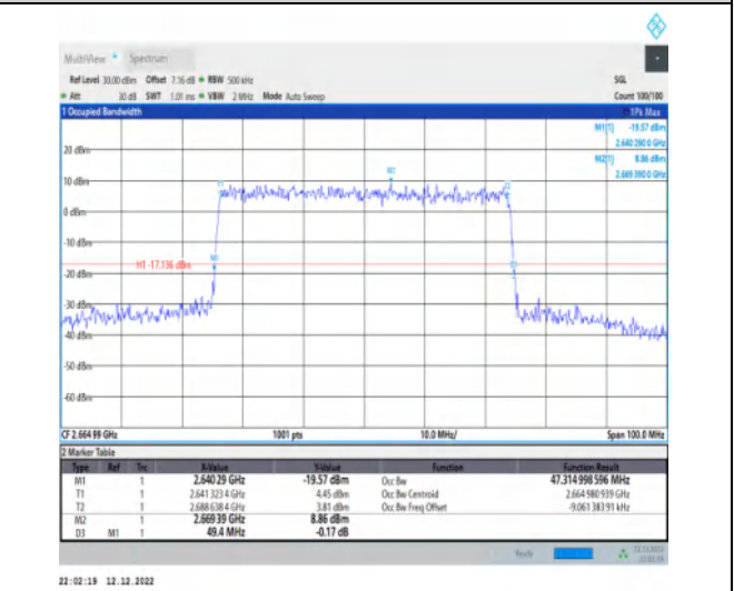
1-N41-30-50-H-9-CP-256QAM-Outer_Full-133@0-A nt1-47.315-49.400-≤50-PASS
