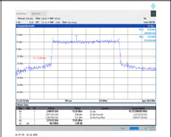
1-N41-30-50-L-7-CP-16QAM-Outer_Full-133@0-Ant 1-47.374-49.400-≤50-PASS
