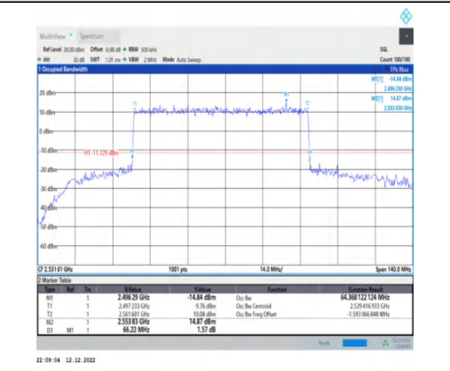
1-N41-30-70-L-1-DFT-QPSK-Outer_Full-180@0-Ant 1-64.368-66.220-≤70-PASS
