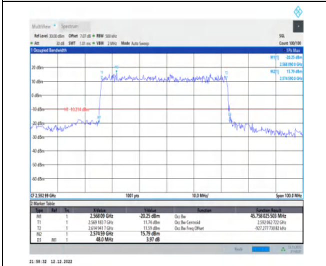
1-N41-30-50-M-1-DFT-QPSK-Outer_Full-128@0-Ant 1-45.758-48.000-≤50-PASS
