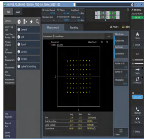
1-N41-30-100-M-4-DFT-64QAM-Outer_Full-270@0-A Ant1-see graph-PASS
