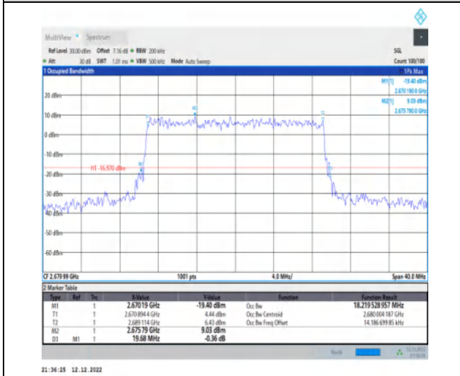
1-N41-30-20-H-9-CP-256QAM-Outer_Full-51@0-Ant 1-18.22-19.680-≤20-PASS
