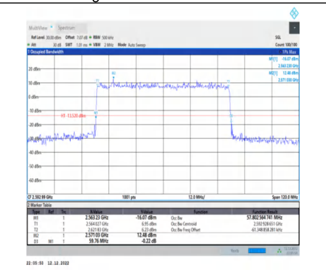
1-N41-30-60-M-5-DFT-256QAM-Outer_Full-162@0-A Ant1-57.803-59.760≤60-PASS
