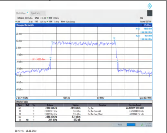
1-N41-30-30-H-9-CP-256QAM-Outer_Full-78@0-Ant 1-27.893-29.400-≤30-PASS
