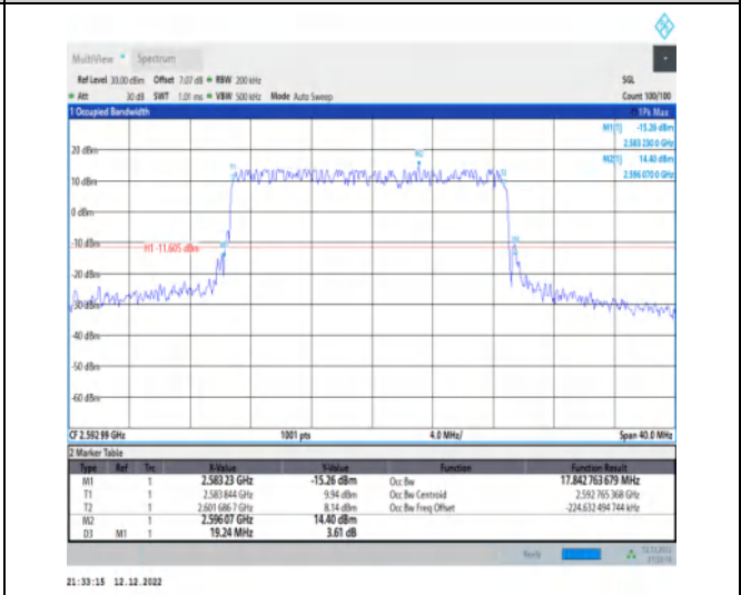
1-N41-30-20-M-3-DFT-16QAM-Outer_Full-50@0-Ant 1-17.843-19.240-≤20-PASS
