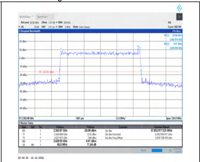
1-N41-30-60-M-9-CP-256QAM-Outer_Full-162@0-A nt1-57.852-60.000-≤60-PASS
