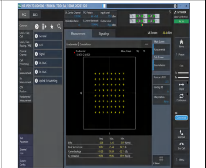
1-N41-30-100-M-8-CP-64QAM-Outer_Full-273@0-Ant1-see graph-PASS
