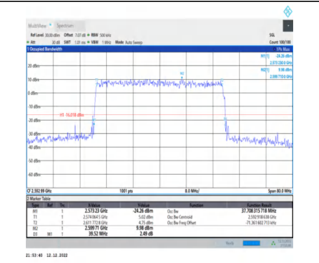
1-N41-30-40-M-9-CP-256QAM-Outer_Full-106@0-Ant nt1-37.708-39.520-≤40-PASS
