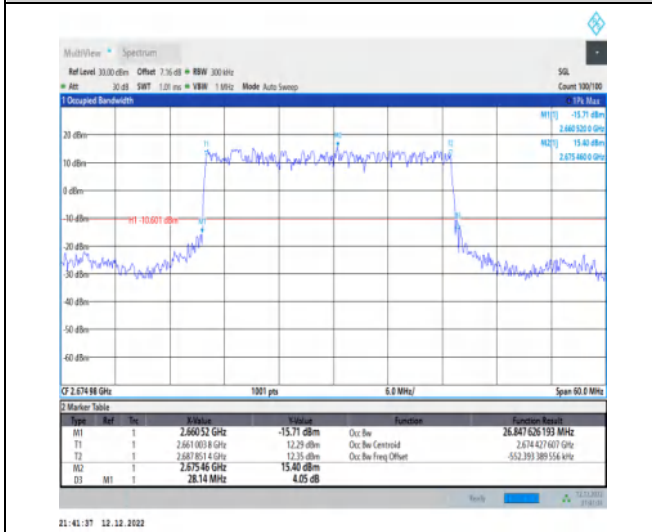
1-N41-30-30-H-2-DFT-PI2BPSK-Outer_Full-75@0-A nt1-26.848-28.140-<30-PASS
