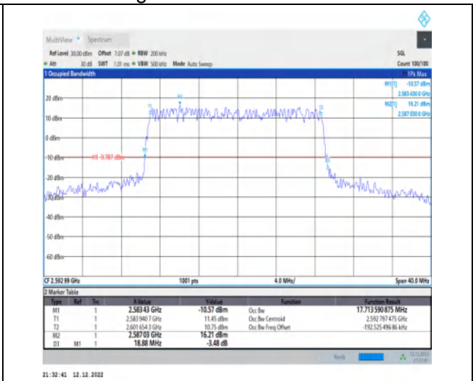
1-N41-30-20-M-1-DFT-QPSK-Outer_Full-50@0-Ant1 -17.714-18.880-≤20-PASS
