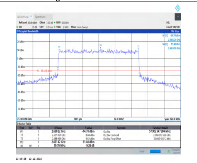
1-N41-30-60-H-8-CP-64QAM-Outer_Full-162@0-Ant 1-57.903-59.760-≤60-PASS
