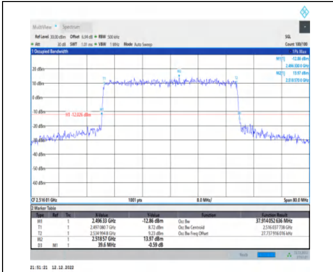
1-N41-30-40-L-7-CP-16QAM-Outer_Full-106@0-Ant 1-37.914-39.600-≤40-PASS
