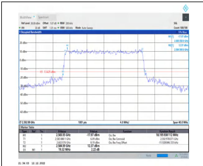
1-N41-30-20-M-8-CP-64QAM-Outer_Full-51@0-Ant 1-18.196-19.320-≤20-PASS
