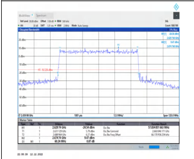
1-N41-30-60-H-9-CP-256QAM-Outer_Full-162@0-A nt1-57.835-60.240-≤60-PASS
