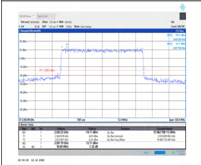
1-N41-30-60-M-6-CP-QPSK-Outer_Full-162@0-Ant 1-57.863-59.640≤60-PASS
