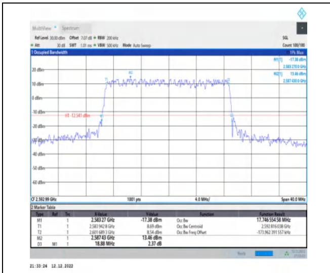
1-N41-30-20-M-4-DFT-64QAM-Outer_Full-50@0-An t1-17.747-18.880-<=20-PASS
