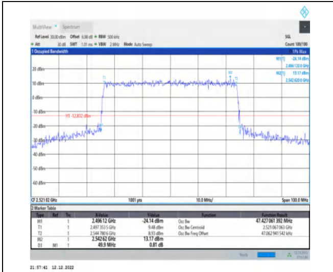
1-N41-30-50-L-8-CP-64QAM-Outer_Full-133@0-Ant 1-47.427-49.900-≤50-PASS
