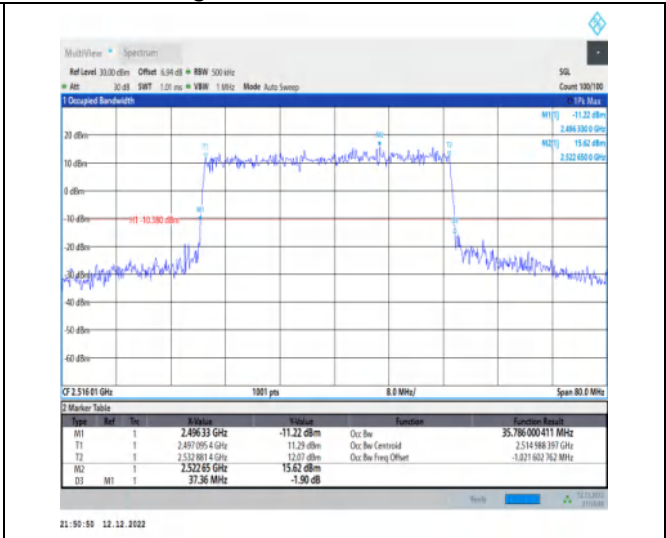
1-N41-30-40-L-4-DFT-64QAM-Outer_Full-100@0-A nt1-35.786-37.360-≤40-PASS
