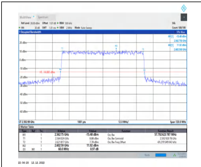
1-N41-30-60-M-8-CP-64QAM-Outer_Full-162@0-An t1-57.793-60.000-≤60-PASS
