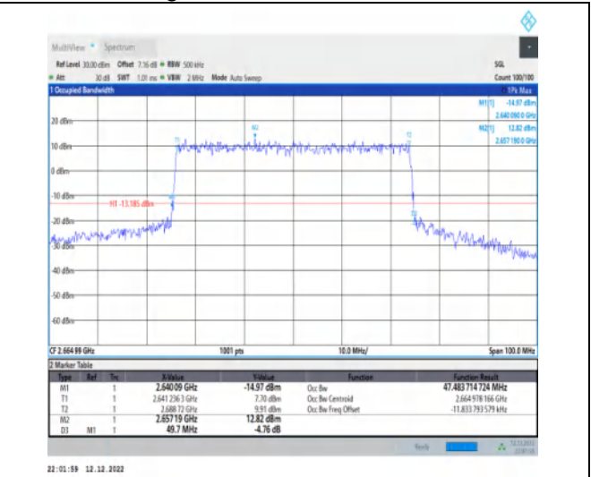
1-N41-30-50-H-7-CP-16QAM-Outer_Full-133@0-Ant 1-47.484-49.700-≤50-PASS
