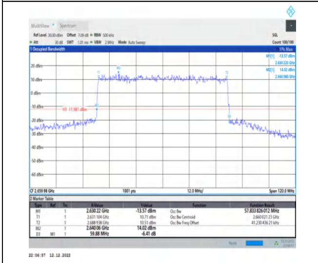
1-N41-30-60-H-1-DFT-QPSK-Outer_Full-162@0-Ant 1-57.834-59.880-≤60-PASS
