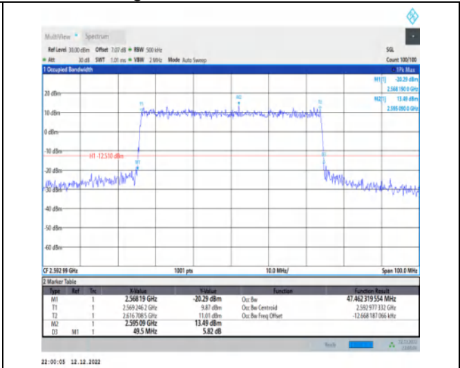
1-N41-30-50-M-8-CP-64QAM-Outer_Full-133@0-Ant 1-47.462-49.500-≤50-PASS
