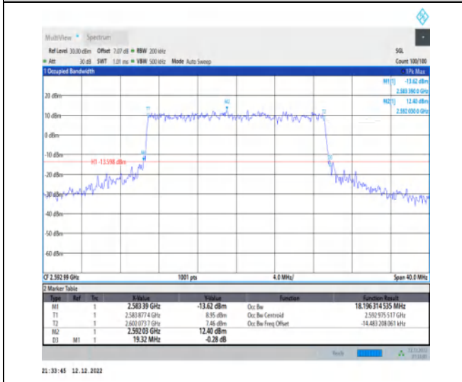
1-N41-30-20-M-6-CP-QPSK-Outer_Full-51@0-Ant1- 18.196-19.320-<=20-PASS
