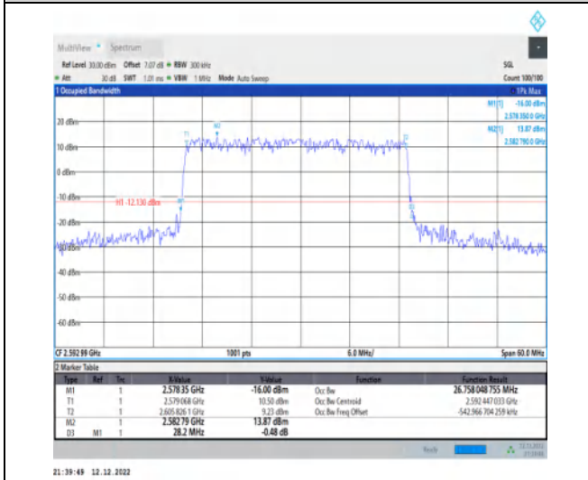
1-N41-30-30-M-3-DFT-16QAM-Outer_Full-75@0-Ant1 t1-26.758-28.200-≤30-PASS
