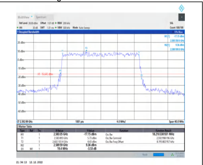
1-N41-30-20-M-9-CP-256QAM-Outer_Full-51@0-Ant 1-18.21-19.400-≤20-PASS
