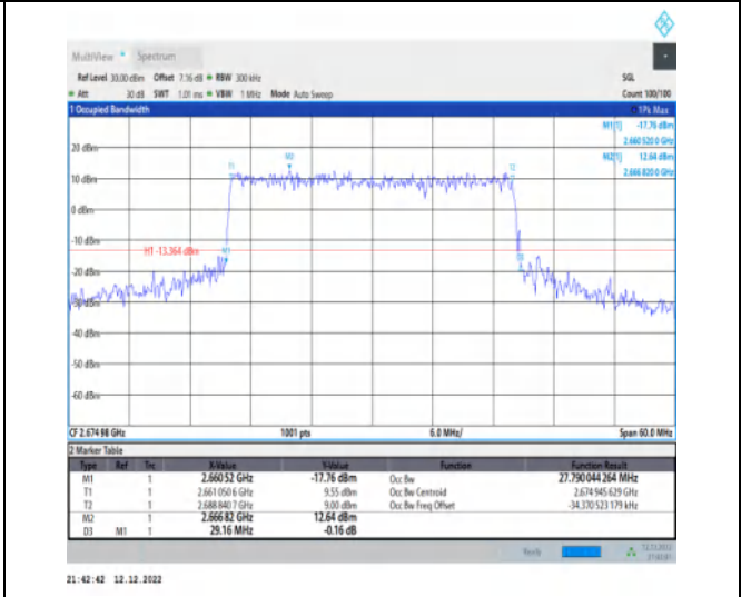
1-N41-30-30-H-7-CP-16QAM-Outer_Full-78@0-Ant1 -27.79-29.160-≤30-PASS
