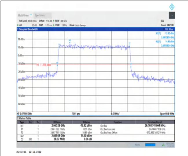
1-N41-30-30-H-4-DFT-64QAM-Outer_Full-75@0-Ant 1-26.769-28.020-≤30-PASS
