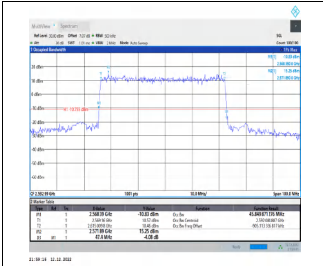
1-N41-30-50-M-3-DFT-16QAM-Outer_Full-128@0-A nt1-45.85-47.400-≤50-PASS
