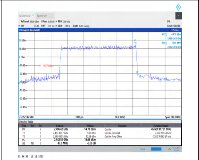
1-N41-30-50-L-3-DFT-16QAM-Outer_Full-128@0-Ant 1-45.602-47.600-≤50-PASS
