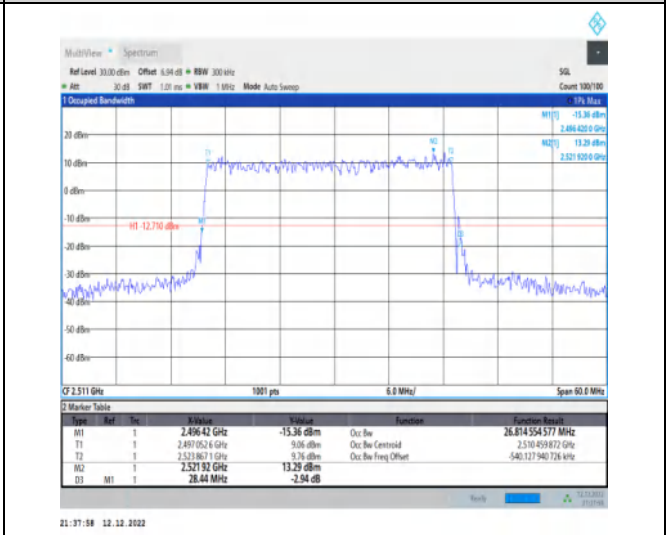
1-N41-30-30-L-5-DFT-256QAM-Outer_Full-75@0-Ant t1-26.815-28.440- \leq 30 -PASS
