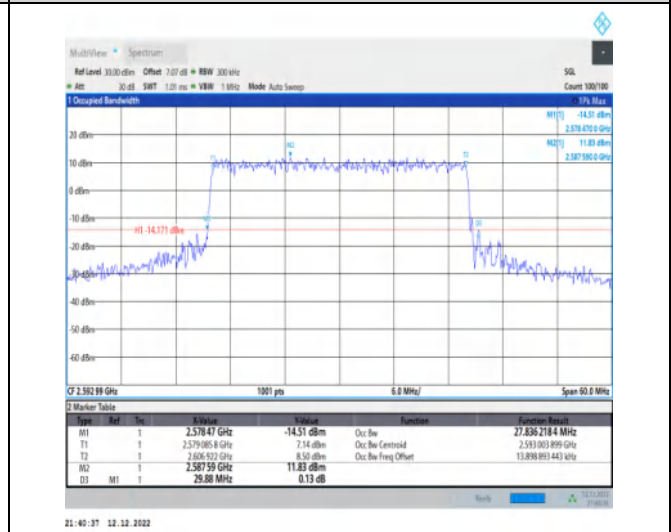
1-N41-30-30-M-8-CP-64QAM-Outer_Full-78@0-Ant1 -27.836-29.880-≤30-PASS
