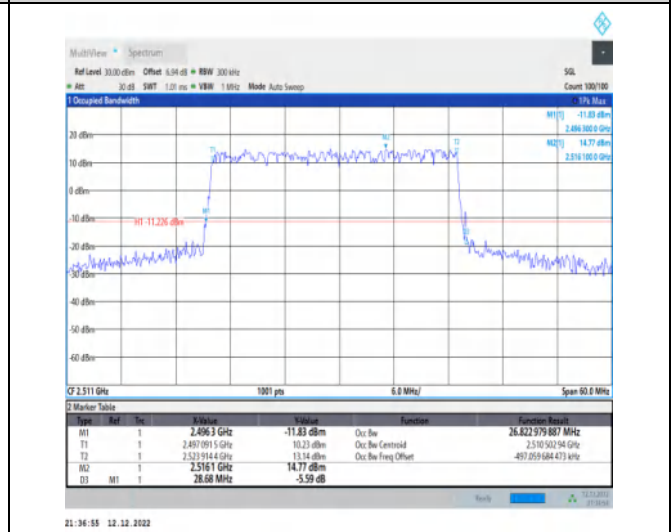
1-N41-30-30-L-1-DFT-QPSK-Outer_Full-75@0-Ant1 26.823-28.680-≤30-PASS
