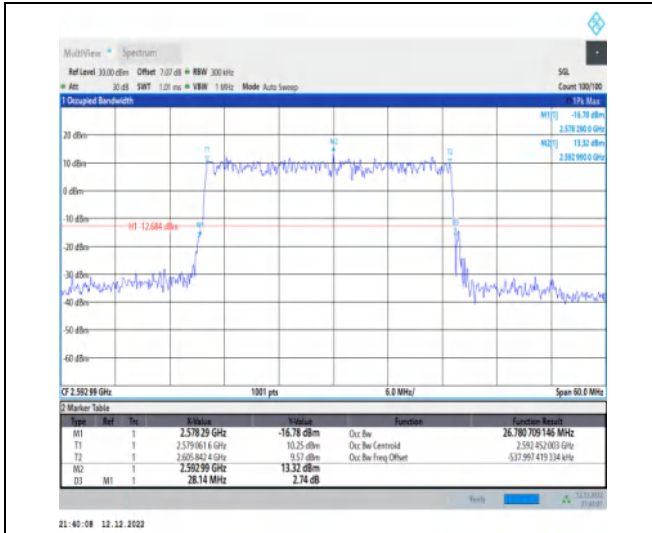
1-N41-30-30-M-5-DFT-256QAM-Outer_Full-75@0-A nt1-26.781-28.140-≤30-PASS
