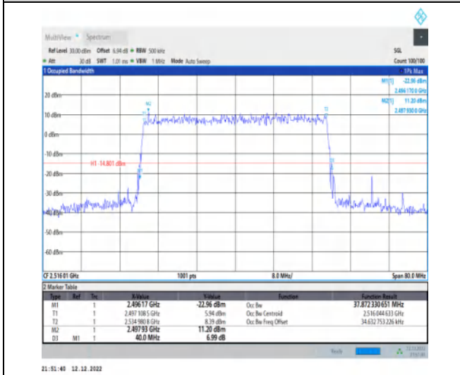
1-N41-30-40-L-9-CP-256QAM-Outer_Full-106@0-A nt1-37.872-40.000-≤40-PASS
