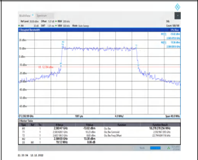
1-N41-30-20-M-7-CP-16QAM-Outer_Full-51@0-Ant1 -18.278-19.120-<=20-PASS
