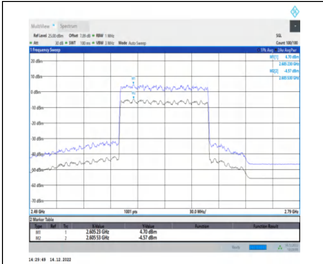
1-N41-30-100-H-1-DFT-256QAM-Outer_Full-270@0 -Ant1-9.27-100%-0.00-9.27-PASS-≤13
