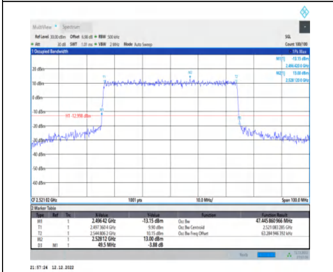
1-N41-30-50-L-6-CP-QPSK-Outer_Full-133@0-Ant1 -47.446-49.500-≤50-PASS
