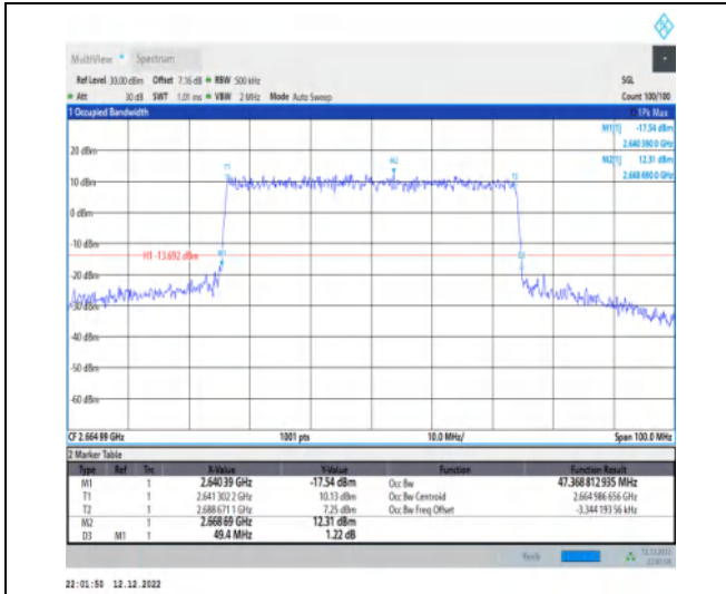
1-N41-30-50-H-6-CP-QPSK-Outer_Full-133@0-Ant1 -47.369-49.400-≤50-PASS
