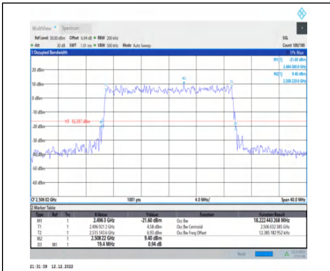
1-N41-30-20-L-9-CP-256QAM-Outer_Full-51@0-Ant 1-18.222-19.400-≤20-PASS
