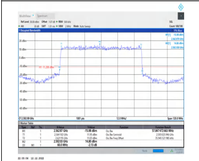
1-N41-30-60-M-2-DFT-PI2BPSK-Outer_Full-162@0-Ant1 Ant1-57.847-60.000-≤60-PASS
