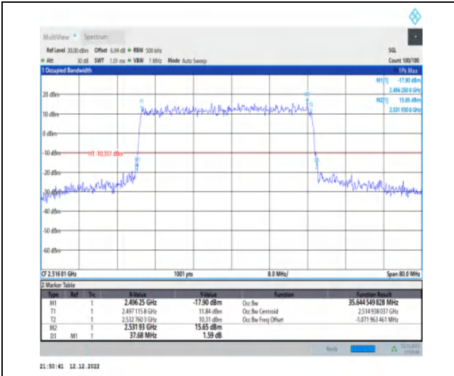
1-N41-30-40-L-3-DFT-16QAM-Outer_Full-100@0-A nt1-35.645-37.680-≤40-PASS
