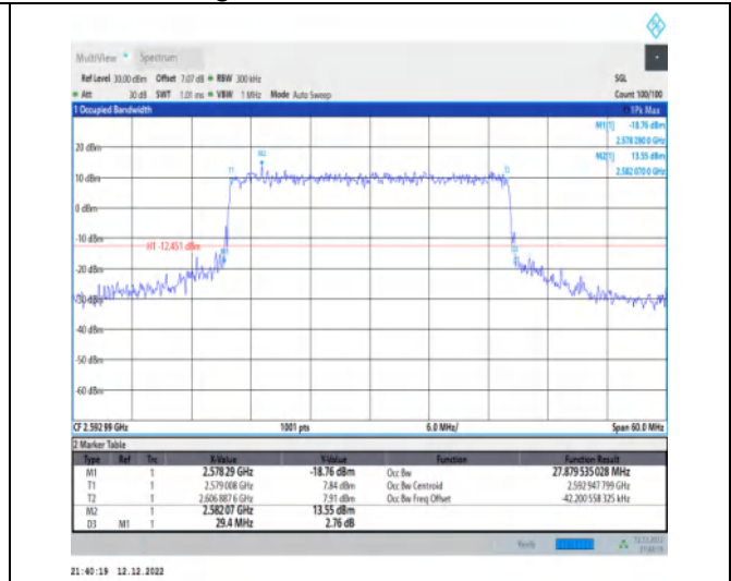
1-N41-30-30-M-6-CP-QPSK-Outer_Full-78@0-Ant1- 27.88-29.400-≤30-PASS
