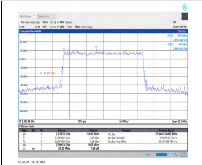
1-N41-30-30-M-9-CP-256QAM-Outer_Full-78@0-An t1-27.944-29.220-<30-PASS
