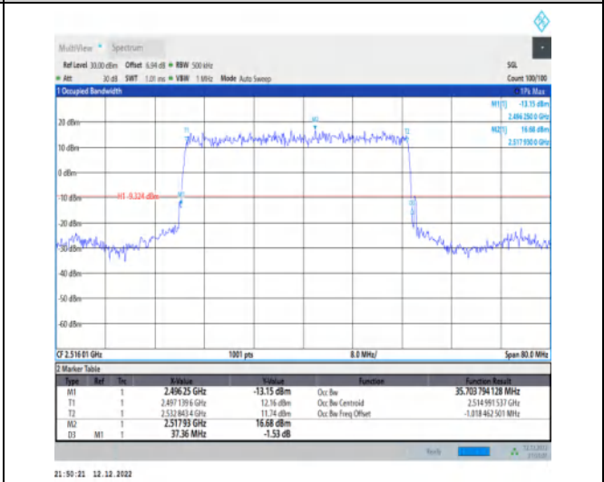
1-N41-30-40-L-2-DFT-PI2BPSK-Outer_Full-100@0-Ant 1-35.704-37.360-≤40-PASS
