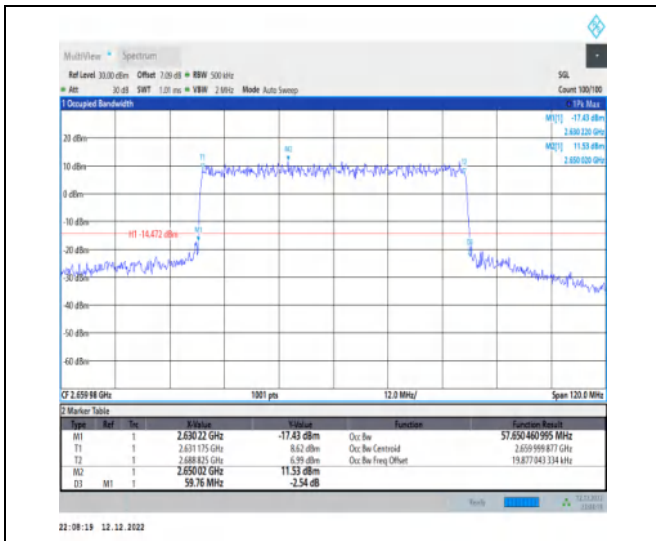
1-N41-30-60-H-7-CP-16QAM-Outer_Full-162@0-Ant 1-57.65-59.760-≤60-PASS
