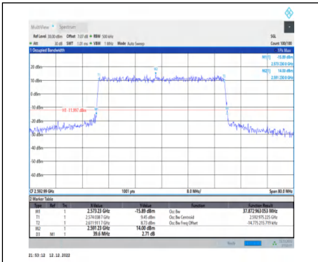
1-N41-30-40-M-6-CP-QPSK-Outer_Full-106@0-Ant 1-37.873-39.600-≤40-PASS
