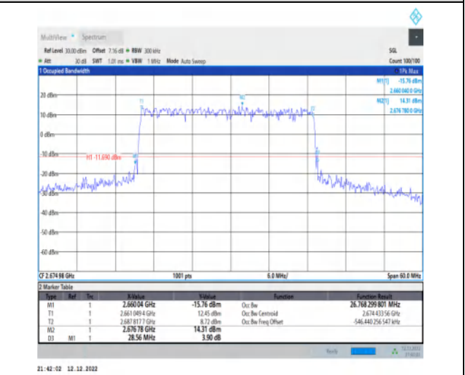
1-N41-30-30-H-3-DFT-16QAM-Outer_Full-75@0-Ant 1-26.768-28.560-<30-PASS
