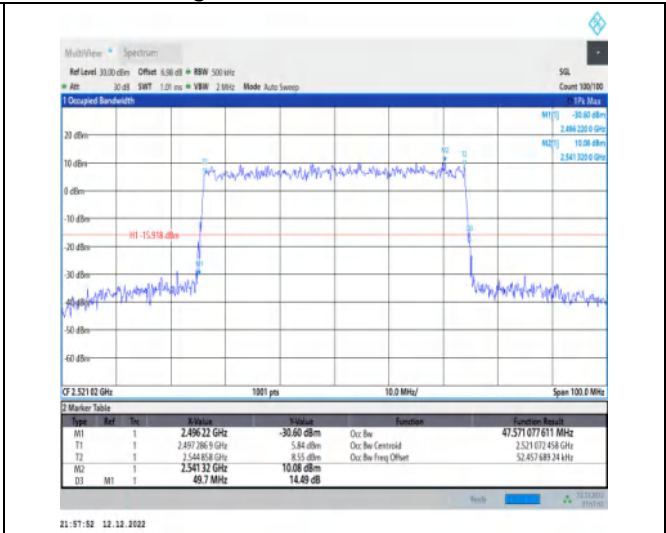
1-N41-30-50-L-9-CP-256QAM-Outer_Full-133@0-Ant t1-47.571-49.700-≤50-PASS
