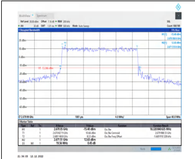
1-N41-30-20-H-7-CP-16QAM-Outer_Full-51@0-Ant1 -18.321-19.560-≤20-PASS
