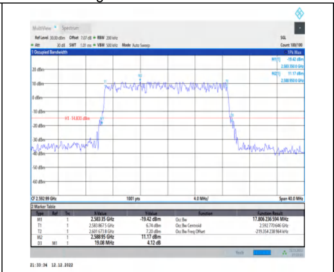
1-N41-30-20-M-5-DFT-256QAM-Outer_Full-50@0-A nt1-17.806-19.080-<=20-PASS
