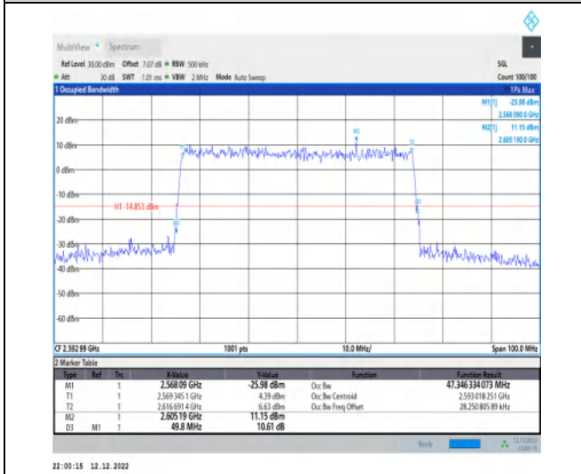
1-N41-30-50-M-9-CP-256QAM-Outer_Full-133@0-A nt1-47.346-49.800-≤50-PASS
