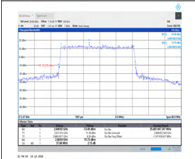
1-N41-30-40-H-3-DFT-16QAM-Outer_Full-100@0-Ant 1-35.681-37.680-≤40-PASS
