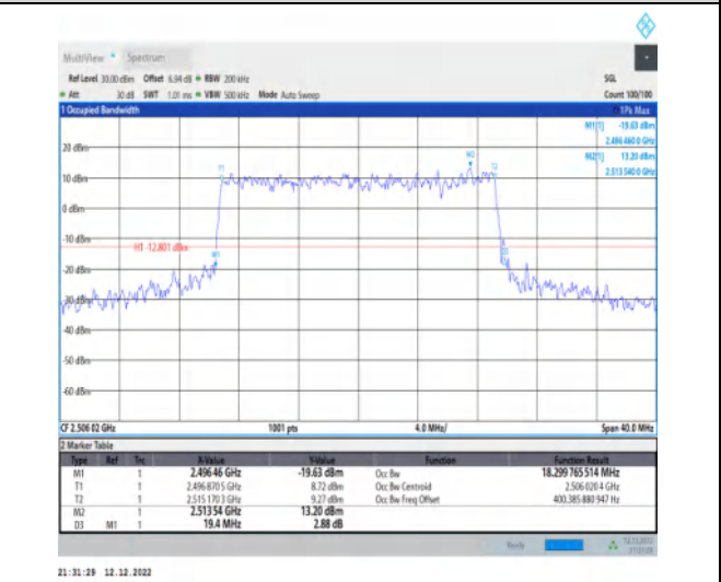
1-N41-30-20-L-8-CP-64QAM-Outer_Full-51@0-Ant1-1 18.3-19.400-≤20-PASS
