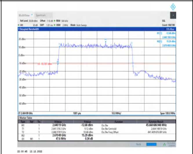
1-N41-30-50-H-1-DFT-QPSK-Outer_Full-128@0-Ant 1-45.661-47.600-≤50-PASS
