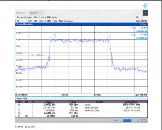
1-N41-30-30-H-5-DFT-256QAM-Outer_Full-75@0-Ant t1-26.876-28.200-≤30-PASS
