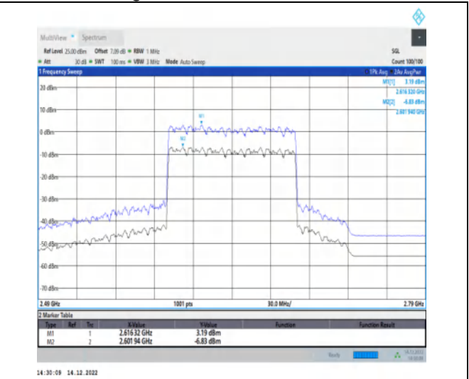
1-N41-30-100-H-2-CP-256QAM-Outer_Full-273@0-A nt1-10.02-100%-0.00-10.02-PASS-≤13
