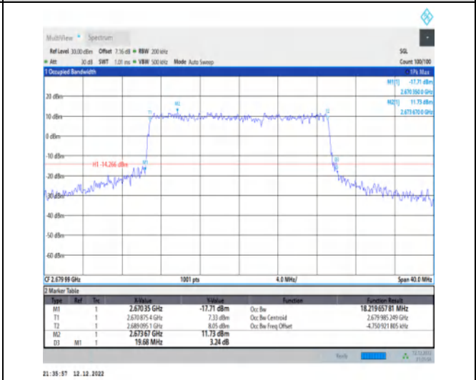
1-N41-30-20-H-6-CP-QPSK-Outer_Full-51@0-Ant1 18.22-19.680-≤20-PASS
