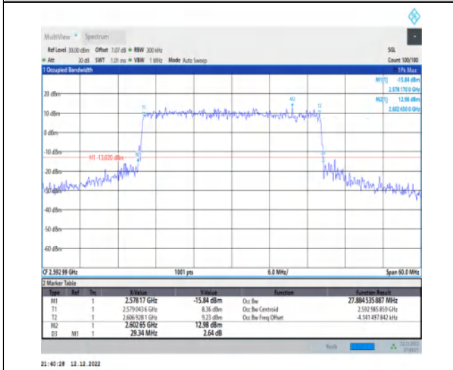
1-N41-30-30-M-7-CP-16QAM-Outer_Full-78@0-Ant 1-27.885-29.340-≤30-PASS
