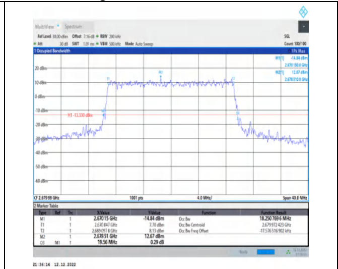
1-N41-30-20-H-8-CP-64QAM-Outer_Full-51@0-Ant1 -18.251-19.560-≤20-PASS
