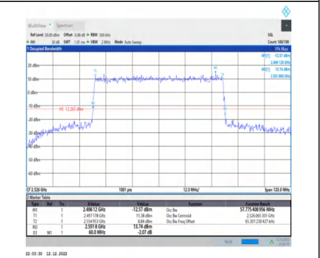
1-N41-30-60-L-4-DFT-64QAM-Outer_Full-162@0-Ant 1-57.775-60.000-≤60-PASS
