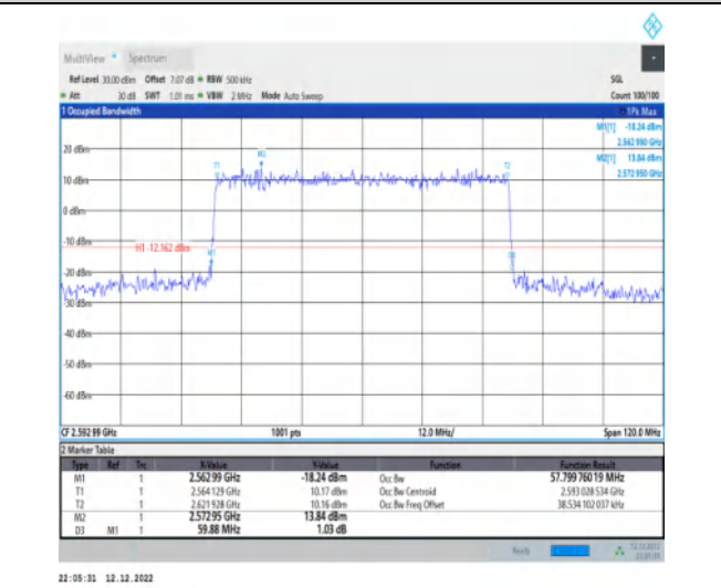
1-N41-30-60-M-3-DFT-16QAM-Outer_Full-162@0-A nt1-57.8-59.880-≤60-PASS
