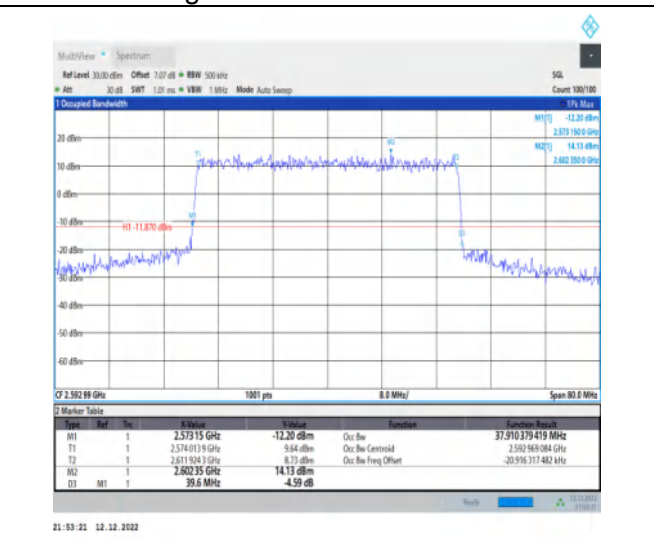
1-N41-30-40-M-7-CP-16QAM-Outer_Full-106@0-Ant 1-37.91-39.600-≤40-PASS
