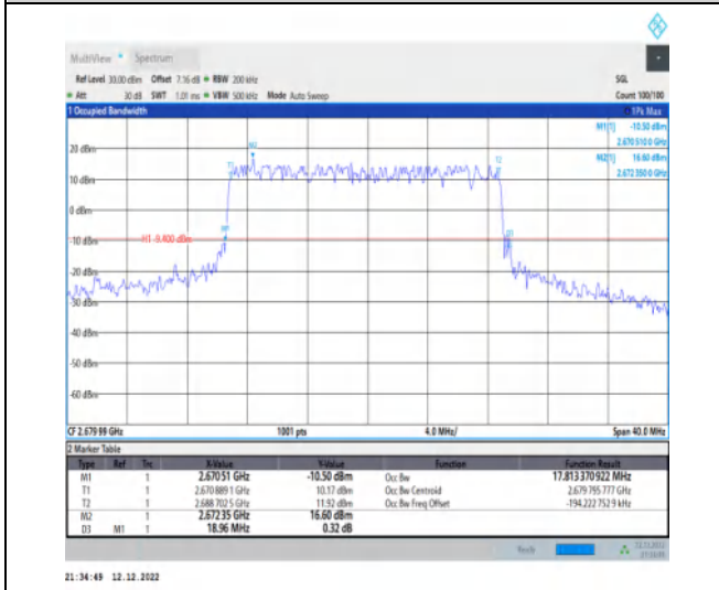
1-N41-30-20-H-1-DFT-QPSK-Outer_Full-50@0-Ant1 -17.813-18.960-≤20-PASS
