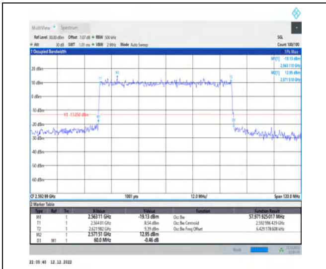
1-N41-30-60-M-4-DFT-64QAM-Outer_Full-162@0-A nt1-57.972-60.000≤60-PASS
