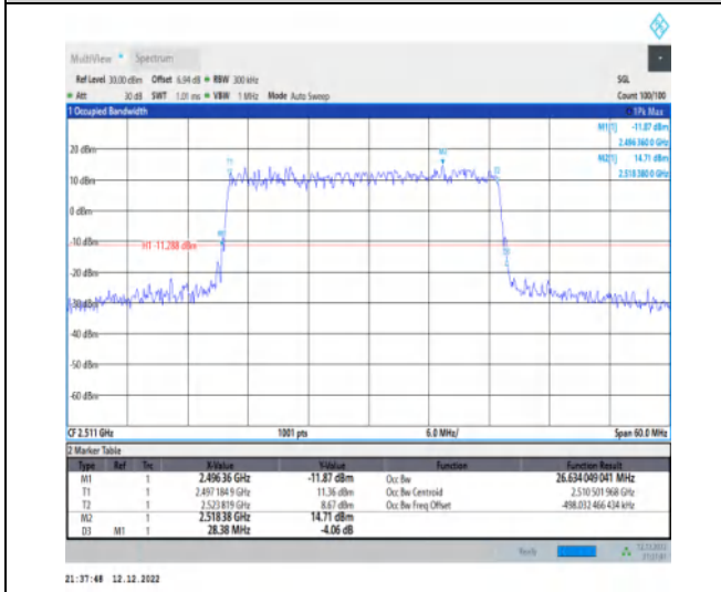
1-N41-30-30-L-4-DFT-64QAM-Outer_Full-75@0-Ant 1-26.634-28.380- \leq 30 -PASS
