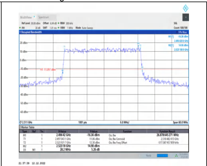
1-N41-30-30-L-3-DFT-16QAM-Outer_Full-75@0-Ant 1-26.879-28.200- \leq 30 -PASS
