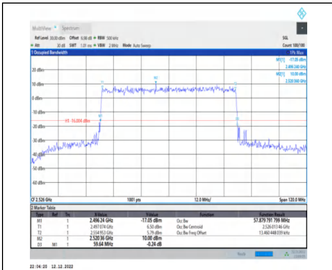
1-N41-30-60-L-9-CP-256QAM-Outer_Full-162@0-A nt1-57.88-59.640-≤60-PASS
