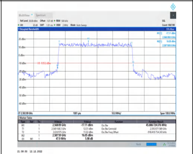
1-N41-30-50-M-2-DFT-PI2BPSK-Outer_Full-128@0-Ant Ant1-45.807-47.900-≤50-PASS
