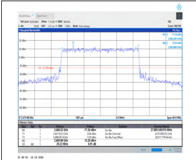
1-N41-30-30-H-8-CP-64QAM-Outer_Full-78@0-Ant1 -27.896-29.220-≤30-PASS
