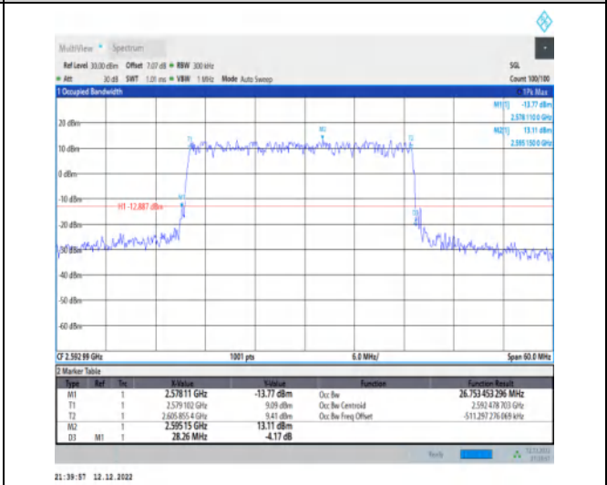
1-N41-30-30-M-4-DFT-64QAM-Outer_Full-75@0-Ant1 1-26.753-28.260-≤30-PASS
