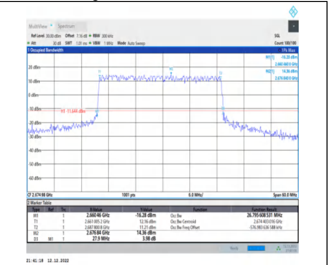
1-N41-30-30-H-1-DFT-QPSK-Outer_Full-75@0-Ant1- 26.796-27.900-<30-PASS
