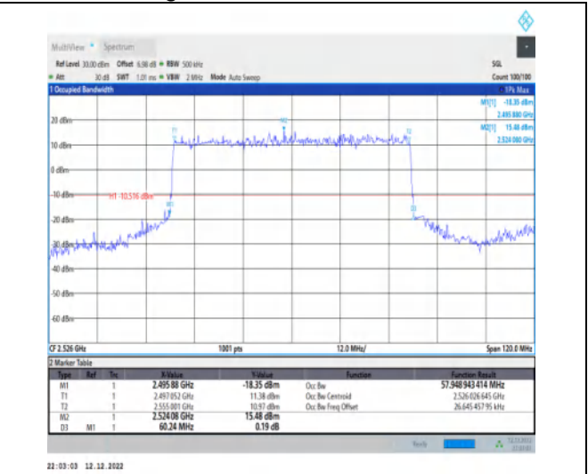
1-N41-30-60-L-2-DFT-PI2BPSK-Outer_Full-162@0-Ant 1-57.949-60.240-≤60-PASS
