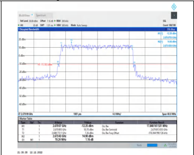
1-N41-30-20-H-4-DFT-64QAM-Outer_Full-50@0-Ant 1-17.84-19.240-≤20-PASS
