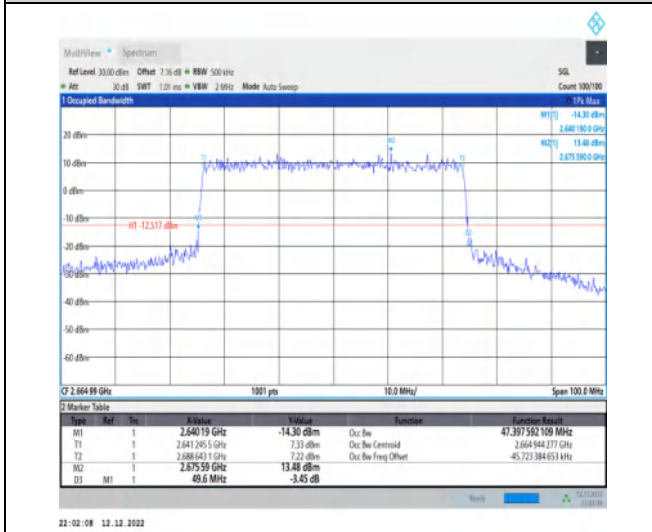
1-N41-30-50-H-8-CP-64QAM-Outer_Full-133@0-Ant 1-47.398-49.600-≤50-PASS
