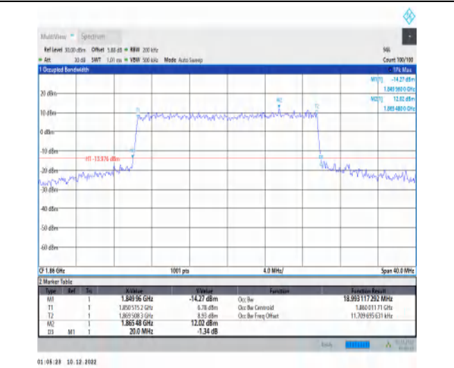
1-N25-15-20-L-7-CP-16QAM-Outer_Full-106@0-Ant 1-18.993-20.000-≤20-PASS
