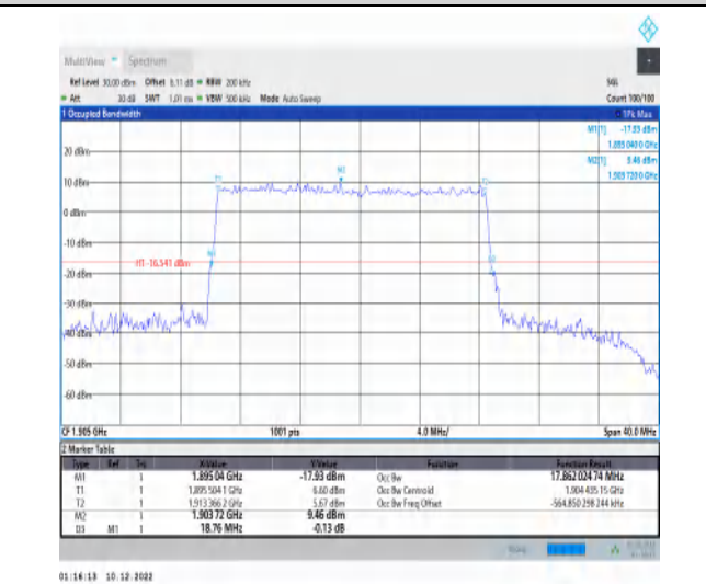
1-N25-15-20-H-1-DFT-QPSK-Outer_Full-100@0-Ant 1-0.313-0.480-≤20-PASS
