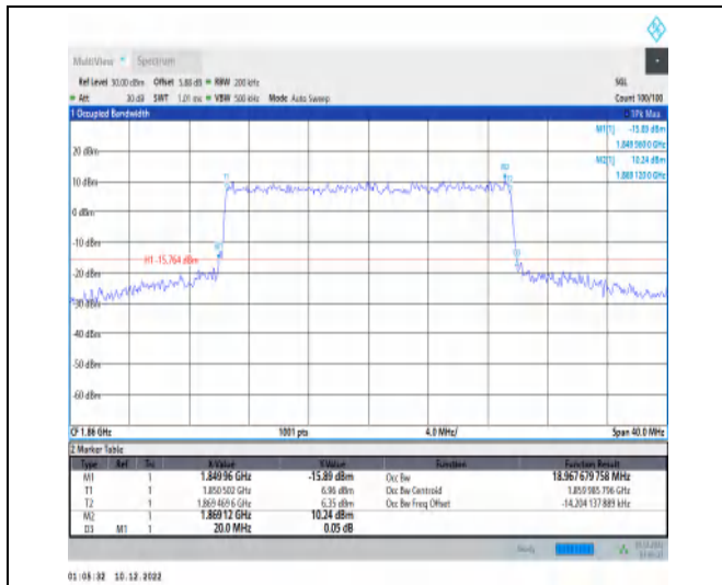
1-N25-15-20-L-8-CP-64QAM-Outer_Full-106@0-Ant 1-18.968-20.000-≤20-PASS
