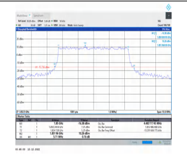
1-N25-15-5-L-4-DFT-64QAM-Outer_Full-25@0-Ant1-4 4.483-5.110-≤5-PASS
