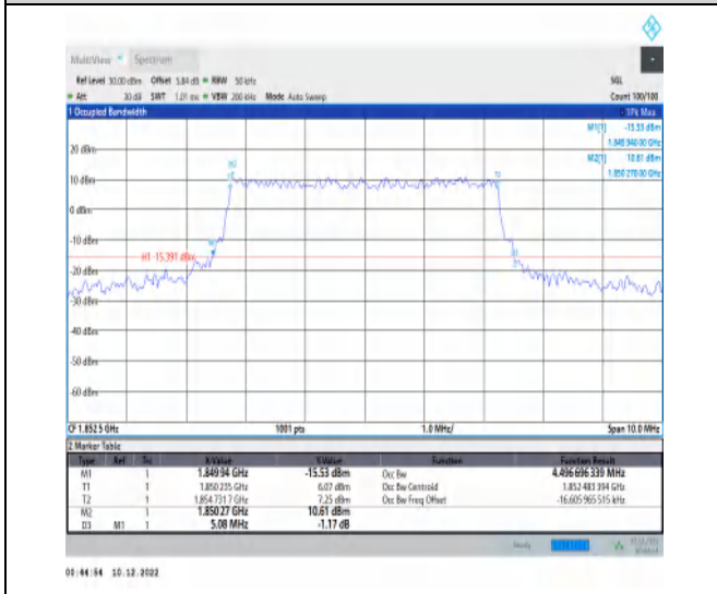
1-N25-15-5-L-3-DFT-16QAM-Outer_Full-25@0-Ant1-4 -4.497-5.080-≤5-PASS
