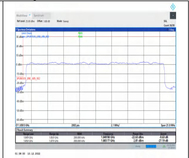
1-N25-15-20-L-3-DFT-PI2BPSK-Outer_Full-100@0-Ant1-1-seegraph-PASS-see graph
