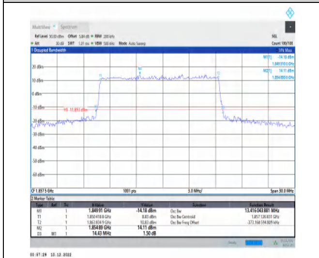
1-N25-15-15-L-1-DFT-QPSK-Outer_Full-75@0-Ant1- 13.416-14.430-≤15-PASS
