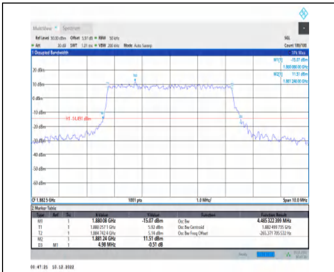
1-N25-15-5-M-4-DFT-64QAM-Outer_Full-25@0-Ant1 -4.485-4.980-≤5-PASS
