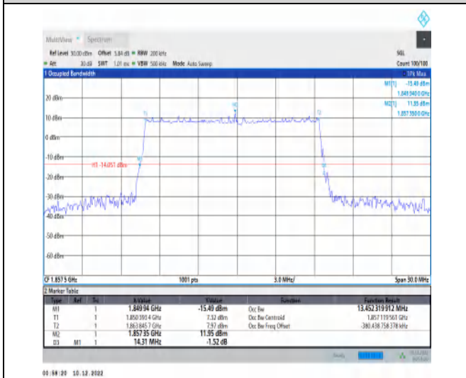
1-N25-15-15-L-5-DFT-256QAM-Outer_Full-75@0-Ant t1-13.452-14.310-≤15-PASS
