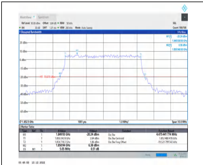
1-N25-15-5-L-9-CP-256QAM-Outer_Full-25@0-Ant1 -4.475-5.050-≤5-PASS
