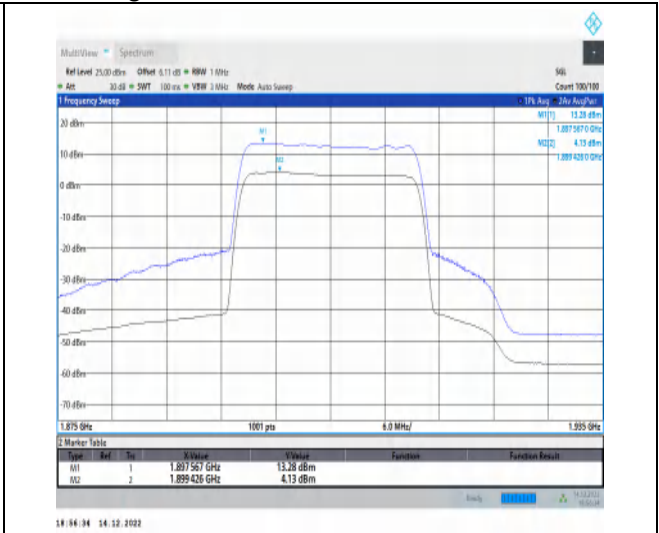
1-N25-15-20-H-2-CP-256QAM-Outer_Full-106@0-A nt1-9.15-100%-0.00-9.15-PASS-≤13
