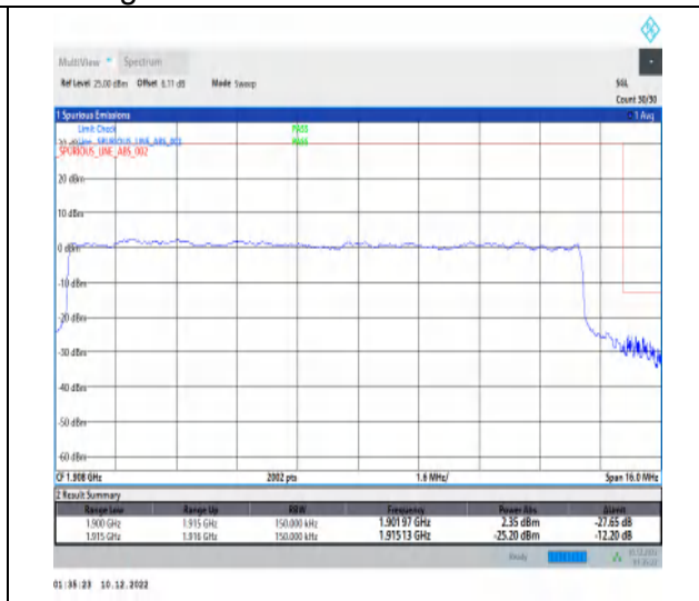
1-N25-15-15-H-3-DFT-PI2BPSK-Outer_Full-75@0-Ant1-1-seegraph-PASS-see graph
