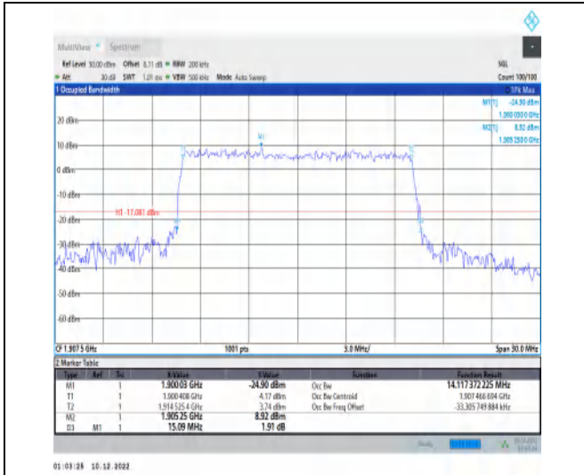
1-N25-15-15-H-9-CP-256QAM-Outer_Full-79@0-Ant 1-14.117-15.090≤15-PASS
