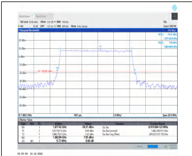
1-N25-15-10-M-5-DFT-256QAM-Outer_Full-50@0-A nt1-8.919-9.720≤10-PASS
