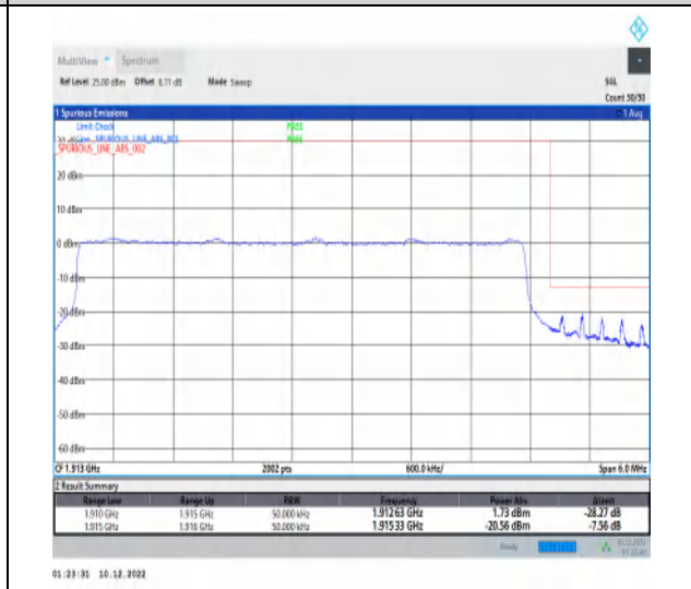
1-N25-15-5-H-6-CP-QPSK-Outer_Full-25@0-Ant1-1-seegraph-PASS-see graph
