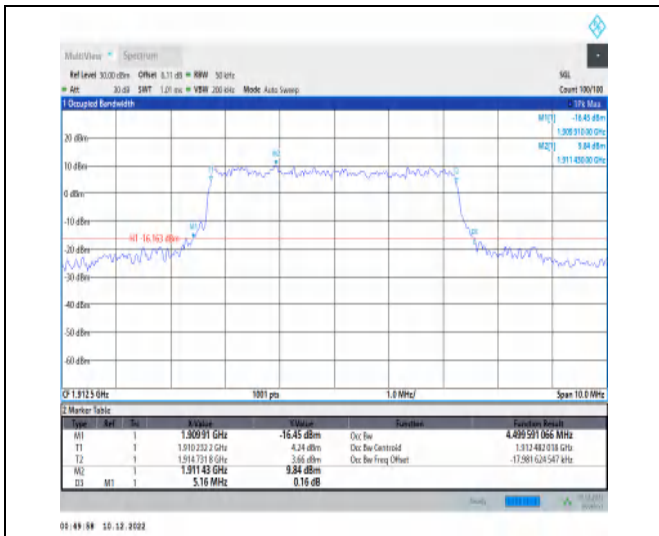
1-N25-15-5-H-7-CP-16QAM-Outer_Full-25@0-Ant1-4.5-5.160-<math>\leq</math>5-PASS
