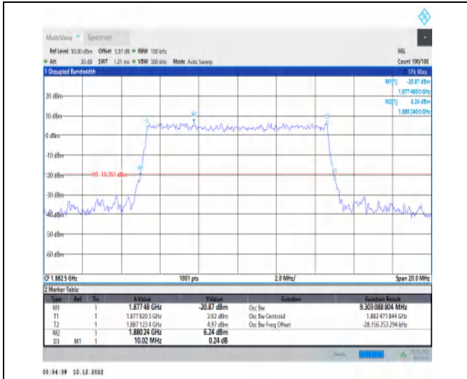
1-N25-15-10-M-9-CP-256QAM-Outer_Full-52@0-An t1-9.303-10.020-≤10-PASS
