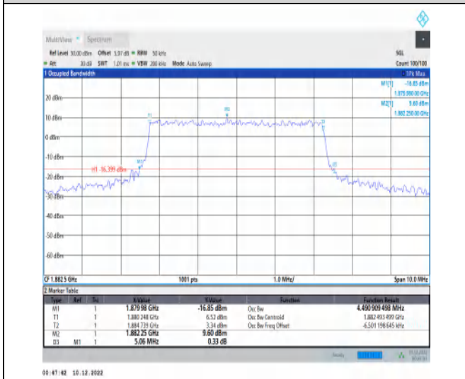
1-N25-15-5-M-6-CP-QPSK-Outer_Full-25@0-Ant1-4 .491-5.060-≤5-PASS
