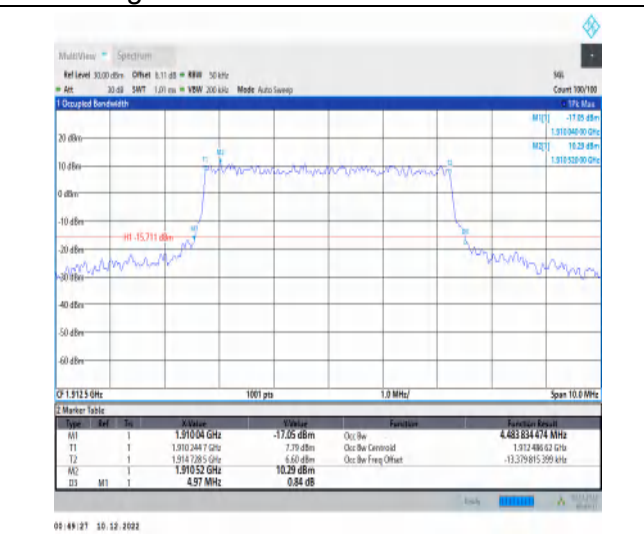
1-N25-15-5-H-4-DFT-64QAM-Outer_Full-25@0-Ant1 -4.484-4.970-≤5-PASS
