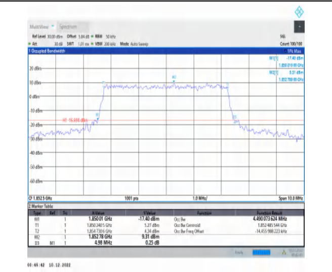
1-N25-15-5-L-8-CP-64QAM-Outer_Full-25@0-Ant1-4 .49-4.980-≤5-PASS
