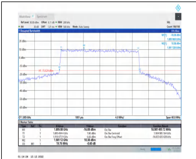
1-N25-15-20-H-6-CP-QPSK-Outer_Full-106@0-Ant1 -18.981-19.760-≤20-PASS
