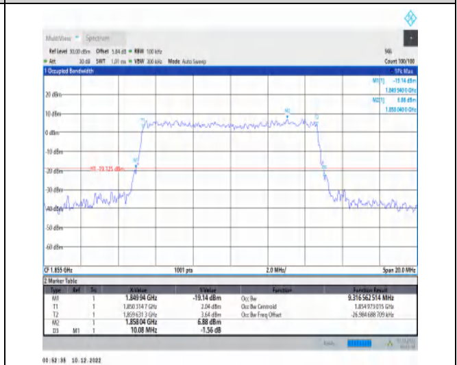
1-N25-15-10-L-9-CP-256QAM-Outer_Full-52@0-Ant1-9.317-10.080-≤10-PASS
