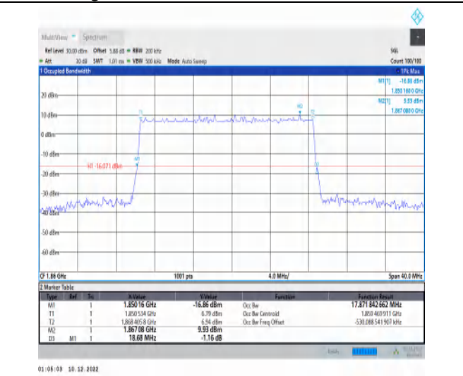
1-N25-15-20-L-5-DFT-256QAM-Outer_Full-100@0-A nt1-17.872-18.680-≤20-PASS
