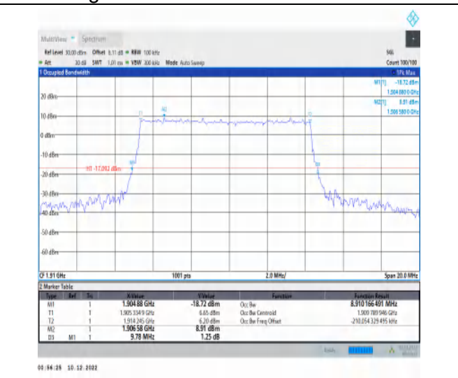
1-N25-15-10-H-5-DFT-256QAM-Outer_Full-50@0-A nt1-8.91-9.780≤10-PASS
