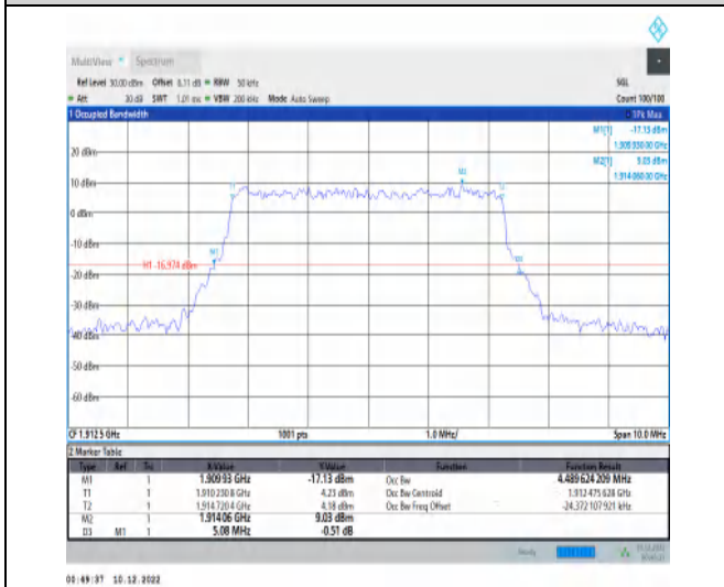
1-N25-15-5-H-5-DFT-256QAM-Outer_Full-25@0-Ant 1-4.49-5.080-≤5-PASS
