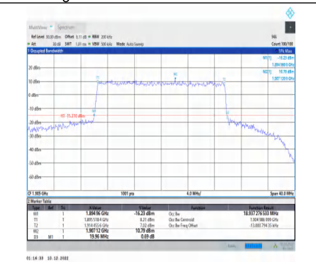
1-N25-15-20-H-7-CP-16QAM-Outer_Full-106@0-Ant 1-18.937-19.960-≤20-PASS
