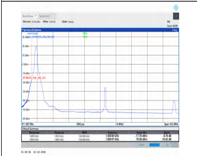
1-N25-15-15-L-4-CP-QPSK-Edge_1RB_Left-1@0-Ant1-1-seegraph-PASS-see graph
