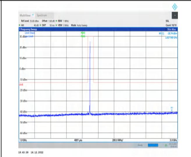
1-N25-15-20-H-1-DFT-PI2BPSK-Inner_1RB_Left-1 @ 1-1000-3000-Ant1-2927.50--39.74--13-PASS
