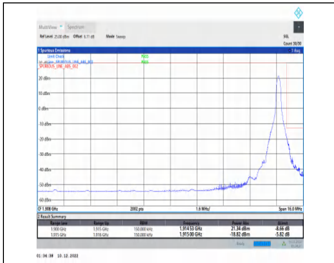
1-N25-15-15-H-2-DFT-PI2BPSK-Edge_1RB_Right-1@78-Ant1-1-seegraph-PASS-see graph
