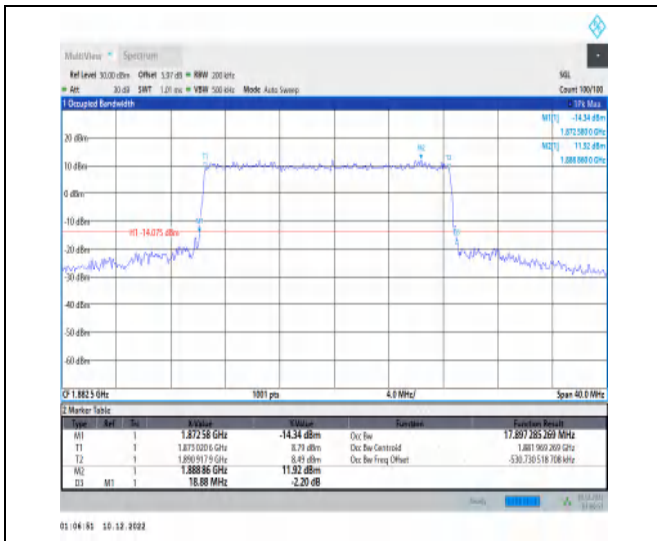
1-N25-15-20-M-3-DFT-16QAM-Outer_Full-100@0-A nt1-17.897-18.880-≤20-PASS
