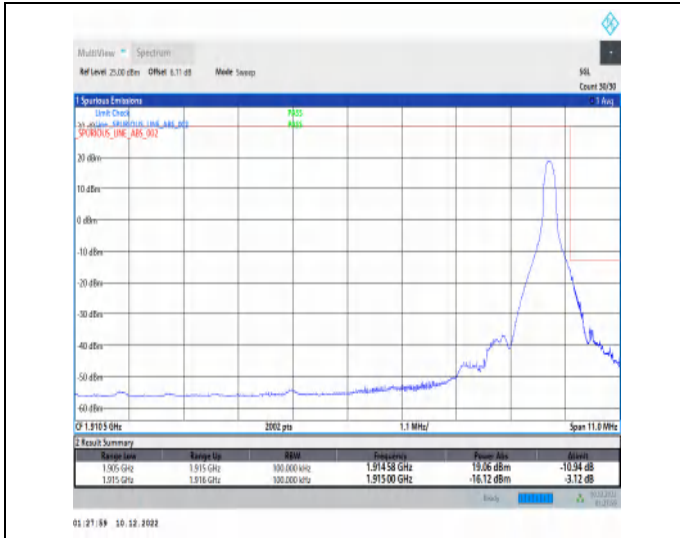
1-N25-15-10-H-2-DFT-PI2BPSK-Edge_1RB_Right-1@51-Ant1-1-seegraph-PASS-see graph
