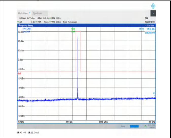
1-N25-15-20-M-1-DFT-PI2BPSK-Inner_1RB_Left-1 @ 1-1000-3000-Ant1-2980.00--39.32--13-PASS
