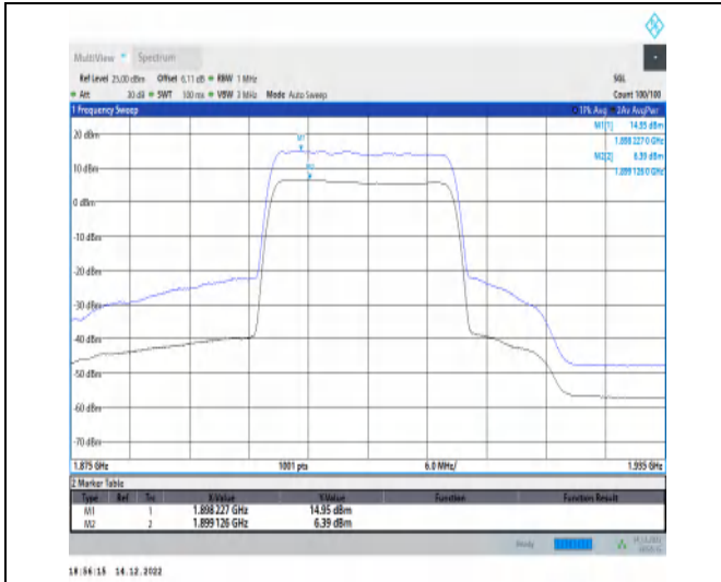
1-N25-15-20-H-1-DFT-256QAM-Outer_Full-100@0-A nt1-8.56-100%-0.00-8.56-PASS-≤13
