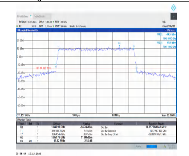
1-N25-15-15-L-8-CP-64QAM-Outer_Full-79@0-Ant1- 14.158-15.120≤15-PASS
