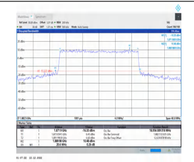
1-N25-15-20-M-6-CP-QPSK-Outer_Full-106@0-Ant1 -18.956-20.600-≤20-PASS
