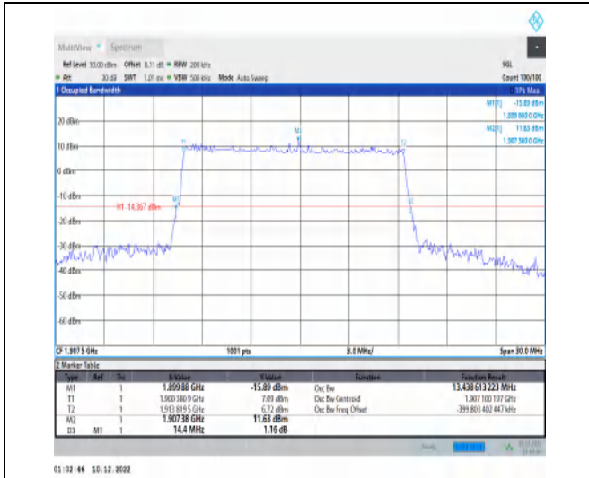
1-N25-15-15-H-5-DFT-256QAM-Outer_Full-75@0-Ant1-13.439-14.400-≤15-PASS
