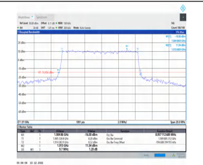
1-N25-15-10-H-3-DFT-16QAM-Outer_Full-50@0-Ant 1-8.957-9.700-≤10-PASS
