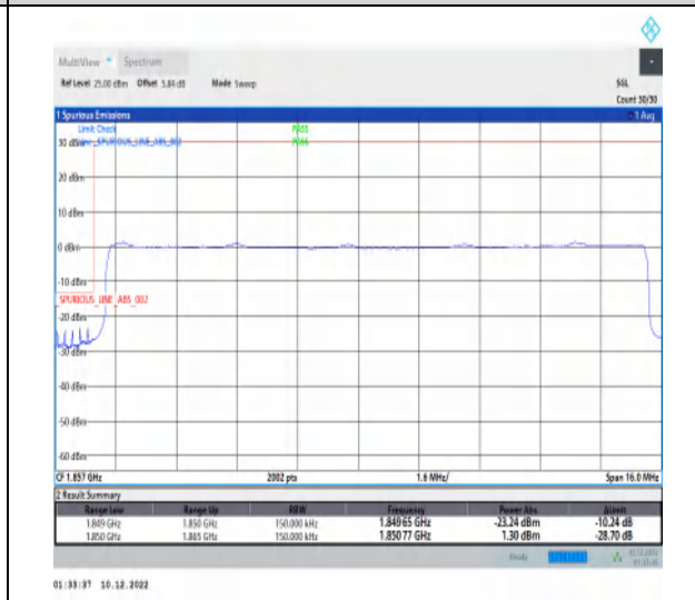
1-N25-15-15-L-6-CP-QPSK-Outer_Full-79@0-Ant1-1-seegraph-PASS-see graph
