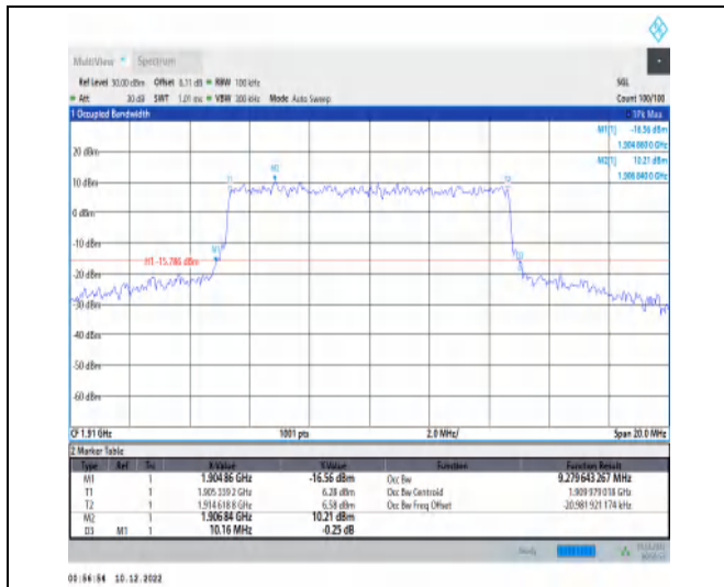
1-N25-15-10-H-8-CP-64QAM-Outer_Full-52@0-Ant1 -9.28-10.160-≤10-PASS
