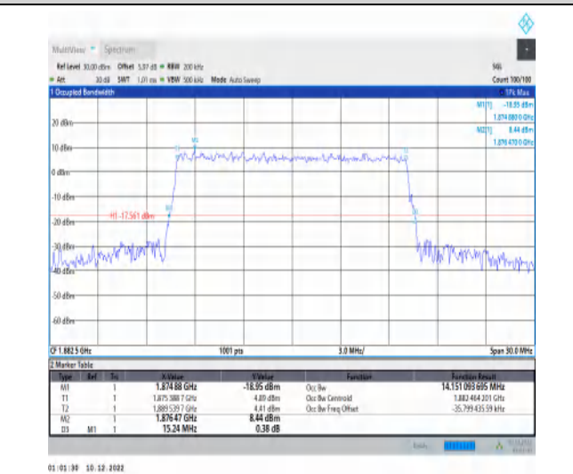
1-N25-15-15-M-9-CP-256QAM-Outer_Full-79@0-Ant1-14.151-15.240-≤15-PASS
