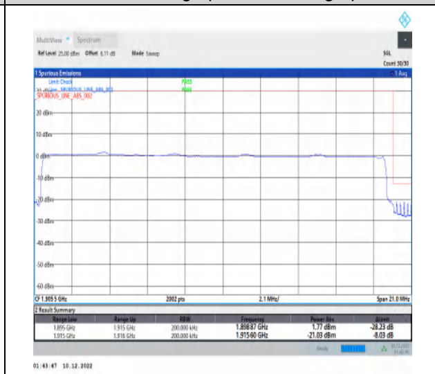
1-N25-15-20-H-6-CP-QPSK-Outer_Full-106@0-Ant1-1-seegraph-PASS-see graph
