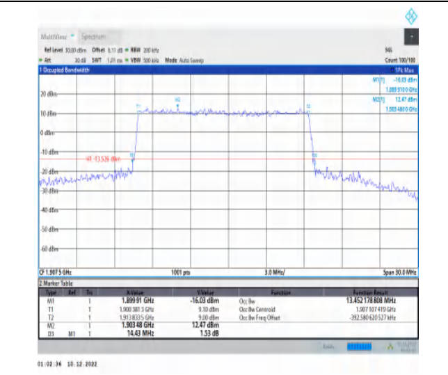
1-N25-15-15-H-4-DFT-64QAM-Outer_Full-75@0-Ant1 1-13.452-14.430≤15-PASS
