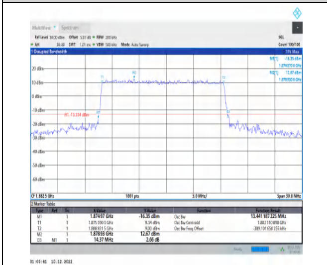
1-N25-15-15-M-4-DFT-64QAM-Outer_Full-75@0-Ant 1-13.441-14.370-≤15-PASS
