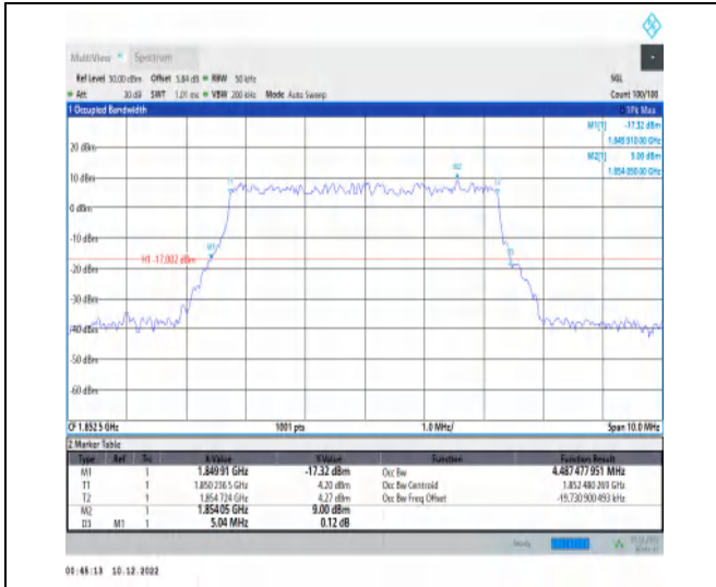
1-N25-15-5-L-5-DFT-256QAM-Outer_Full-25@0-Ant 1-4.487-5.040-≤5-PASS
