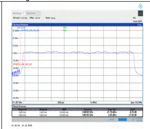
1-N25-15-15-L-3-DFT-PI2BPSK-Outer_Full-75@0-Ant1-1-seegraph-PASS-see graph
