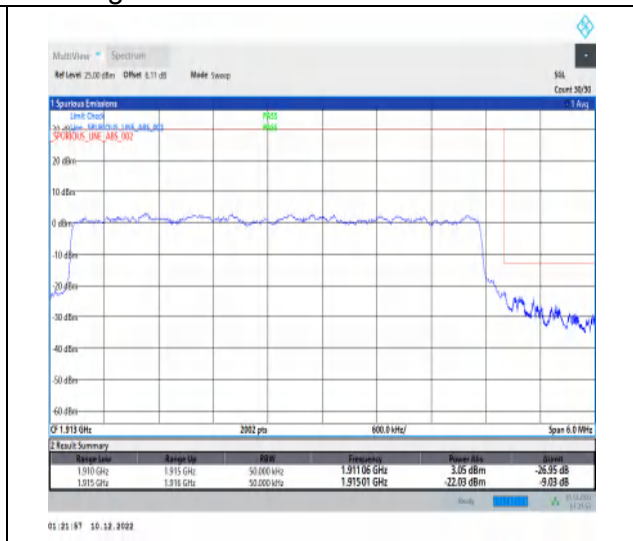
1-N25-15-5-H-3-DFT-PI2BPSK-Outer_Full-25@0-Ant1-1-seegraph-PASS-see graph
