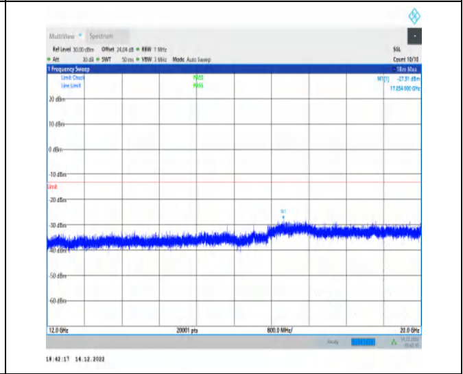
1-N25-15-20-M-1-DFT-PI2BPSK-Inner_1RB_Left-1 @ 1-12000-20000-Ant1-17054.00--27.91--13-PASS
