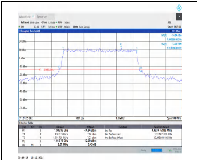
1-N25-15-5-H-3-DFT-16QAM-Outer_Full-25@0-Ant1 -4.483-5.010-≤5-PASS
