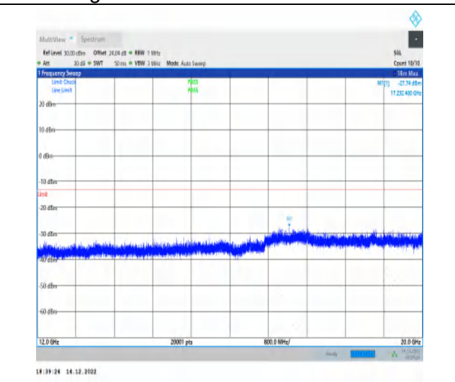
1-N25-15-20-L-1-DFT-PI2BPSK-Inner_1RB_Left-1 @1-12000-20000-Ant1-17232.40--27.74--13-PASS
