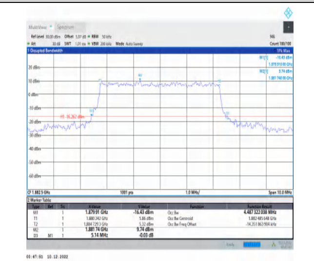
1-N25-15-5-M-7-CP-16QAM-Outer_Full-25@0-Ant1- 4.487-5.140-≤5-PASS
