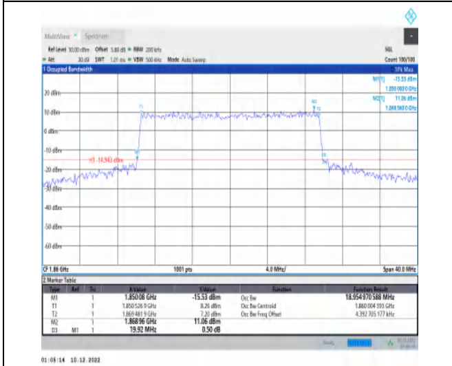
1-N25-15-20-L-6-CP-QPSK-Outer_Full-106@0-Ant1 -18.955-19.920-≤20-PASS
