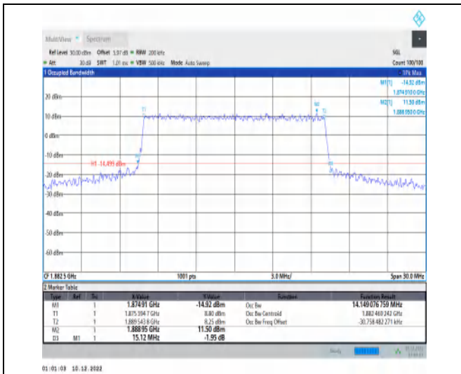
1-N25-15-15-M-6-CP-QPSK-Outer_Full-79@0-Ant1-14.149-15.120-≤15-PASS
