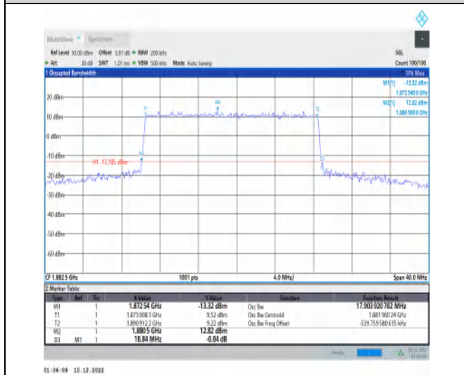
1-N25-15-20-M-1-DFT-QPSK-Outer_Full-100@0-Ant 1-17.904-18.840-≤20-PASS
