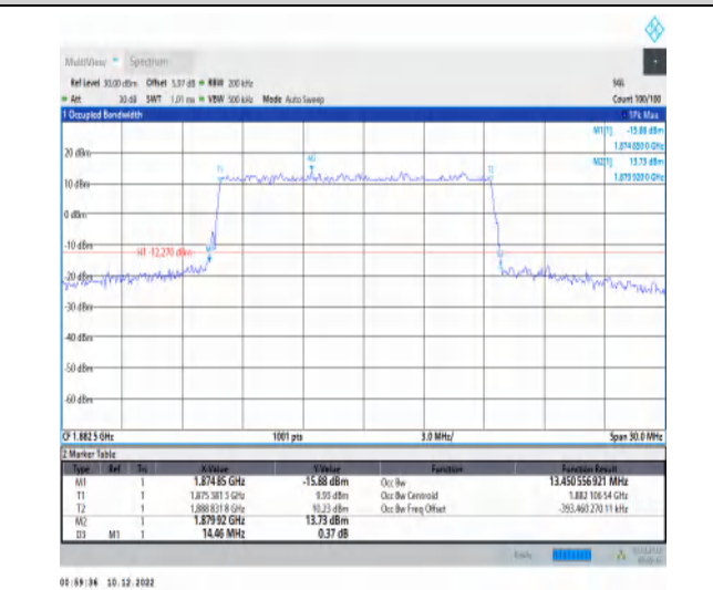
1-N25-15-15-M-1-DFT-QPSK-Outer_Full-75@0-Ant1 -13.451-14.460≤15-PASS
