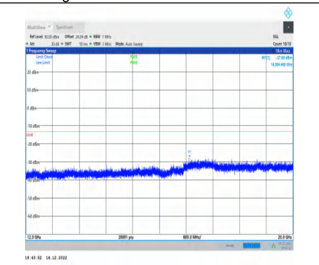
1-N25-15-20-H-1-DFT-PI2BPSK-Inner_1RB_Left-1@ 1-12000-20000-Ant1-16904.40--27.69--13-PASS
