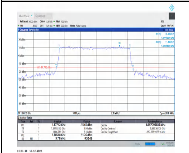
1-N25-15-10-M-3-DFT-16QAM-Outer_Full-50@0-Ant1 1-8.958-9.780-≤10-PASS
