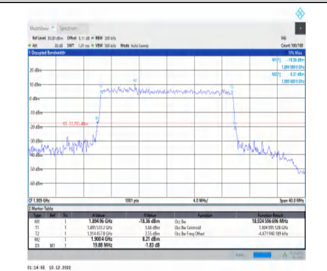
1-N25-15-20-H-9-CP-256QAM-Outer_Full-106@0-A nt1-18.925-19.880-≤20-PASS
