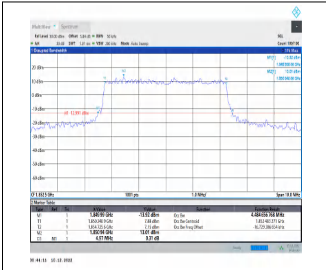
1-N25-15-5-L-1-DFT-QPSK-Outer_Full-25@0-Ant1-4 .485-4.970-≤5-PASS
