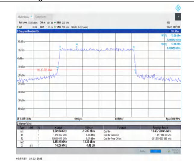
1-N25-15-15-L-4-DFT-64QAM-Outer_Full-75@0-Ant 1-13.453-14.250-≤15-PASS
