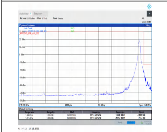
1-N25-15-15-H-5-CP-QPSK-Edge_1RB_Right-1@78-Ant1-1-seegraph-PASS-see graph
