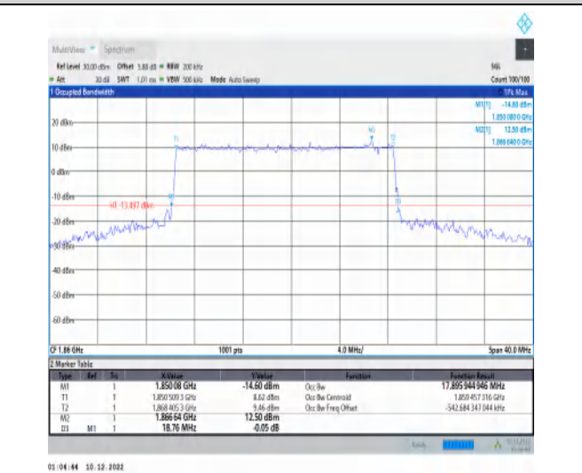
1-N25-15-20-L-3-DFT-16QAM-Outer_Full-100@0-Ant 1-17.896-18.760≤20-PASS
