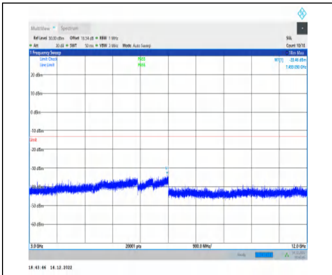
1-N25-15-20-H-1-DFT-PI2BPSK-Inner_1RB_Left-1 @1-3000-12000-Ant1-7459.05--33.46--13-PASS
