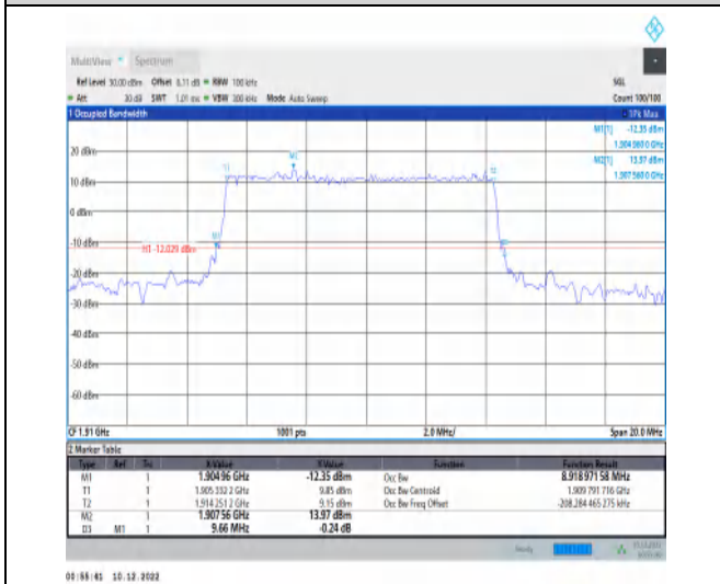
1-N25-15-10-H-2-DFT-PI2BPSK-Outer_Full-50@0-A nt1-8.919-9.660-≤10-PASS
