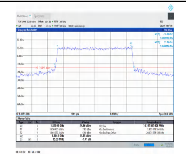
1-N25-15-15-L-6-CP-QPSK-Outer_Full-79@0-Ant1-1 4.148-15.090-≤15-PASS
