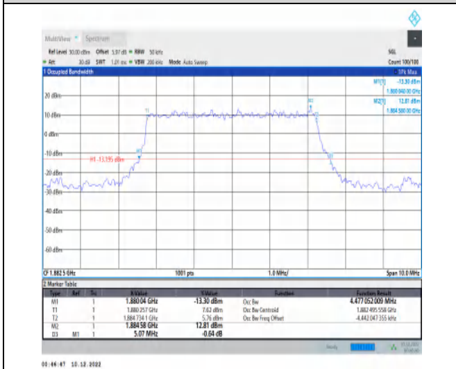
1-N25-15-5-M-2-DFT-P12BPSK-Outer_Full-25@0-An t1-4.477-5.070-≤5-PASS
