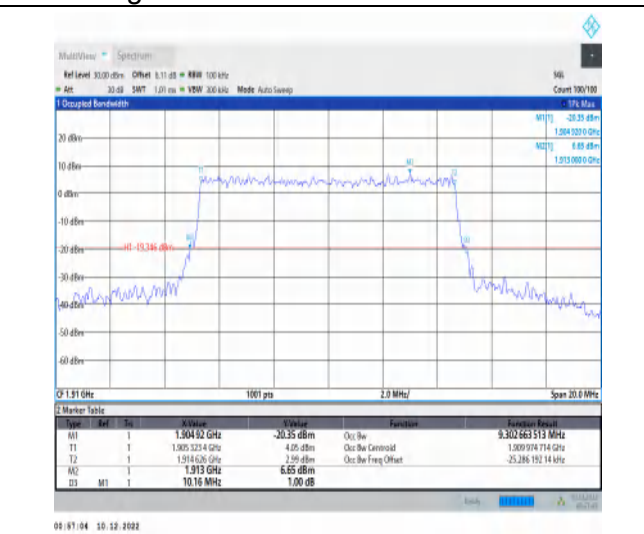
1-N25-15-10-H-9-CP-256QAM-Outer_Full-52@0-Ant 1-9.303-10.160-≤10-PASS
