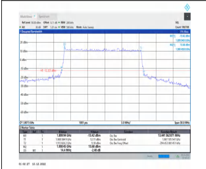
1-N25-15-15-H-3-DFT-16QAM-Outer_Full-75@0-Ant1 1-13.441-14.400≤15-PASS
