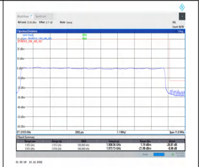
1-N25-15-10-H-6-CP-QPSK-Outer_Full-52@0-Ant1-1-seegraph-PASS-see graph
