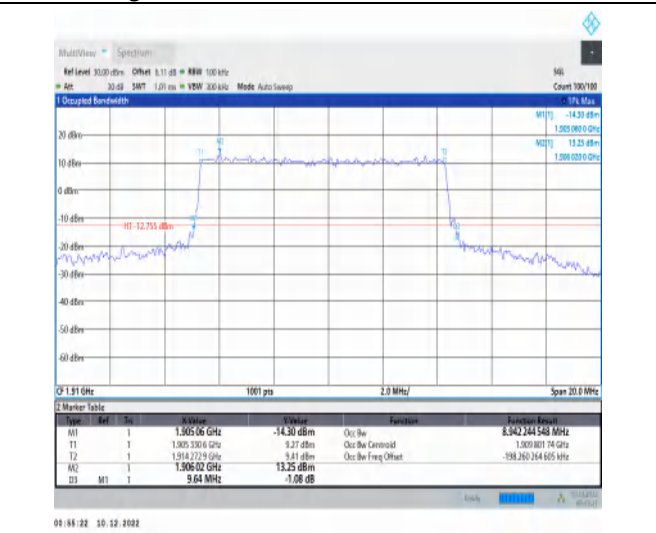
1-N25-15-10-H-1-DFT-QPSK-Outer_Full-50@0-Ant1 -8.942-9.640-≤10-PASS
