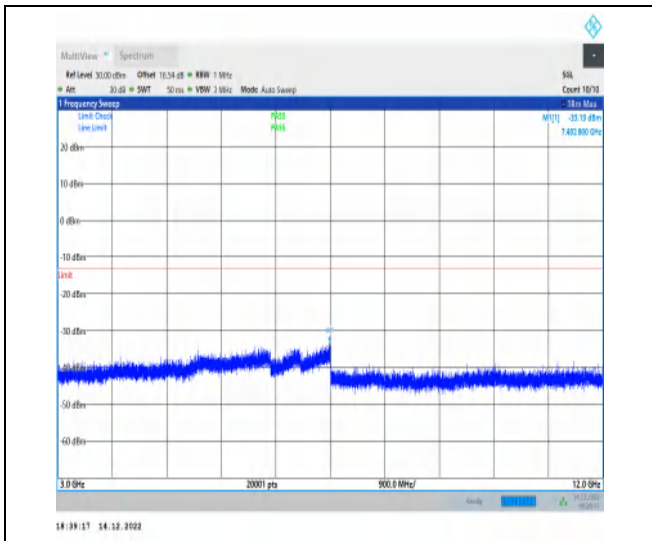
1-N25-15-20-L-1-DFT-PI2BPSK-Inner_1RB_Left-1 @1-3000-12000-Ant1-7492.80--33.19--13-PASS
