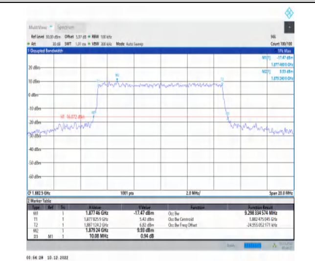
1-N25-15-10-M-8-CP-64QAM-Outer_Full-52@0-Ant1 -9.298-10.080≤10-PASS
