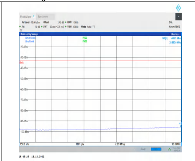
1-N25-15-20-H-1-DFT-PI2BPSK-Inner_1RB_Left-1 @ 1-0.15-30-Ant1-29.88--95.87--33-PASS
