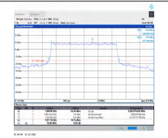
1-N25-15-10-H-7-CP-16QAM-Outer_Full-52@0-Ant1 -9.303-10.060≤10-PASS
