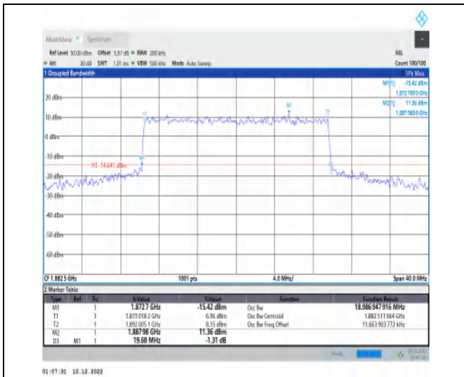
1-N25-15-20-M-7-CP-16QAM-Outer_Full-106@0-An t1-18.987-19.680-≤20-PASS
