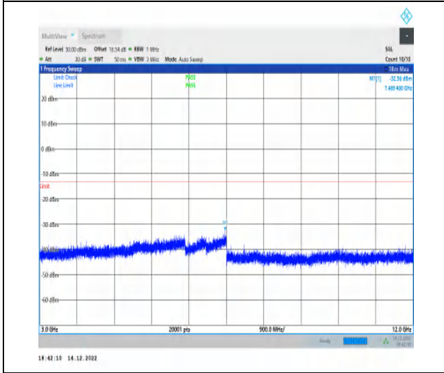
1-N25-15-20-M-1-DFT-PI2BPSK-Inner_1RB_Left-1 @ 1-3000-12000-Ant1-7469.40--32.56--13-PASS
