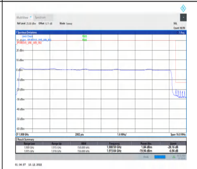
1-N25-15-15-H-6-CP-QPSK-Outer_Full-79@0-Ant1-1-seegraph-PASS-see graph
