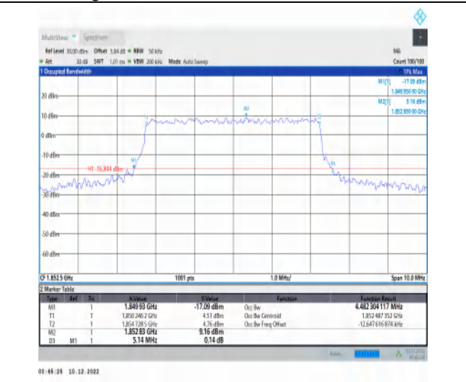
1-N25-15-5-L-6-CP-QPSK-Outer_Full-25@0-Ant1-4. 482-5.140-≤5-PASS
