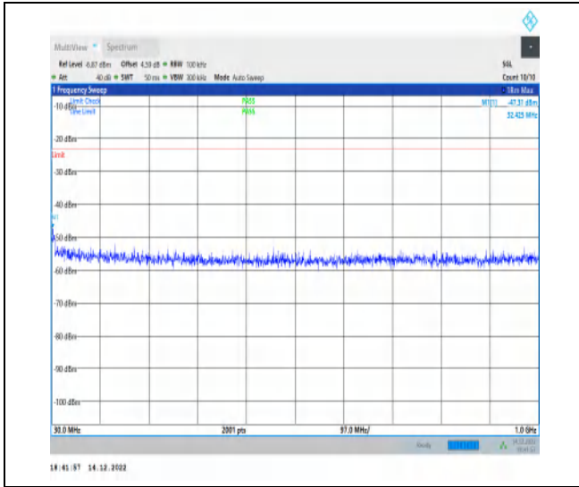
1-N25-15-20-M-1-DFT-PI2BPSK-Inner_1RB_Left-1 @ 1-30-1000-Ant1-32.43--47.31--23-PASS
