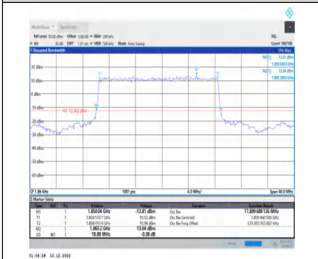
1-N25-15-20-L-2-DFT-PI2BPSK-Outer_Full-100@0-Ant1 1-17.9-18.880≤20-PASS
