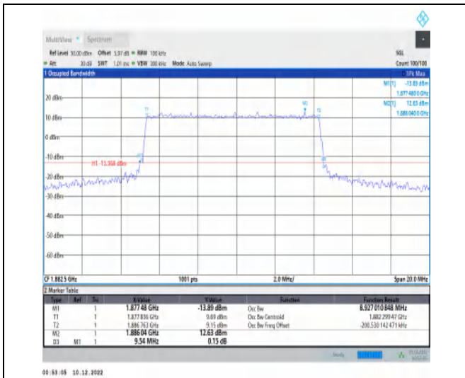
1-N25-15-10-M-1-DFT-QPSK-Outer_Full-50@0-Ant1 -8.927-9.540-≤10-PASS
