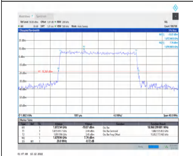
1-N25-15-20-M-9-CP-256QAM-Outer_Full-106@0-A nt1-18.96-20.000-≤20-PASS
