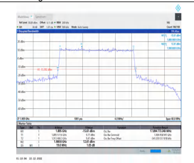
1-N25-15-20-H-3-DFT-16QAM-Outer_Full-100@0-Ant1-17.895-19.000-≤20-PASS
