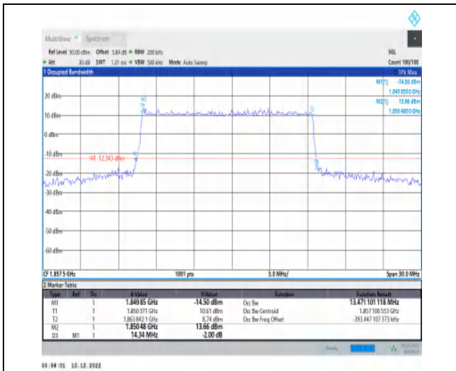
1-N25-15-15-L-3-DFT-16QAM-Outer_Full-75@0-Ant 1-13.471-14.340-≤15-PASS
