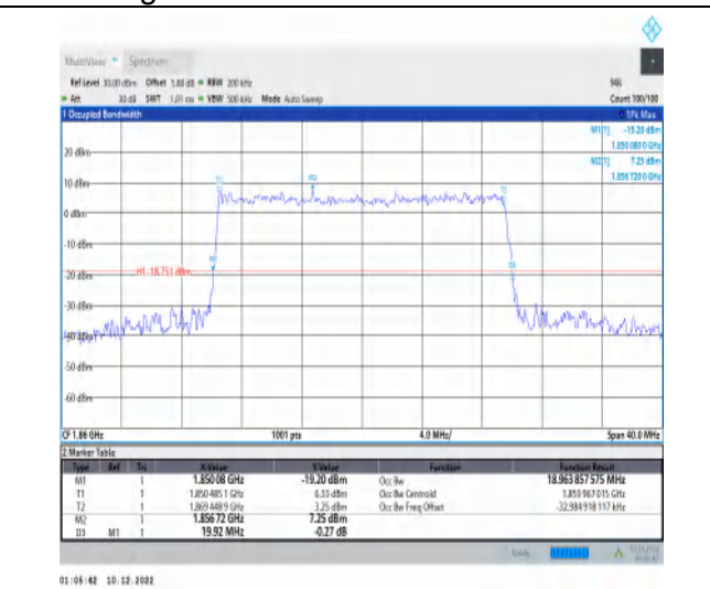
1-N25-15-20-L-9-CP-256QAM-Outer_Full-106@0-Ant t1-18.964-19.920-≤20-PASS
