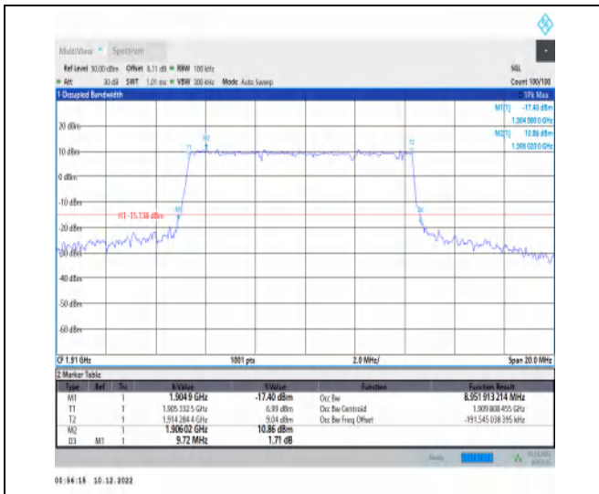
1-N25-15-10-H-4-DFT-64QAM-Outer_Full-50@0-Ant 1-8.952-9.720≤10-PASS
