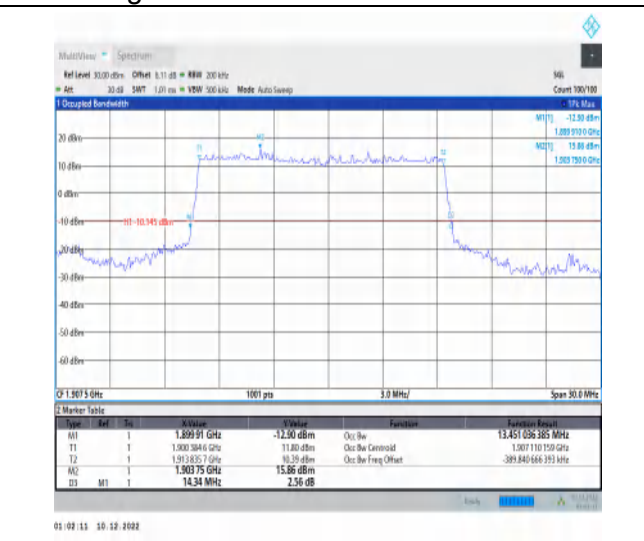
1-N25-15-15-H-2-DFT-PI2BPSK-Outer_Full-75@0-Ant1 -13.451-14.340≤15-PASS
