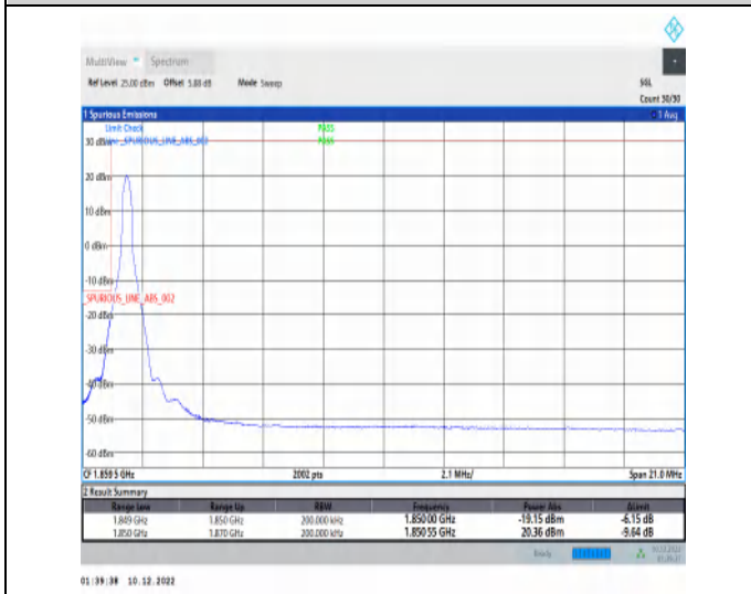
1-N25-15-20-L-4-CP-QPSK-Edge_1RB_Left-1@0-Ant1-1-seegraph-PASS-see graph
