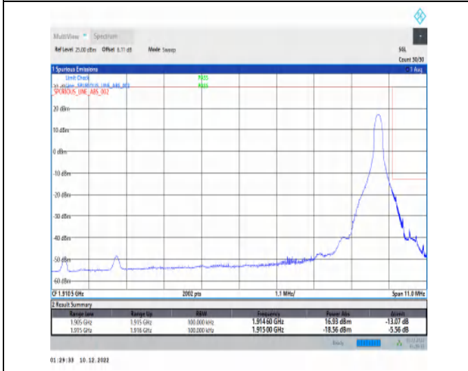
1-N25-15-10-H-5-CP-QPSK-Edge_1RB_Right-1@51-Ant1-1-seegraph-PASS-see graph
