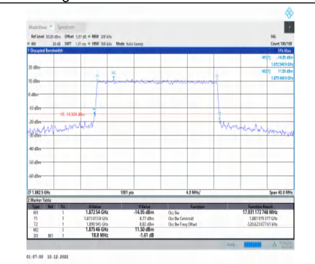
1-N25-15-20-M-4-DFT-64QAM-Outer_Full-100@0-A nt1-17.931-18.800-≤20-PASS
