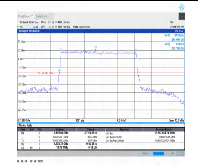
1-N25-15-20-H-5-DFT-256QAM-Outer_Full-100@0-Ant1-17.862-18.760-≤20-PASS
