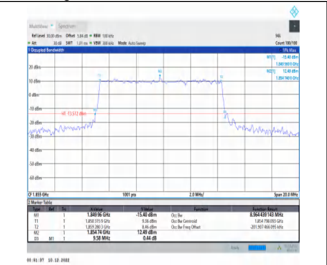
1-N25-15-10-L-3-DFT-16QAM-Outer_Full-50@0-Ant 1-8.964-9.580-≤10-PASS
