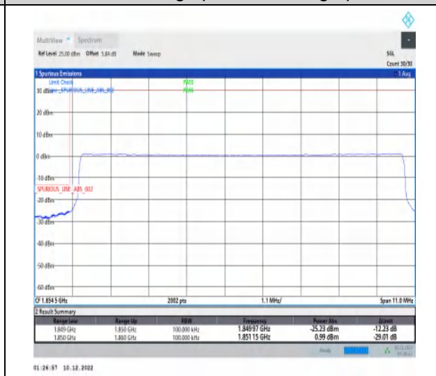
1-N25-15-10-L-6-CP-QPSK-Outer_Full-52@0-Ant1-1-seegraph-PASS-see graph
