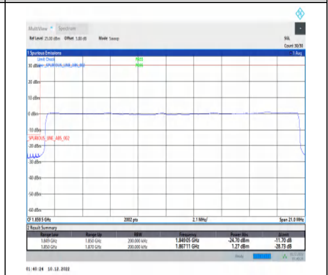
1-N25-15-20-L-6-CP-QPSK-Outer_Full-106@0-Ant1-1-seegraph-PASS-see graph
