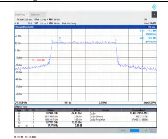
1-N25-15-15-M-3-DFT-16QAM-Outer_Full-75@0-Ant 1-13.436-14.370-≤15-PASS
