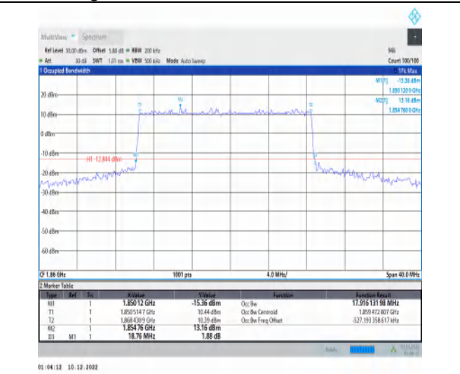
1-N25-15-20-L-1-DFT-QPSK-Outer_Full-100@0-Ant 1-17.916-18.760≤20-PASS
