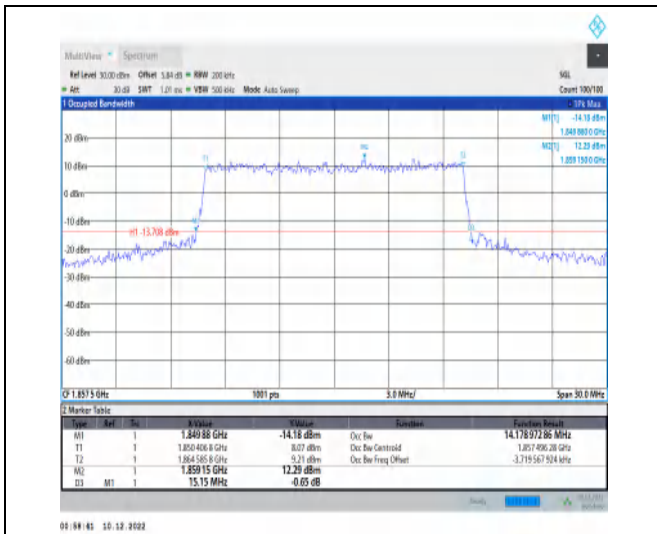
1-N25-15-15-L-7-CP-16QAM-Outer_Full-79@0-Ant1 -14.179-15.150≤15-PASS
