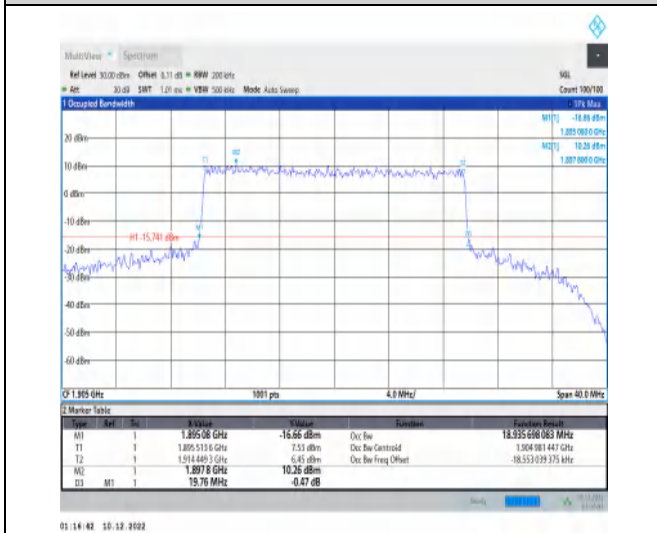
1-N25-15-20-H-8-CP-64QAM-Outer_Full-106@0-Ant 1-18.936-19.760-≤20-PASS
