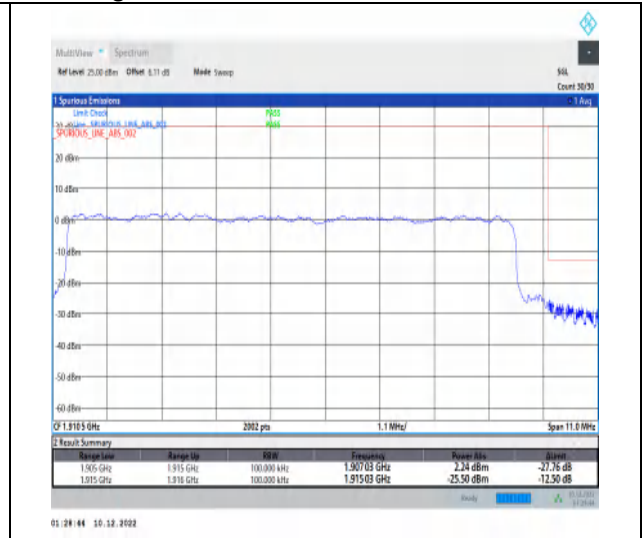
1-N25-15-10-H-3-DFT-PI2BPSK-Outer_Full-50@0-Ant1-1-seegraph-PASS-see graph
