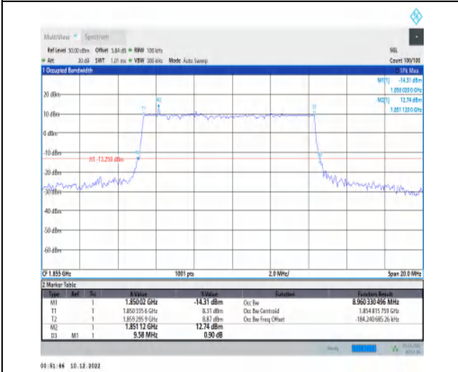
1-N25-15-10-L-4-DFT-64QAM-Outer_Full-50@0-Ant 1-8.96-9.580-≤10-PASS
