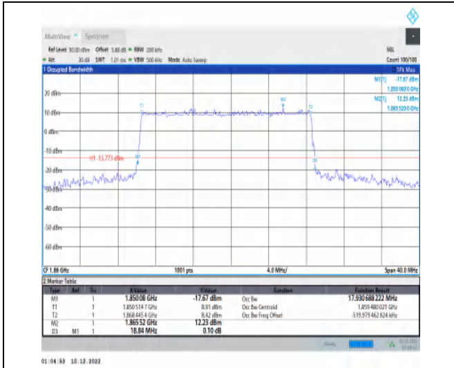
1-N25-15-20-L-4-DFT-64QAM-Outer_Full-100@0-An t1-17.931-18.840-≤20-PASS
