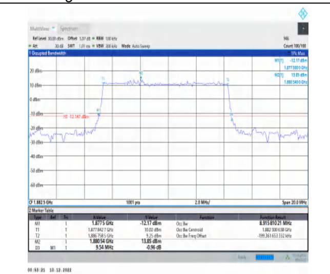
1-N25-15-10-M-2-DFT-PI2BPSK-Outer_Full-50@0-Ant1 8.916-9.540-≤10-PASS
