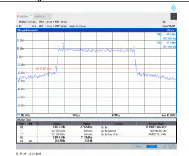
1-N25-15-20-M-8-CP-64QAM-Outer_Full-106@0-Ant 1-18.951-20.000-≤20-PASS
