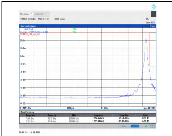
1-N25-15-20-H-2-DFT-PI2BPSK-Edge_1RB_Right-1@105-Ant1-1-seegraph-PASS-see graph
