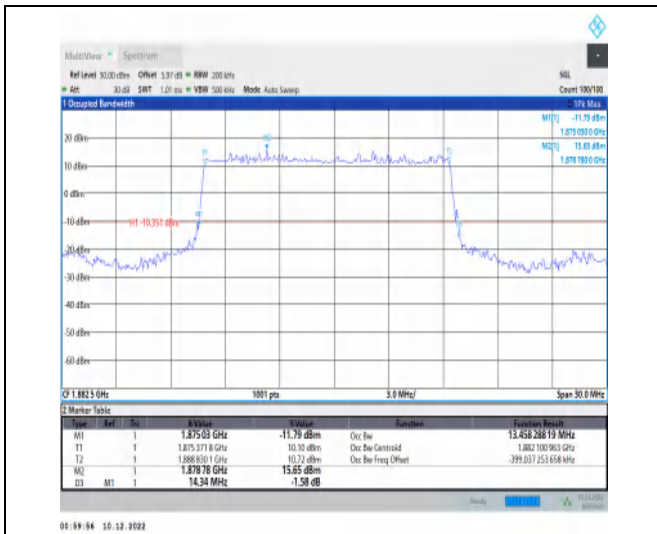
1-N25-15-15-M-2-DFT-PI2BPSK-Outer_Full-75@0-A nt1-13.458-14.340-≤15-PASS
