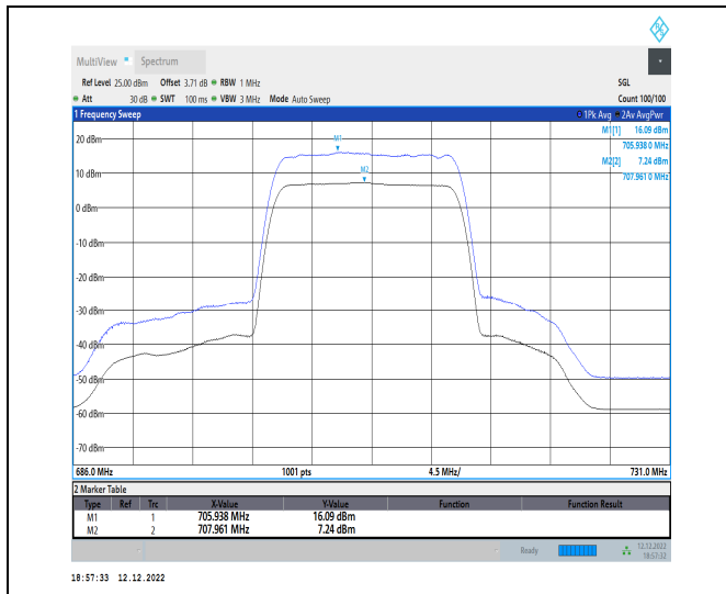
1-N12-15-15-H-1-DFT-256QAM-Outer_Full-75@0-An t1-8.85-100%-0.00-8.85-PASS-≤13
