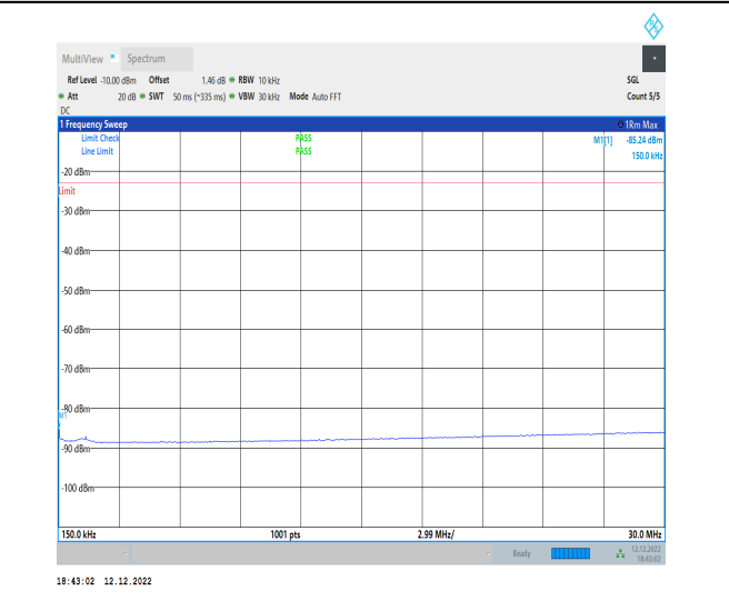
1-N12-15-15-M-1-DFT-PI2BPSK-Inner_1RB_Left-1 @ 1-0.15-30-Ant1-0.15--85.24--23-PASS
