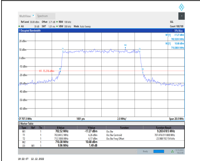
1-N12-15-10-M-7-CP-16QAM-Outer_Full-52@0-Ant 1-9.266-9.960-≤10-PASS
