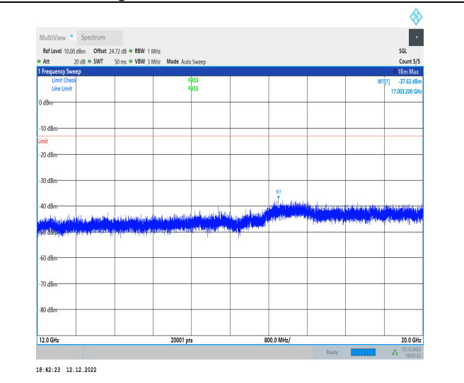
1-N12-15-15-L-1-DFT-PI2BPSK-Inner_1RB_Left-1 @ 1-12000-20000-Ant1-17003.20--37.63--13-PASS
