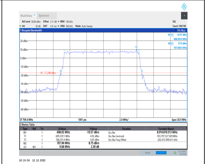
1-N12-15-10-L-5-DFT-256QAM-Outer_Full-50@0-Ant t1-8.917-9.680-≤10-PASS
