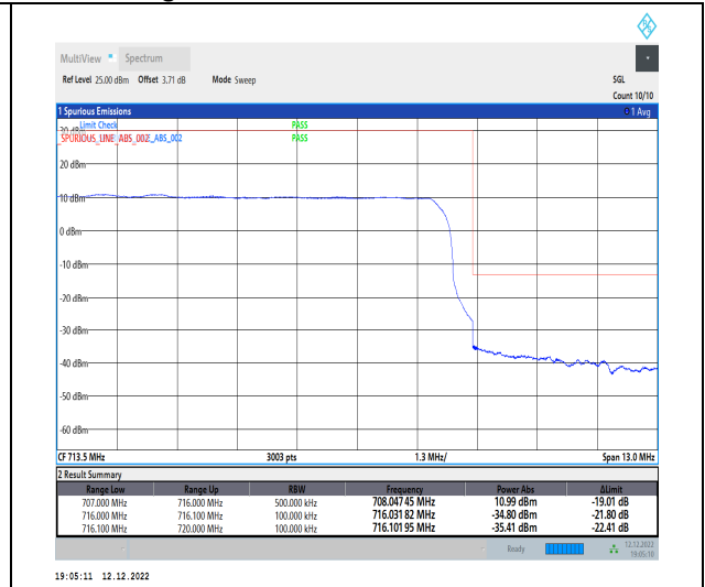
1-N12-15-10-H-3-DFT-PI2BPSK-Outer_Full-50@0-Ant1-1--PASS-see graph
