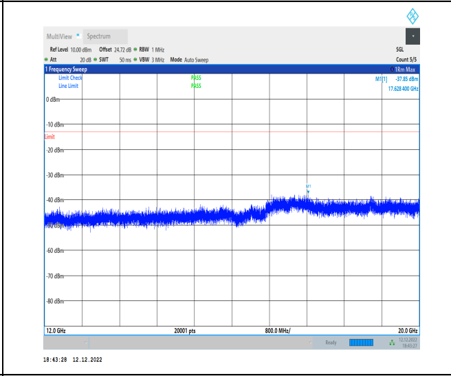
1-N12-15-15-M-1-DFT-PI2BPSK-Inner_1RB_Left-1 @ 1-12000-20000-Ant1-17628.40--37.85--13-PASS
