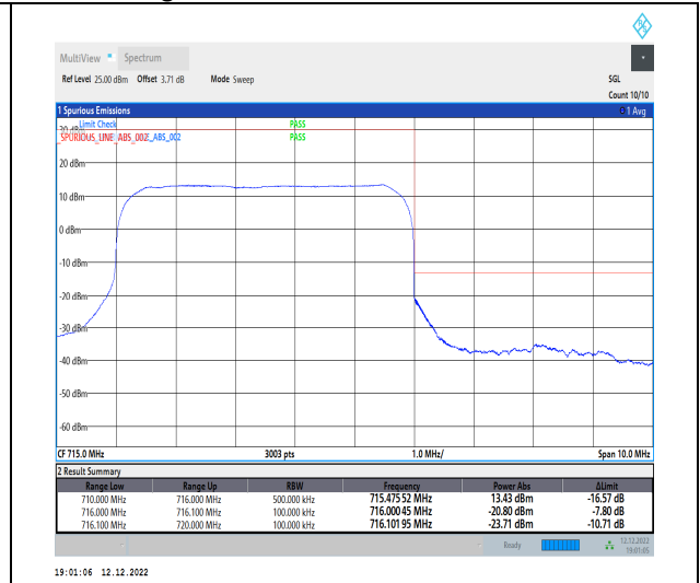
1-N12-15-5-H-3-DFT-PI2BPSK-Outer_Full-25@0-Ant1-1--PASS-see graph
