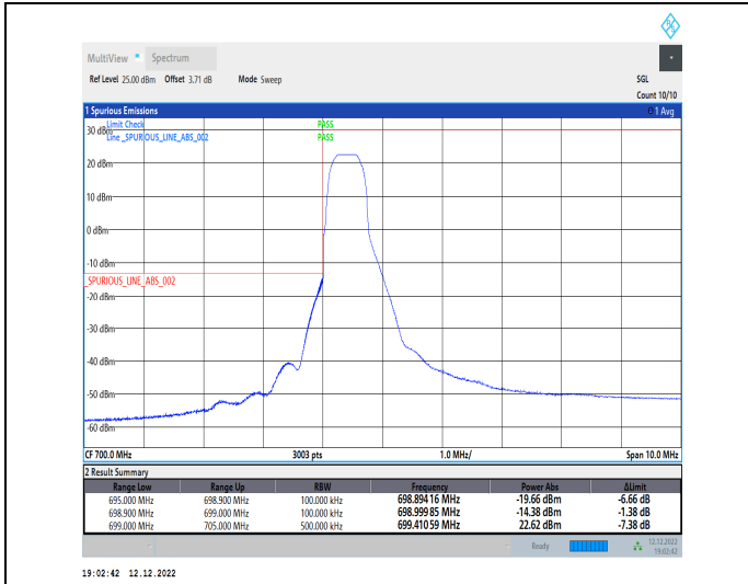
1-N12-15-10-L-1-DFT-PI2BPSK-Edge_1RB_Left-1@0-Ant1-1--PASS-see graph
