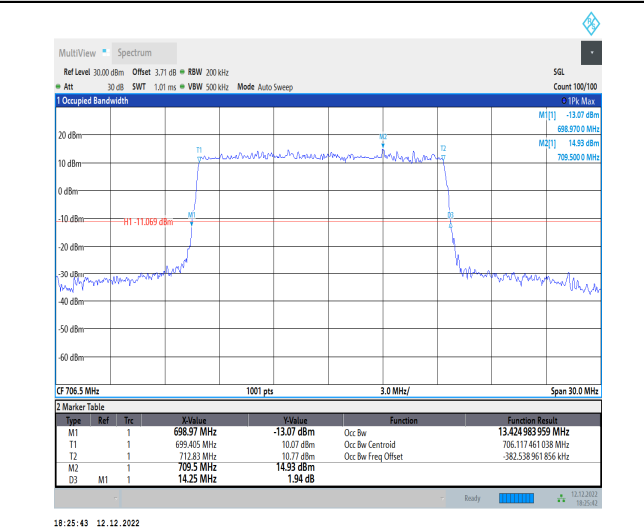
1-N12-15-15-L-2-DFT-PI2BPSK-Outer_Full-75@0-A nt1-13.425-14.250-≤15-PASS
