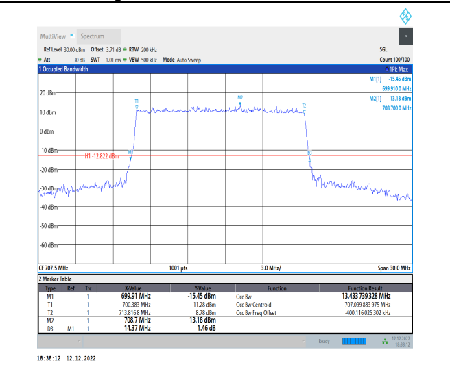
1-N12-15-15-M-3-DFT-16QAM-Outer_Full-75@0-Ant 1-13.434-14.370-≤15-PASS
