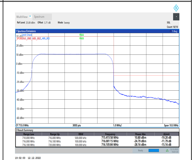
1-N12-15-5-H-6-CP-QPSK-Outer_Full-25@0-Ant1-1--PASS-see graph
