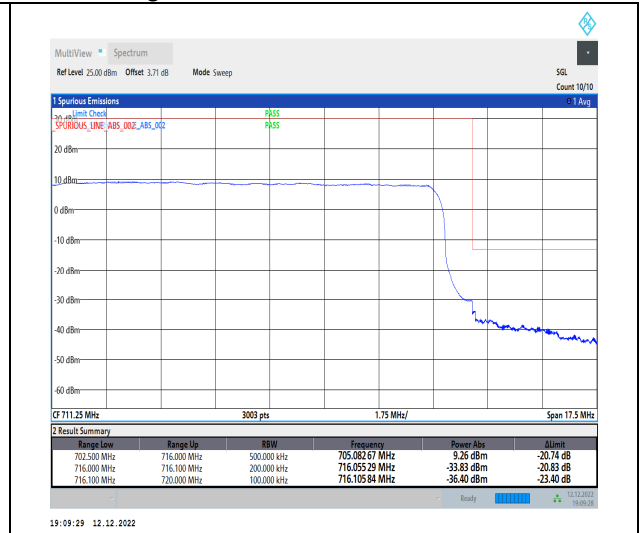
1-N12-15-15-H-3-DFT-PI2BPSK-Outer_Full-75@0-Ant1-1--PASS-see graph
