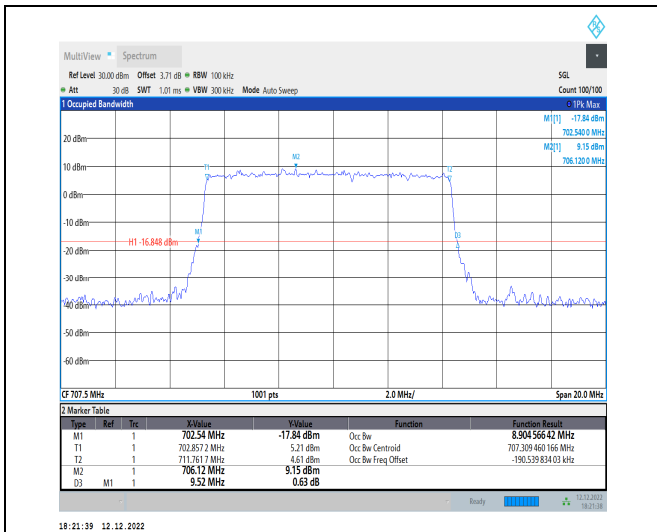
1-N12-15-10-M-5-DFT-256QAM-Outer_Full-50@0-A nt1-8.905-9.520-≤10-PASS
