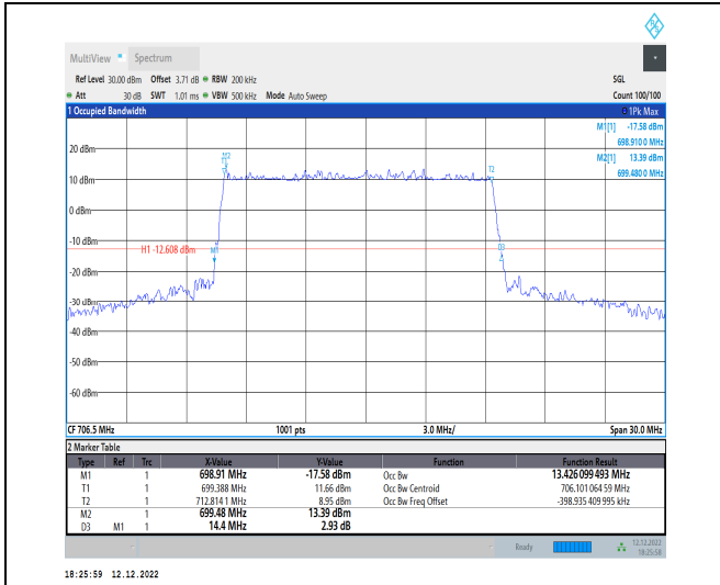
1-N12-15-15-L-3-DFT-16QAM-Outer_Full-75@0-Ant t1-13.426-14.400-≤15-PASS
