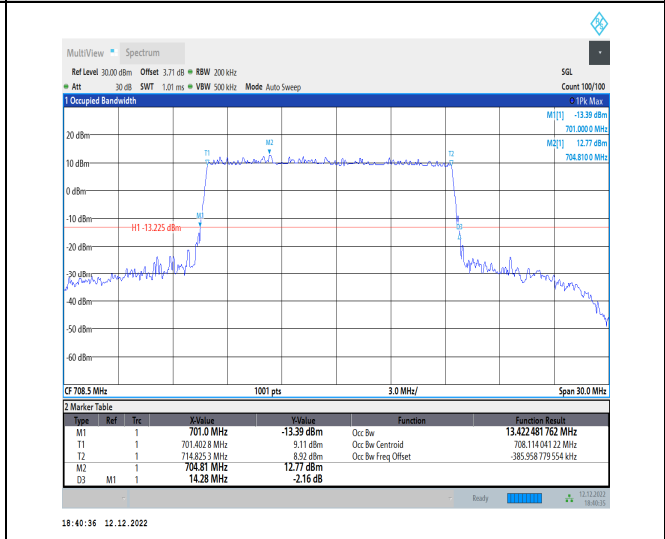
1-N12-15-15-H-4-DFT-64QAM-Outer_Full-75@0-Ant1 1-13.422-14.280≤15-PASS
