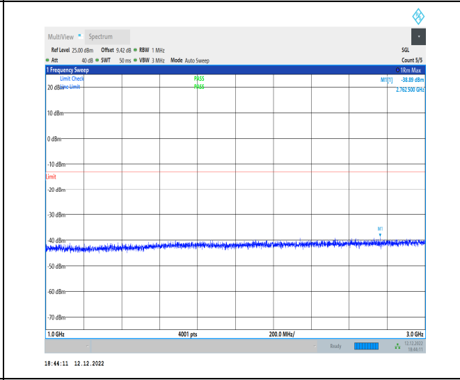
1-N12-15-15-H-1-DFT-PI2BPSK-Inner_1RB_Left-1 @ 1-1000-3000-Ant1-2762.50--38.89--13-PASS
