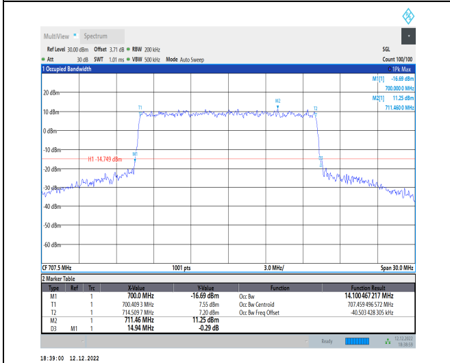
1-N12-15-15-M-8-CP-64QAM-Outer_Full-79@0-Ant1-14.1-14.940-≤15-PASS
