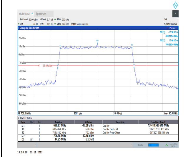
1-N12-15-15-L-5-DFT-256QAM-Outer_Full-75@0-An t1-13.412-14.250-≤15-PASS
