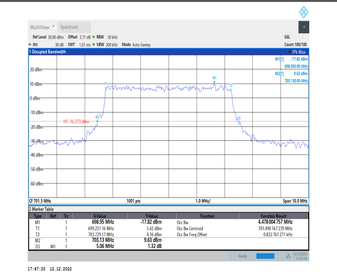
1-N12-15-5-L-8-CP-64QAM-Outer_Full-25@0-Ant1-4 .478-5.060-≤5-PASS
