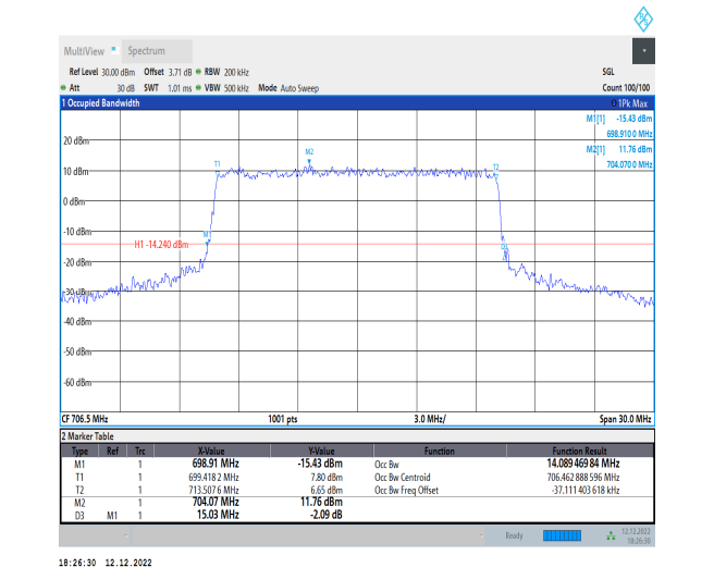
1-N12-15-15-L-6-CP-QPSK-Outer_Full-79@0-Ant1-1 t1-14.089-15.030-≤15-PASS
