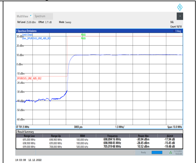
1-N12-15-10-L-3-DFT-PI2BPSK-Outer_Full-50@0-Ant1-1--PASS-see graph
