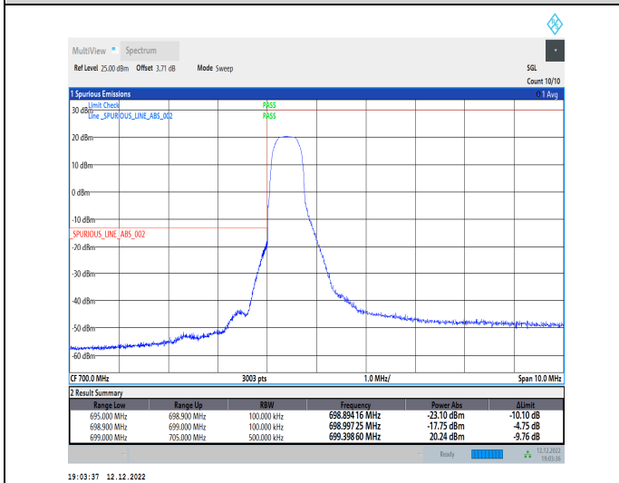
1-N12-15-10-L-4-CP-QPSK-Edge_1RB_Left-1@0-Ant1-1--PASS-see graph
