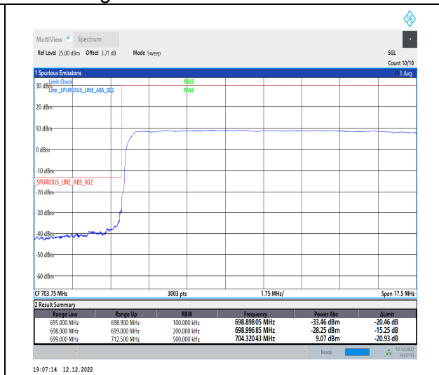
1-N12-15-15-L-3-DFT-PI2BPSK-Outer_Full-75@0-Ant1-1--PASS-see graph
