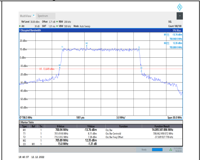
1-N12-15-15-H-6-CP-QPSK-Outer_Full-79@0-Ant1- 14.095-15.000-≤15-PASS
