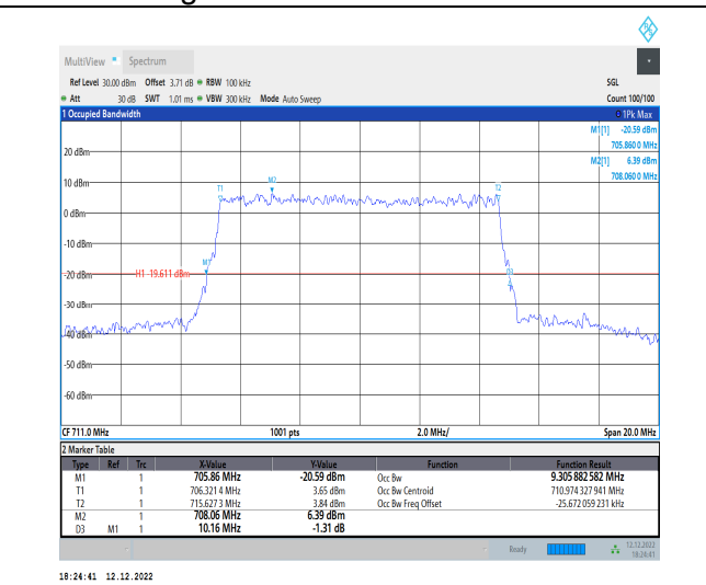
1-N12-15-10-H-9-CP-256QAM-Outer_Full-52@0-Ant 1-9.306-10.160-≤10-PASS
