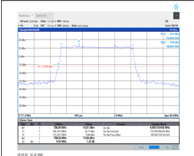
1-N12-15-10-H-2-DFT-PI2BPSK-Outer_Full-50@0-A nt1-8.906-9.540-≤10-PASS
