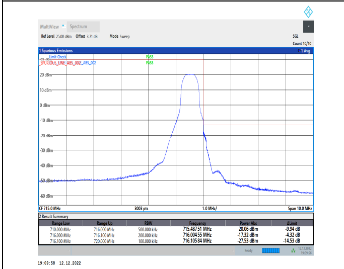
1-N12-15-15-H-5-CP-QPSK-Edge_1RB_Right-1@78-Ant1-1--PASS-see graph
