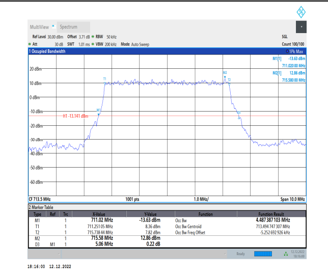
1-N12-15-5-H-2-DFT-PI2BPSK-Outer_Full-25@0-Ant1-4.487-5.060-≤5-PASS
