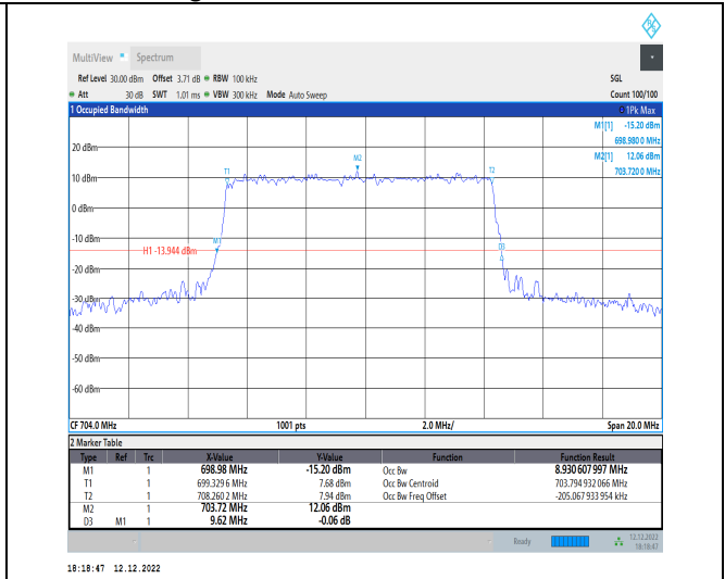
1-N12-15-10-L-3-DFT-16QAM-Outer_Full-50@0-Ant 1-8.931-9.620-≤10-PASS
