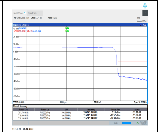
1-N12-15-15-H-6-CP-QPSK-Outer_Full-79@0-Ant1-1--PASS-see graph
