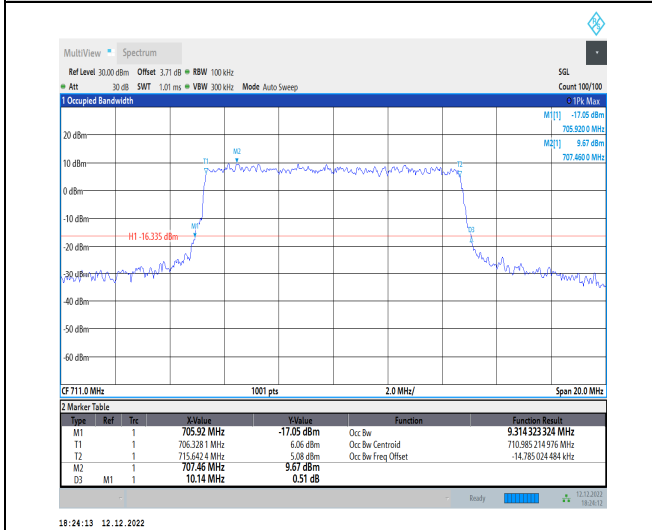
1-N12-15-10-H-6-CP-QPSK-Outer_Full-52@0-Ant1 9.314-10.140-≤10-PASS
