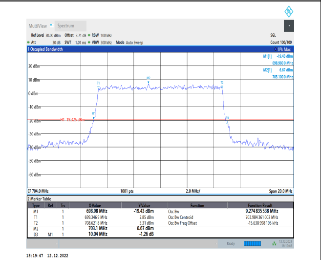
1-N12-15-10-L-9-CP-256QAM-Outer_Full-52@0-Ant1-9.275-10.040-≤10-PASS
