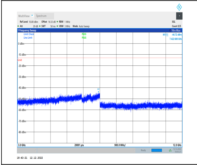
1-N12-15-15-M-1-DFT-PI2BPSK-Inner_1RB_Left-1 @ 1-3000-12000-Ant1-7422.60--44.72--13-PASS
