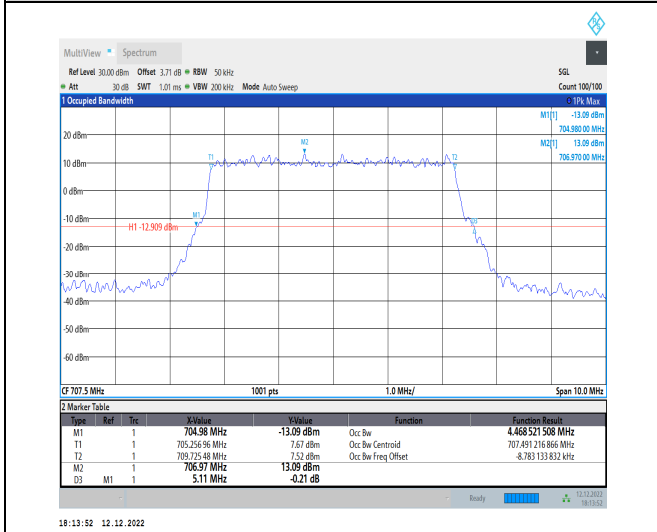
1-N12-15-5-M-2-DFT-P12BPSK-Outer_Full-25@0-An t1-4.469-5.110-≤5-PASS
