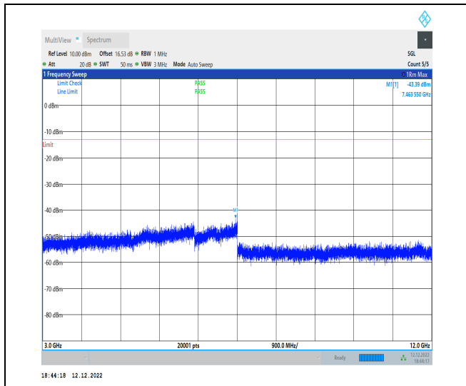
1-N12-15-15-H-1-DFT-PI2BPSK-Inner_1RB_Left-1 @1-3000-12000-Ant1-7463.55--43.39--13-PASS
