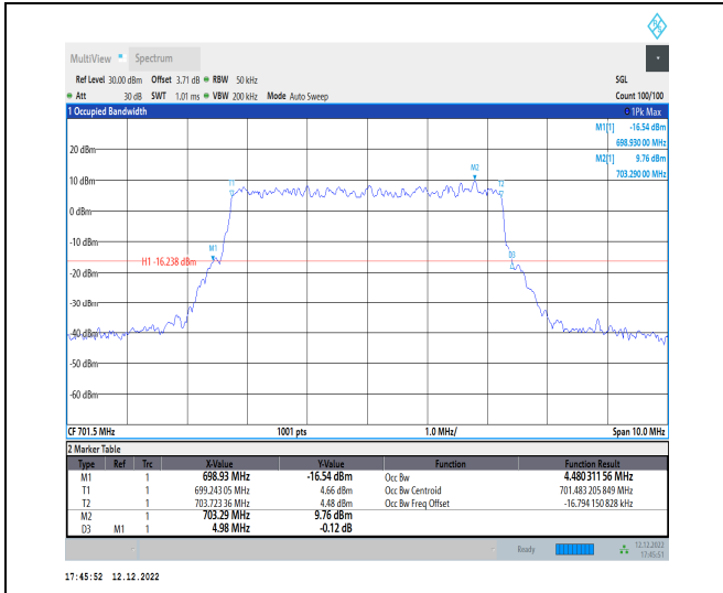
1-N12-15-5-L-5-DFT-256QAM-Outer_Full-25@0-Ant 1-4.48-4.980-≤5-PASS
