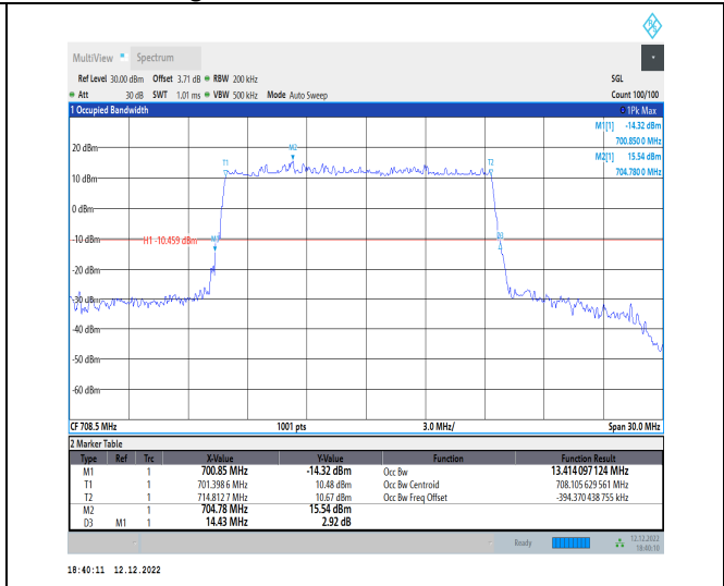
1-N12-15-15-H-2-DFT-PI2BPSK-Outer_Full-75@0-Ant1 -13.414-14.430≤15-PASS
