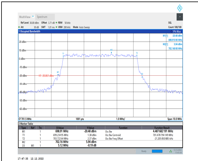
1-N12-15-5-L-9-CP-256QAM-Outer_Full-25@0-Ant1 -4.488-5.120-≤5-PASS
