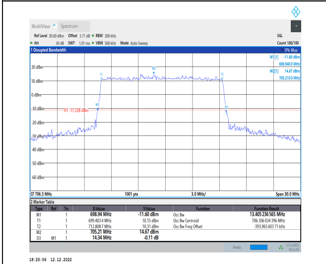
1-N12-15-15-L-1-DFT-QPSK-Outer_Full-75@0-Ant1- 13.405-14.340-≤15-PASS
