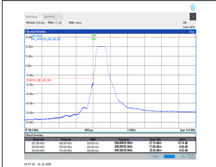
1-N12-15-15-L-4-CP-QPSK-Edge_1RB_Left-1@0-Ant1-1--PASS-see graph
