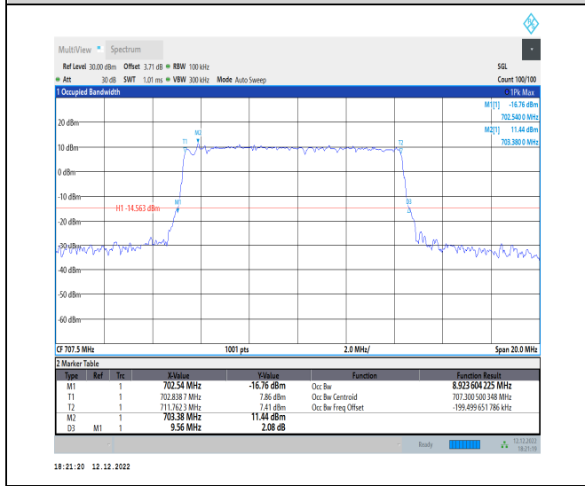
1-N12-15-10-M-3-DFT-16QAM-Outer_Full-50@0-Ant1 1-8.924-9.560-≤10-PASS
