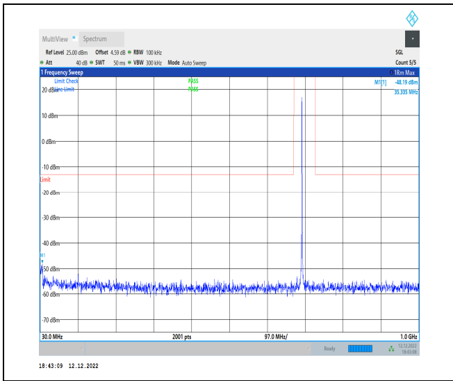
1-N12-15-15-M-1-DFT-PI2BPSK-Inner_1RB_Left-1 @ 1-30-1000-Ant1-35.34--48.19--13-PASS
