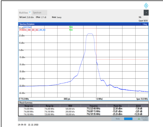
1-N12-15-15-H-2-DFT-PI2BPSK-Edge_1RB_Right-1@78-Ant1-1--PASS-see graph
