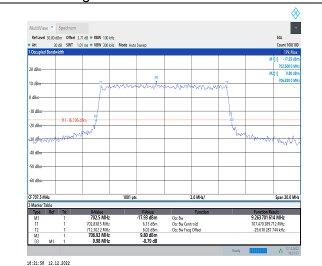
1-N12-15-10-M-6-CP-QPSK-Outer_Full-52@0-Ant1- 9.264-9.980-≤10-PASS
