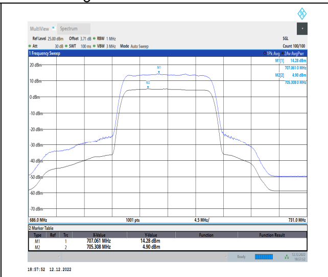
1-N12-15-15-H-2-CP-256QAM-Outer_Full-79@0-An t1-9.38-100%-0.00-9.38-PASS-≤13
