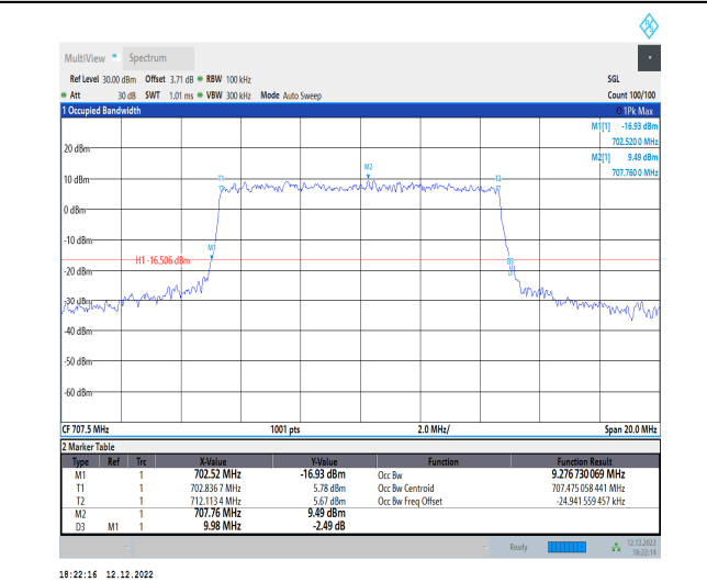
1-N12-15-10-M-8-CP-64QAM-Outer_Full-52@0-Ant1 -9.277-9.980-≤10-PASS
