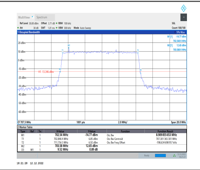
1-N12-15-10-M-4-DFT-64QAM-Outer_Full-50@0-Ant1 1-8.91-9.520-≤10-PASS
