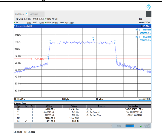
1-N12-15-15-L-8-CP-64QAM-Outer_Full-79@0-Ant1- 14.122-14.910-≤15-PASS
