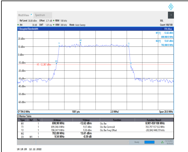
1-N12-15-10-L-2-DFT-PI2BPSK-Outer_Full-50@0-A nt1-8.901-9.540-≤10-PASS
