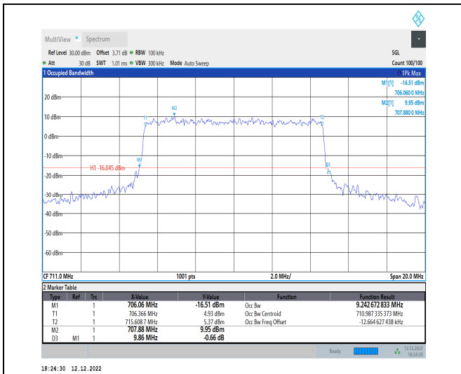
1-N12-15-10-H-8-CP-64QAM-Outer_Full-52@0-Ant1 -9.243-9.860-≤10-PASS
