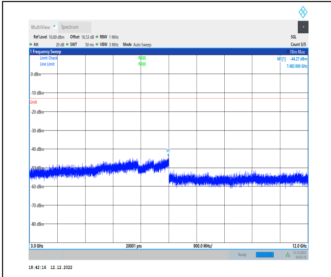
1-N12-15-15-L-1-DFT-PI2BPSK-Inner_1RB_Left-1 @ 1-3000-12000-Ant1-7482.00--44.27--13-PASS
