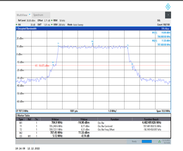
1-N12-15-5-M-3-DFT-16QAM-Outer_Full-25@0-Ant1 -4.482-5.120-≤5-PASS
