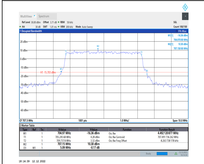
1-N12-15-5-M-6-CP-QPSK-Outer_Full-25@0-Ant1-4 .492-5.090-≤5-PASS
