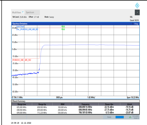
1-N12-15-15-L-6-CP-QPSK-Outer_Full-79@0-Ant1-1--PASS-see graph
