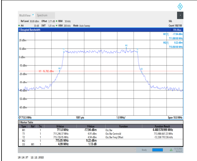
1-N12-15-5-H-5-DFT-256QAM-Outer_Full-25@0-Ant 1-4.481-4.990-≤5-PASS
