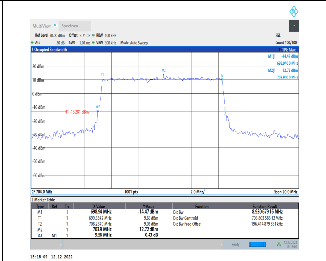
1-N12-15-10-L-1-DFT-QPSK-Outer_Full-50@0-Ant1-8.931-9.560-≤10-PASS
