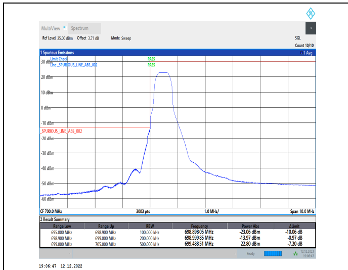
1-N12-15-15-L-1-DFT-PI2BPSK-Edge_1RB_Left-1@0-Ant1-1--PASS-see graph
