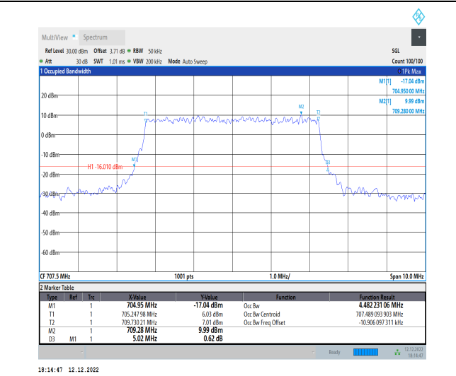
1-N12-15-5-M-7-CP-16QAM-Outer_Full-25@0-Ant1- 4.482-5.020-≤5-PASS
