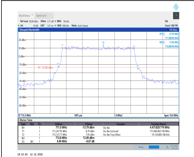
1-N12-15-5-H-1-DFT-QPSK-Outer_Full-25@0-Ant1-4.476-4.940-≤5-PASS
