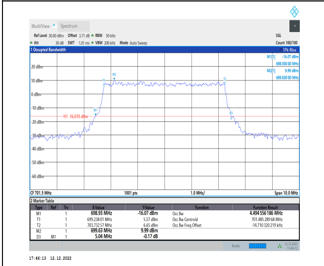
1-N12-15-5-L-7-CP-16QAM-Outer_Full-25@0-Ant1- 4.495-5.040-≤5-PASS
