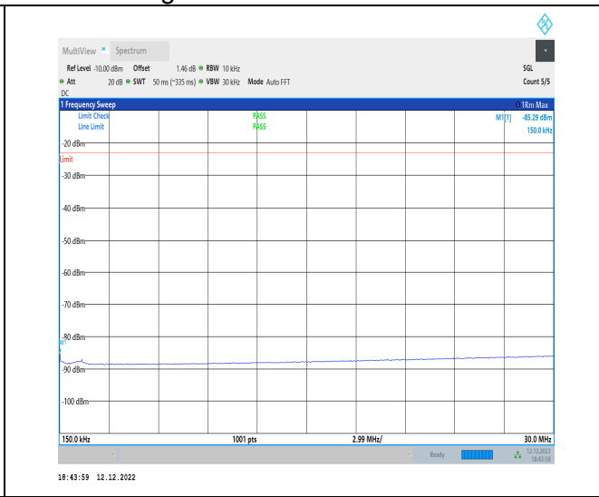
1-N12-15-15-H-1-DFT-PI2BPSK-Inner_1RB_Left-1 @ 1-0.15-30-Ant1-0.15--85.29--23-PASS
