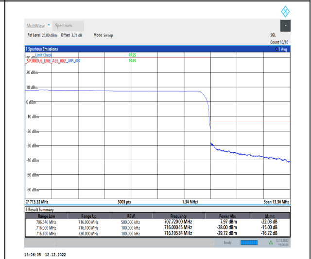
1-N12-15-10-H-6-CP-QPSK-Outer_Full-52@0-Ant1-1--PASS-see graph
