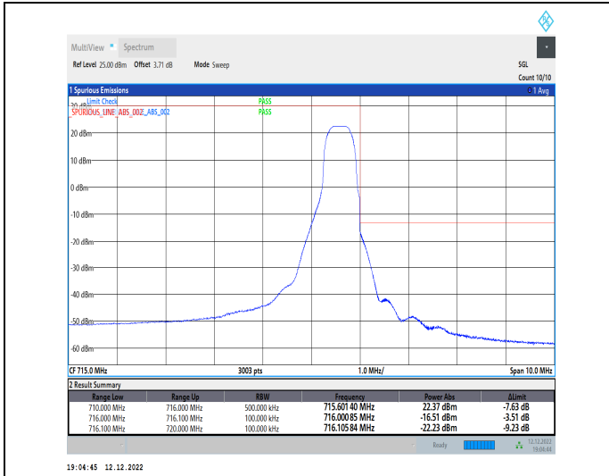
1-N12-15-10-H-2-DFT-PI2BPSK-Edge_1RB_Right-1@51-Ant1-1--PASS-see graph
