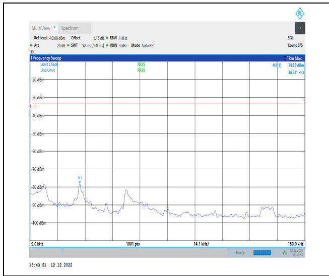
1-N12-15-15-H-1-DFT-PI2BPSK-Inner_1RB_Left-1 @ 1-0.009-0.15-Ant1-0.03--78.33--33-PASS
