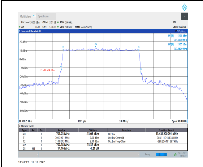
1-N12-15-15-H-3-DFT-16QAM-Outer_Full-75@0-Ant1 1-13.431-14.160≤15-PASS
