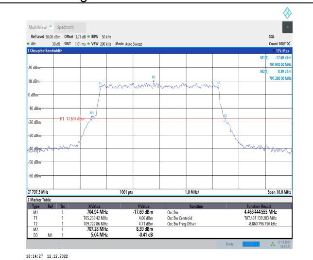
1-N12-15-5-M-5-DFT-256QAM-Outer_Full-25@0-Ant 1-4.463-5.040-≤5-PASS
