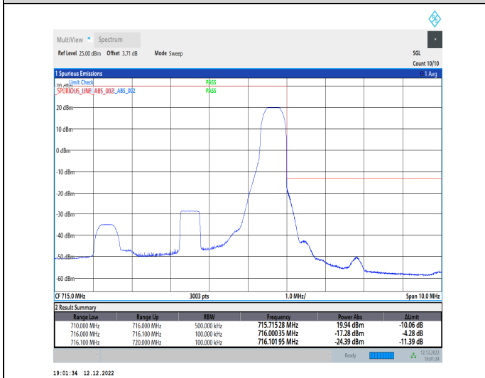
1-N12-15-5-H-5-CP-QPSK-Edge_1RB_Right-1@24-Ant1-1--PASS-see graph
