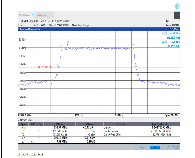
1-N12-15-10-L-4-DFT-64QAM-Outer_Full-50@0-Ant 1-8.942-9.620-≤10-PASS
