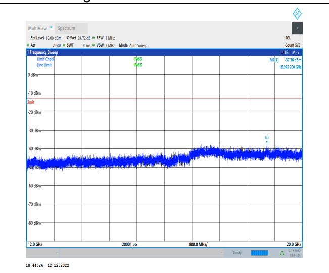
1-N12-15-15-H-1-DFT-PI2BPSK-Inner_1RB_Left-1@ 1-12000-20000-Ant1-18975.20--37.36--13-PASS
