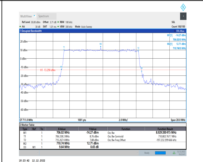
1-N12-15-10-H-3-DFT-16QAM-Outer_Full-50@0-Ant 1-8.929-9.640-≤10-PASS
