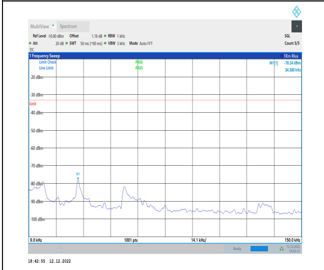
1-N12-15-15-M-1-DFT-PI2BPSK-Inner_1RB_Left-1 @ 1-0.009-0.15-Ant1-0.03--78.24--33-PASS
