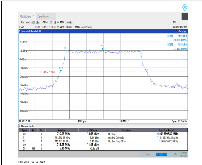
1-N12-15-5-H-3-DFT-16QAM-Outer_Full-25@0-Ant1 -4.495-5.160-≤5-PASS
