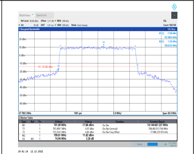
1-N12-15-15-H-8-CP-64QAM-Outer_Full-79@0-Ant1 -14.145-14.940-≤15-PASS
