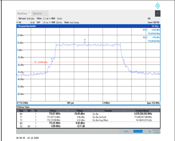
1-N12-15-5-H-6-CP-QPSK-Outer_Full-25@0-Ant1-4. 476-4.990-≤5-PASS
