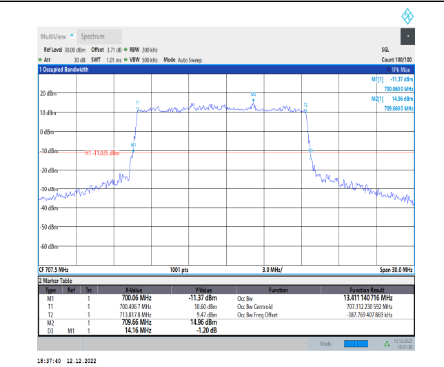
1-N12-15-15-M-1-DFT-QPSK-Outer_Full-75@0-Ant1 -13.411-14.160-≤15-PASS
