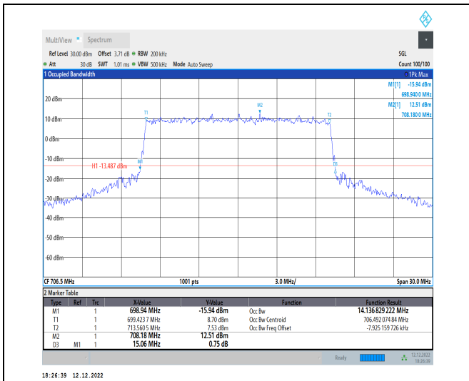
1-N12-15-15-L-7-CP-16QAM-Outer_Full-79@0-Ant1 -14.137-15.060-≤15-PASS
