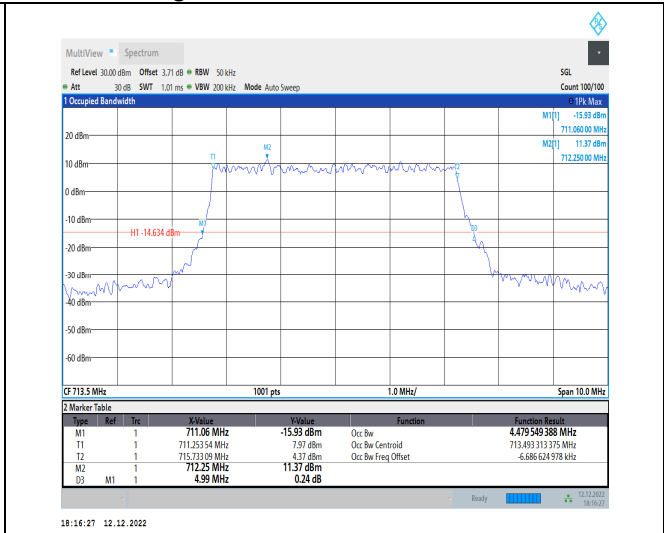
1-N12-15-5-H-4-DFT-64QAM-Outer_Full-25@0-Ant1 -4.48-4.990-≤5-PASS
