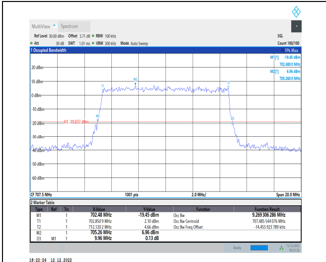
1-N12-15-10-M-9-CP-256QAM-Outer_Full-52@0-An t1-9.269-9.960-≤10-PASS
