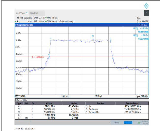
1-N12-15-10-H-4-DFT-64QAM-Outer_Full-50@0-Ant 1-8.934-9.500-≤10-PASS
