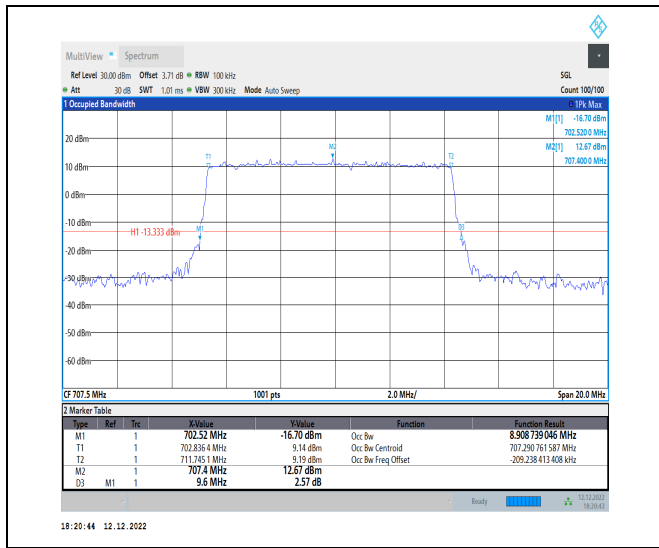
1-N12-15-10-M-1-DFT-QPSK-Outer_Full-50@0-Ant1 -8.909-9.600-≤10-PASS
