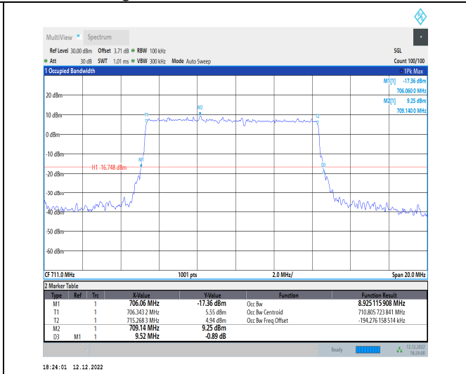
1-N12-15-10-H-5-DFT-256QAM-Outer_Full-50@0-A nt1-8.925-9.520-≤10-PASS
