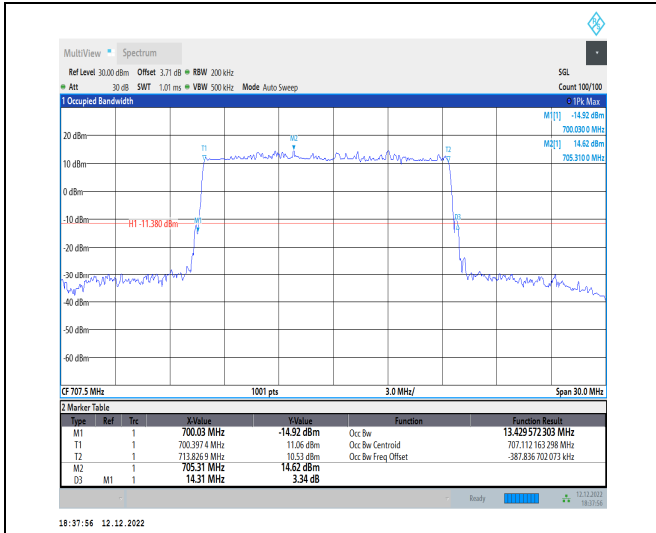
1-N12-15-15-M-2-DFT-PI2BPSK-Outer_Full-75@0-A nt1-13.43-14.310-≤15-PASS
