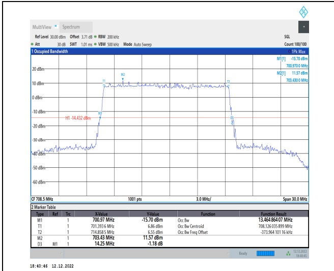
1-N12-15-15-H-5-DFT-256QAM-Outer_Full-75@0-A nt1-13.465-14.250-≤15-PASS
