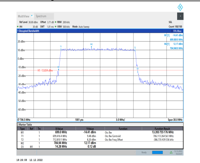
1-N12-15-15-L-4-DFT-64QAM-Outer_Full-75@0-Ant t1-13.394-14.280-≤15-PASS
