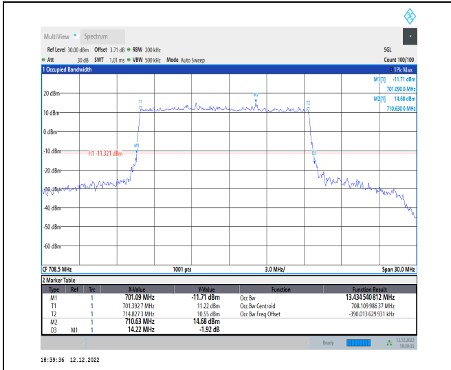
1-N12-15-15-H-1-DFT-QPSK-Outer_Full-75@0-Ant1 -13.435-14.220≤15-PASS
