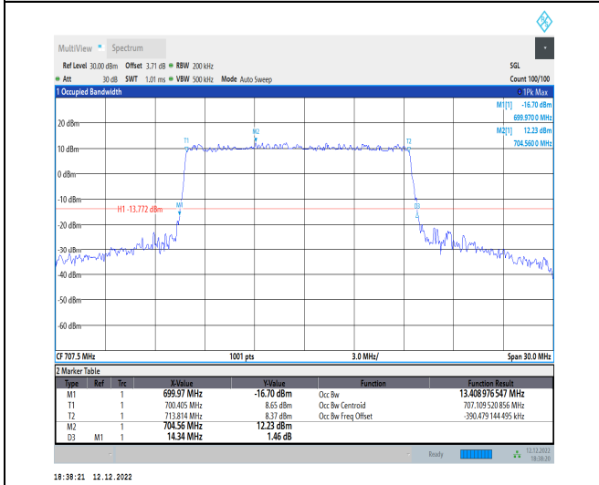
1-N12-15-15-M-4-DFT-64QAM-Outer_Full-75@0-Ant 1-13.409-14.340-≤15-PASS
