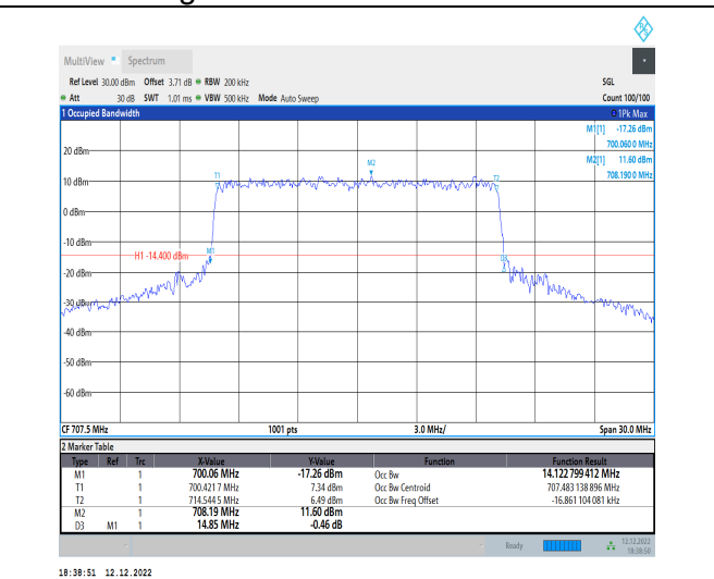
1-N12-15-15-M-7-CP-16QAM-Outer_Full-79@0-Ant1-14.123-14.850-≤15-PASS
