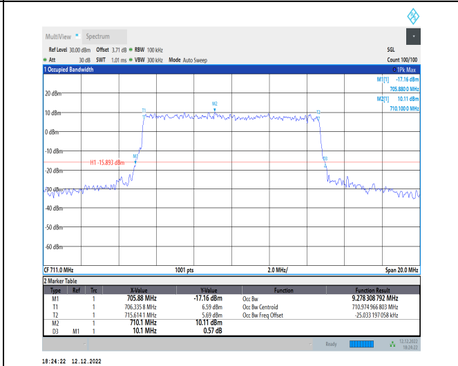
1-N12-15-10-H-7-CP-16QAM-Outer_Full-52@0-Ant1 -9.278-10.100-≤10-PASS
