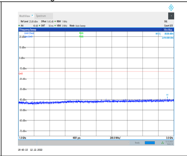
1-N12-15-15-M-1-DFT-PI2BPSK-Inner_1RB_Left-1 @ 1-1000-3000-Ant1-2916.50--38.86--13-PASS
