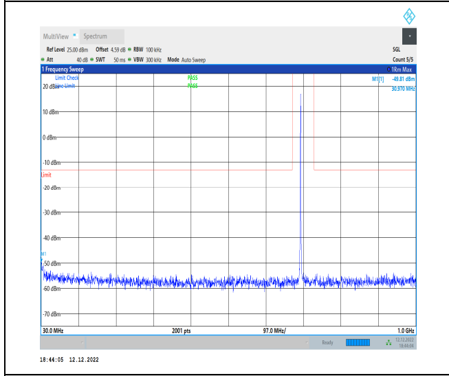
1-N12-15-15-H-1-DFT-PI2BPSK-Inner_1RB_Left-1 @ 1-30-1000-Ant1-30.97--49.81--13-PASS
