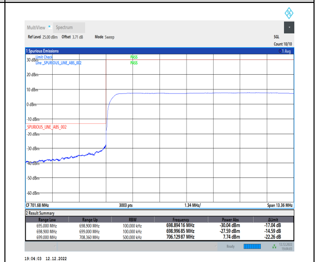
1-N12-15-10-L-6-CP-QPSK-Outer_Full-52@0-Ant1-1--PASS-see graph
