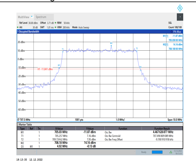
1-N12-15-5-M-1-DFT-QPSK-Outer_Full-25@0-Ant1- 4.468-4.920-≤5-PASS
