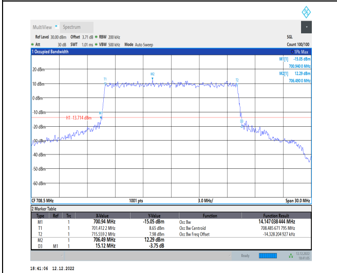
1-N12-15-15-H-7-CP-16QAM-Outer_Full-79@0-Ant1 -14.147-15.120-≤15-PASS
