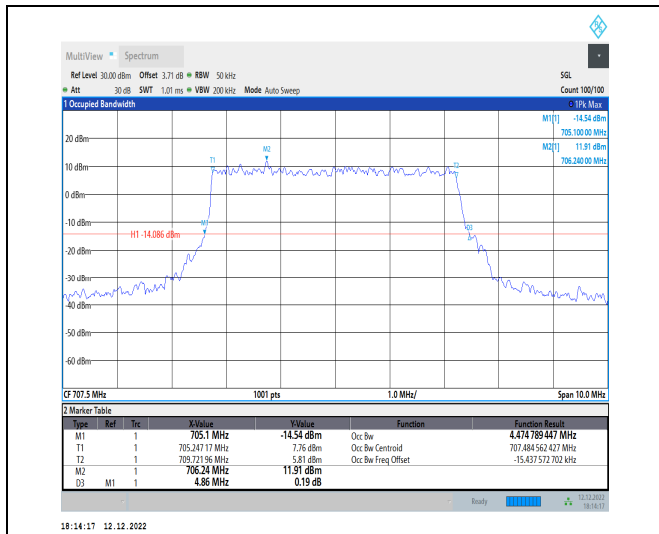
1-N12-15-5-M-4-DFT-64QAM-Outer_Full-25@0-Ant1 -4.475-4.860-≤5-PASS
