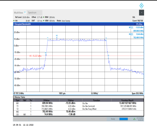
1-N12-15-15-M-5-DFT-256QAM-Outer_Full-75@0-A nt1-13.462-14.400-≤15-PASS
