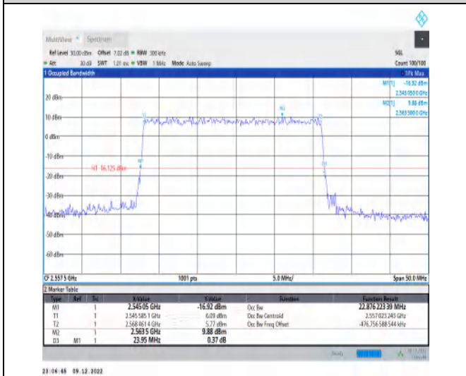
1-N7-15-25-H-5-DFT-256QAM-Outer_Full-128@0-A nt1-22.876-23.950-≤25-PASS
