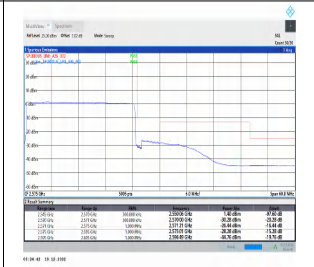
1-N7-15-25-H-6-CP-QPSK-Outer_Full-133@0-Ant1-1--PASS-see graph
