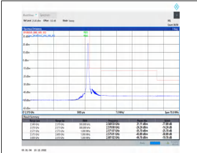
1-N7-15-30-H-2-DFT-PI2BPSK-Edge_1RB_Right-1@159-Ant1-1--PASS-see graph
