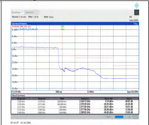
1-N7-15-20-H-3-DFT-PI2BPSK-Outer_Full-100@0-Ant1-1--PASS-see graph
