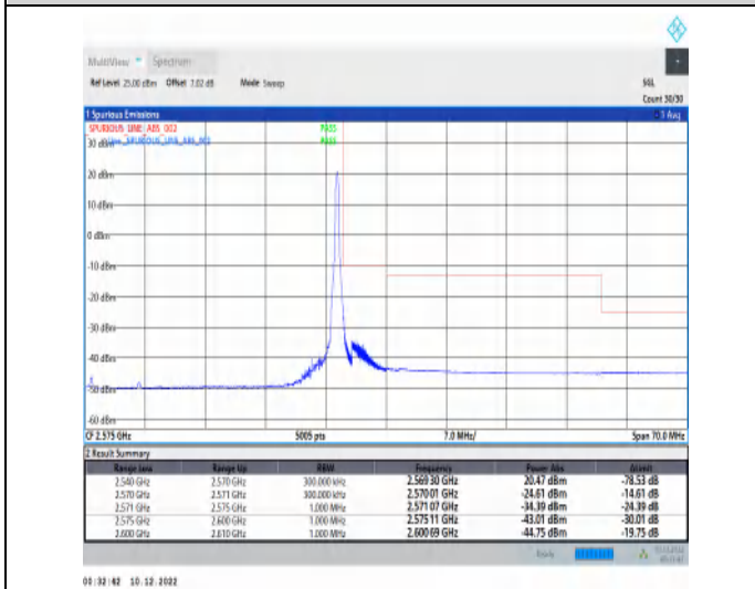
1-N7-15-30-H-5-CP-QPSK-Edge_1RB_Right-1@159-Ant1-1--PASS-see graph
