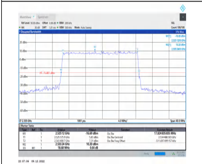
1-N7-15-20-M-5-DFT-256QAM-Outer_Full-100@0-A nt1-17.825-18.680-≤20-PASS
