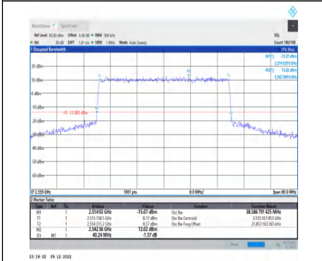
1-N7-15-40-M-4-DFT-64QAM-Outer_Full-216@0-Ant 1-38.587-40.240-≤40-PASS
