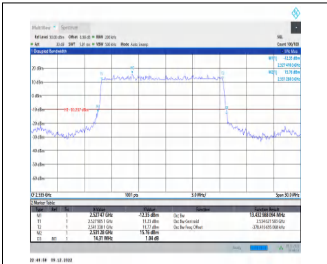
1-N7-15-15-M-2-DFT-PI2BPSK-Outer_Full-75@0-Ant1 t1-13.433-14.310-≤15-PASS
