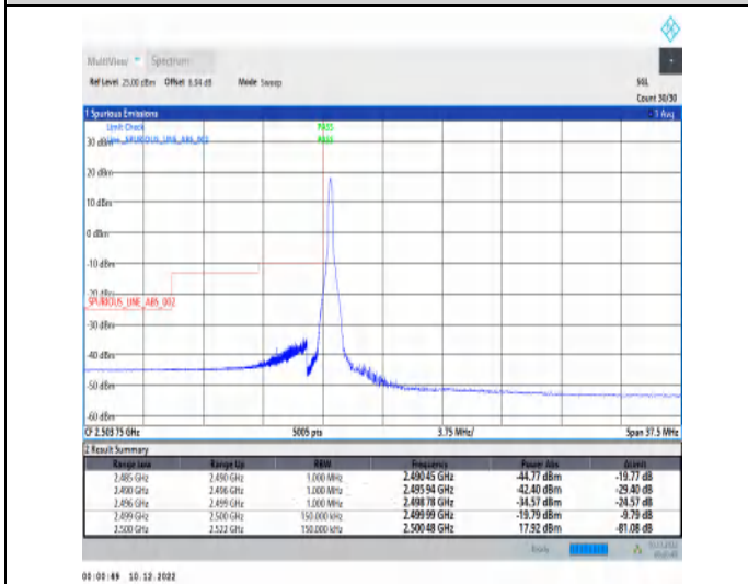
1-N7-15-15-L-4-CP-QPSK-Edge_1RB_Left-1@0-Ant1-1--PASS-see graph
