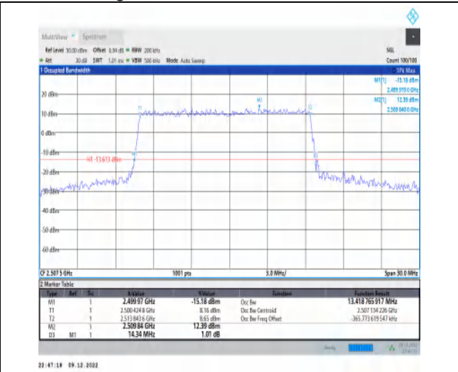
1-N7-15-15-L-4-DFT-64QAM-Outer_Full-75@0-Ant1-13.419-14.340-≤15-PASS
