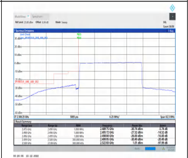
1-N7-15-25-L-6-CP-QPSK-Outer_Full-133@0-Ant1-1--PASS-see graph
