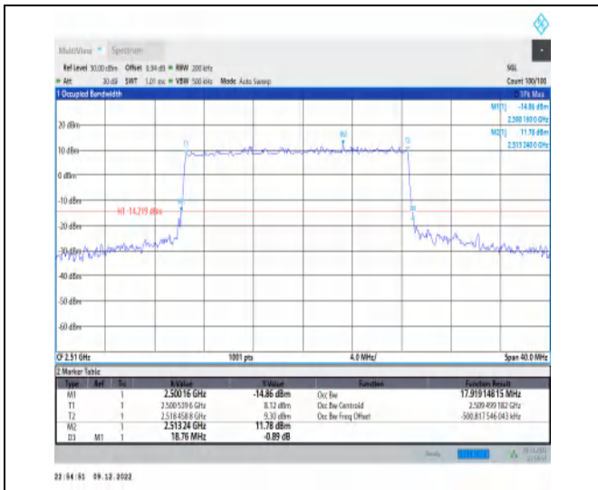
1-N7-15-20-L-4-DFT-64QAM-Outer_Full-100@0-Ant 1-17.919-18.760-≤20-PASS
