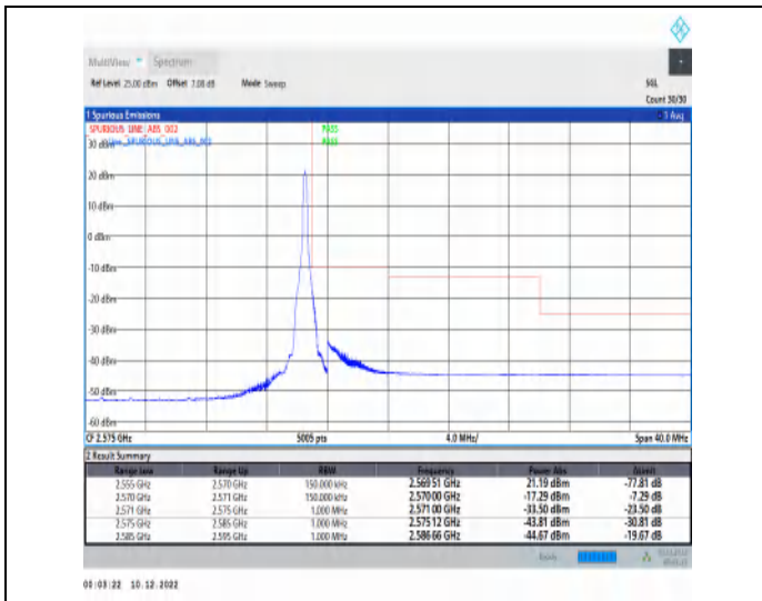
1-N7-15-15-H-2-DFT-PI2BPSK-Edge_1RB_Right-1@78-Ant1-1--PASS-see graph
