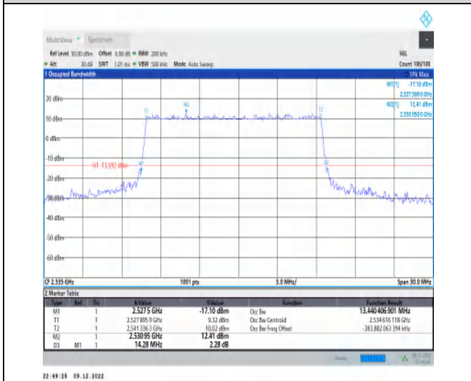
1-N7-15-15-M-4-DFT-64QAM-Outer_Full-75@0-Ant1 -13.44-14.280-≤15-PASS
