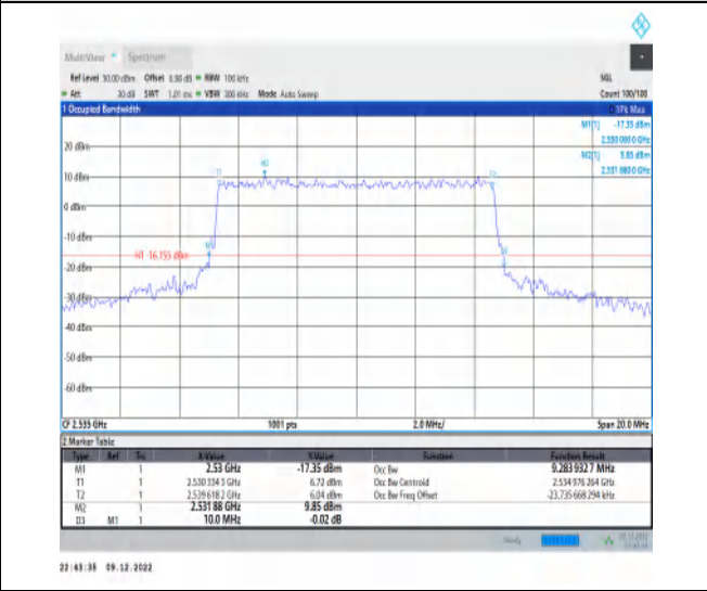
1-N7-15-10-M-8-CP-64QAM-Outer_Full-52@0-Ant1-9. 9.284-10.000-≤10-PASS
