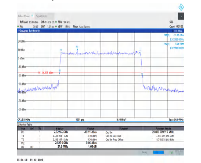
1-N7-15-25-M-9-CP-256QAM-Outer_Full-133@0-Ant1 1-23.806-24.800-≤25-PASS
