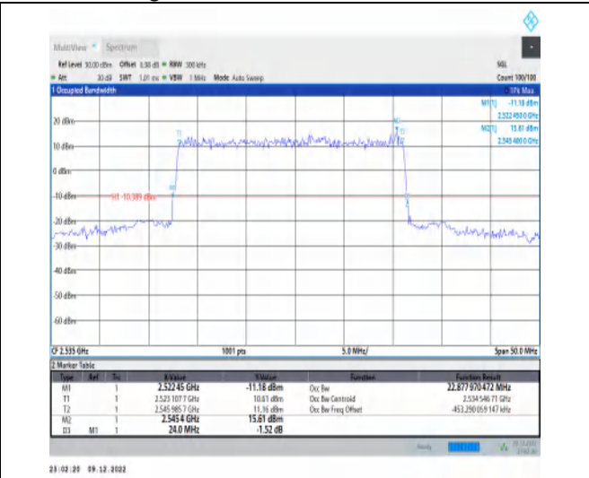
1-N7-15-25-M-1-DFT-QPSK-Outer_Full-128@0-Ant1 -22.878-24.000-≤25-PASS
