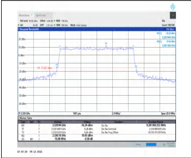
1-N7-15-10-M-7-CP-16QAM-Outer_Full-52@0-Ant1-9. 9.282-10.080-≤10-PASS
