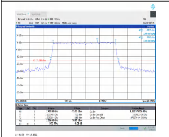
1-N7-15-10-L-4-DFT-64QAM-Outer_Full-50@0-Ant1- 8.956-9.720-≤10-PASS
