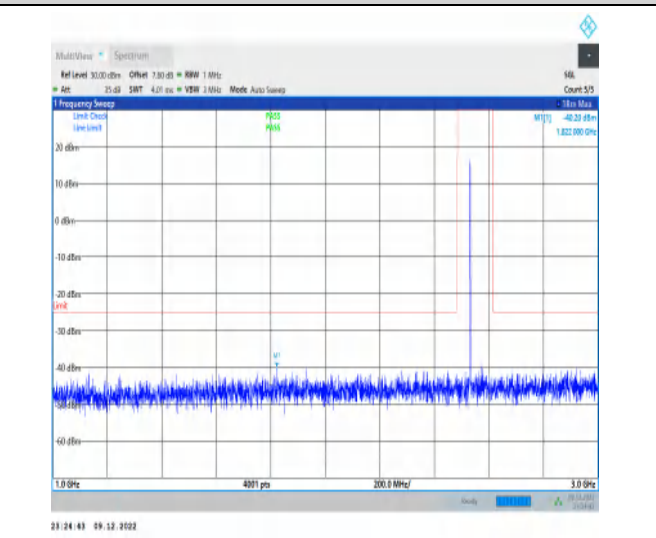
1-N7-15-40-H-1-DFT-PI2BPSK-Inner_1RB_Left-1@ -1000-3000-Ant1-1822.00--40.20--25-PASS
