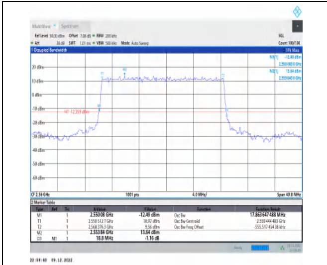
1-N7-15-20-H-2-DFT-PI2BPSK-Outer_Full-100@0-A nt1-17.864-18.800-≤20-PASS
