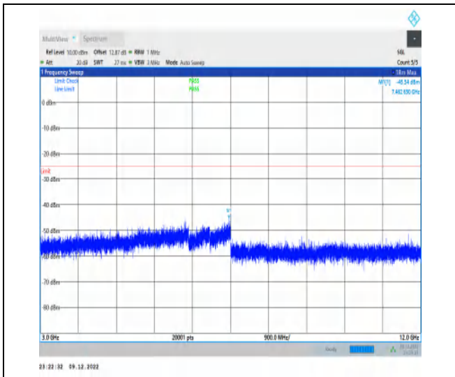
1-N7-15-40-L-1-DFT-PI2BPSK-Inner_1RB_Left-1@ 1-3000-12000-Ant1-7462.65--45.54--25-PASS
