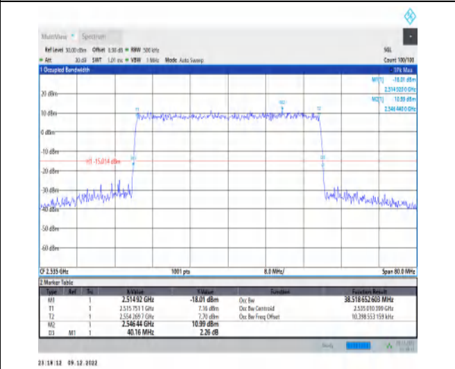
1-N7-15-40-M-5-DFT-256QAM-Outer_Full-216@0-A nt1-38.519-40.160-≤40-PASS
