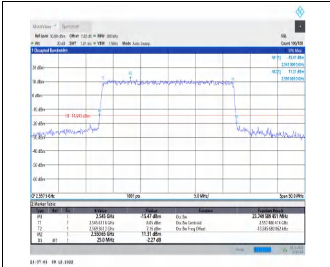
1-N7-15-25-H-7-CP-16QAM-Outer_Full-133@0-Ant1 -23.75-25.000-≤25-PASS
