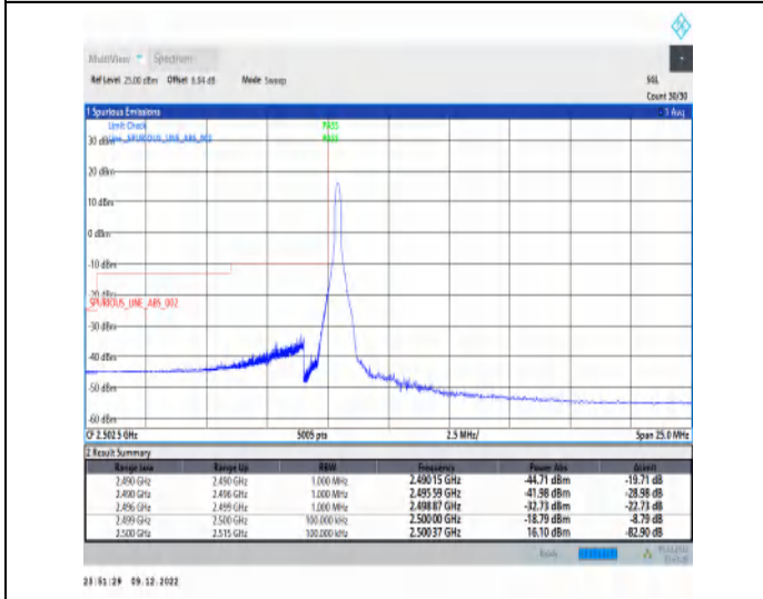
1-N7-15-10-L-4-CP-QPSK-Edge_1RB_Left-1@0-Ant1-1--PASS-see graph
