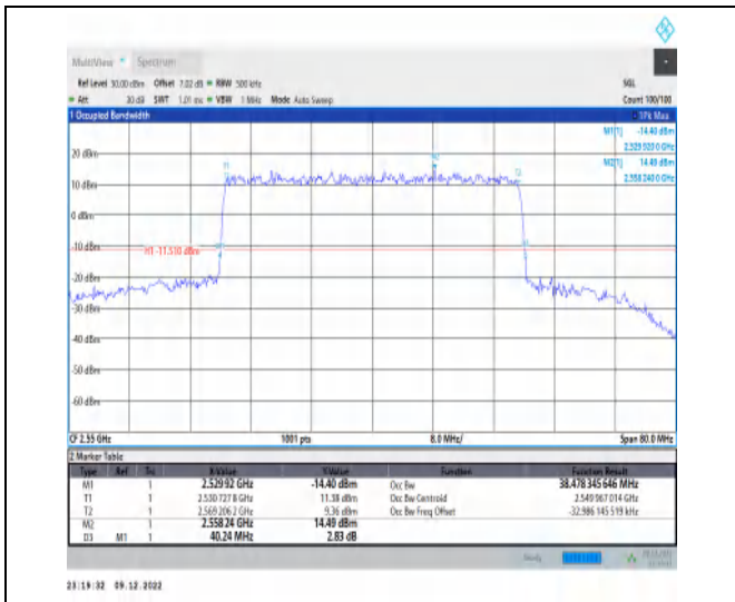
1-N7-15-40-H-1-DFT-QPSK-Outer_Full-216@0-Ant1 -38.478-40.240-≤40-PASS
