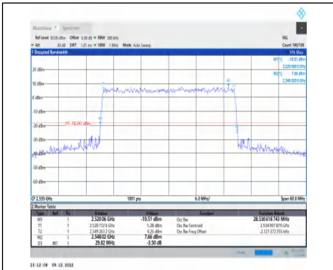
1-N7-15-30-M-9-CP-256QAM-Outer_Full-160@0-Ant 1-28.531-29.820-≤30-PASS
