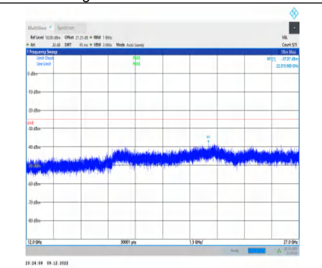
1-N7-15-40-H-1-DFT-PI2BPSK-Inner_1RB_Left-1@ -12000-27000-Ant1-22015.00--37.97--25-PASS
