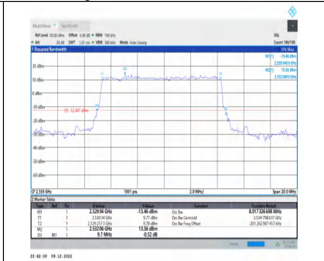
1-N7-15-10-M-2-DFT-PI2BPSK-Outer_Full-50@0-An t1-8.917-9.700-≤10-PASS
