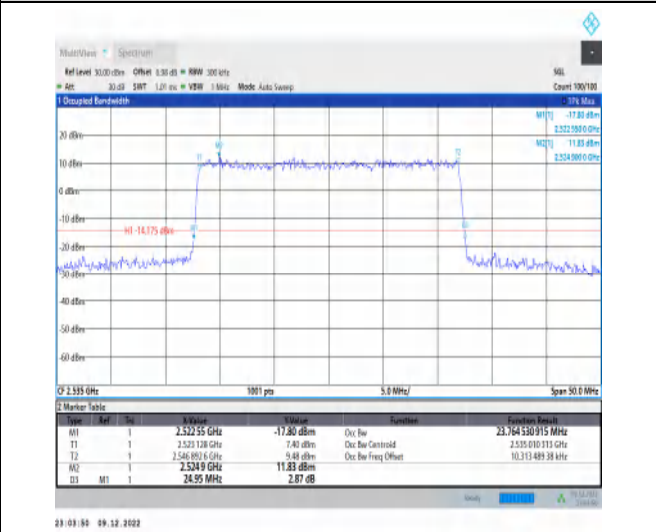
1-N7-15-25-M-3-DFT-16QAM-Outer_Full-128@0-Ant 1-22.993-24.000-≤25-PASS
