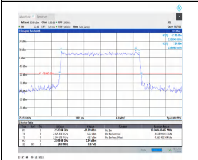
1-N7-15-20-M-9-CP-256QAM-Outer_Full-106@0-Ant 1-19.04-20.000-≤20-PASS
