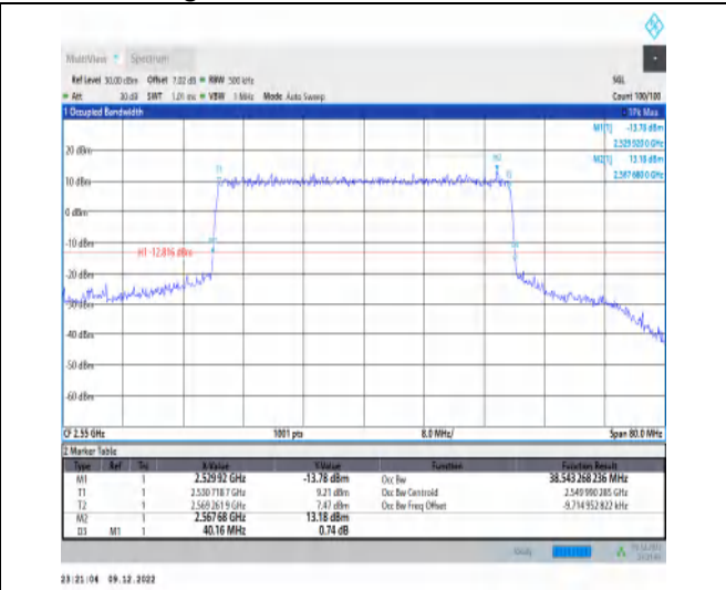
1-N7-15-40-H-6-CP-QPSK-Outer_Full-216@0-Ant1-38.543-40.160-≤40-PASS
