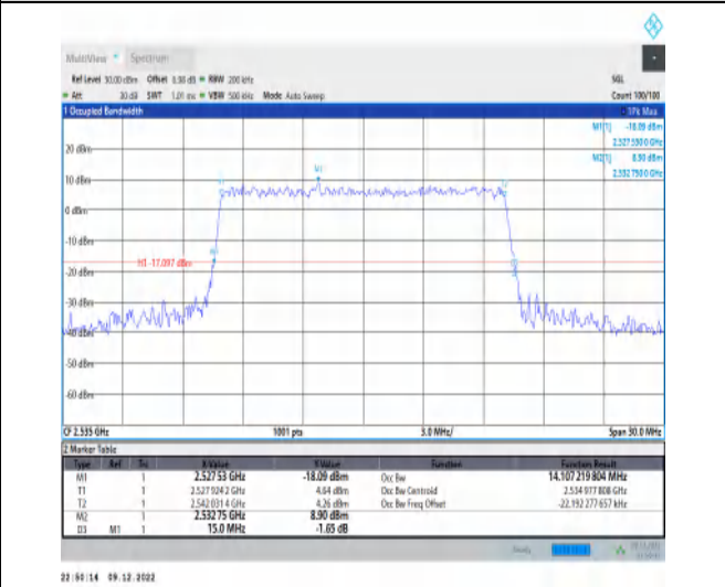
1-N7-15-15-M-9-CP-256QAM-Outer_Full-79@0-Ant1- -14.107-15.000-≤15-PASS
