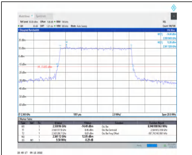
1-N7-15-10-H-4-DFT-64QAM-Outer_Full-50@0-Ant1 -8.949-9.580-≤10-PASS
