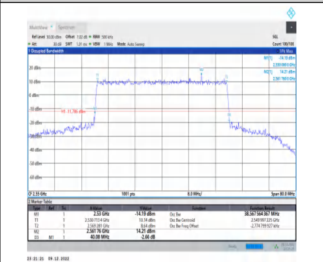
1-N7-15-40-H-8-CP-64QAM-Outer_Full-216@0-Ant1-38.568-40.080-≤40-PASS
