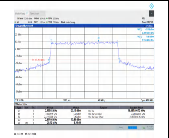
1-N7-15-20-L-7-CP-16QAM-Outer_Full-106@0-Ant1 -18.958-20.120-≤20-PASS
