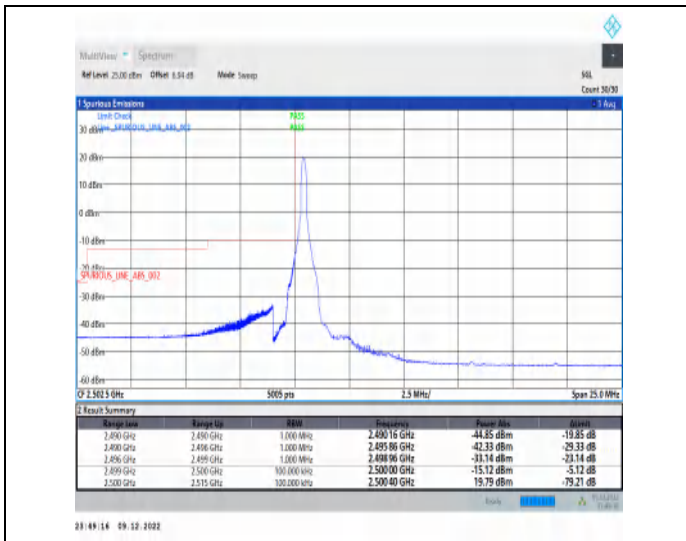
1-N7-15-10-L-1-DFT-PI2BPSK-Edge_1RB_Left-1@0-Ant1-1--PASS-see graph
