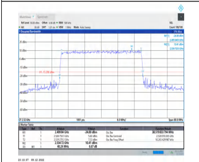
1-N7-15-40-L-5-DFT-256QAM-Outer_Full-216@0-Ant t1-38.52-40.240-≤40-PASS
