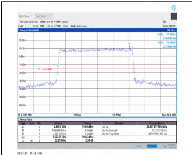
1-N7-15-25-L-5-DFT-256QAM-Outer_Full-128@0-An t1-22.808-23.950-<25-PASS
