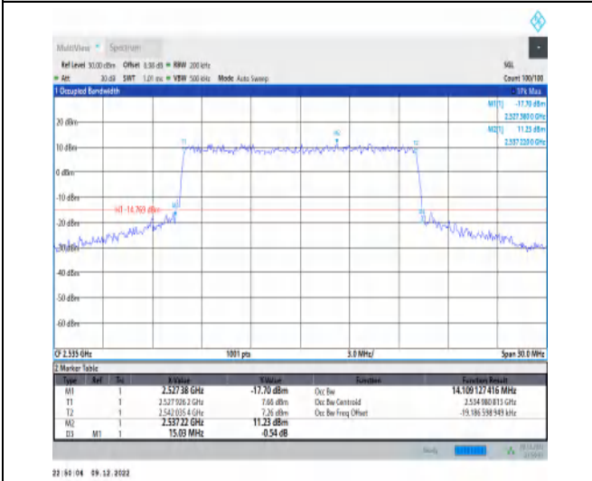
1-N7-15-15-M-8-CP-64QAM-Outer_Full-79@0-Ant1- 14.109-15.030-≤15-PASS
