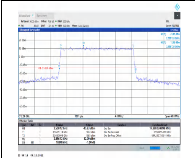
1-N7-15-20-H-4-DFT-64QAM-Outer_Full-100@0-Ant 1-17.888-18.880-≤20-PASS
