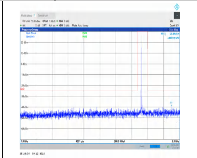
1-N7-15-40-M-1-DFT-PI2BPSK-Inner_1RB_Left-1@ -1000-3000-Ant1-2895.50--39.34--25-PASS
