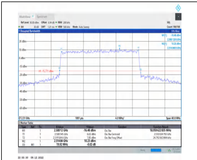
1-N7-15-20-L-8-CP-64QAM-Outer_Full-106@0-Ant1 -18.96-19.920-≤20-PASS
