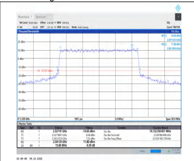
1-N7-15-15-M-3-DFT-16QAM-Outer_Full-75@0-Ant1 -13.464-14.520-≤15-PASS
