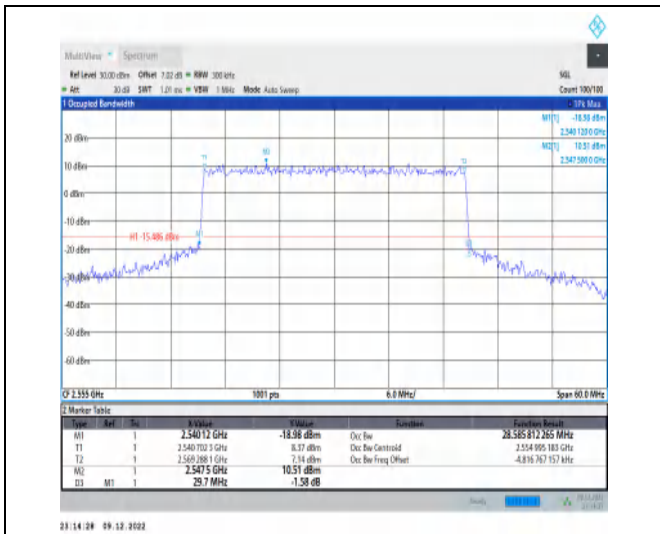
1-N7-15-30-H-8-CP-64QAM-Outer_Full-160@0-Ant1 -28.586-29.700-≤30-PASS
