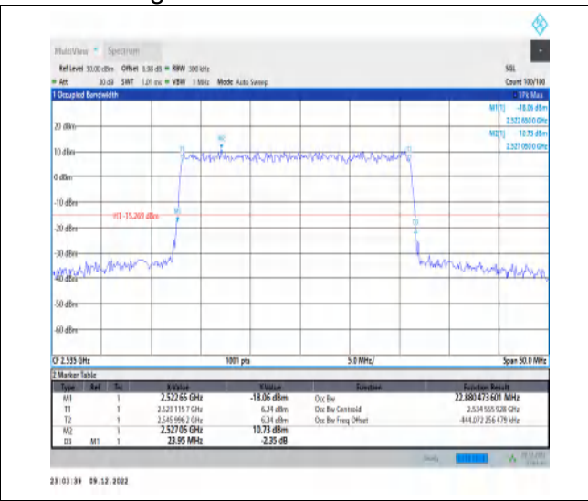
1-N7-15-25-M-5-DFT-256QAM-Outer_Full-128@0-A nt1-22.88-23.950-≤25-PASS
