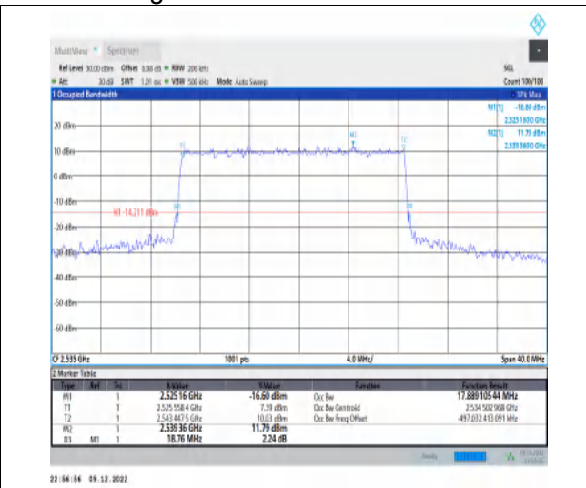
1-N7-15-20-M-4-DFT-64QAM-Outer_Full-100@0-Ant 1-17.889-18.760-≤20-PASS
