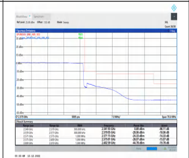
1-N7-15-30-H-6-CP-QPSK-Outer_Full-160@0-Ant1-1--PASS-see graph
