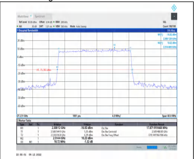
1-N7-15-20-L-5-DFT-256QAM-Outer_Full-100@0-An t1-17.872-18.720-≤20-PASS
