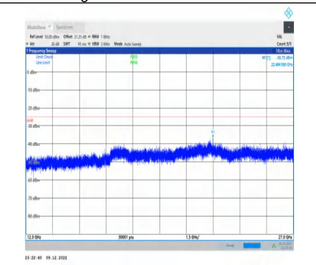
1-N7-15-40-L-1-DFT-PI2BPSK-Inner_1RB_Left-1@ 1-12000-27000-Ant1-22484.50--36.72--25-PASS
