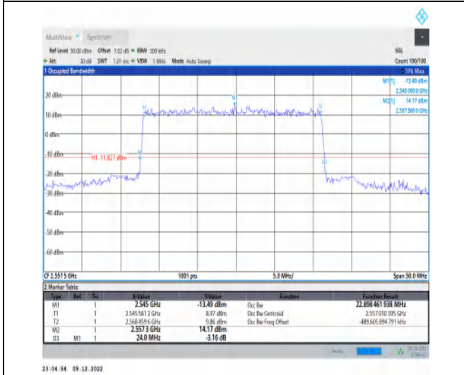
1-N7-15-25-H-1-DFT-QPSK-Outer_Full-128@0-Ant1 -22.898-24.000-≤25-PASS
