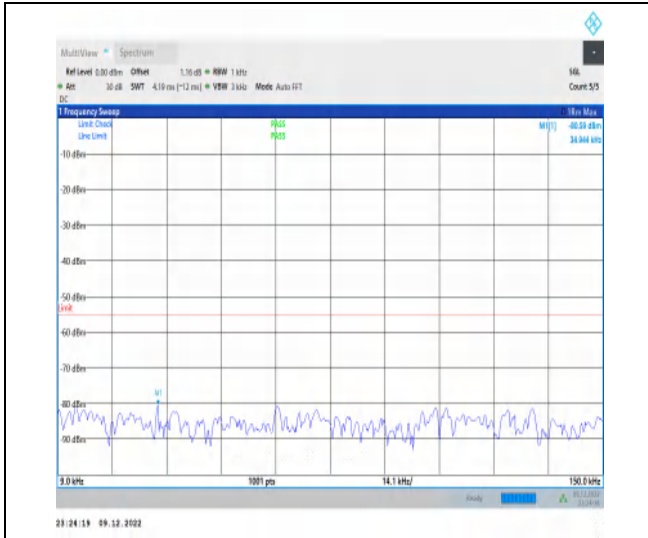
1-N7-15-40-H-1-DFT-PI2BPSK-Inner_1RB_Left-1@ 1-0.009-0.15-Ant1-0.03--80.59--55-PASS
