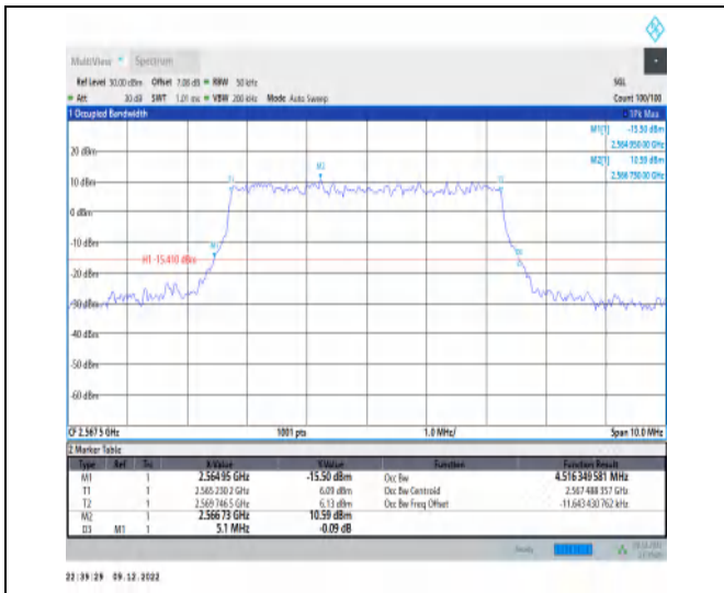
1-N7-15-5-H-7-CP-16QAM-Outer_Full-25@0-Ant1-4. 516-5.100-≤5-PASS
