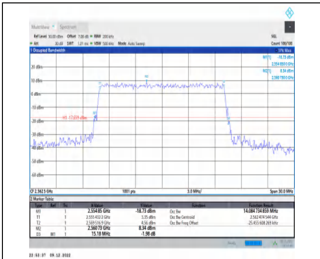
1-N7-15-15-H-9-CP-256QAM-Outer_Full-79@0-Ant1 -14.085-15.180-≤15-PASS
