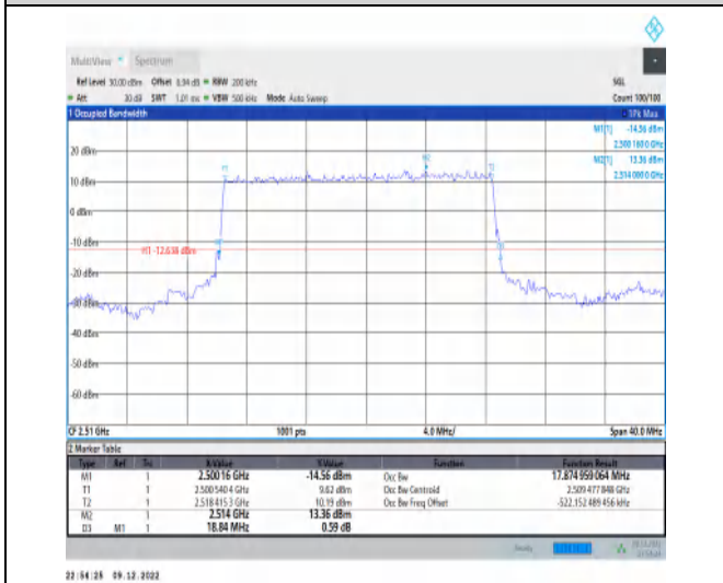
1-N7-15-20-L-2-DFT-PI2BPSK-Outer_Full-100@0-Ant1- 17.875-18.840-≤20-PASS
