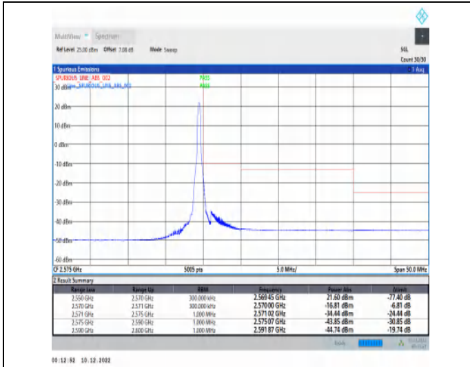
1-N7-15-20-H-2-DFT-PI2BPSK-Edge_1RB_Right-1@105-Ant1-1--PASS-see graph
