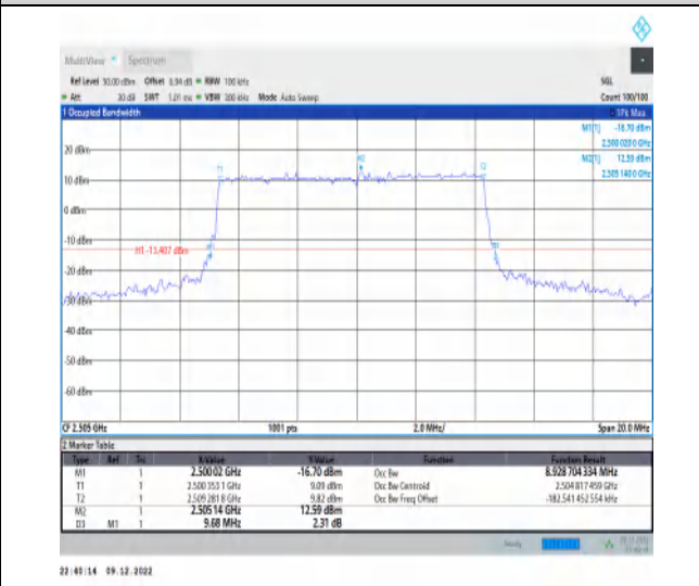
1-N7-15-10-L-1-DFT-QPSK-Outer_Full-50@0-Ant1-8. .929-9.680-≤10-PASS
