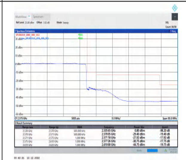
1-N7-15-40-H-6-CP-QPSK-Outer_Full-216@0-Ant 1-1--PASS-see graph
