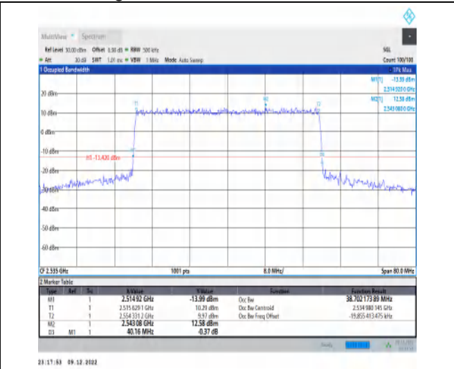
1-N7-15-40-M-3-DFT-16QAM-Outer_Full-216@0-Ant 1-38.702-40.160-≤40-PASS
