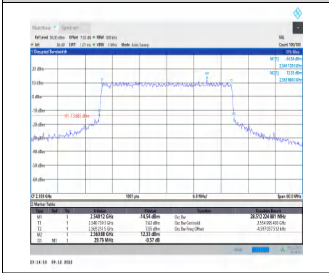
1-N7-15-30-H-6-CP-QPSK-Outer_Full-160@0-Ant1 28.512-29.760-≤30-PASS
