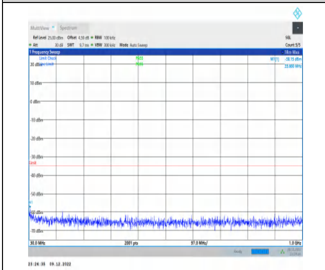
1-N7-15-40-H-1-DFT-PI2BPSK-Inner_1RB_Left-1@ 1-30-1000-Ant1-33.88--58.15--35-PASS
