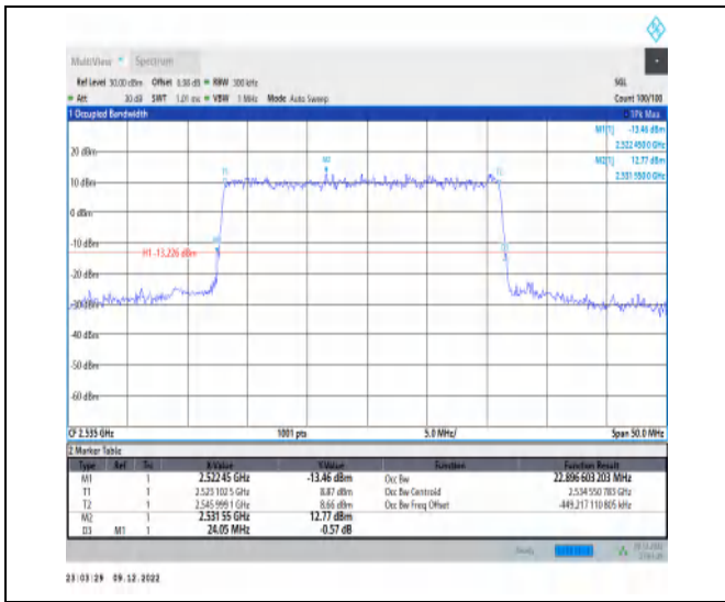
1-N7-15-25-M-4-DFT-64QAM-Outer_Full-128@0-Ant 1-22.897-24.050-≤25-PASS
