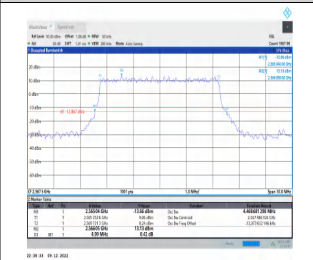
1-N7-15-5-H-2-DFT-PI2BPSK-Outer_Full-25@0-Ant1-4 1-4.469-4.990-≤5-PASS
