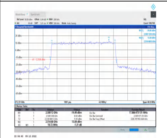
1-N7-15-20-L-3-DFT-16QAM-Outer_Full-100@0-Ant1- 1-17.866-18.720-≤20-PASS
