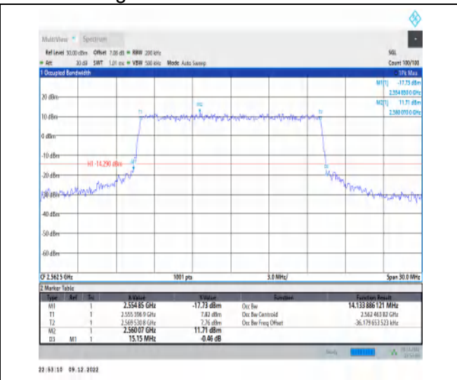
1-N7-15-15-H-6-CP-QPSK-Outer_Full-79@0-Ant1-1 4.134-15.150-≤15-PASS
