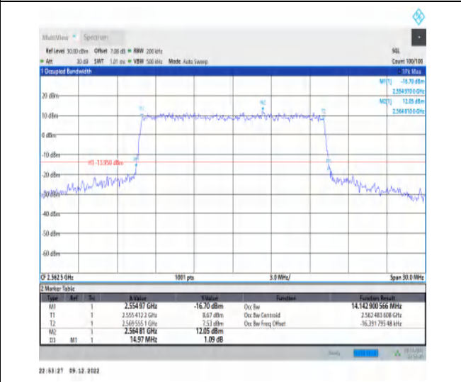
1-N7-15-15-H-8-CP-64QAM-Outer_Full-79@0-Ant1- 14.143-14.970-≤15-PASS
