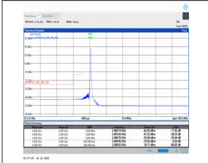
1-N7-15-40-L-4-CP-QPSK-Edge_1RB_Left-1@0-Ant1-1--PASS-see graph
