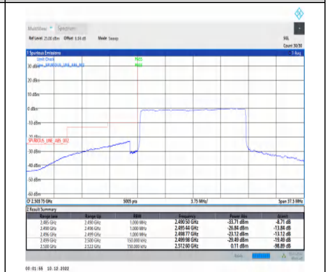
1-N7-15-15-L-6-CP-QPSK-Outer_Full-79@0-Ant1-1--PASS-see graph
