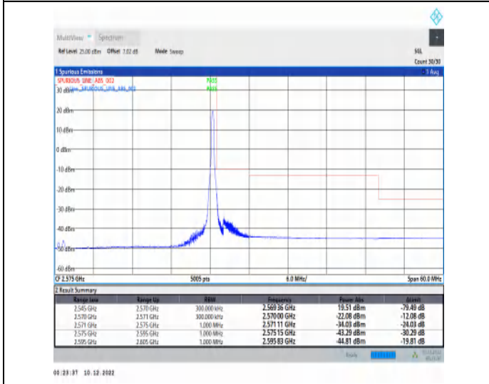
1-N7-15-25-H-5-CP-QPSK-Edge_1RB_Right-1@132-Ant1-1--PASS-see graph
