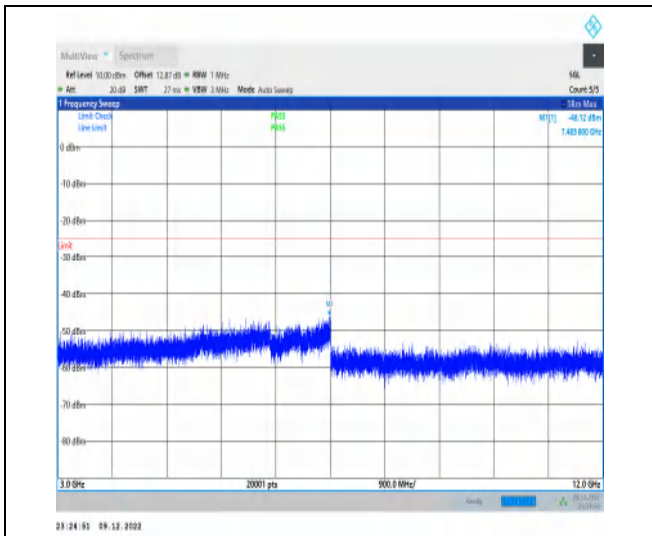
1-N7-15-40-H-1-DFT-PI2BPSK-Inner_1RB_Left-1@ 1-3000-12000-Ant1-7483.80--46.12--25-PASS
