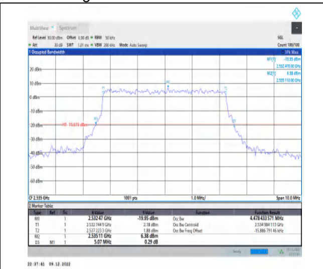
1-N7-15-5-M-9-CP-256QAM-Outer_Full-25@0-Ant1-4 4.478-5.070-≤5-PASS
