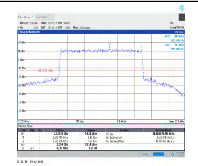
1-N7-15-40-H-4-DFT-64QAM-Outer_Full-216@0-Ant1 1-38.587-40.160-≤40-PASS
