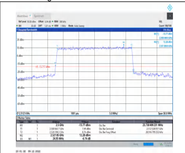
1-N7-15-25-L-6-CP-QPSK-Outer_Full-133@0-Ant1-2 3.73-24.950-<25-PASS
