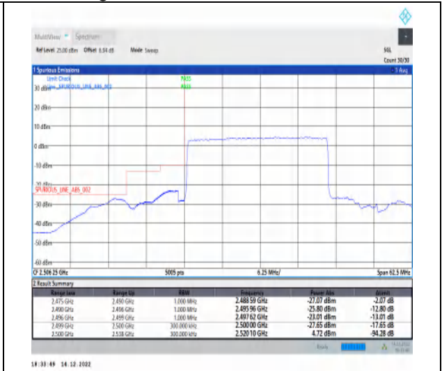
1-N7-15-25-L-3-DFT-PI2BPSK-Outer_Full-128@0-Ant1-1--PASS-see graph
