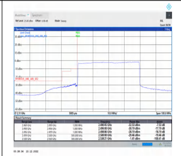
1-N7-15-40-L-6-CP-QPSK-Outer_Full-216@0-Ant1-1--PASS-see graph
