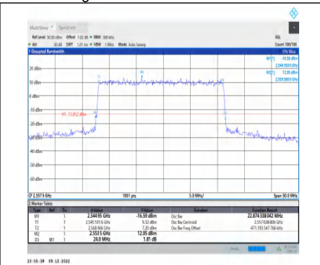
1-N7-15-25-H-4-DFT-64QAM-Outer_Full-128@0-Ant 1-22.874-24.000-≤25-PASS
