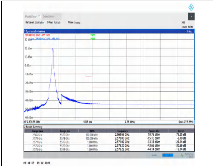
1-N7-15-5-H-2-DFT-PI2BPSK-Edge_1RB_Right-1@24-Ant1-1--PASS-see graph
