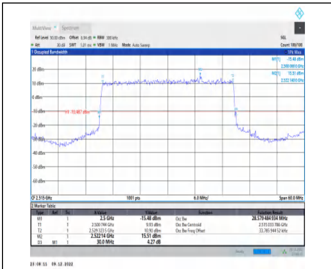
1-N7-15-30-L-2-DFT-PI2BPSK-Outer_Full-160@0-Ant nt1-28.579-30.000-≤30-PASS
