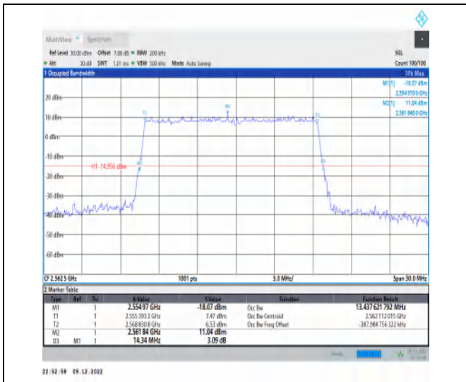
1-N7-15-15-H-5-DFT-256QAM-Outer_Full-75@0-Ant 1-13.438-14.340-≤15-PASS
