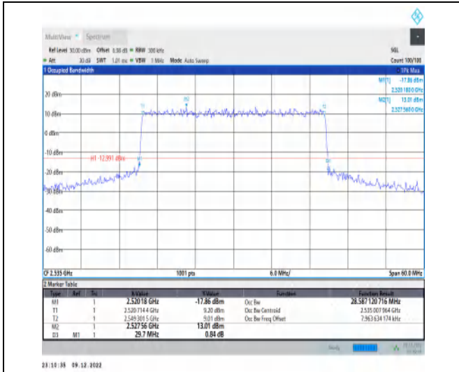
1-N7-15-30-M-1-DFT-QPSK-Outer_Full-160@0-Ant1 -28.587-29.700-≤30-PASS
