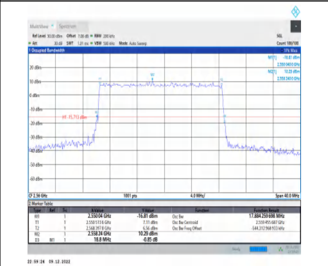
1-N7-15-20-H-5-DFT-256QAM-Outer_Full-100@0-A nt1-17.884-18.800-≤20-PASS
