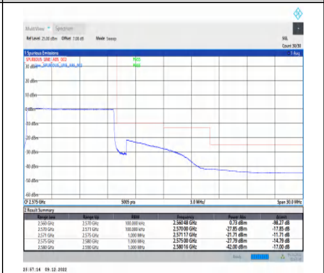
1-N7-15-10-H-6-CP-QPSK-Outer_Full-52@0-Ant1 -1--PASS-see graph
