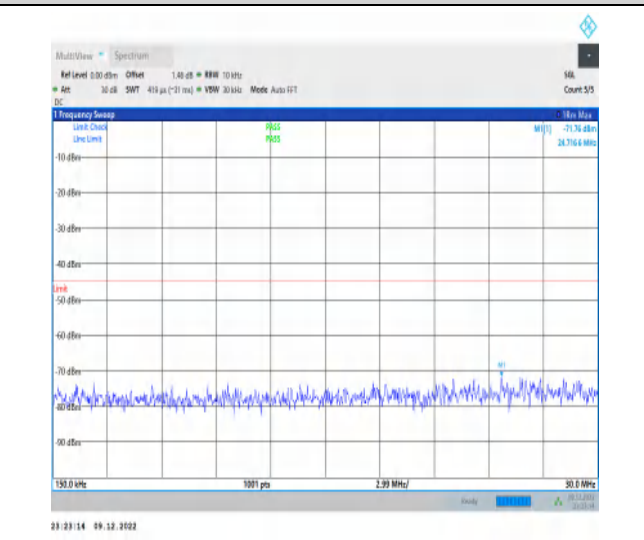
1-N7-15-40-M-1-DFT-PI2BPSK-Inner_1RB_Left-1@ 1-0.15-30-Ant1-24.72--71.76--45-PASS
