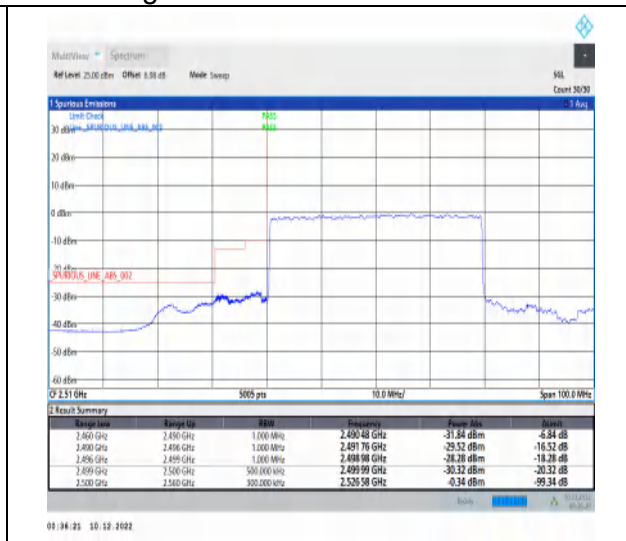
1-N7-15-40-L-3-DFT-PI2BPSK-Outer_Full-216@0 -Ant1-1--PASS-see graph
