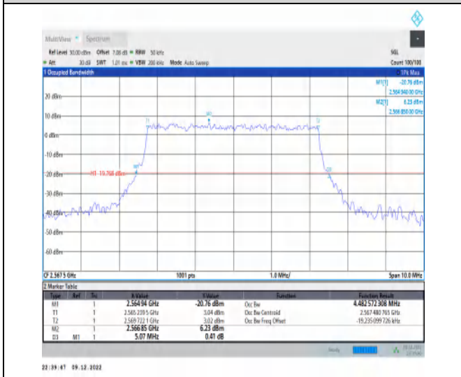
1-N7-15-5-H-9-CP-256QAM-Outer_Full-25@0-Ant1-4. 4.483-5.070-≤5-PASS
