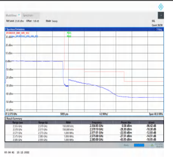
1-N7-15-15-H-6-CP-QPSK-Outer_Full-79@0-Ant1-1--PASS-see graph
