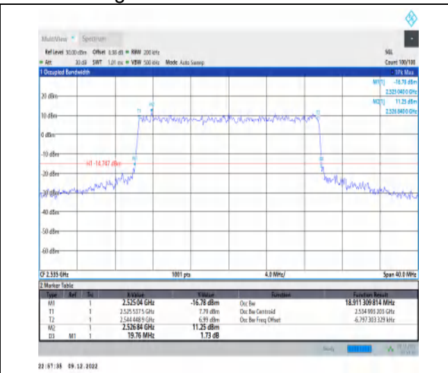
1-N7-15-20-M-8-CP-64QAM-Outer_Full-106@0-Ant1 -18.911-19.760-≤20-PASS
