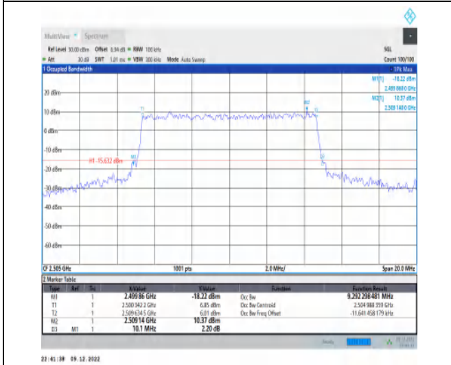
1-N7-15-10-L-8-CP-64QAM-Outer_Full-52@0-Ant1-9. 292-10.100-≤10-PASS
