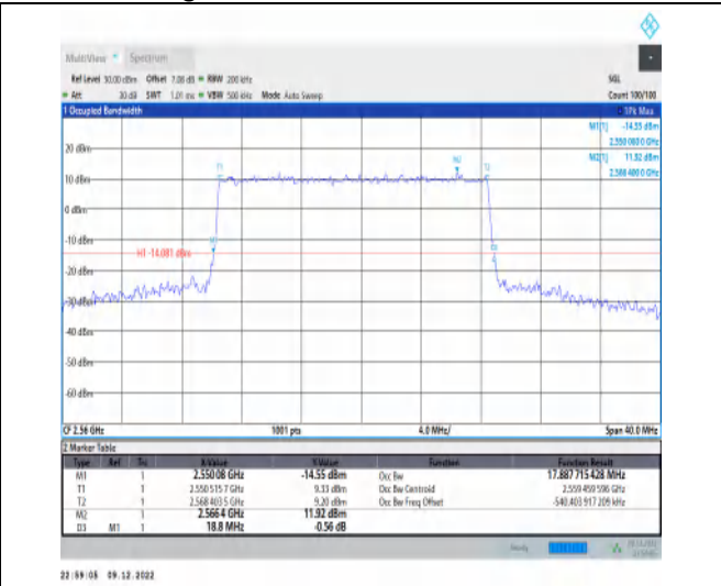
1-N7-15-20-H-3-DFT-16QAM-Outer_Full-100@0-Ant 1-17.888-18.800-≤20-PASS
