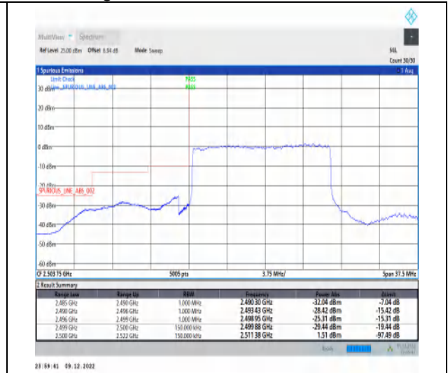
1-N7-15-15-L-3-DFT-PI2BPSK-Outer_Full-75@0-Ant1-1--PASS-see graph
