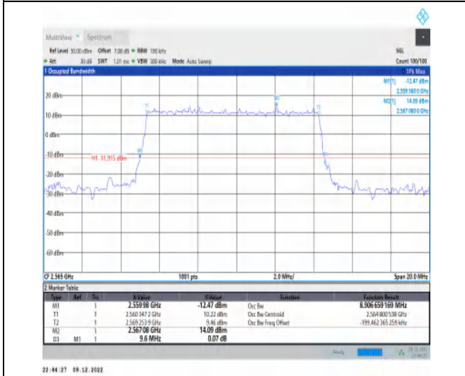
1-N7-15-10-H-2-DFT-P12BPSK-Outer_Full-50@0-Ant1 t1-8.907-9.600≤10-PASS
