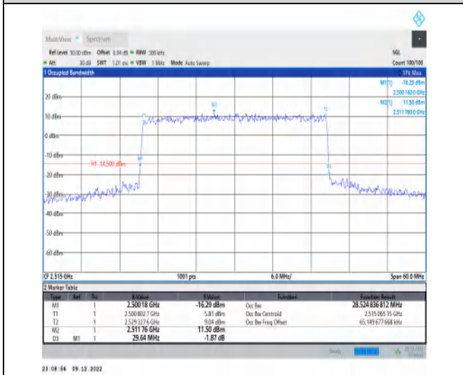
1-N7-15-30-L-4-DFT-64QAM-Outer_Full-160@0-Ant 1-28.525-29.640-≤30-PASS
