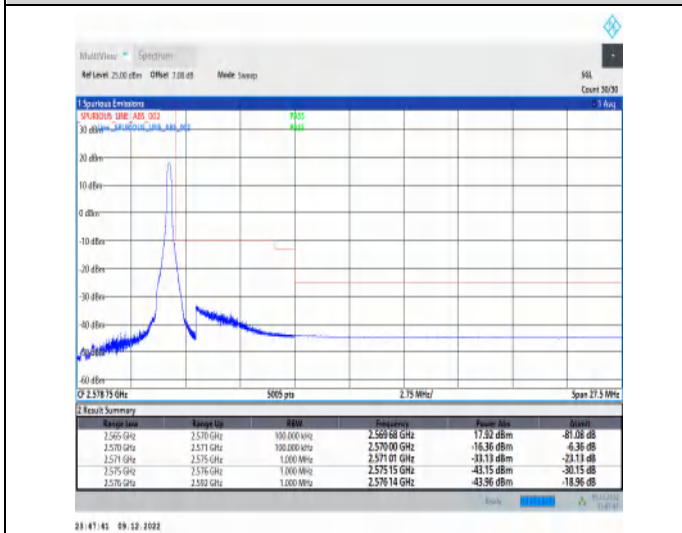
1-N7-15-5-H-5-CP-QPSK-Edge_1RB_Right-1@24-Ant1-1--PASS-see graph
