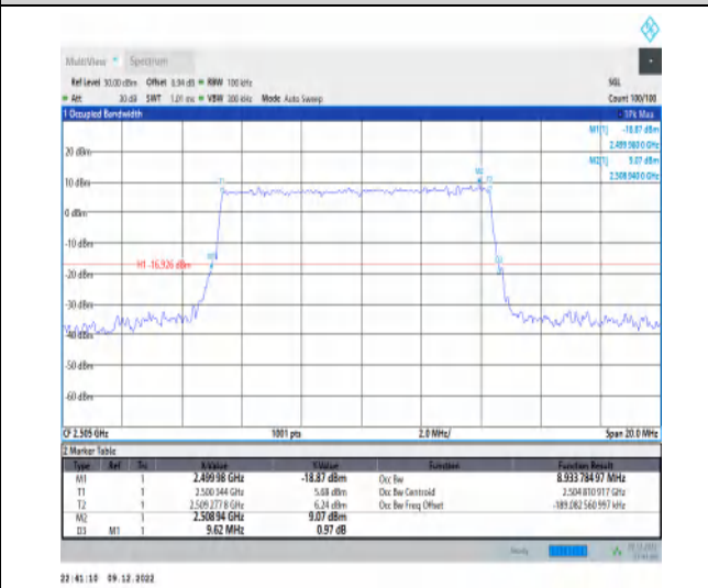
1-N7-15-10-L-5-DFT-256QAM-Outer_Full-50@0-Ant 1-8.934-9.620-≤10-PASS
