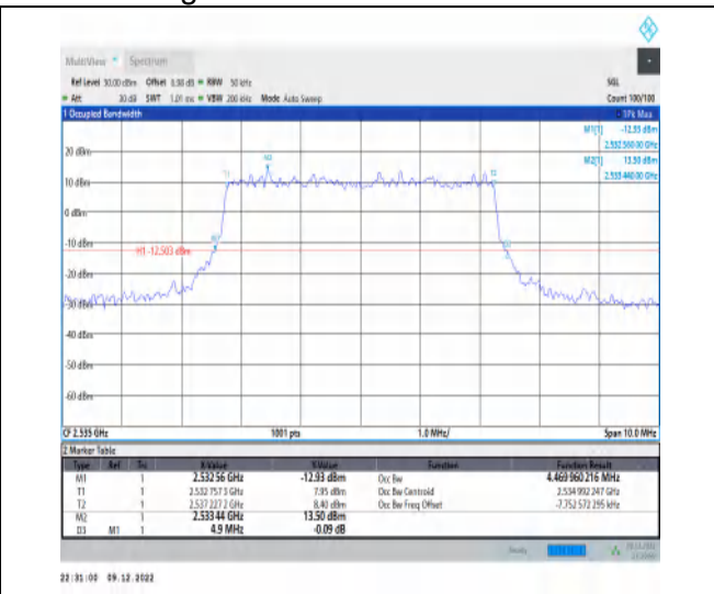
1-N7-15-5-M-1-DFT-QPSK-Outer_Full-25@0-Ant1-4.47-4.900-≤5-PASS
