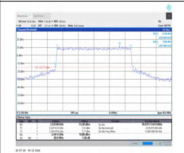
1-N7-15-20-M-6-CP-QPSK-Outer_Full-106@0-Ant1 18.919-20.000-≤20-PASS
