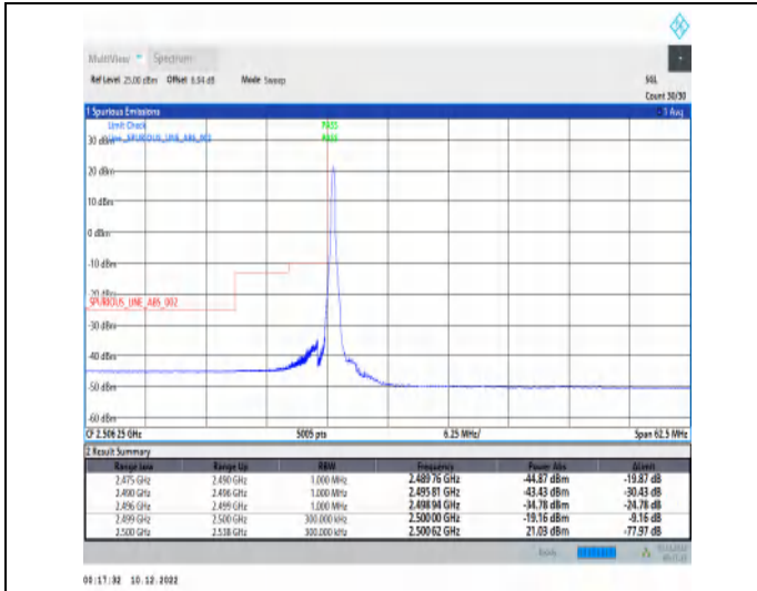
1-N7-15-25-L-1-DFT-PI2BPSK-Edge_1RB_Left-1@0-Ant1-1--PASS-see graph
