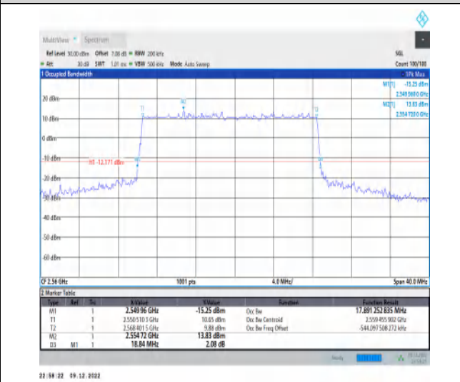
1-N7-15-20-H-1-DFT-QPSK-Outer_Full-100@0-Ant1 -17.891-18.840-≤20-PASS
