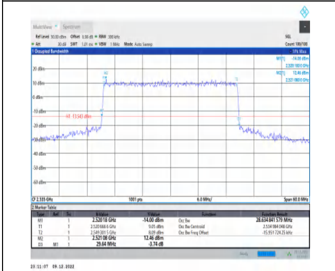
1-N7-15-30-M-3-DFT-16QAM-Outer_Full-160@0-Ant1 1-28.635-29.640-≤30-PASS
