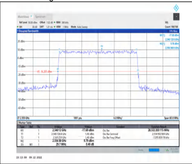
1-N7-15-30-H-5-DFT-256QAM-Outer_Full-160@0-A nt1-28.532-29.700-≤30-PASS
