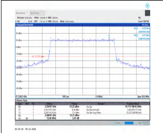
1-N7-15-15-H-7-CP-16QAM-Outer_Full-79@0-Ant1- 14.115-15.060-≤15-PASS
