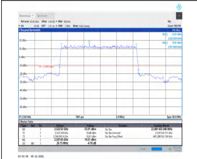
1-N7-15-25-M-2-DFT-PI2BPSK-Outer_Full-128@0-A nt1-22.901-24.150-≤25-PASS
