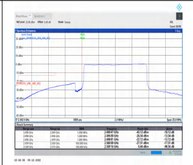
1-N7-15-10-L-6-CP-QPSK-Outer_Full-52@0-Ant1-1--PASS-see graph
