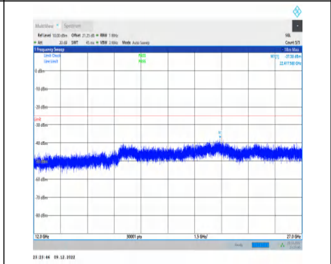
1-N7-15-40-M-1-DFT-PI2BPSK-Inner_1RB_Left-1@ -12000-27000-Ant1-22417.50--37.58--25-PASS
