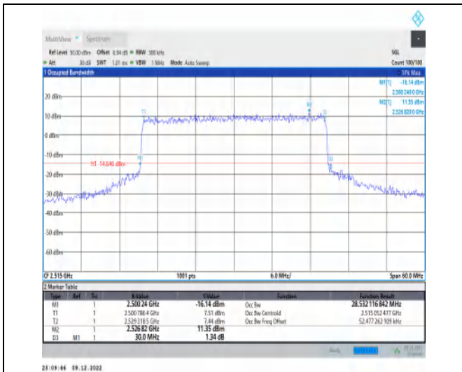
1-N7-15-30-L-6-CP-QPSK-Outer_Full-160@0-Ant1-2 8.532-30.000-≤30-PASS
