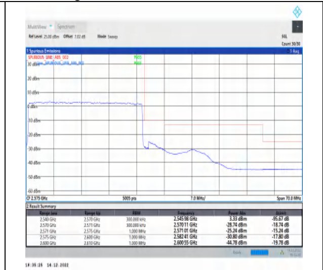
1-N7-15-30-H-3-DFT-PI2BPSK-Outer_Full-160@0-Ant1-1--PASS-see graph
