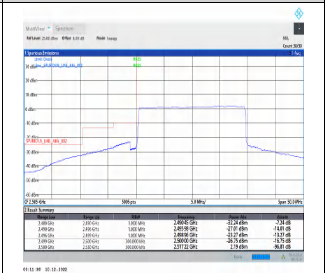
1-N7-15-20-L-6-CP-QPSK-Outer_Full-106@0-Ant1-1--PASS-see graph
