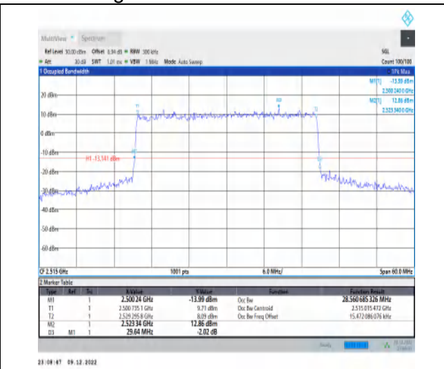
1-N7-15-30-L-3-DFT-16QAM-Outer_Full-160@0-Ant 1-28.561-29.640-≤30-PASS
