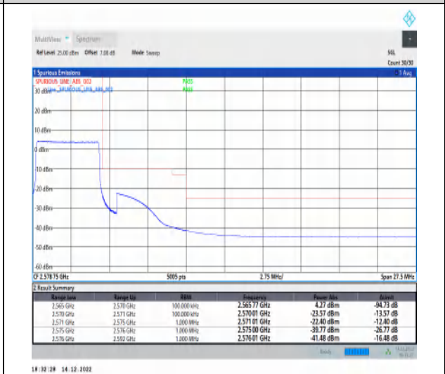
1-N7-15-5-H-6-CP-QPSK-Outer_Full-25@0-Ant1-1--PASS-see graph
