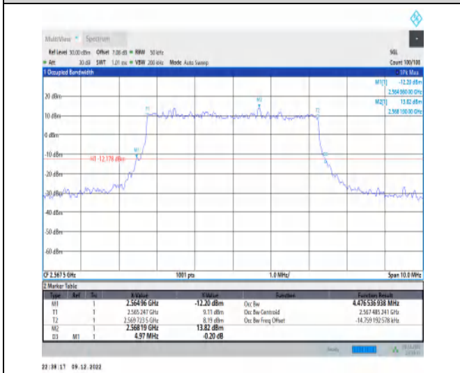
1-N7-15-5-H-1-DFT-QPSK-Outer_Full-25@0-Ant1-4. 477-4.970-≤5-PASS
