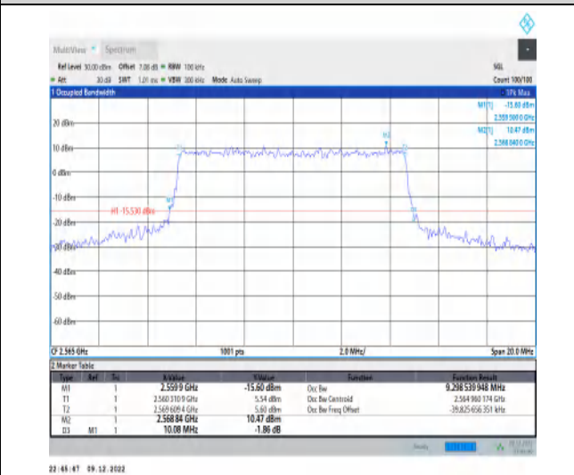
1-N7-15-10-H-7-CP-16QAM-Outer_Full-52@0-Ant1-9. 9.299-10.080-≤10-PASS
