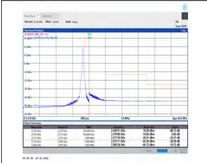
1-N7-15-15-H-5-CP-QPSK-Edge_1RB_Right-1@78-Ant1-1--PASS-see graph
