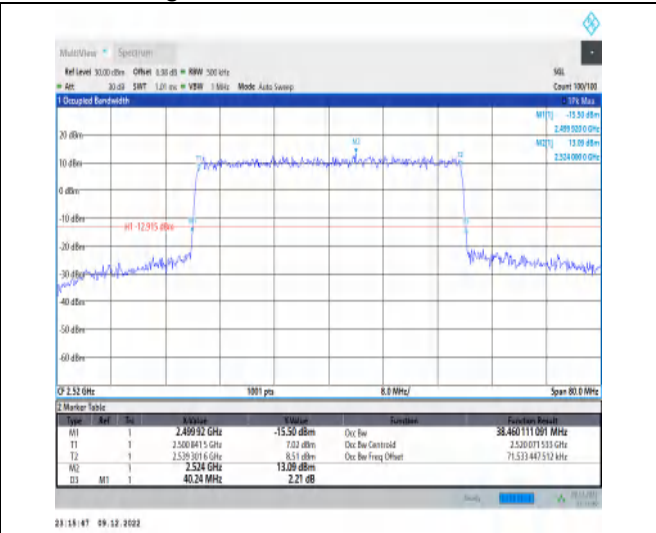
1-N7-15-40-L-4-DFT-64QAM-Outer_Full-216@0-Ant 1-38.46-40.240-≤40-PASS
