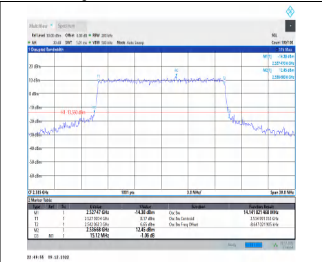
1-N7-15-15-M-7-CP-16QAM-Outer_Full-79@0-Ant1- 14.142-15.120-≤15-PASS
