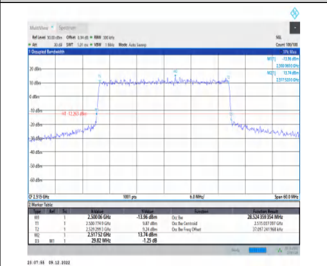
1-N7-15-30-L-1-DFT-QPSK-Outer_Full-160@0-Ant1 28.524-29.820-≤30-PASS
