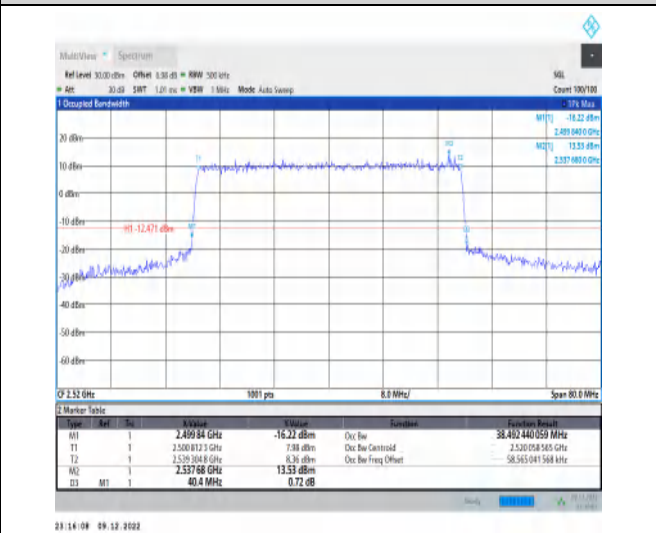
1-N7-15-40-L-6-CP-QPSK-Outer_Full-216@0-Ant1-3 8.492-40.400-≤40-PASS
