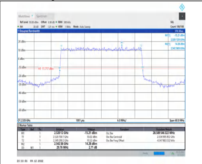
1-N7-15-30-M-2-DFT-PI2BPSK-Outer_Full-160@0-Ant1 -28.59-29.760-≤30-PASS
