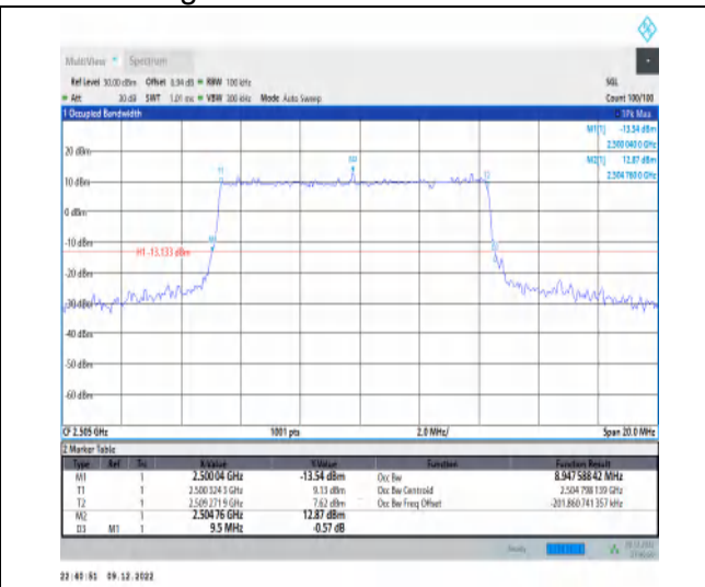
1-N7-15-10-L-3-DFT-16QAM-Outer_Full-50@0-Ant1- 8.948-9.500-≤10-PASS
