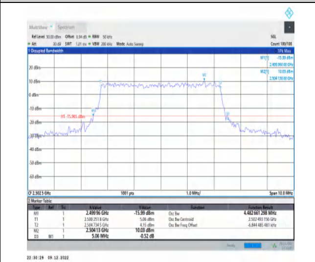
1-N7-15-5-L-8-CP-64QAM-Outer_Full-25@0-Ant1-4.482-5.060-≤5-PASS
