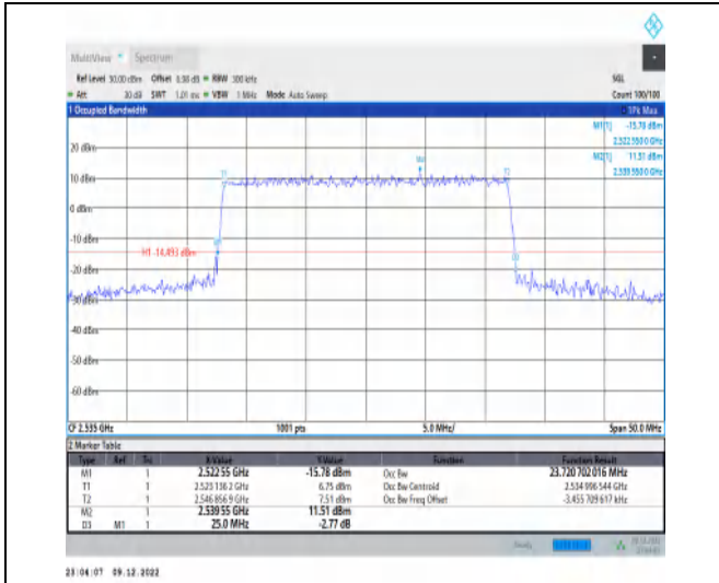
1-N7-15-25-M-8-CP-64QAM-Outer_Full-133@0-Ant1 -23.721-25.000-≤25-PASS
