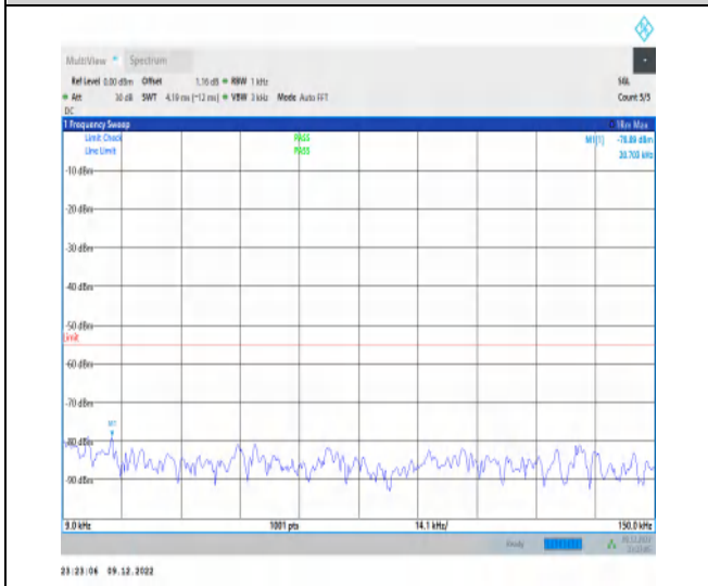
1-N7-15-40-M-1-DFT-PI2BPSK-Inner_1RB_Left-1@ 1-0.009-0.15-Ant1-0.02--78.89--55-PASS
