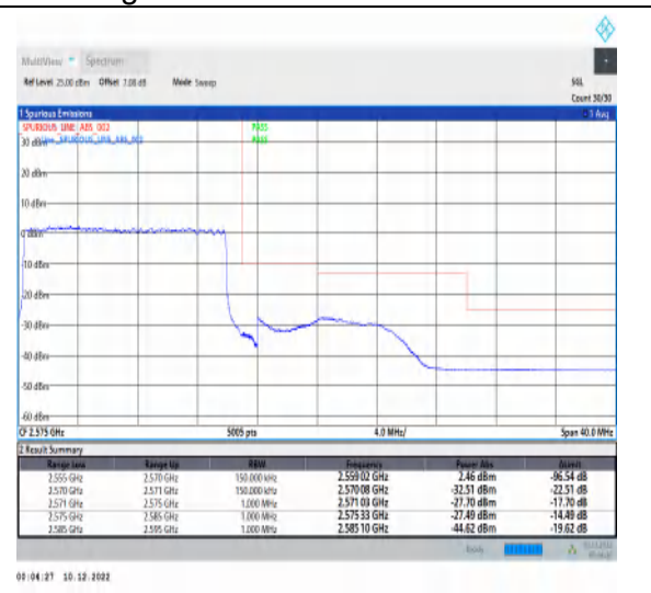
1-N7-15-15-H-3-DFT-PI2BPSK-Outer_Full-75@0-Ant1-1--PASS-see graph
