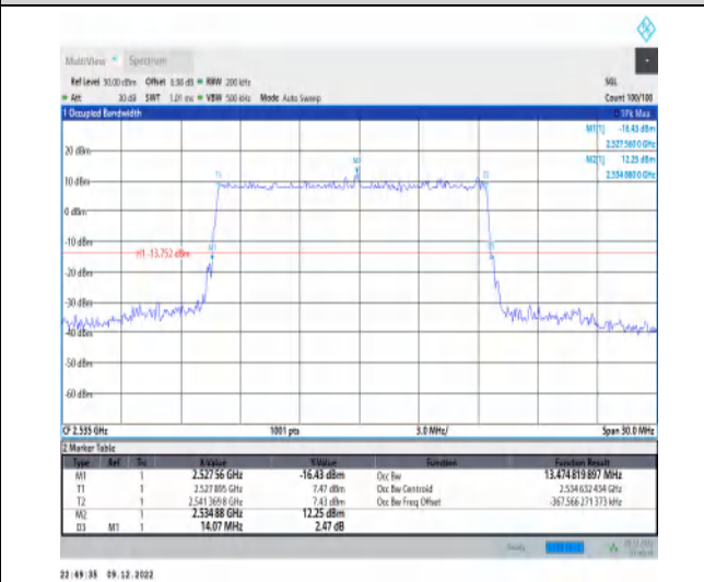
1-N7-15-15-M-5-DFT-256QAM-Outer_Full-75@0-Ant1 1-13.475-14.070-≤15-PASS
