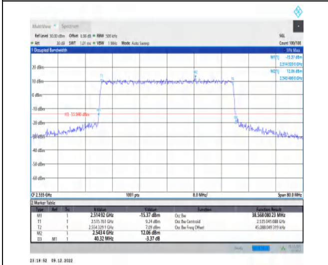
1-N7-15-40-M-8-CP-64QAM-Outer_Full-216@0-Ant1-38.568-40.320-≤40-PASS
