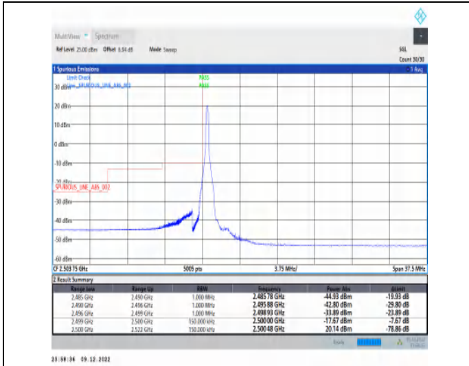
1-N7-15-15-L-1-DFT-PI2BPSK-Edge_1RB_Left-1@0-Ant1-1--PASS-see graph
