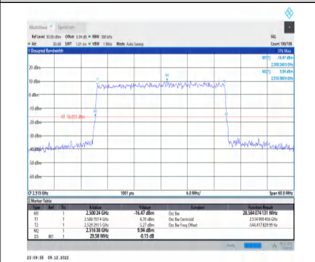
1-N7-15-30-L-5-DFT-256QAM-Outer_Full-160@0-Ant t1-28.584-29.580-≤30-PASS
