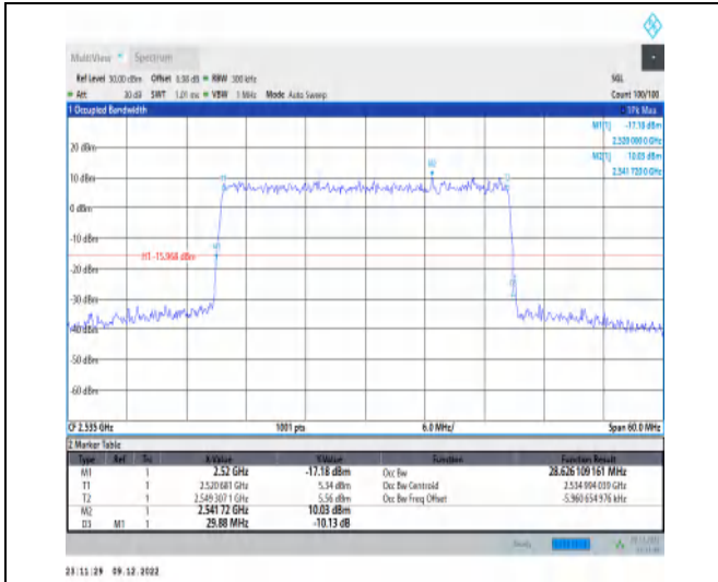
1-N7-15-30-M-5-DFT-256QAM-Outer_Full-160@0-Ant1-28.626-29.880-≤30-PASS
