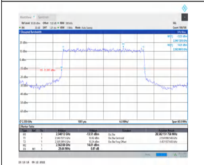
1-N7-15-30-H-2-DFT-PI2BPSK-Outer_Full-160@0-A nt1-28.582-29.640-≤30-PASS
