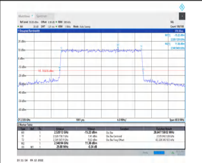
1-N7-15-30-M-4-DFT-64QAM-Outer_Full-160@0-Ant1 1-28.647-29.880-≤30-PASS
