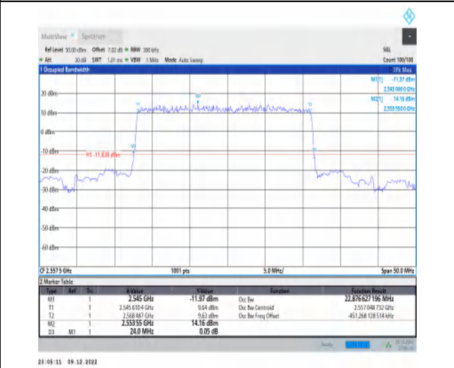
1-N7-15-25-H-2-DFT-PI2BPSK-Outer_Full-128@0-Ant1 -22.877-24.000-≤25-PASS
