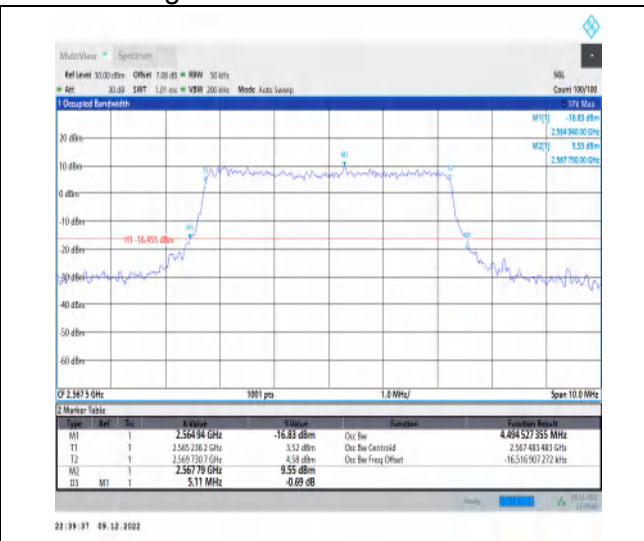
1-N7-15-5-H-8-CP-64QAM-Outer_Full-25@0-Ant1-4. 495-5.110-≤5-PASS
