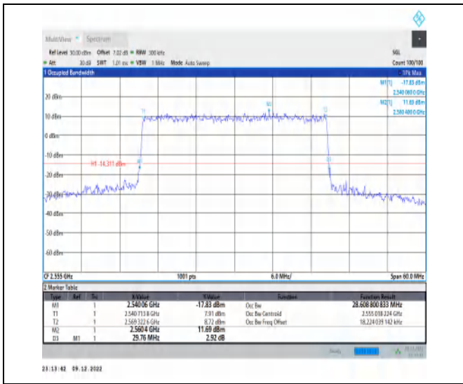
1-N7-15-30-H-4-DFT-64QAM-Outer_Full-160@0-Ant 1-28.609-29.760-≤30-PASS
