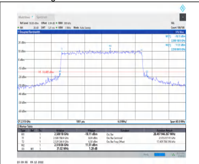
1-N7-15-30-L-7-CP-16QAM-Outer_Full-160@0-Ant1 -28.498-31.020-≤30-PASS
