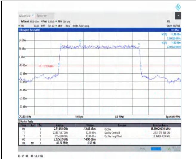
1-N7-15-40-M-2-DFT-PI2BPSK-Outer_Full-216@0-A nt1-38.499-40.240-≤40-PASS
