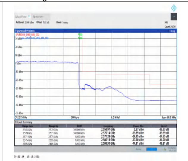
1-N7-15-25-H-3-DFT-PI2BPSK-Outer_Full-128@0-Ant1-1--PASS-see graph
