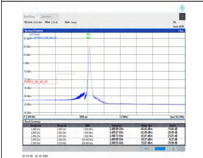
1-N7-15-20-L-4-CP-QPSK-Edge_1RB_Left-1@0-Ant1-1--PASS-see graph
