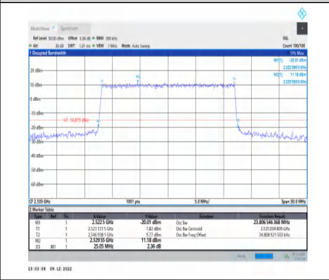
1-N7-15-25-M-7-CP-16QAM-Outer_Full-133@0-Ant1 -23.807-25.050-≤25-PASS
