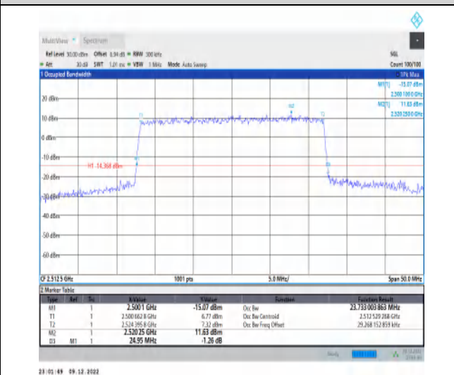
1-N7-15-25-L-8-CP-64QAM-Outer_Full-133@0-Ant1 -23.733-24.950-<25-PASS
