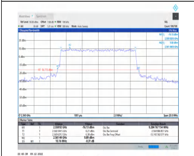
1-N7-15-10-H-6-CP-QPSK-Outer_Full-52@0-Ant1-9. 285-10.160-≤10-PASS
