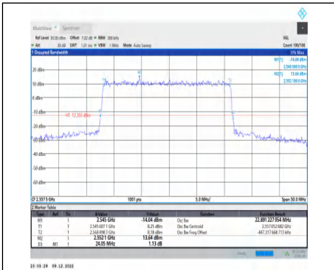
1-N7-15-25-H-3-DFT-16QAM-Outer_Full-128@0-Ant 1-22.891-24.050-≤25-PASS
