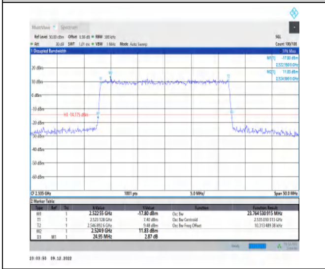
1-N7-15-25-M-6-CP-QPSK-Outer_Full-133@0-Ant1- 23.765-24.950-≤25-PASS
