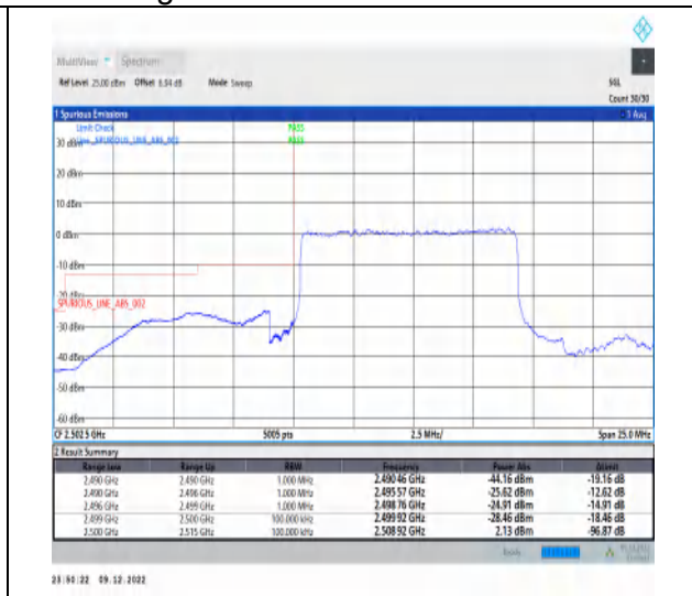
1-N7-15-10-L-3-DFT-PI2BPSK-Outer_Full-50@0-Ant1-1--PASS-see graph
