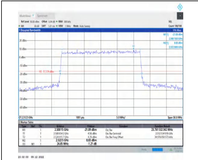
1-N7-15-25-L-9-CP-256QAM-Outer_Full-133@0-Ant 1-23.762-24.850-≤25-PASS
