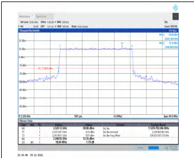
1-N7-15-20-M-3-DFT-16QAM-Outer_Full-100@0-Ant 1-17.877-18.640-≤20-PASS
