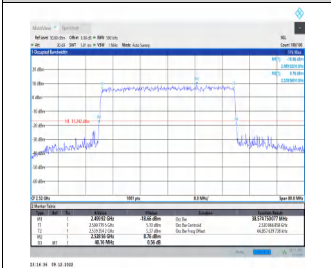
1-N7-15-40-L-9-CP-256QAM-Outer_Full-216@0-Ant 1-38.575-40.160-≤40-PASS
