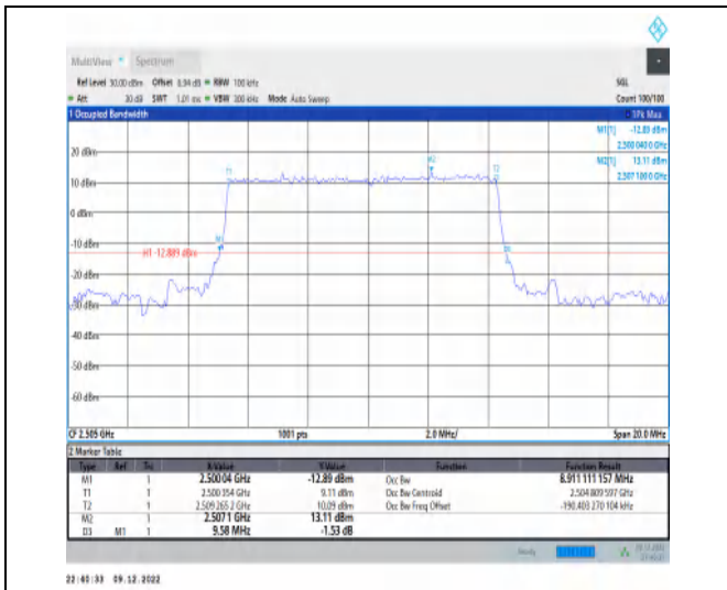
1-N7-15-10-L-2-DFT-PI2BPSK-Outer_Full-50@0-Ant 1-8.911-9.580-≤10-PASS
