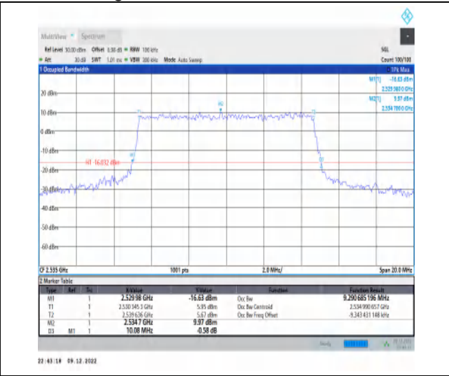
1-N7-15-10-M-6-CP-QPSK-Outer_Full-52@0-Ant1-9. 291-10.080-≤10-PASS
