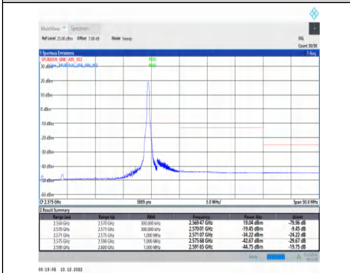
1-N7-15-20-H-5-CP-QPSK-Edge_1RB_Right-1@105-Ant1-1--PASS-see graph
