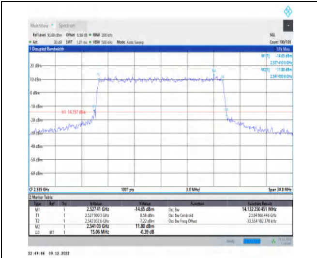
1-N7-15-15-M-6-CP-QPSK-Outer_Full-79@0-Ant1-1 4.132-15.060-≤15-PASS
