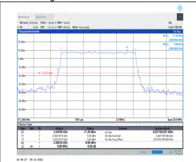
1-N7-15-10-H-5-DFT-256QAM-Outer_Full-50@0-Ant 1-8.927-9.680-≤10-PASS
