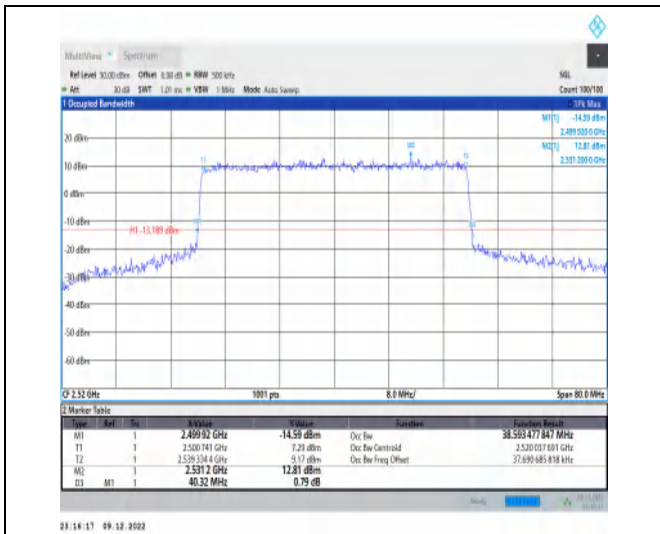
1-N7-15-40-L-7-CP-16QAM-Outer_Full-216@0-Ant1 -38.593-40.320-≤40-PASS
