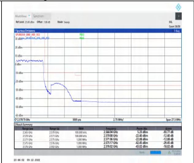
1-N7-15-5-H-3-DFT-PI2BPSK-Outer_Full-25@0-Ant1-1--PASS-see graph
