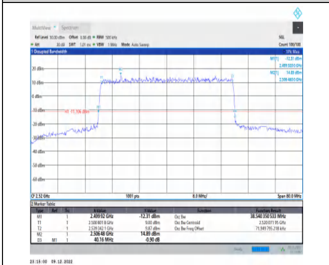
1-N7-15-40-L-1-DFT-QPSK-Outer_Full-216@0-Ant1- 38.54-40.160-≤40-PASS
