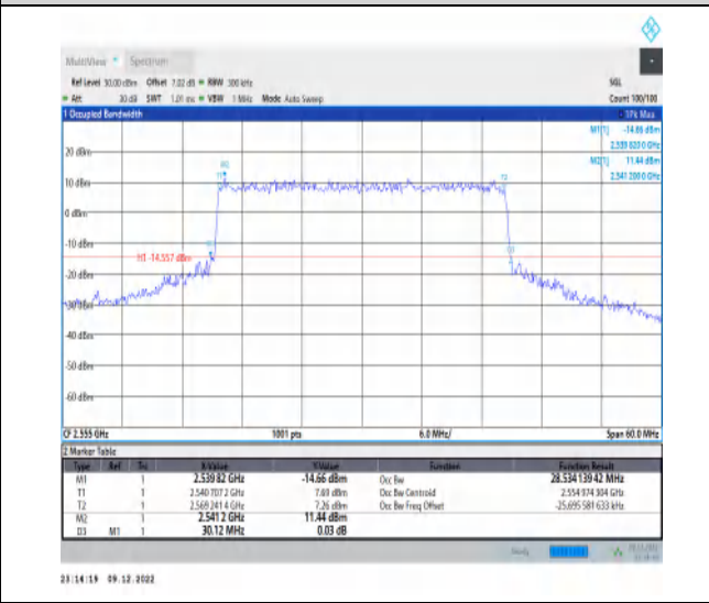
1-N7-15-30-H-7-CP-16QAM-Outer_Full-160@0-Ant1 -28.534-30.120-≤30-PASS
