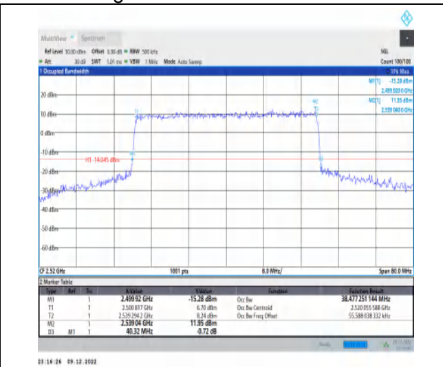
1-N7-15-40-L-8-CP-64QAM-Outer_Full-216@0-Ant1 -38.477-40.320-≤40-PASS
