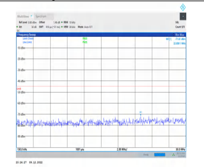
1-N7-15-40-H-1-DFT-PI2BPSK-Inner_1RB_Left-1@ -0.15-30-Ant1-22.03--71.61--45-PASS
