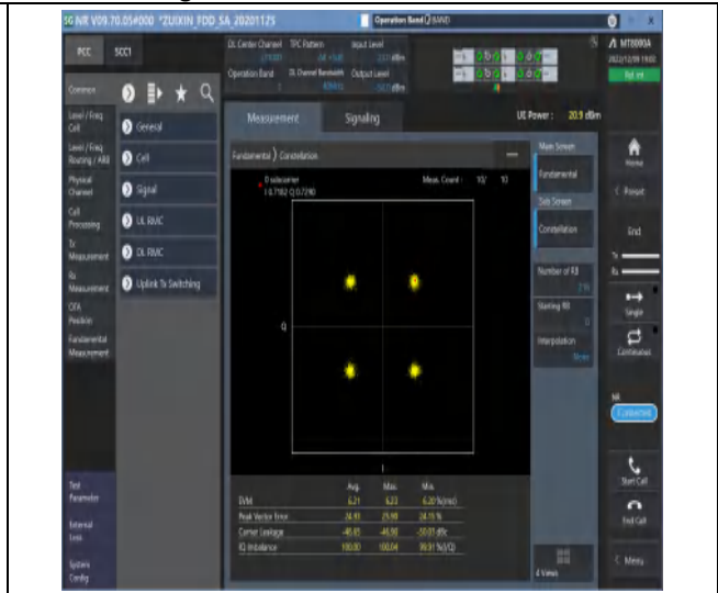
1-N7-15-40-M-6-CP-QPSK-Outer_Full-216@0-Ant1-see graph-PASS
