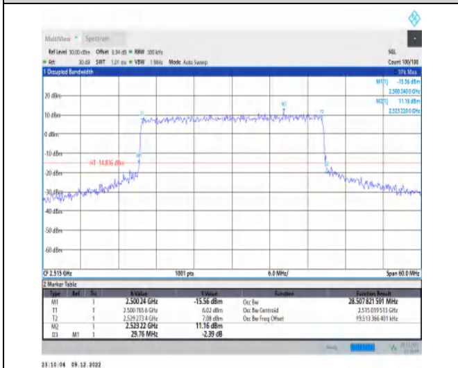
1-N7-15-30-L-8-CP-64QAM-Outer_Full-160@0-Ant1 -28.508-29.760-≤30-PASS
