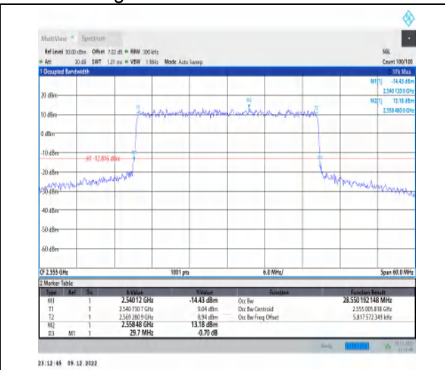
1-N7-15-30-H-1-DFT-QPSK-Outer_Full-160@0-Ant1 -28.55-29.700-≤30-PASS
