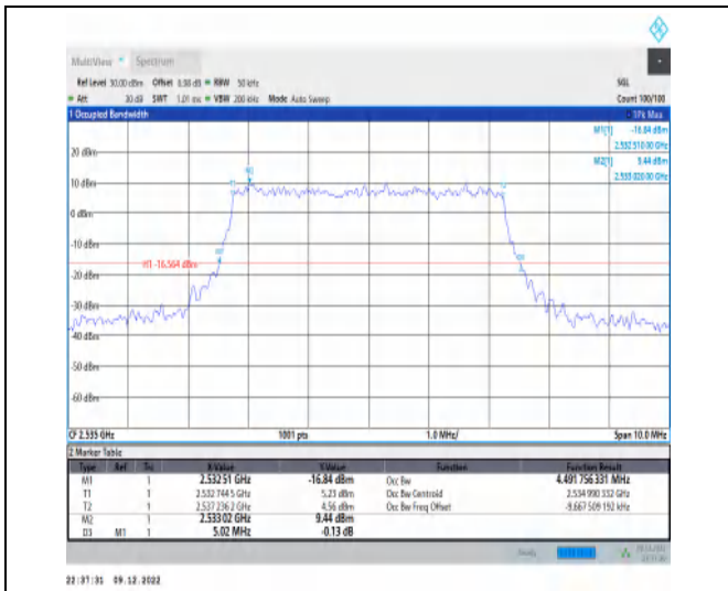
1-N7-15-5-M-8-CP-64QAM-Outer_Full-25@0-Ant1-4 .492-5.020-≤5-PASS
