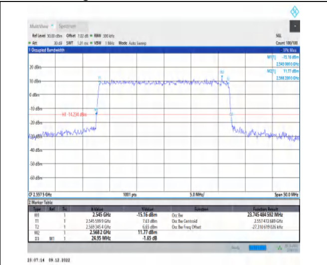
1-N7-15-25-H-8-CP-64QAM-Outer_Full-133@0-Ant1 -23.745-24.950-≤25-PASS
