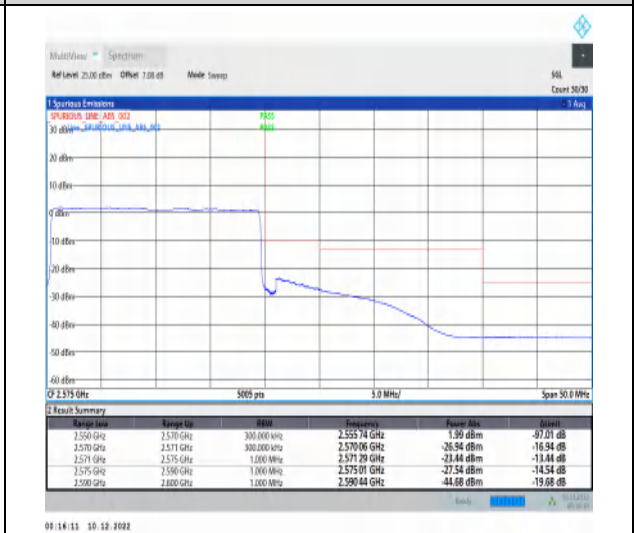
1-N7-15-20-H-6-CP-QPSK-Outer_Full-106@0-Ant1-1--PASS-see graph
