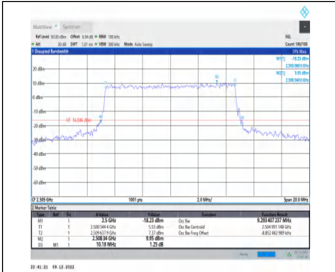
1-N7-15-10-L-6-CP-QPSK-Outer_Full-52@0-Ant1-9. 293-10.180-≤10-PASS
