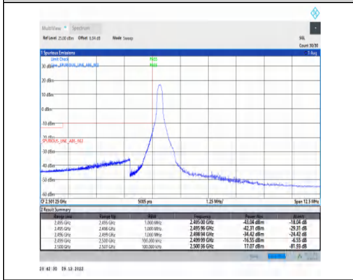
1-N7-15-5-L-4-CP-QPSK-Edge_1RB_Left-1@0-Ant1-1--PASS-see graph
