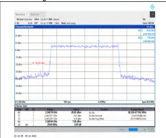
1-N7-15-30-H-9-CP-256QAM-Outer_Full-160@0-Ant1 1-28.526-29.640-≤30-PASS
