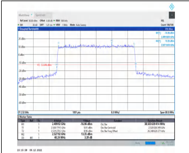
1-N7-15-40-L-3-DFT-16QAM-Outer_Full-216@0-Ant 1-38.504-40.240-≤40-PASS
