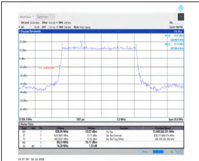
1-N5-15-15-M-2-DFT-P12BPSK-Outer_Full-75@0-An t1-13.449-14.280-≤15-PASS
