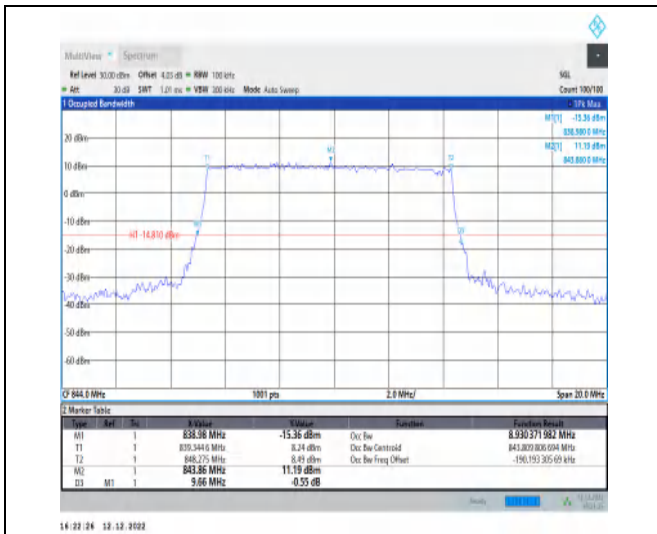
1-N5-15-10-H-4-DFT-64QAM-Outer_Full-50@0-Ant1 -8.93-9.660-≤10-PASS
