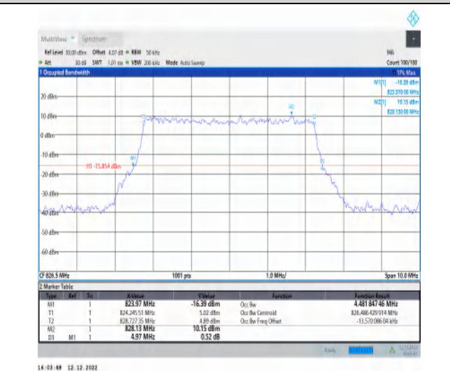
1-N5-15-5-L-8-CP-64QAM-Outer_Full-25@0-Ant1-4. 482-4.970≤5-PASS
