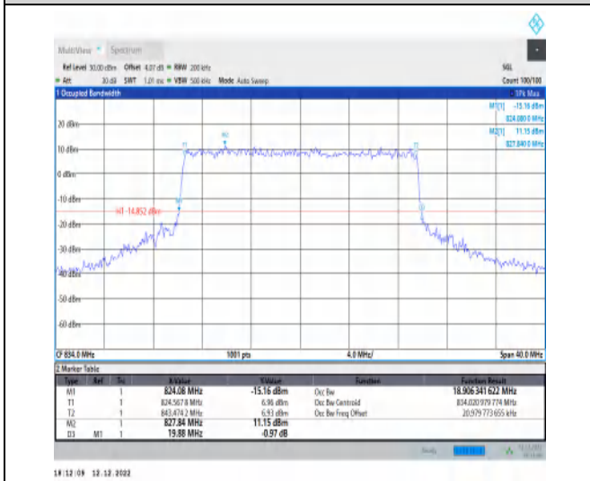
1-N5-15-20-L-6-CP-QPSK-Outer_Full-106@0-Ant1- 18.906-19.880-≤20-PASS
