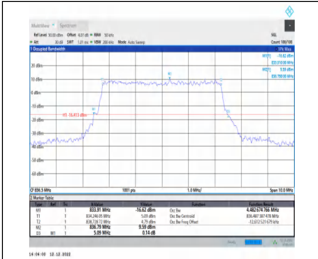
1-N5-15-5-M-8-CP-64QAM-Outer_Full-25@0-Ant1-4 .483-5.090-≤5-PASS
