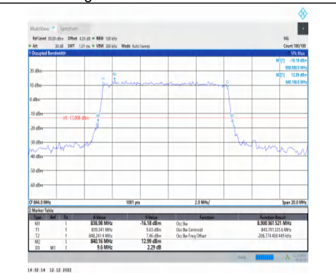
1-N5-15-10-H-1-DFT-QPSK-Outer_Full-50@0-Ant1 8.9-9.600-≤10-PASS
