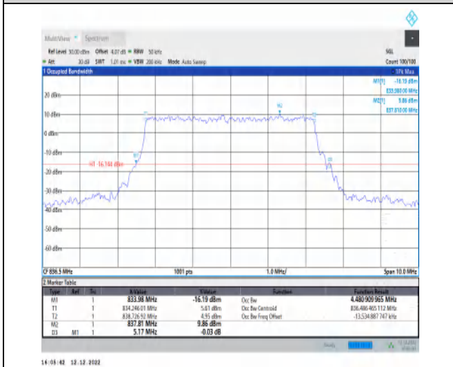
1-N5-15-5-M-6-CP-QPSK-Outer_Full-25@0-Ant1-4.481-5.170-≤5-PASS
