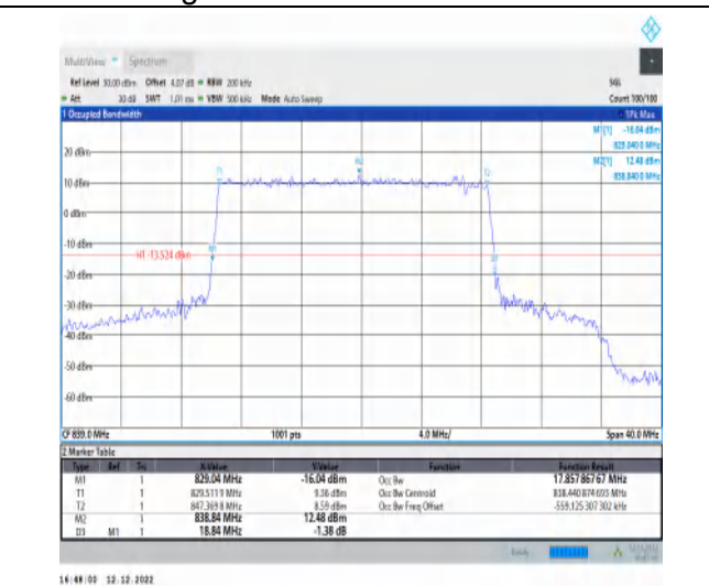
1-N5-15-20-H-3-DFT-16QAM-Outer_Full-100@0-Ant 1-17.858-18.840-≤20-PASS
