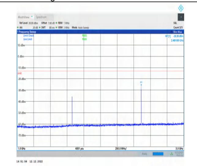
1-N5-15-20-H-1-DFT-PI2BPSK-Inner_1RB_Left-1@1 -1000-3000-Ant1-2489.00--26.38--13-PASS
