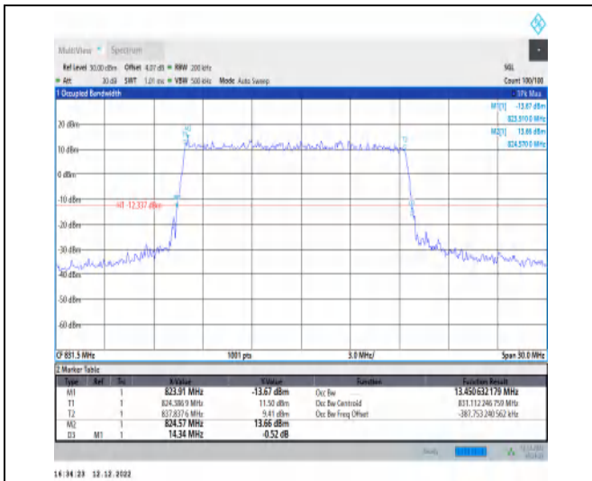
1-N5-15-15-L-3-DFT-16QAM-Outer_Full-75@0-Ant1 -13.451-14.340≤15-PASS
