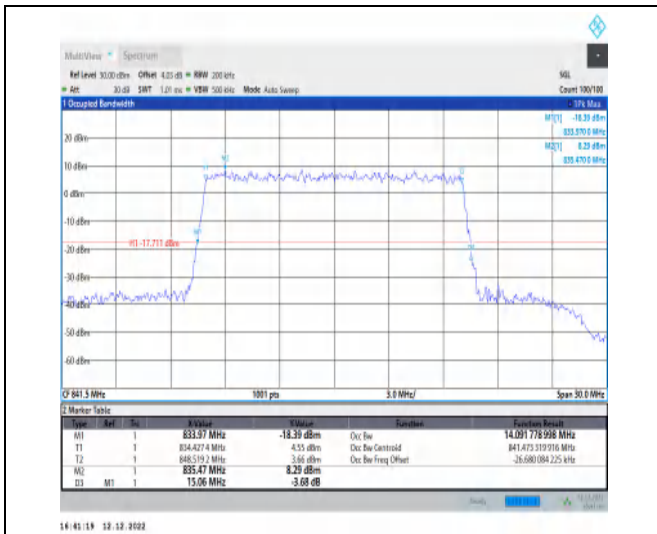
1-N5-15-15-H-9-CP-256QAM-Outer_Full-79@0-Ant1 -14.092-15.060-≤15-PASS
