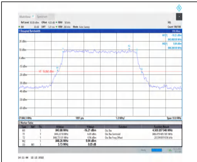
1-N5-15-5-H-7-CP-16QAM-Outer_Full-25@0-Ant1-4. 503-5.150-≤5-PASS
