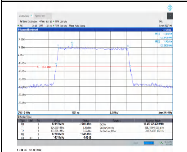
1-N5-15-15-L-5-DFT-256QAM-Outer_Full-75@0-Ant 1-13.438-14.310≤15-PASS
