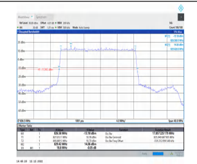
1-N5-15-20-M-2-DFT-PI2BPSK-Outer_Full-100@0-Ant1 1-17.857-18.800-≤20-PASS
