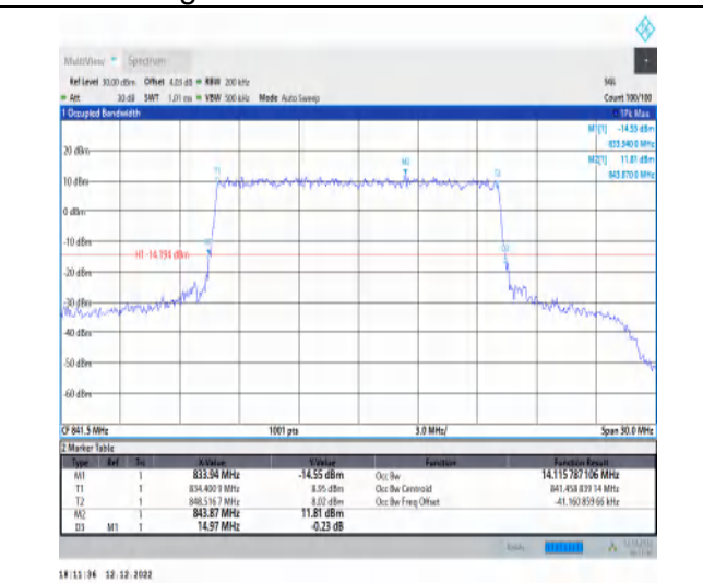
1-N5-15-15-H-6-CP-QPSK-Outer_Full-79@0-Ant1-1 4.116-14.970≤15-PASS
