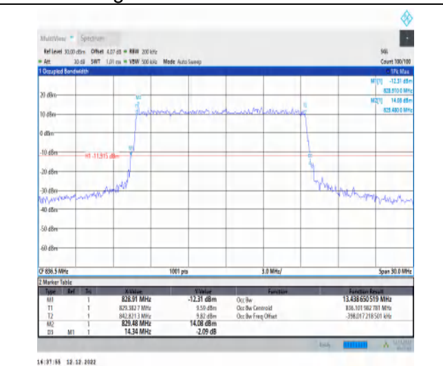
1-N5-15-15-M-3-DFT-16QAM-Outer_Full-75@0-Ant1 -13.439-14.340-≤15-PASS
