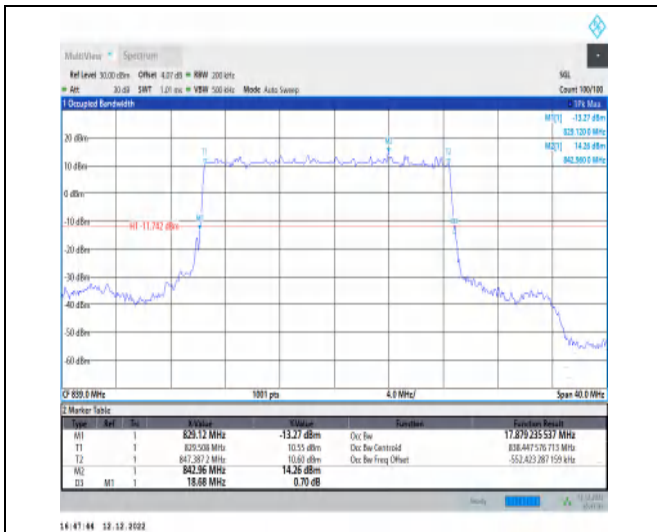
1-N5-15-20-H-2-DFT-PI2BPSK-Outer_Full-100@0-A nt1-17.879-18.680-≤20-PASS
