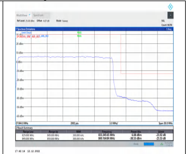
1-N5-15-20-H-3-DFT-PI2BPSK-Outer_Full-100@0-Ant1-1-seegraph-PASS-see graph
