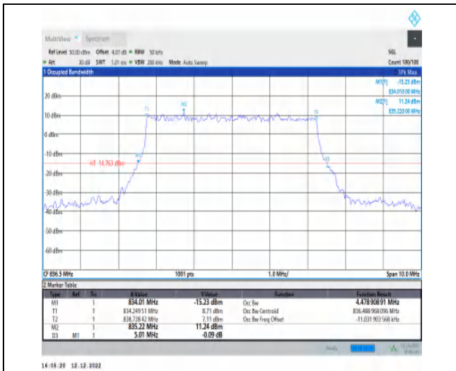
1-N5-15-5-M-4-DFT-64QAM-Outer_Full-25@0-Ant1-4.479-5.010-≤5-PASS
