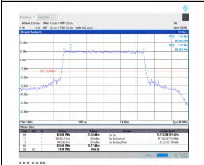
1-N5-15-15-H-7-CP-16QAM-Outer_Full-79@0-Ant1- 14.119-14.940≤15-PASS
