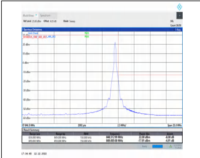
1-N5-15-15-H-2-DFT-PI2BPSK-Edge_1RB_Right-1@78-Ant1-1-seegraph-PASS-see graph
