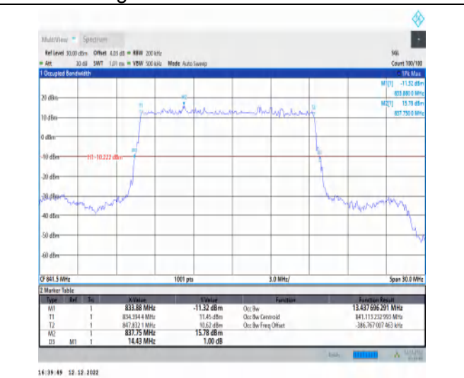
1-N5-15-15-H-2-DFT-PI2BPSK-Outer_Full-75@0-Ant1-13.438-14.430-≤15-PASS
