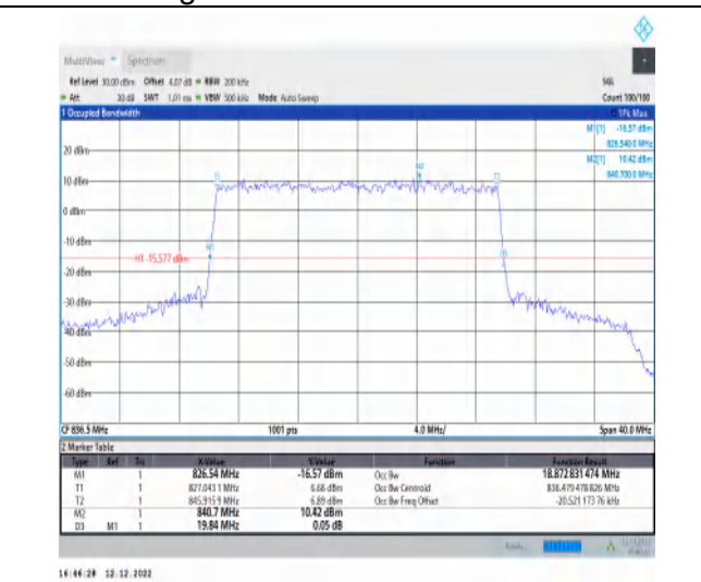
1-N5-15-20-M-8-CP-64QAM-Outer_Full-106@0-Ant1 -18.873-19.840-≤20-PASS
