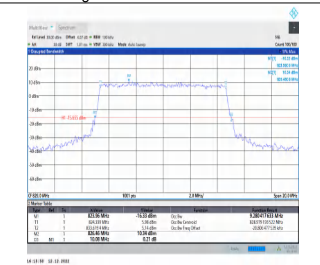
1-N5-15-10-L-7-CP-16QAM-Outer_Full-52@0-Ant1-9. .28-10.080-≤10-PASS
