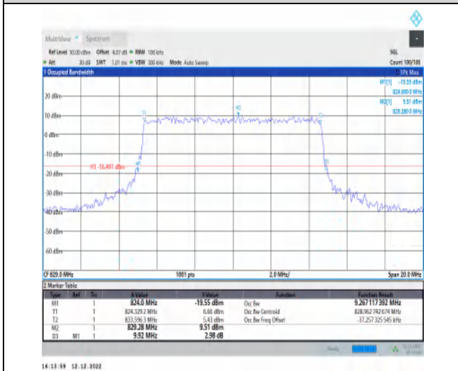
1-N5-15-10-L-8-CP-64QAM-Outer_Full-52@0-Ant1-9. 9.267-9.920-≤10-PASS
