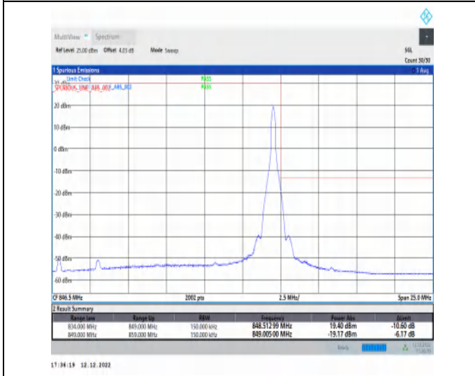
1-N5-15-15-H-5-CP-QPSK-Edge_1RB_Right-1@78-Ant1-1-seegraph-PASS-see graph
