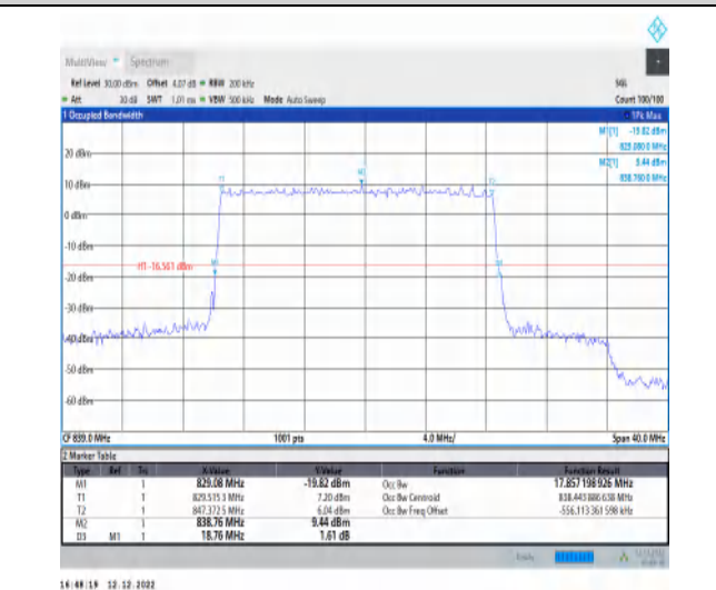
1-N5-15-20-H-5-DFT-256QAM-Outer_Full-100@0-A nt1-17.857-18.760-≤20-PASS
