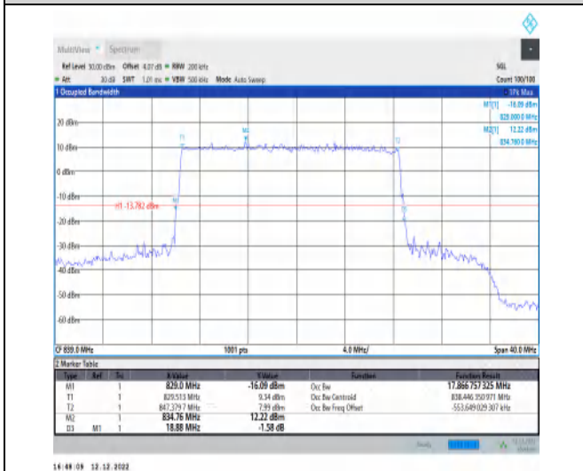
1-N5-15-20-H-4-DFT-64QAM-Outer_Full-100@0-Ant 1-17.867-18.880-≤20-PASS
