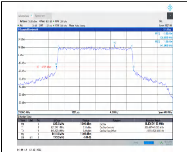
1-N5-15-20-M-7-CP-16QAM-Outer_Full-106@0-Ant 1-18.877-19.920-≤20-PASS
