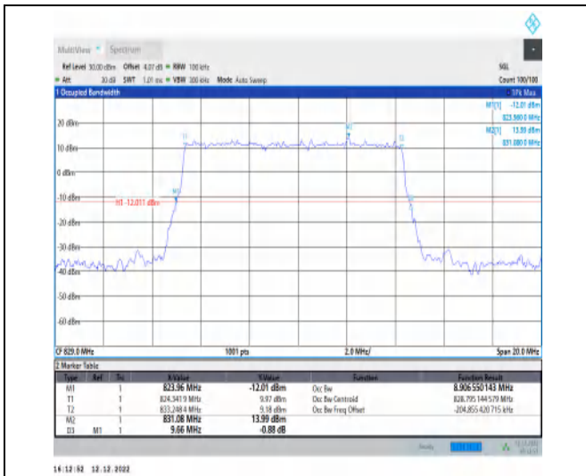
1-N5-15-10-L-2-DFT-PI2BPSK-Outer_Full-50@0-Ant1 1-8.907-9.660≤10-PASS
