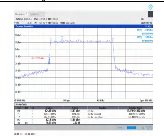
1-N5-15-20-L-1-DFT-QPSK-Outer_Full-100@0-Ant1- 17.879-18.640-≤20-PASS
