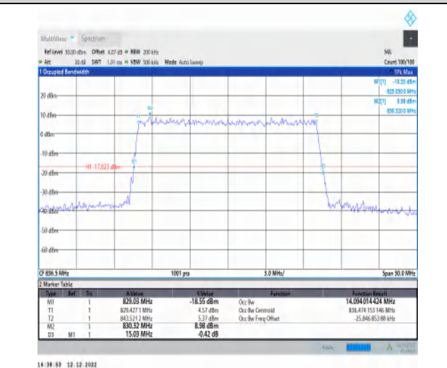
1-N5-15-15-M-9-CP-256QAM-Outer_Full-79@0-Ant1- -14.094-15.030-≤15-PASS
