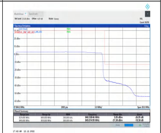
1-N5-15-20-H-6-CP-QPSK-Outer_Full-106@0-Ant1-1-seegraph-PASS-see graph
