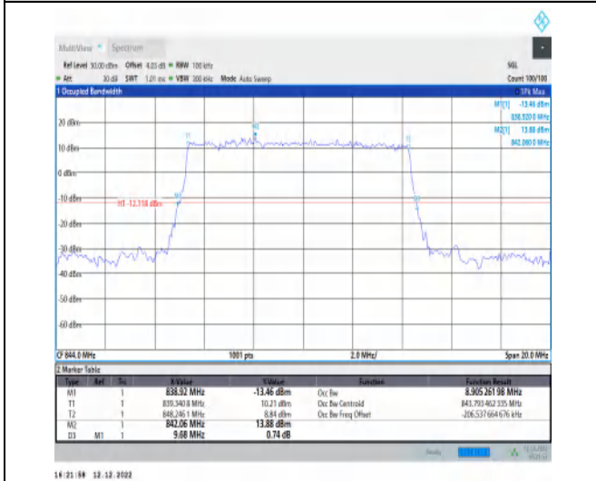
1-N5-15-10-H-2-DFT-P12BPSK-Outer_Full-50@0-An t1-8.905-9.680-≤10-PASS
