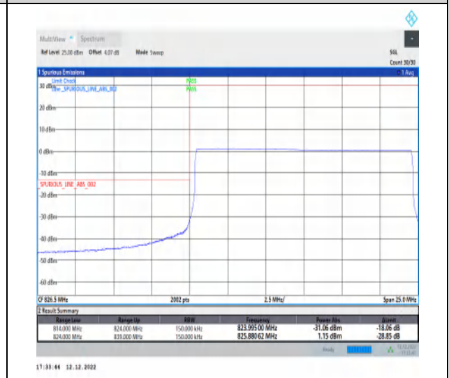
1-N5-15-15-L-6-CP-QPSK-Outer_Full-79@0-Ant1-1-seegraph-PASS-see graph
