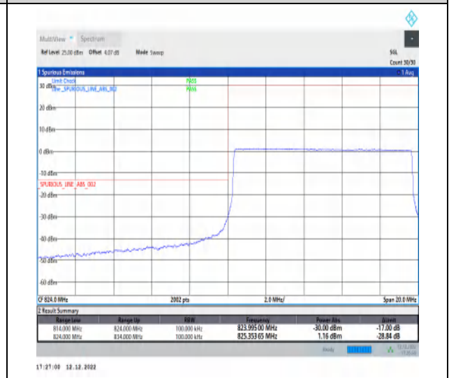
1-N5-15-10-L-6-CP-QPSK-Outer_Full-52@0-Ant1-1-seegraph-PASS-see graph
