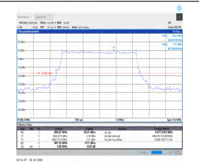
1-N5-15-5-H-6-CP-QPSK-Outer_Full-25@0-Ant1-4.477-5.060-≤5-PASS
