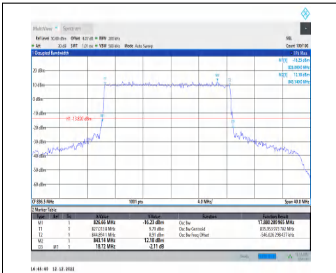
1-N5-15-20-M-3-DFT-16QAM-Outer_Full-100@0-Ant 1-17.88-18.720-≤20-PASS
