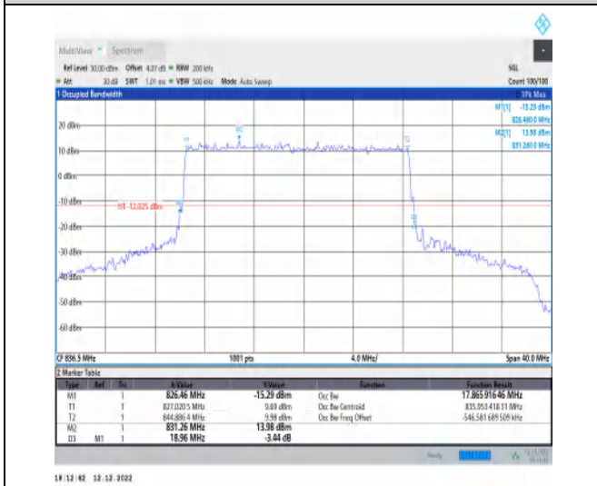
1-N5-15-20-M-1-DFT-QPSK-Outer_Full-100@0-Ant1 -17.866-18.960-≤20-PASS
