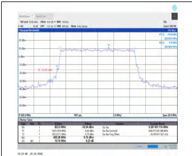
1-N5-15-10-L-6-CP-QPSK-Outer_Full-52@0-Ant1-9. 287-10.160-≤10-PASS
