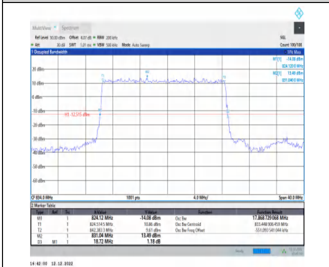
1-N5-15-20-L-2-DFT-PI2BPSK-Outer_Full-100@0-A nt1-17.869-18.720-≤20-PASS
