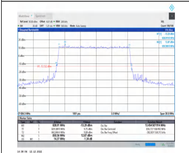
1-N5-15-15-M-4-DFT-64QAM-Outer_Full-75@0-Ant1 -13.455-14.370-≤15-PASS
