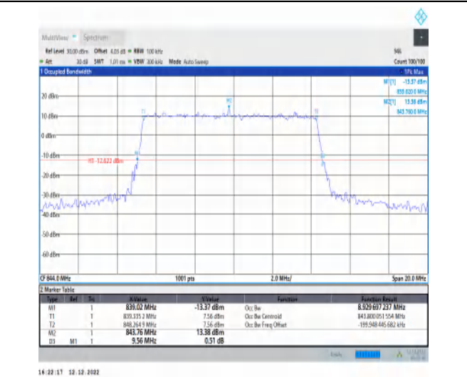
1-N5-15-10-H-3-DFT-16QAM-Outer_Full-50@0-Ant1 -8.93-9.560-≤10-PASS
