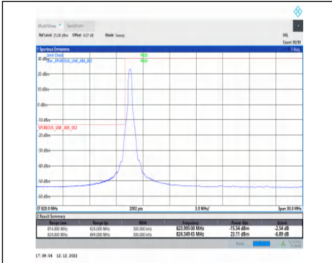
1-N5-15-20-L-1-DFT-PI2BPSK-Edge_1RB_Left-1@0-Ant1-1-seegraph-PASS-see graph
