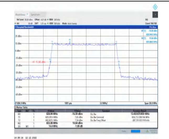
1-N5-15-15-M-5-DFT-256QAM-Outer_Full-75@0-Ant 1-13.434-14.400-≤15-PASS
