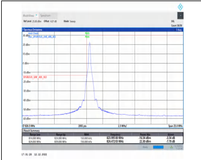
1-N5-15-15-L-1-DFT-PI2BPSK-Edge_1RB_Left-1@0-Ant1-1-seegraph-PASS-see graph
