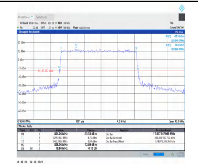
1-N5-15-20-L-3-DFT-16QAM-Outer_Full-100@0-Ant 1-17.847-18.840-≤20-PASS
