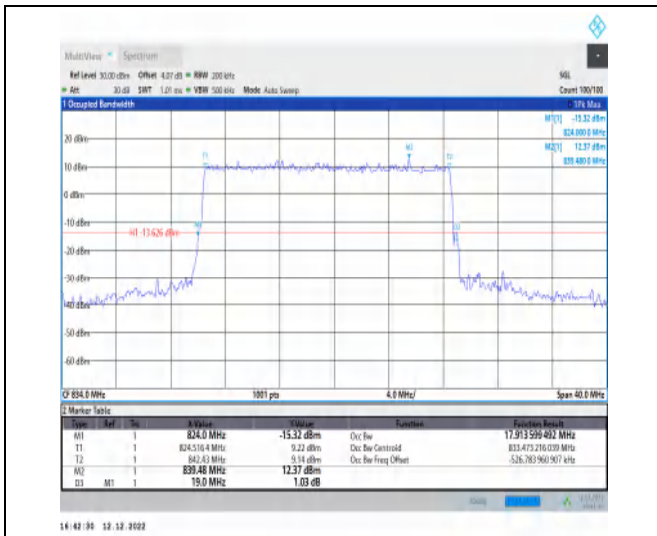
1-N5-15-20-L-4-DFT-64QAM-Outer_Full-100@0-Ant 1-17.914-19.000-≤20-PASS
