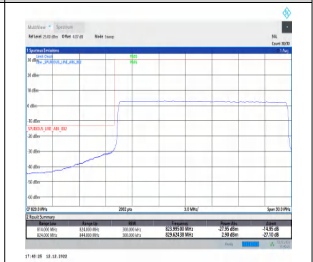
1-N5-15-20-L-6-CP-QPSK-Outer_Full-106@0-Ant1-1-seegraph-PASS-see graph
