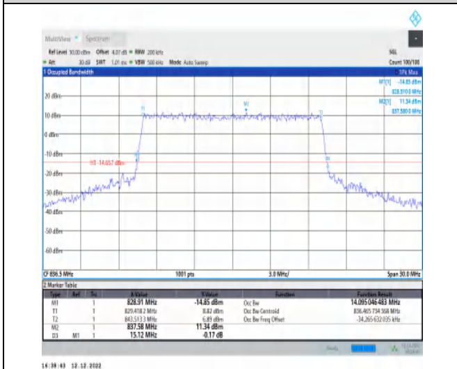
1-N5-15-15-M-8-CP-64QAM-Outer_Full-79@0-Ant1- 14.095-15.120-≤15-PASS
