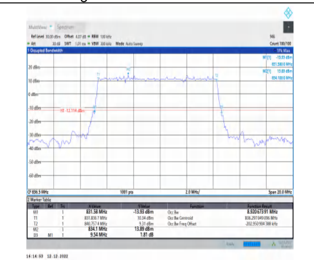
1-N5-15-10-M-2-DFT-PI2BPSK-Outer_Full-50@0-An t1-8.921-9.540-≤10-PASS
