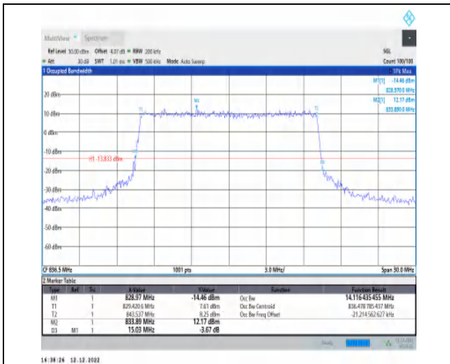
1-N5-15-15-M-6-CP-QPSK-Outer_Full-79@0-Ant1-1 4.116-15.030-≤15-PASS
