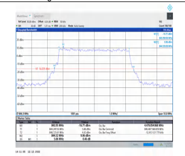
1-N5-15-5-H-8-CP-64QAM-Outer_Full-25@0-Ant1-4. 476-5.060-≤5-PASS
