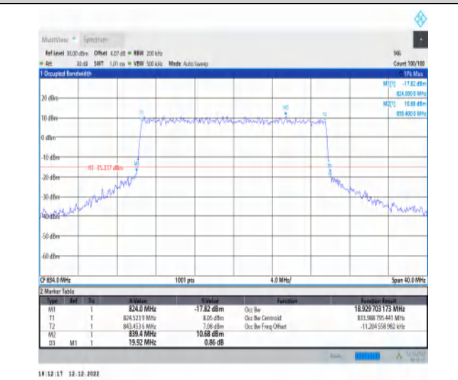
1-N5-15-20-L-7-CP-16QAM-Outer_Full-106@0-Ant1- 18.93-19.920-≤20-PASS
