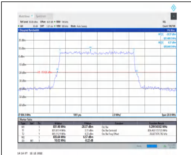
1-N5-15-10-M-9-CP-256QAM-Outer_Full-52@0-Ant 1-9.3-10.020-≤10-PASS
