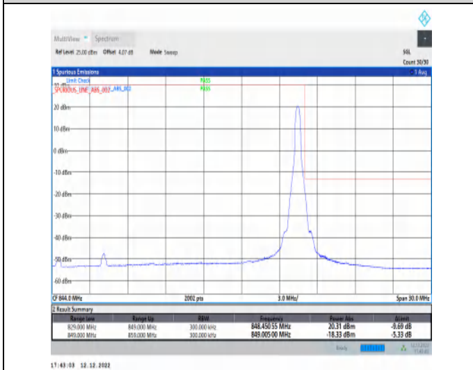
1-N5-15-20-H-5-CP-QPSK-Edge_1RB_Right-1@105-Ant1-1-seegraph-PASS-see graph
