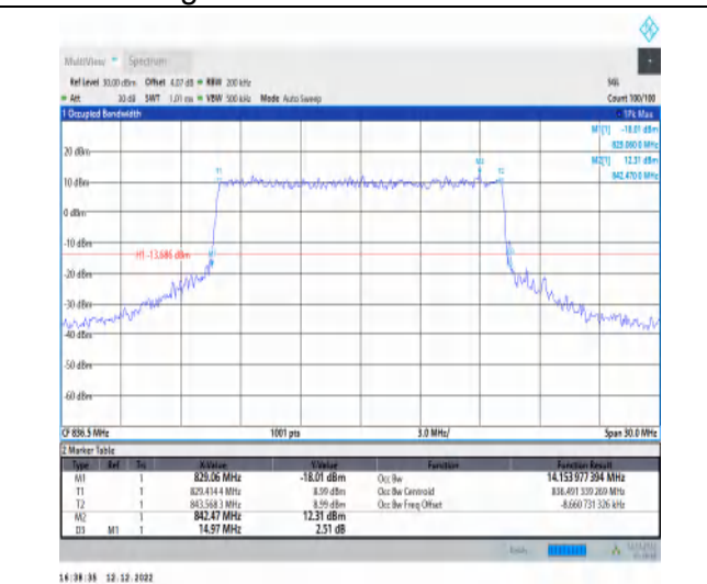
1-N5-15-15-M-7-CP-16QAM-Outer_Full-79@0-Ant1- 14.154-14.970-≤15-PASS
