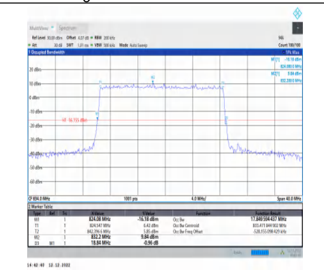
1-N5-15-20-L-5-DFT-256QAM-Outer_Full-100@0-An t1-17.85-18.840-≤20-PASS
