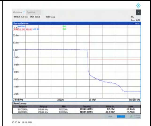
1-N5-15-15-H-6-CP-QPSK-Outer_Full-79@0-Ant1-1-seegraph-PASS-see graph
