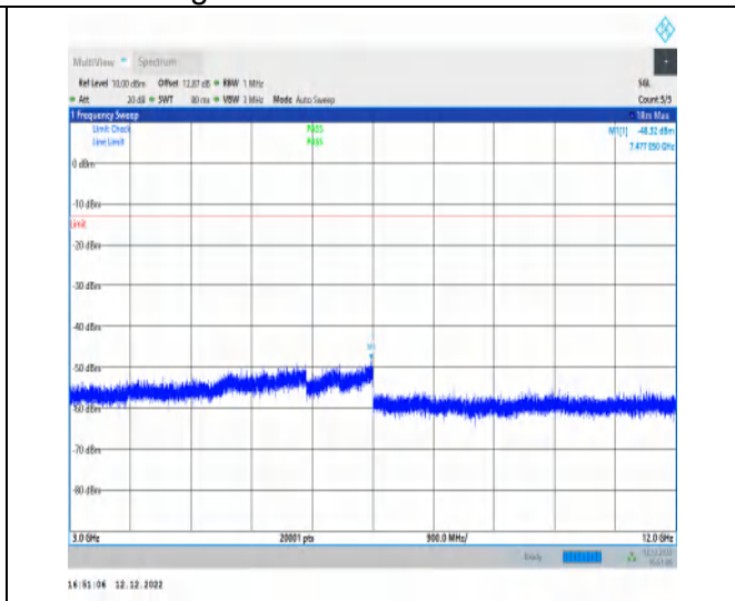
1-N5-15-20-M-1-DFT-PI2BPSK-Inner_1RB_Left-1@ 1-3000-12000-Ant1-7477.05--48.32--13-PASS
