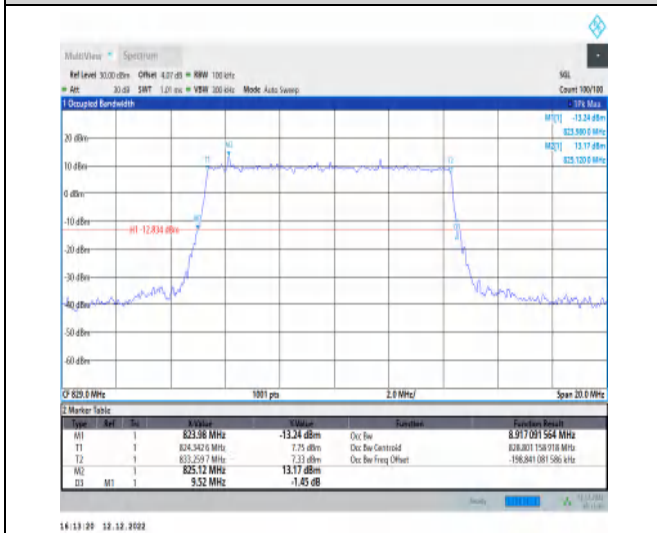
1-N5-15-10-L-4-DFT-64QAM-Outer_Full-50@0-Ant1 -8.917-9.520≤10-PASS
