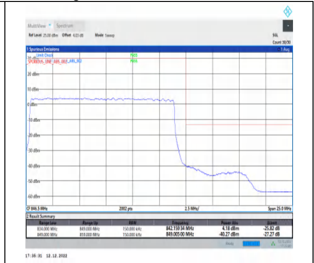
1-N5-15-15-H-3-DFT-PI2BPSK-Outer_Full-75@0-Ant1-1-seegraph-PASS-see graph
