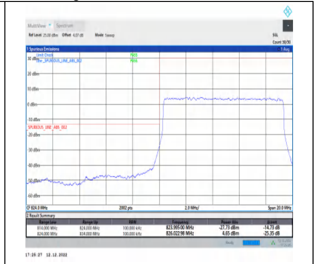
1-N5-15-10-L-3-DFT-PI2BPSK-Outer_Full-50@0-Ant1-1-seegraph-PASS-see graph
