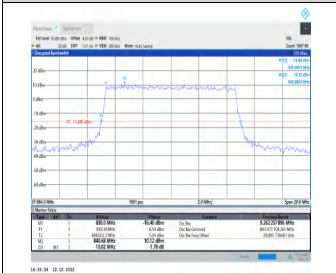
1-N5-15-10-H-6-CP-QPSK-Outer_Full-52@0-Ant1-9. 262-10.020-≤10-PASS
