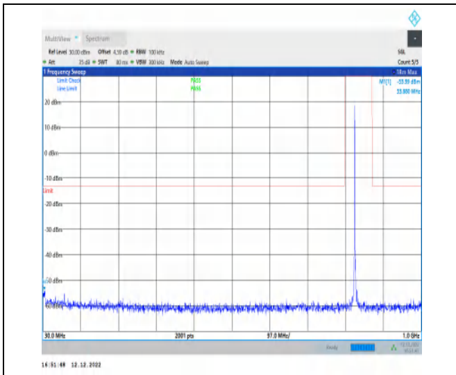
1-N5-15-20-H-1-DFT-PI2BPSK-Inner_1RB_Left-1@1 -30-1000-Ant1-33.88--53.99--13-PASS
