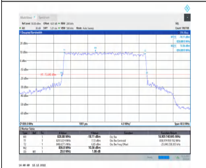
1-N5-15-20-H-8-CP-64QAM-Outer_Full-106@0-Ant1-18.905-20.000-<=20-PASS
