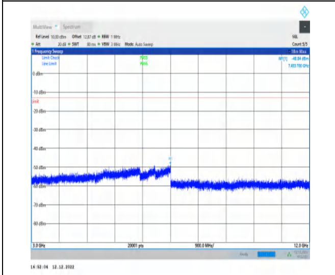
1-N5-15-20-H-1-DFT-PI2BPSK-Inner_1RB_Left-1@1 -3000-12000-Ant1-7493.70--48.84--13-PASS
