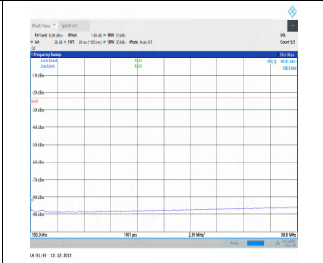
1-N5-15-20-H-1-DFT-PI2BPSK-Inner_1RB_Left-1@1 -0.15-30-Ant1-0.15--85.31--23-PASS
