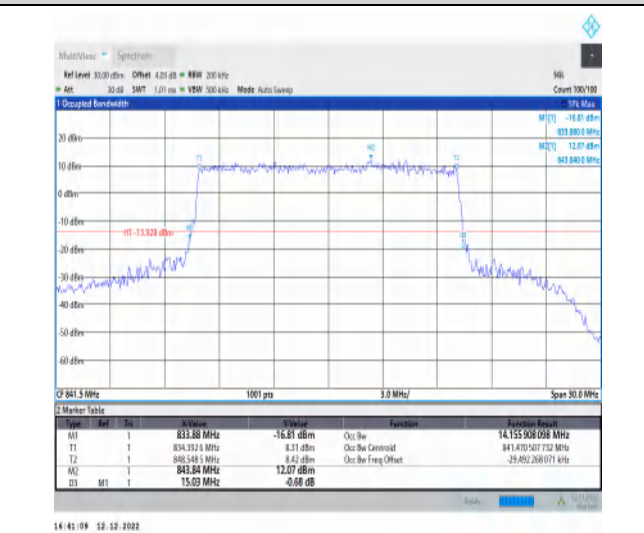
1-N5-15-15-H-8-CP-64QAM-Outer_Full-79@0-Ant1- 14.156-15.030≤15-PASS
