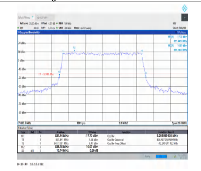
1-N5-15-10-M-6-CP-QPSK-Outer_Full-52@0-Ant1-9. 292-10.140-≤10-PASS
