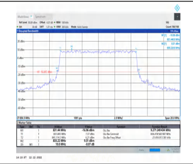
1-N5-15-10-M-8-CP-64QAM-Outer_Full-52@0-Ant1-8 9.271-10.000-≤10-PASS
