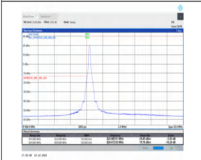
1-N5-15-15-L-4-CP-QPSK-Edge_1RB_Left-1@0-Ant1-1-seegraph-PASS-see graph
