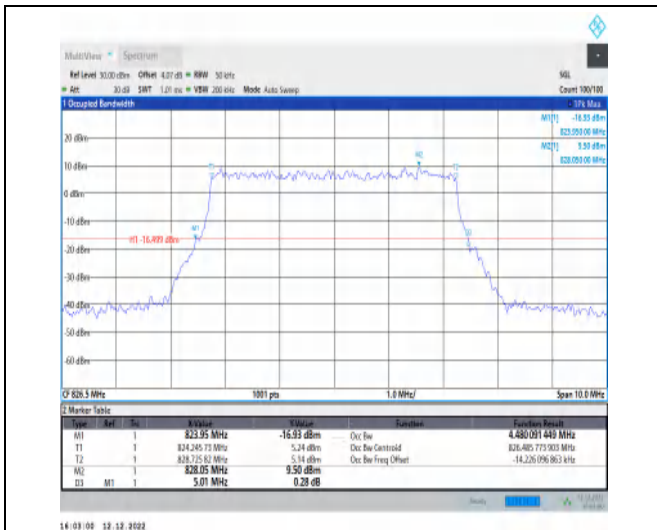
1-N5-15-5-L-5-DFT-256QAM-Outer_Full-25@0-Ant1 -4.48-5.010≤5-PASS
