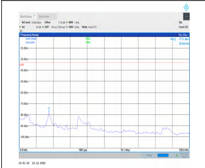
1-N5-15-20-H-1-DFT-PI2BPSK-Inner_1RB_Left-1@1 -0.009-0.15-Ant1-0.03--77.71--33-PASS
