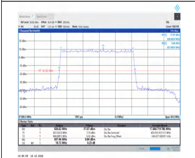
1-N5-15-20-M-5-DFT-256QAM-Outer_Full-100@0-A nt1-17.867-18.720-≤20-PASS
