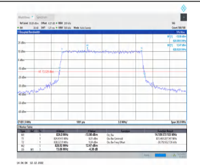
1-N5-15-15-L-6-CP-QPSK-Outer_Full-79@0-Ant1-14 .109-15.060≤15-PASS
