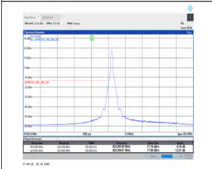
1-N5-15-10-L-4-CP-QPSK-Edge_1RB_Left-1@0-Ant1-1-seegraph-PASS-see graph
