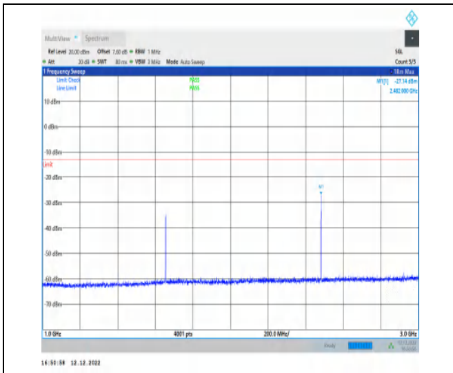
1-N5-15-20-M-1-DFT-PI2BPSK-Inner_1RB_Left-1@ 1-1000-3000-Ant1-2482.00--27.14--13-PASS
