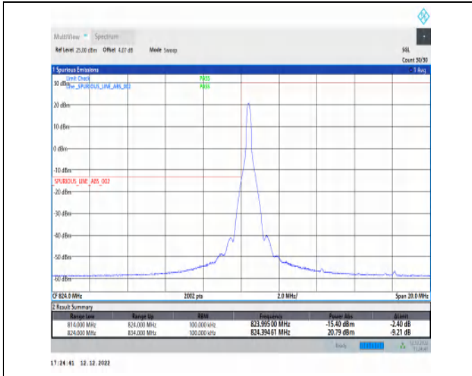
1-N5-15-10-L-1-DFT-PI2BPSK-Edge_1RB_Left-1@0-Ant1-1-seegraph-PASS-see graph
