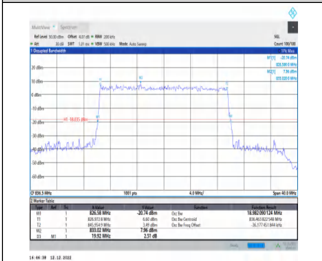
1-N5-15-20-M-9-CP-256QAM-Outer_Full-106@0-An t1-18.982-19.920-≤20-PASS
