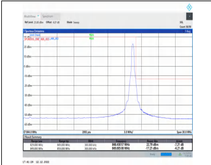
1-N5-15-20-H-2-DFT-PI2BPSK-Edge_1RB_Right-1@105-Ant1-1-seegraph-PASS-see graph
