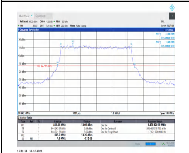
1-N5-15-5-H-1-DFT-QPSK-Outer_Full-25@0-Ant1-4. 478-4.900-≤5-PASS
