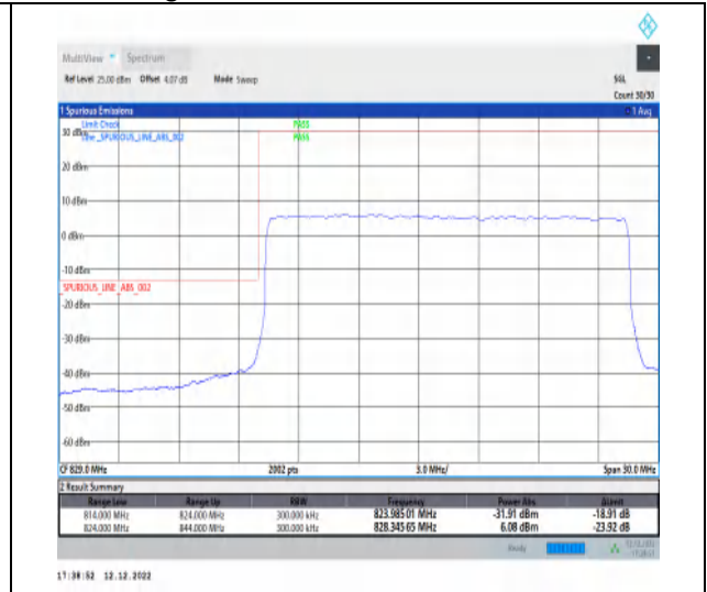
1-N5-15-20-L-3-DFT-PI2BPSK-Outer_Full-100@0-Ant1-1-seegraph-PASS-see graph
