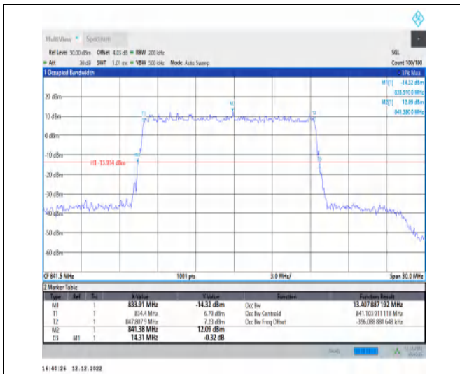
1-N5-15-15-H-5-DFT-256QAM-Outer_Full-75@0-Ant 1-13.408-14.310≤15-PASS
