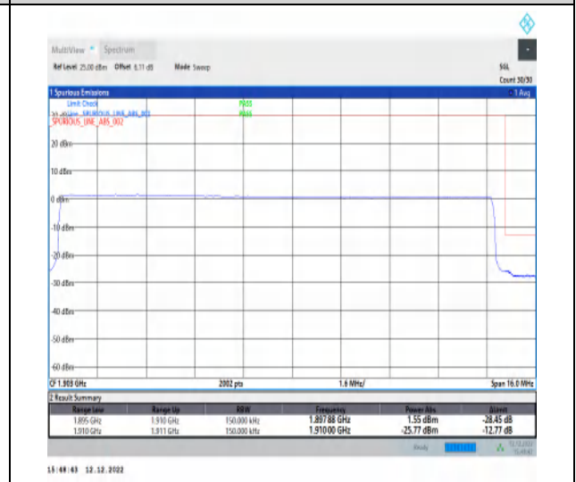
1-N2-PC3-15-15-H-6-CP-QPSK-Outer_Full-79@0-Ant1-1-seegraph-PASS-see graph
