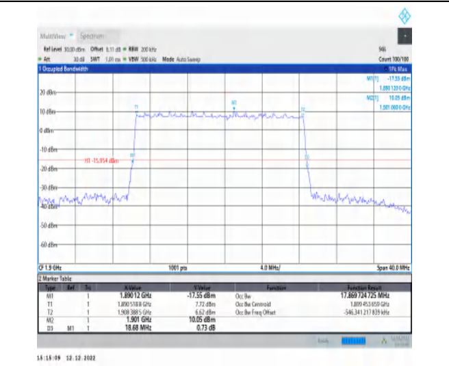
1-N2-PC3-15-20-H-5-DFT-256QAM-Outer_Full-100 @0-Ant1-17.87-18.680-≤20-PASS
