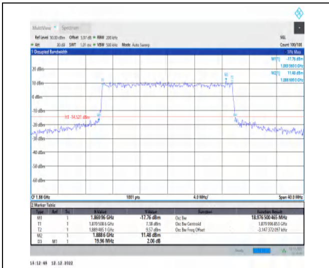
1-N2-PC3-15-20-M-7-CP-16QAM-Outer_Full-106@0 -Ant1-18.977-19.960-≤20-PASS
