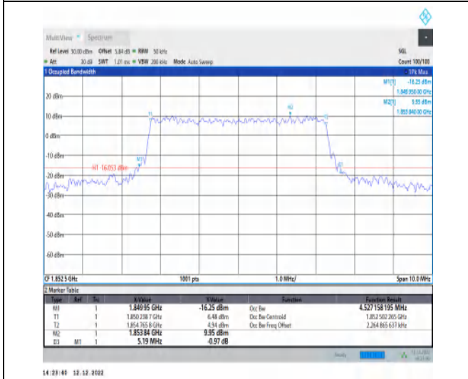
1-N2-PC3-15-5-L-7-CP-16QAM-Outer_Full-25@0-Ant1-4.527-5.190-≤5-PASS
