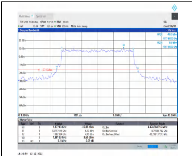
1-N2-PC3-15-5-M-8-CP-64QAM-Outer_Full-25@0-A nt1-4.475-5.100-≤5-PASS
