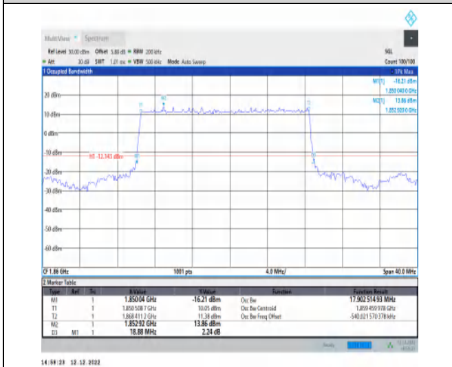
1-N2-PC3-15-20-L-2-DFT-PI2BPSK-Outer_Full-100 @0-Ant1-17.903-18.880-≤20-PASS
