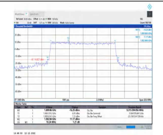
1-N2-PC3-15-10-H-7-CP-16QAM-Outer_Full-52@0- Ant1-9.315-10.240-≤10-PASS
