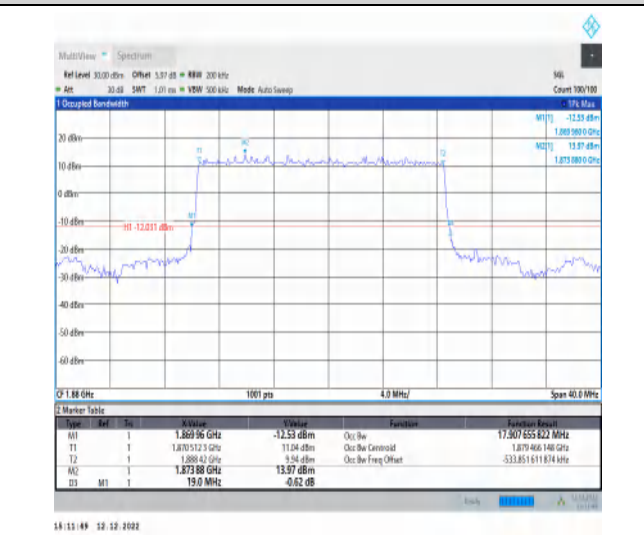
1-N2-PC3-15-20-M-2-DFT-PI2BPSK-Outer_Full-100@0-Ant1-17.908-19.000-≤20-PASS
