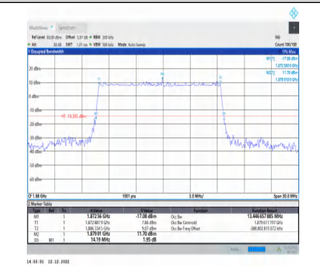
1-N2-PC3-15-15-M-5-DFT-256QAM-Outer_Full-75@0-Ant1-13.447-14.190-≤15-PASS
