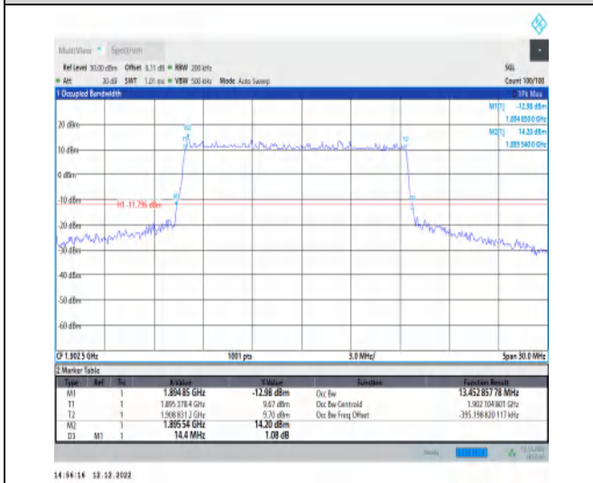
1-N2-PC3-15-15-H-3-DFT-16QAM-Outer_Full-75@0-Ant1-13.453-14.400-≤15-PASS
