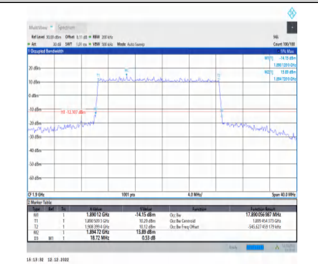
1-N2-PC3-15-20-H-1-DFT-QPSK-Outer_Full-100@0- Ant1-17.89-18.720-≤20-PASS
