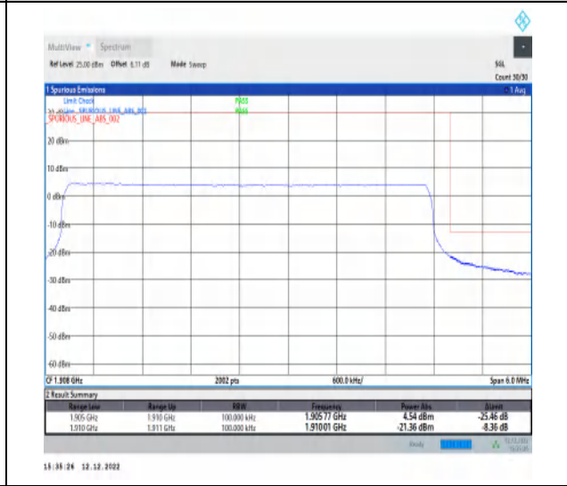
1-N2-PC3-15-5-H-6-CP-QPSK-Outer_Full-25@0-A nt1-1-seegraph-PASS-see graph
