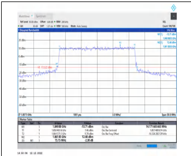
1-N2-PC3-15-15-L-7-CP-16QAM-Outer_Full-79@0-Ant1-14.172-15.150-≤15-PASS
