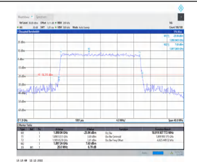
1-N2-PC3-15-20-H-9-CP-256QAM-Outer_Full-106@0-Ant1-18.919-20.000-≤20-PASS
