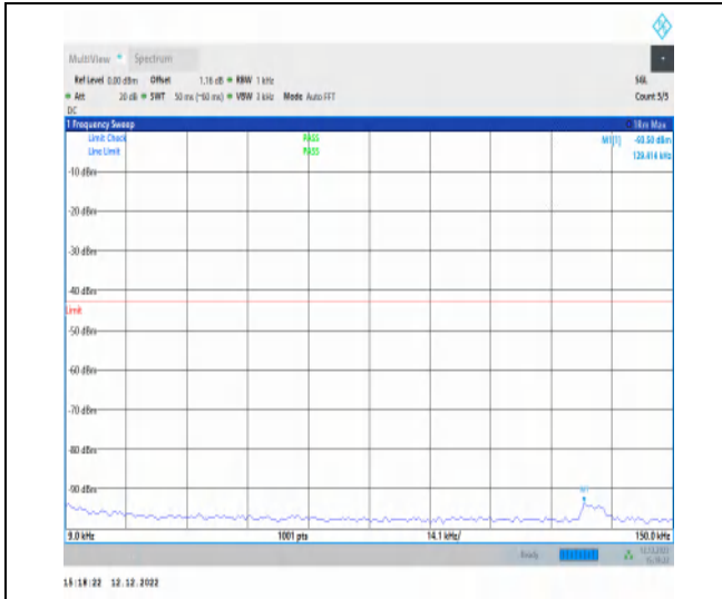
1-N2-PC3-15-20-H-1-DFT-PI2BPSK-Inner_1RB_Lef t-1@1-0.009-0.15-Ant1-0.13--93.50--43-PASS
