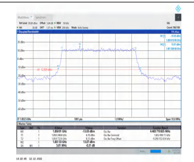
1-N2-PC3-15-5-L-2-DFT-PI2BPSK-Outer_Full-25@0 -Ant1-4.484-5.010-≤5-PASS
