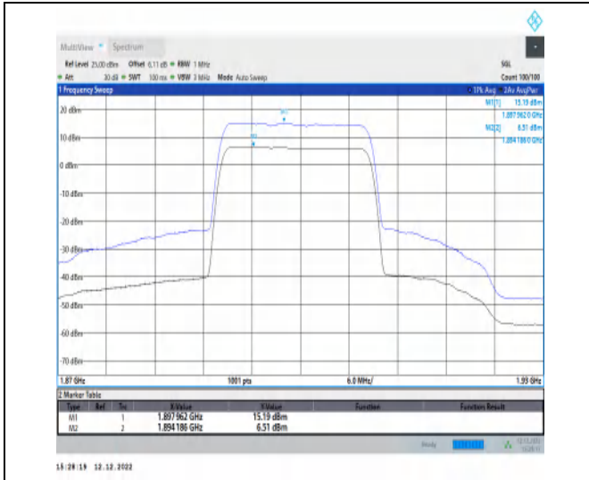
1-N2-PC3-15-20-H-1-DFT-256QAM-Outer_Full-100 @0-Ant1-8.68-100%-0.00-8.68-PASS-≤13
