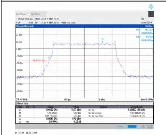
1-N2-PC3-15-5-H-5-DFT-256QAM-Outer_Full-25@0-Ant1-4.489-5.030-≤5-PASS
