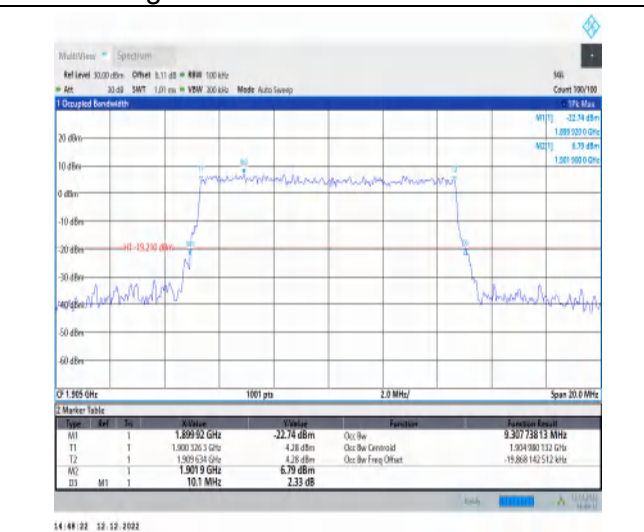
1-N2-PC3-15-10-H-9-CP-256QAM-Outer_Full-52@0-Ant1-9.308-10.100-≤10-PASS
