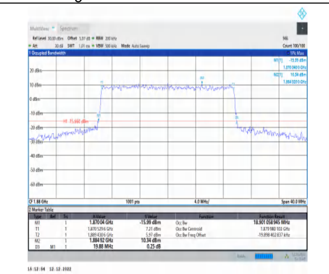
1-N2-PC3-15-20-M-8-CP-64QAM-Outer_Full-106@0 -Ant1-18.901-19.880-≤20-PASS
