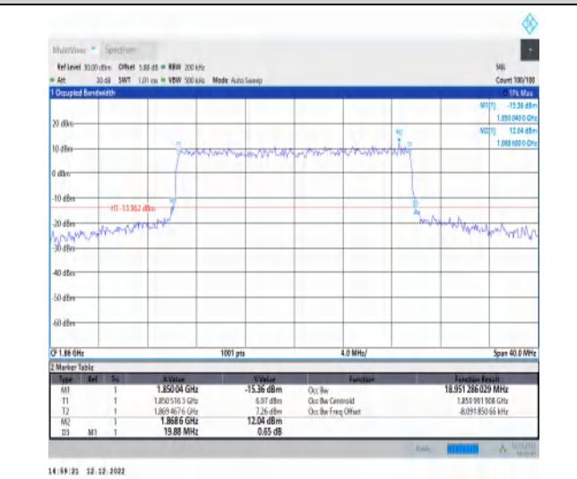
1-N2-PC3-15-20-L-7-CP-16QAM-Outer_Full-106@0- Ant1-18.951-19.880-≤20-PASS
