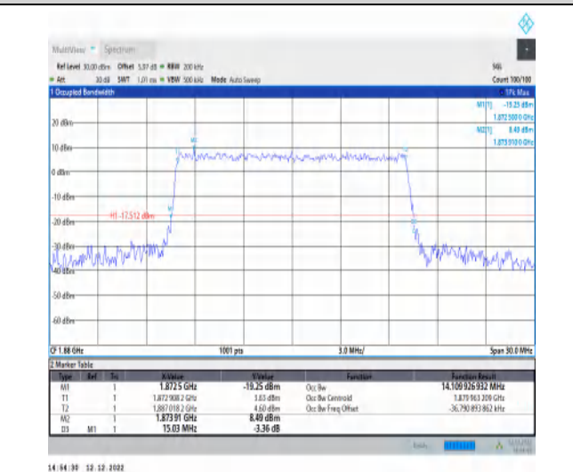
1-N2-PC3-15-15-M-9-CP-256QAM-Outer_Full-79@0- -Ant1-14.11-15.030-≤15-PASS
