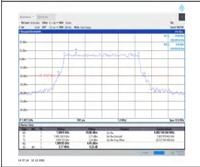
1-N2-PC3-15-5-H-9-CP-256QAM-Outer_Full-25@0-A Ant1-4.485-5.170-≤5-PASS
