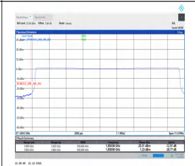
1-N2-PC3-15-10-L-6-CP-QPSK-Outer_Full-52@0-Ant1-1-seegraph-PASS-see graph
