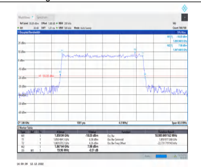
1-N2-PC3-15-20-L-9-CP-256QAM-Outer_Full-106@0-Ant1-18.986-19.960-≤20-PASS
