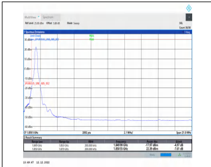
1-N2-PC3-15-20-L-1-DFT-PI2BPSK-Edge_1RB_Left-1@0-Ant1-1-seegraph-PASS-see graph
