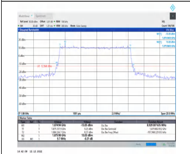
1-N2-PC3-15-10-M-3-DFT-16QAM-Outer_Full-50@0-Ant1-8.929-9.700-≤10-PASS
