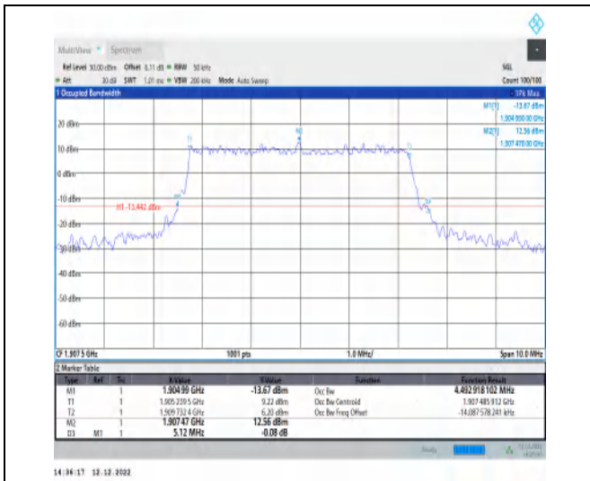
1-N2-PC3-15-5-H-3-DFT-16QAM-Outer_Full-25@0-Ant1-4.493-5.120-≤5-PASS
