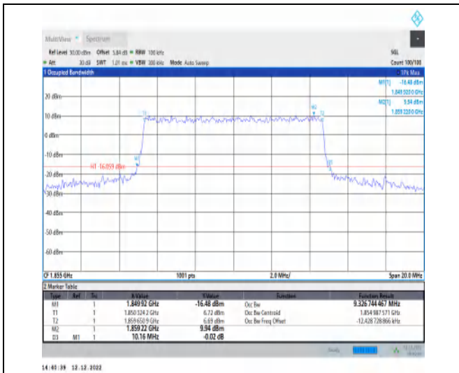
1-N2-PC3-15-10-L-6-CP-QPSK-Outer_Full-52@0-A nt1-9.327-10.160-≤10-PASS
