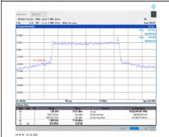
1-N2-PC3-15-20-L-6-CP-QPSK-Outer_Full-106@0- Ant1-18.923-20.000-≤20-PASS
