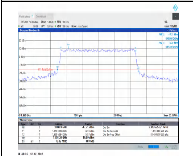
1-N2-PC3-15-10-L-8-CP-64QAM-Outer_Full-52@0-A Ant1-9.304-10.120-≤10-PASS
