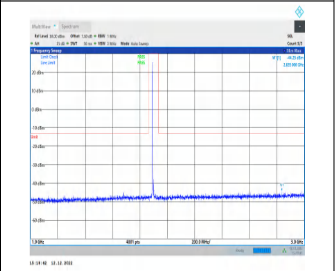
1-N2-PC3-15-20-H-1-DFT-PI2BPSK-Inner_1RB_Left- 1@1-1000-3000-Ant1-2835.00--44.25--13-PASS
