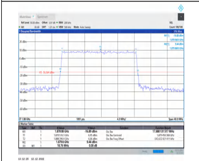
1-N2-PC3-15-20-M-5-DFT-256QAM-Outer_Full-100@0-Ant1-17.88-18.760-≤20-PASS
