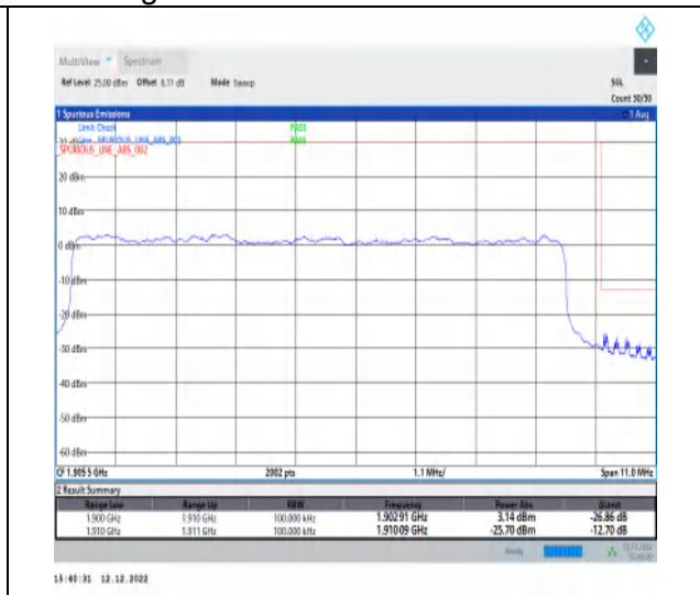
1-N2-PC3-15-10-H-3-DFT-PI2BPSK-Outer_Full-50@0-Ant1-1-seegraph-PASS-see graph
