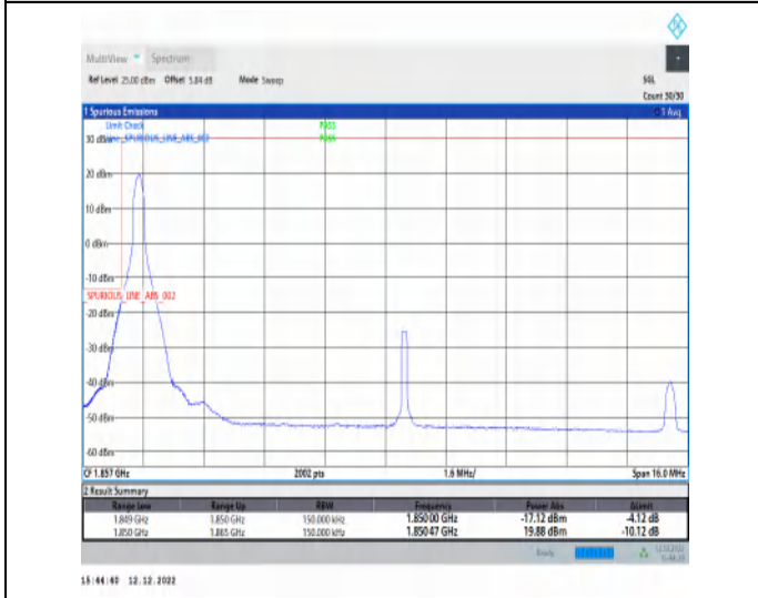
1-N2-PC3-15-15-L-4-CP-QPSK-Edge_1RB_Left-1@0-Ant1-1-seegraph-PASS-see graph
