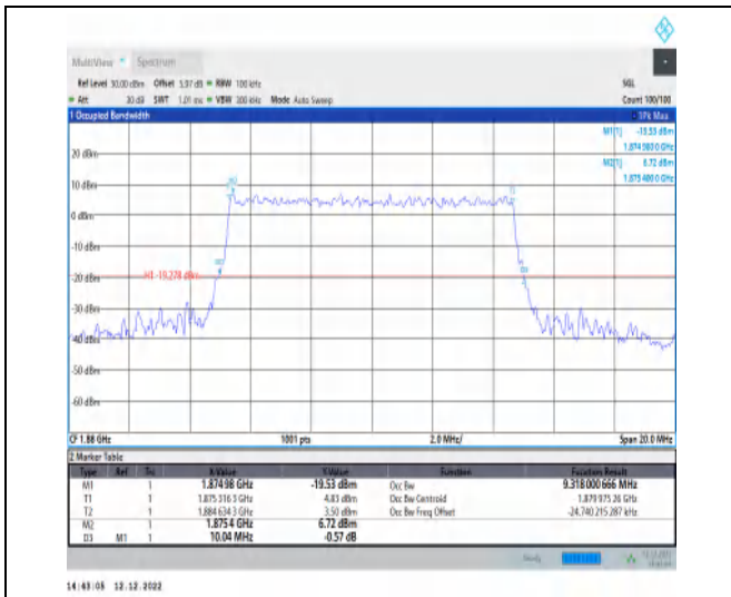
1-N2-PC3-15-10-M-9-CP-256QAM-Outer_Full-52@0 -Ant1-9.318-10.040-≤10-PASS
