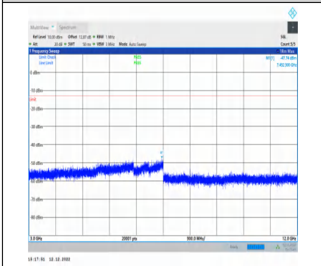
1-N2-PC3-15-20-M-1-DFT-PI2BPSK-Inner_1RB_Lef t-1@1-3000-12000-Ant1-7452.30--47.74--13-PASS
