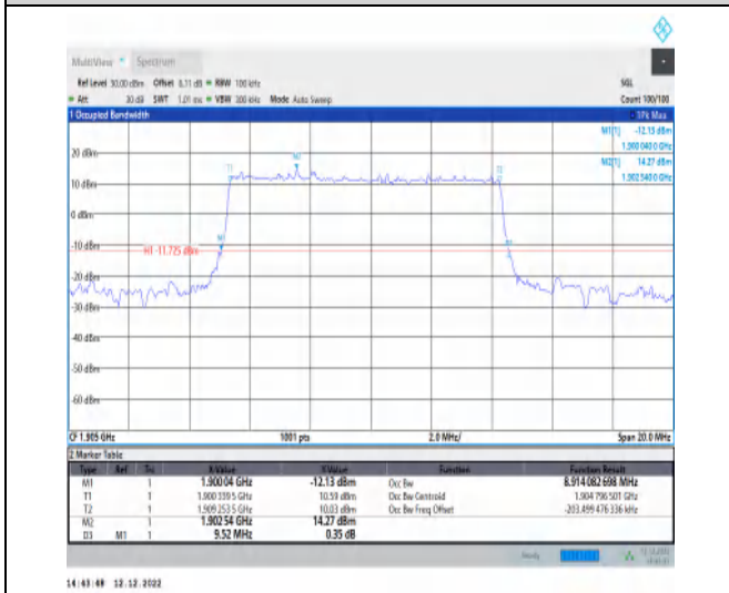
1-N2-PC3-15-10-H-2-DFT-PI2BPSK-Outer_Full-50@0- Ant1-8.914-9.520-≤10-PASS
