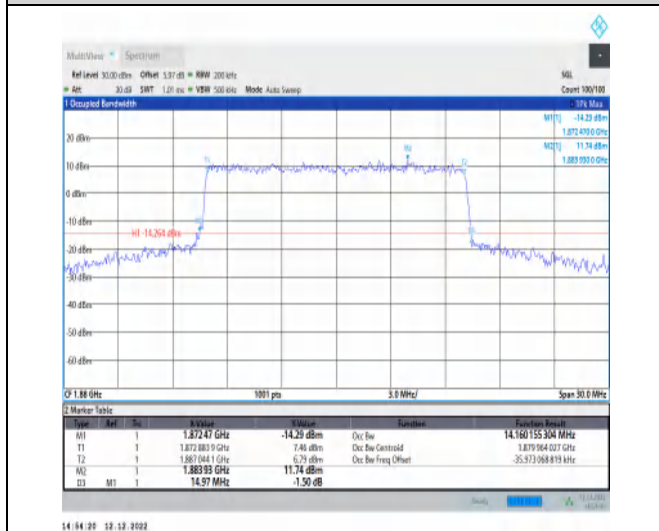
1-N2-PC3-15-15-M-8-CP-64QAM-Outer_Full-79@0- Ant1-14.16-14.970-≤15-PASS
