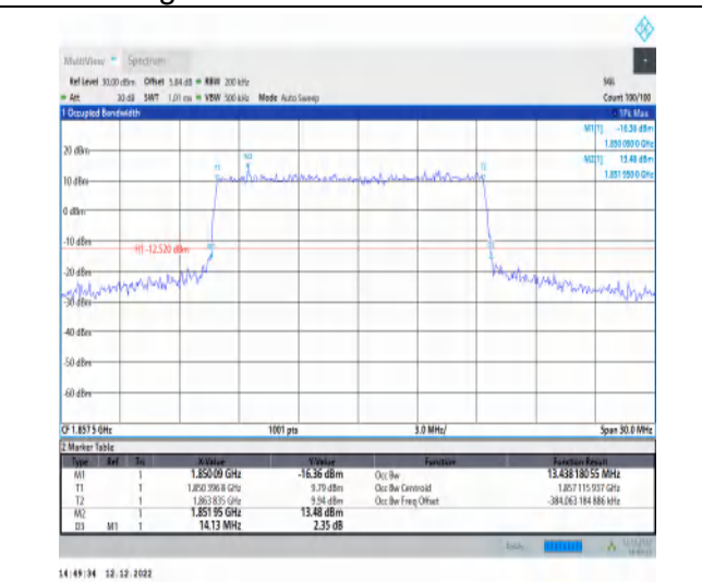
1-N2-PC3-15-15-L-4-DFT-64QAM-Outer_Full-75@0-Ant1-13.438-14.130-≤15-PASS
