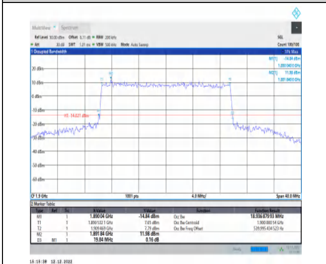
1-N2-PC3-15-20-H-8-CP-64QAM-Outer_Full-106@0-Ant1-18.937-19.840-≤20-PASS
