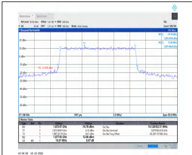
1-N2-PC3-15-15-M-6-CP-QPSK-Outer_Full-79@0-A Ant1-14.128-14.970-≤15-PASS
