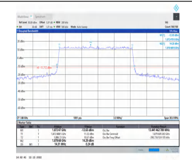
1-N2-PC3-15-15-M-1-DFT-QPSK-Outer_Full-75@0-Ant1-13.441-14.310-≤15-PASS
