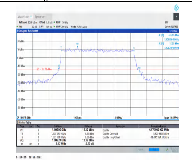
1-N2-PC3-15-5-H-4-DFT-64QAM-Outer_Full-25@0-Ant1-4.476-4.970-≤5-PASS
