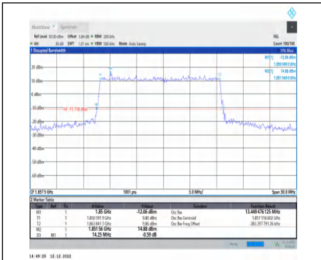
1-N2-PC3-15-15-L-3-DFT-16QAM-Outer_Full-75@0-Ant1-13.449-14.250-≤15-PASS
