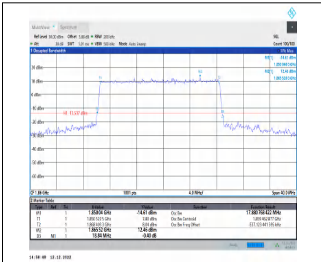
1-N2-PC3-15-20-L-4-DFT-64QAM-Outer_Full-100@ 0-Ant1-17.881-18.840-≤20-PASS
