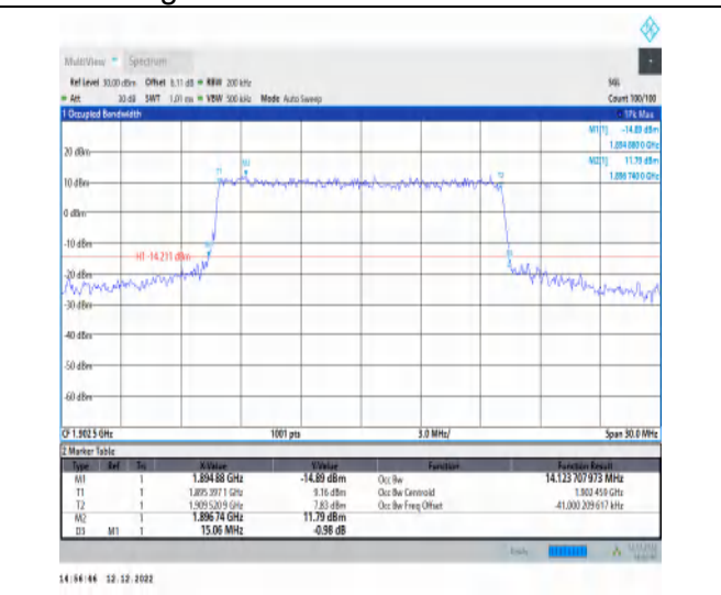
1-N2-PC3-15-15-H-6-CP-QPSK-Outer_Full-79@0-Ant1-14.124-15.060-≤15-PASS
