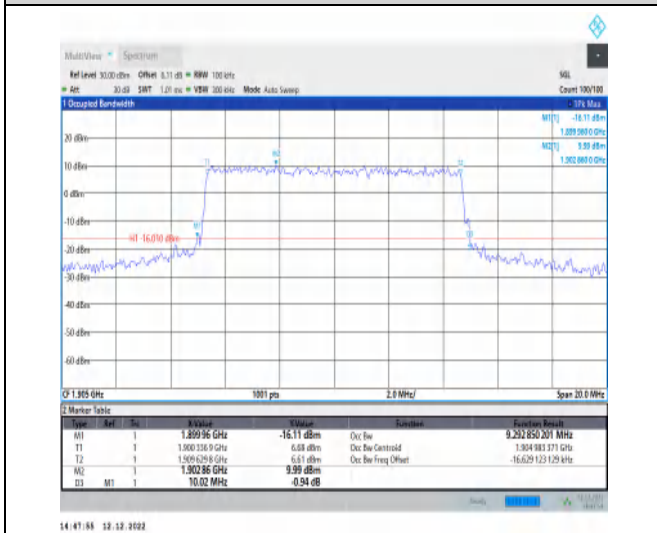
1-N2-PC3-15-10-H-6-CP-QPSK-Outer_Full-52@0-A nt1-9.293-10.020-≤10-PASS
