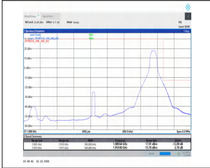
1-N2-PC3-15-5-H-5-CP-QPSK-Edge_1RB_Right-1@2 4-Ant1-1-seegraph-PASS-see graph
