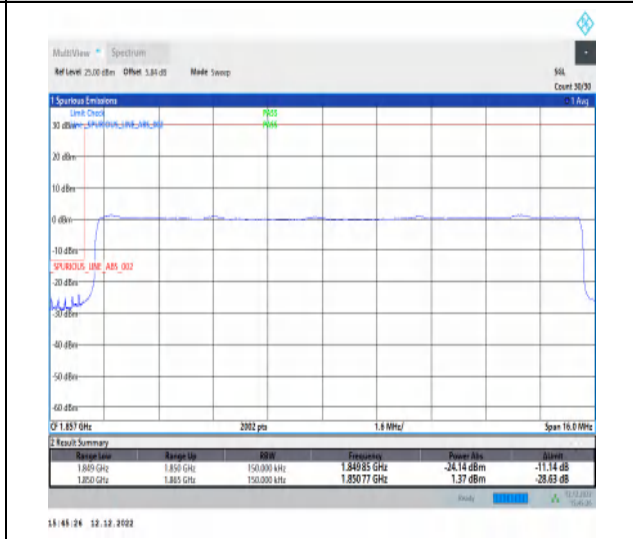
1-N2-PC3-15-15-L-6-CP-QPSK-Outer_Full-79@0-Ant1-1-seegraph-PASS-see graph
