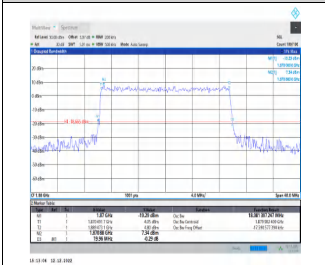
1-N2-PC3-15-20-M-9-CP-256QAM-Outer_Full-106@0 -Ant1-18.981-19.960-≤20-PASS
