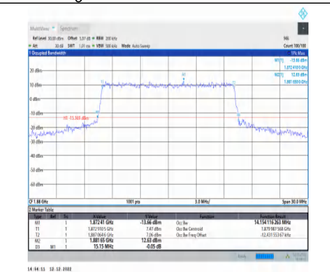
1-N2-PC3-15-15-M-7-CP-16QAM-Outer_Full-79@0- Ant1-14.154-15.150-≤15-PASS
