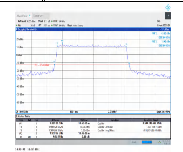
1-N2-PC3-15-10-H-1-DFT-QPSK-Outer_Full-50@0- Ant1-8.944-9.680-≤10-PASS
