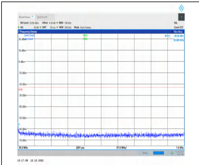
1-N2-PC3-15-20-M-1-DFT-PI2BPSK-Inner_1RB_Lef t-1@1-30-1000-Ant1-30.49--59.36--23-PASS
