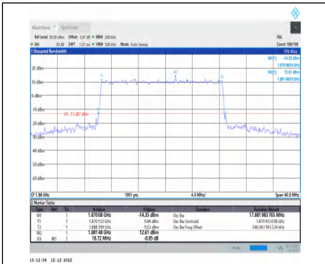
1-N2-PC3-15-20-M-3-DFT-16QAM-Outer_Full-100@0-Ant1-17.882-18.720-≤20-PASS
