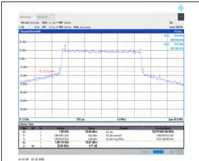
1-N2-PC3-15-20-H-6-CP-QPSK-Outer_Full-106@0-Ant1-18.919-20.040-≤20-PASS
