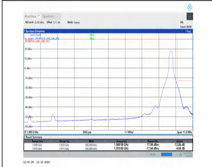
1-N2-PC3-15-10-H-5-CP-QPSK-Edge_1RB_Right-1@51-Ant1-1-seegraph-PASS-see graph
