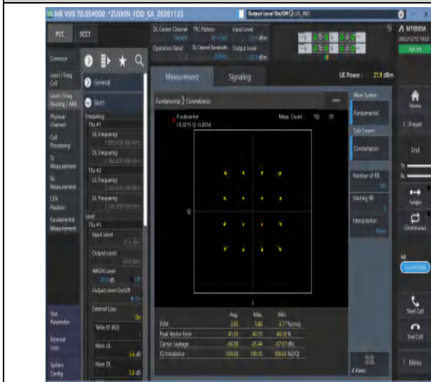
1-N2-PC3-15-20-M-3-DFT-16QAM-Outer_Full-100@ 0-Ant1-see graph-PASS
