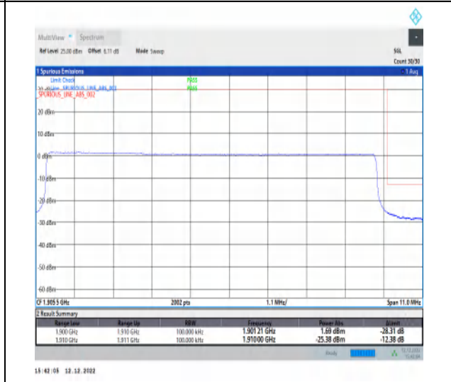
1-N2-PC3-15-10-H-6-CP-QPSK-Outer_Full-52@0-Ant1-1-seegraph-PASS-see graph
