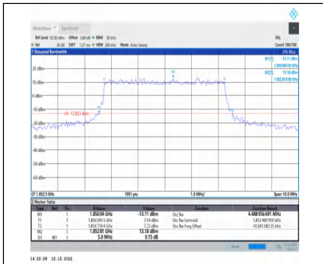
1-N2-PC3-15-5-L-1-DFT-QPSK-Outer_Full-25@0-An t1-4.489-5.000-≤5-PASS
