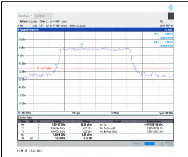
1-N2-PC3-15-5-H-7-CP-16QAM-Outer_Full-25@0-A nt1-4.492-5.030-≤5-PASS
