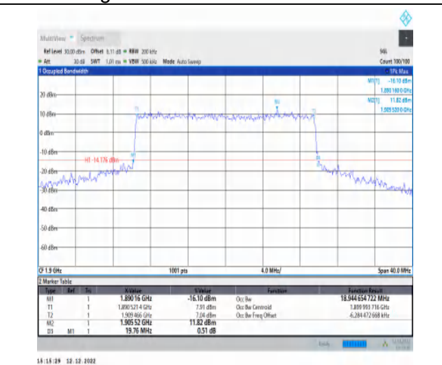
1-N2-PC3-15-20-H-7-CP-16QAM-Outer_Full-106@0-Ant1-18.945-19.760-≤20-PASS
