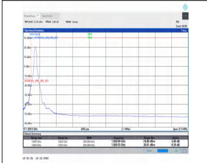
1-N2-PC3-15-20-L-4-CP-QPSK-Edge_1RB_Left-1@0-Ant1-1-seegraph-PASS-see graph
