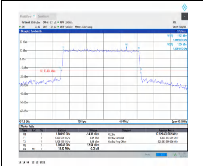
1-N2-PC3-15-20-H-4-DFT-64QAM-Outer_Full-100 @0-Ant1-17.929-18.920-≤20-PASS
