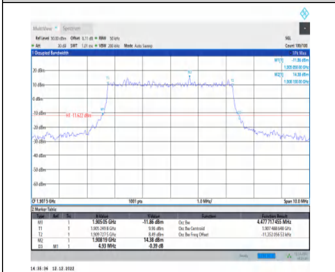
1-N2-PC3-15-5-H-1-DFT-QPSK-Outer_Full-25@0-A nt1-4.478-4.930-≤5-PASS
