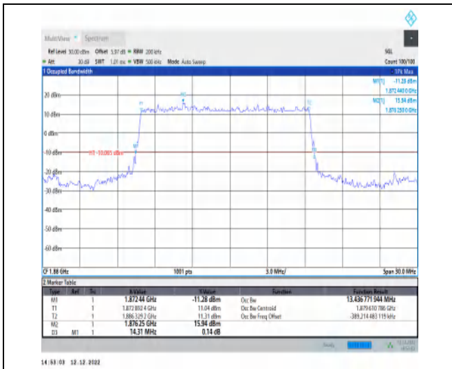
1-N2-PC3-15-15-M-2-DFT-PI2BPSK-Outer_Full-75 @0-Ant1-13.437-14.310-≤15-PASS
