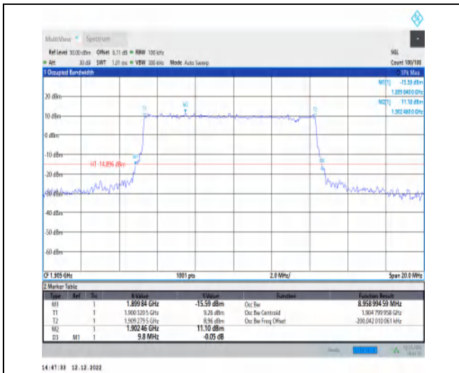
1-N2-PC3-15-10-H-4-DFT-64QAM-Outer_Full-50@0 -Ant1-8.959-9.800-≤10-PASS
