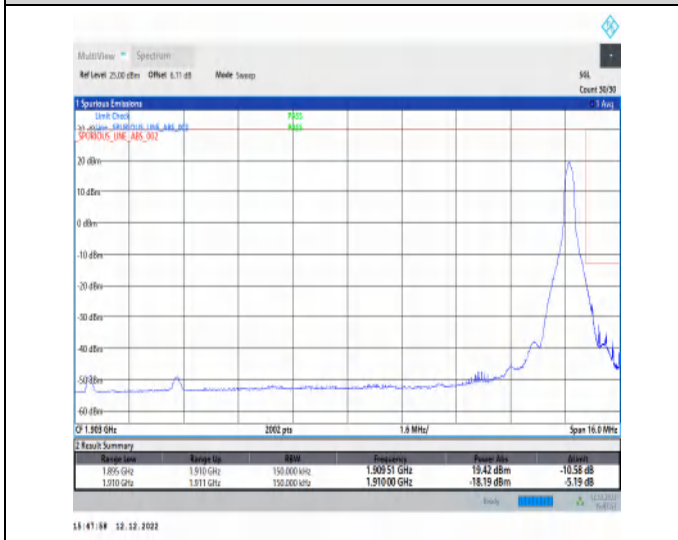
1-N2-PC3-15-15-H-5-CP-QPSK-Edge_1RB_Right-1@78-Ant1-1-seegraph-PASS-see graph
