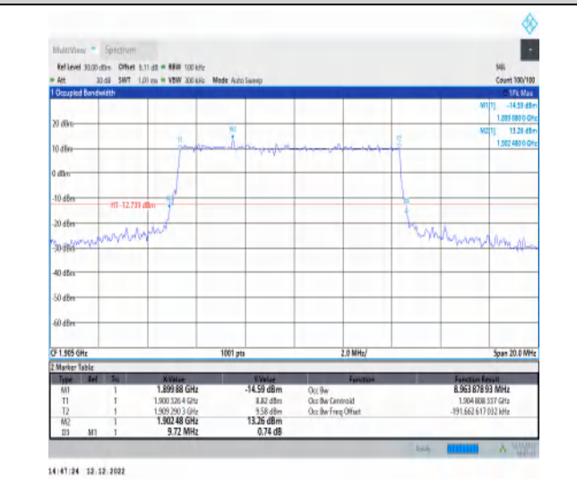
1-N2-PC3-15-10-H-3-DFT-16QAM-Outer_Full-50@0- Ant1-8.964-9.720-≤10-PASS
