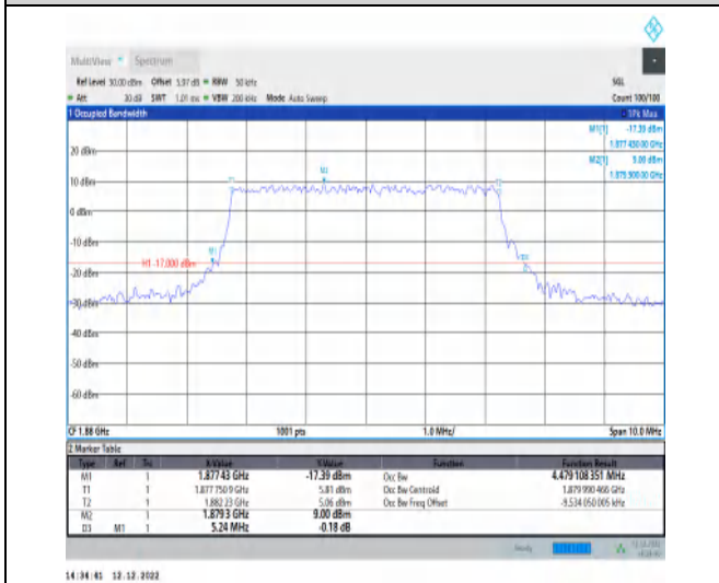
1-N2-PC3-15-5-M-6-CP-QPSK-Outer_Full-25@0-Ant1-4.479-5.240-≤5-PASS
