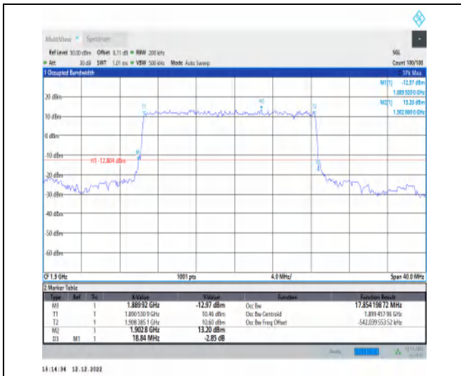
1-N2-PC3-15-20-H-2-DFT-PI2BPSK-Outer_Full-100 @0-Ant1-17.854-18.840-≤20-PASS
