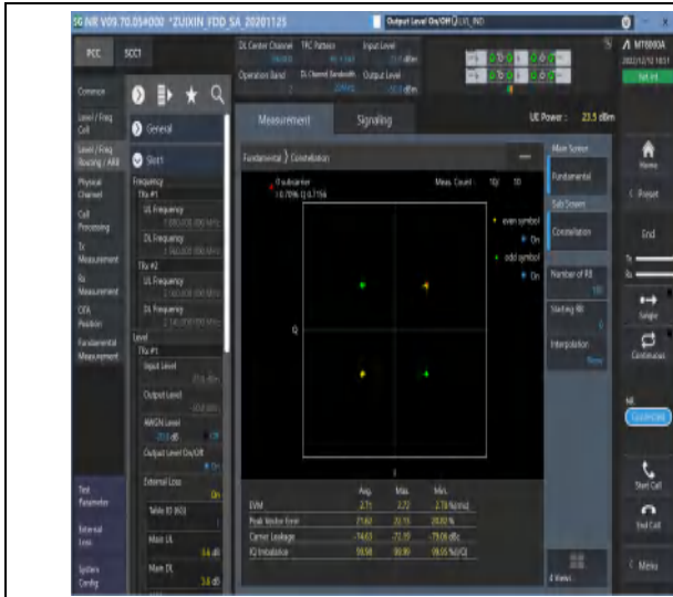
1-N2-PC3-15-20-M-1-DFT-PI2BPSK-Outer_Full-100 @0-Ant1-see graph-PASS
