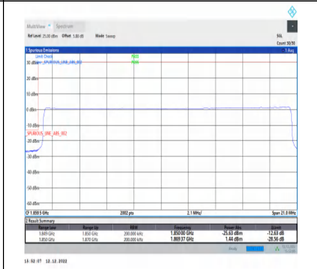
1-N2-PC3-15-20-L-6-CP-QPSK-Outer_Full-106@0-Ant1-1-seegraph-PASS-see graph
