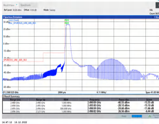
41-41-10MHz-15MHz-QPSK-QPSK-39703-39823-50RB#0-75RB#0
