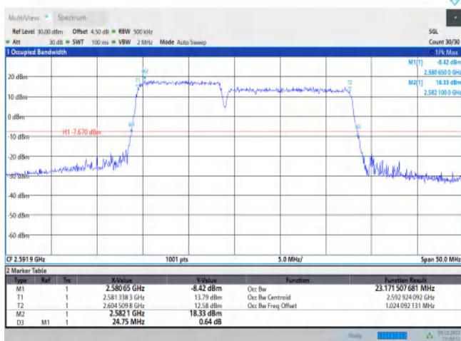
41-41-10MHz-15MHz-QPSK-QPSK-40549-40669-50RB#0-75RB#0
