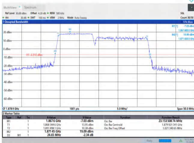
2-2-10MHz-15MHz-QPSK-QPSK-18829-18949-50RB#0-75RB#0
