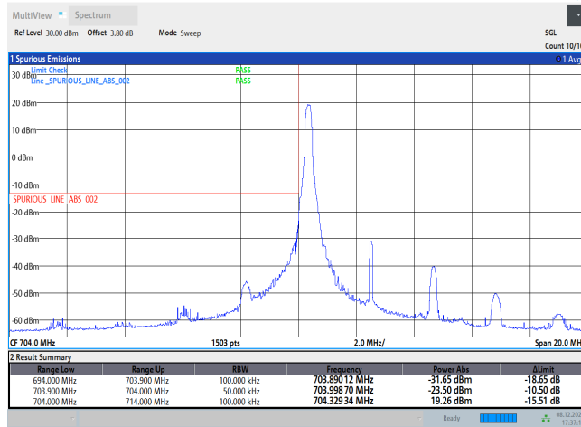
Band17-5MHz-QPSK-23755-25RB#0
