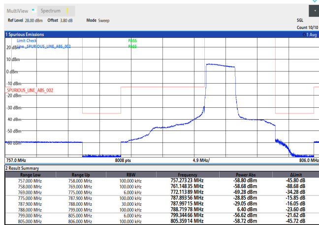
Band14-5MHz-QPSK-23305-25RB#0
