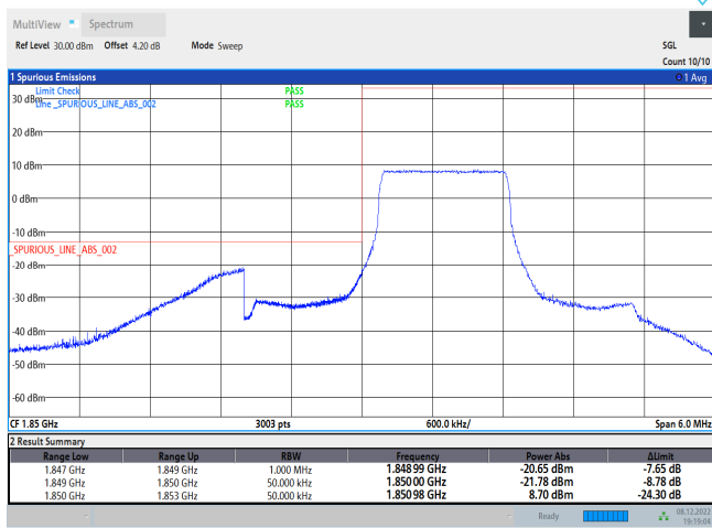
Band2-1.4MHz-QPSK-18607-6RB#0
