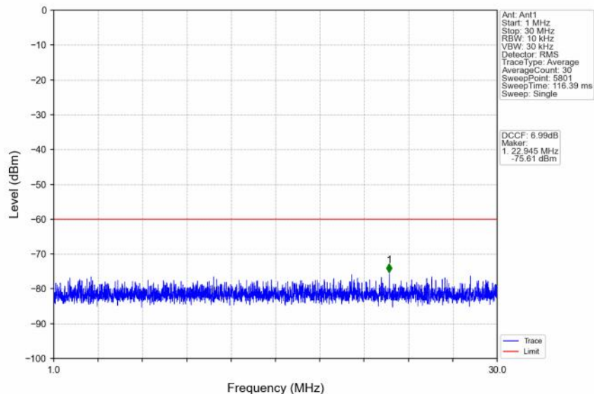
n48_30kHz_SISO_NTNV_40MHz_DFT-s-OFDM QPSK_3624.99MHz_Edge_1RB_Left
