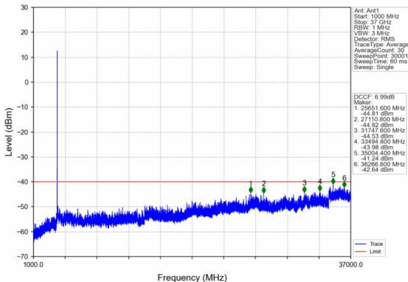
n48_30kHz_SISO_NTNV_30MHz_DFT-s-OFDM QPSK_3565.02MHz_Edge_1RB_Left
