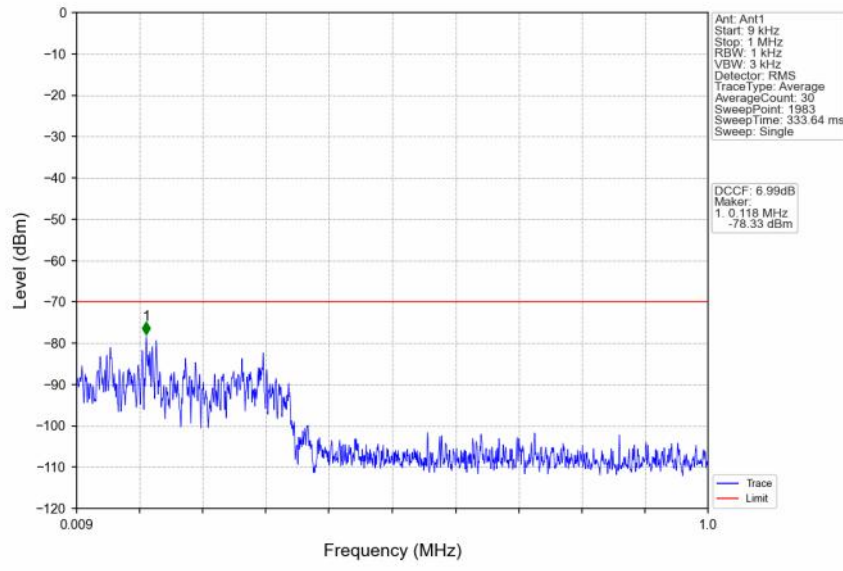
n48_30kHz_SISO_NTNV_30MHz_DFT-s-OFDM PI/2 BPSK_3684.99MHz_Inner_1RB_Right
