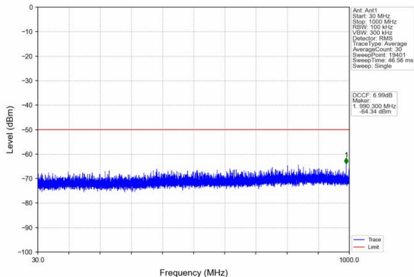
n48_30kHz_SISO_NTNV_30MHz_DFT-s-OFDM QPSK_3565.02MHz_Inner_1RB_Left
