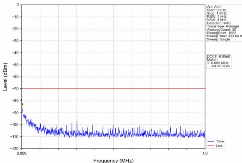
n48_30kHz_SISO_NTNV_30MHz_DFT-s-OFDM QPSK_3565.02MHz_Outer_Full
