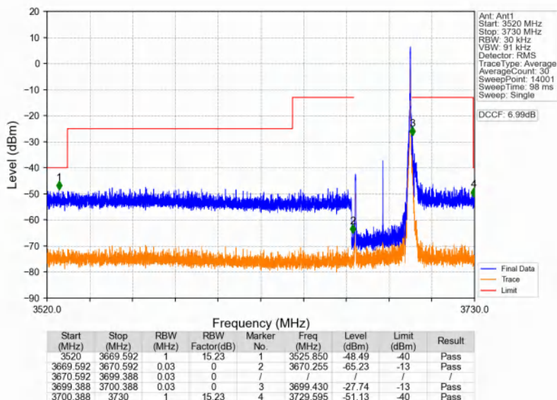
n48_30kHz_SISO_NTV_30MHz_CP-OFDM QPSK_3684.99MHz_Inner_1RB_Right
