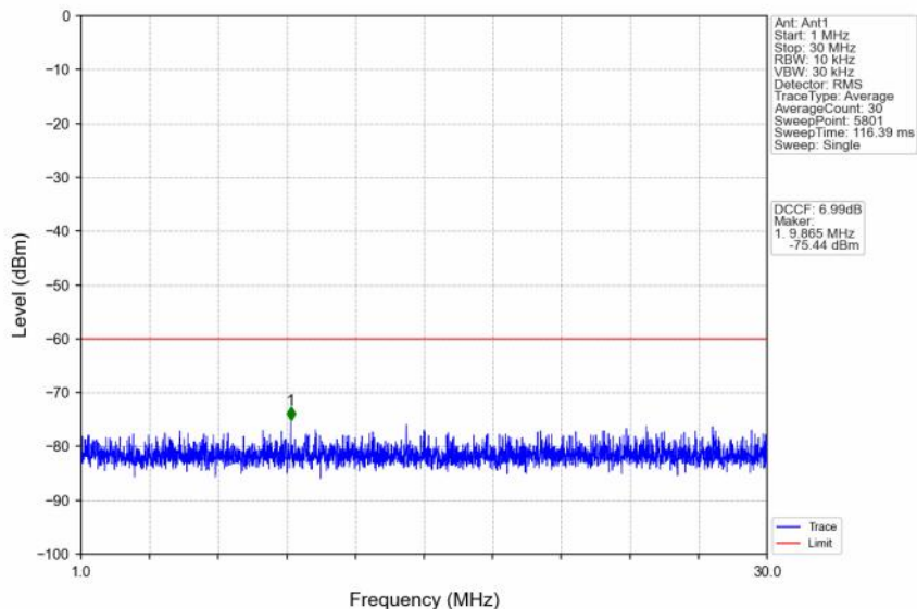
n48_30kHz_SISO_NTNV_30MHz_DFT-s-OFDM QPSK_3624.99MHz_Edge_1RB_Left
