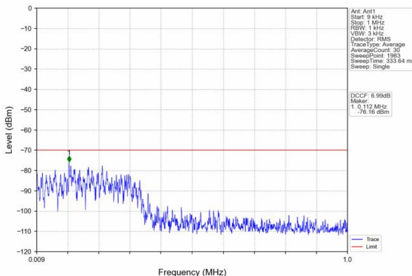
n48_30kHz_SISO_NTNV_30MHz_DFT-s-OFDM QPSK_3624.99MHz_Edge_1RB_Left
