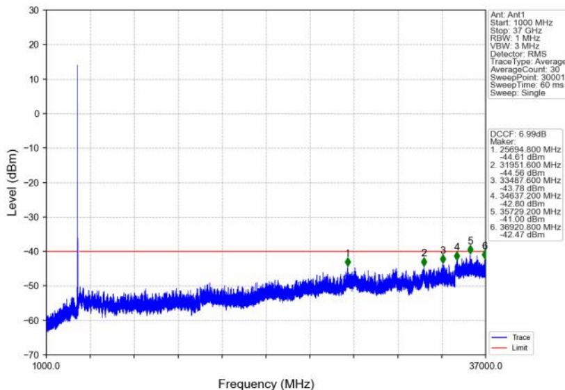
n48_30kHz_SISO_NTNV_30MHz_CP-OFDM_QPSK_3624.99MHz_Edge_1RB_Left
