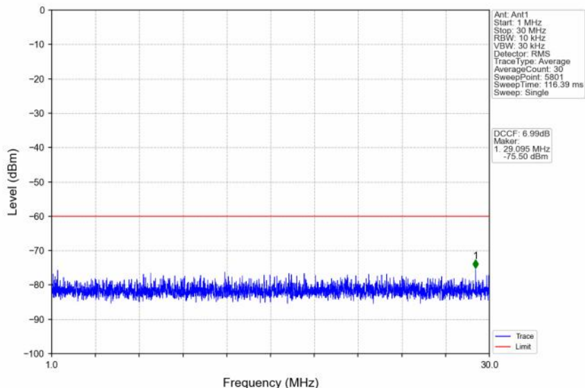
n48_30kHz_SISO_NTV_30MHz_DFT-s-OFDM QPSK_3684.99MHz_Edge_1RB_Right
