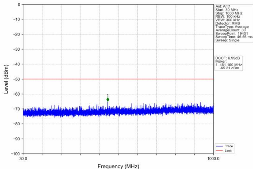
n48_30kHz_SISO_NTNV_30MHz_CP-OFDM QPSK_3565.02MHz_Outer_Full
