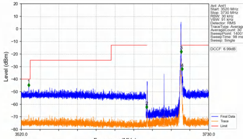
n48_30kHz_SISO_NTNV_40MHz_CP-OFDM QPSK_3679.98MHz_Edge_1RB_Right
