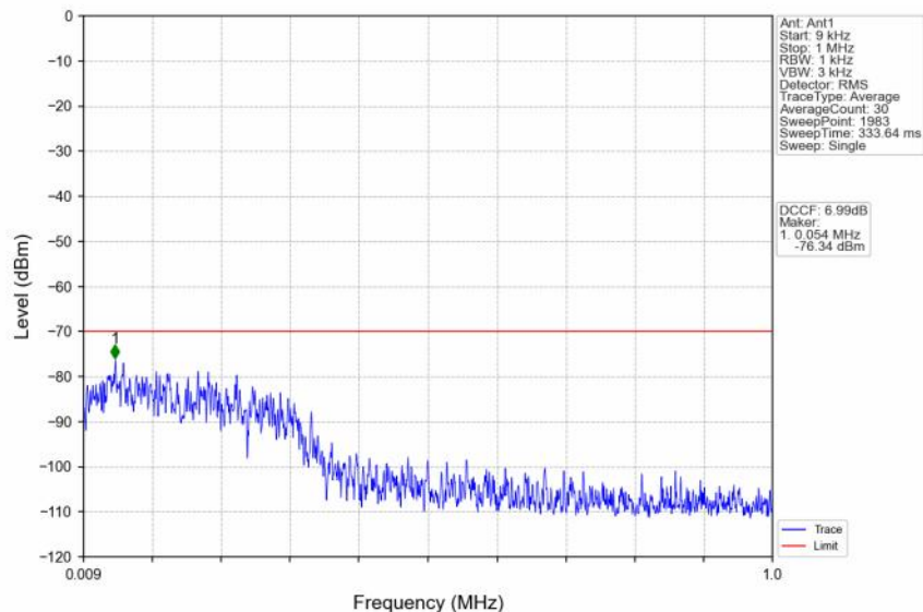
n48_30kHz_SISO_NTNV_40MHz_CP-OFDM QPSK_3624.99MHz_Edge_1RB_Left
