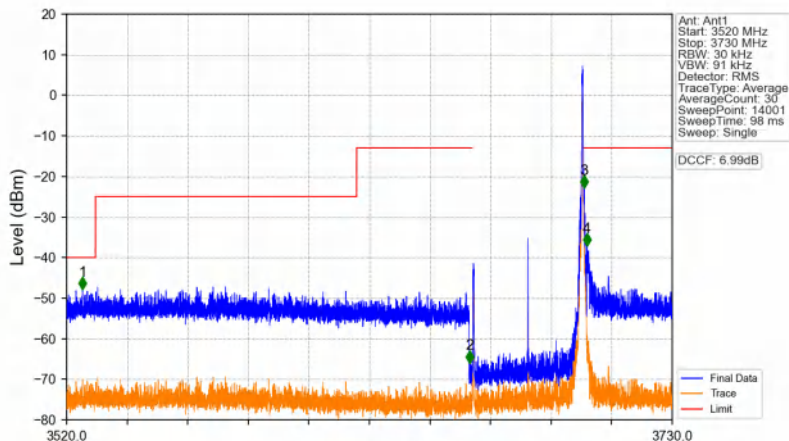
n48_30kHz_SISO_NTNV_40MHz_DFT-s-OFDM PI/2 BPSK_3679.98MHz_Edge_1RB_Right
