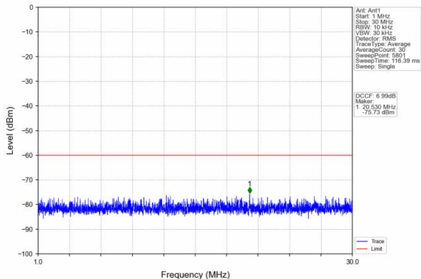
n48_30kHz_SISO_NTNV_40MHz_CP-OFDM QPSK_3679.98MHz_Edge_1RB_Right
