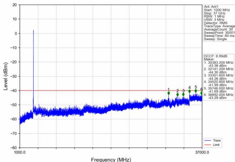
n48_30kHz_SISO_NTNV_30MHz_DFT-s-OFDM PI/2 BPSK_3684.99MHz_Outer_Full
