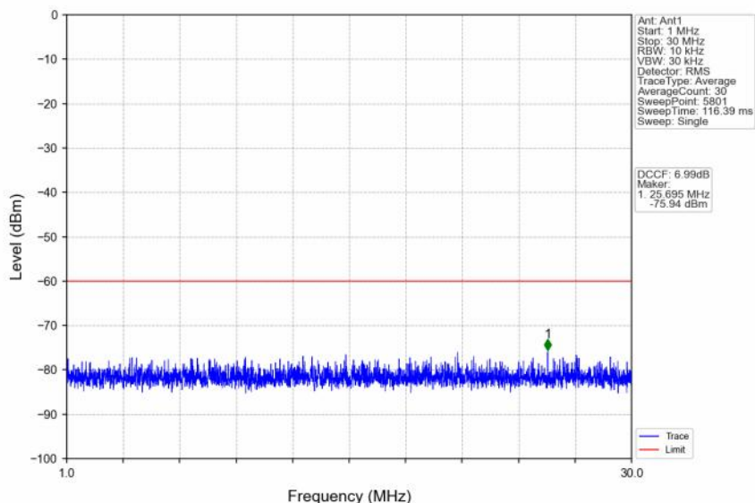
n48_30kHz_SISO_NTNV_30MHz_DFT-s-OFDM QPSK_3565.02MHz_Edge_1RB_Left
