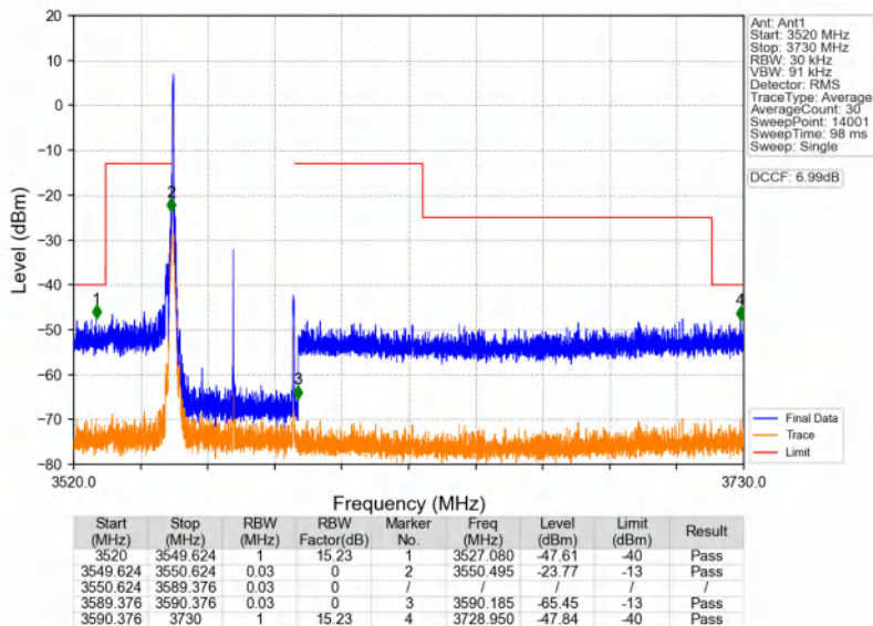
n48_30kHz_SISO_NTNV_40MHz_DFT-s-OFDM QPSK_3570MHz_Edge_1RB_Left
