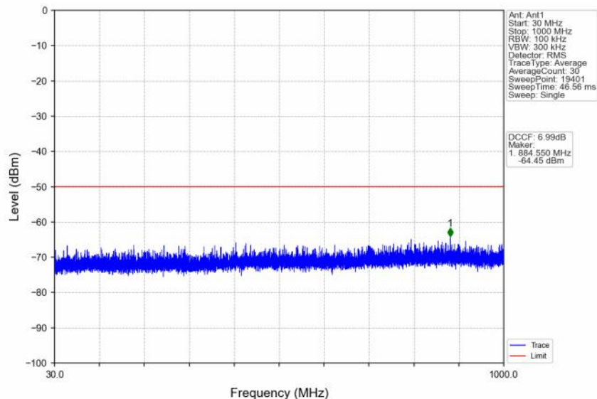
n48_30kHz_SISO_NTNV_30MHz_DFT-s-OFDM QPSK_3565.02MHz_Edge_1RB_Left
