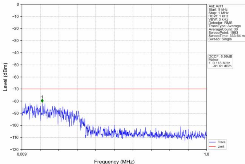
n48_30kHz_SISO_NTNV_30MHz_CP-OFDM QPSK_3684.99MHz_Edge_1RB_Right
