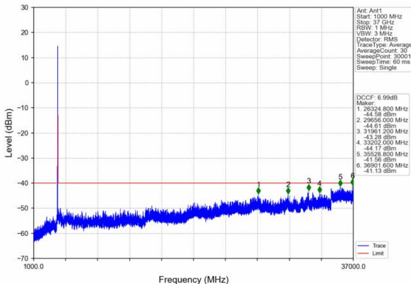
n48_30kHz_SISO_NTNV_40MHz_DFT-s-OFDM QPSK_3570MHz_Edge_1RB_Left
