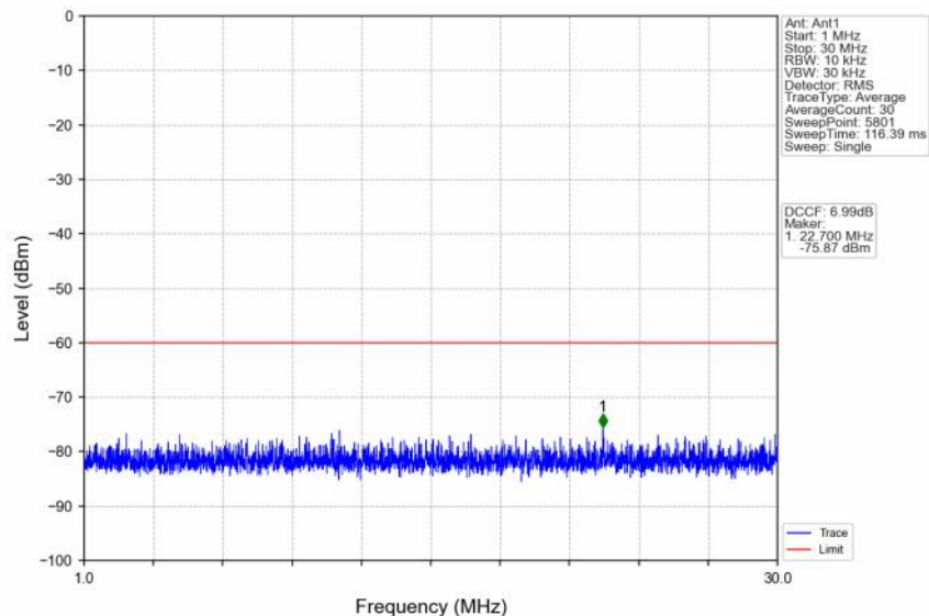
n48_30kHz_SISO_NTNV_30MHz_DFT-s-OFDM QPSK_3684.99MHz_Outer_Full
