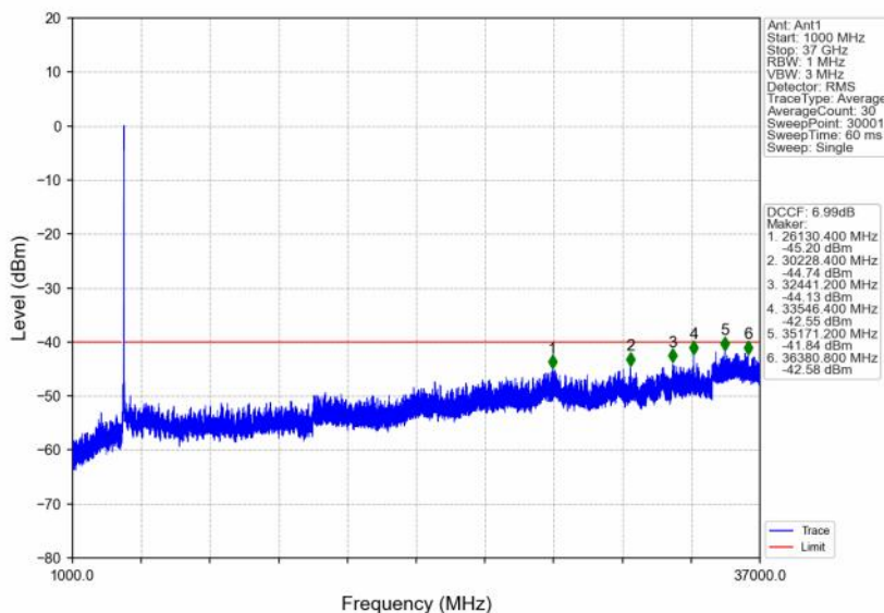
n48_30kHz_SISO_NTNV_30MHz_DFT-s-OFDM QPSK_3684.99MHz_Inner_1RB_Right
