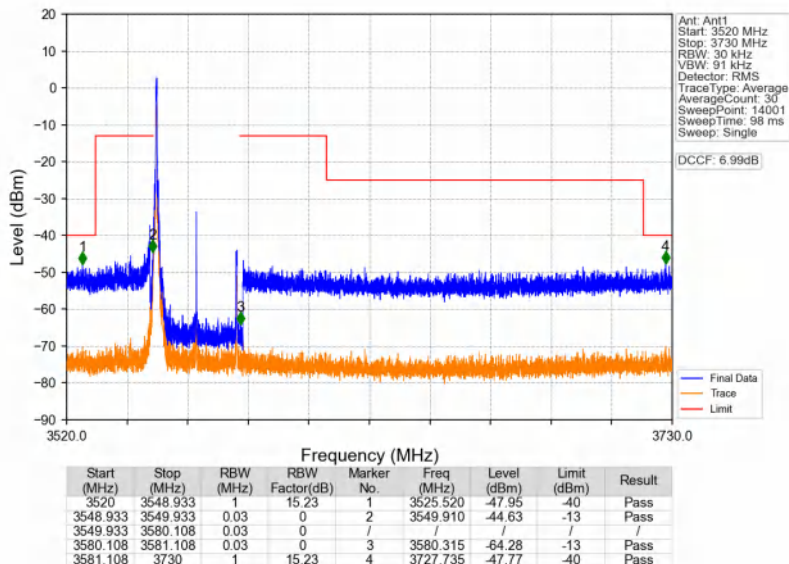
n48_30kHz_SISO_NTNV_30MHz_CP-OFDM QPSK_3565.02MHz_Edge_1RB_Left
