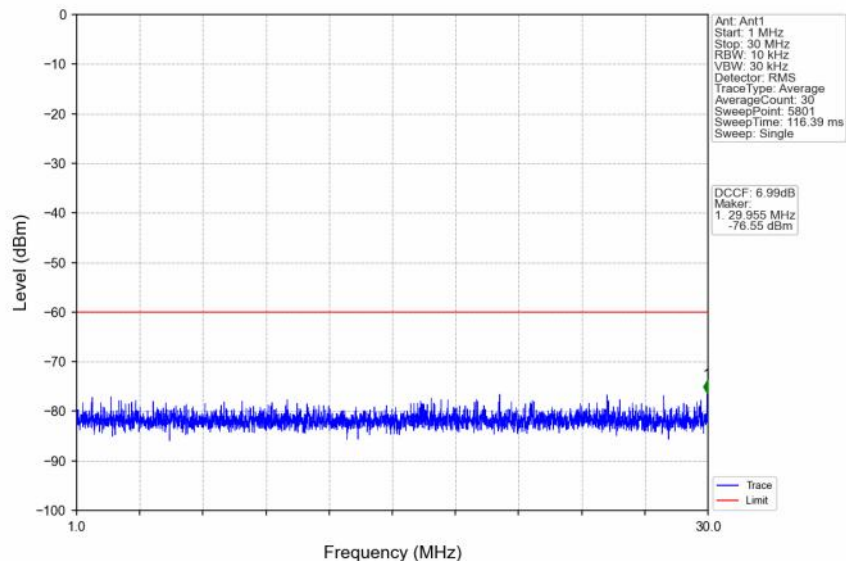
n48_30kHz_SISO_NTNV_40MHz_DFT-s-OFDM QPSK_3679.98MHz_Outer_Full
