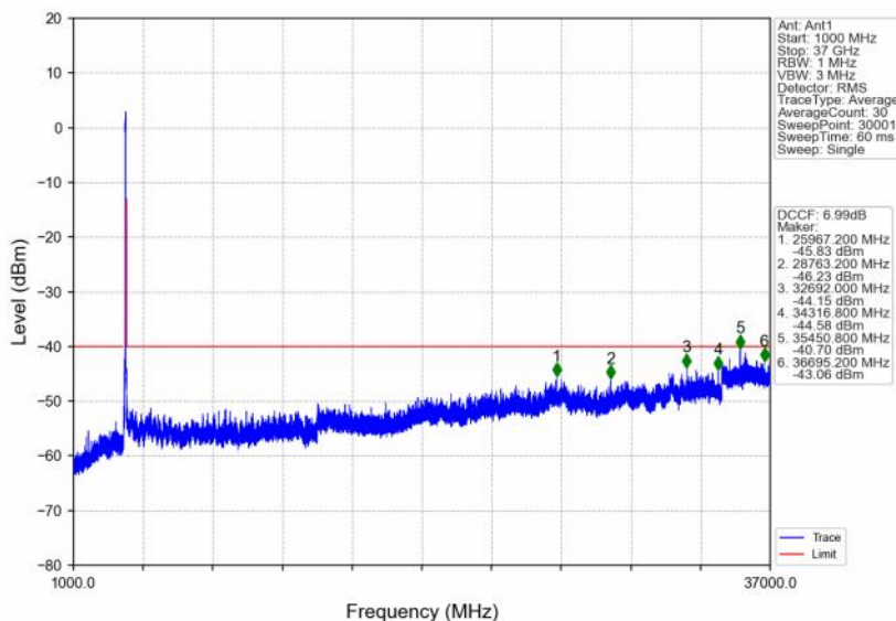
n48_30kHz_SISO_NTNV_40MHz_DFT-s-OFDM QPSK_3679.98MHz_Inner_1RB_Right
