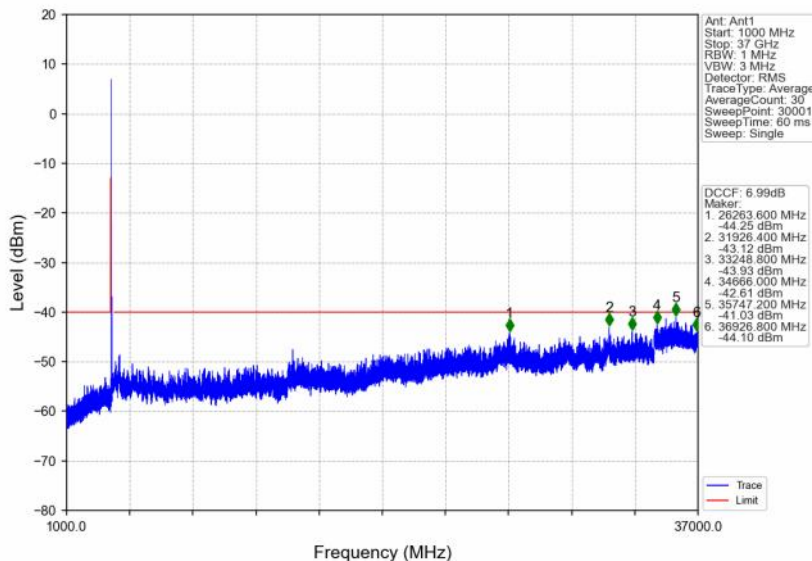
n48_30kHz_SISO_NTNV_40MHz_CP-OFDM QPSK_3570MHz_Outer_Full
