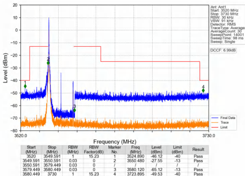
n48_30kHz_SISO_NTNV_30MHz_DFT-s-OFDM QPSK_3565.02MHz_Inner_1RB_Left
