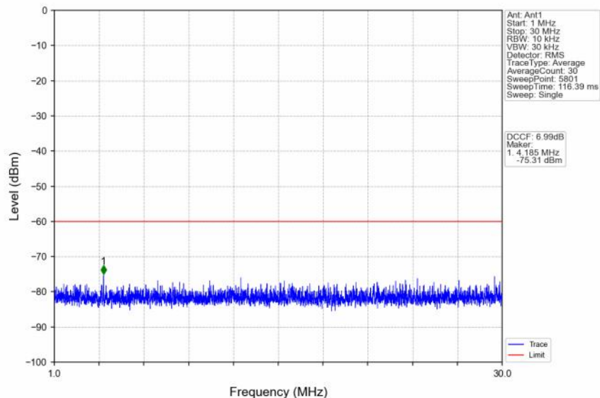
n48_30kHz_SISO_NTNV_30MHz_CP-OFDM QPSK_3684.99MHz_Edge_1RB_Right
