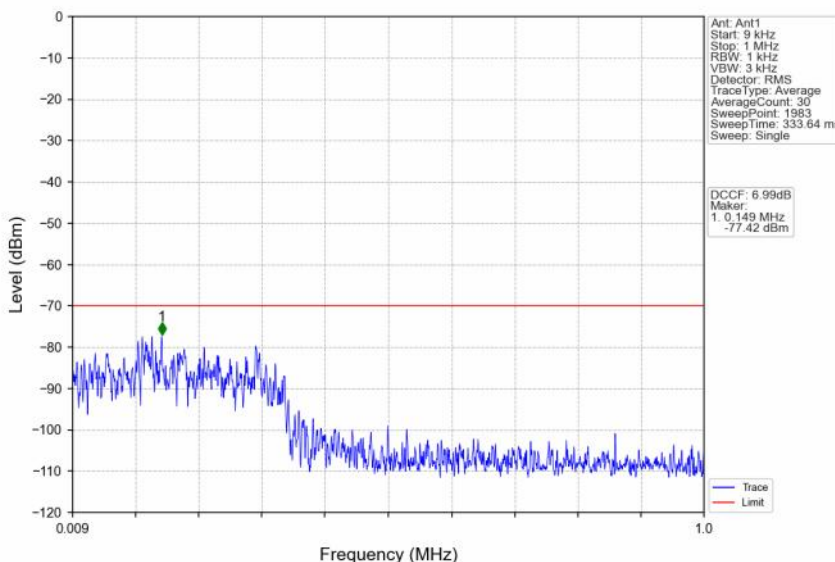
n48_30kHz_SISO_NTNV_40MHz_DFT-s-OFDM QPSK_3624.99MHz_Edge_1RB_Left
