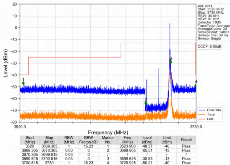
n48_30kHz_SISO_NTNV_30MHz_CP-OFDM QPSK_3684.99MHz_Edge_1RB_Right
