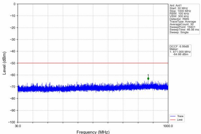
n48_30kHz_SISO_NTNV_30MHz_DFT-s-OFDM QPSK_3624.99MHz_Edge_1RB_Left
