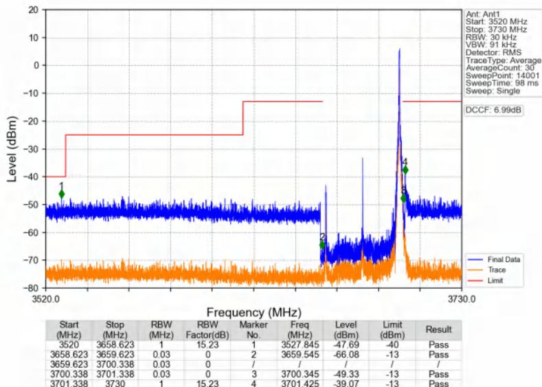
n48_30kHz_SISO_NTNV_40MHz_CP-OFDM QPSK_3679.98MHz_Inner_1RB_Right
