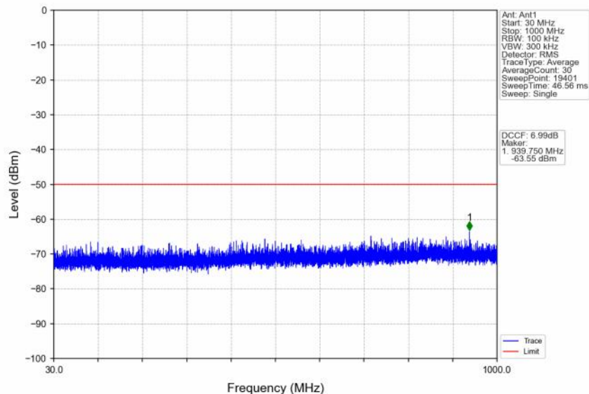
n48_30kHz_SISO_NTNV_40MHz_CP-OFDM QPSK_3624.99MHz_Edge_1RB_Left
