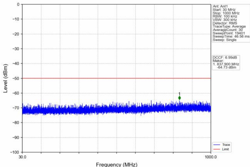
n48_30kHz_SISO_NTNV_40MHz_CP-OFDM QPSK_3679.98MHz_Inner_1RB_Right
