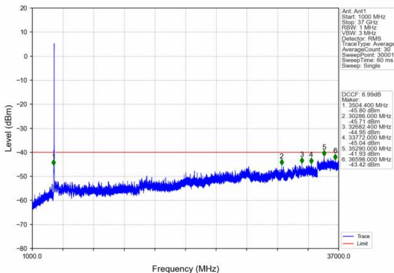
n48_30kHz_SISO_NTNV_30MHz_DFT-s-OFDM QPSK_3565.02MHz_Inner_1RB_Left
