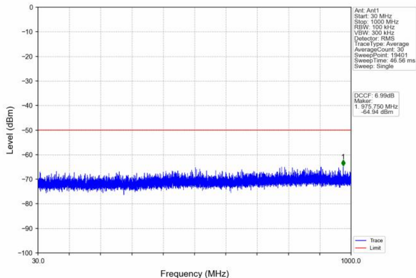
n48_30kHz_SISO_NTNV_40MHz_DFT-s-OFDM QPSK_3570MHz_Edge_1RB_Left
