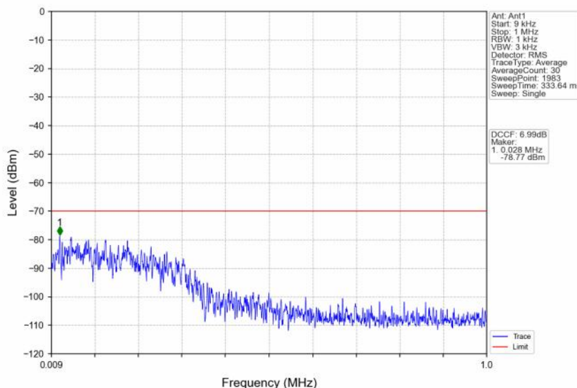
n48_30kHz_SISO_NTV_30MHz_CP-OFDM QPSK_3684.99MHz_Inner_1RB_Right
