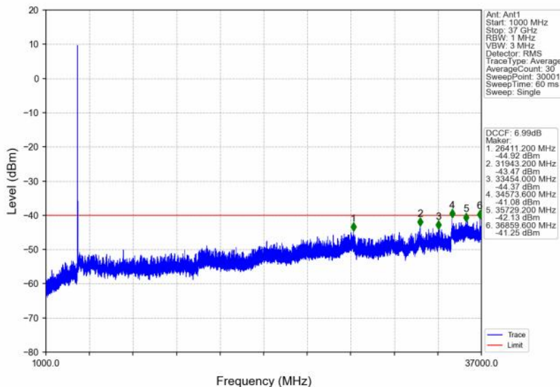
n48_30kHz_SISO_NTNV_40MHz_DFT-s-OFDM QPSK_3679.98MHz_Edge_1RB_Right
