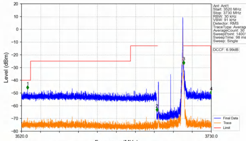
n48_30kHz_SISO_NTNV_30MHz_DFT-s-OFDM PI/2 BPSK_3684.99MHz_Inner_1RB_Right
