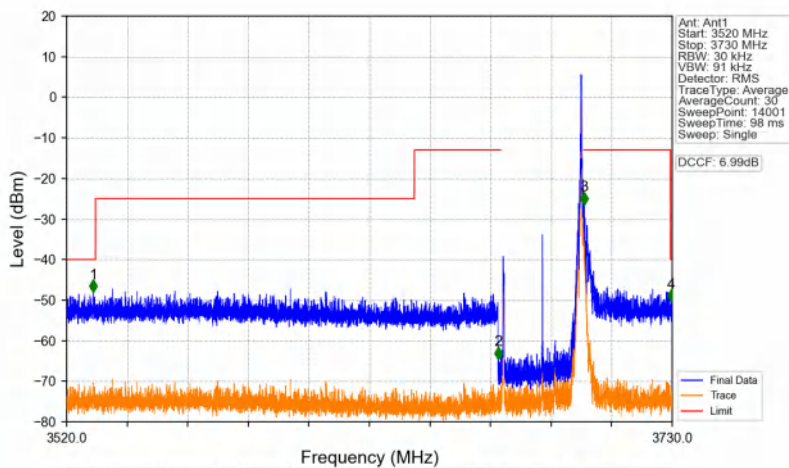
n48_30kHz_SISO_NTNV_30MHz_DFT-s-OFDM QPSK_3684.99MHz_Inner_1RB_Right
