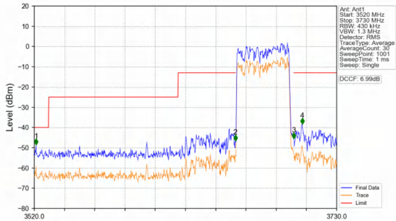
n48_30kHz_SISO_NTNV_40MHz_DFT-s-OFDM PI/2 BPSK_3679.98MHz_Outer_Full
