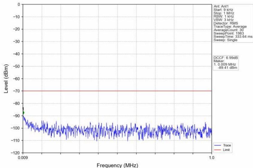
n48_30kHz_SISO_NTNV_40MHz_CP-OFDM QPSK_3570MHz_Outer_Full
