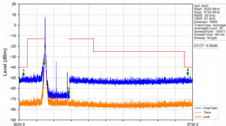
n48_30kHz_SISO_NTNV_30MHz_CP-OFDM QPSK_3565.02MHz_Inner_1RB_Left
