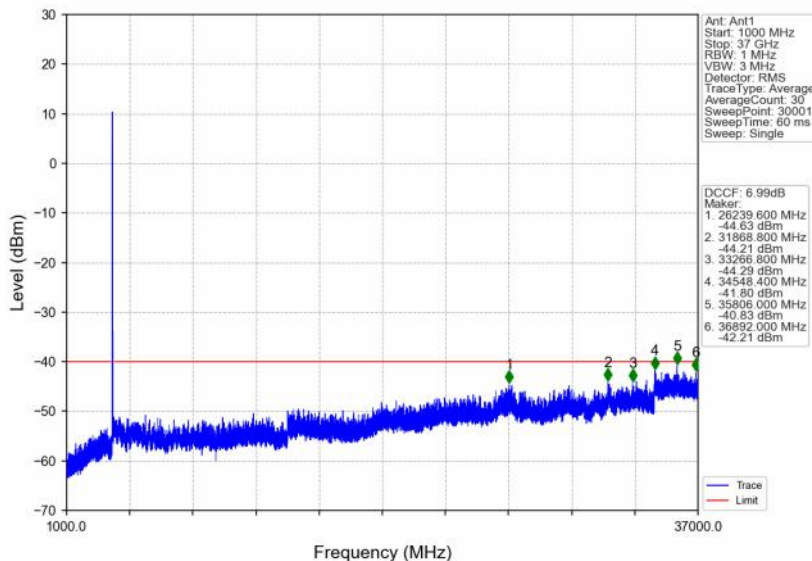
n48_30kHz_SISO_NTNV_30MHz_DFT-s-OFDM QPSK_3684.99MHz_Edge_1RB_Right
