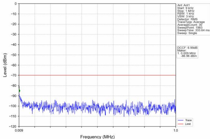
n48_30kHz_SISO_NTNV_30MHz_CP-OFDM QPSK_3565.02MHz_Outer_Full
