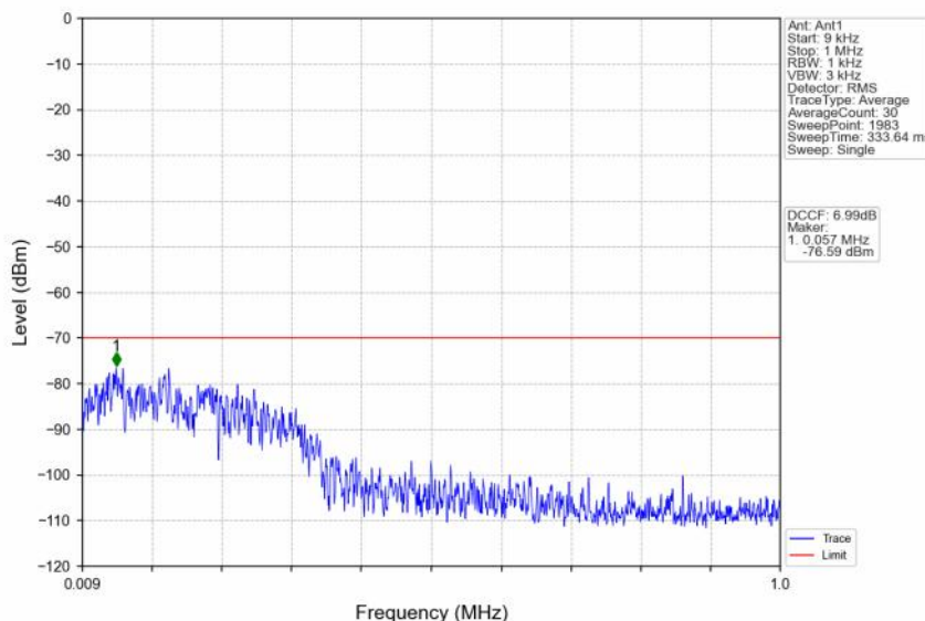
n48_30kHz_SISO_NTNV_30MHz_CP-OFDM QPSK_3565.02MHz_Edge_1RB_Left
