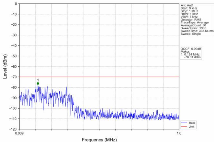
n48_30kHz_SISO_NTNV_40MHz_DFT-s-OFDM QPSK_3679.98MHz_Inner_1RB_Right
