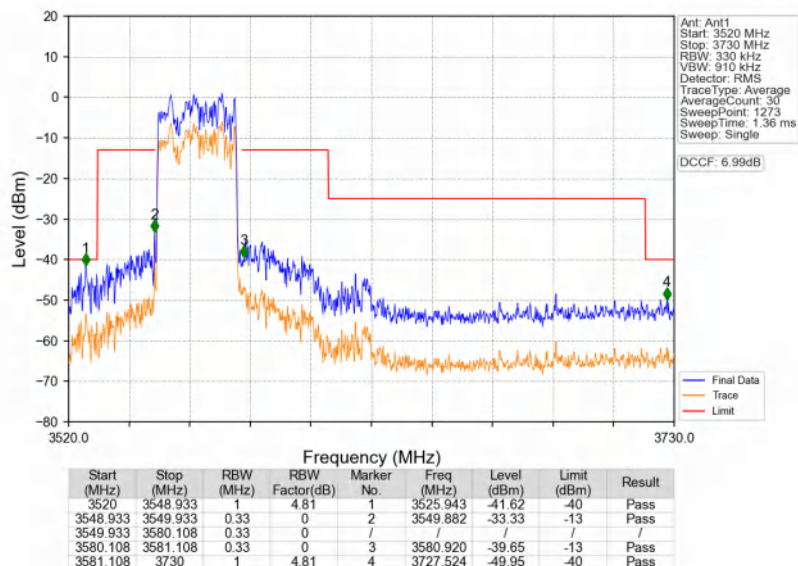
n48_30kHz_SISO_NTNV_30MHz_DFT-s-OFDM QPSK_3565.02MHz_Outer_Full
