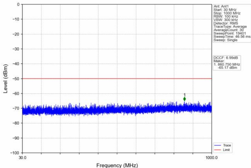
n48_30kHz_SISO_NTNV_40MHz_CP-OFDM QPSK_3570MHz_Outer_Full
