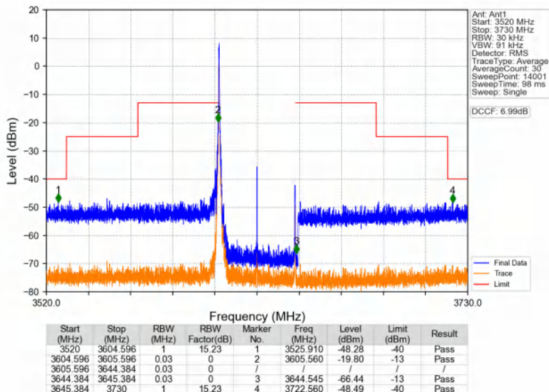
n48_30kHz_SISO_NTNV_40MHz_DFT-s-OFDM QPSK_3624.99MHz_Edge_1RB_Left
