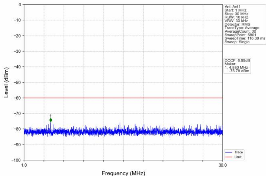
n48_30kHz_SISO_NTNV_40MHz_DFT-s-OFDM QPSK_3570MHz_Outer_Full
