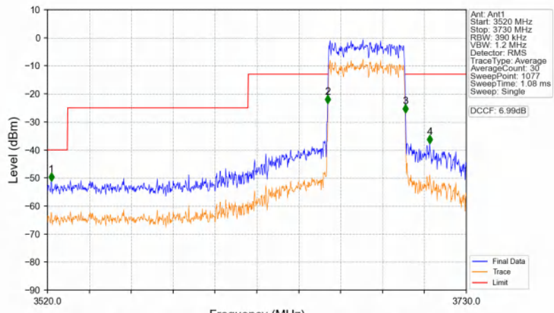
n48_30kHz_SISO_NTNV_40MHz_CP-OFDM QPSK_3679.98MHz_Outer_Full
