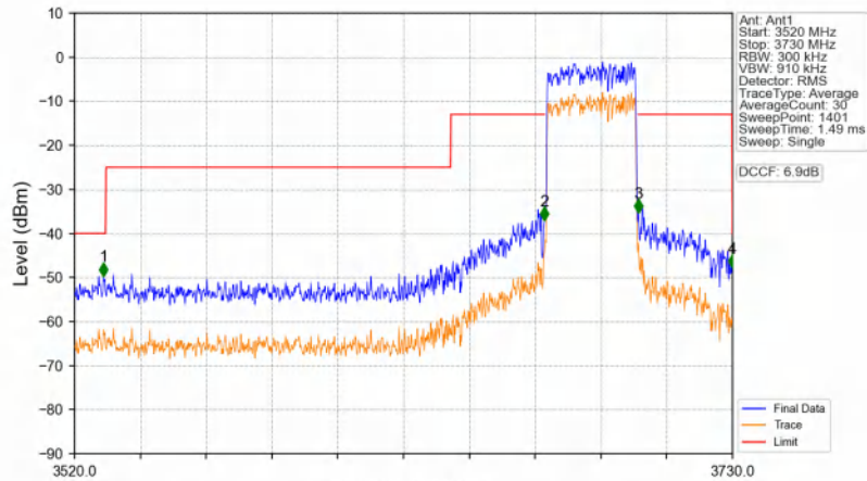
n48_30kHz_SISO_NTV_30MHz_CP-OFDM QPSK_3684.99MHz_Outer_Full
