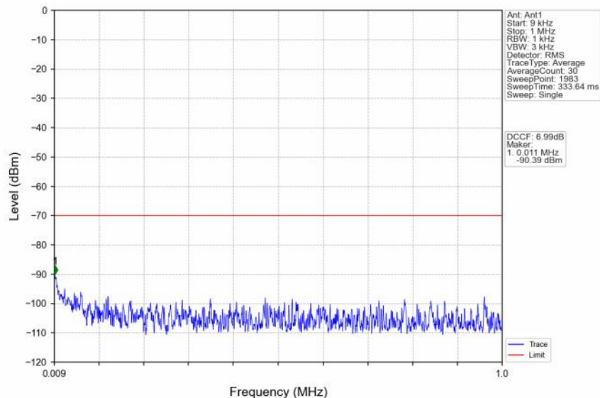
n48_30kHz_SISO_NTNV_40MHz_CP-OFDM QPSK_3679.98MHz_Outer_Full
