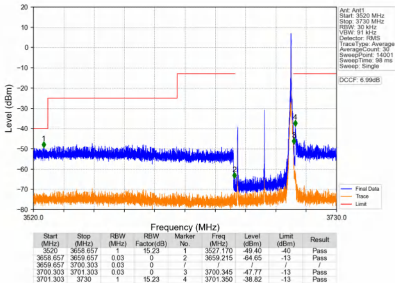
n48_30kHz_SISO_NTNV_40MHz_DFT-s-OFDM PI/2 BPSK_3679.98MHz_Inner_1RB_Right
