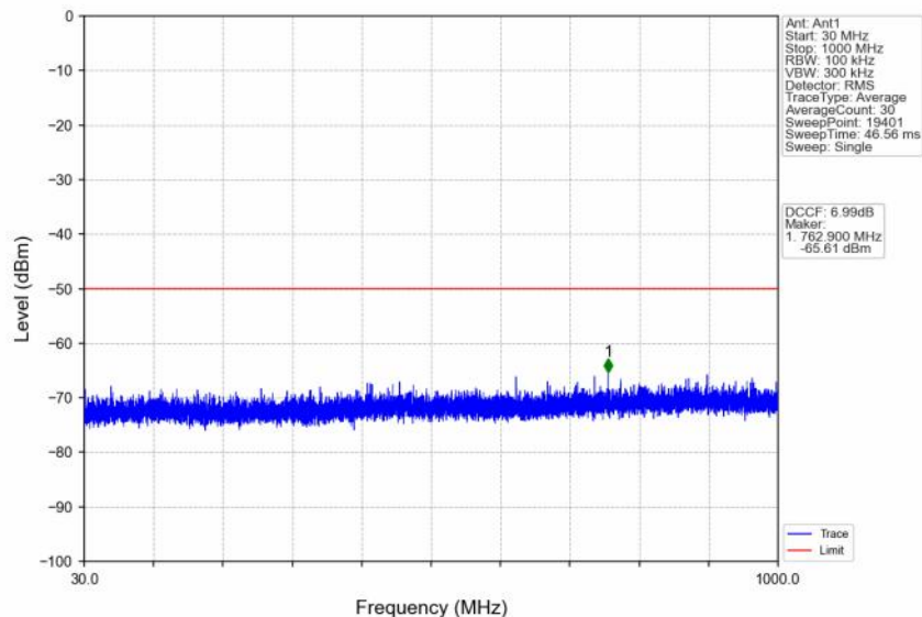
n48_30kHz_SISO_NTNV_40MHz_CP-OFDM QPSK_3679.98MHz_Outer_Full
