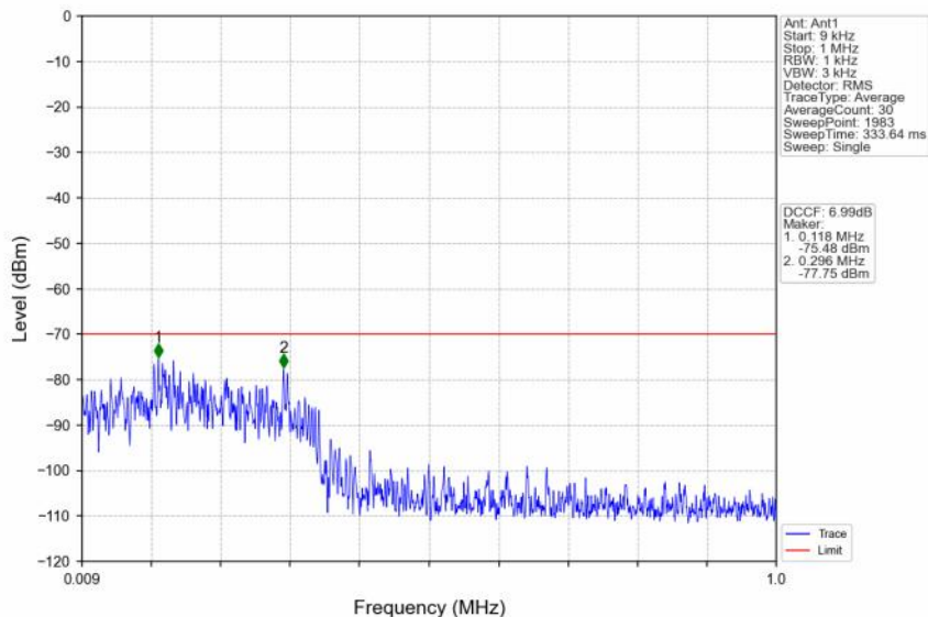
n48_30kHz_SISO_NTNV_30MHz_DFT-s-OFDM QPSK_3565.02MHz_Edge_1RB_Left
