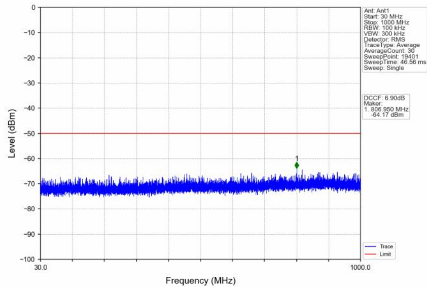
n48_30kHz_SISO_NTNV_30MHz_CP-OFDM QPSK_3684.99MHz_Outer_Full
