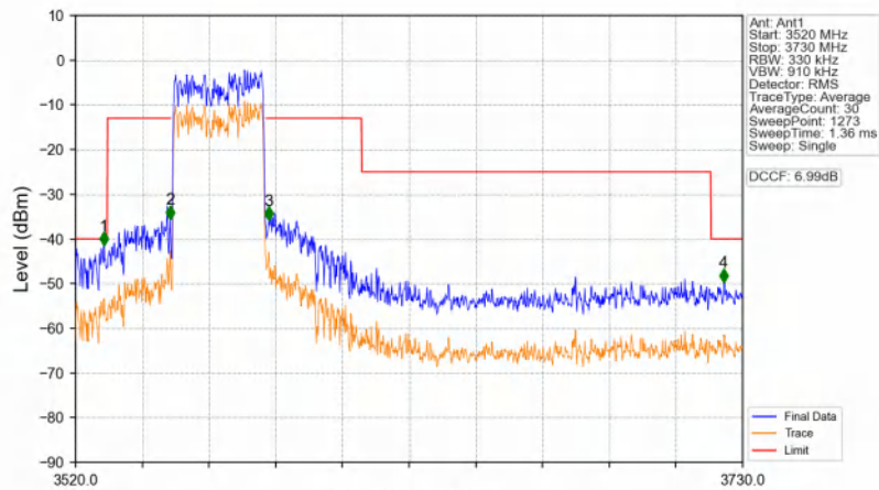
n48_30kHz_SISO_NTNV_30MHz_CP-OFDM QPSK_3565.02MHz_Outer_Full
