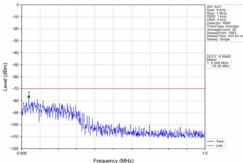
n48_30kHz_SISO_NTNV_40MHz_CP-OFDM QPSK_3679.98MHz_Inner_1RB_Right
