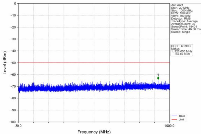
n48_30kHz_SISO_NTNV_30MHz_CP-OFDM QPSK_3624.99MHz_Edge_1RB_Left
