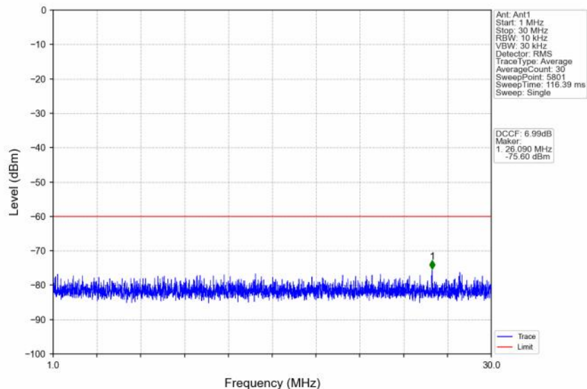
n48_30kHz_SISO_NTNV_30MHz_CP-OFDM QPSK_3565.02MHz_Inner_1RB_Left
