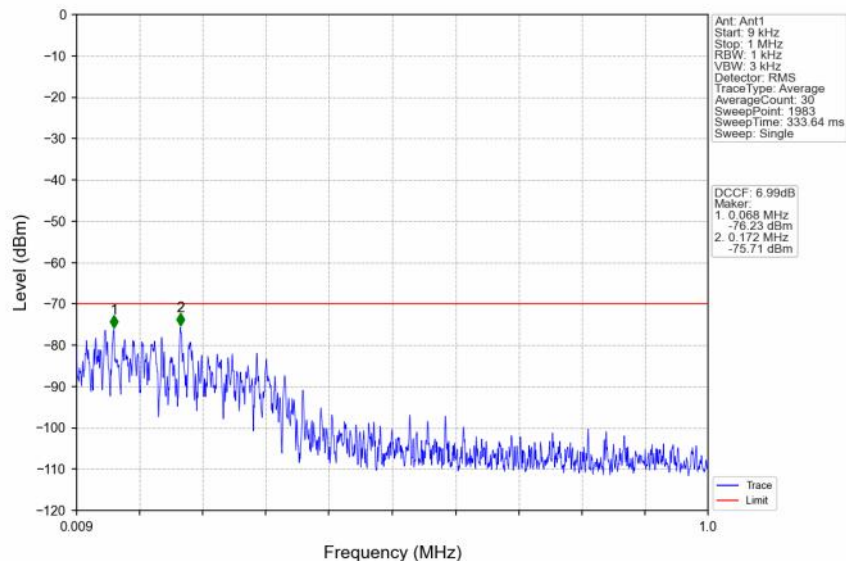
n48_30kHz_SISO_NTNV_30MHz_CP-OFDM QPSK_3624.99MHz_Edge_1RB_Left
