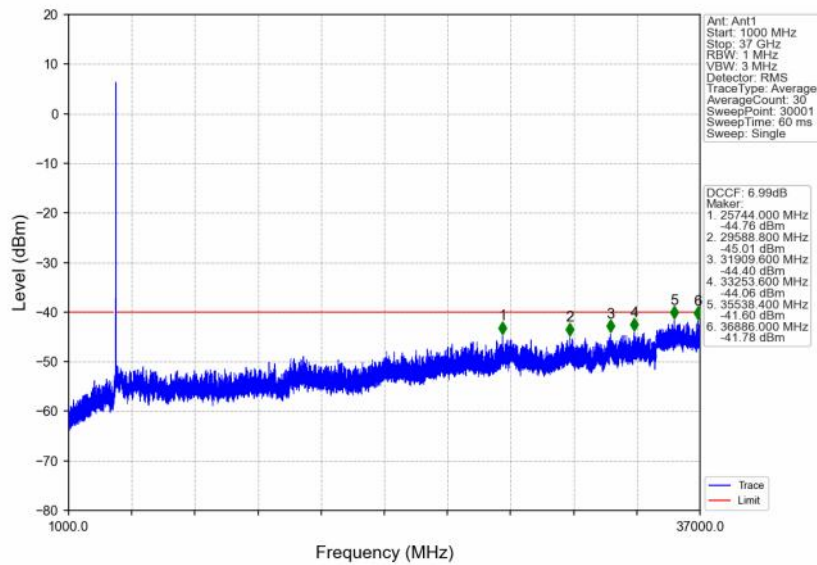
n48_30kHz_SISO_NTV_30MHz_CP-OFDM QPSK_3684.99MHz_Outer_Full
