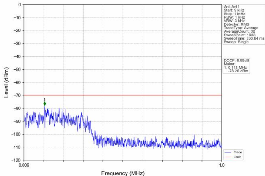
n48_30kHz_SISO_NTNV_30MHz_DFT-s-OFDM QPSK_3684.99MHz_Inner_1RB_Right
