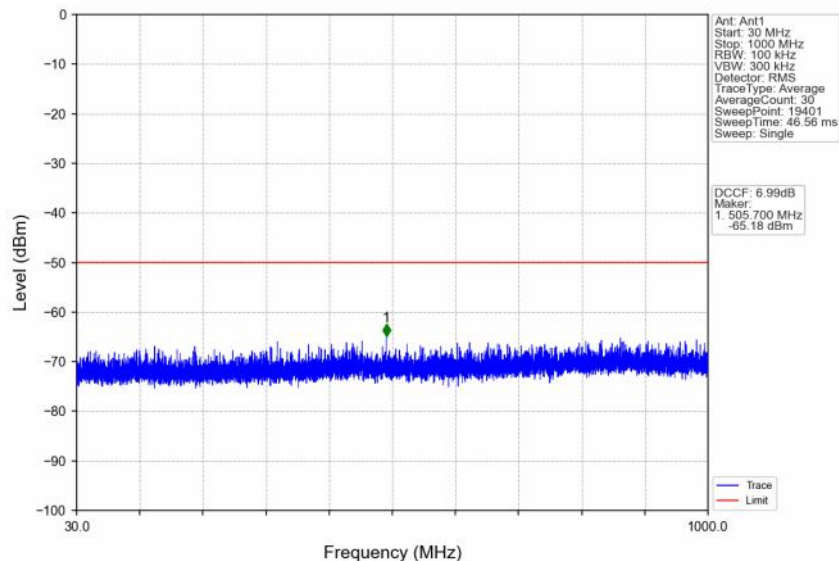
n48_30kHz_SISO_NTNV_30MHz_DFT-s-OFDM QPSK_3684.99MHz_Edge_1RB_Right
