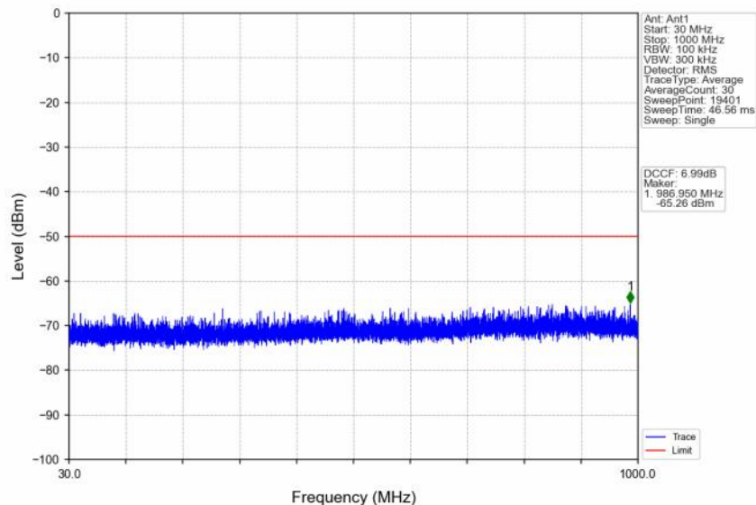
n48_30kHz_SISO_NTNV_30MHz_DFT-s-OFDM QPSK_3684.99MHz_Inner_1RB_Right
