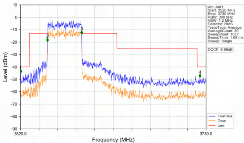
n48_30kHz_SISO_NTNV_40MHz_CP-OFDM QPSK_3570MHz_Outer_Full
