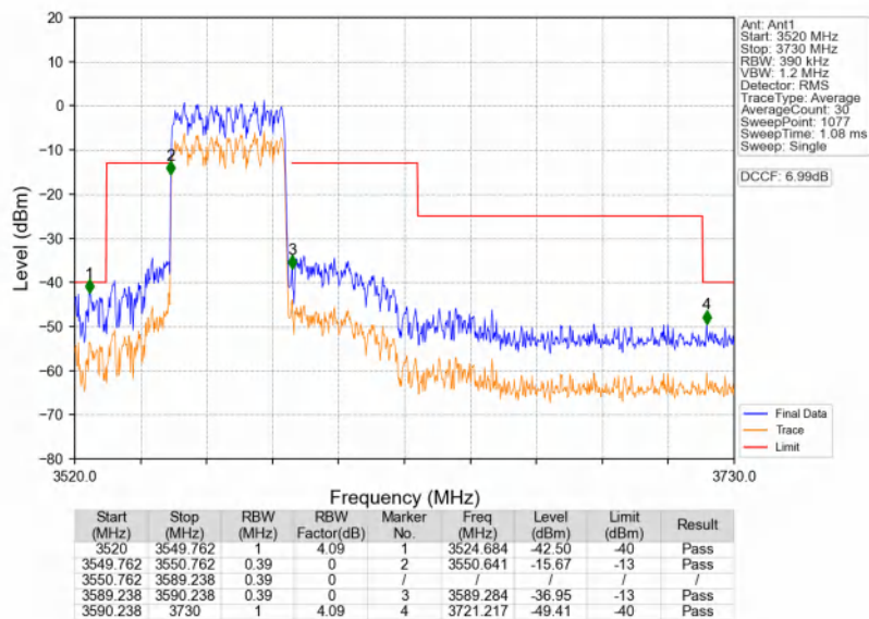
n48_30kHz_SISO_NTNV_40MHz_DFT-s-OFDM QPSK_3570MHz_Outer_Full
