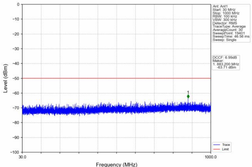
n48_30kHz_SISO_NTNV_30MHz_CP-OFDM QPSK_3684.99MHz_Inner_1RB_Right
