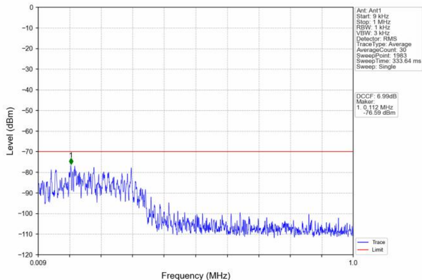
n48_30kHz_SISO_NTNV_40MHz_DFT-s-OFDM_QPSK_3570MHz_Edge_1RB_Left
