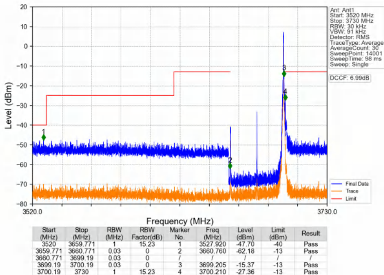
n48_30kHz_SISO_NTNV_40MHz_DFT-s-OFDM QPSK_3679.98MHz_Edge_1RB_Right
