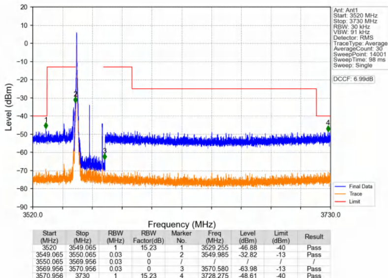
n48_30kHz_SISO_NTNV_20MHz_CP-OFDM QPSK_3560.01MHz_Edge_1RB_Left
