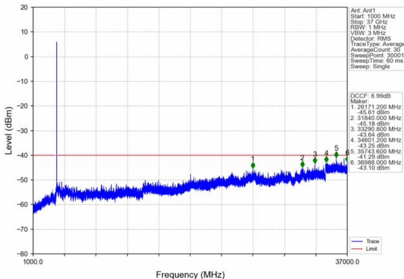
n48_30kHz_SISO_NTNV_10MHz_DFT-s-OFDM QPSK_3694.98MHz_Inner_1RB_Right
