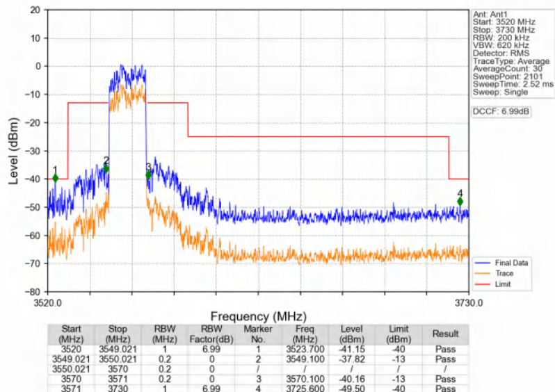
n48_30kHz_SISO_NTNV_20MHz_DFT-s-OFDM QPSK_3560.01MHz_Outer_Full
