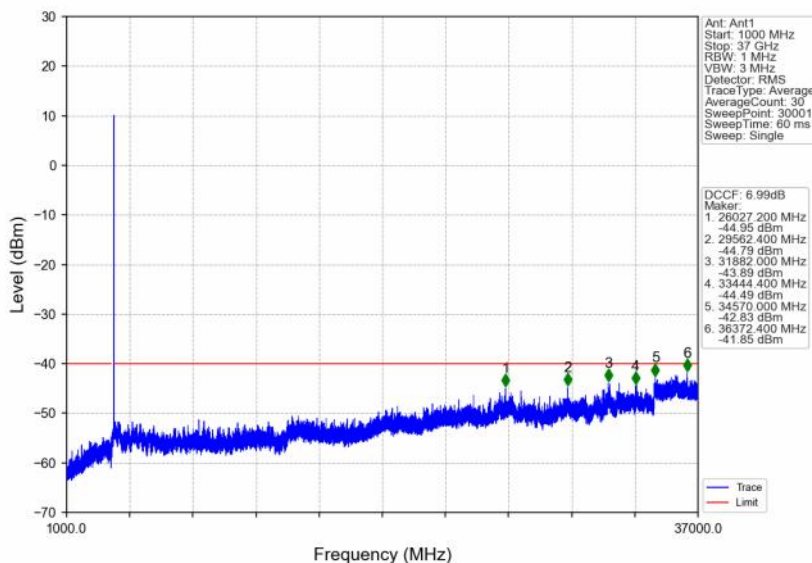
n48_30kHz_SISO_NTV_10MHz_CP-OFDM QPSK_3694.98MHz_Outer_Full
