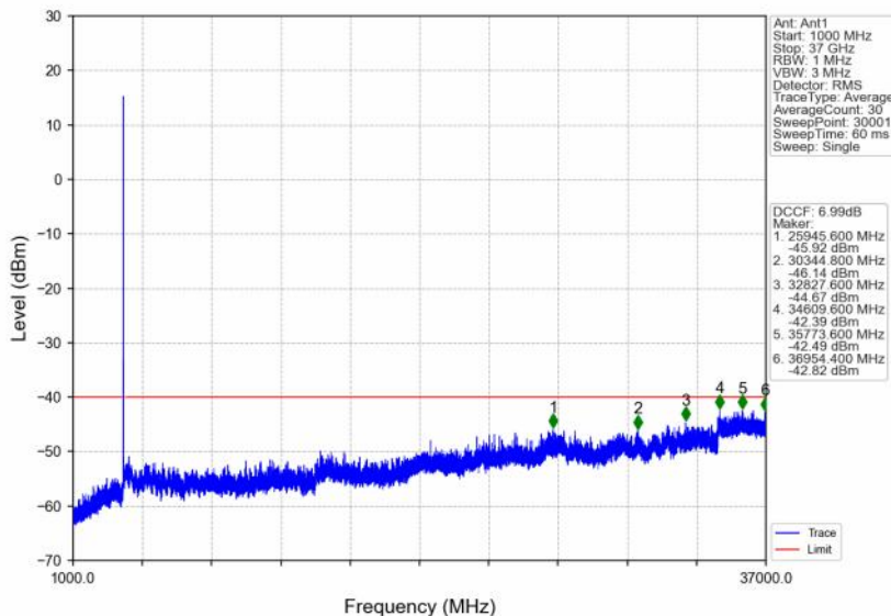
n48_30kHz_SISO_NTNV_10MHz_DFT-s-OFDM QPSK_3694.98MHz_Edge_1RB_Right
