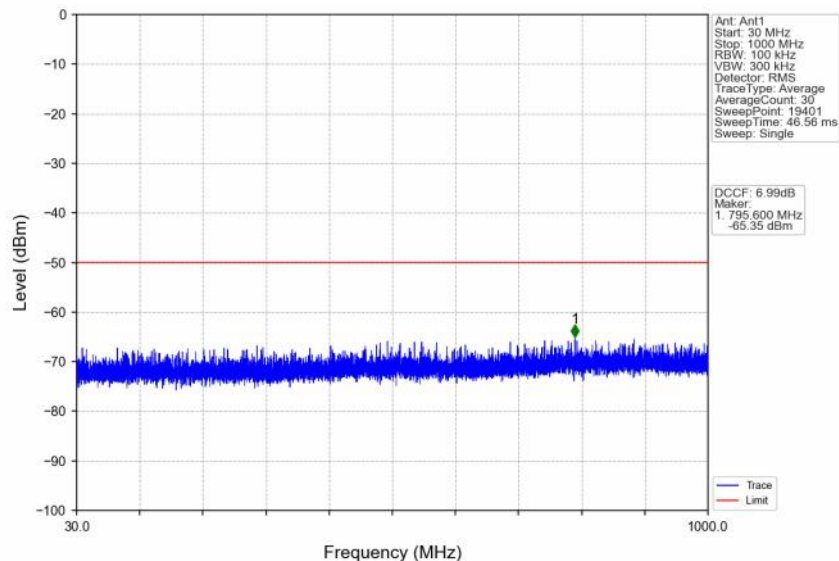
n48_30kHz_SISO_NTNV_20MHz_DFT-s-OFDM QPSK_3690MHz_Edge_1RB_Right
