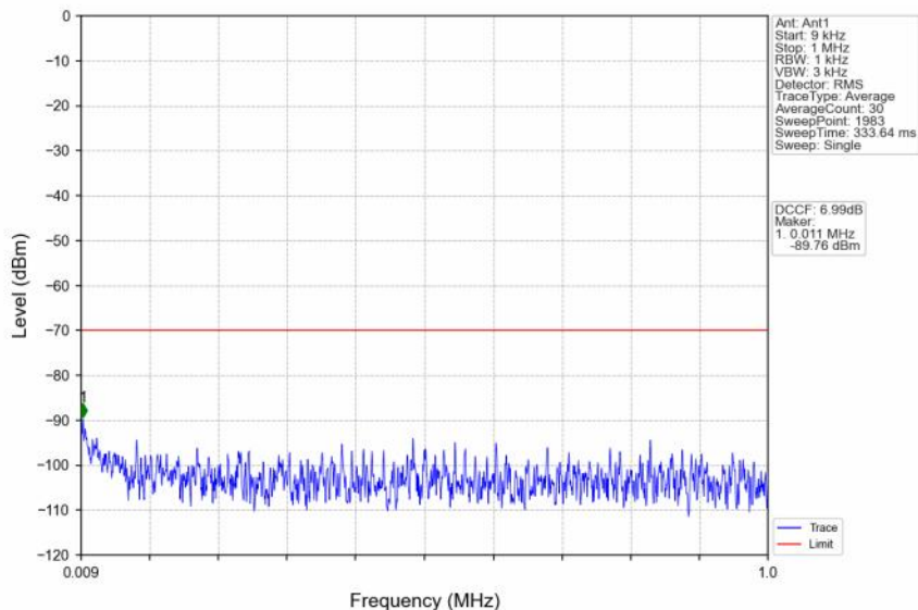
n48_30kHz_SISO_NTNV_20MHz_CP-OFDM QPSK_3690MHz_Outer_Full
