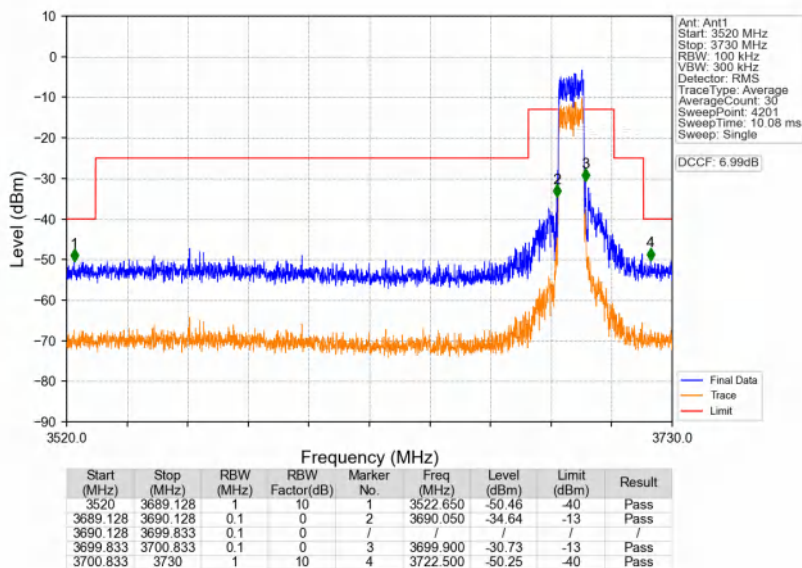
n48_30kHz_SISO_NTV_10MHz_CP-OFDM QPSK_3694.98MHz_Outer_Full
