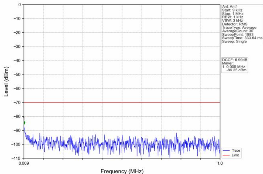
n48_30kHz_SISO_NTNV_20MHz_CP-OFDM QPSK_3560.01MHz_Outer_Full
