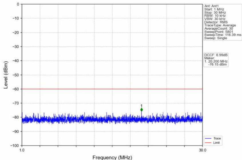
n48_30kHz_SISO_NTNV_20MHz_DFT-s-OFDM QPSK_3624.99MHz_Edge_1RB_Left
