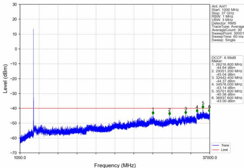
n48_30kHz_SISO_NTNV_20MHz_CP-OFDM QPSK_3560.01MHz_Outer_Full
