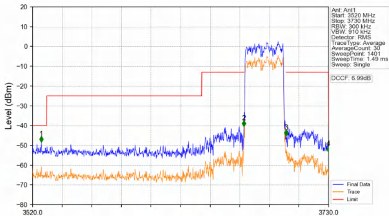
n48_30kHz_SISO_NTNV_30MHz_DFT-s-OFDM PI/2 BPSK_3684.99MHz_Outer_Full
