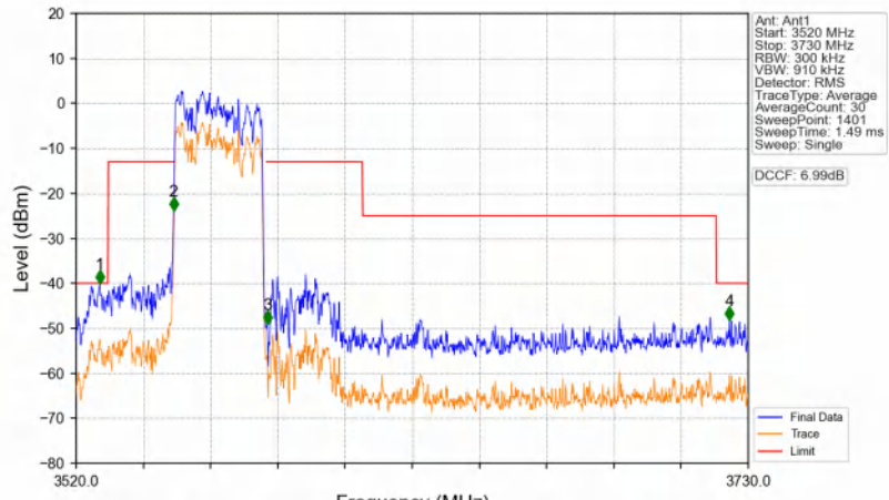
n48_30kHz_SISO_NTNV_30MHz_DFT-s-OFDM PI/2 BPSK_3565.02MHz_Outer_Full
