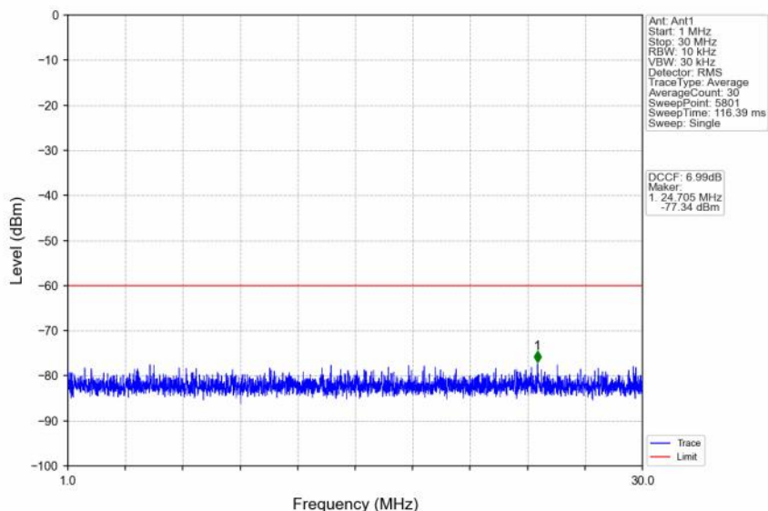
n48_30kHz_SISO_NTNV_10MHz_DFT-s-OFDM QPSK_3694.98MHz_Edge_1RB_Right
