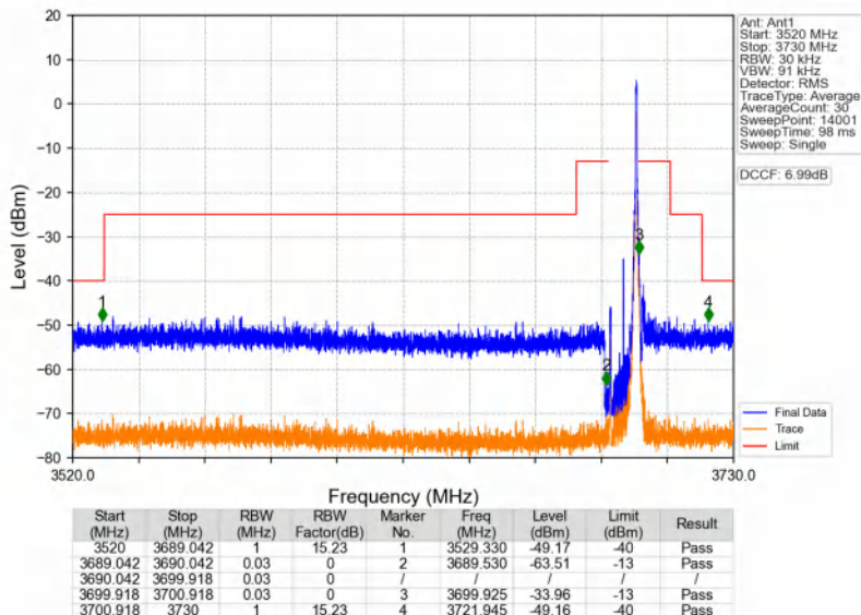
n48_30kHz_SISO_NTNV_10MHz_CP-OFDM QPSK_3694.98MHz_Edge_1RB_Right
