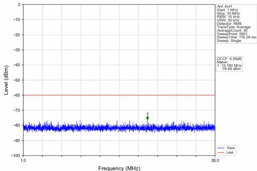
n48_30kHz_SISO_NTNV_10MHz_CP-OFDM QPSK_3694.98MHz_Inner_1RB_Right
