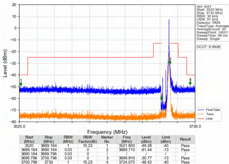
n48_30kHz_SISO_NTNV_10MHz_DFT-s-OFDM QPSK_3694.98MHz_Inner_1RB_Right
