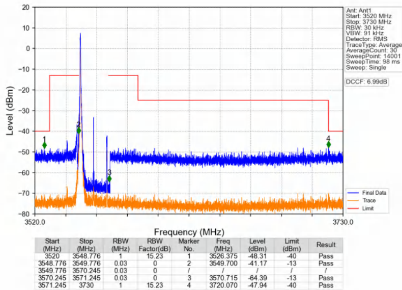
n48_30kHz_SISO_NTNV_20MHz_DFT-s-OFDM QPSK_3560.01MHz_Edge_1RB_Left
