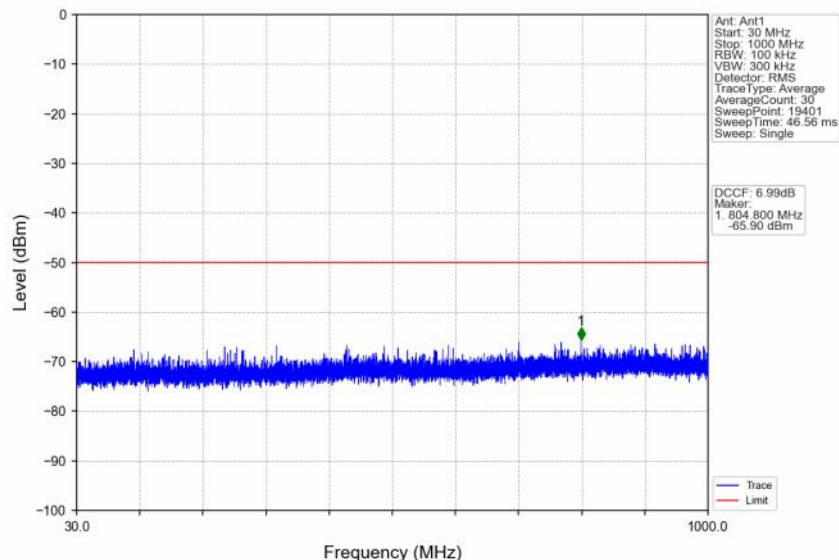
n48_30kHz_SISO_NTNV_10MHz_CP-OFDM QPSK_3694.98MHz_Inner_1RB_Right
