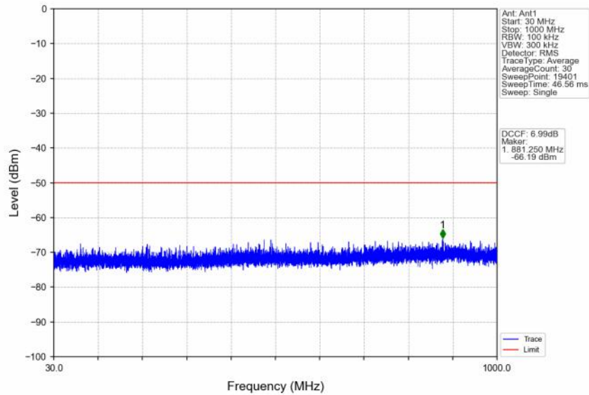
n48_30kHz_SISO_NTNV_10MHz_CP-OFDM QPSK_3624.99MHz_Edge_1RB_Left
