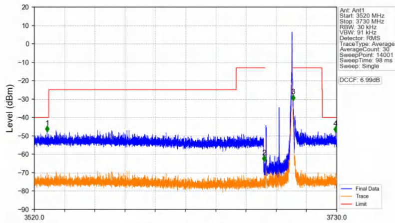
n48_30kHz_SISO_NTNV_20MHz_CP-OFDM QPSK_3690MHz_Edge_1RB_Right
