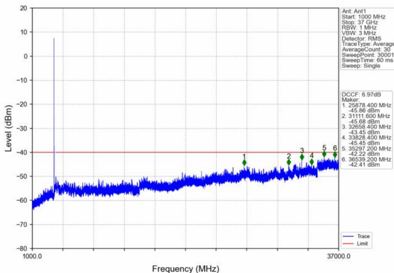
n48_30kHz_SISO_NTNV_10MHz_CP-OFDM QPSK_3555MHz_Outer_Full
