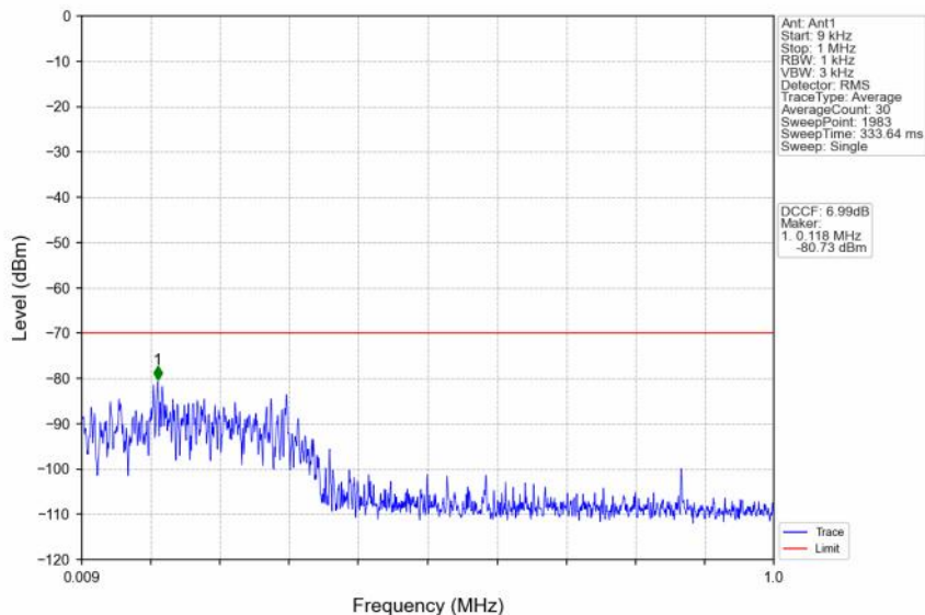
n48_30kHz_SISO_NTNV_10MHz_DFT-s-OFDM QPSK_3694.98MHz_Edge_1RB_Right
