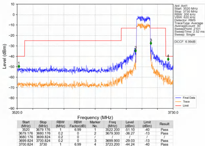
n48_30kHz_SISO_NTNV_20MHz_CP-OFDM QPSK_3690MHz_Outer_Full
