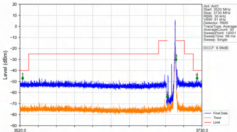
n48_30kHz_SISO_NTNV_10MHz_DFT-s-OFDM PI/2 BPSK_3694.98MHz_Edge_1RB_Right
