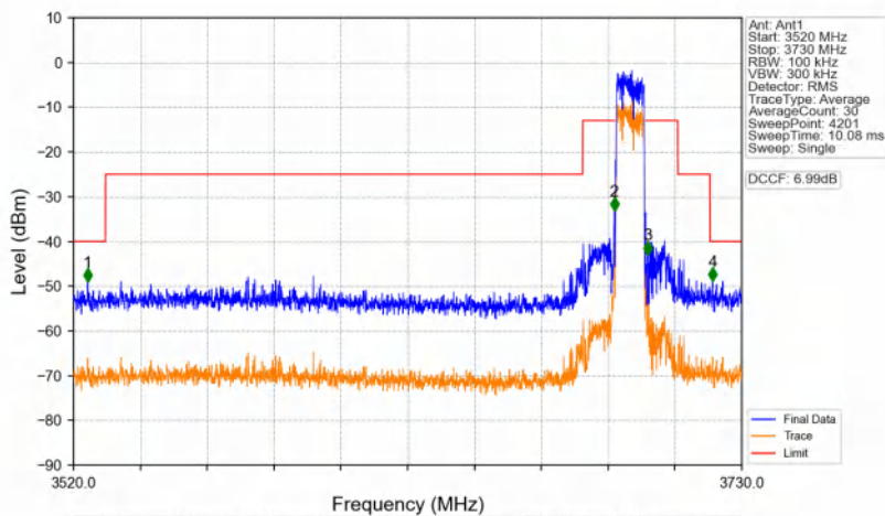
n48_30kHz_SISO_NTNV_10MHz_DFT-s-OFDM PI/2 BPSK_3694.98MHz_Outer_Full
