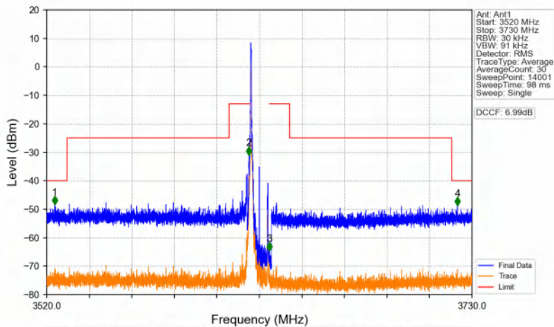
n48_30kHz_SISO_NTNV_10MHz_DFT-s-OFDM PI/2 BPSK_3624.99MHz_Edge_1RB_Left
