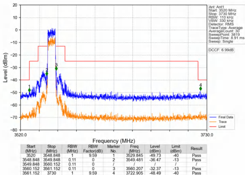
n48_30kHz_SISO_NTNV_10MHz_DFT-s-OFDM PI/2 BPSK_3555MHz_Outer_Full
