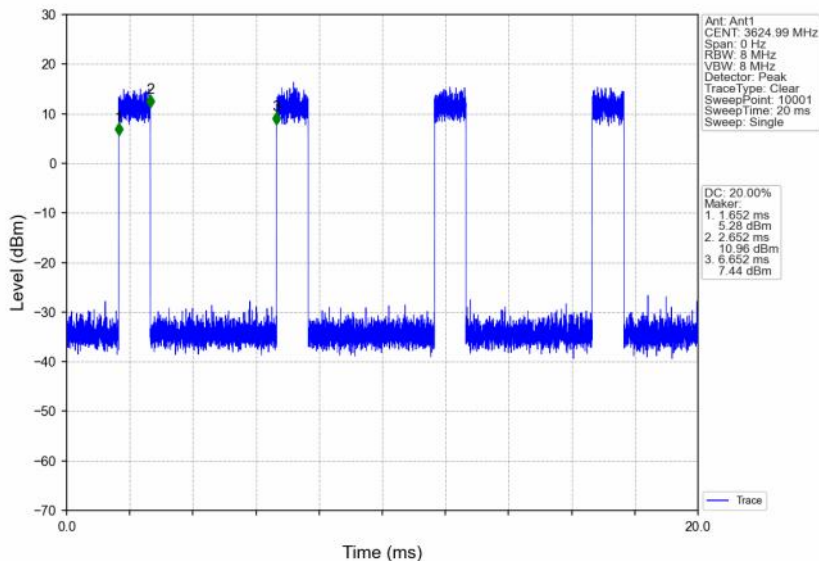
n48_30kHz_SISO_NTNV_30MHz_CP-OFDM 256 QAM_3624.99MHz_Inner_Full
