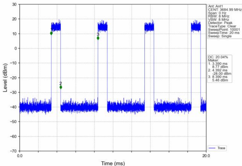
n48_30kHz_SISO_NTNV_30MHz_CP-OFDM 16 QAM_3684.99MHz_Inner_Full
