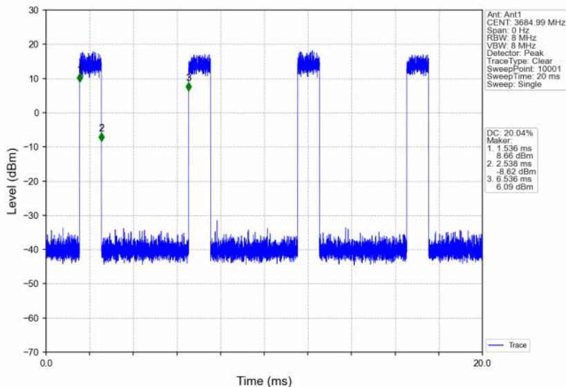
n48_30kHz_SISO_NTNV_30MHz_CP-OFDM 64 QAM_3684.99MHz_Inner_Full
