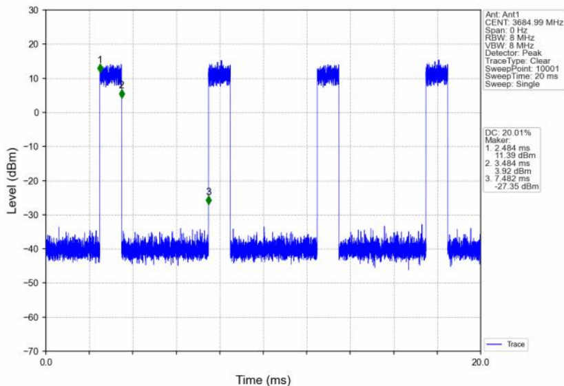
n48_30kHz_SISO_NTNV_30MHz_CP-OFDM 256 QAM_3684.99MHz_Inner_Full
