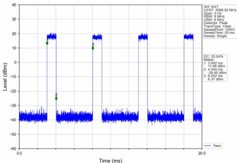
n48_30kHz_SISO_NTNV_40MHz_DFT-s-OFDM 16 QAM_3570MHz_Inner_Full
