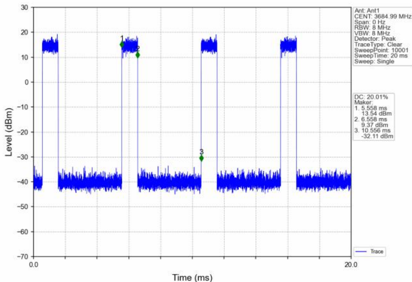
n48_30kHz_SISO_NTNV_30MHz_CP-OFDM QPSK_3684.99MHz_Inner_Full
