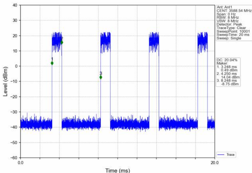
n48_30kHz_SISO_NTNV_40MHz_DFT-s-OFDM 16 QAM_3570MHz_Inner_1RB_Right
