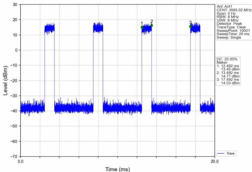
n48_30kHz_SISO_NTNV_30MHz_CP-OFDM 64 QAM_3565.02MHz_Inner_Full
