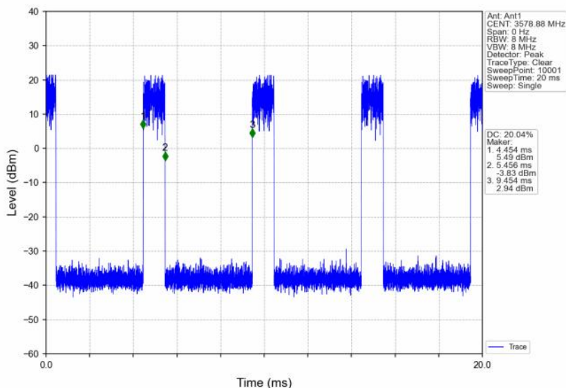
n48_30kHz_SISO_NTNV_30MHz_CP-OFDM 64 QAM_3565.02MHz_Edge_1RB_Right
