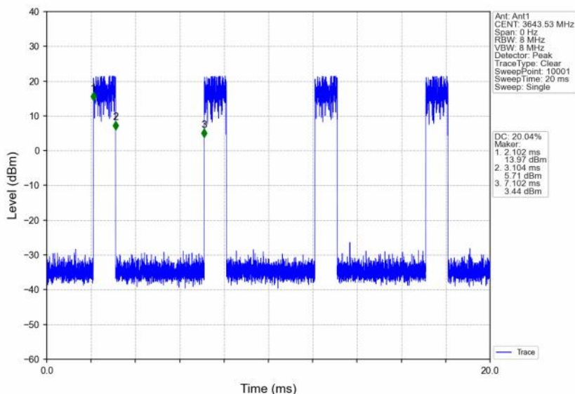
n48_30kHz_SISO_NTNV_40MHz_DFT-s-OFDM 16 QAM_3624.99MHz_Inner_1RB_Right
