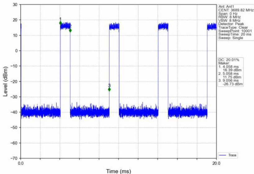
n48_30kHz_SISO_NTNV_20MHz_DFT-s-OFDM 64 QAM_3690MHz_Inner_Full
