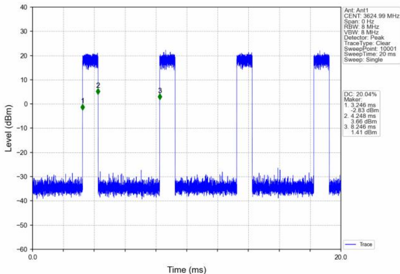
n48_30kHz_SISO_NTNV_10MHz_CP-OFDM 64 QAM_3624.99MHz_Inner_Full
