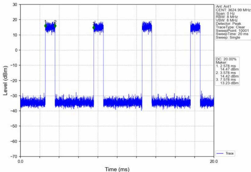
n48_30kHz_SISO_NTNV_10MHz_CP-OFDM 256 QAM_3624.99MHz_Inner_Full
