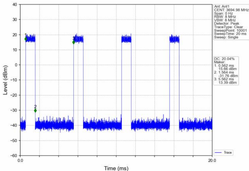
n48_30kHz_SISO_NTNV_10MHz_DFT-s-OFDM 64 QAM_3694.98MHz_Inner_Full
