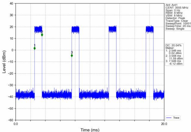
n48_30kHz_SISO_NTNV_10MHz_CP-OFDM 64 QAM_3555MHz_Inner_Full
