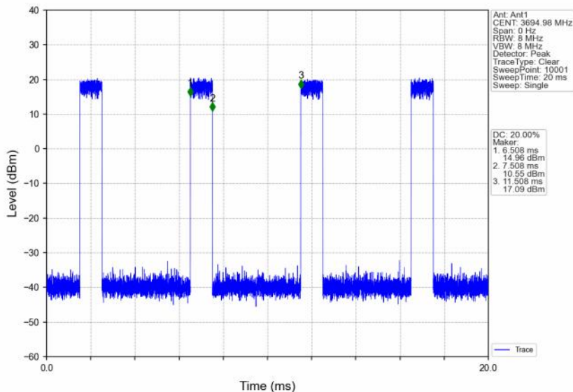
n48_30kHz_SISO_NTNV_10MHz_CP-OFDM QPSK_3694.98MHz_Inner_Full
