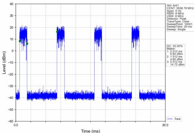
n48_30kHz_SISO_NTNV_10MHz_CP-OFDM 64 QAM_3555MHz_Inner_1RB_Right
