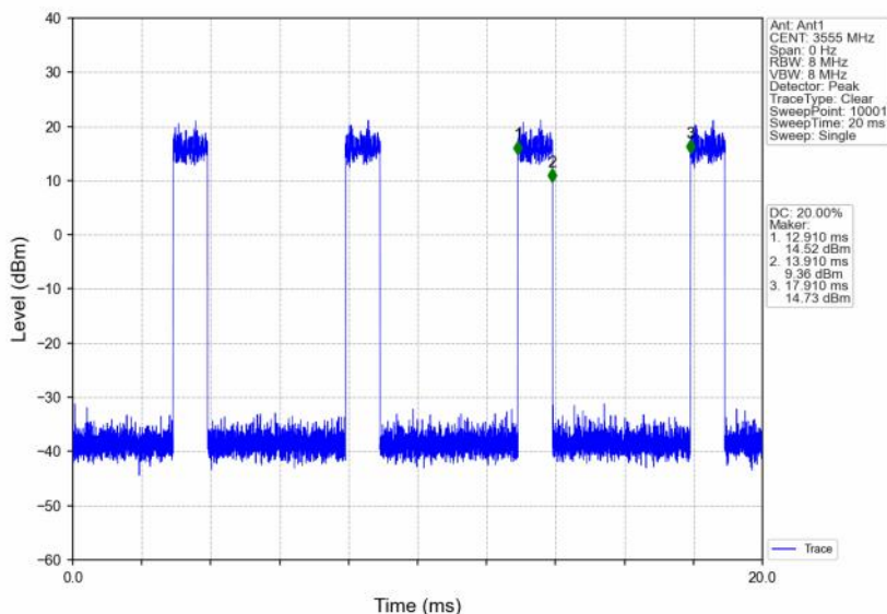
n48_30kHz_SISO_NTNV_10MHz_DFT-s-OFDM 256 QAM_3555MHz_Inner_Full
