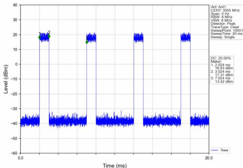
n48_30kHz_SISO_NTNV_10MHz_DFT-s-OFDM 64 QAM_3555MHz_Inner_Full
