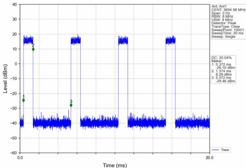
n48_30kHz_SISO_NTNV_10MHz_DFT-s-OFDM 256 QAM_3694.98MHz_Inner_Full
