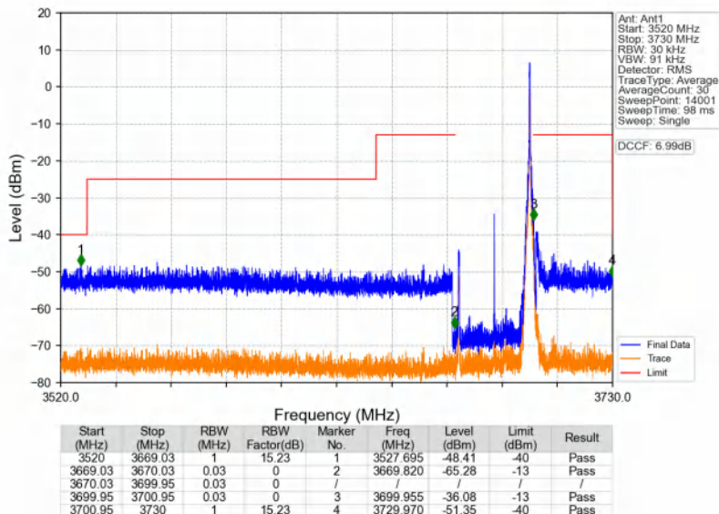
n48_30kHz_SISO_NTV_30MHz_CP-OFDM QPSK_3684.99MHz_Inner_1RB_Right
