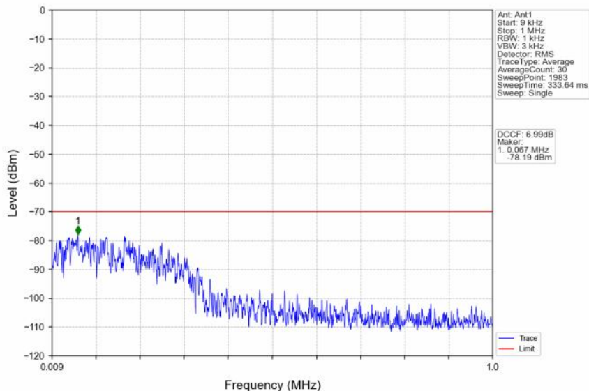
n48_30kHz_SISO_NTNV_30MHz_CP-OFDM QPSK_3624.99MHz_Edge_1RB_Left
