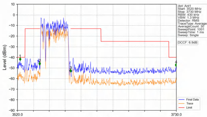
n48_30kHz_SISO_NTNV_40MHz_DFT-s-OFDM PI/2 BPSK_3570MHz_Outer_Full
