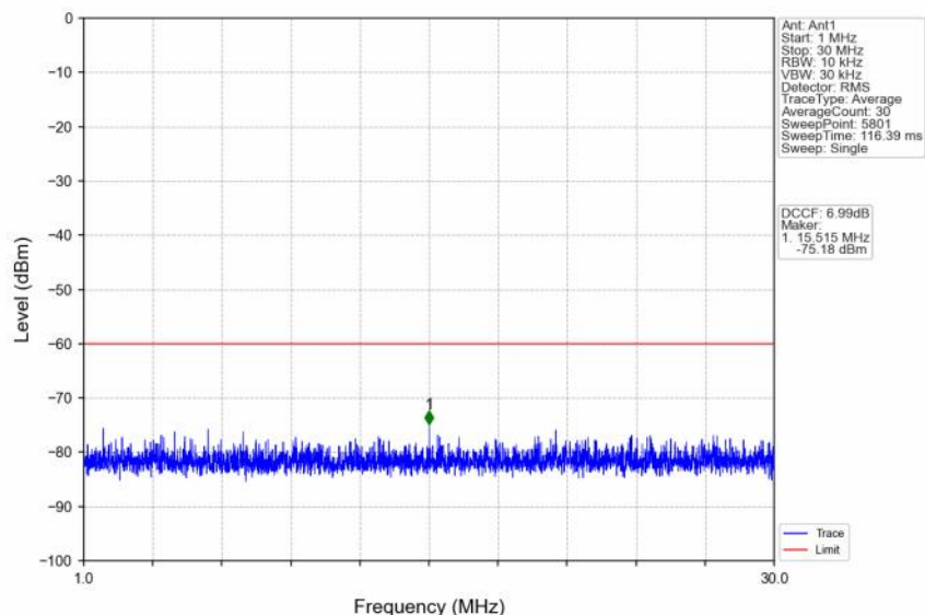
n48_30kHz_SISO_NTV_30MHz_DFT-s-OFDM QPSK_3684.99MHz_Edge_1RB_Right
