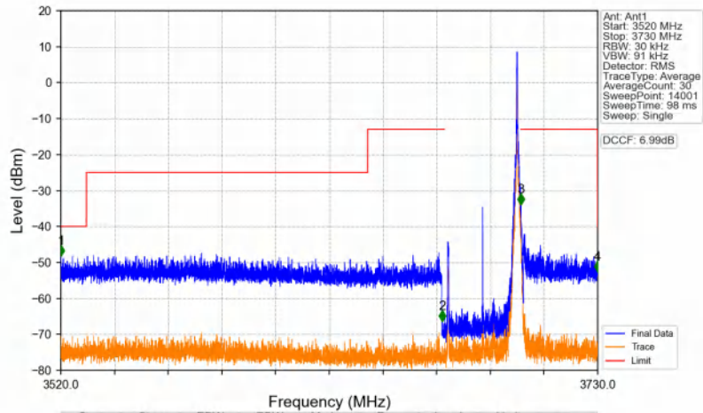
n48_30kHz_SISO_NTNV_30MHz_DFT-s-OFDM QPSK_3684.99MHz_Inner_1RB_Right
