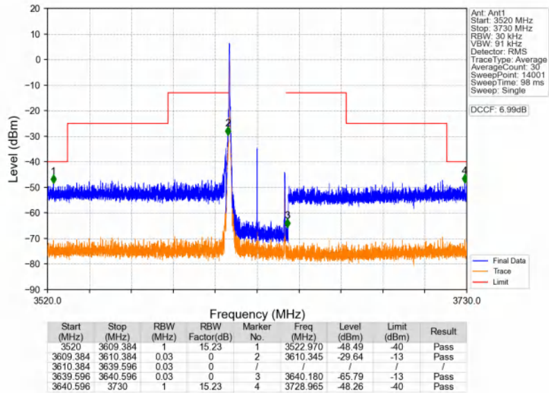
n48_30kHz_SISO_NTNV_30MHz_CP-OFDM QPSK_3624.99MHz_Edge_1RB_Left
