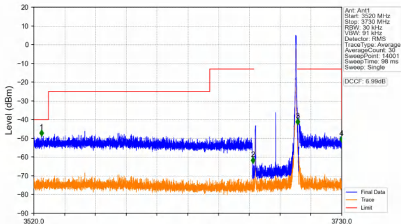
n48_30kHz_SISO_NTNV_30MHz_CP-OFDM QPSK_3684.99MHz_Edge_1RB_Right
