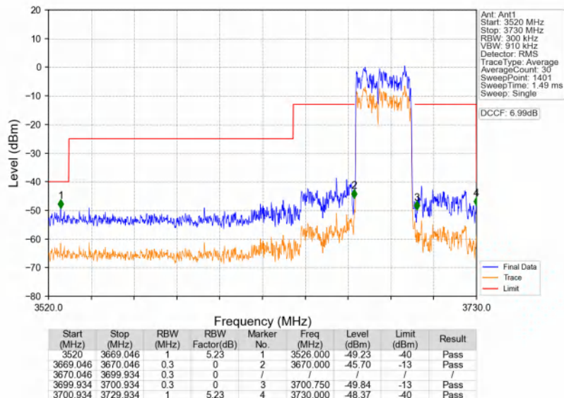
n48_30kHz_SISO_NTNV_30MHz_DFT-s-OFDM_QPSK_3684.99MHz_Outer_Full
