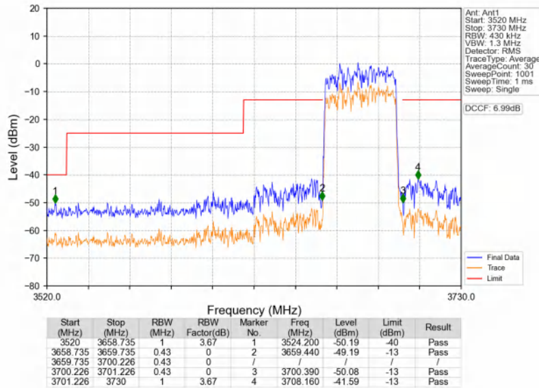
n48_30kHz_SISO_NTNV_40MHz_DFT-s-OFDM QPSK_3679.98MHz_Outer_Full
