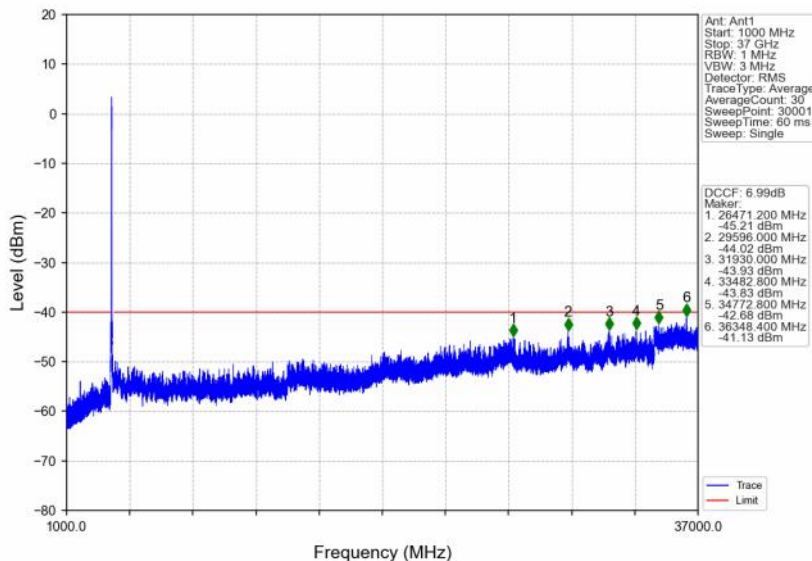
n48_30kHz_SISO_NTNV_30MHz_DFT-s-OFDM QPSK_3565.02MHz_Inner_1RB_Left
