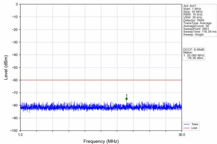
n48_30kHz_SISO_NTNV_30MHz_CP-OFDM QPSK_3565.02MHz_Outer_Full
