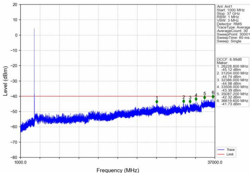
n48_30kHz_SISO_NTNV_30MHz_CP-OFDM QPSK_3565.02MHz_Outer_Full
