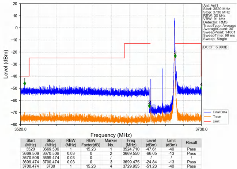
n48_30kHz_SISO_NTNV_30MHz_DFT-s-OFDM QPSK_3684.99MHz_Edge_1RB_Right
