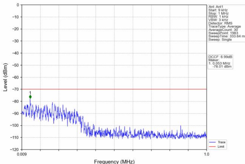
n48_30kHz_SISO_NTNV_30MHz_CP-OFDM QPSK_3684.99MHz_Edge_1RB_Right
