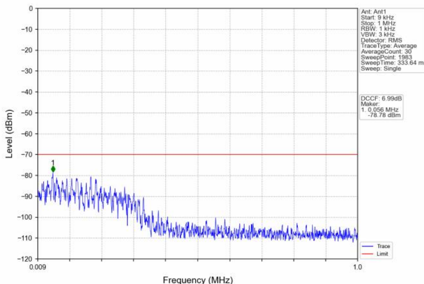
n48_30kHz_SISO_NTNV_40MHz_CP-OFDM QPSK_3679.98MHz_Edge_1RB_Right
