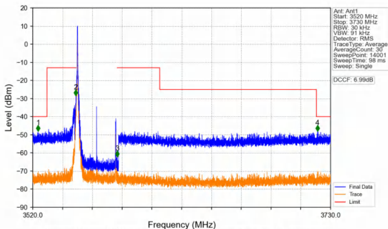
n48_30kHz_SISO_NTNV_30MHz_DFT-s-OFDM QPSK_3565.02MHz_Inner_1RB_Left
