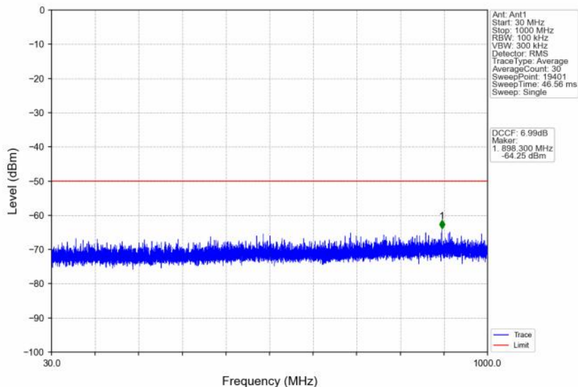
n48_30kHz_SISO_NTNV_30MHz_DFT-s-OFDM QPSK_3565.02MHz_Edge_1RB_Left
