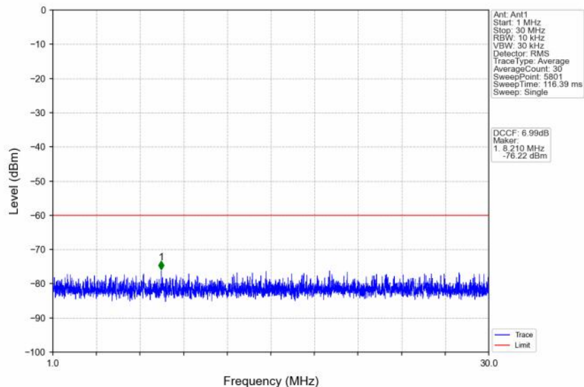
n48_30kHz_SISO_NTNV_30MHz_CP-OFDM QPSK_3565.02MHz_Edge_1RB_Left
