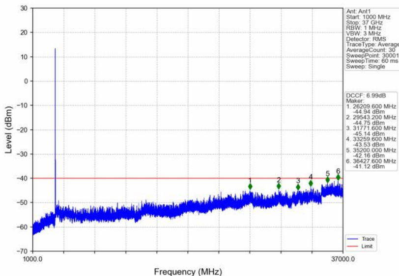
n48_30kHz_SISO_NTNV_40MHz_DFT-s-OFDM QPSK_3679.98MHz_Edge_1RB_Right
