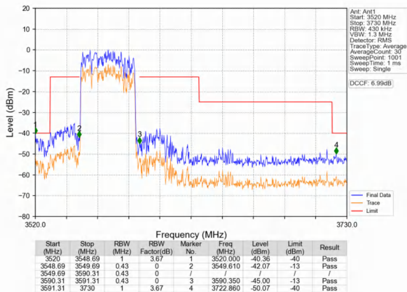
n48_30kHz_SISO_NTNV_40MHz_DFT-s-OFDM QPSK_3570MHz_Outer_Full
