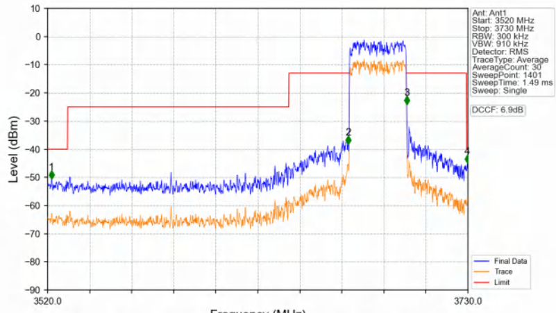
n48_30kHz_SISO_NTV_30MHz_CP-OFDM QPSK_3684.99MHz_Outer_Full
