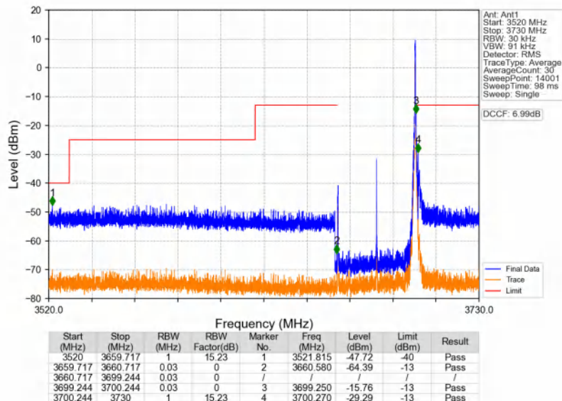
n48_30kHz_SISO_NTNV_40MHz_DFT-s-OFDM PI/2 BPSK_3679.98MHz_Edge_1RB_Right
