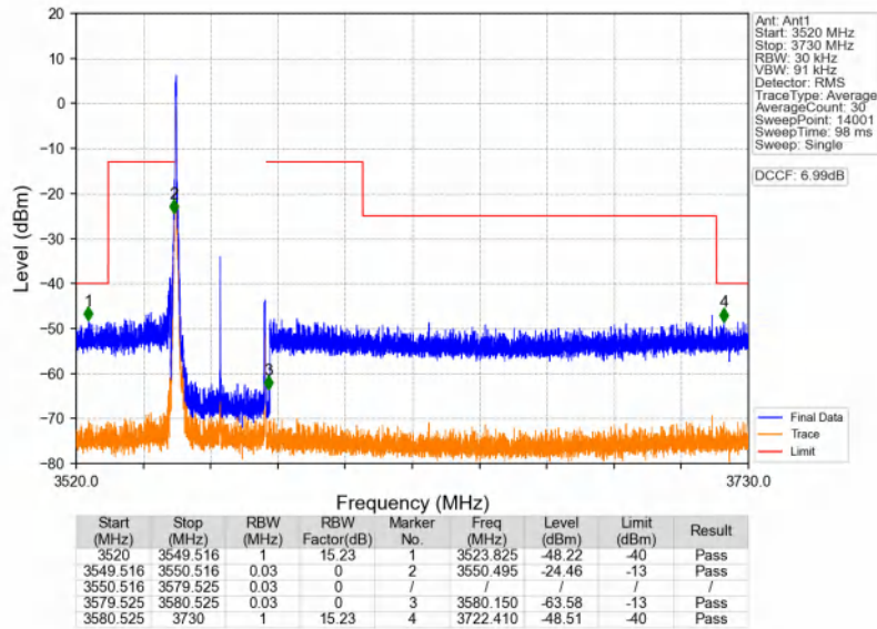
n48_30kHz_SISO_NTNV_30MHz_CP-OFDM QPSK_3565.02MHz_Edge_1RB_Left
