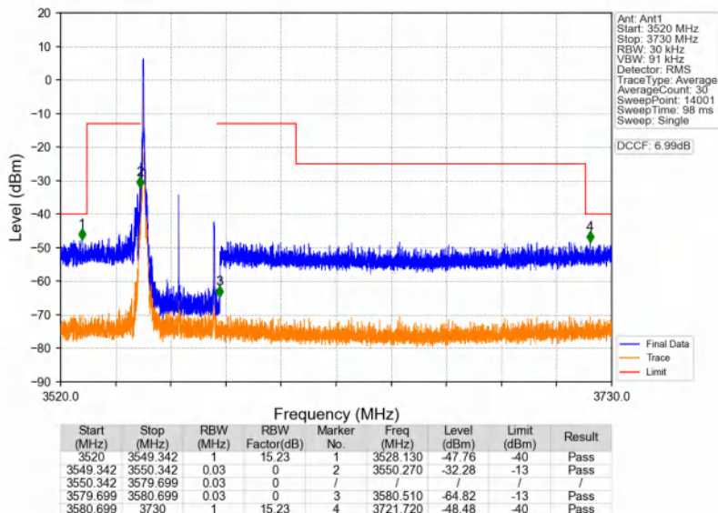
n48_30kHz_SISO_NTNV_30MHz_CP-OFDM QPSK_3565.02MHz_Inner_1RB_Left
