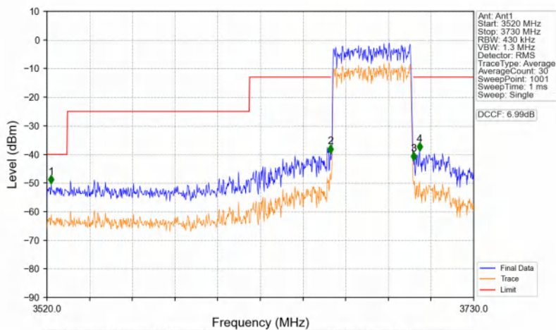
n48_30kHz_SISO_NTNV_40MHz_CP-OFDM QPSK_3679.98MHz_Outer_Full
