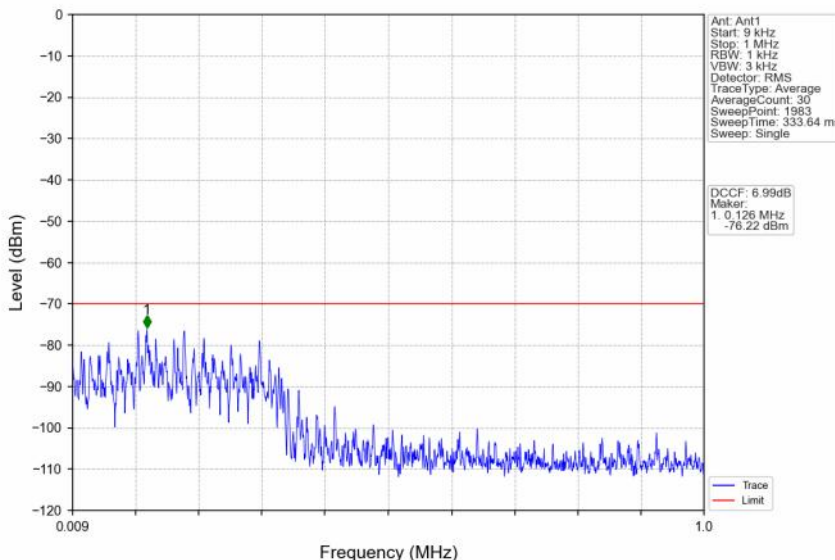
n48_30kHz_SISO_NTNV_30MHz_DFT-s-OFDM QPSK_3624.99MHz_Edge_1RB_Left
