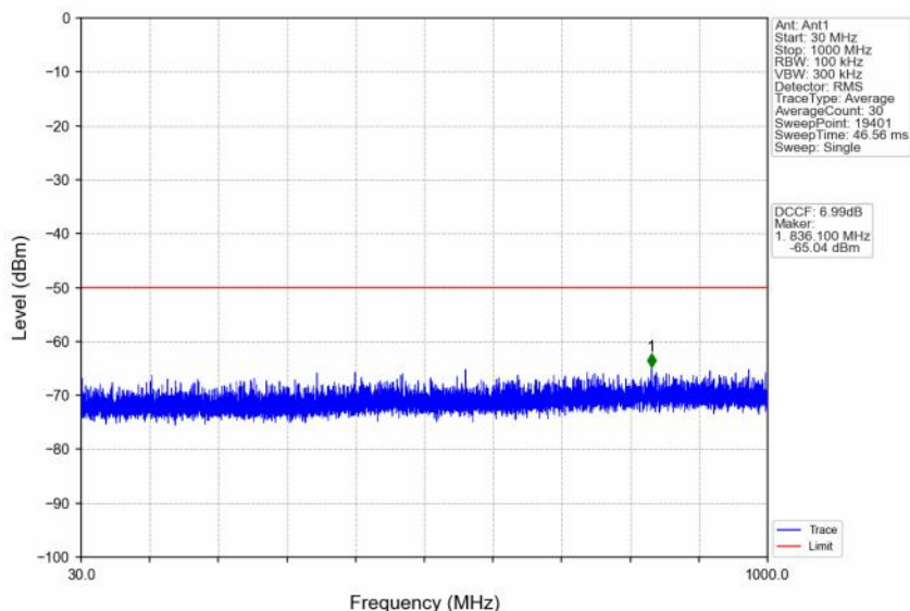
n48_30kHz_SISO_NTNV_30MHz_CP-OFDM QPSK_3684.99MHz_Inner_1RB_Right
