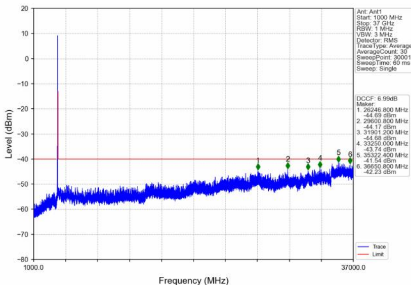
n48_30kHz_SISO_NTNV_40MHz_CP-OFDM QPSK_3679.98MHz_Outer_Full
