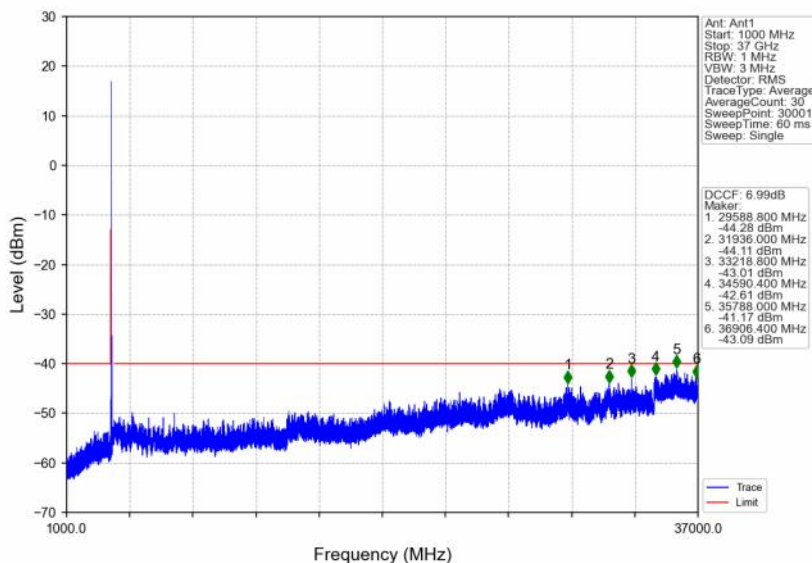
n48_30kHz_SISO_NTNV_40MHz_CP-OFDM QPSK_3624.99MHz_Edge_1RB_Left
