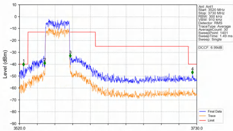
n48_30kHz_SISO_NTNV_30MHz_CP-OFDM QPSK_3565.02MHz_Outer_Full
