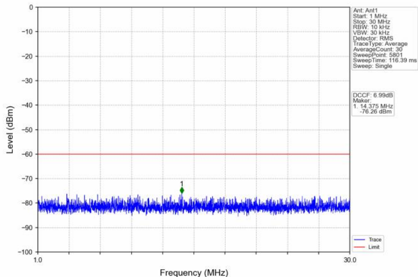
n48_30kHz_SISO_NTNV_40MHz_CP-OFDM QPSK_3679.98MHz_Inner_1RB_Right
