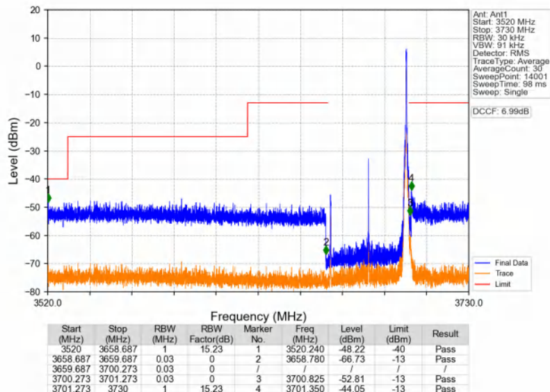
n48_30kHz_SISO_NTNV_40MHz_CP-OFDM QPSK_3679.98MHz_Edge_1RB_Right
