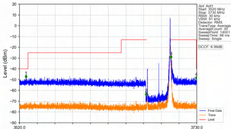
n48_30kHz_SISO_NTNV_30MHz_DFT-s-OFDM PI/2 BPSK_3684.99MHz_Inner_1RB_Right
