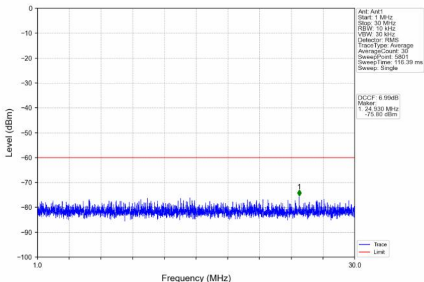
n48_30kHz_SISO_NTNV_30MHz_DFT-s-OFDM QPSK_3565.02MHz_Inner_1RB_Left
