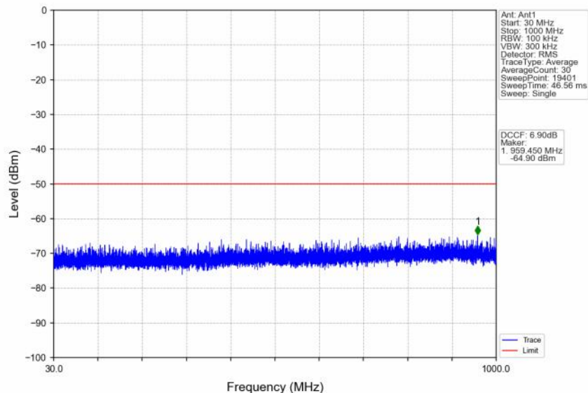
n48_30kHz_SISO_NTNV_30MHz_CP-OFDM QPSK_3684.99MHz_Outer_Full
