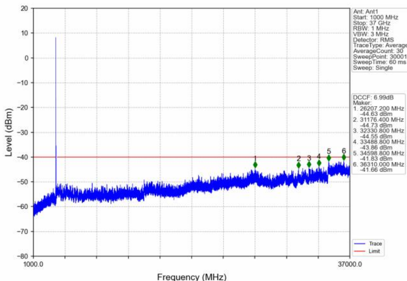
n48_30kHz_SISO_NTNV_30MHz_DFT-s-OFDM QPSK_3565.02MHz_Edge_1RB_Left
