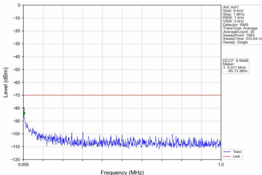
n48_30kHz_SISO_NTNV_30MHz_DFT-s-OFDM QPSK_3565.02MHz_Outer_Full
