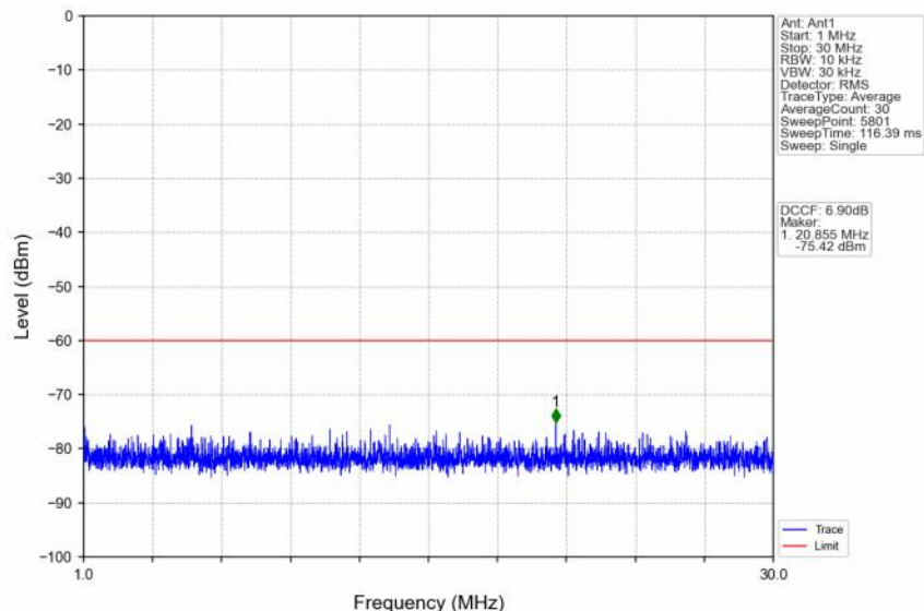
n48_30kHz_SISO_NTNV_30MHz_CP-OFDM QPSK_3684.99MHz_Outer_Full
