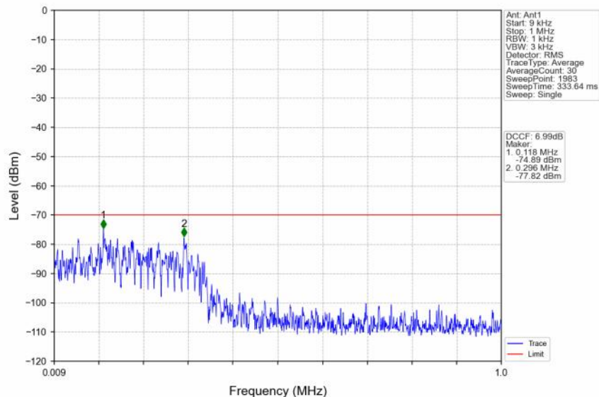
n48_30kHz_SISO_NTNV_30MHz_DFT-s-OFDM QPSK_3565.02MHz_Edge_1RB_Left
