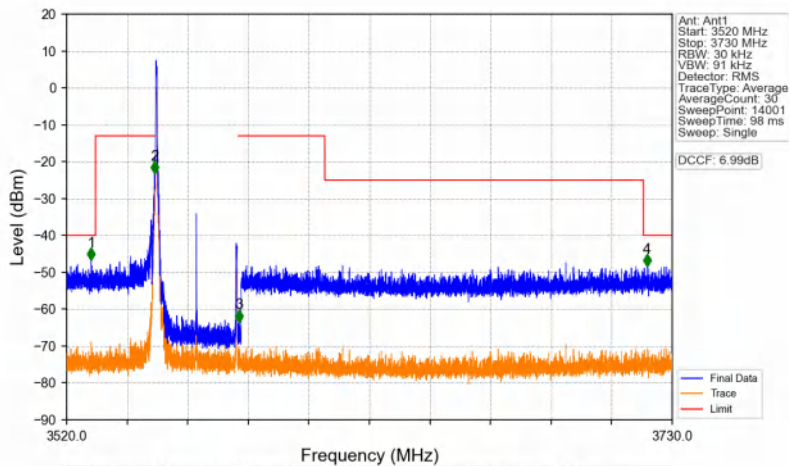
n48_30kHz_SISO_NTNV_30MHz_DFT-s-OFDM QPSK_3565.02MHz_Edge_1RB_Left
