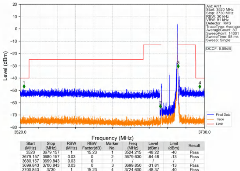
n48_30kHz_SISO_NTNV_20MHz_CP-OFDM_QPSK_3690MHz_Edge_1RB_Right
