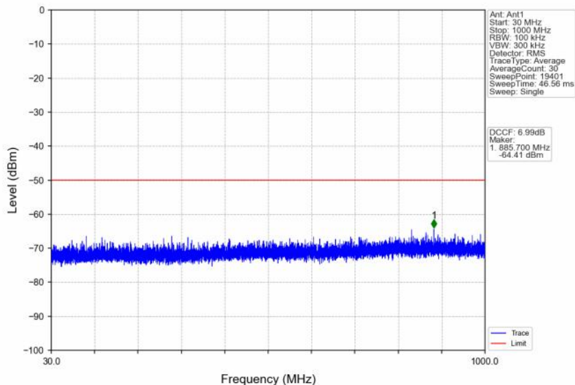
n48_30kHz_SISO_NTNV_20MHz_DFT-s-OFDM QPSK_3560.01MHz_Edge_1RB_Left
