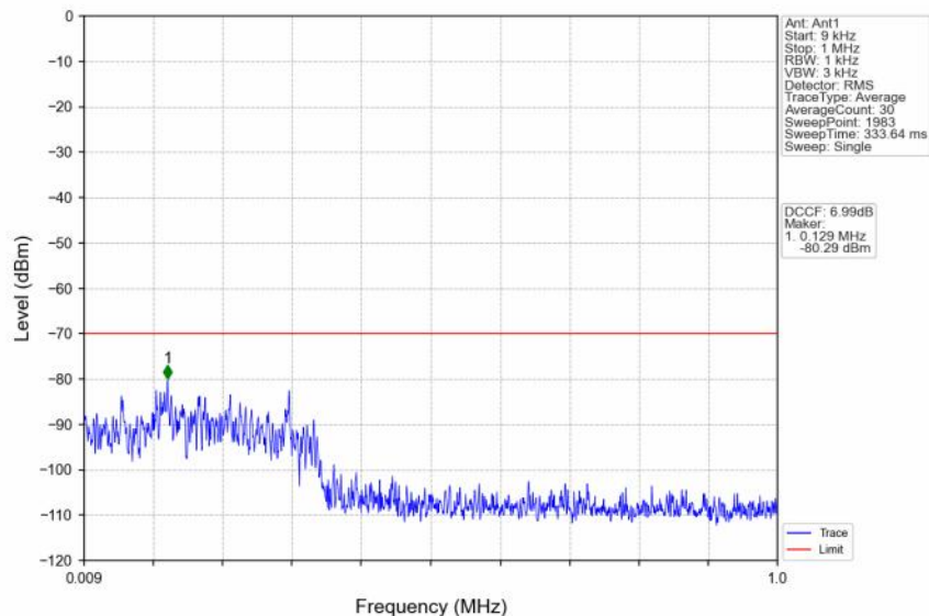
n48_30kHz_SISO_NTNV_10MHz_DFT-s-OFDM QPSK_3694.98MHz_Edge_1RB_Right
