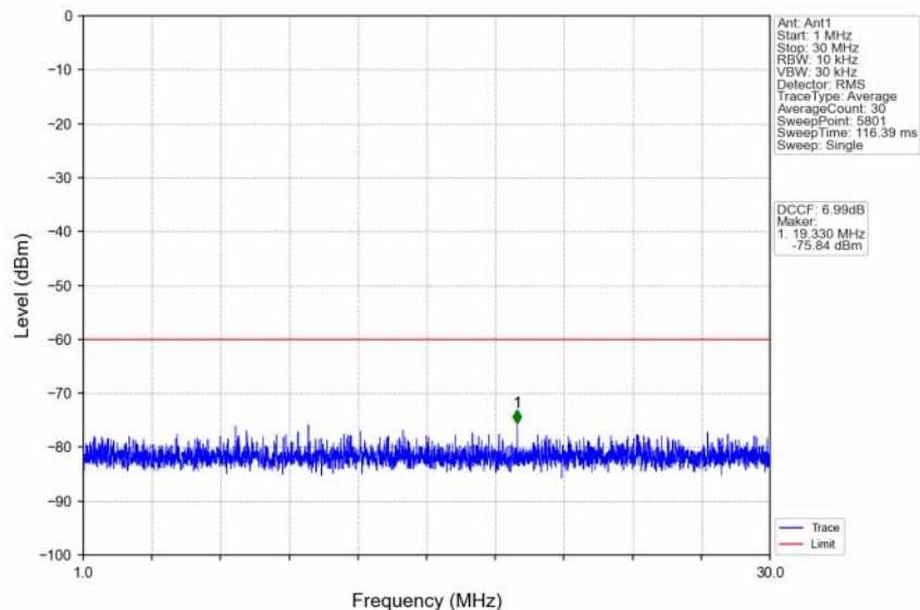
n48_30kHz_SISO_NTNV_10MHz_DFT-s-OFDM QPSK_3694.98MHz_Outer_Full
