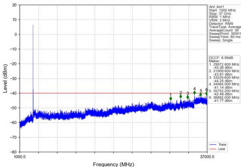
n48_30kHz_SISO_NTNV_20MHz_CP-OFDM QPSK_3560.01MHz_Outer_Full
