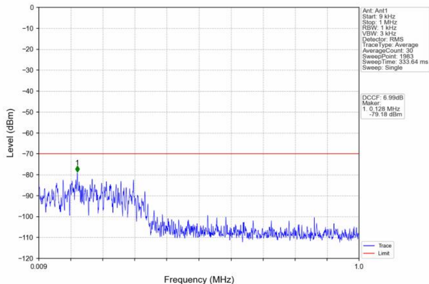
n48_30kHz_SISO_NTNV_20MHz_DFT-s-OFDM QPSK_3690MHz_Edge_1RB_Right
