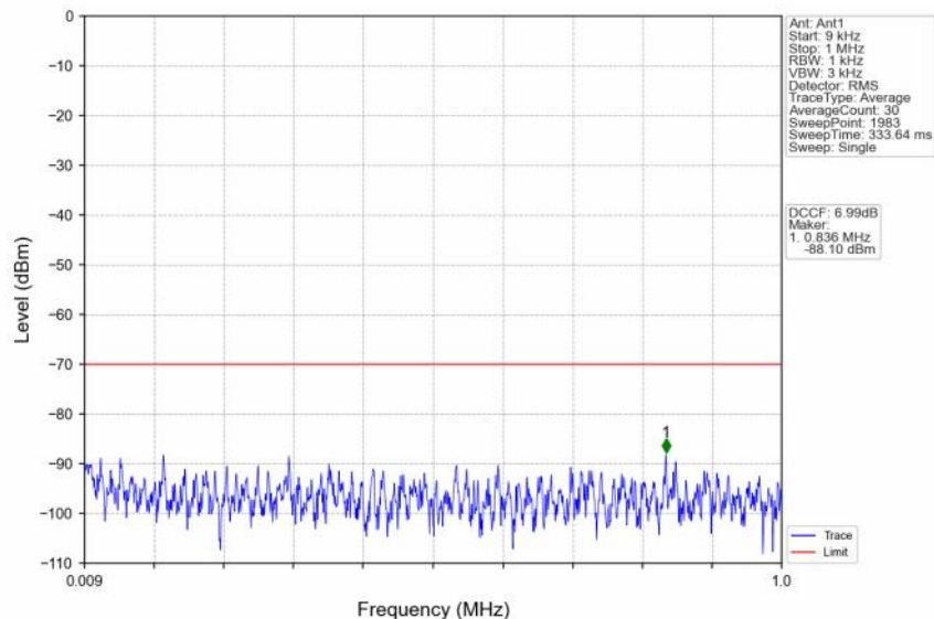
n48_30kHz_SISO_NTNV_10MHz_CP-OFDM QPSK_3555MHz_Outer_Full
