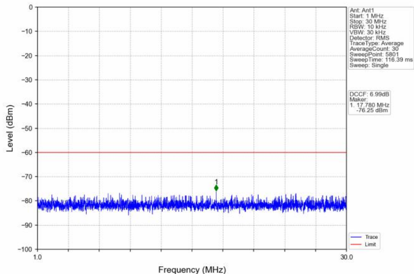
n48_30kHz_SISO_NTNV_20MHz_DFT-s-OFDM QPSK_3560.01MHz_Outer_Full
