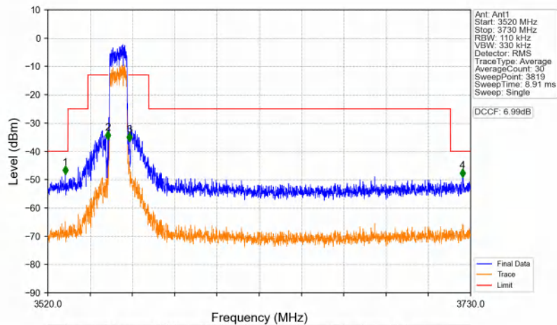
n48_30kHz_SISO_NTNV_10MHz_CP-OFDM QPSK_3555MHz_Outer_Full
