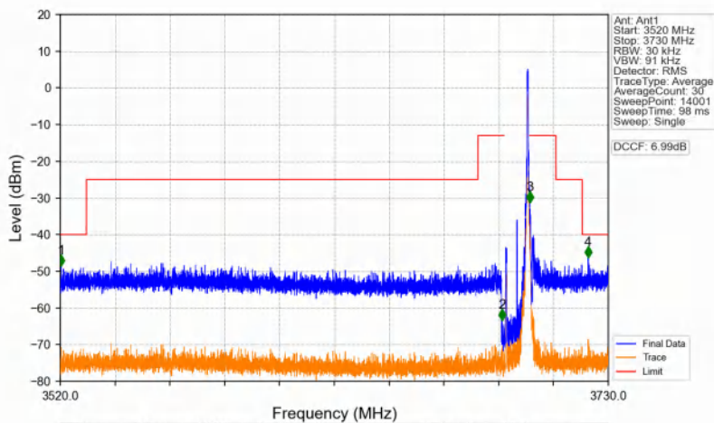
n48_30kHz_SISO_NTNV_10MHz_DFT-s-OFDM QPSK_3694.98MHz_Edge_1RB_Right
