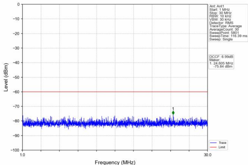
n48_30kHz_SISO_NTNV_20MHz_CP-OFDM QPSK_3690MHz_Edge_1RB_Right
