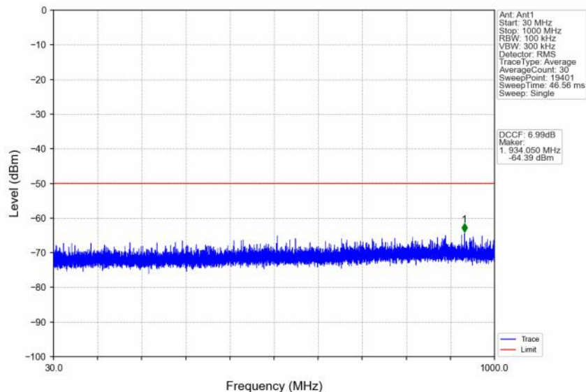
n48_30kHz_SISO_NTNV_10MHz_CP-OFDM QPSK_3694.98MHz_Outer_Full
