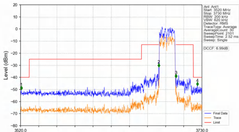
n48_30kHz_SISO_NTNV_20MHz_DFT-s-OFDM QPSK_3690MHz_Outer_Full
