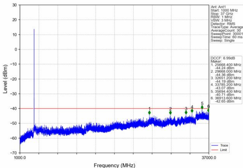
n48_30kHz_SISO_NTNV_20MHz_DFT-s-OFDM QPSK_3560.01MHz_Edge_1RB_Left
