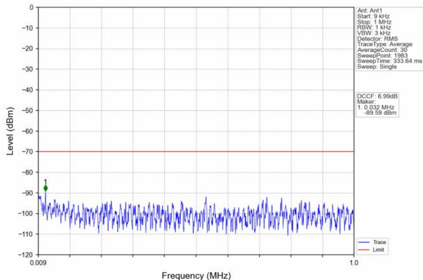
n48_30kHz_SISO_NTNV_10MHz_CP-OFDM QPSK_3694.98MHz_Outer_Full
