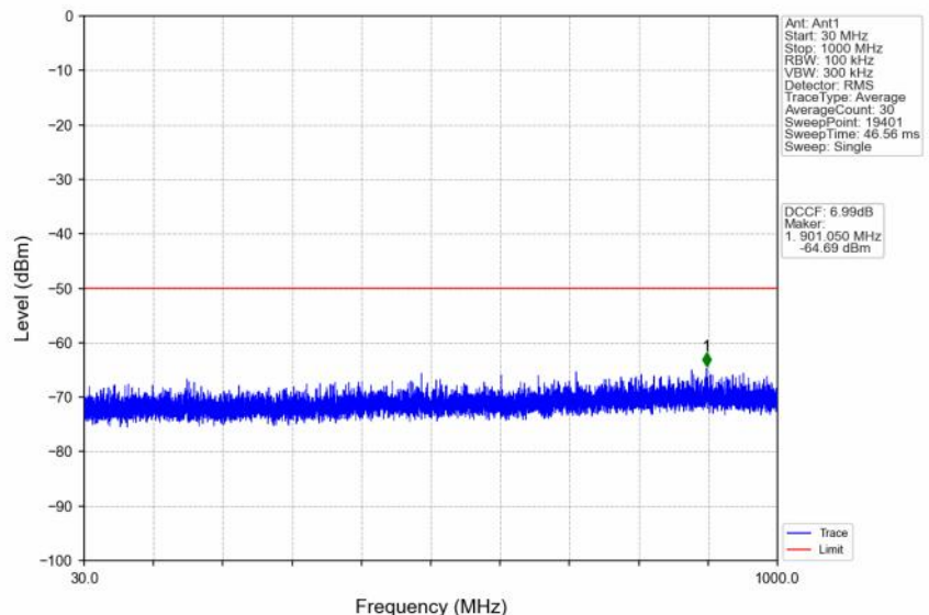
n48_30kHz_SISO_NTNV_20MHz_DFT-s-OFDM QPSK_3690MHz_Outer_Full
