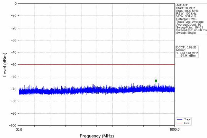
n48_30kHz_SISO_NTNV_10MHz_CP-OFDM QPSK_3555MHz_Outer_Full
