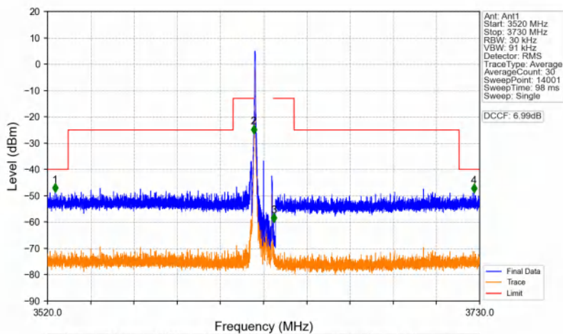
n48_30kHz_SISO_NTNV_10MHz_CP-OFDM QPSK_3624.99MHz_Edge_1RB_Left
