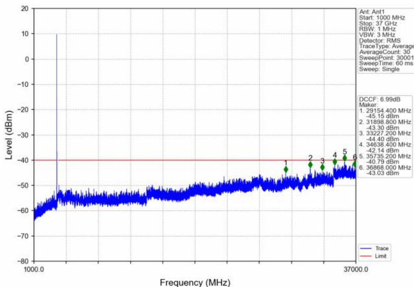
n48_30kHz_SISO_NTNV_10MHz_CP-OFDM QPSK_3624.99MHz_Edge_1RB_Left
