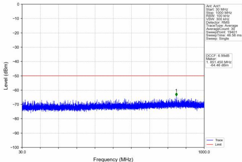
n48_30kHz_SISO_NTNV_10MHz_DFT-s-OFDM QPSK_3694.98MHz_Inner_1RB_Right
