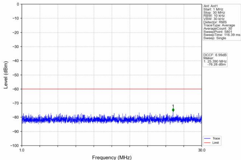
n48_30kHz_SISO_NTNV_10MHz_CP-OFDM QPSK_3694.98MHz_Edge_1RB_Right
