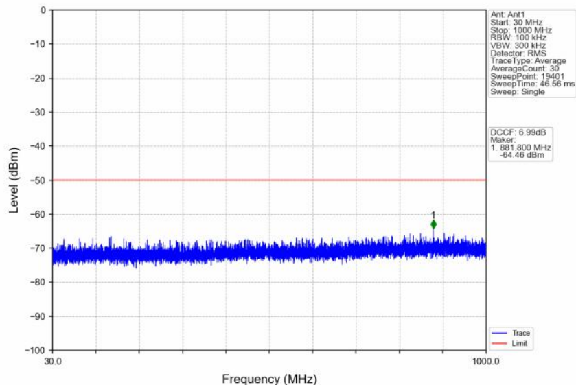
n48_30kHz_SISO_NTNV_10MHz_CP-OFDM QPSK_3624.99MHz_Edge_1RB_Left
