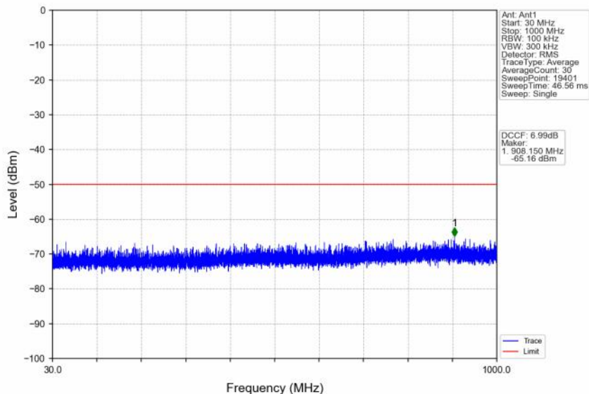
n48_30kHz_SISO_NTNV_10MHz_DFT-s-OFDM QPSK_3694.98MHz_Edge_1RB_Right
