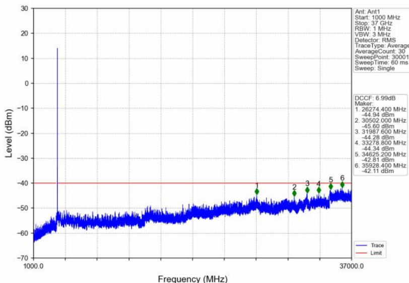
n48_30kHz_SISO_NTNV_10MHz_DFT-s-OFDM QPSK_3694.98MHz_Edge_1RB_Right
