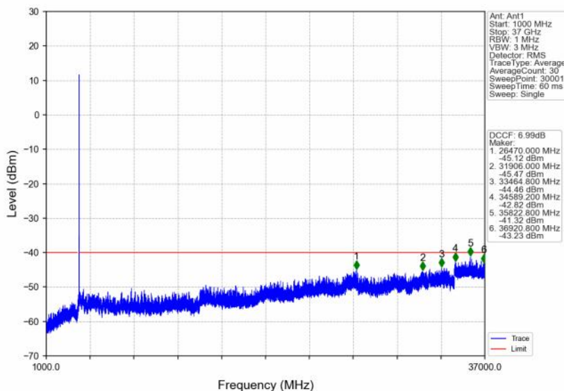
n48_30kHz_SISO_NTNV_10MHz_CP-OFDM QPSK_3694.98MHz_Outer_Full
