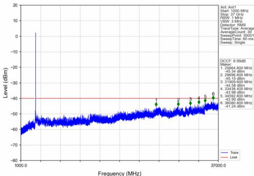
n48_30kHz_SISO_NTNV_20MHz_CP-OFDM QPSK_3690MHz_Outer_Full
