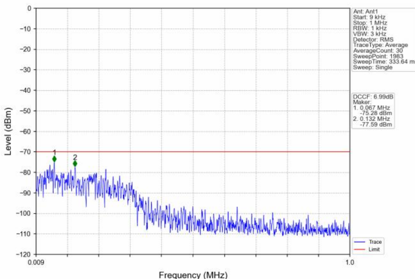
n48_30kHz_SISO_NTNV_20MHz_CP-OFDM QPSK_3560.01MHz_Edge_1RB_Left
