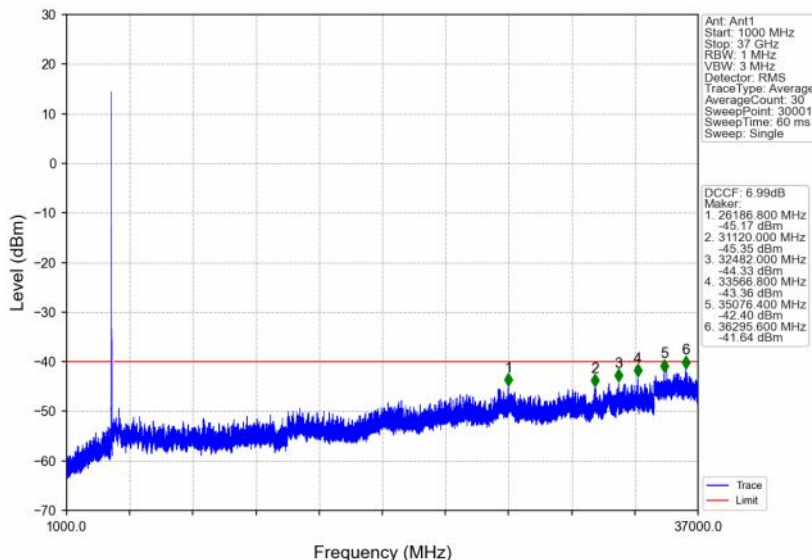
n48_30kHz_SISO_NTNV_20MHz_DFT-s-OFDM QPSK_3560.01MHz_Edge_1RB_Left
