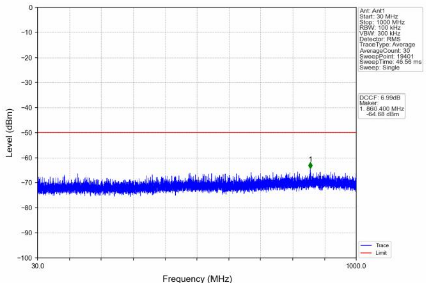
n48_30kHz_SISO_NTNV_10MHz_CP-OFDM QPSK_3694.98MHz_Inner_1RB_Right
