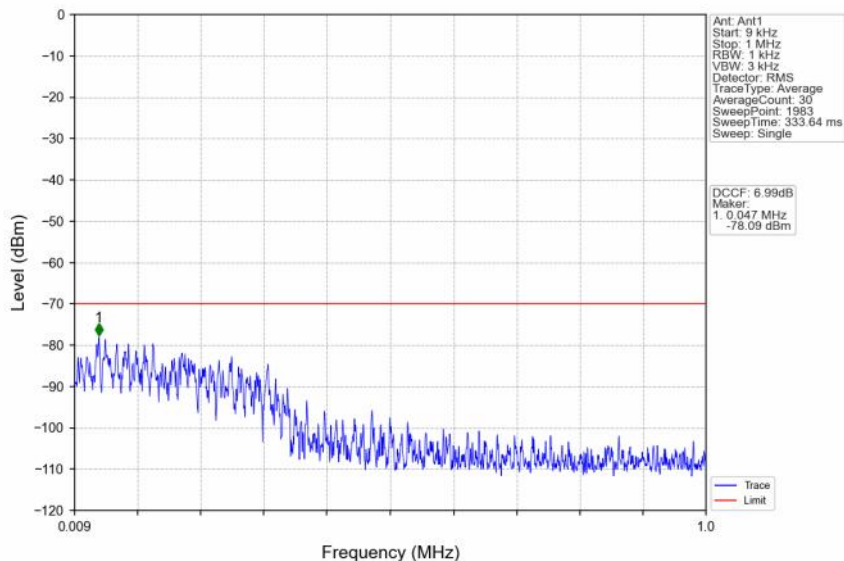
n48_30kHz_SISO_NTNV_10MHz_CP-OFDM QPSK_3624.99MHz_Edge_1RB_Left
