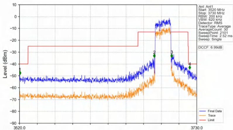
n48_30kHz_SISO_NTNV_20MHz_CP-OFDM QPSK_3690MHz_Outer_Full
