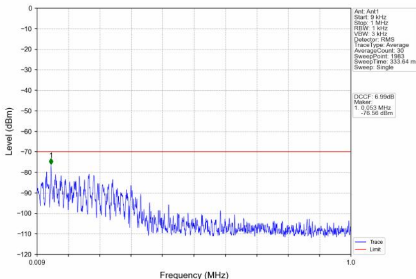
n48_30kHz_SISO_NTNV_20MHz_CP-OFDM_QPSK_3690MHz_Edge_1RB_Right
