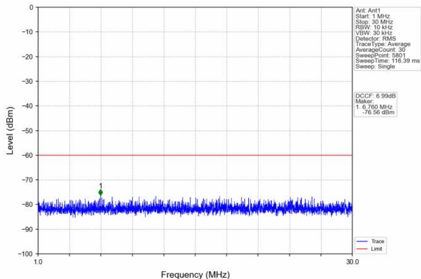
n48_30kHz_SISO_NTNV_20MHz_CP-OFDM QPSK_3560.01MHz_Edge_1RB_Left
