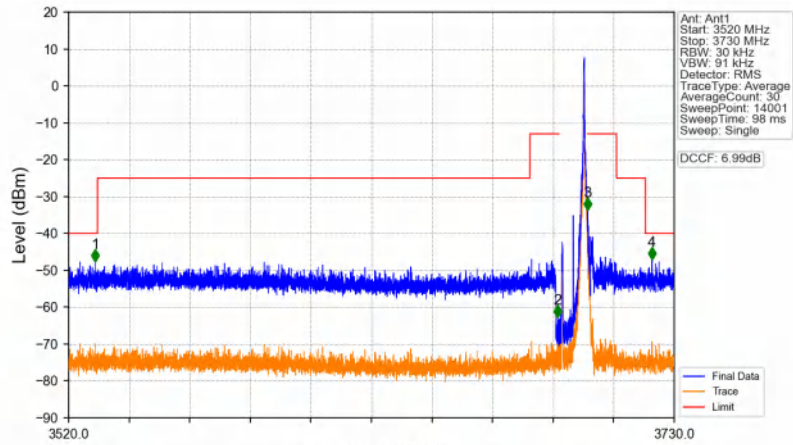
n48_30kHz_SISO_NTNV_10MHz_DFT-s-OFDM QPSK_3694.98MHz_Inner_1RB_Right
