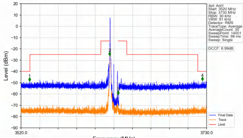
n48_30kHz_SISO_NTNV_10MHz_DFT-s-OFDM PI/2 BPSK_3624.99MHz_Edge_1RB_Left
