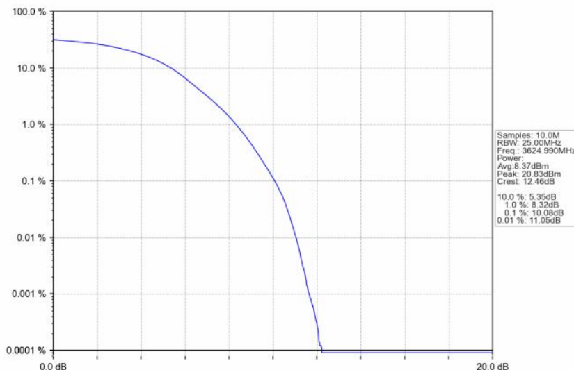
n48_30kHz_SISO_NTNV_30MHz_DFT-s-OFDM_256_QAM_3624.99MHz_Outer_Full
