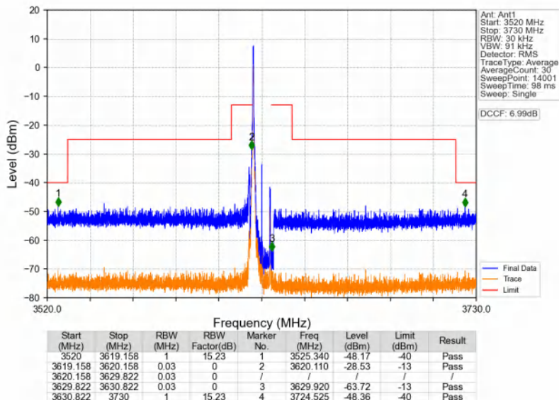
n48_30kHz_SISO_NTNV_10MHz_DFT-s-OFDM QPSK_3624.99MHz_Edge_1RB_Left
