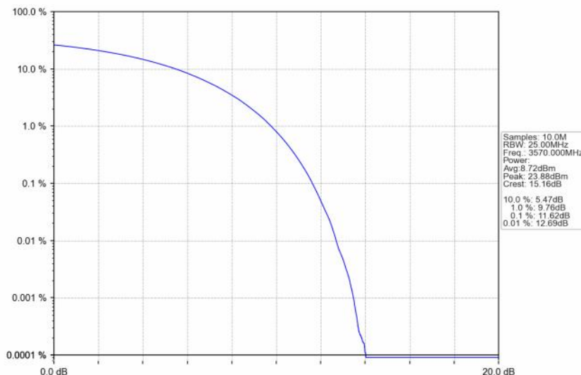
n48_30kHz_SISO_NTNV_40MHz_CP-OFDM QPSK_3570MHz_Outer_Full
