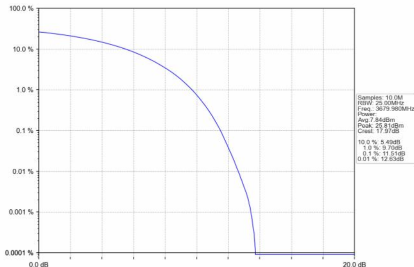
n48_30kHz_SISO_NTNV_40MHz_CP-OFDM QPSK_3679.98MHz_Outer_Full
