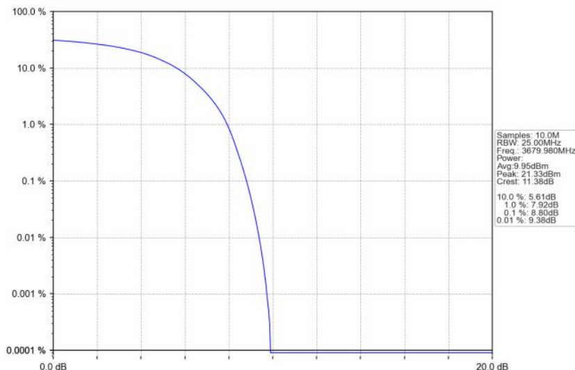
n48_30kHz_SISO_NTNV_40MHz_DFT-s-OFDM QPSK_3679.98MHz_Outer_Full
