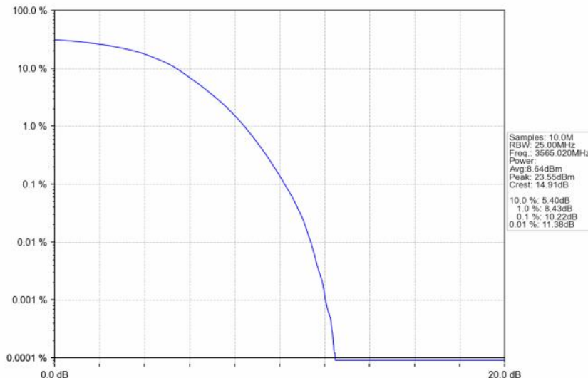
n48_30kHz_SISO_NTNV_30MHz_DFT-s-OFDM_256_QAM_3565.02MHz_Outer_Full
