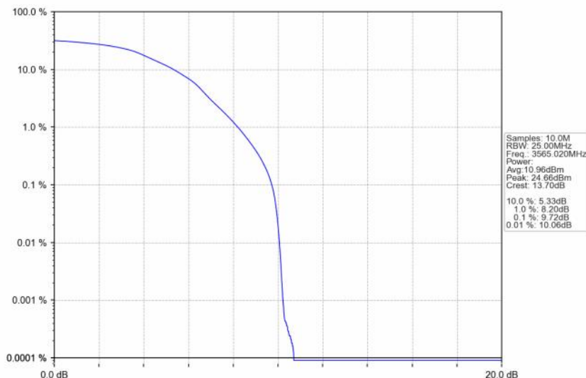
n48_30kHz_SISO_NTNV_30MHz_DFT-s-OFDM_16_QAM_3565.02MHz_Outer_Full
