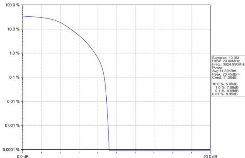
n48_30kHz_SISO_NTNV_20MHz_DFT-s-OFDM QPSK_3624.99MHz_Outer_Full
