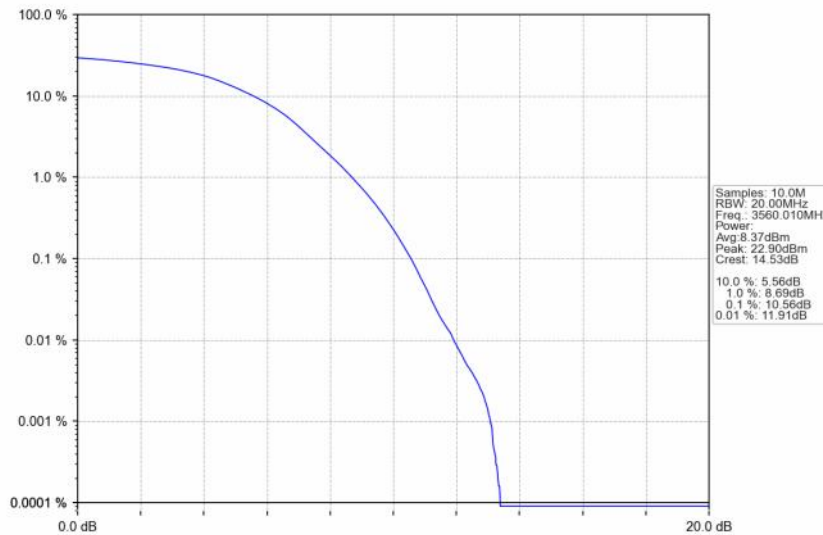
n48_30kHz_SISO_NTNV_20MHz_DFT-s-OFDM 256 QAM_3560.01MHz_Outer_Full
