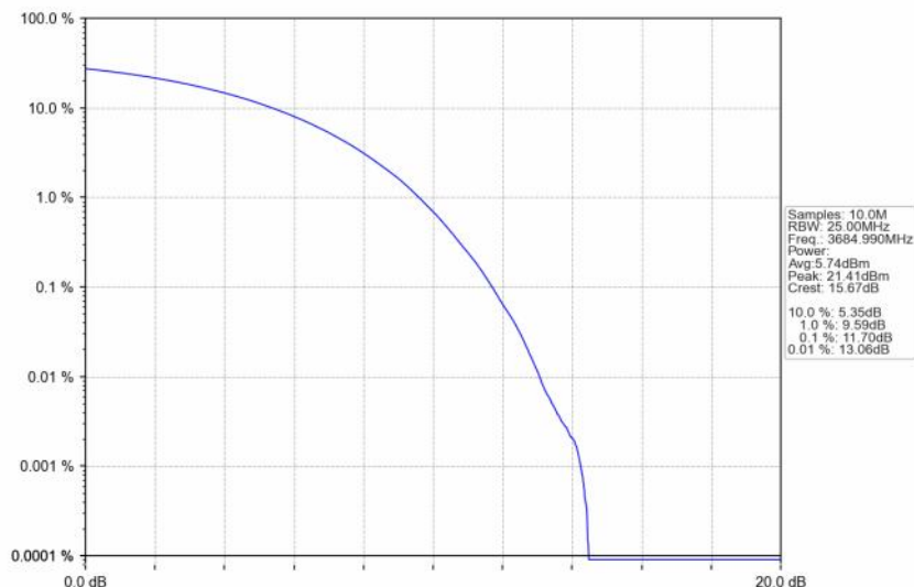
n48_30kHz_SISO_NTNV_30MHz_CP-OFDM 256 QAM_3684.99MHz_Outer_Full
