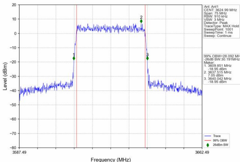
n48_30kHz_SISO_NTNV_30MHz_CP-OFDM 256 QAM_3624.99MHz_Outer_Full
