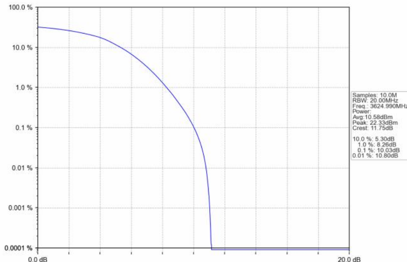
n48_30kHz_SISO_NTNV_20MHz_DFT-s-OFDM 64 QAM_3624.99MHz_Outer_Full
