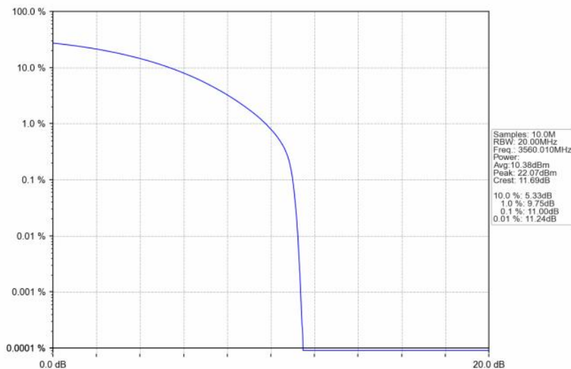
n48_30kHz_SISO_NTNV_20MHz_CP-OFDM QPSK_3560.01MHz_Outer_Full
