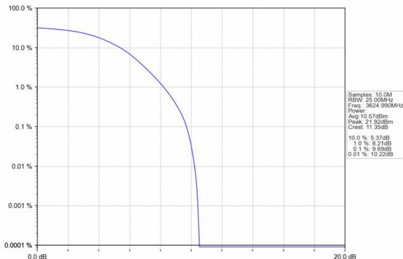
n48_30kHz_SISO_NTNV_30MHz_DFT-s-OFDM_16_QAM_3624.99MHz_Outer_Full
