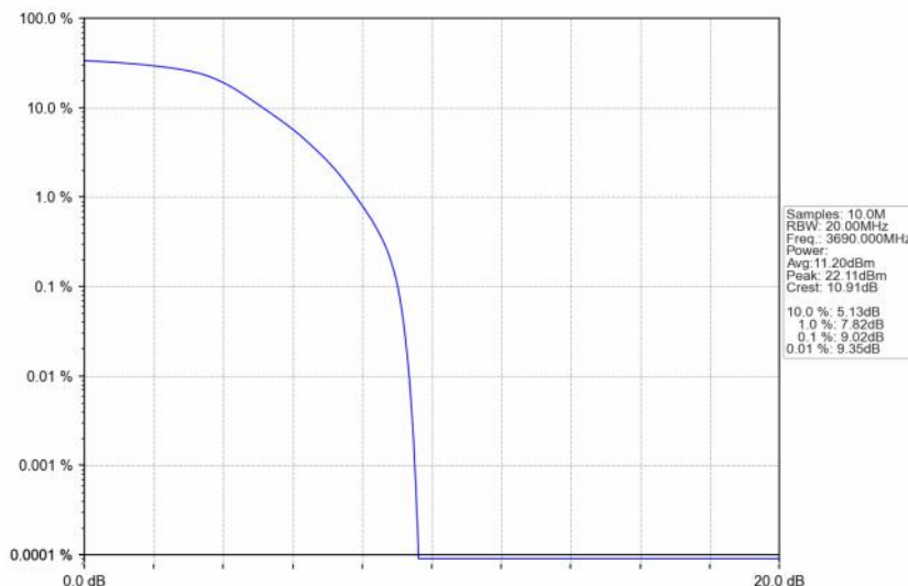
n48_30kHz_SISO_NTNV_20MHz_DFT-s-OFDM QPSK_3690MHz_Outer_Full
