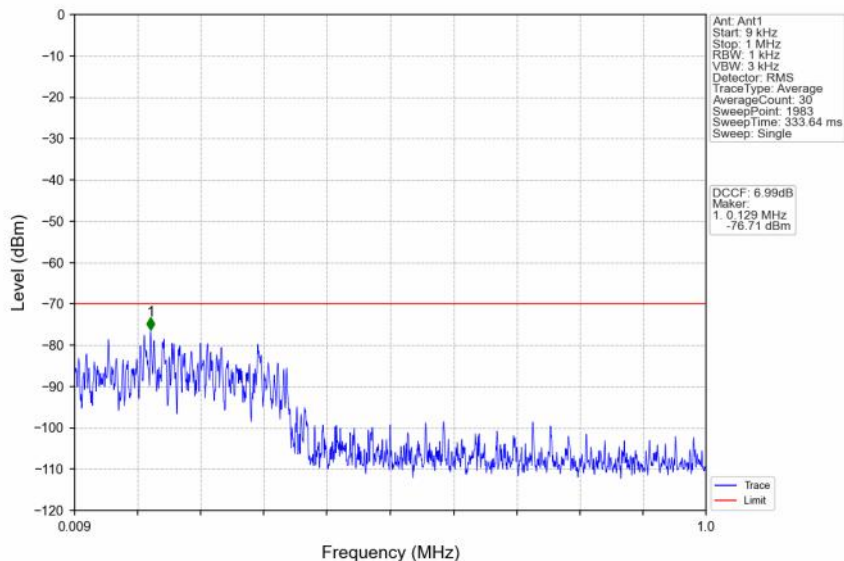
n48_30kHz_SISO_NTNV_10MHz_DFT-s-OFDM_QPSK_3555MHz_Edge_1RB_Left
