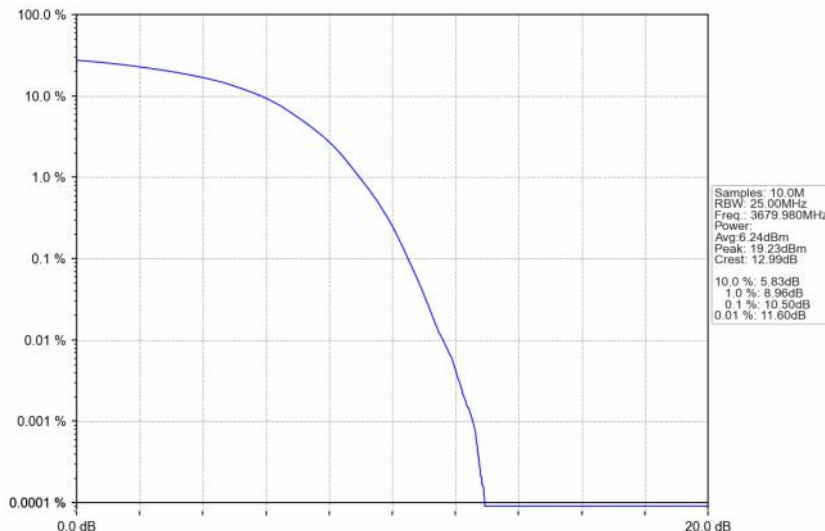
n48_30kHz_SISO_NTNV_40MHz_DFT-s-OFDM 256 QAM_3679.98MHz_Outer_Full
