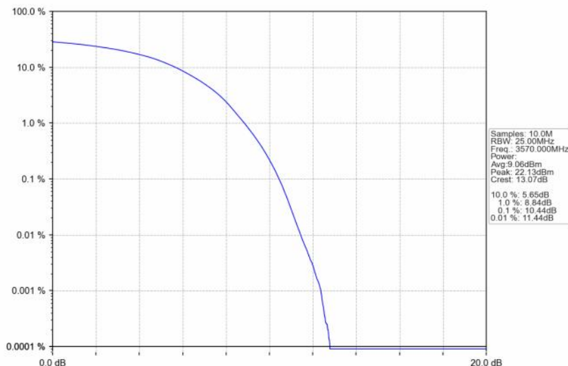
n48_30kHz_SISO_NTNV_40MHz_DFT-s-OFDM 64 QAM_3570MHz_Outer_Full
