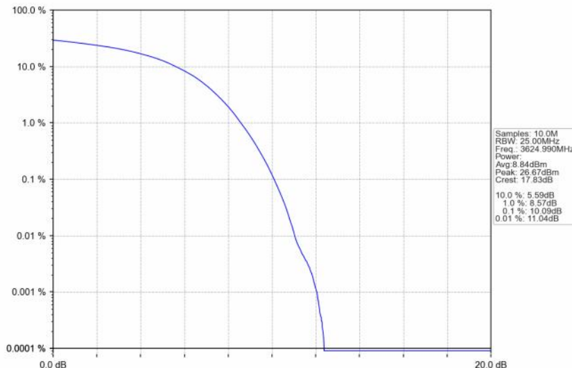
n48_30kHz_SISO_NTNV_40MHz_DFT-s-OFDM 64 QAM_3624.99MHz_Outer_Full
