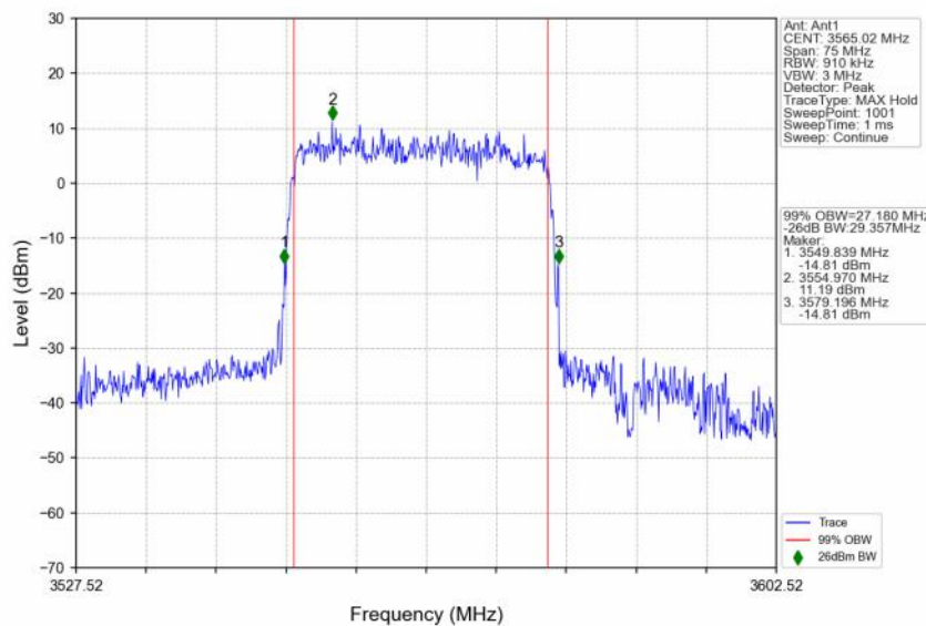
n48_30kHz_SISO_NTNV_30MHz_DFT-s-OFDM 64 QAM_3565.02MHz_Outer_Full
