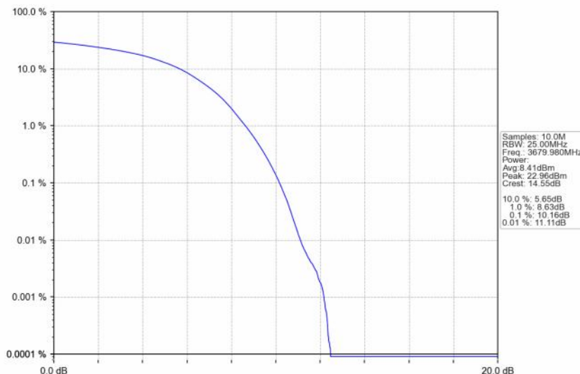
n48_30kHz_SISO_NTNV_40MHz_DFT-s-OFDM 64 QAM_3679.98MHz_Outer_Full
