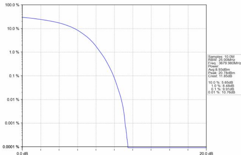
n48_30kHz_SISO_NTNV_40MHz_DFT-s-OFDM 16 QAM_3679.98MHz_Outer_Full
