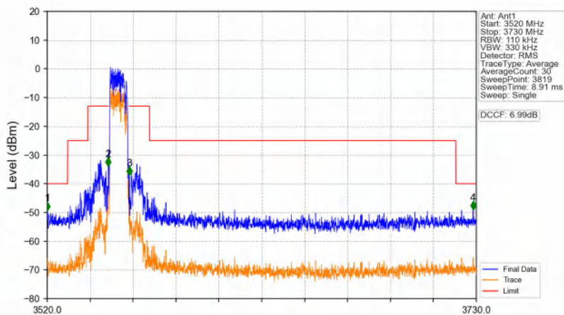
n48_30kHz_SISO_NTNV_10MHz_DFT-s-OFDM PI/2 BPSK_3555MHz_Outer_Full
