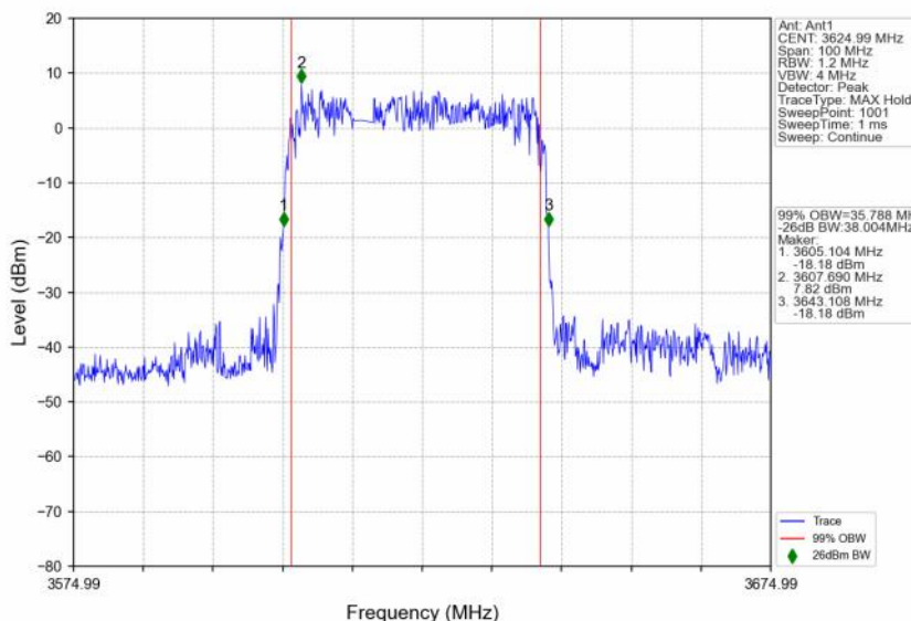
n48_30kHz_SISO_NTNV_40MHz_DFT-s-OFDM 256 QAM_3624.99MHz_Outer_Full
