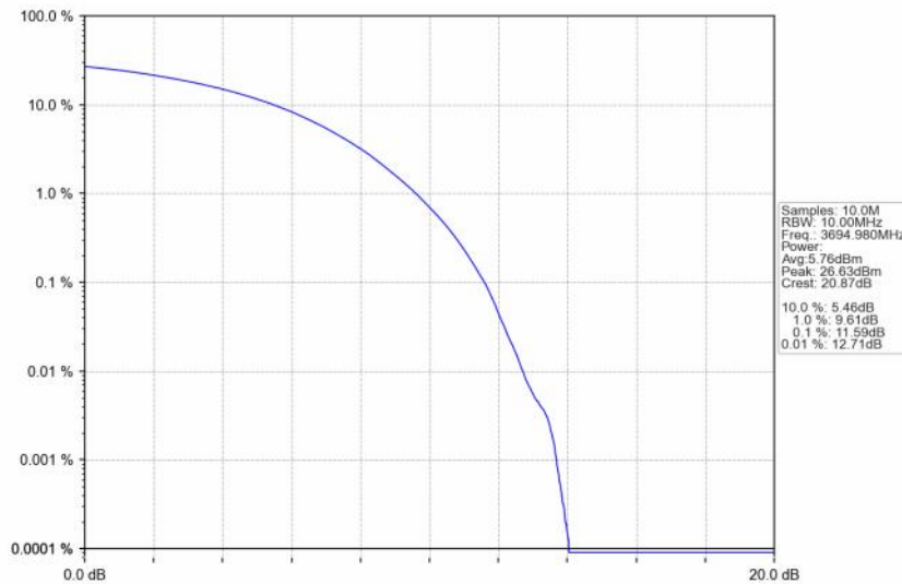
n48_30kHz_SISO_NTNV_10MHz_CP-OFDM 256 QAM_3694.98MHz_Outer_Full
