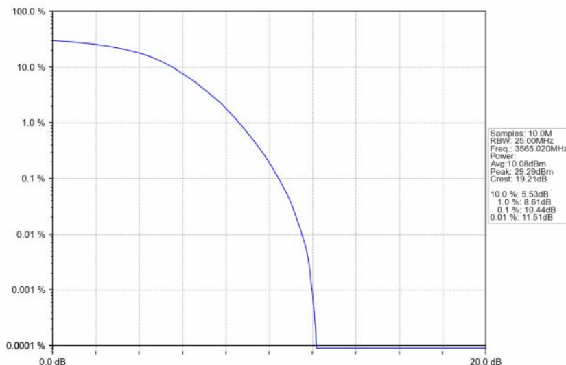
n48_30kHz_SISO_NTNV_30MHz_DFT-s-OFDM 64 QAM_3565.02MHz_Outer_Full
