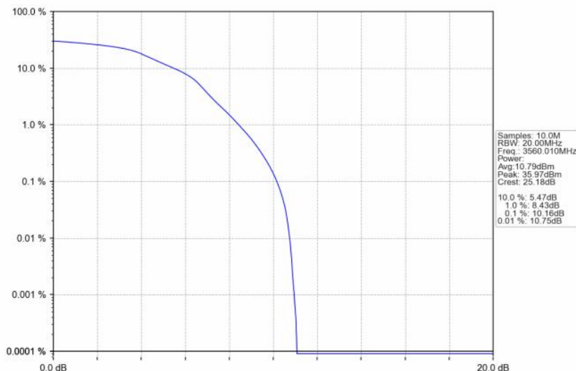
n48_30kHz_SISO_NTNV_20MHz_DFT-s-OFDM_16_QAM_3560.01MHz_Outer_Full
