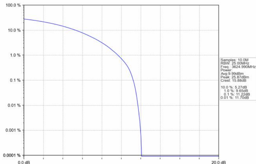
n48_30kHz_SISO_NTNV_30MHz_CP-OFDM QPSK_3624.99MHz_Outer_Full
