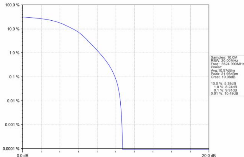
n48_30kHz_SISO_NTNV_20MHz_DFT-s-OFDM_16_QAM_3624.99MHz_Outer_Full
