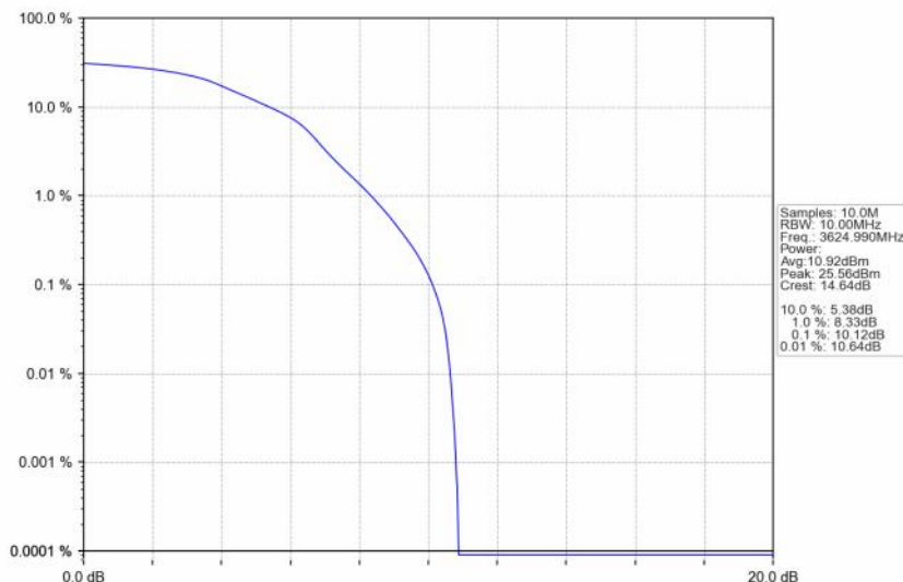
n48_30kHz_SISO_NTNV_10MHz_DFT-s-OFDM_16 QAM_3624.99MHz_Outer_Full
