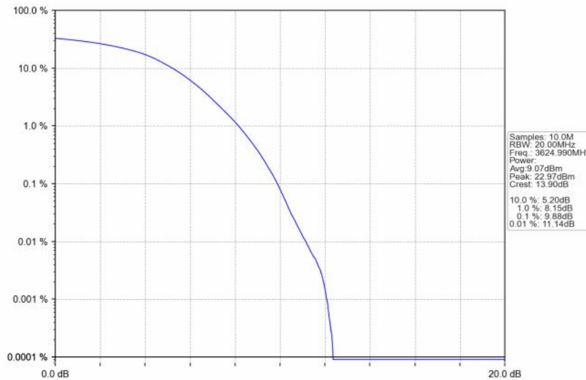
n48_30kHz_SISO_NTNV_20MHz_DFT-s-OFDM 256 QAM_3624.99MHz_Outer_Full
