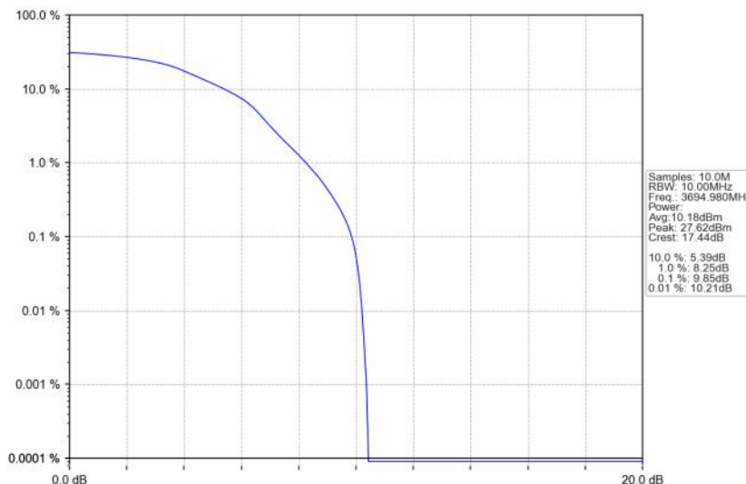
n48_30kHz_SISO_NTNV_10MHz_DFT-s-OFDM 16 QAM_3694.98MHz_Outer_Full
