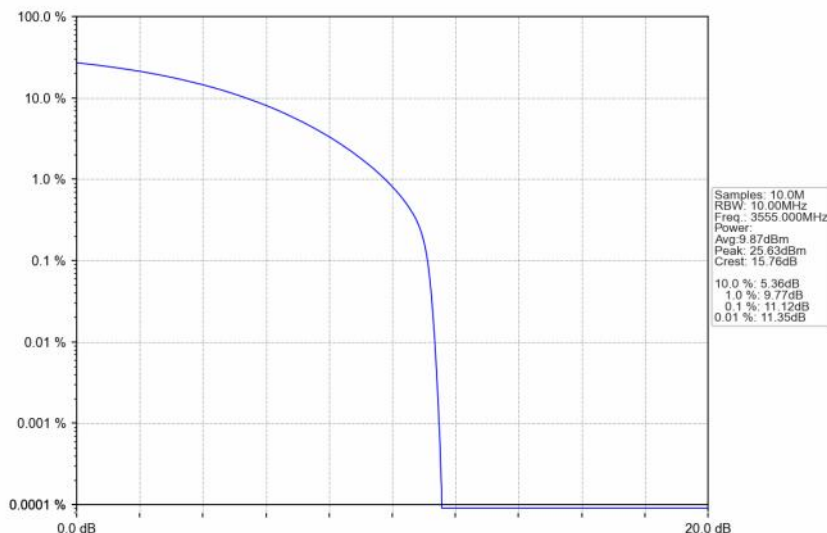
n48_30kHz_SISO_NTNV_10MHz_CP-OFDM QPSK_3555MHz_Outer_Full
