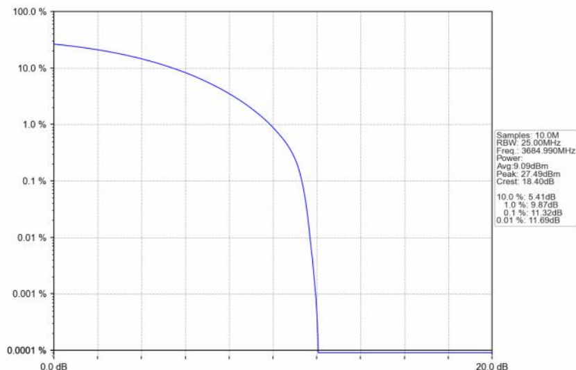
n48_30kHz_SISO_NTNV_30MHz_CP-OFDM QPSK_3684.99MHz_Outer_Full
