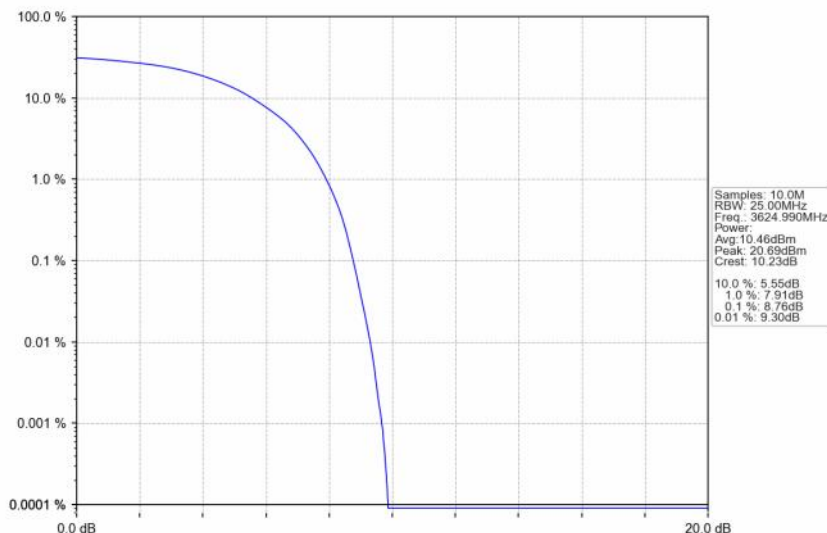
n48_30kHz_SISO_NTNV_40MHz_DFT-s-OFDM QPSK_3624.99MHz_Outer_Full
