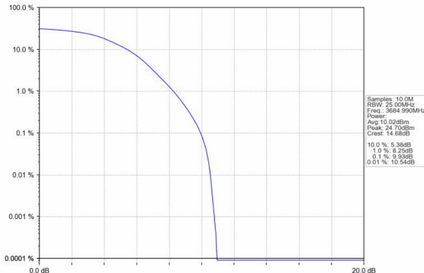
n48_30kHz_SISO_NTNV_30MHz_DFT-s-OFDM 16 QAM_3684.99MHz_Outer_Full
