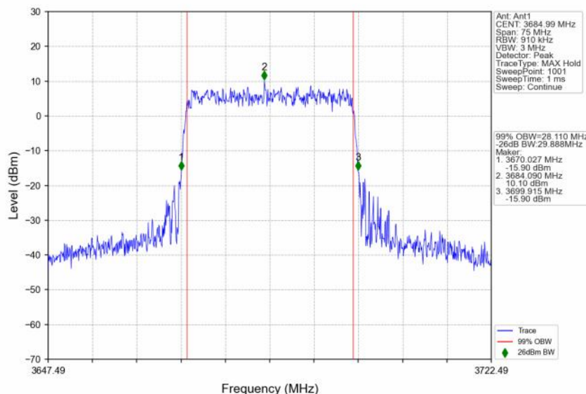
n48_30kHz_SISO_NTNV_30MHz_CP-OFDM 64 QAM_3684.99MHz_Outer_Full
