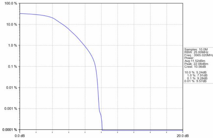
n48_30kHz_SISO_NTNV_30MHz_DFT-s-OFDM QPSK_3565.02MHz_Outer_Full
