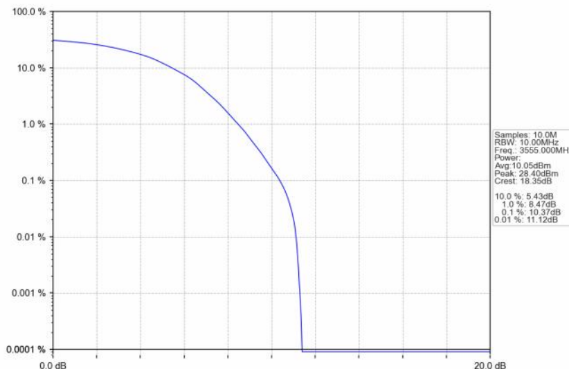
n48_30kHz_SISO_NTNV_10MHz_DFT-s-OFDM 64 QAM_3555MHz_Outer_Full
