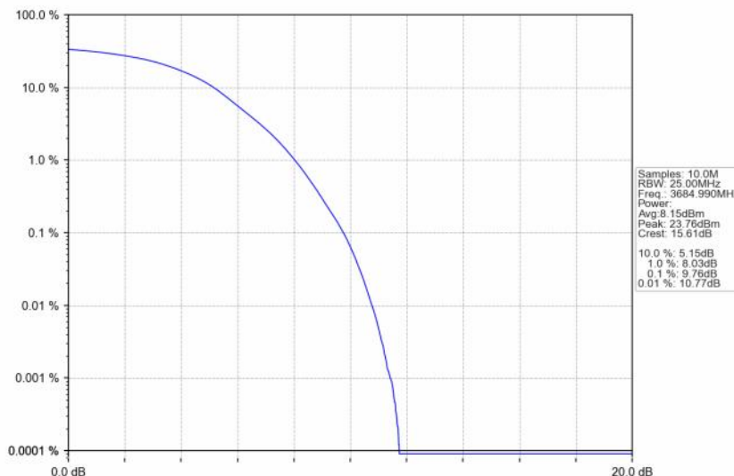
n48_30kHz_SISO_NTNV_30MHz_DFT-s-OFDM 256 QAM_3684.99MHz_Outer_Full
