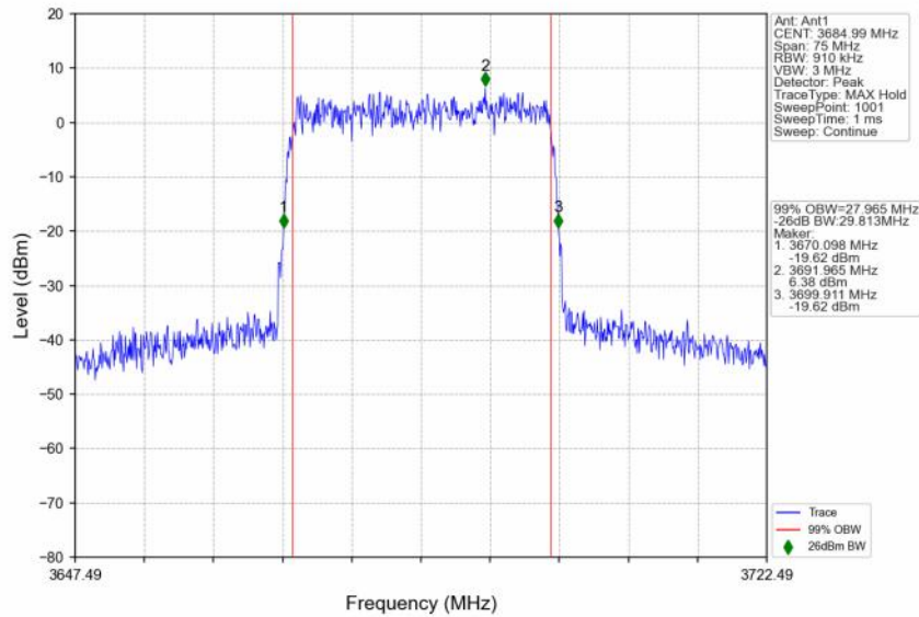
n48_30kHz_SISO_NTNV_30MHz_CP-OFDM 256 QAM_3684.99MHz_Outer_Full
