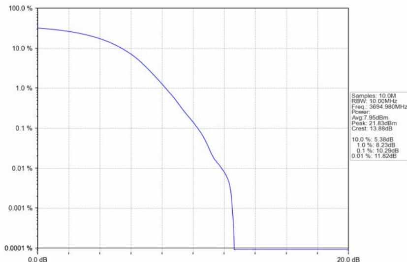
n48_30kHz_SISO_NTNV_10MHz_DFT-s-OFDM 256 QAM_3694.98MHz_Outer_Full
