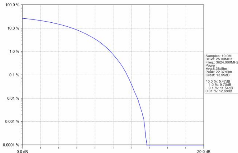
n48_30kHz_SISO_NTNV_40MHz_CP-OFDM QPSK_3624.99MHz_Outer_Full
