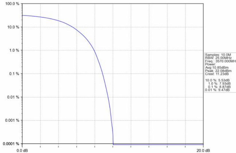
n48_30kHz_SISO_NTNV_40MHz_DFT-s-OFDM QPSK_3570MHz_Outer_Full
