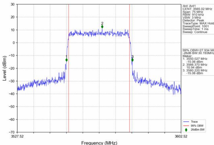
n48_30kHz_SISO_NTNV_30MHz_CP-OFDM QPSK_3565.02MHz_Outer_Full
