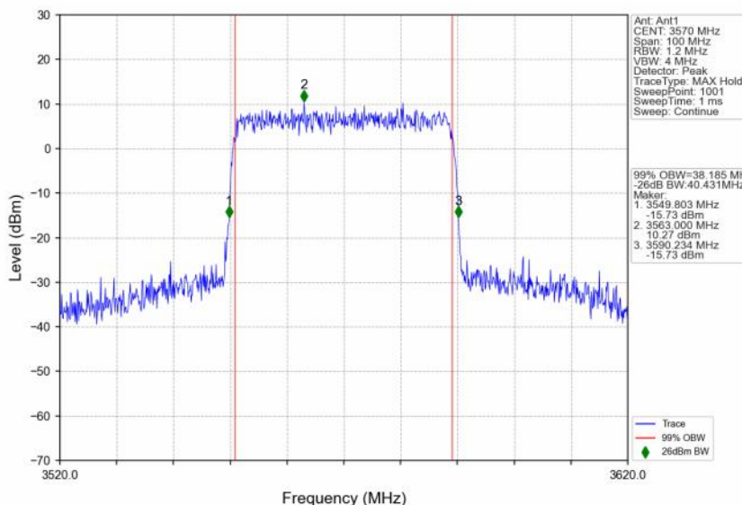
n48_30kHz_SISO_NTNV_40MHz_CP-OFDM QPSK_3570MHz_Outer_Full
