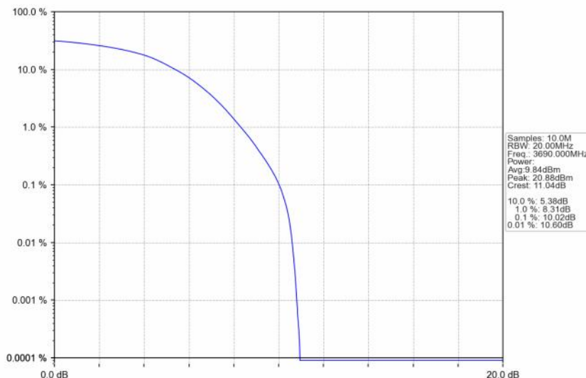
n48_30kHz_SISO_NTNV_20MHz_DFT-s-OFDM 64 QAM_3690MHz_Outer_Full
