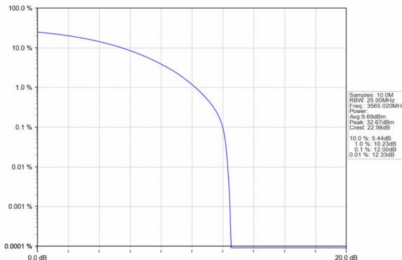
n48_30kHz_SISO_NTNV_30MHz_CP-OFDM QPSK_3565.02MHz_Outer_Full
