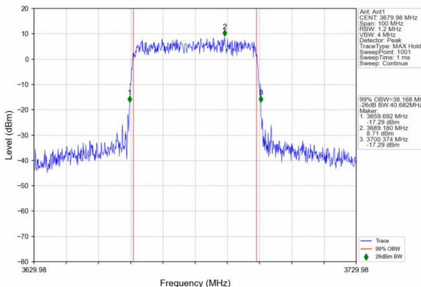
n48_30kHz_SISO_NTNV_40MHz_CP-OFDM 64 QAM_3679.98MHz_Outer_Full
