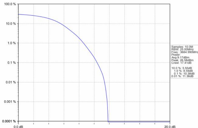
n48_30kHz_SISO_NTNV_30MHz_DFT-s-OFDM_64_QAM_3684.99MHz_Outer_Full
