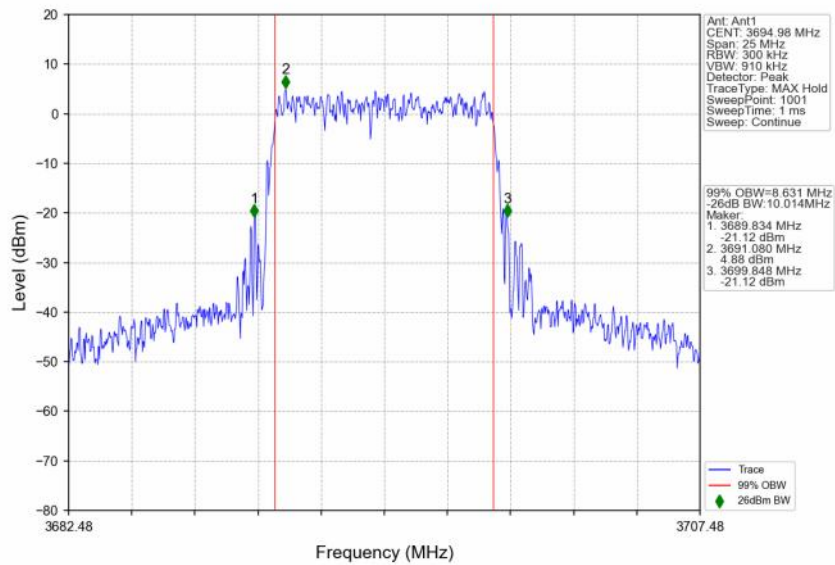
n48_30kHz_SISO_NTNV_10MHz_CP-OFDM 256 QAM_3694.98MHz_Outer_Full
