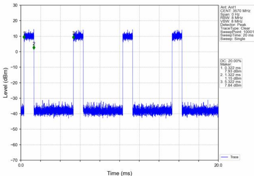
n48_30kHz_SISO_NTNV_40MHz_CP-OFDM 256 QAM_3570MHz_Inner_Full
