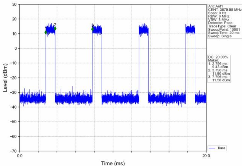
n48_30kHz_SISO_NTNV_40MHz_CP-OFDM 64 QAM_3679.98MHz_Inner_Full
