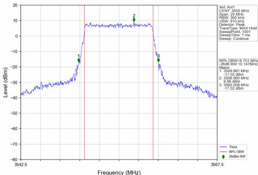
n48_30kHz_SISO_NTNV_10MHz_CP-OFDM 64 QAM_3555MHz_Outer_Full
