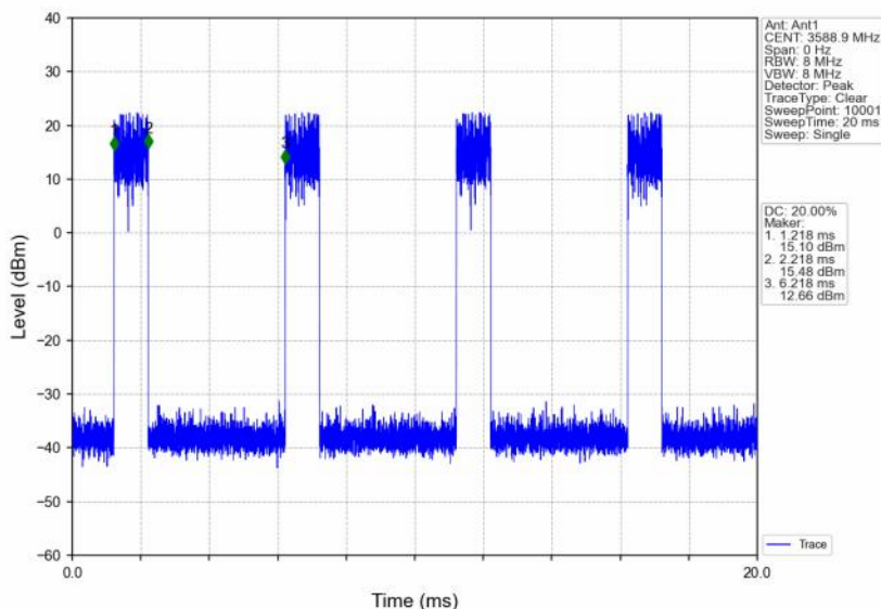
n48_30kHz_SISO_NTNV_40MHz_CP-OFDM 16 QAM_3570MHz_Edge_1RB_Right
