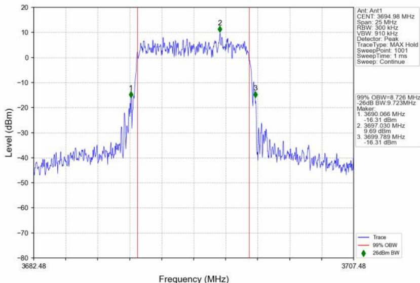
n48_30kHz_SISO_NTNV_10MHz_CP-OFDM 64 QAM_3694.98MHz_Outer_Full
