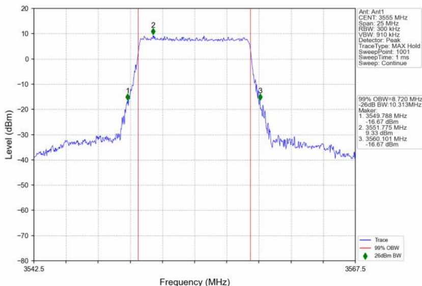
n48_30kHz_SISO_NTNV_10MHz_DFT-s-OFDM 64 QAM_3555MHz_Outer_Full
