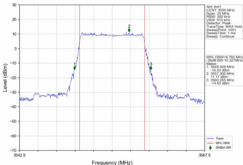
n48_30kHz_SISO_NTNV_10MHz_DFT-s-OFDM QPSK_3555MHz_Outer_Full
