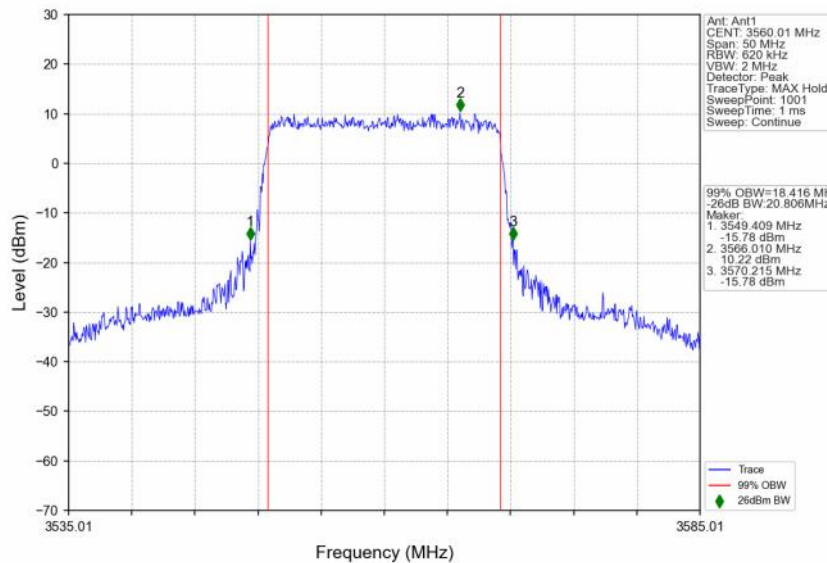
n48_30kHz_SISO_NTNV_20MHz_CP-OFDM QPSK_3560.01MHz_Outer_Full
