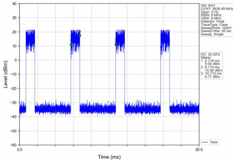
n48_30kHz_SISO_NTNV_30MHz_CP-OFDM_16_QAM_3624.99MHz_Inner_1RB_Right
