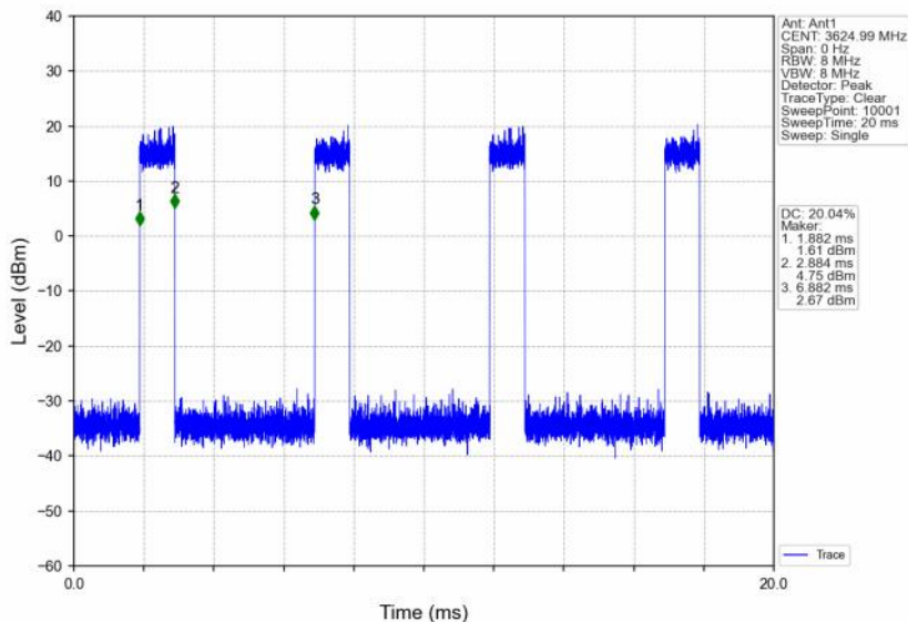
n48_30kHz_SISO_NTNV_30MHz_CP-OFDM 16 QAM_3624.99MHz_Inner_Full
