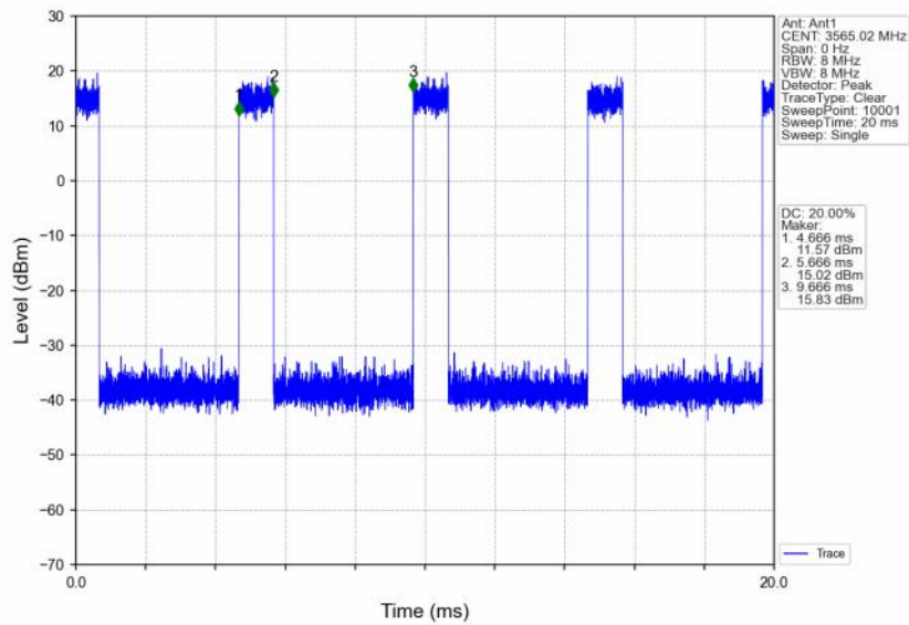
n48_30kHz_SISO_NTNV_30MHz_CP-OFDM 16 QAM_3565.02MHz_Inner_Full
