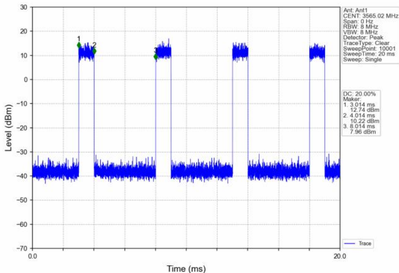
n48_30kHz_SISO_NTNV_30MHz_CP-OFDM 256 QAM_3565.02MHz_Inner_Full
