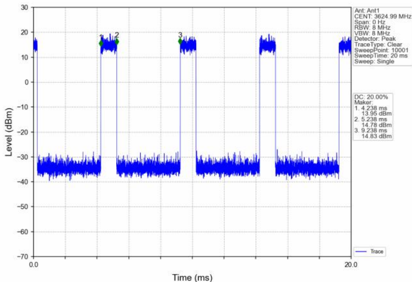
n48_30kHz_SISO_NTNV_30MHz_CP-OFDM 64 QAM_3624.99MHz_Inner_Full
