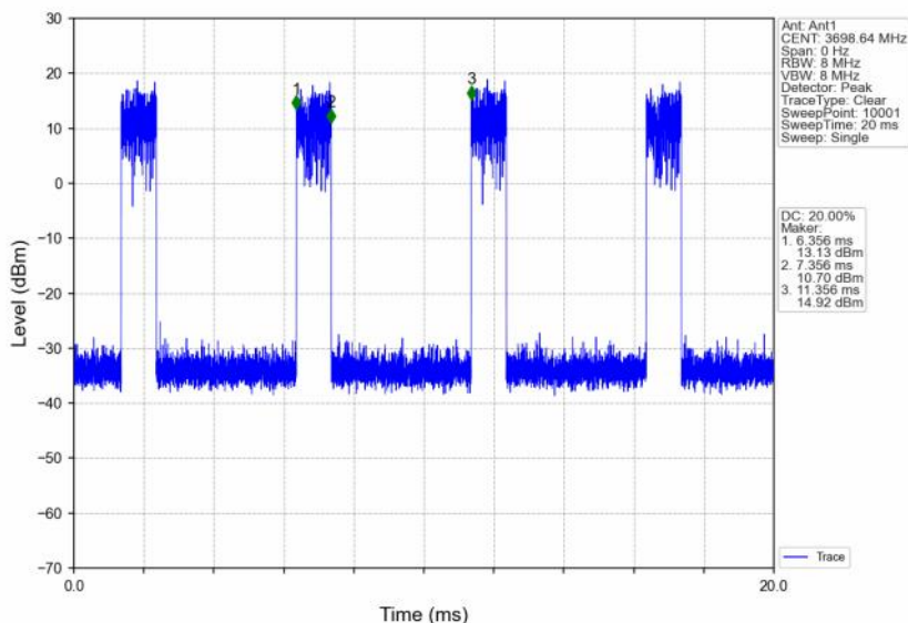
n48_30kHz_SISO_NTNV_20MHz_CP-OFDM 256 QAM_3690MHz_Inner_1RB_Right
