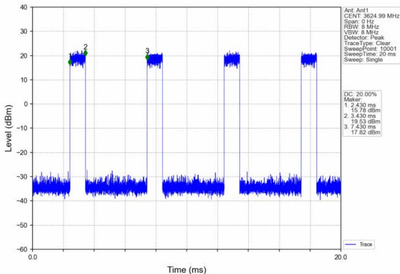
n48_30kHz_SISO_NTNV_10MHz_CP-OFDM QPSK_3624.99MHz_Inner_Full
