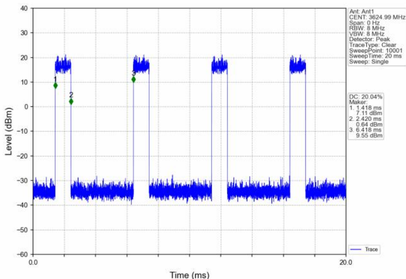
n48_30kHz_SISO_NTNV_10MHz_DFT-s-OFDM 256 QAM_3624.99MHz_Inner_Full
