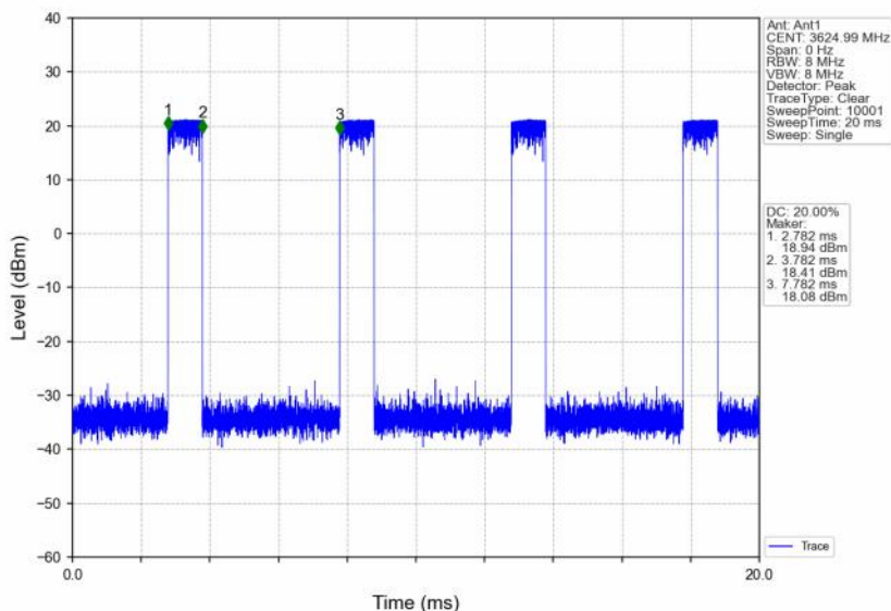
n48_30kHz_SISO_NTNV_10MHz_CP-OFDM QPSK_3624.99MHz_Inner_Full
