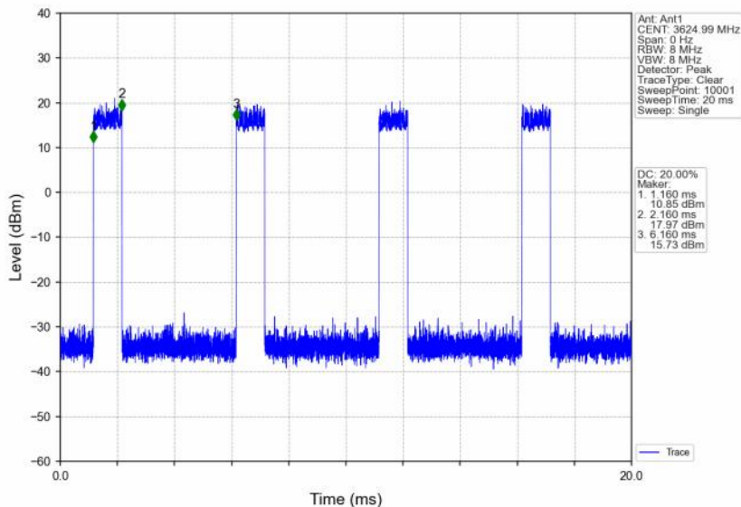
n48_30kHz_SISO_NTNV_10MHz_DFT-s-OFDM 256 QAM_3624.99MHz_Inner_Full
