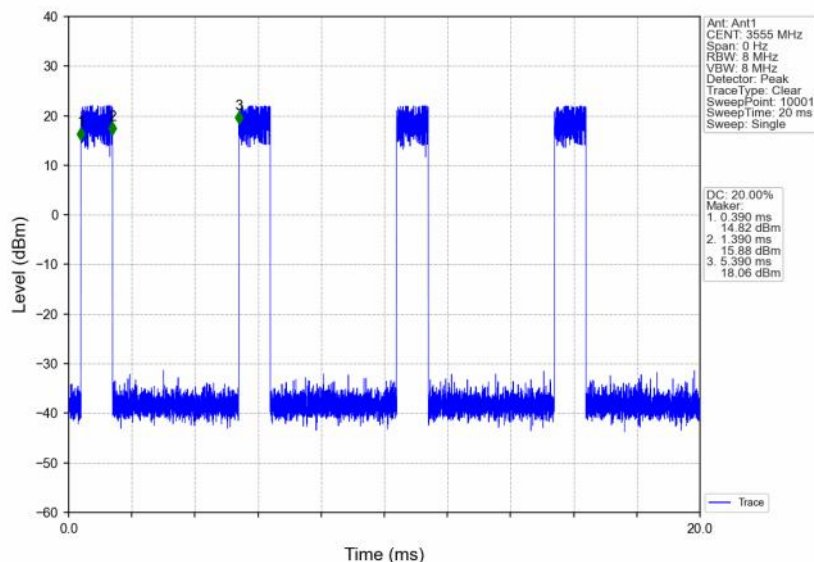
n48_30kHz_SISO_NTNV_10MHz_CP-OFDM 64 QAM_3555MHz_Inner_Full
