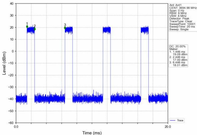
n48_30kHz_SISO_NTNV_10MHz_CP-OFDM 16 QAM_3694.98MHz_Inner_Full
