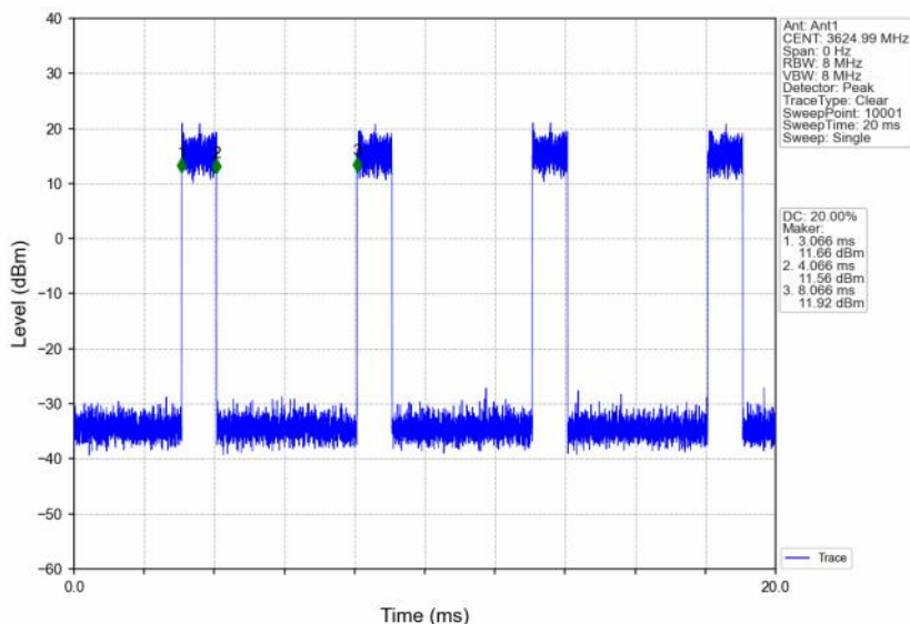
n48_30kHz_SISO_NTNV_10MHz_CP-OFDM 256 QAM_3624.99MHz_Inner_Full
