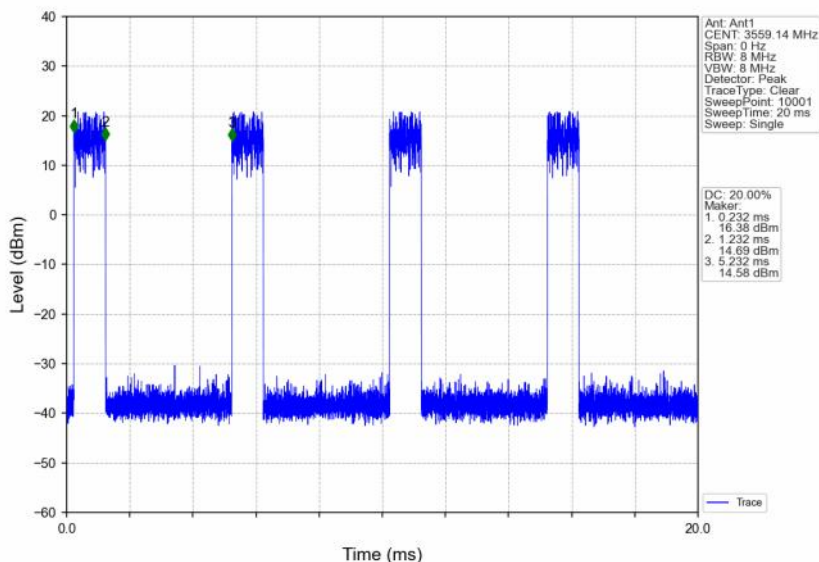
n48_30kHz_SISO_NTNV_10MHz_DFT-s-OFDM_16 QAM_3555MHz_Edge_1RB_Right
