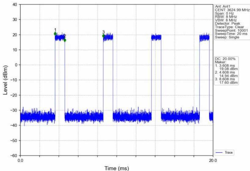
n48_30kHz_SISO_NTNV_10MHz_DFT-s-OFDM_16_QAM_3624.99MHz_Inner_Full
