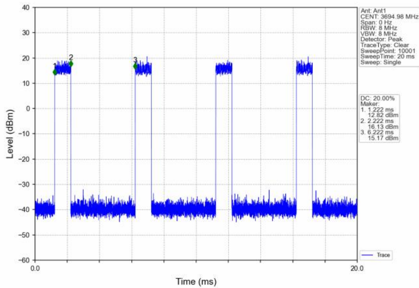
n48_30kHz_SISO_NTNV_10MHz_DFT-s-OFDM 256 QAM_3694.98MHz_Inner_Full
