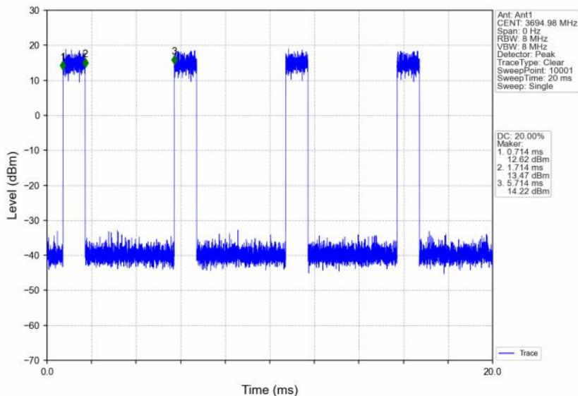
n48_30kHz_SISO_NTNV_10MHz_CP-OFDM 256 QAM_3694.98MHz_Inner_Full
