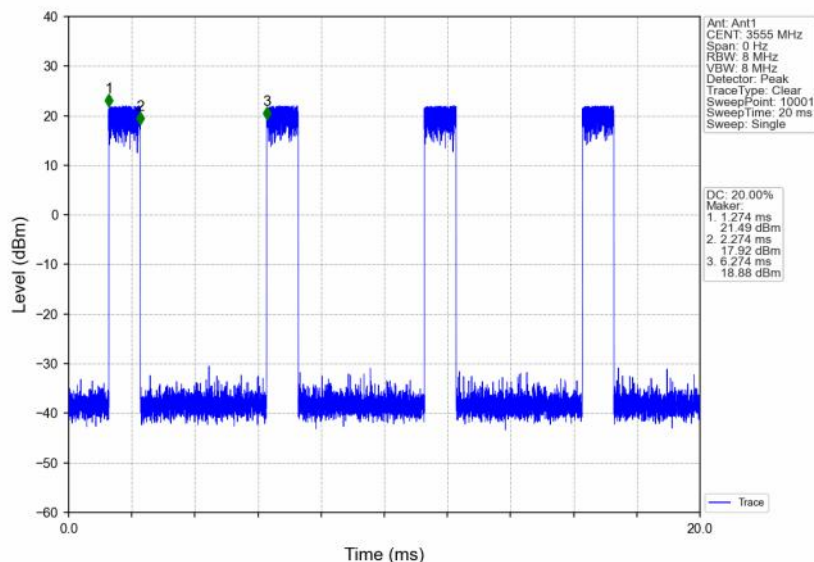
n48_30kHz_SISO_NTNV_10MHz_CP-OFDM_16 QAM_3555MHz_Inner_Full
