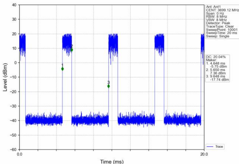
n48_30kHz_SISO_NTNV_10MHz_CP-OFDM QPSK_3694.98MHz_Edge_1RB_Right
