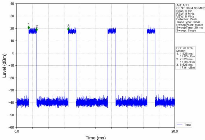
n48_30kHz_SISO_NTNV_10MHz_DFT-s-OFDM_16_QAM_3694.98MHz_Inner_Full
