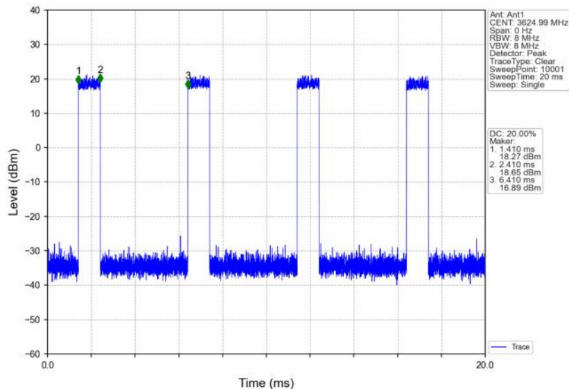
n48_30kHz_SISO_NTNV_10MHz_DFT-s-OFDM QPSK_3624.99MHz_Inner_Full
