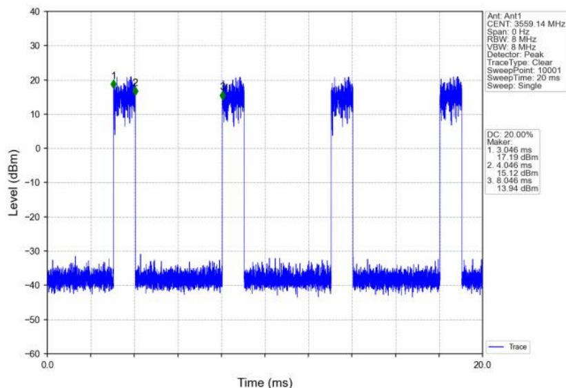
n48_30kHz_SISO_NTNV_10MHz_DFT-s-OFDM 64 QAM_3555MHz_Edge_1RB_Right
