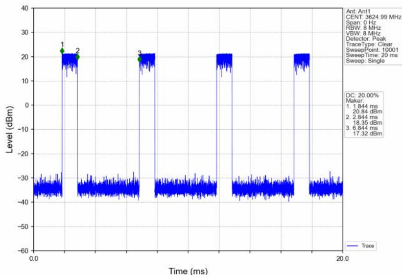
n48_30kHz_SISO_NTNV_10MHz_CP-OFDM_16 QAM_3624.99MHz_Inner_Full
