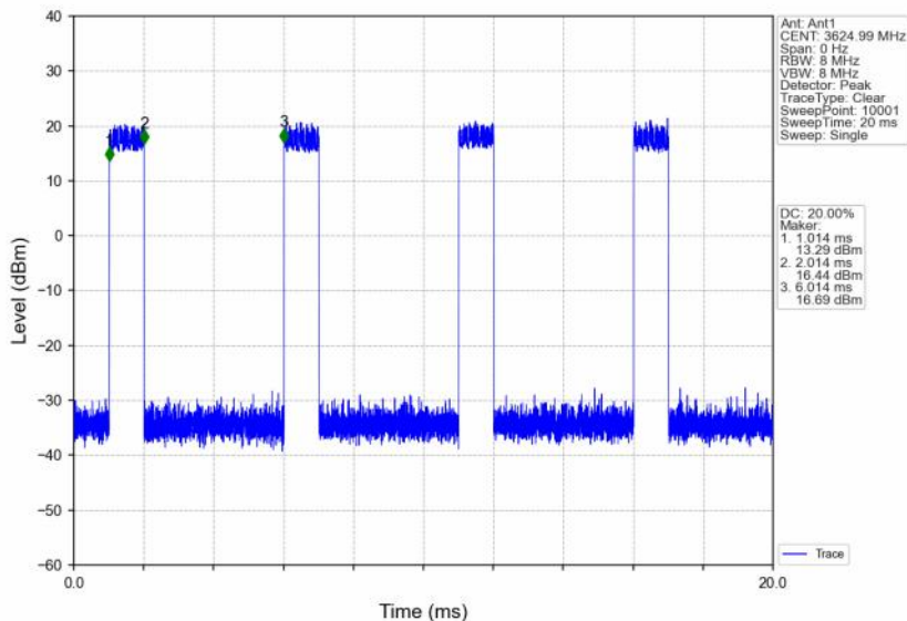
n48_30kHz_SISO_NTNV_10MHz_DFT-s-OFDM 64 QAM_3624.99MHz_Inner_Full
