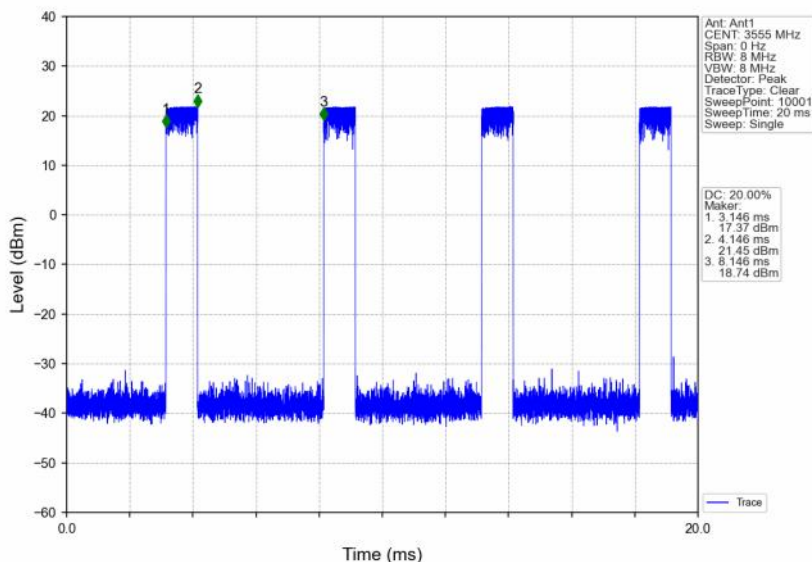
n48_30kHz_SISO_NTNV_10MHz_CP-OFDM QPSK_3555MHz_Inner_Full
