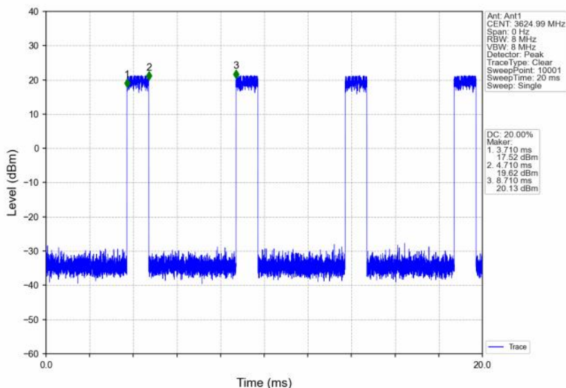
n48_30kHz_SISO_NTNV_10MHz_DFT-s-OFDM_16_QAM_3624.99MHz_Inner_Full
