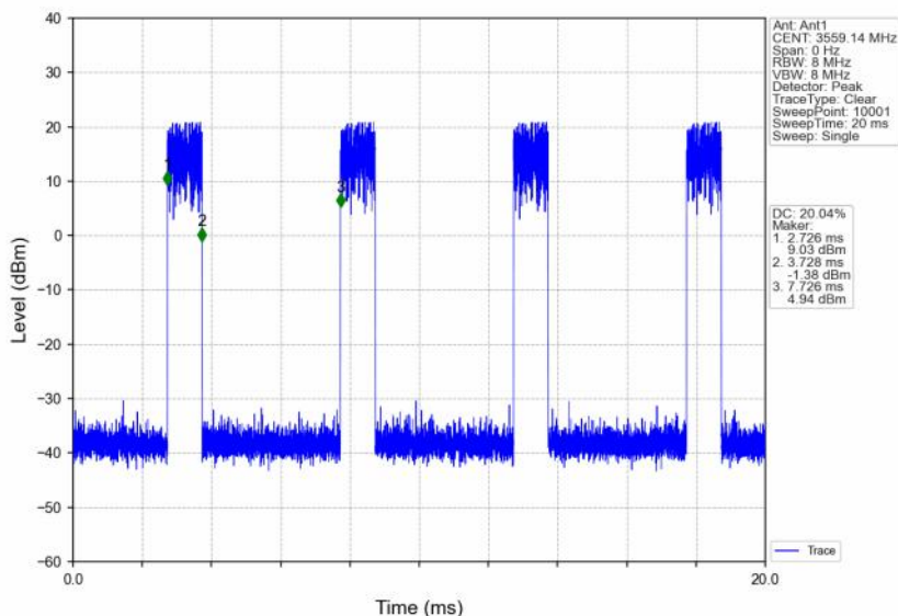
n48_30kHz_SISO_NTNV_10MHz_CP-OFDM_QPSK_3555MHz_Edge_1RB_Right
