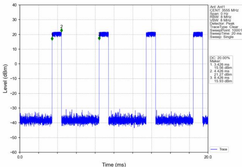
n48_30kHz_SISO_NTNV_10MHz_DFT-s-OFDM QPSK_3555MHz_Inner_Full
