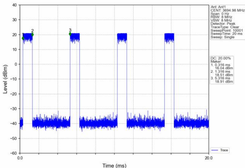
n48_30kHz_SISO_NTNV_10MHz_CP-OFDM 16 QAM_3694.98MHz_Inner_Full
