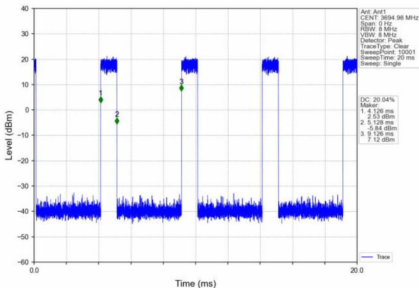
n48_30kHz_SISO_NTNV_10MHz_CP-OFDM 64 QAM_3694.98MHz_Inner_Full
