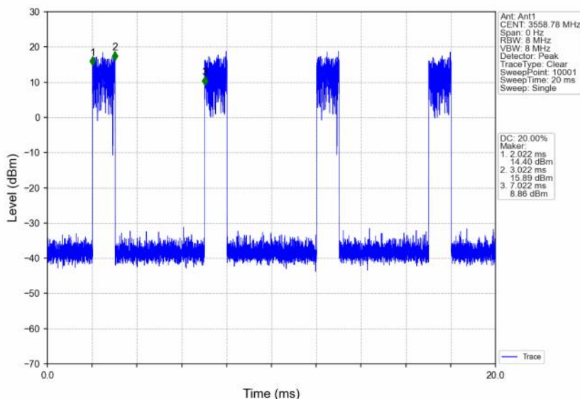
n48_30kHz_SISO_NTNV_10MHz_CP-OFDM 256 QAM_3555MHz_Inner_1RB_Right
