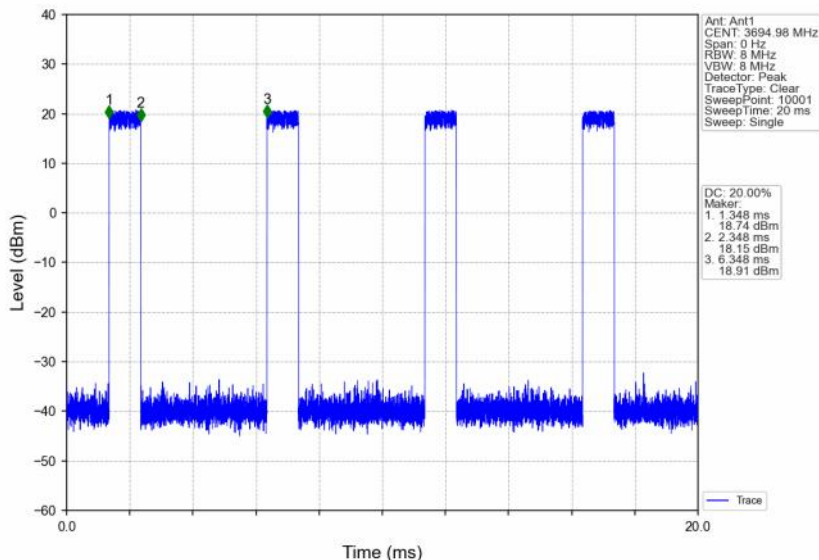
n48_30kHz_SISO_NTNV_10MHz_DFT-s-OFDM PI/2 BPSK_3694.98MHz_Inner_Full
