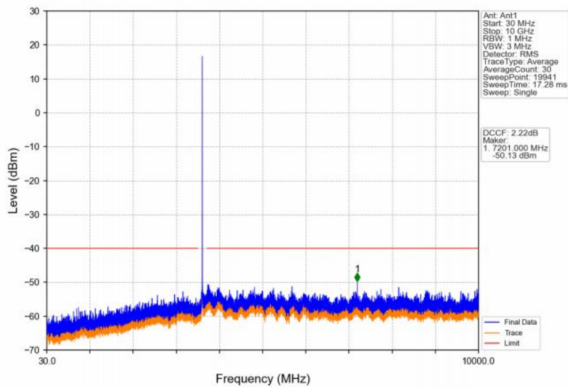
Band48_10MHz_64QAM_MCH_3625MHz_RB_1_0_NTNV
