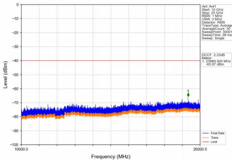
Band48_20MHz_16QAM_MCH_3625MHz_RB_1_0_NTNV
