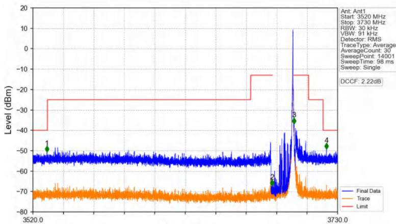
Band48_15MHz_64QAM_HCH_3692.5MHz_RB_1_74_NTNV
