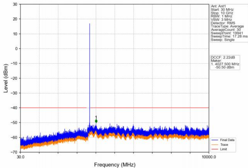
Band48_10MHz_64QAM_HCH_3695MHz_RB_1_0_NTNV
