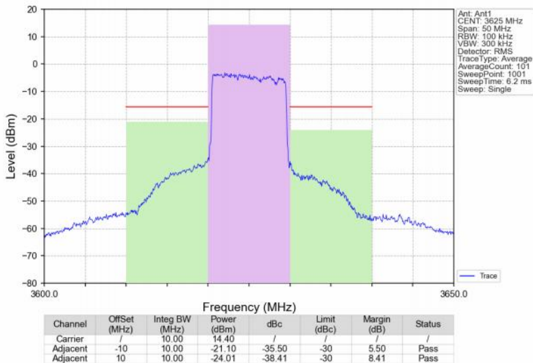
Band48_10MHz_256QAM_MCH_3625MHz_RB_50_0_NTNV
