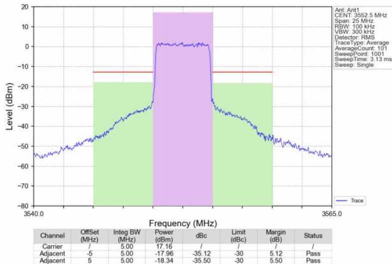
Band48_5MHz_16QAM_LCH_3552.5MHz_RB_25_0_NTNV
