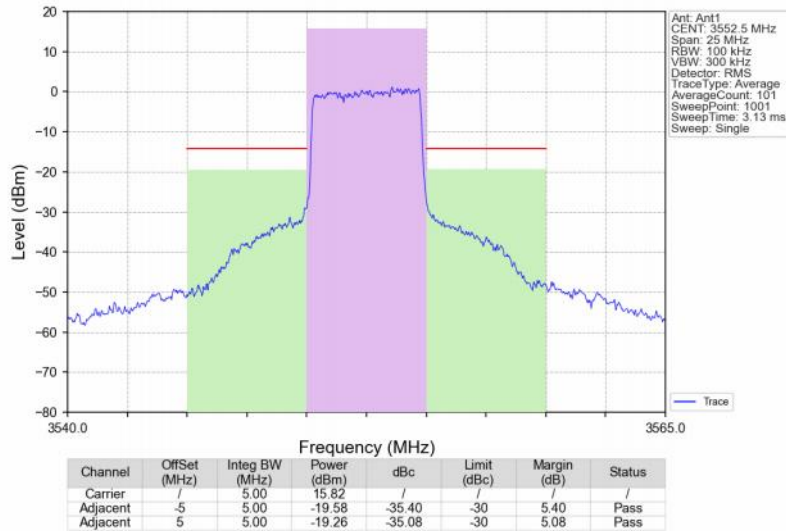
Band48_5MHz_256QAM_LCH_3552.5MHz_RB_25_0_NTNV
