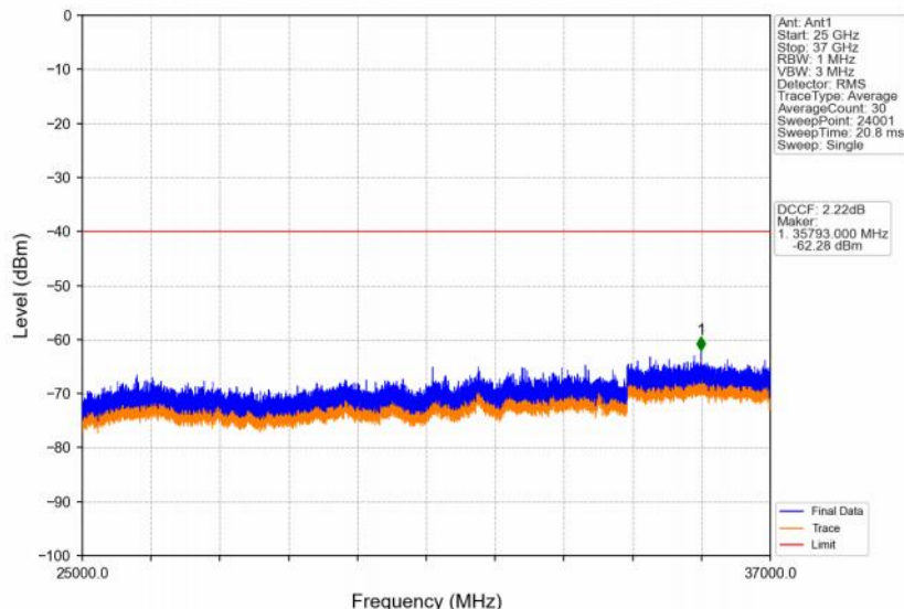
Band48_15MHz_64QAM_HCH_3692.5MHz_RB_1_74_NTNV
