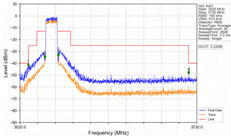
Band48_15MHz_16QAM_LCH_3557.5MHz_RB_75_0_NTNV
