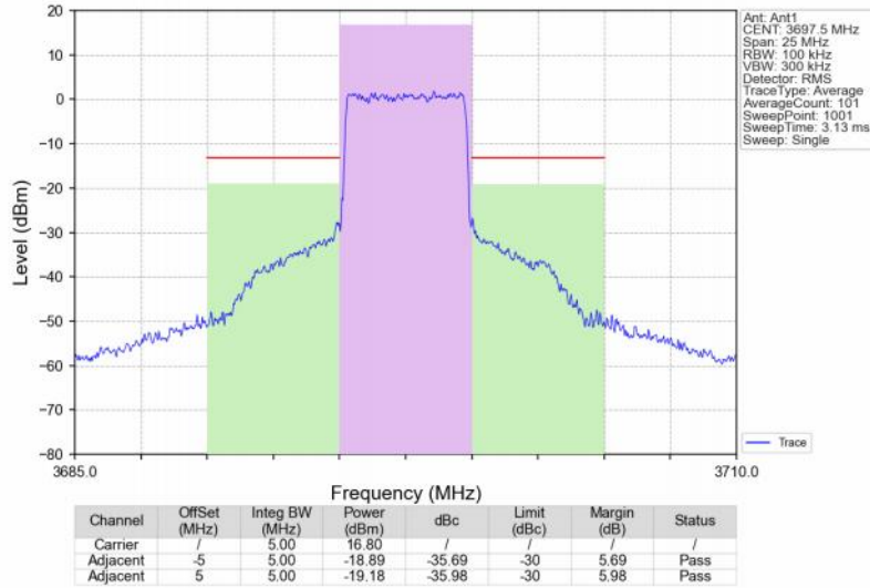
Band48_5MHz_64QAM_HCH_3697.5MHz_RB_25_0_NTNV
