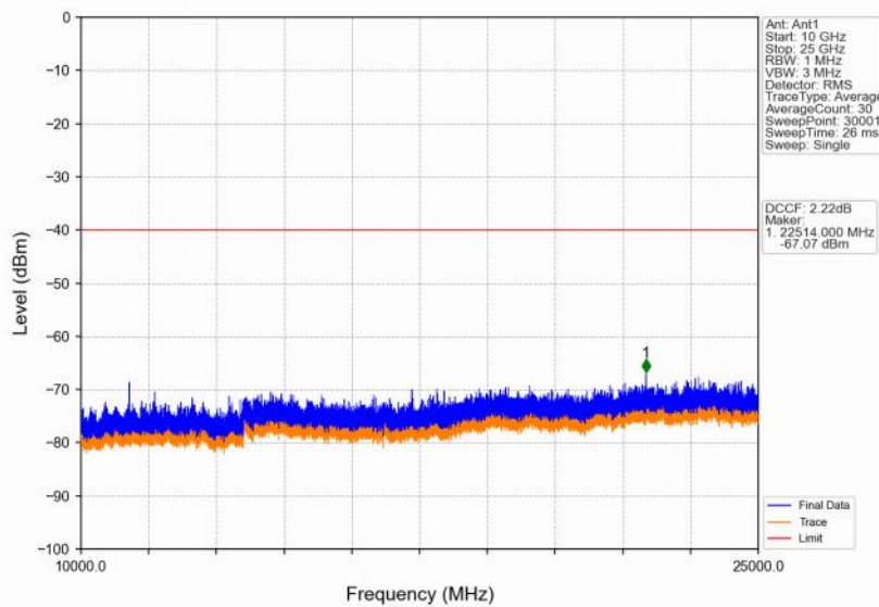
Band48_10MHz_64QAM_HCH_3695MHz_RB_1_0_NTNV
