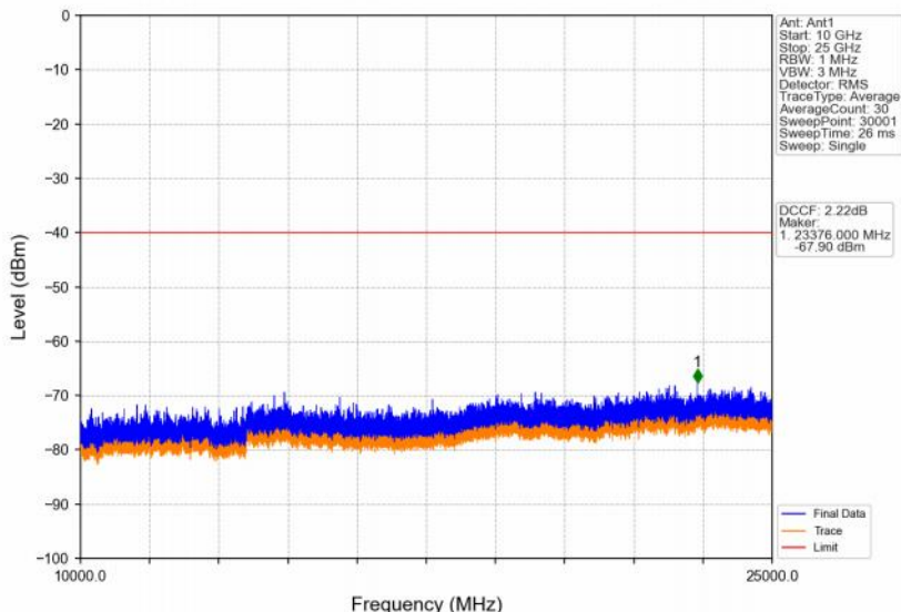
Band48_15MHz_64QAM_LCH_3557.5MHz_RB_1_0_NTNV
