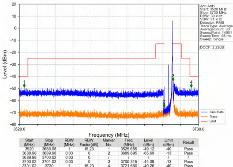
Band48_10MHz_256QAM_HCH_3695MHz_RB_50_0_NTNV
