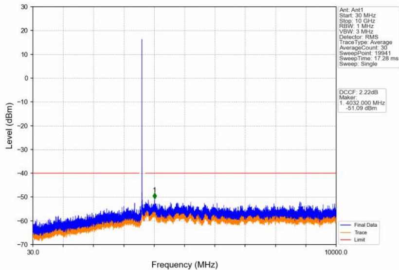
Band48_20MHz_16QAM_MCH_3625MHz_RB_1_0_NTNV
