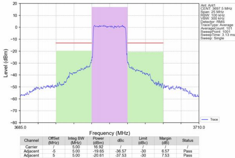
Band48_5MHz_QPSK_HCH_3697.5MHz_RB_25_0_NTNV
