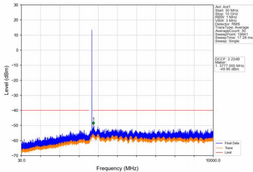
Band48_10MHz_256QAM_HCH_3695MHz_RB_1_0_NTNV
