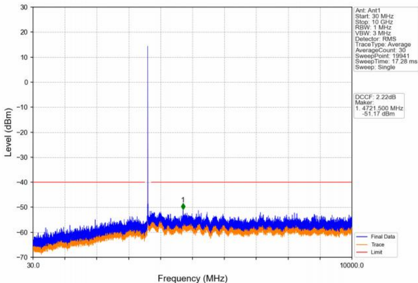
Band48_15MHz_16QAM_MCH_3625MHz_RB_1_0_NTNV
