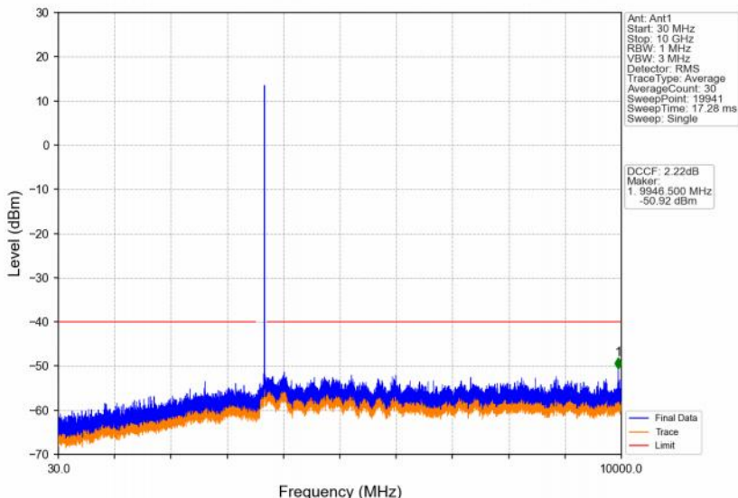
Band48_20MHz_64QAM_HCH_3690MHz_RB_1_0_NTNV
