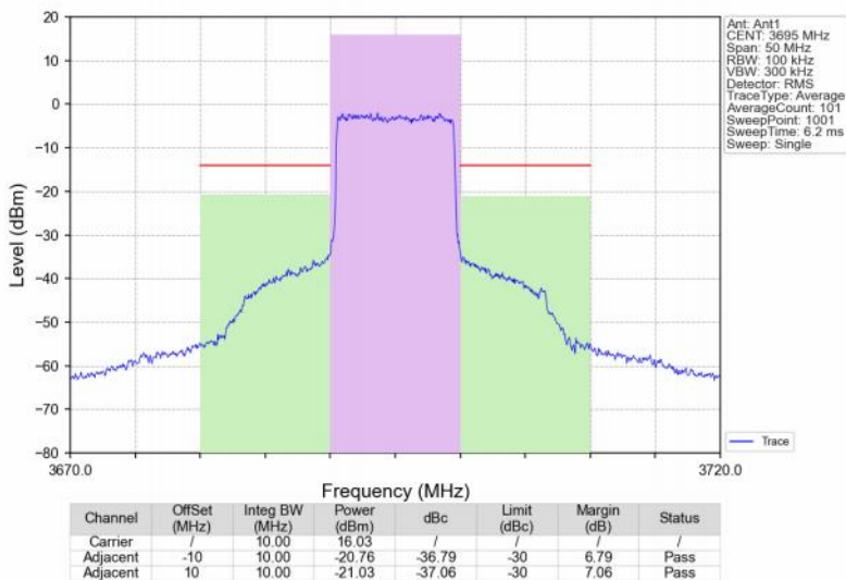
Band48_10MHz_256QAM_HCH_3695MHz_RB_50_0_NTNV
