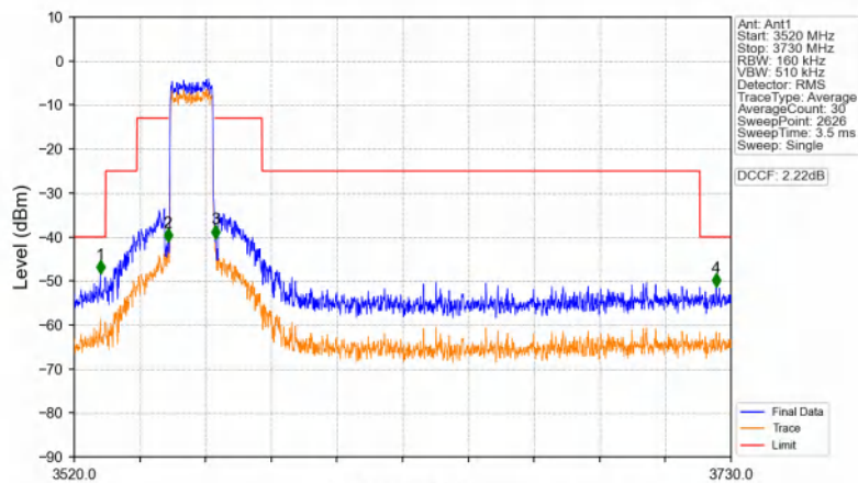
Band48_15MHz_256QAM_LCH_3557.5MHz_RB_75_0_NTNV
