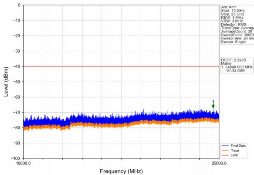
Band48_10MHz_256QAM_MCH_3625MHz_RB_1_0_NTNV
