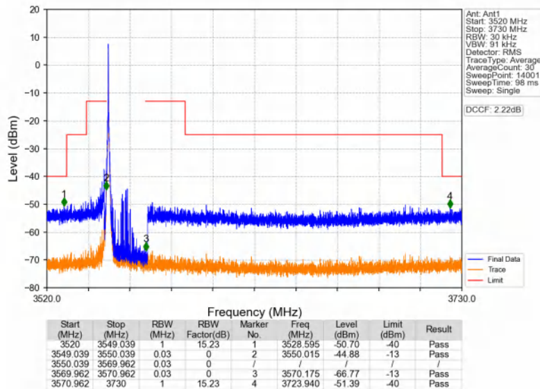
Band48_20MHz_64QAM_LCH_3560MHz_RB_1_0_NTNV
