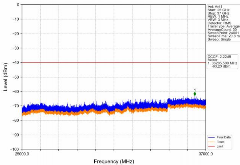
Band48_20MHz_64QAM_LCH_3560MHz_RB_1_0_NTNV
