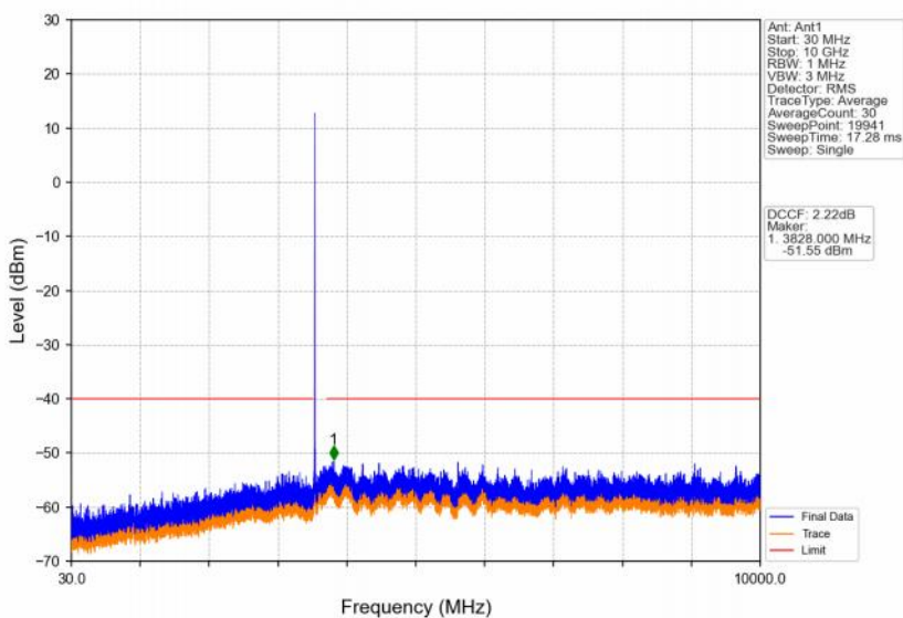
Band48_15MHz_64QAM_LCH_3557.5MHz_RB_1_0_NTNV
