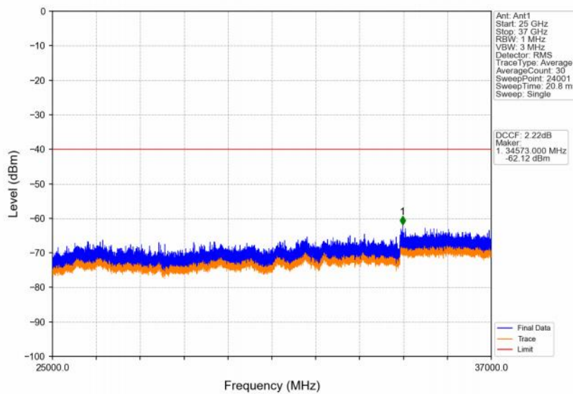
Band48_10MHz_256QAM_HCH_3695MHz_RB_1_0_NTNV
