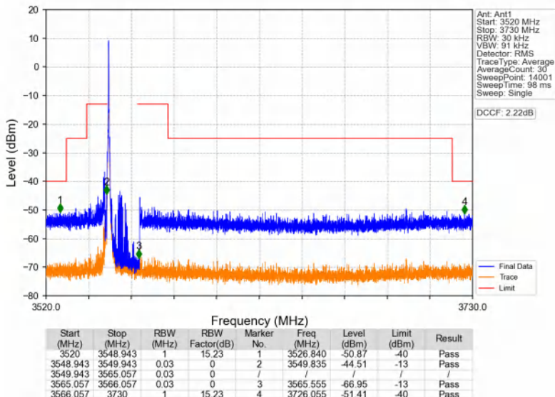
Band48_15MHz_64QAM_LCH_3557.5MHz_RB_1_0_NTNV
