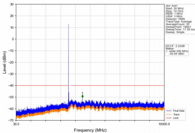
Band48_20MHz_64QAM_LCH_3560MHz_RB_1_0_NTNV
