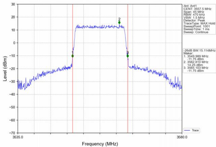
Band48_15MHz_256QAM_LCH_3557.5MHz_RB_75_0_NTNV
