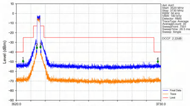
Band48_5MHz_16QAM_LCH_3552.5MHz_RB_25_0_NTNV
