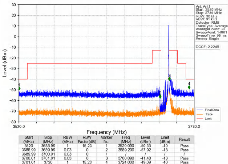
Band48_10MHz_16QAM_HCH_3695MHz_RB_50_0_NTNV
