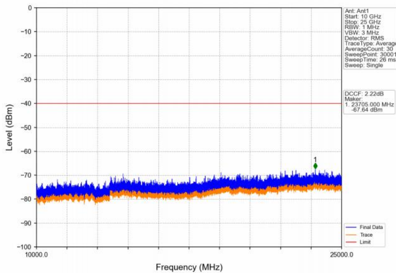
Band48_5MHz_256QAM_MCH_3625MHz_RB_1_0_NTNV
