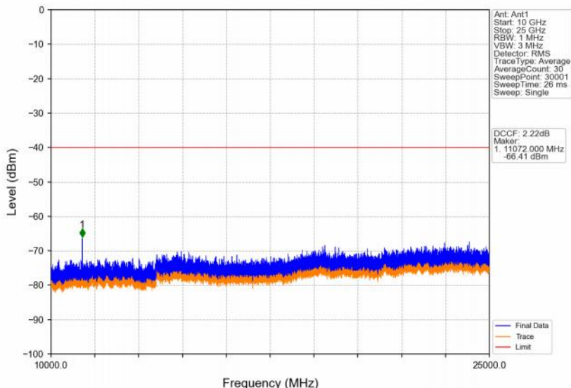
Band48_10MHz_16QAM_HCH_3695MHz_RB_1_0_NTNV
