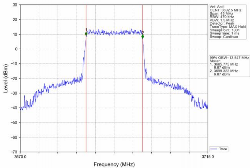
Band48_15MHz_256QAM_HCH_3692.5MHz_RB_75_0_NTNV
