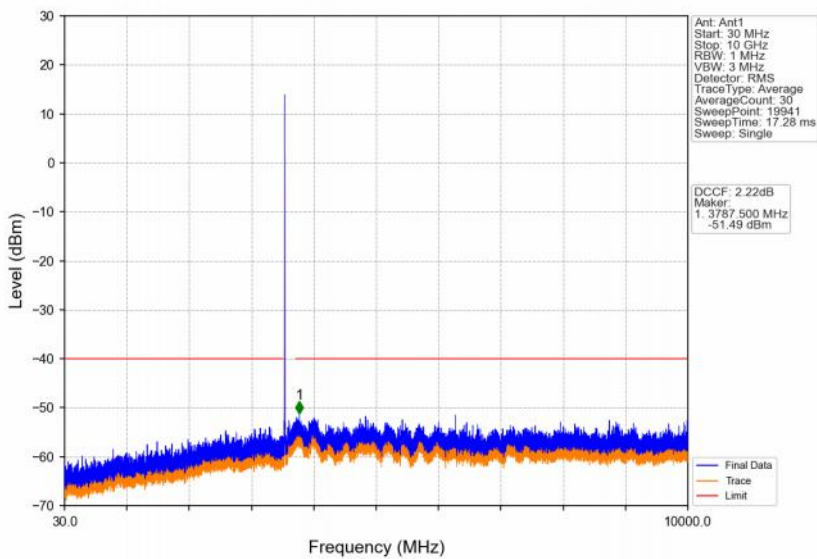
Band48_5MHz_64QAM_LCH_3552.5MHz_RB_1_0_NTNV
