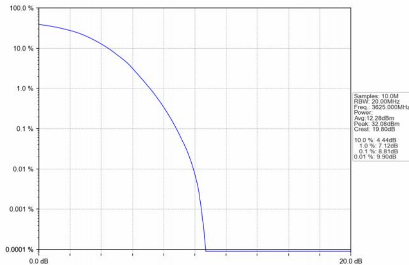
Band48_20MHz_64QAM_MCH_3625MHz_RB_100_0_NTNV
