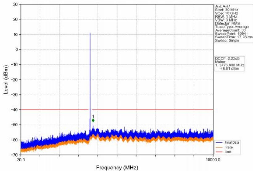
Band48_5MHz_256QAM_MCH_3625MHz_RB_1_0_NTNV
