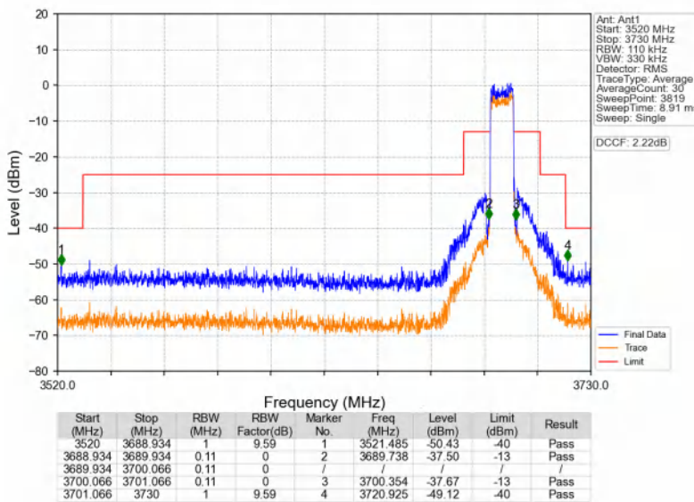
Band48_10MHz_16QAM_HCH_3695MHz_RB_50_0_NTNV
