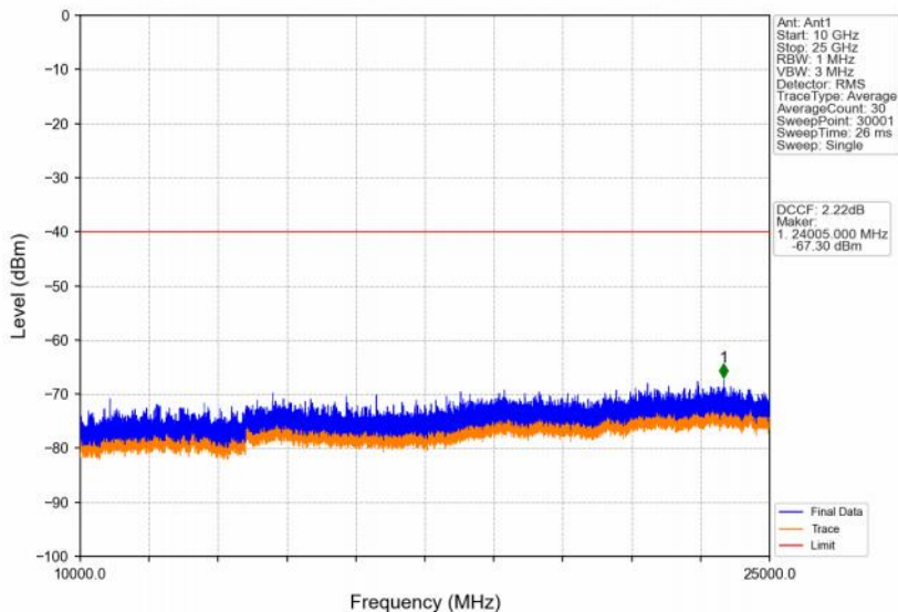
Band48_10MHz_64QAM_LCH_3555MHz_RB_1_0_NTNV
