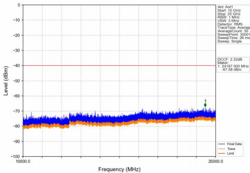
Band48_5MHz_16QAM_LCH_3552.5MHz_RB_1_0_NTNV
