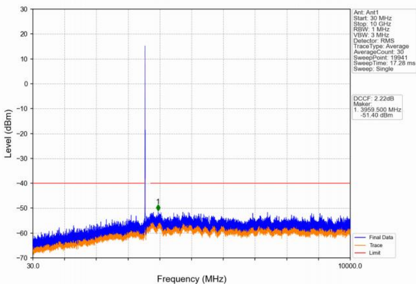
Band48_10MHz_64QAM_LCH_3555MHz_RB_1_0_NTNV
