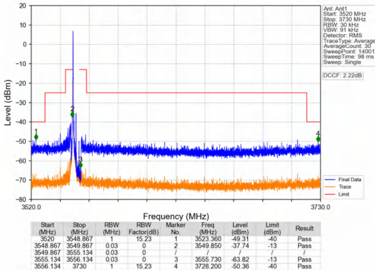
Band48_5MHz_64QAM_LCH_3552.5MHz_RB_1_0_NTNV
