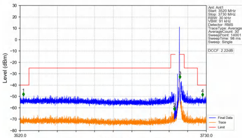
Band48_5MHz_64QAM_HCH_3697.5MHz_RB_1_24_NTNV
