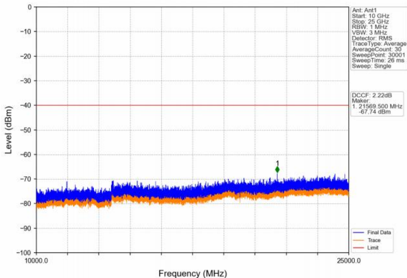
Band48_5MHz_QPSK_LCH_3552.5MHz_RB_1_0_NTNV
