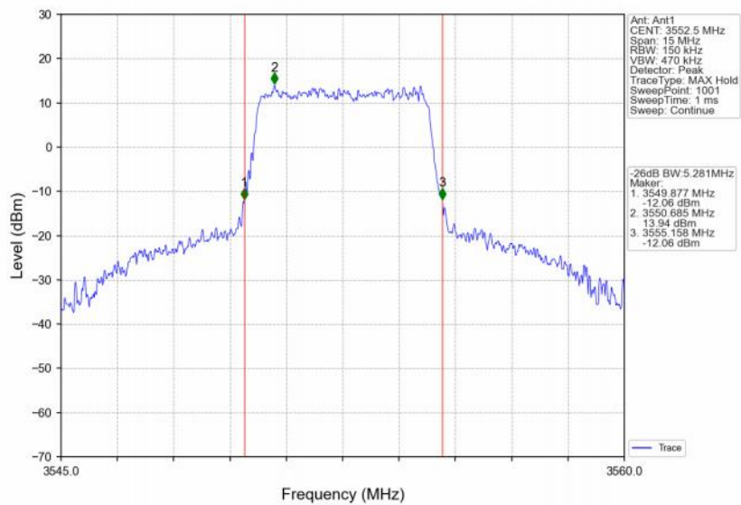
Band48_5MHz_256QAM_LCH_3552.5MHz_RB_25_0_NTNV
