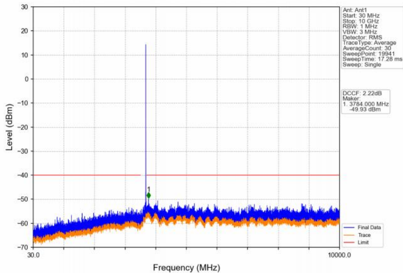
Band48_5MHz_64QAM_HCH_3697.5MHz_RB_1_0_NTNV
