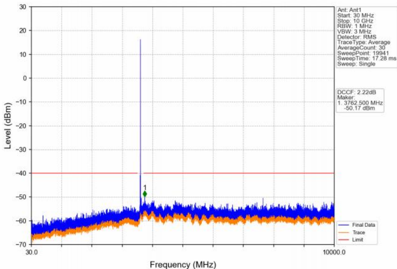
Band48_10MHz_16QAM_MCH_3625MHz_RB_1_0_NTNV
