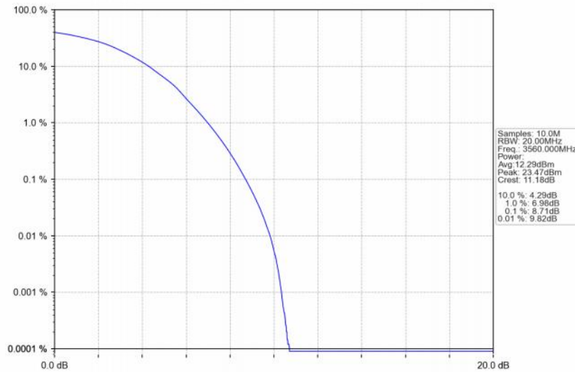
Band48_20MHz_64QAM_LCH_3560MHz_RB_100_0_NTNV
