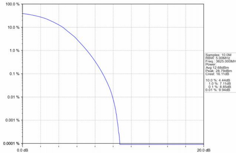
Band48_5MHz_16QAM_MCH_3625MHz_RB_25_0_NTNV
