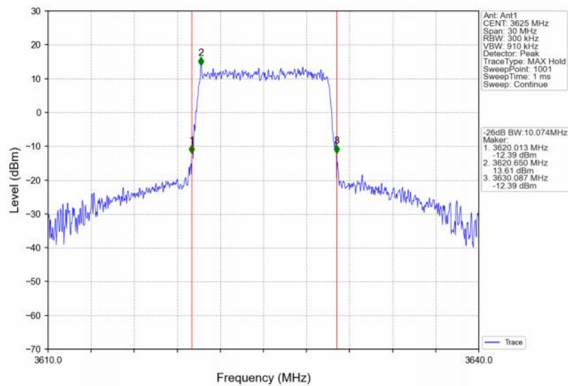
Band48_10MHz_64QAM_MCH_3625MHz_RB_50_0_NTNV
