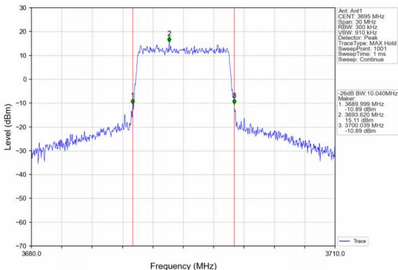
Band48_10MHz_16QAM_HCH_3695MHz_RB_50_0_NTNV
