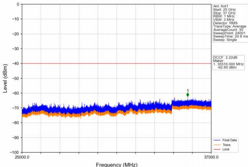
Band48_5MHz_64QAM_HCH_3697.5MHz_RB_1_24_NTNV
