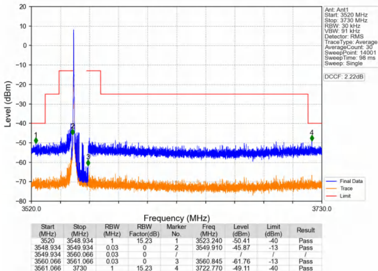
Band48_10MHz_64QAM_LCH_3555MHz_RB_1_0_NTNV
