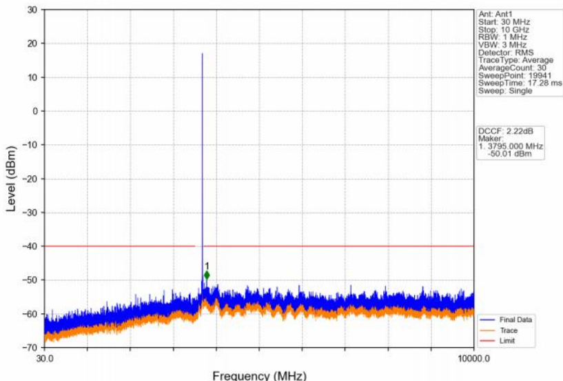
Band48_5MHz_QPSK_HCH_3697.5MHz_RB_1_0_NTNV
