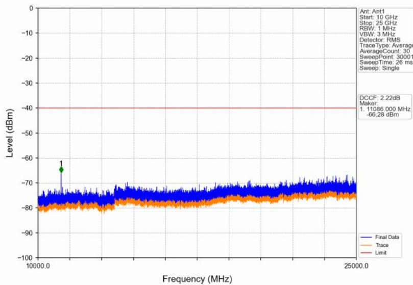
Band48_5MHz_64QAM_HCH_3697.5MHz_RB_1_0_NTNV
