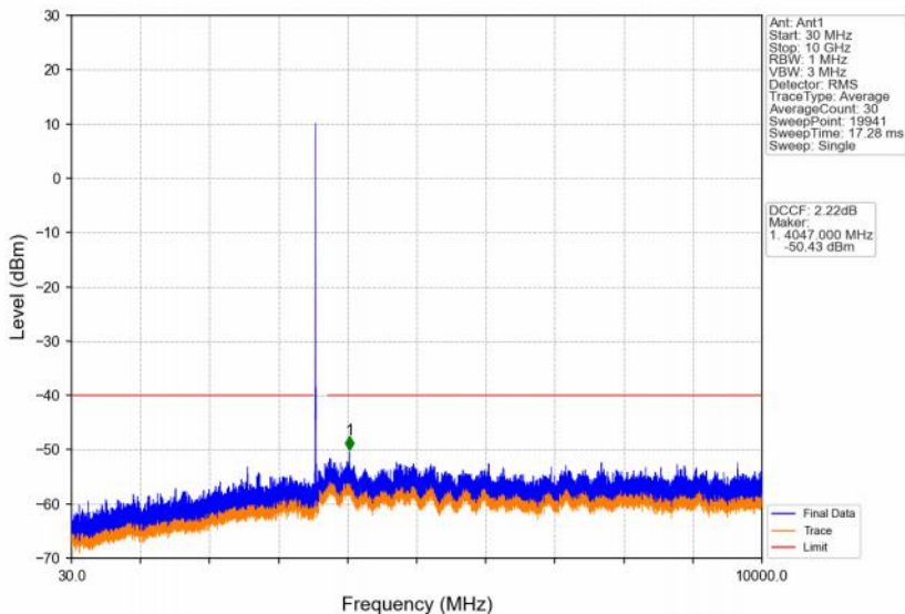
Band48_5MHz_256QAM_LCH_3552.5MHz_RB_1_0_NTNV
