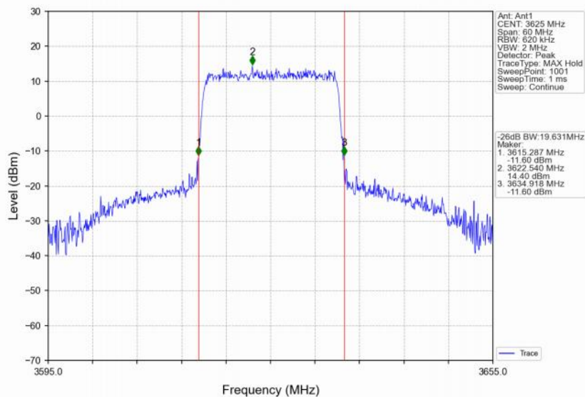
Band48_20MHz_64QAM_MCH_3625MHz_RB_100_0_NTNV
