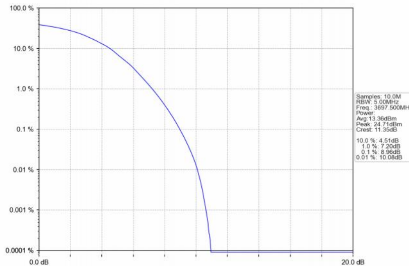
Band48_5MHz_16QAM_HCH_3697.5MHz_RB_25_0_NTNV
