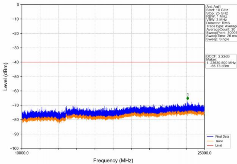
Band48_5MHz_16QAM_MCH_3625MHz_RB_1_0_NTNV
