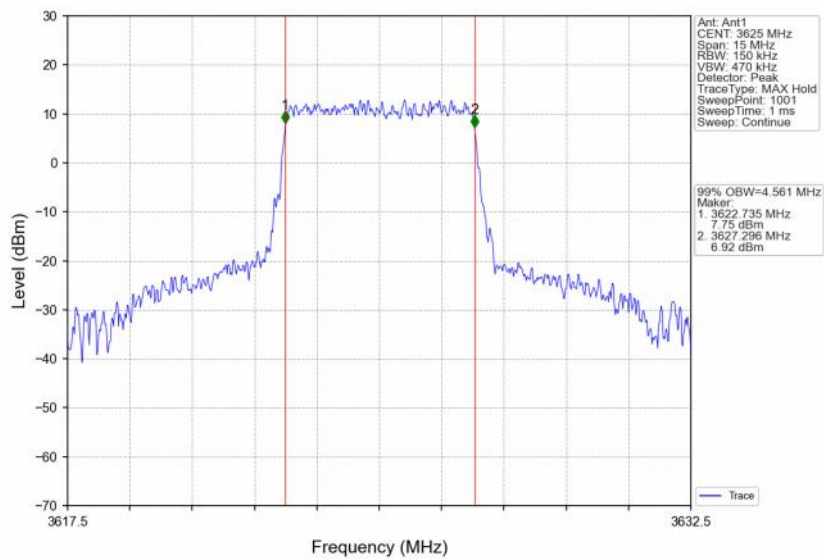
Band48_5MHz_64QAM_MCH_3625MHz_RB_25_0_NTNV
