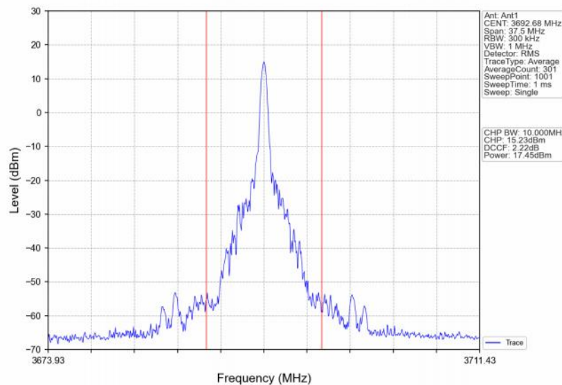
Band48_15MHz_64QAM_HCH_3692.5MHz_RB_1_38_NTNV
