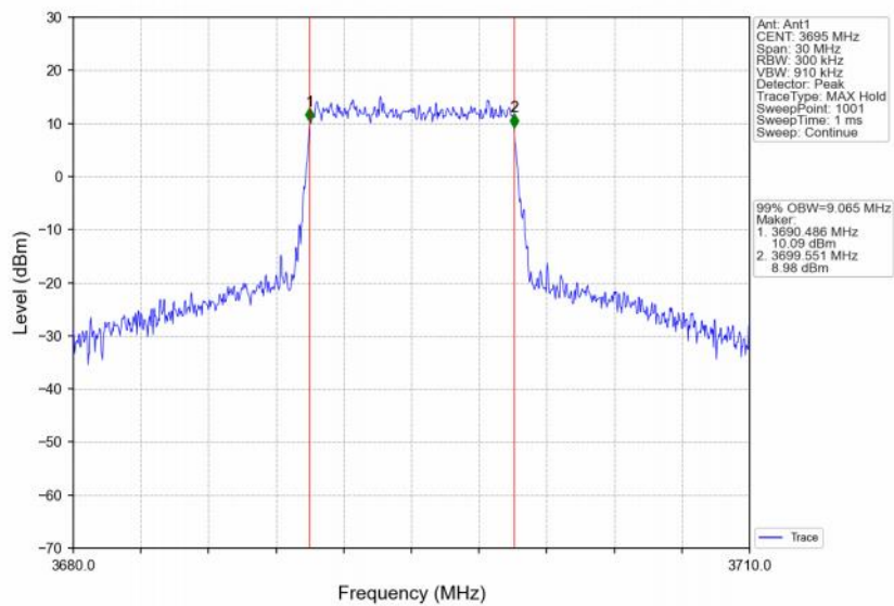
Band48_10MHz_16QAM_HCH_3695MHz_RB_50_0_NTNV
