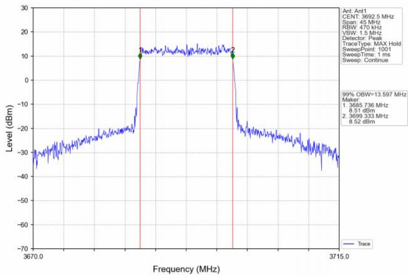
Band48_15MHz_16QAM_HCH_3692.5MHz_RB_75_0_NTNV
