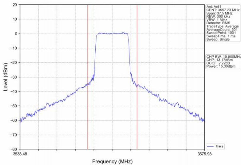
Band48_15MHz_16QAM_LCH_3557.5MHz_RB_36_18_NTNV
