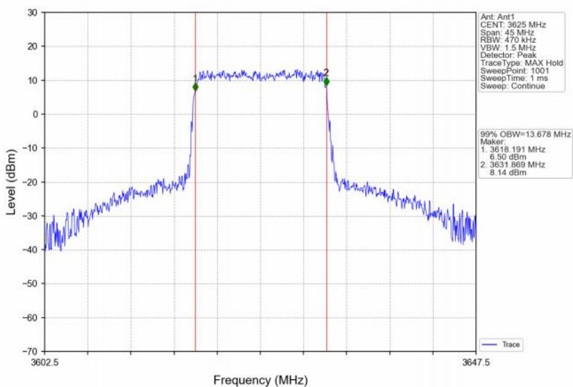
Band48_15MHz_64QAM_MCH_3625MHz_RB_75_0_NTNV
