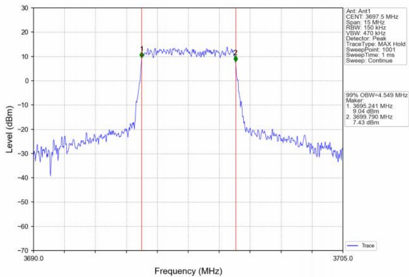
Band48_5MHz_16QAM_HCH_3697.5MHz_RB_25_0_NTNV
