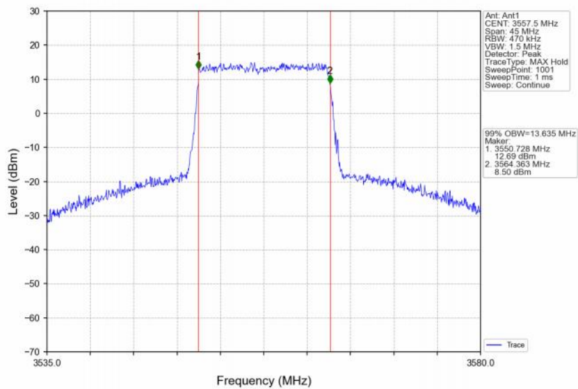
Band48_15MHz_16QAM_LCH_3557.5MHz_RB_75_0_NTNV
