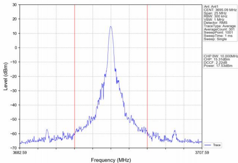
Band48_10MHz_64QAM_HCH_3695MHz_RB_1_25_NTNV
