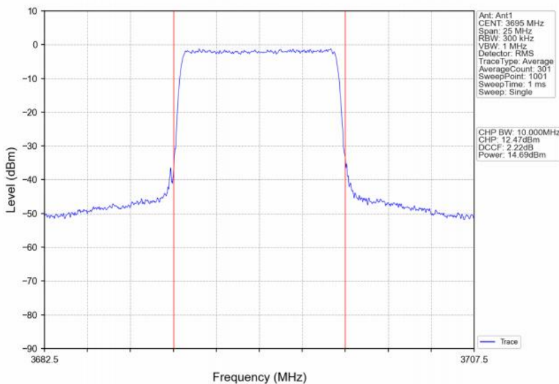
Band48_10MHz_256QAM_HCH_3695MHz_RB_50_0_NTNV
