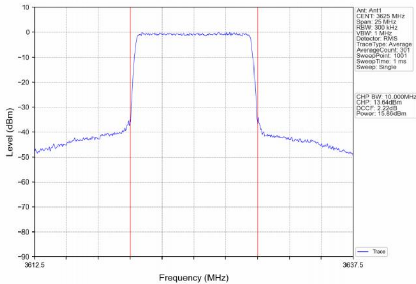
Band48_10MHz_64QAM_MCH_3625MHz_RB_50_0_NTNV
