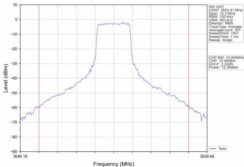
Band48_5MHz_256QAM_LCH_3552.5MHz_RB_12_6_NTNV
