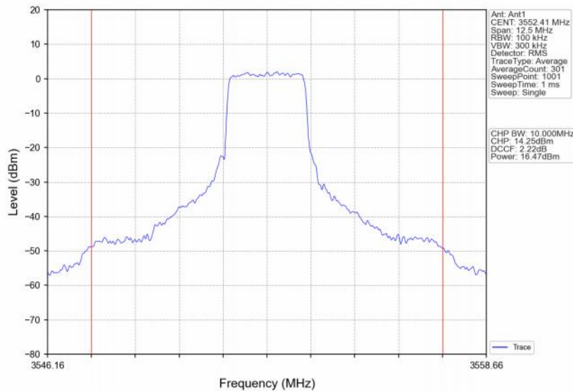
Band48_5MHz_QPSK_LCH_3552.5MHz_RB_12_13_NTNV
