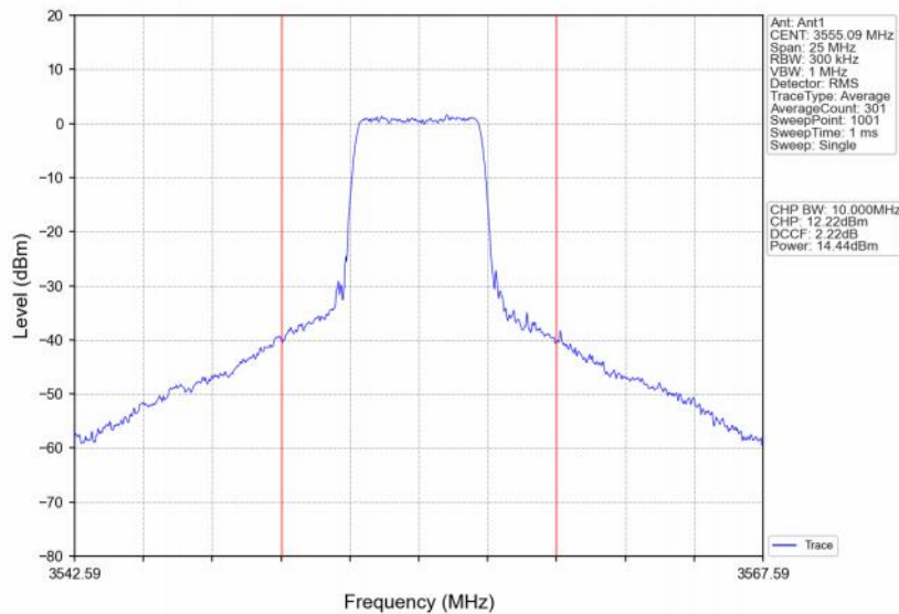
Band48_10MHz_64QAM_LCH_3555MHz_RB_25_25_NTNV
