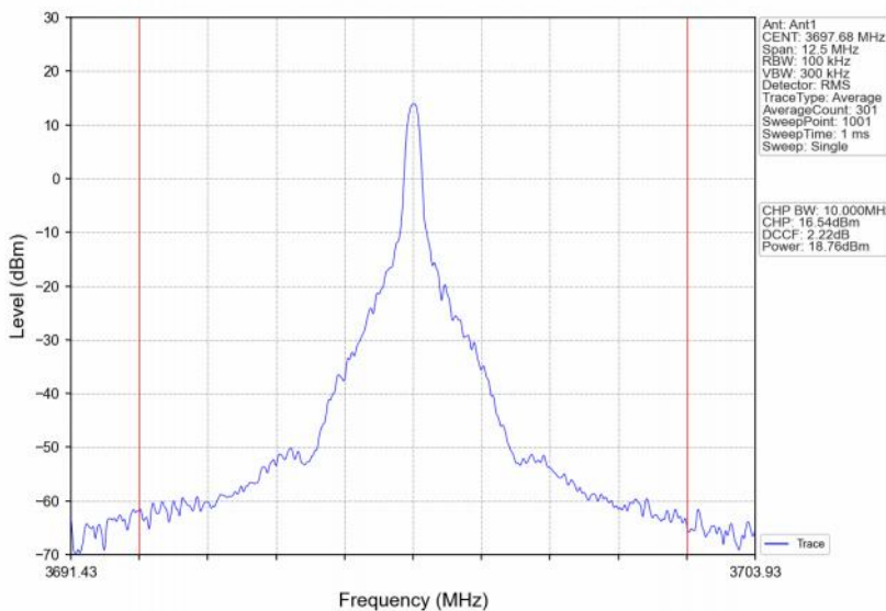
Band48_5MHz_QPSK_HCH_3697.5MHz_RB_1_13_NTNV
