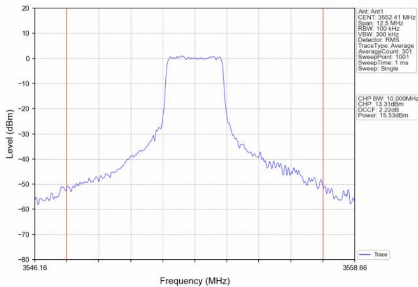
Band48_5MHz_16QAM_LCH_3552.5MHz_RB_12_6_NTNV
