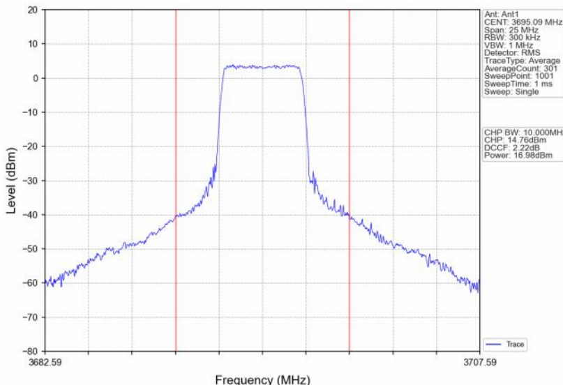
Band48_10MHz_64QAM_HCH_3695MHz_RB_25_25_NTNV
