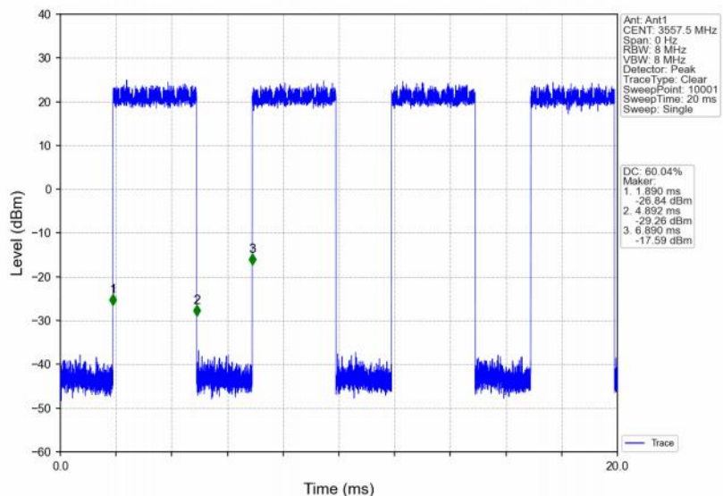
Band48_15MHz_256QAM_LCH_3557.5MHz_RB_75_0_NTNV
