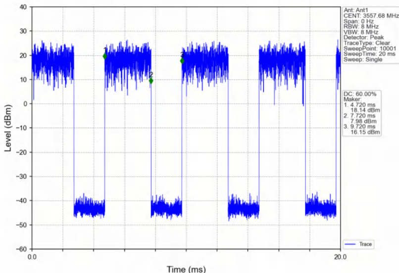
Band48_15MHz_256QAM_LCH_3557.5MHz_RB_1_74_NTNV
