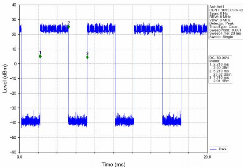
Band48_10MHz_256QAM_HCH_3695MHz_RB_25_13_NTNV
