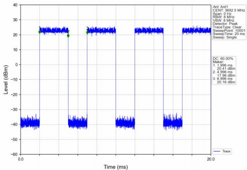
Band48_15MHz_16QAM_HCH_3692.5MHz_RB_75_0_NTNV
