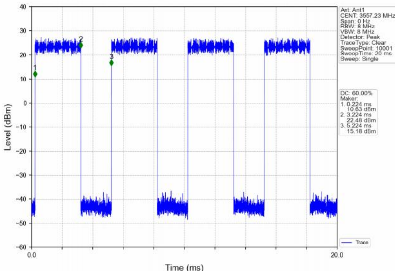
Band48_15MHz_64QAM_LCH_3557.5MHz_RB_36_39_NTNV
