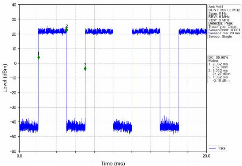
Band48_15MHz_16QAM_LCH_3557.5MHz_RB_75_0_NTNV
