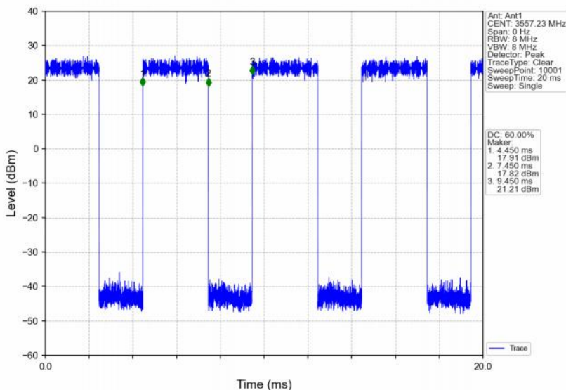
Band48_15MHz_16QAM_LCH_3557.5MHz_RB_36_18_NTNV
