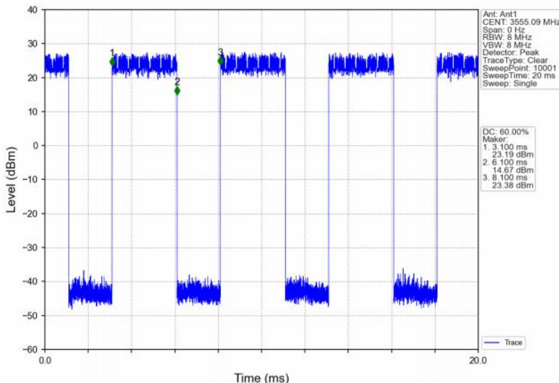
Band48_10MHz_64QAM_LCH_3555MHz_RB_25_25_NTNV
