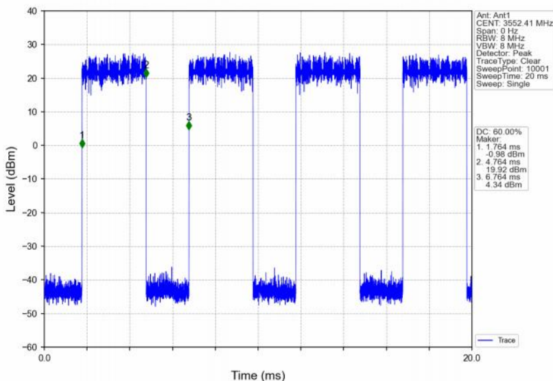
Band48_5MHz_256QAM_LCH_3552.5MHz_RB_12_6_NTNV
