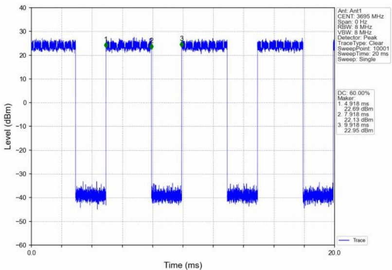
Band48_10MHz_16QAM_HCH_3695MHz_RB_50_0_NTNV
