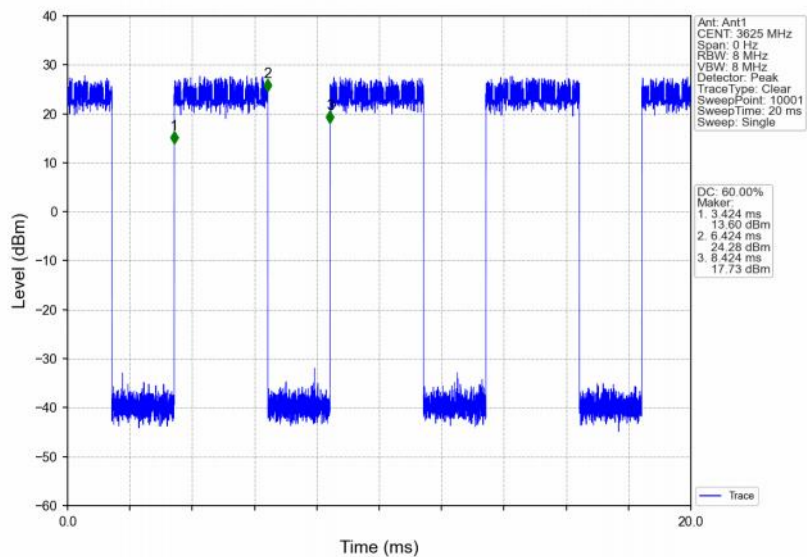
Band48_5MHz_64QAM_MCH_3625MHz_RB_25_0_NTNV
