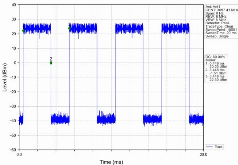
Band48_5MHz_16QAM_HCH_3697.5MHz_RB_12_6_NTNV
