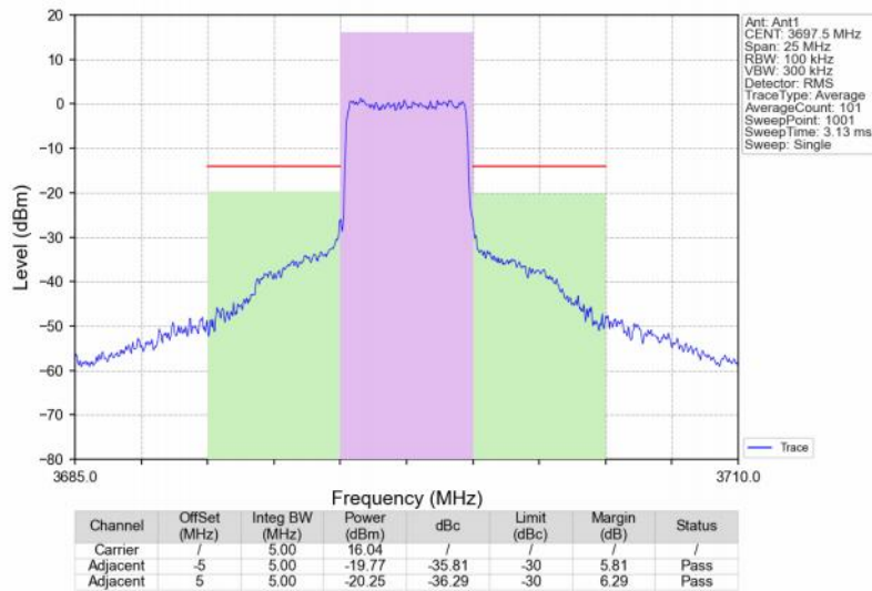
Band48_5MHz_16QAM_HCH_3697.5MHz_RB_25_0_NTNV
