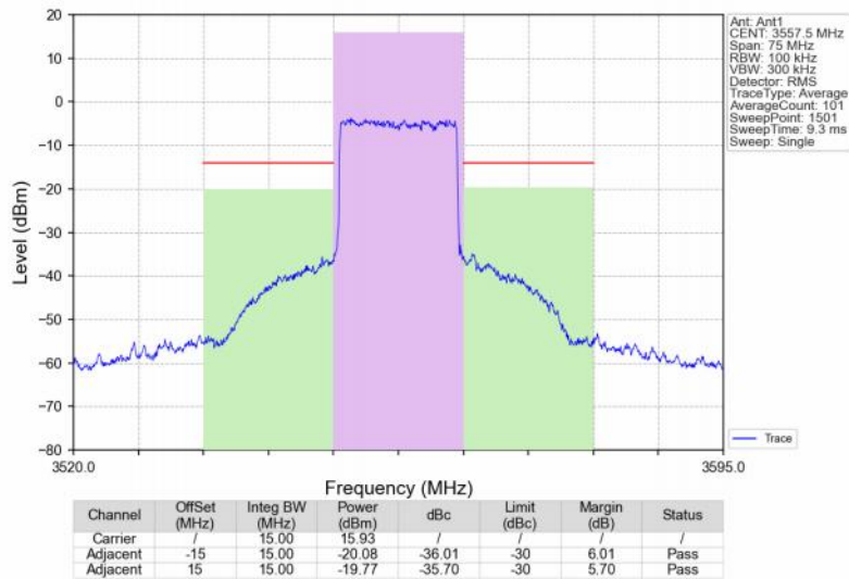
Band48_15MHz_256QAM_LCH_3557.5MHz_RB_75_0_NTNV
