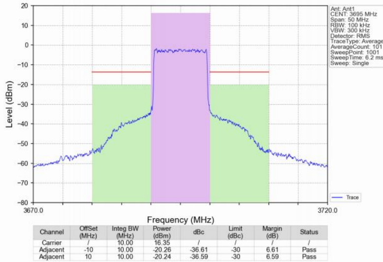
Band48_10MHz_64QAM_HCH_3695MHz_RB_50_0_NTNV
