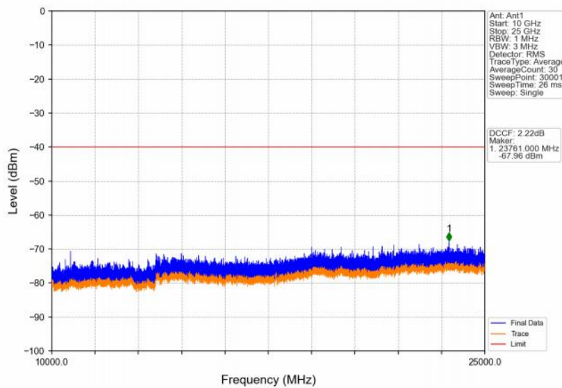
Band48_15MHz_256QAM_LCH_3557.5MHz_RB_1_0_NTNV
