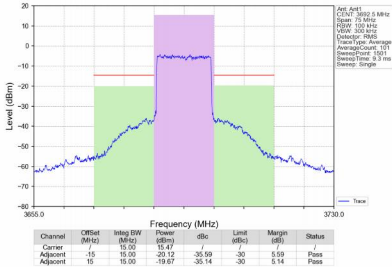
Band48_15MHz_64QAM_HCH_3692.5MHz_RB_75_0_NTNV
