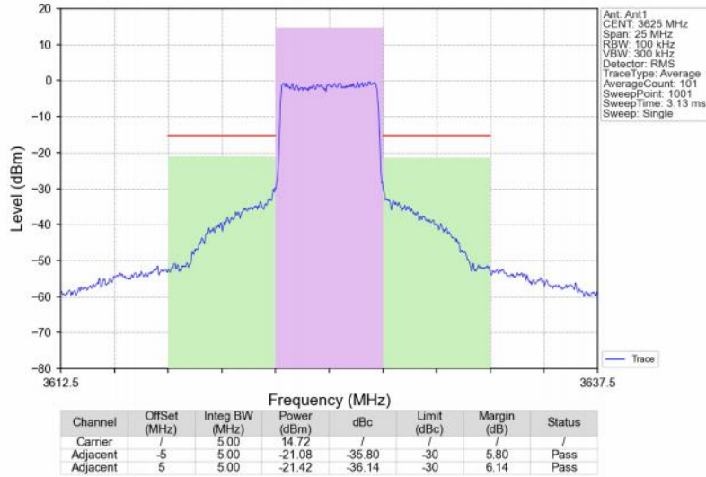
Band48_5MHz_256QAM_MCH_3625MHz_RB_25_0_NTNV
