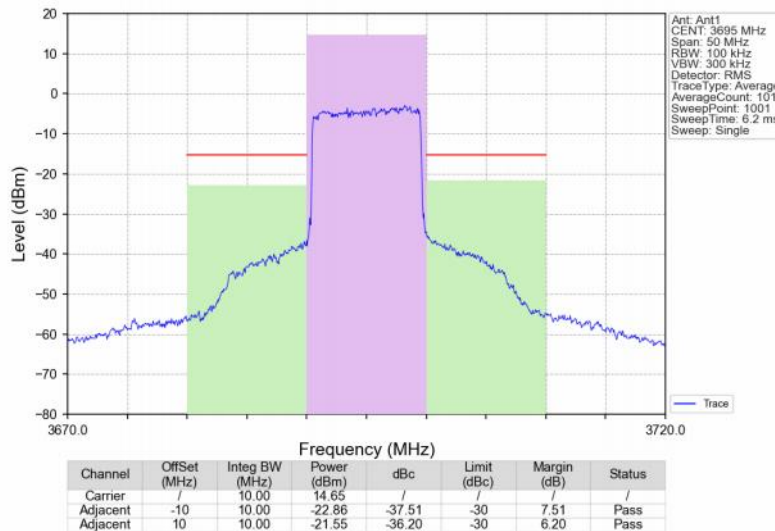
Band48_10MHz_256QAM_HCH_3695MHz_RB_50_0_NTNV
