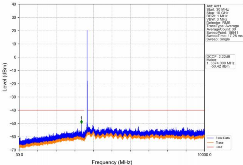
Band48_20MHz_64QAM_HCH_3690MHz_RB_1_0_NTNV
