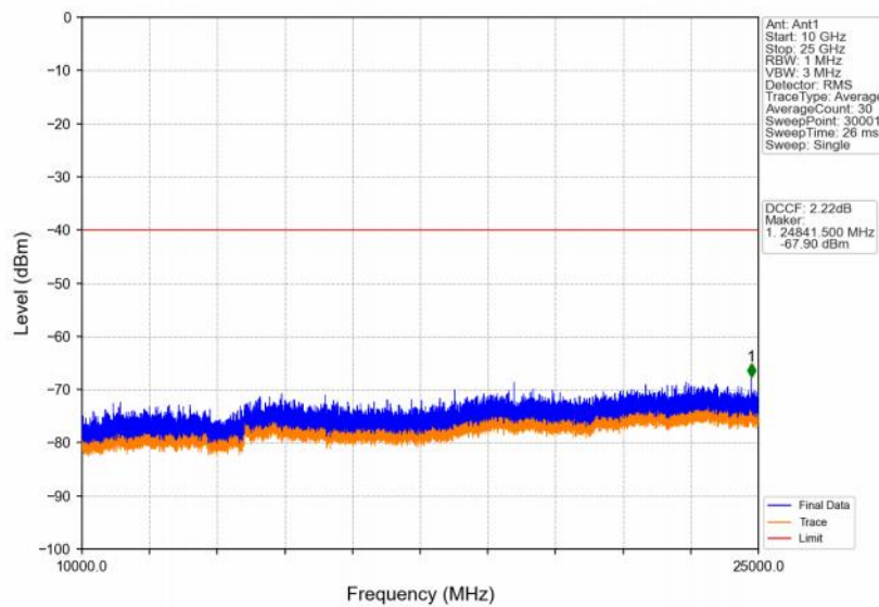
Band48_15MHz_256QAM_MCH_3625MHz_RB_1_0_NTNV
