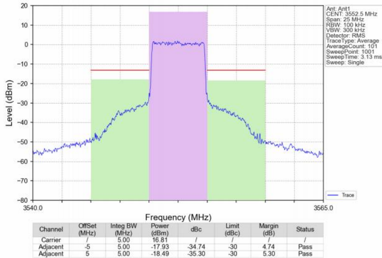
Band48_5MHz_64QAM_LCH_3552.5MHz_RB_25_0_NTNV
