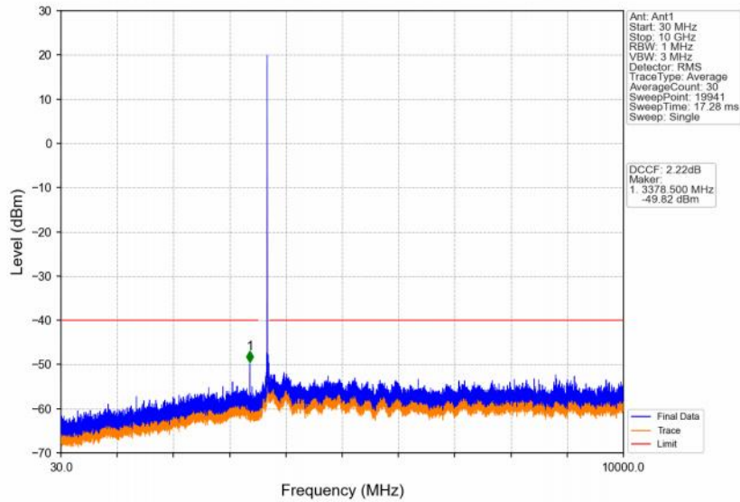
Band48_15MHz_64QAM_HCH_3692.5MHz_RB_1_0_NTNV
