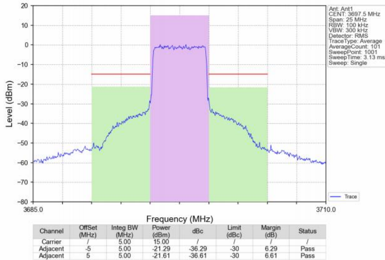
Band48_5MHz_256QAM_HCH_3697.5MHz_RB_25_0_NTNV
