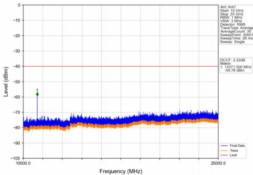
Band48_10MHz_64QAM_HCH_3695MHz_RB_1_0_NTV
