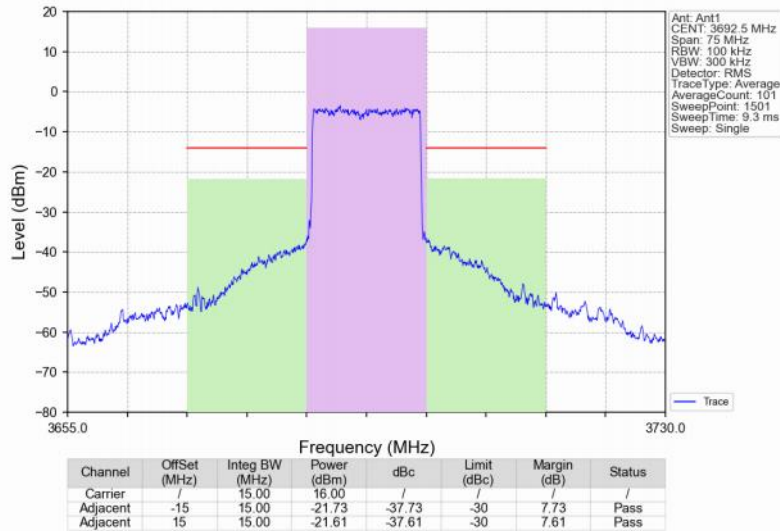
Band48_15MHz_QPSK_HCH_3692.5MHz_RB_75_0_NTNV
