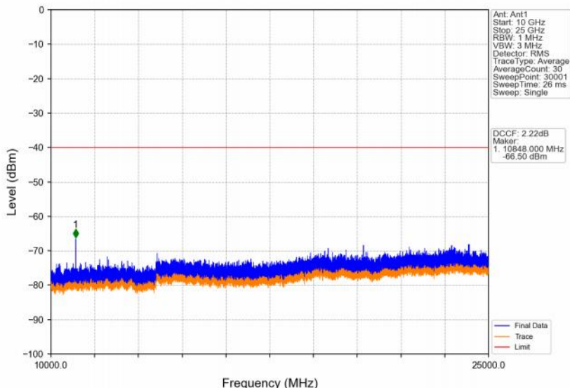
Band48_20MHz_64QAM_MCH_3625MHz_RB_1_0_NTNV
