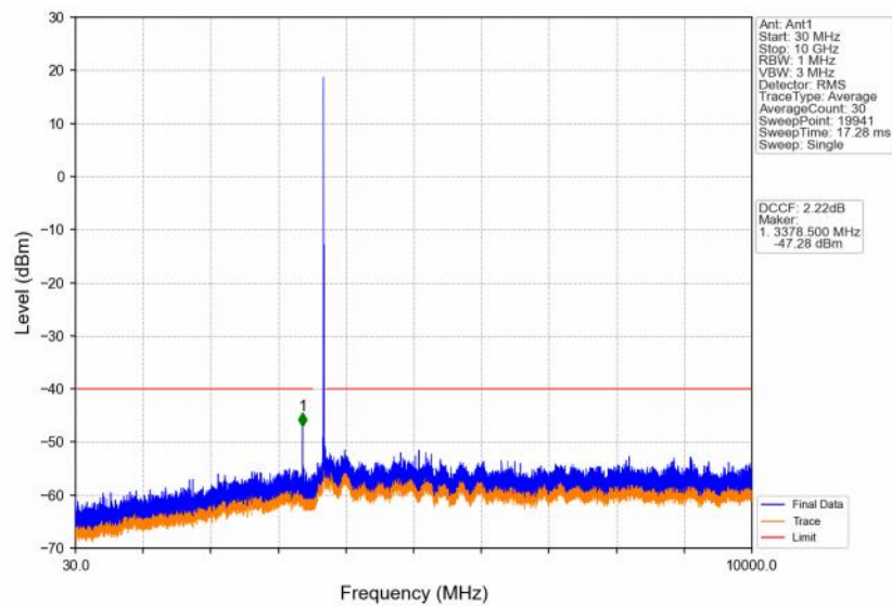
Band48_15MHz_16QAM_HCH_3692.5MHz_RB_1_0_NTNV
