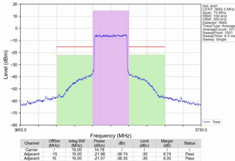
Band48_15MHz_256QAM_HCH_3692.5MHz_RB_75_0_NTNV
