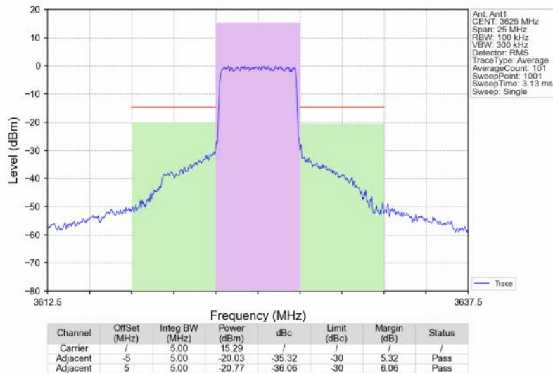
Band48_5MHz_64QAM_MCH_3625MHz_RB_25_0_NTNV
