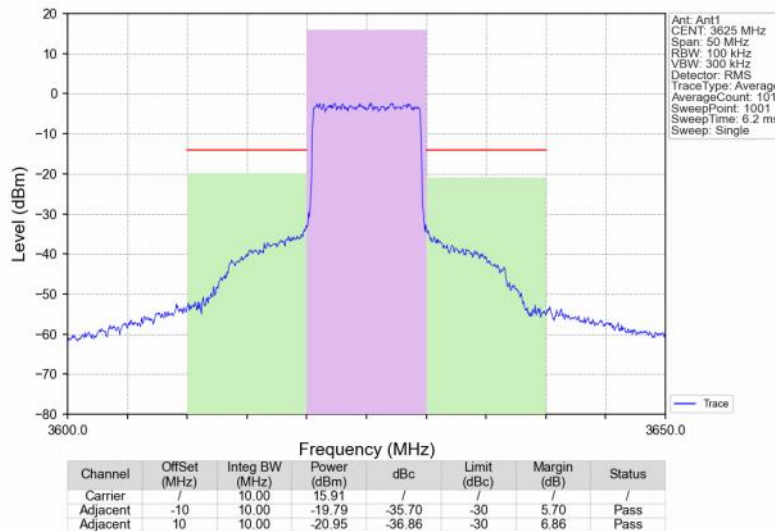
Band48_10MHz_64QAM_MCH_3625MHz_RB_50_0_NTNV
