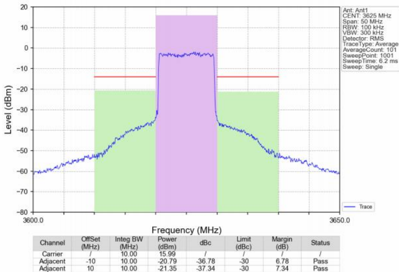
Band48_10MHz_16QAM_MCH_3625MHz_RB_50_0_NTNV
