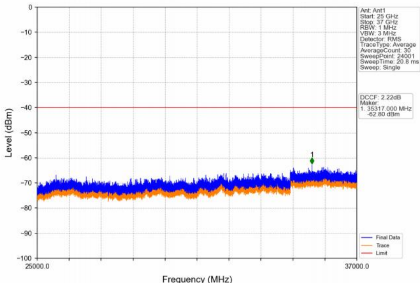
Band48_10MHz_256QAM_HCH_3695MHz_RB_1_0_NTNV
