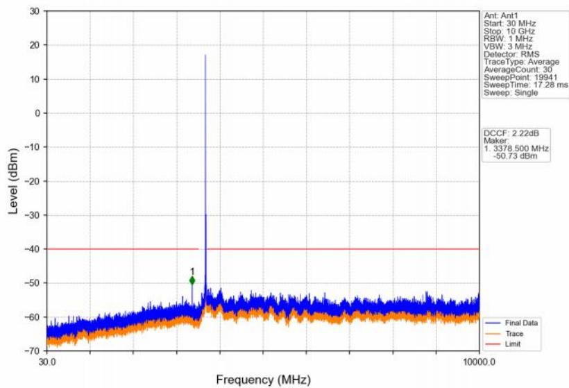
Band48_15MHz_256QAM_HCH_3692.5MHz_RB_1_0_NTNV
