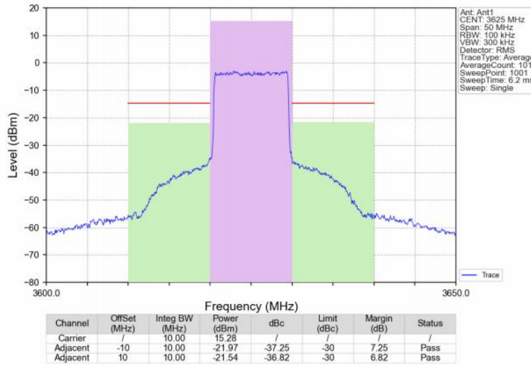
Band48_10MHz_256QAM_MCH_3625MHz_RB_50_0_NTNV
