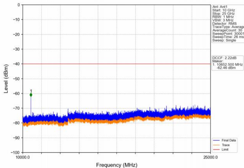
Band48_15MHz_16QAM_LCH_3557.5MHz_RB_1_0_NTNV
