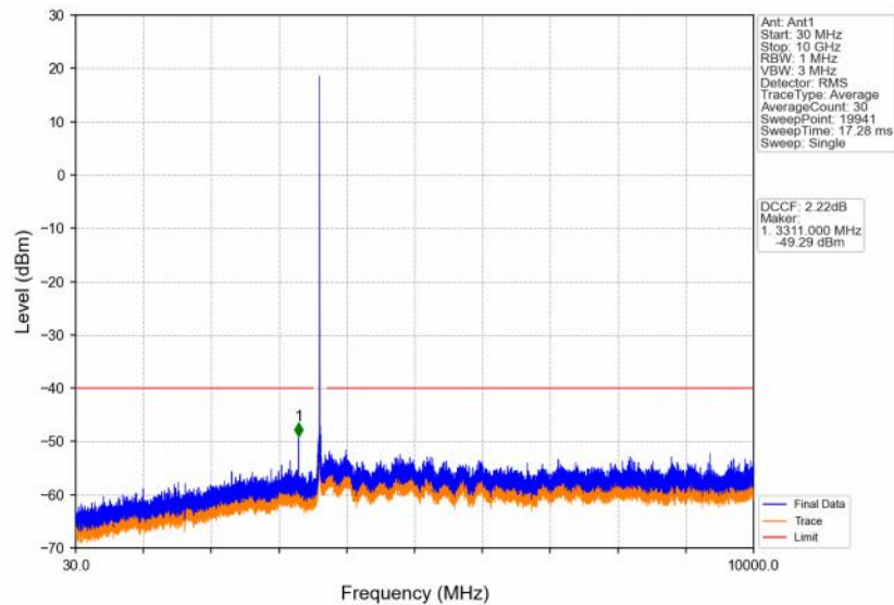
Band48_15MHz_16QAM_MCH_3625MHz_RB_1_0_NTNV
