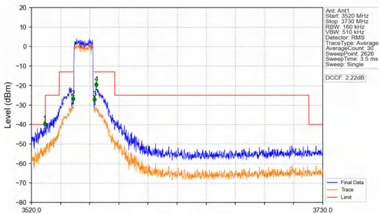
Band48_15MHz_16QAM_LCH_3557.5MHz_RB_75_0_NTNV
