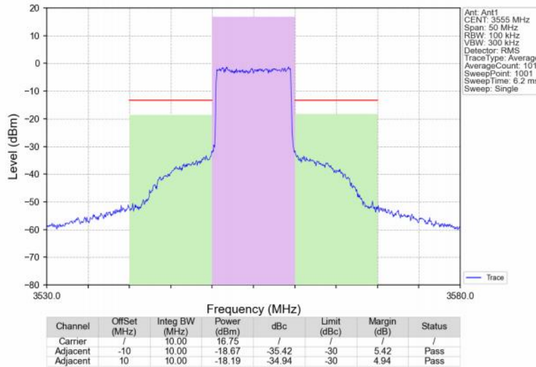
Band48_10MHz_64QAM_LCH_3555MHz_RB_50_0_NTNV
