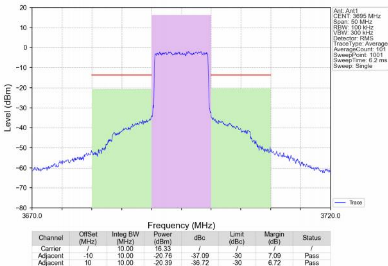
Band48_10MHz_16QAM_HCH_3695MHz_RB_50_0_NTNV
