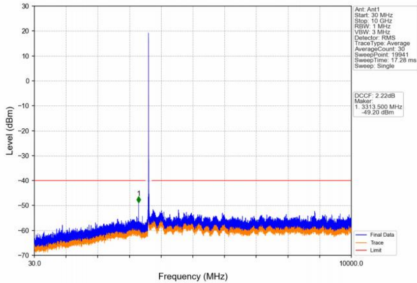
Band48_10MHz_256QAM_MCH_3625MHz_RB_1_0_NTNV
