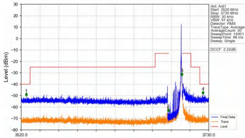
Band48_15MHz_64QAM_HCH_3692.5MHz_RB_1_74_NTNV
