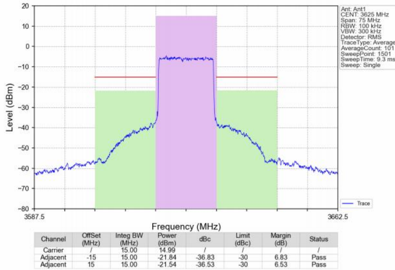
Band48_15MHz_256QAM_MCH_3625MHz_RB_75_0_NTNV
