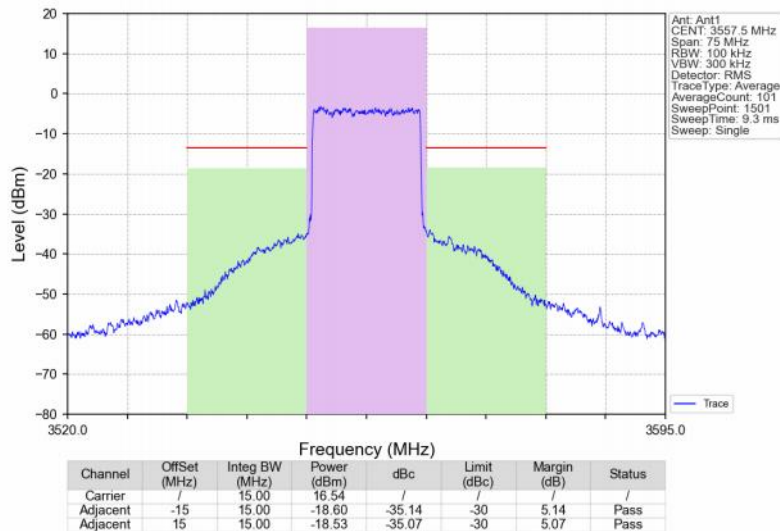
Band48_15MHz_16QAM_LCH_3557.5MHz_RB_75_0_NTNV
