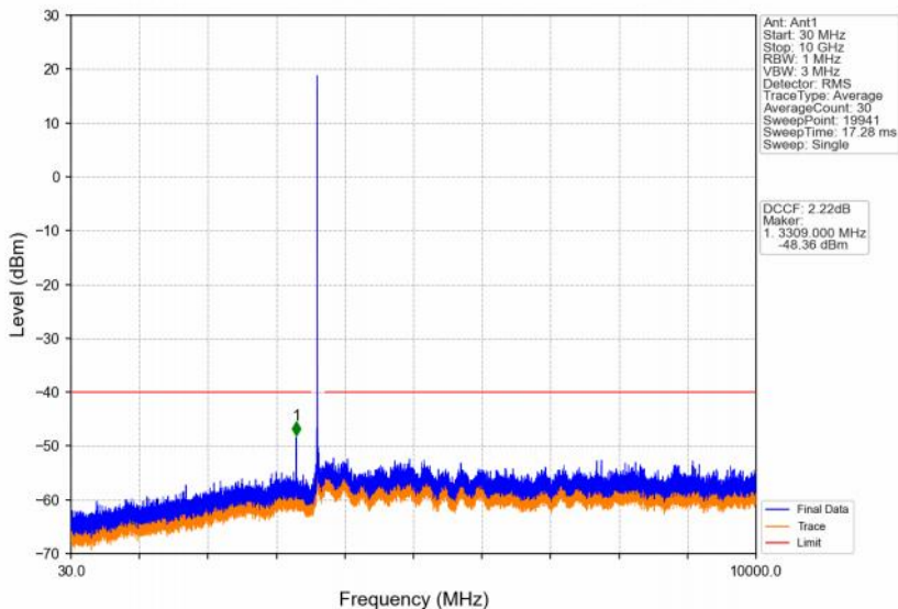
Band48_20MHz_16QAM_MCH_3625MHz_RB_1_0_NTNV
