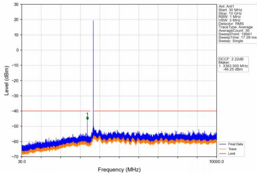
Band48_10MHz_64QAM_HCH_3695MHz_RB_1_0_NTV
