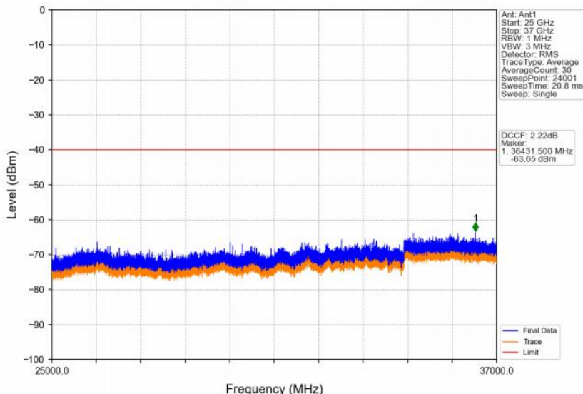
Band48_15MHz_16QAM_LCH_3557.5MHz_RB_75_0_NTNV
