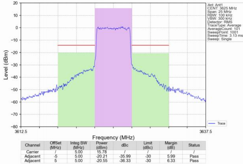
Band48_5MHz_16QAM_MCH_3625MHz_RB_25_0_NTNV
