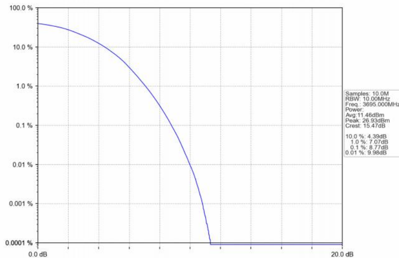
Band48_10MHz_256QAM_HCH_3695MHz_RB_50_0_NTNV
