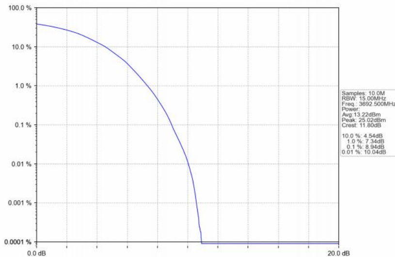
Band48_15MHz_QPSK_HCH_3692.5MHz_RB_75_0_NTNV
