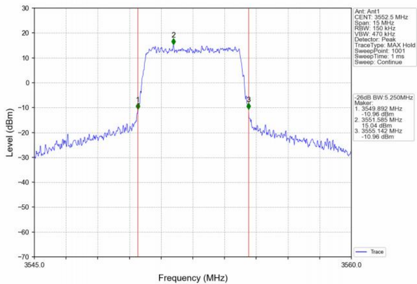
Band48_5MHz_16QAM_LCH_3552.5MHz_RB_25_0_NTNV
