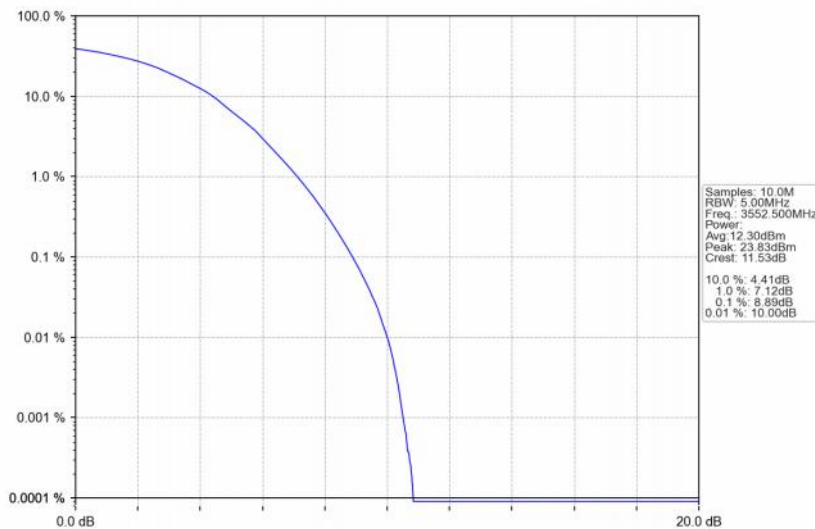
Band48_5MHz_64QAM_LCH_3552.5MHz_RB_25_0_NTNV
