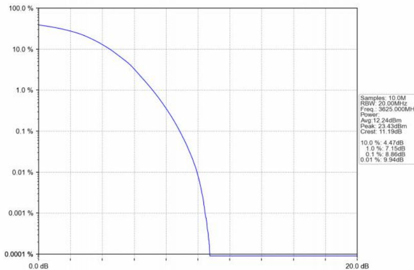
Band48_20MHz_64QAM_MCH_3625MHz_RB_100_0_NTNV
