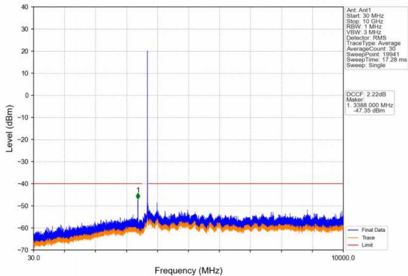
Band48_5MHz_QPSK_HCH_3697.5MHz_RB_1_0_NTNV
