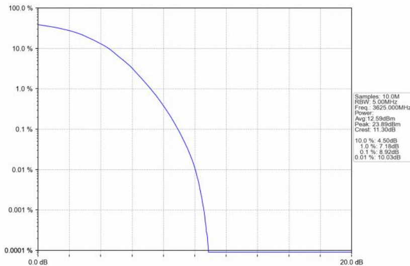
Band48_5MHz_16QAM_MCH_3625MHz_RB_25_0_NTNV
