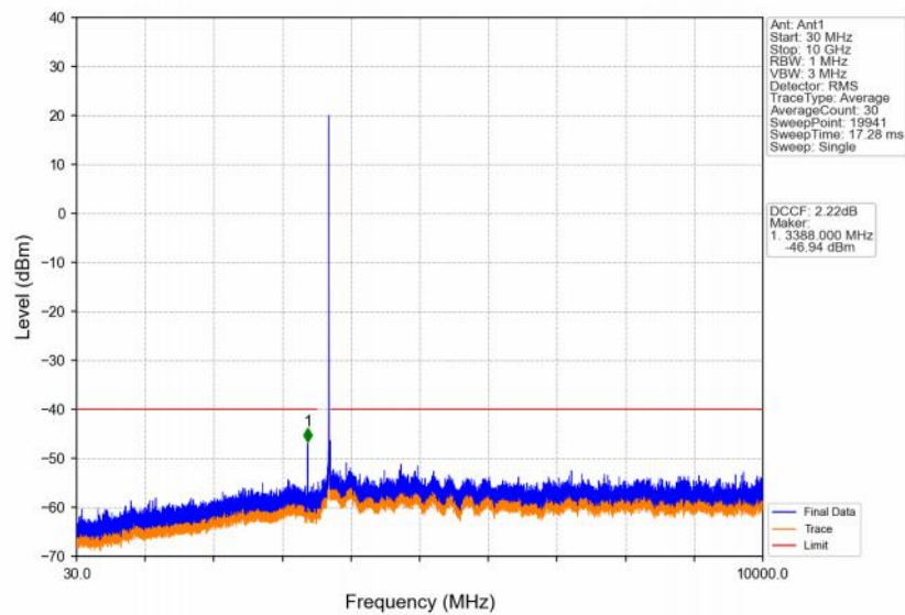
Band48_5MHz_16QAM_HCH_3697.5MHz_RB_1_0_NTNV
