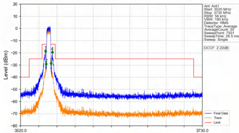
Band48_5MHz_256QAM_LCH_3552.5MHz_RB_25_0_NTNV
