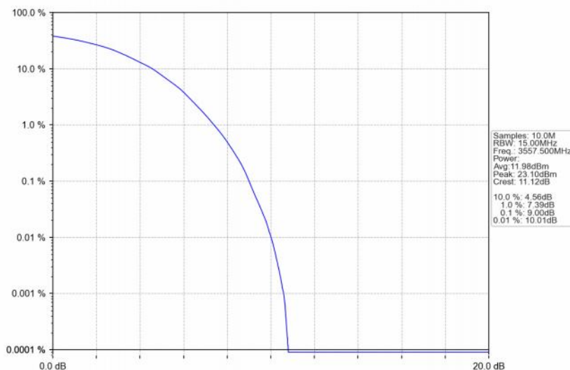
Band48_15MHz_16QAM_LCH_3557.5MHz_RB_75_0_NTNV
