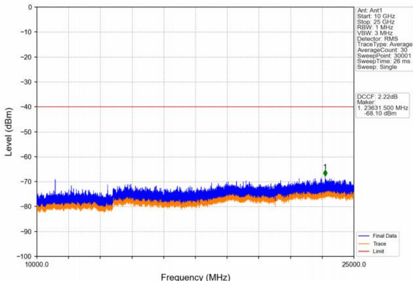
Band48_5MHz_64QAM_MCH_3625MHz_RB_1_0_NTNV
