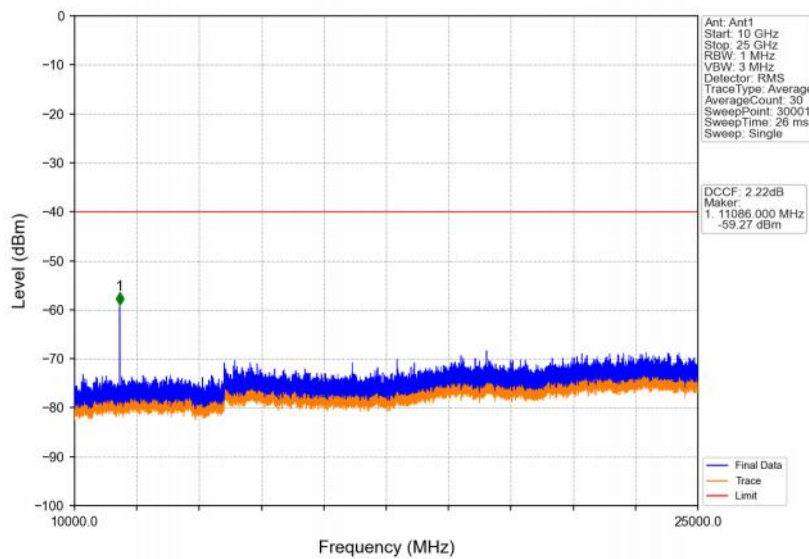
Band48_5MHz_QPSK_HCH_3697.5MHz_RB_1_0_NTNV
