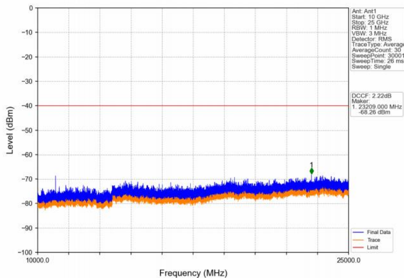
Band48_10MHz_16QAM_MCH_3625MHz_RB_1_0_NTNV
