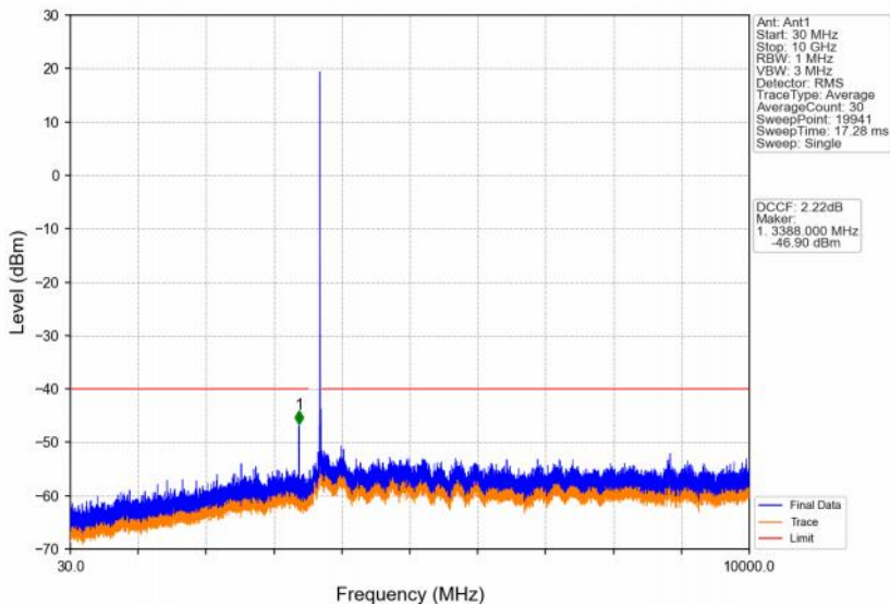
Band48_5MHz_64QAM_HCH_3697.5MHz_RB_1_0_NTNV
