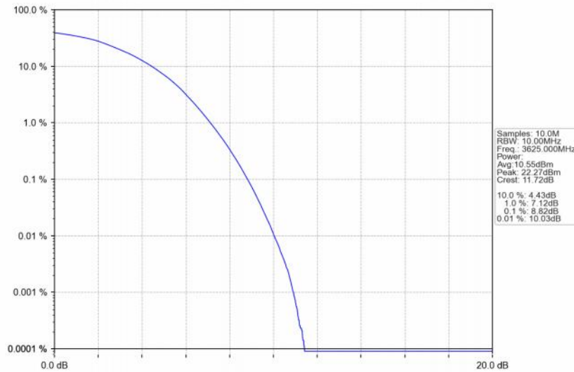
Band48_10MHz_256QAM_MCH_3625MHz_RB_50_0_NTNV
