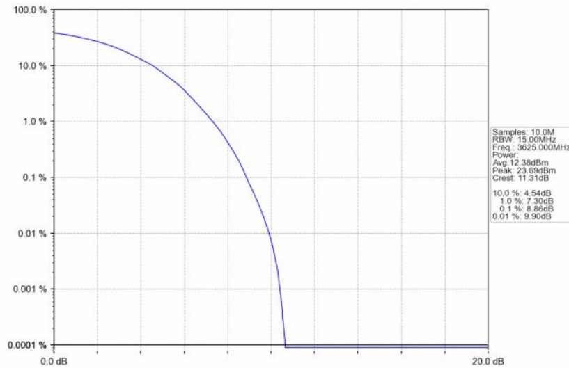
Band48_15MHz_64QAM_MCH_3625MHz_RB_75_0_NTNV
