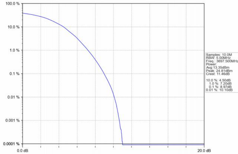
Band48_5MHz_64QAM_HCH_3697.5MHz_RB_25_0_NTNV
