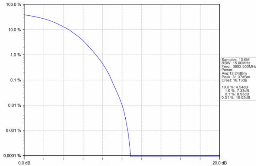
Band48_15MHz_64QAM_HCH_3692.5MHz_RB_75_0_NTNV
