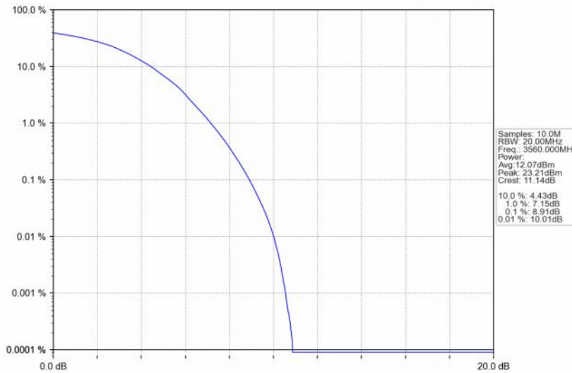
Band48_20MHz_64QAM_LCH_3560MHz_RB_100_0_NTNV
