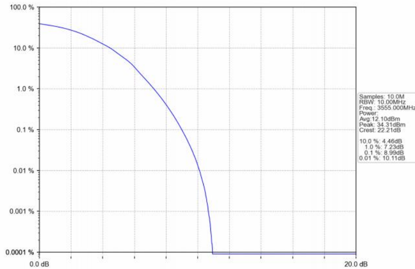
Band48_10MHz_64QAM_LCH_3555MHz_RB_50_0_NTNV
