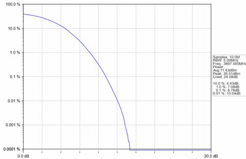
Band48_5MHz_256QAM_HCH_3697.5MHz_RB_25_0_NTNV
