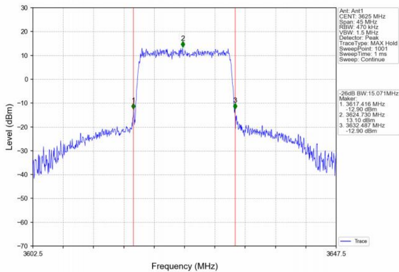
Band48_15MHz_64QAM_MCH_3625MHz_RB_75_0_NTNV
