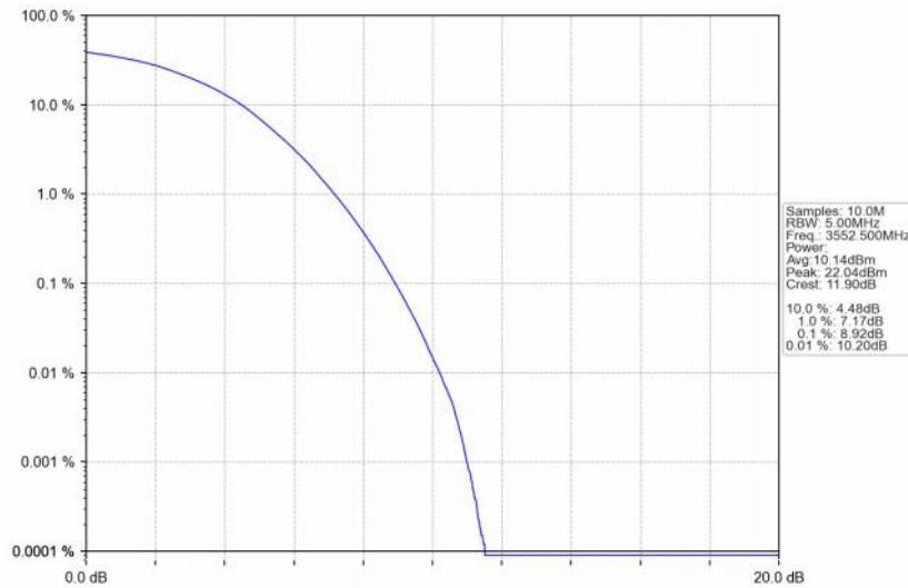
Band48_5MHz_256QAM_LCH_3552.5MHz_RB_25_0_NTNV
