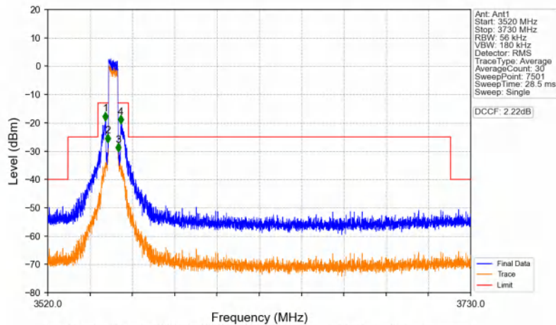
Band48_5MHz_16QAM_LCH_3552.5MHz_RB_25_0_NTNV
