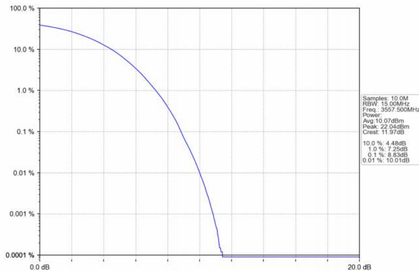
Band48_15MHz_256QAM_LCH_3557.5MHz_RB_75_0_NTNV
