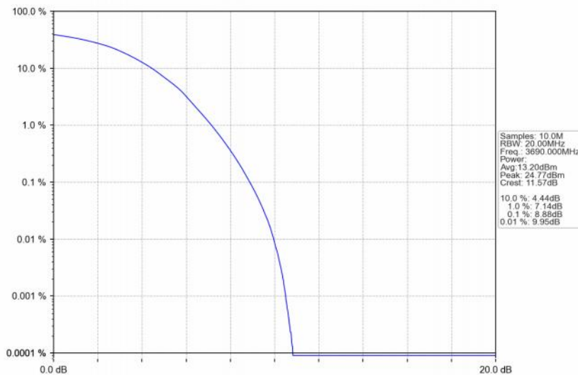
Band48_20MHz_64QAM_HCH_3690MHz_RB_100_0_NTNV
