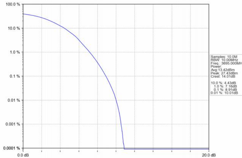
Band48_10MHz_64QAM_HCH_3695MHz_RB_50_0_NTNV
