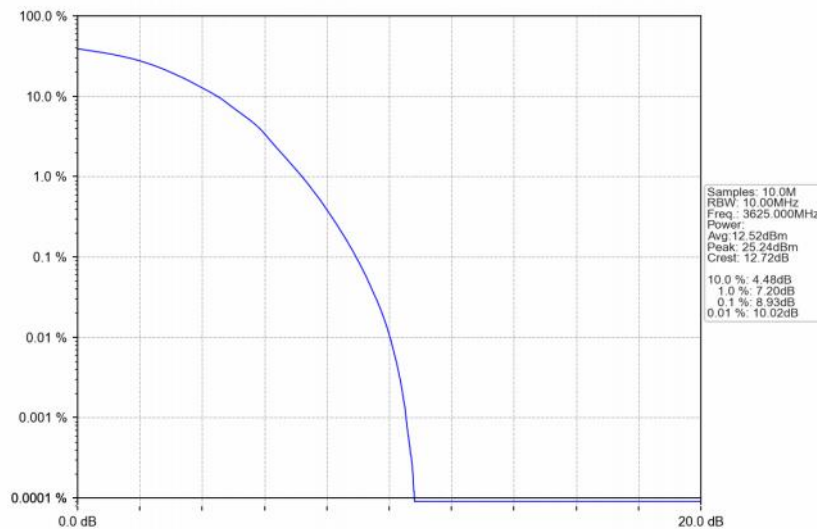
Band48_10MHz_64QAM_MCH_3625MHz_RB_50_0_NTNV
