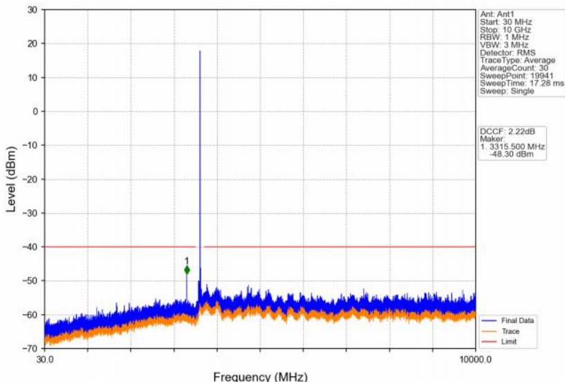
Band48_5MHz_256QAM_MCH_3625MHz_RB_1_0_NTNV
