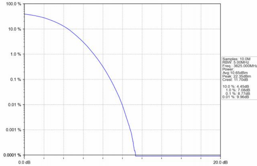
Band48_5MHz_256QAM_MCH_3625MHz_RB_25_0_NTNV
