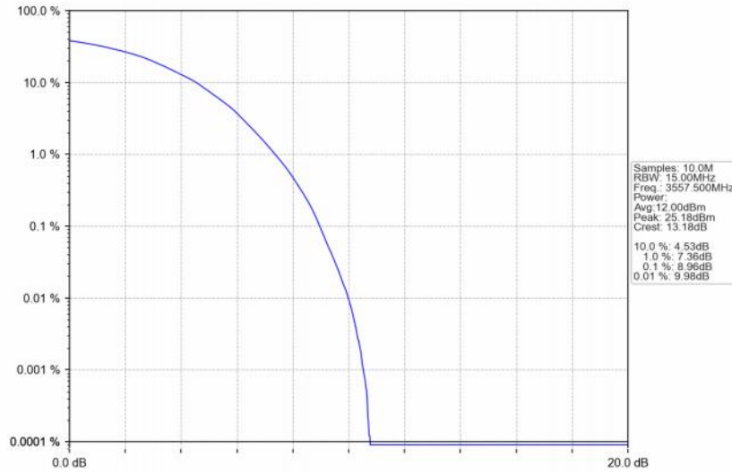
Band48_15MHz_64QAM_LCH_3557.5MHz_RB_75_0_NTNV
