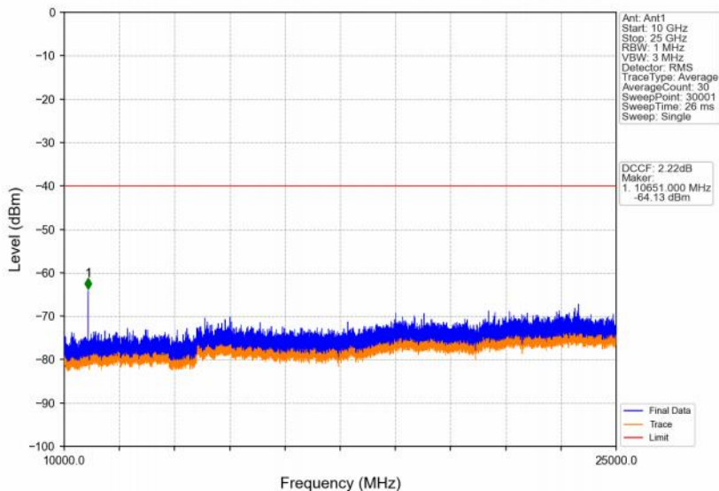
Band48_5MHz_64QAM_LCH_3552.5MHz_RB_1_0_NTNV
