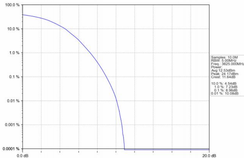
Band48_5MHz_64QAM_MCH_3625MHz_RB_25_0_NTNV
