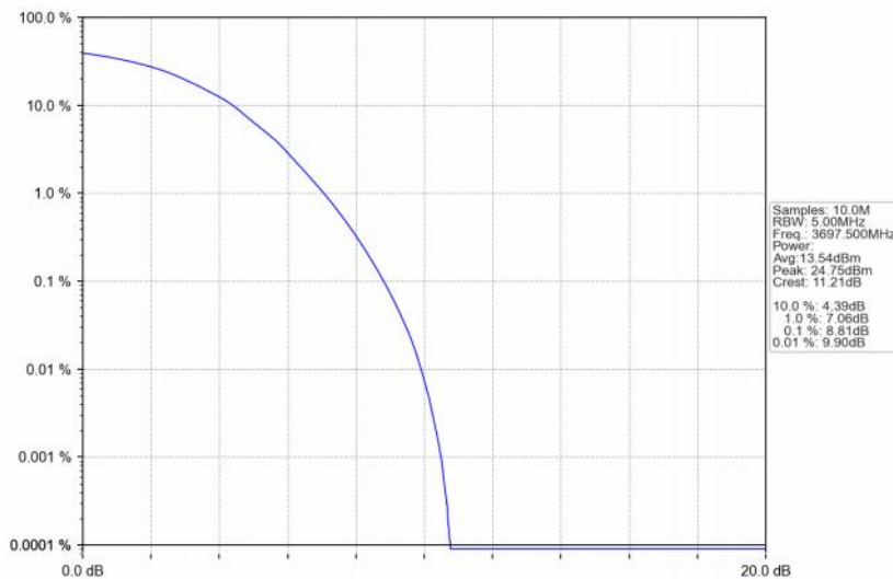
Band48_5MHz_16QAM_HCH_3697.5MHz_RB_25_0_NTNV
