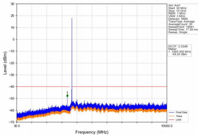
Band48_10MHz_16QAM_HCH_3695MHz_RB_1_0_NTNV
